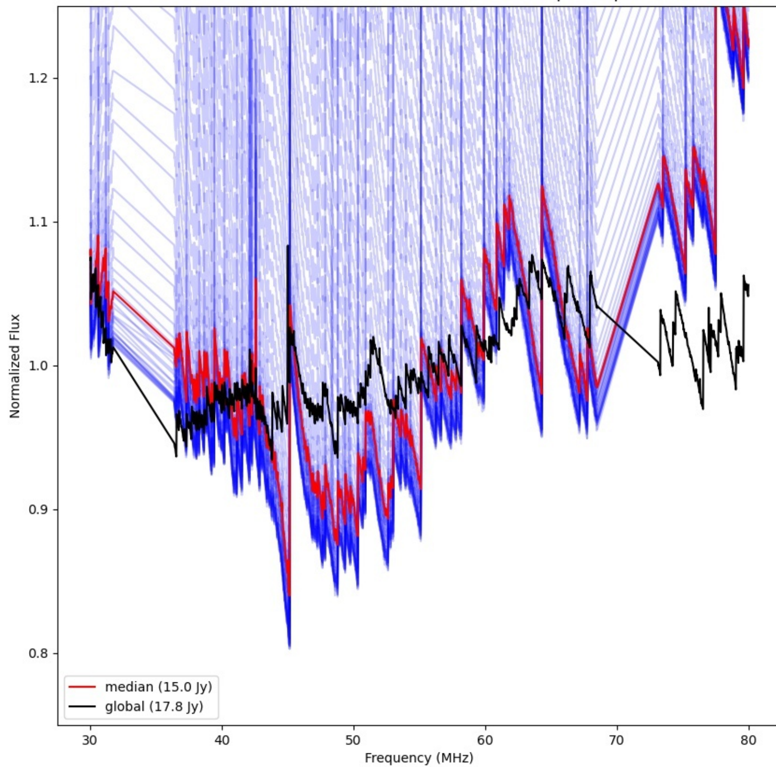
LWA038 - Correlator# 077 - XX - FLAGS:BadSpecShape
