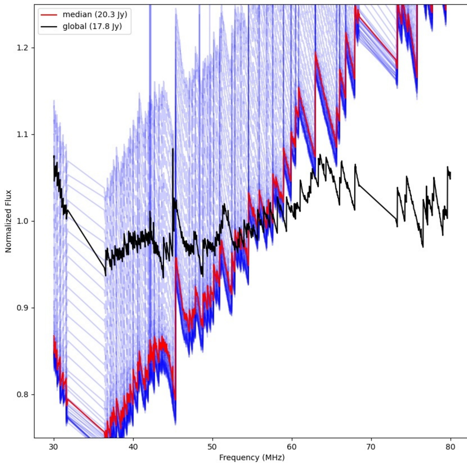
LWA129 - Correlator# 180 - XX - FLAGS:Good
