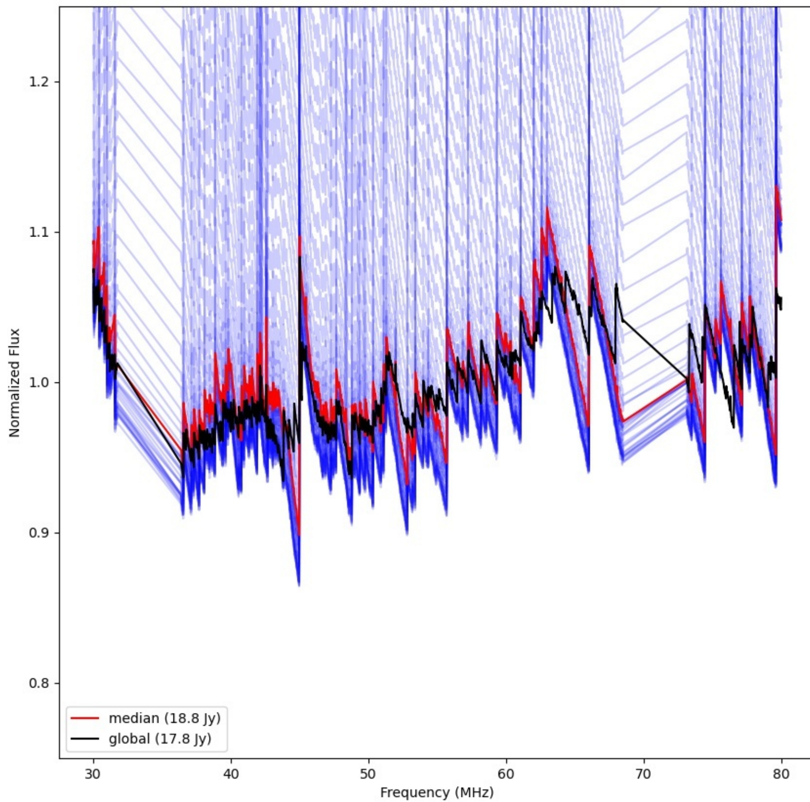
LWA072 - Correlator# 171 - XX - FLAGS:Good
