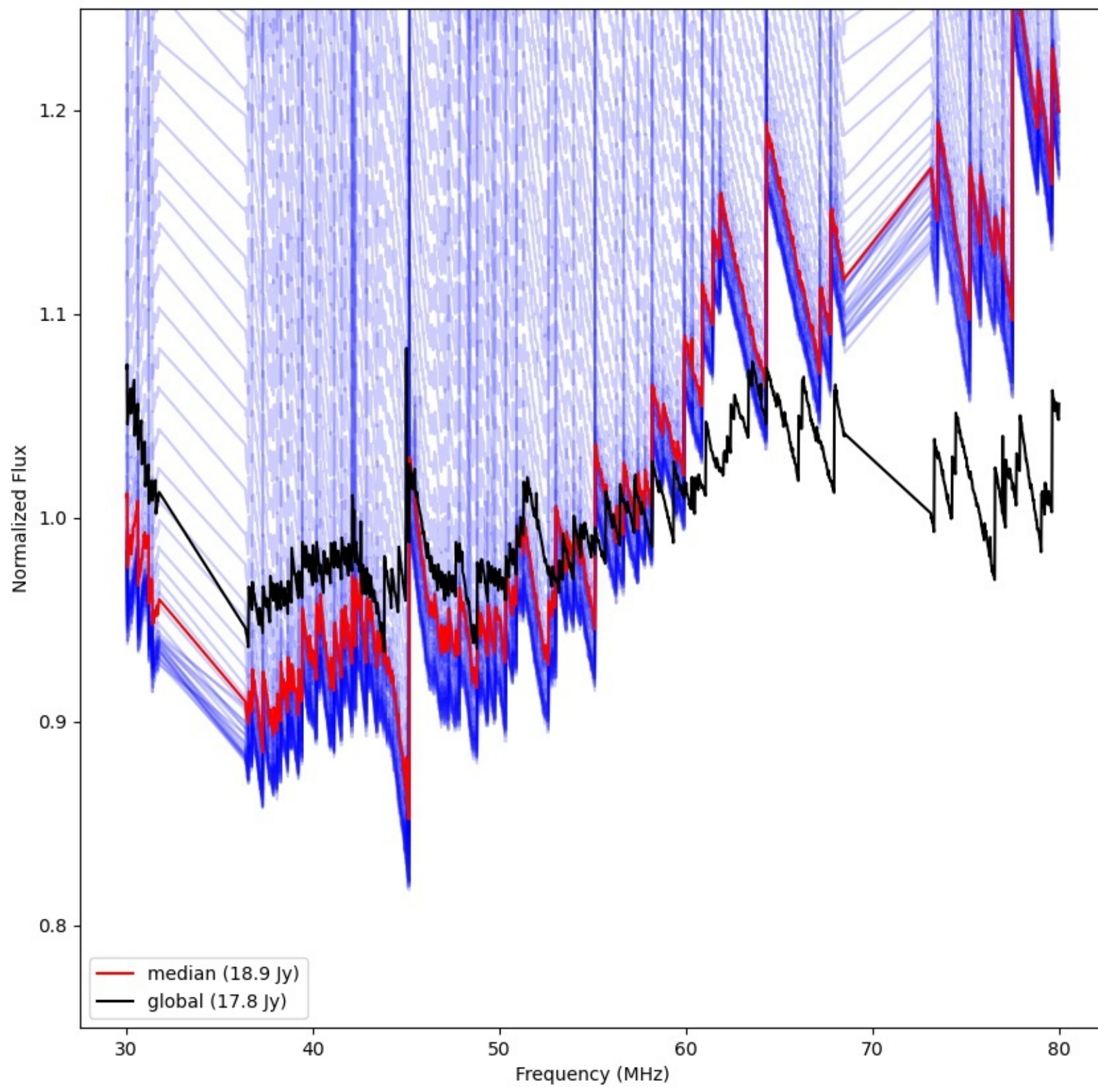
LWA230 - Correlator# 303 - XX - FLAGS:Good
