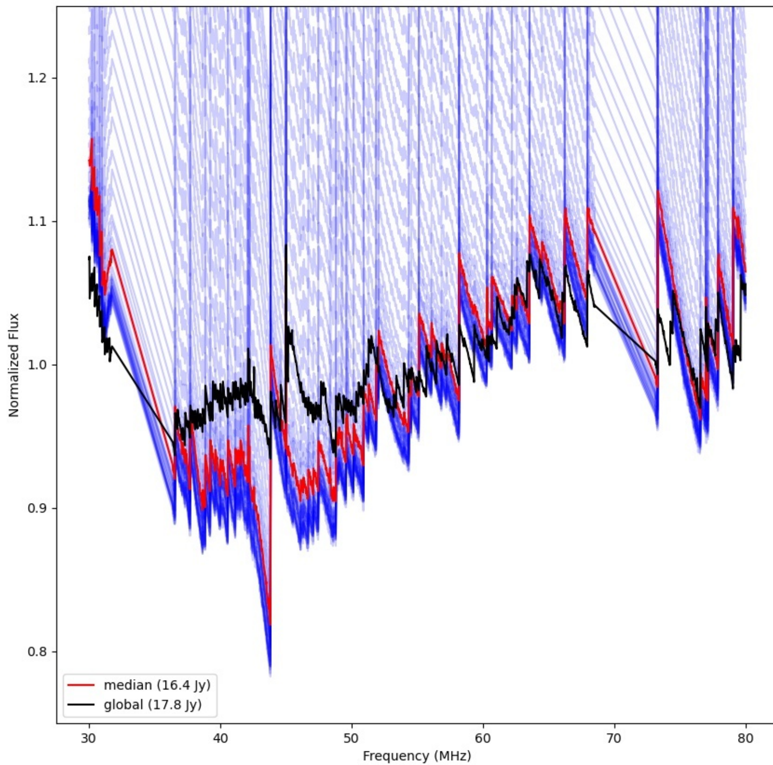
LWA353 - Correlator# 031 - XX - FLAGS:Good
