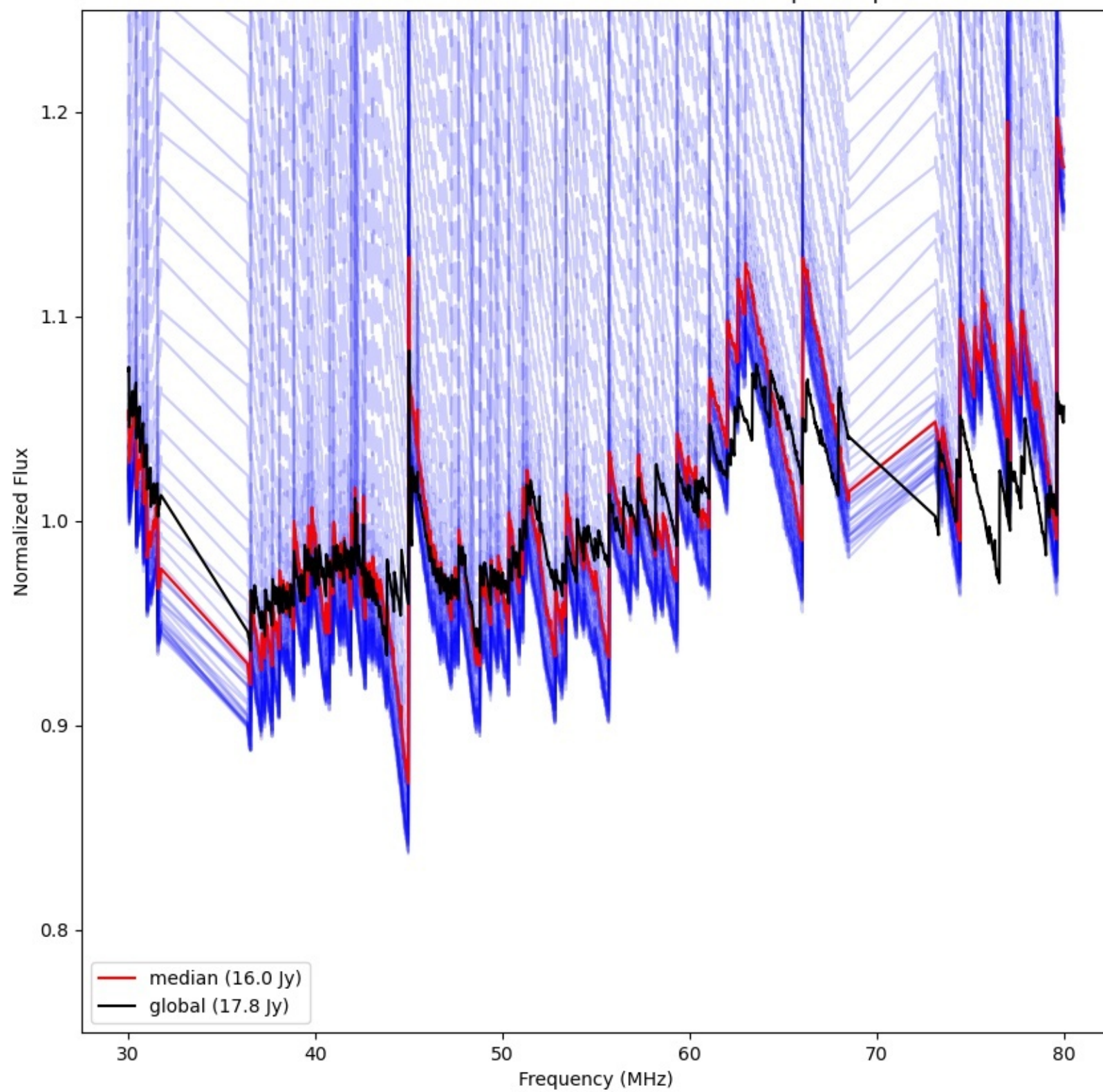
LWA143 - Correlator# 210 - XX - FLAGS:BadSpecShape
