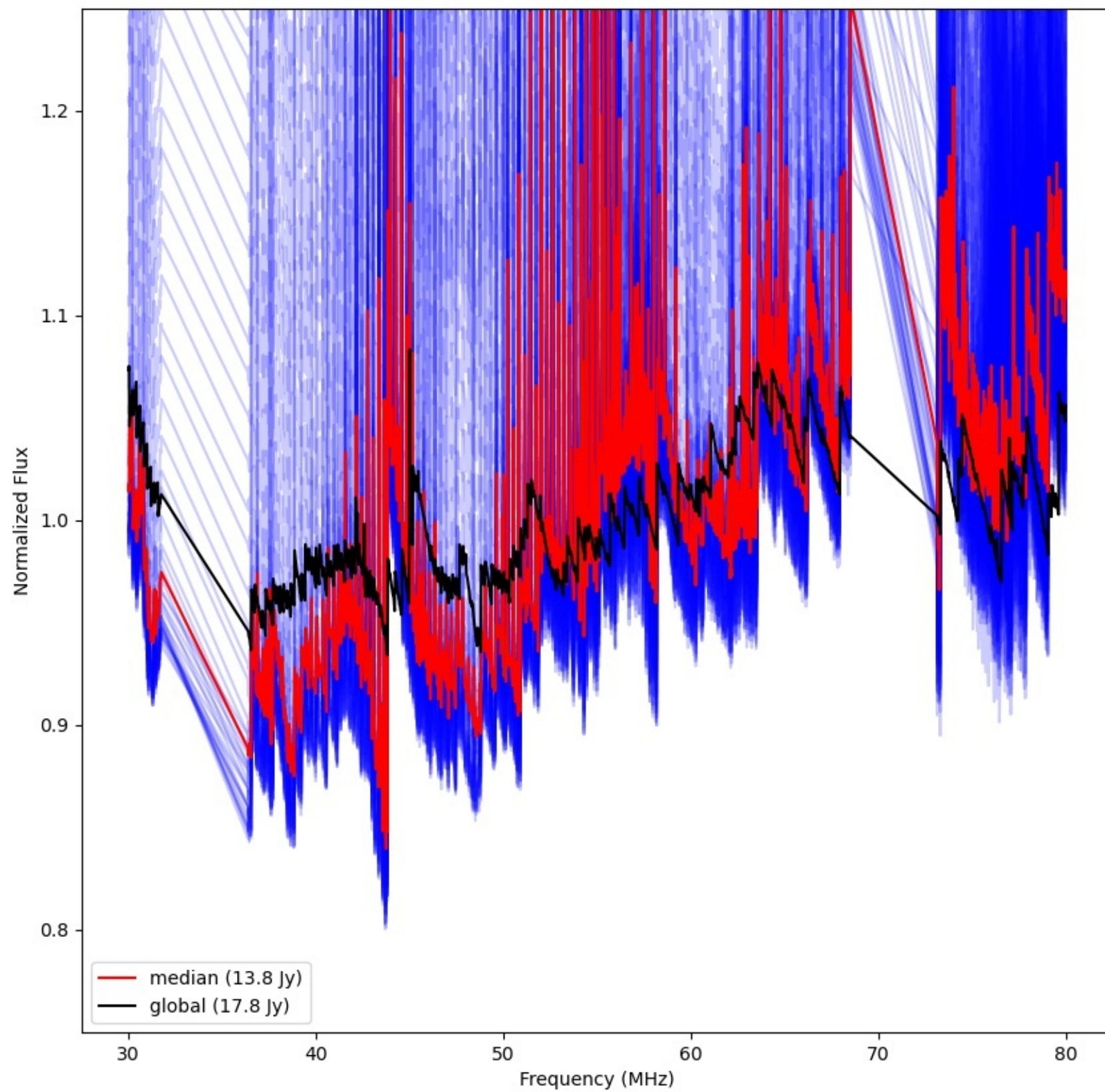
LWA302 - Correlator# 092 - XX - FLAGS:Good
