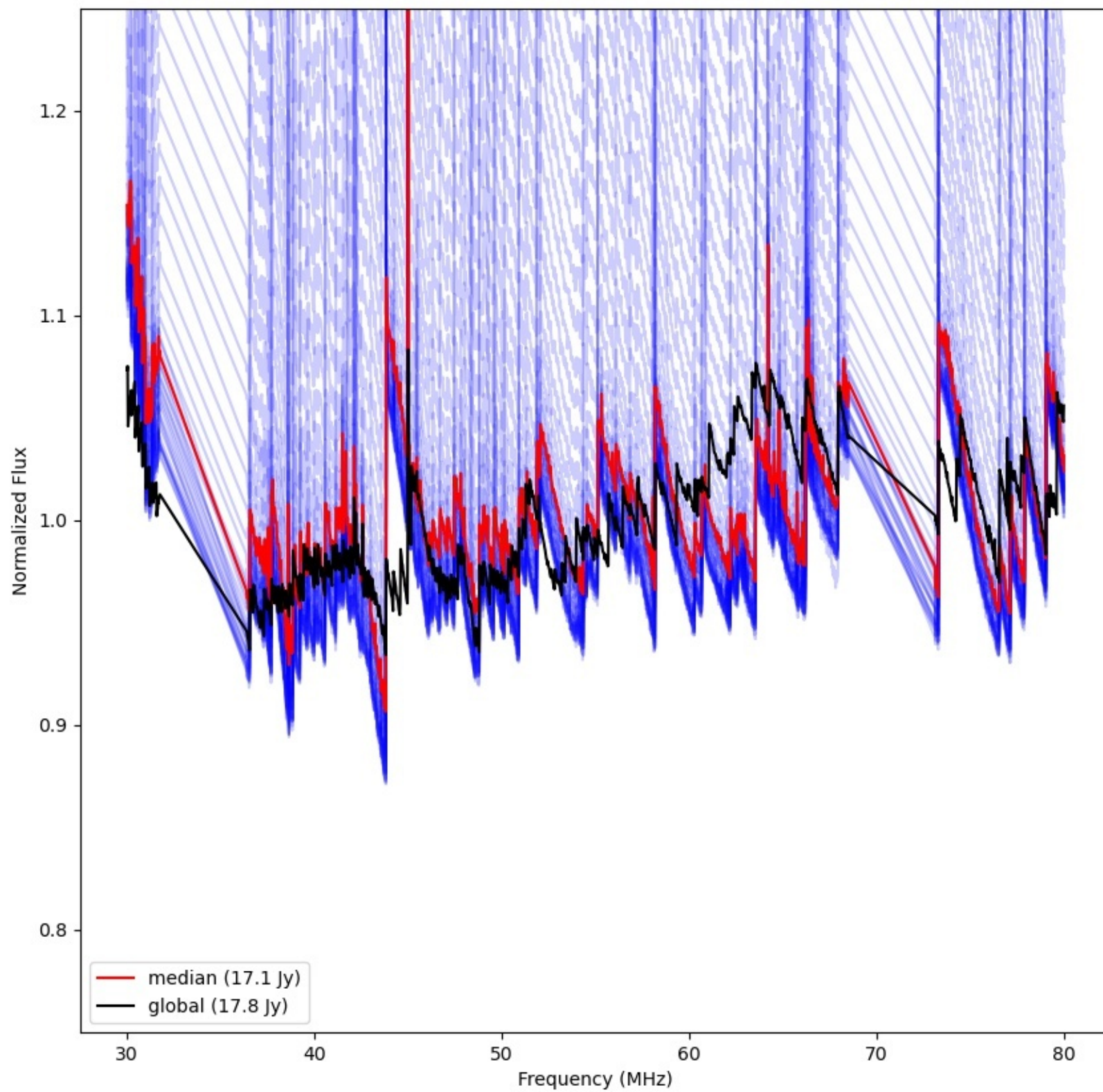
LWA341 - Correlator# 029 - XX - FLAGS:Good
