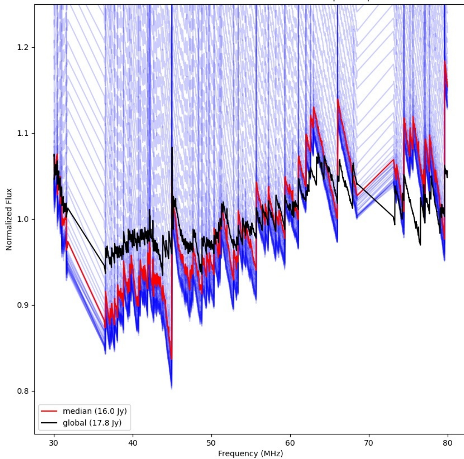
LWA206 - Correlator# 296 - XX - FLAGS:BadSpecShape
