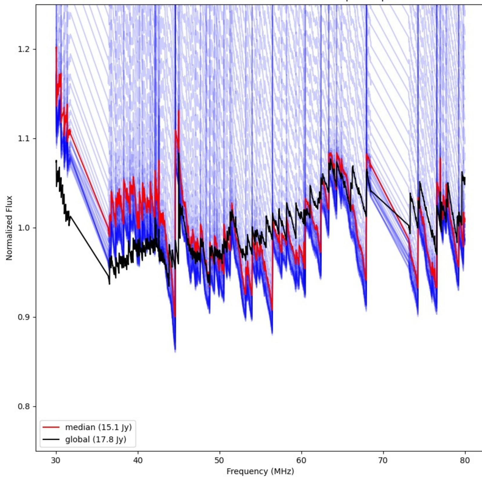
LWA215 - Correlator# 331 - XX - FLAGS:BadSpecShape
