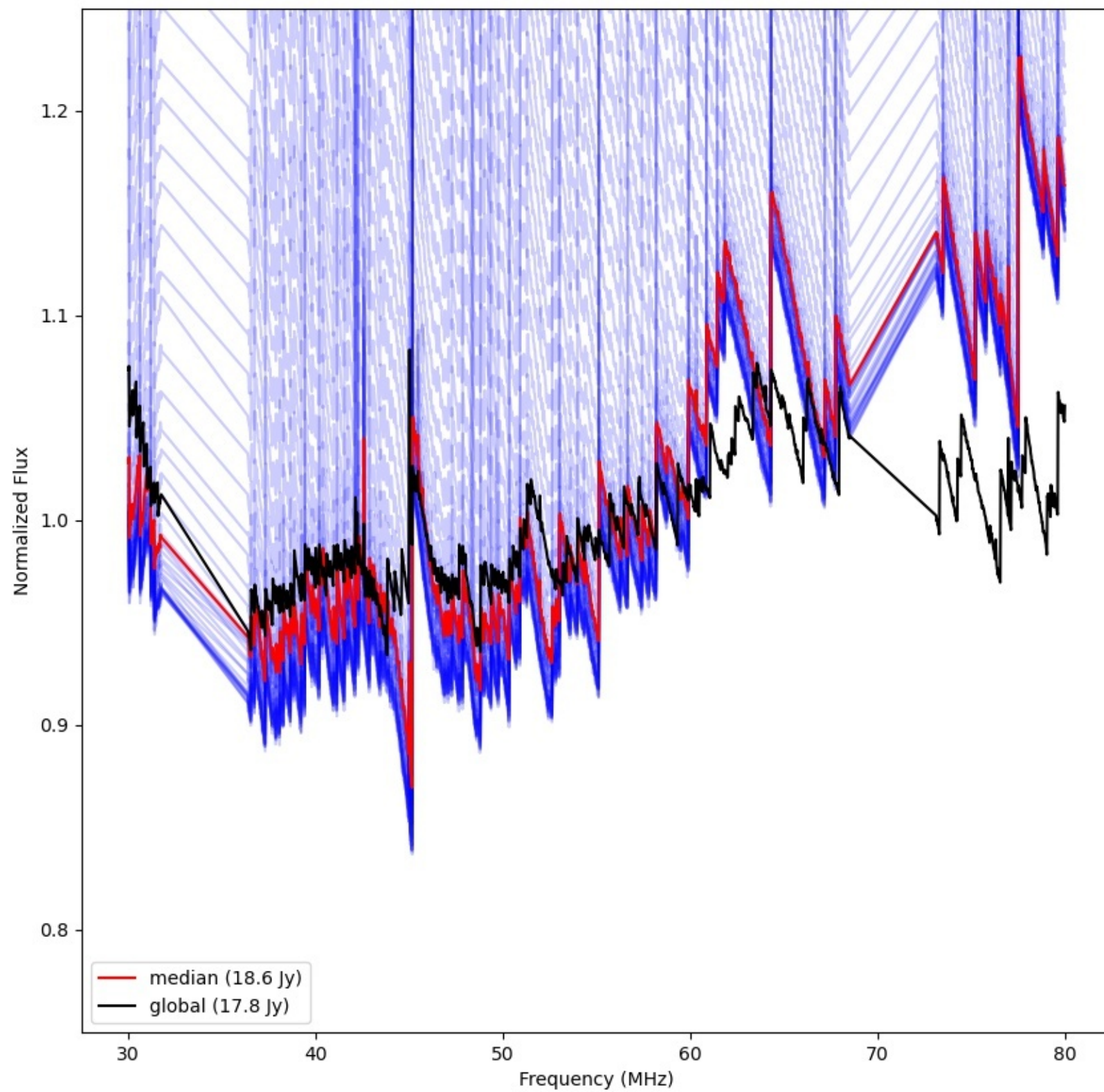
LWA037 - Correlator# 181 - XX - FLAGS:Good
