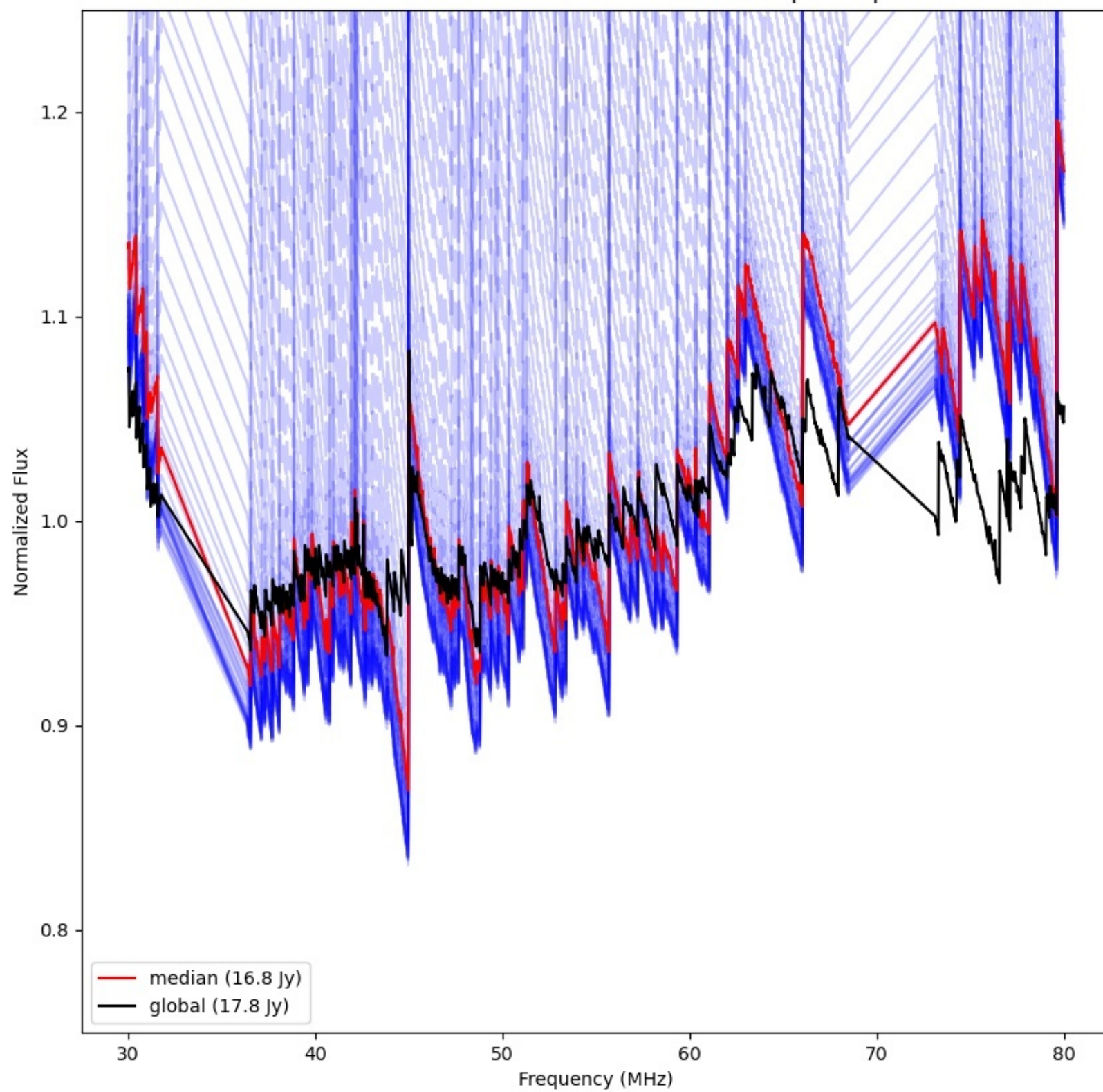
LWA240 - Correlator# 312 - XX - FLAGS:BadSpecShape
