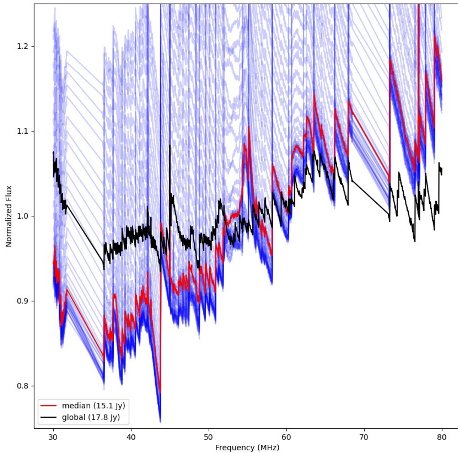
LWA351 - Correlator# 060 - XX - FLAGS:Good
