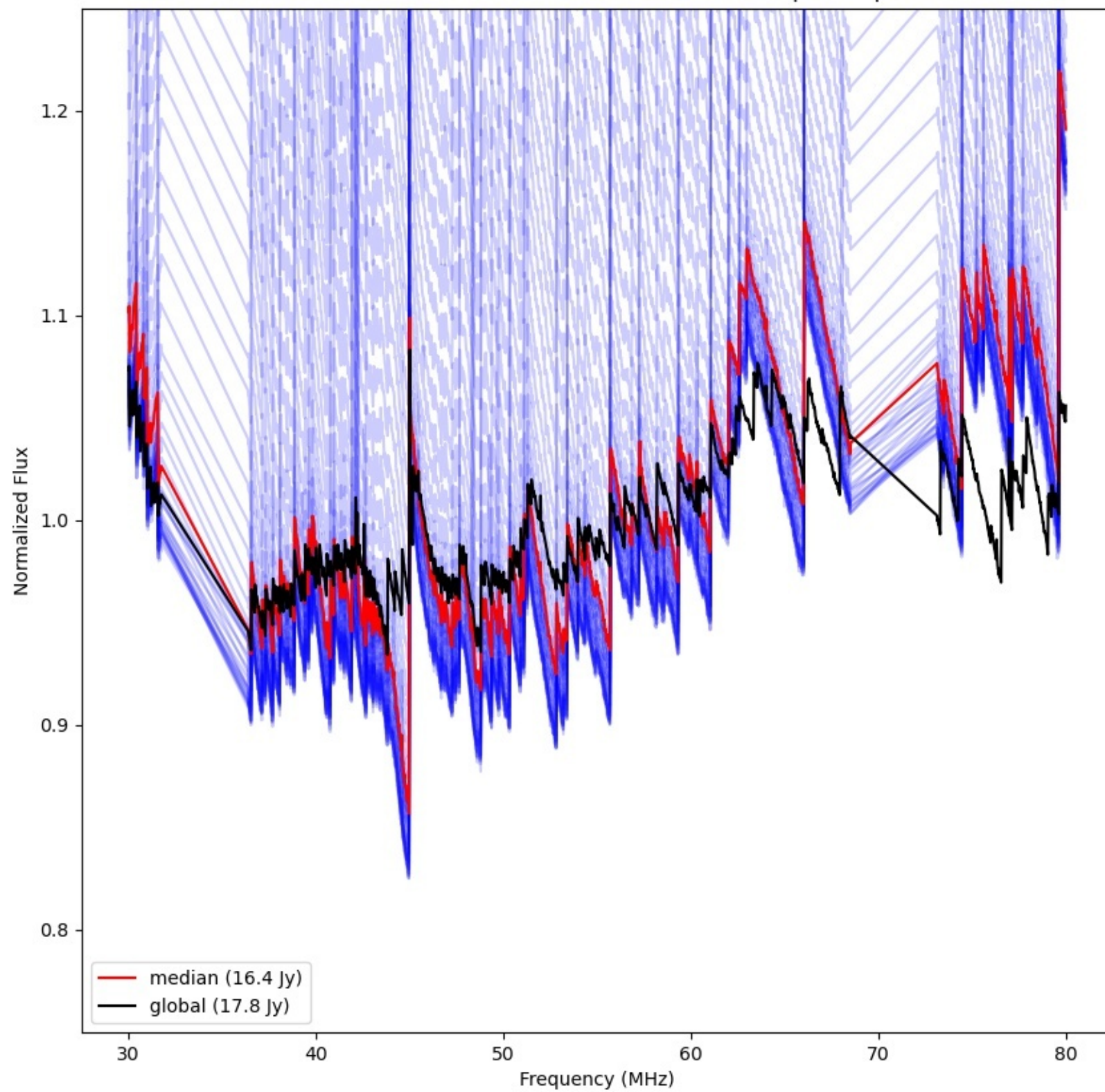
LWA245 - Correlator# 341 - XX - FLAGS:BadSpecShape
