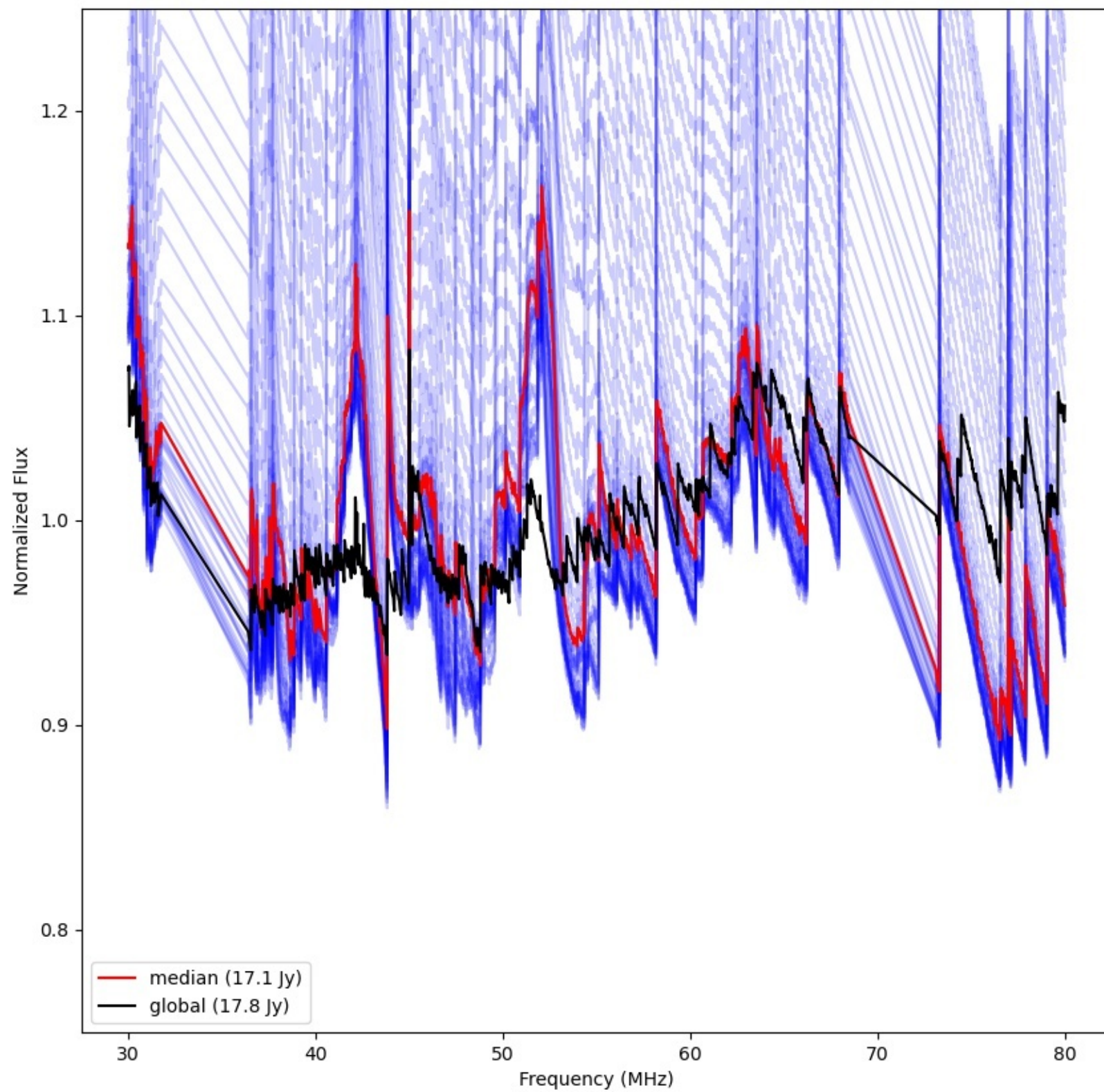
LWA336 - Correlator# 056 - XX - FLAGS:Good
