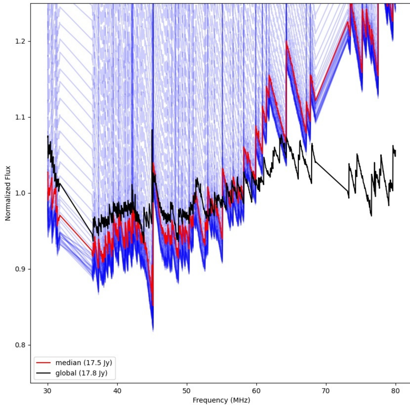
LWA226 - Correlator# 304 - XX - FLAGS:Good
