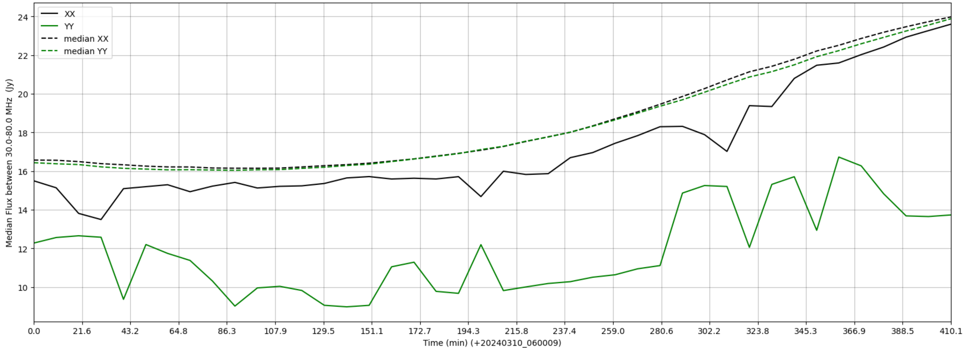
LWA120 - Correlator# 208 - XX FLAGS:BadSpecShape - YY FLAGS:HighTimeVar+BadSpecShape
