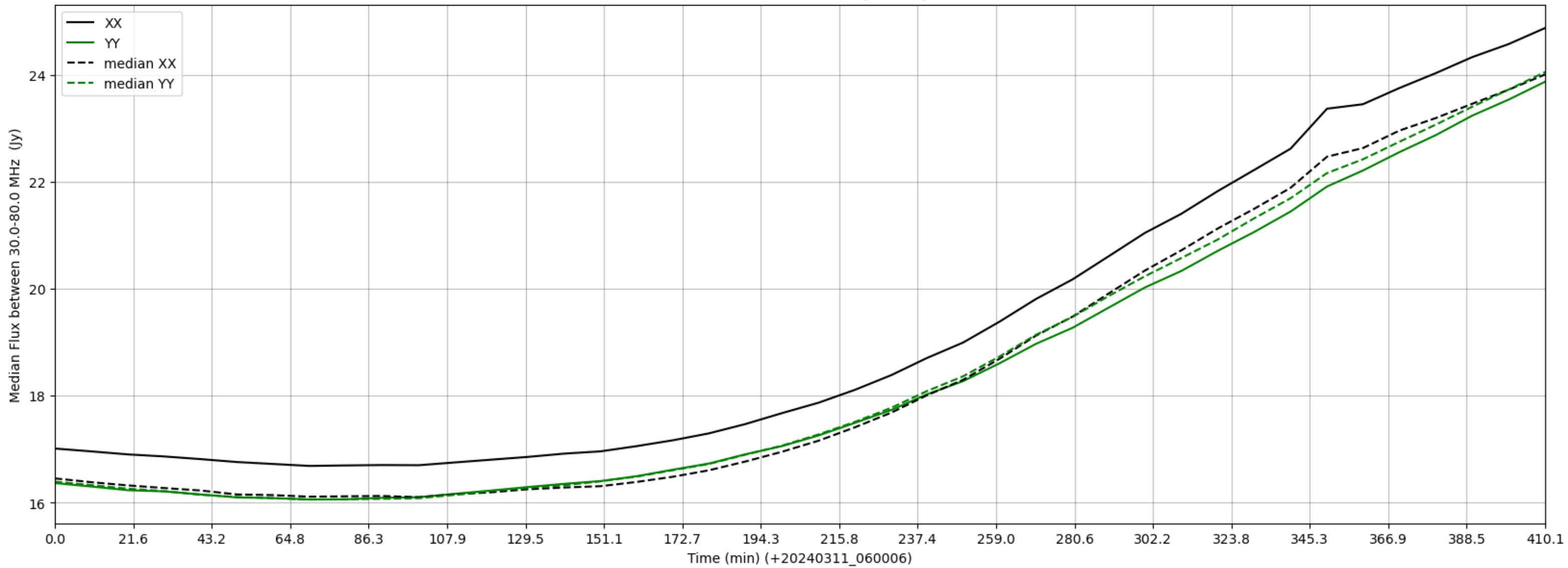
LWA126 - Correlator# 226 - XX FLAGS:BadSpecShape - YY FLAGS:Good
