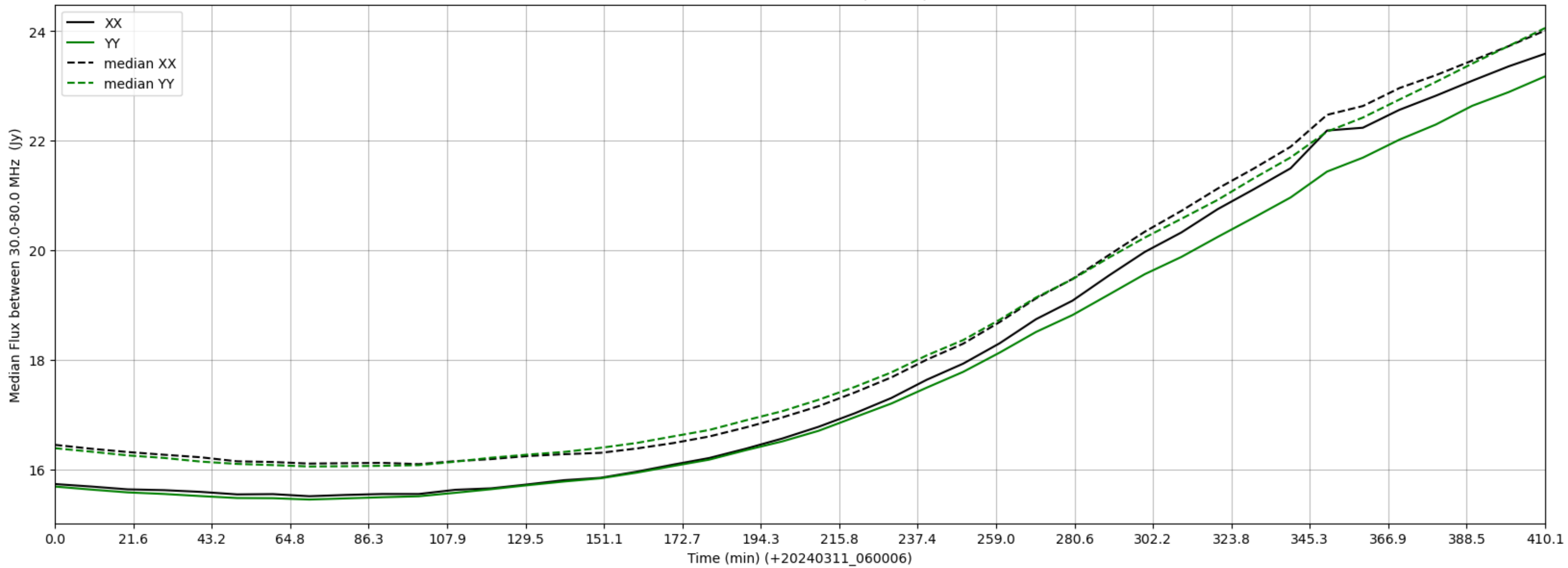
LWA089 - Correlator# 144 - XX FLAGS:BadSpecShape - YY FLAGS:Good
