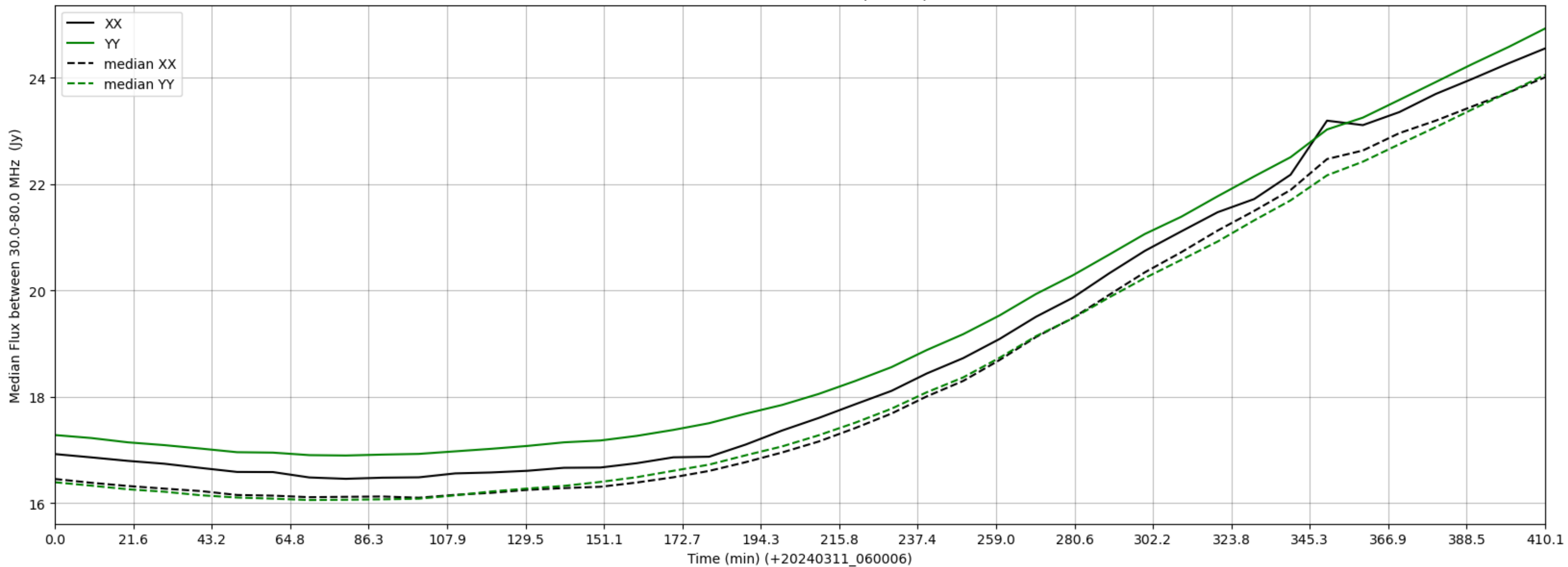
LWA057 - Correlator# 134 - XX FLAGS:BadSpecShape - YY FLAGS:Good
