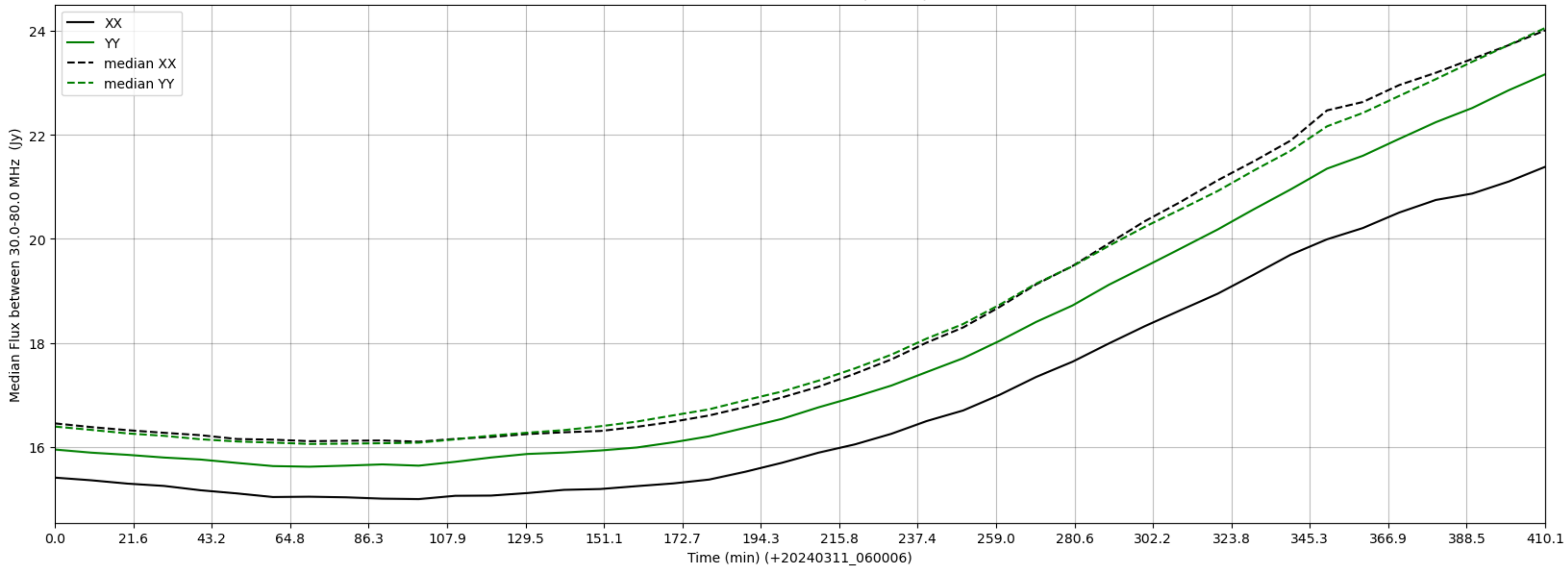
LWA312 - Correlator# 019 - XX FLAGS:BadSpecShape - YY FLAGS:Good
