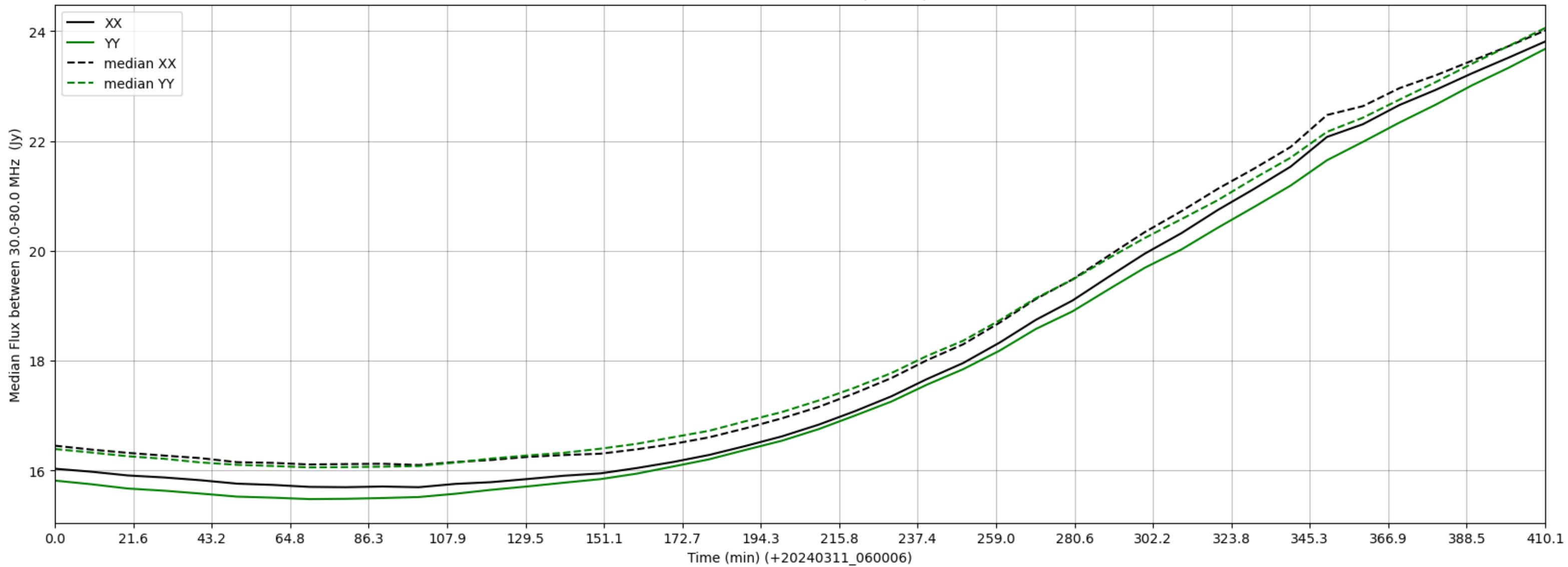
LWA094 - Correlator# 151 - XX FLAGS:BadSpecShape - YY FLAGS:Good
