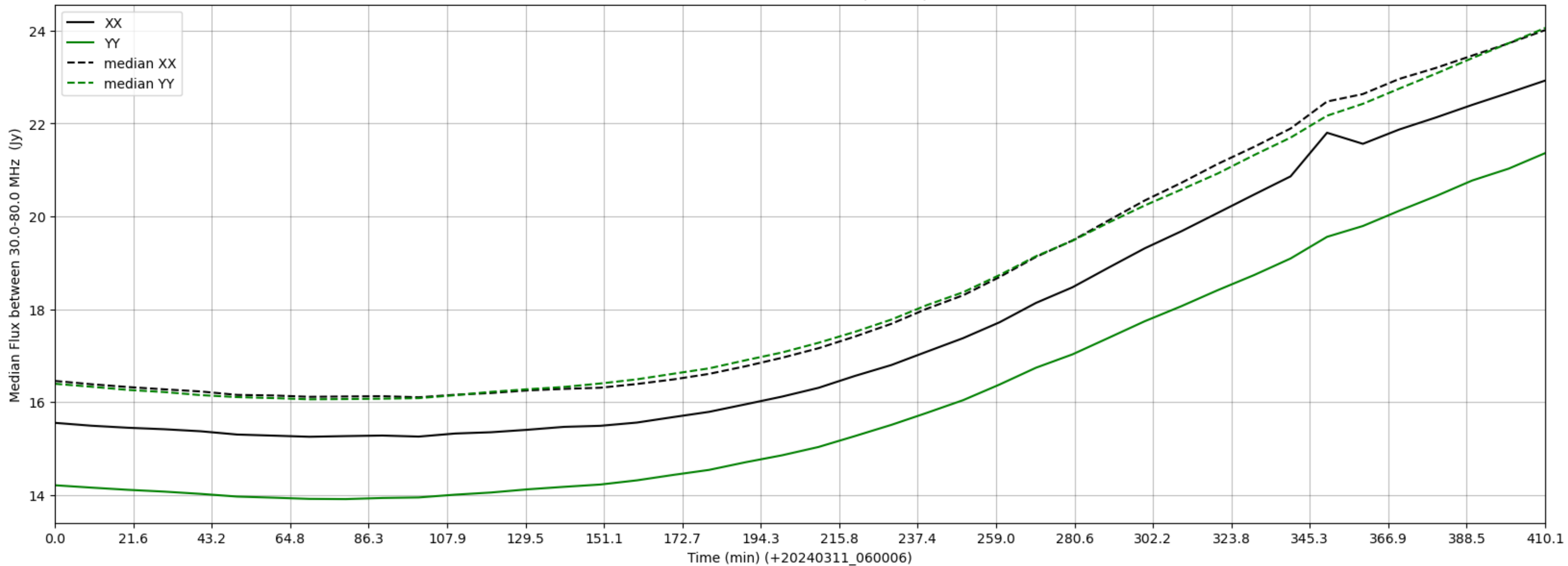
LWA190 - Correlator# 244 - XX FLAGS:BadSpecShape - YY FLAGS:Good
