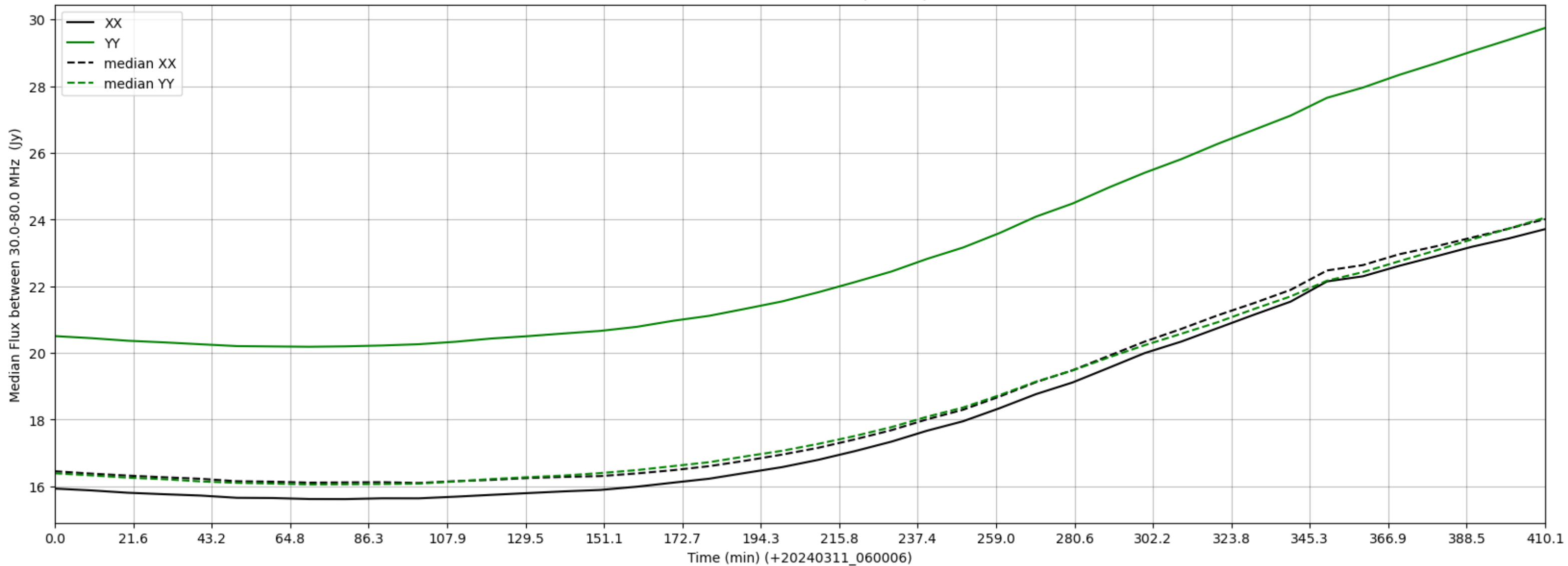
LWA246 - Correlator# 340 - XX FLAGS:BadSpecShape - YY FLAGS:Good
