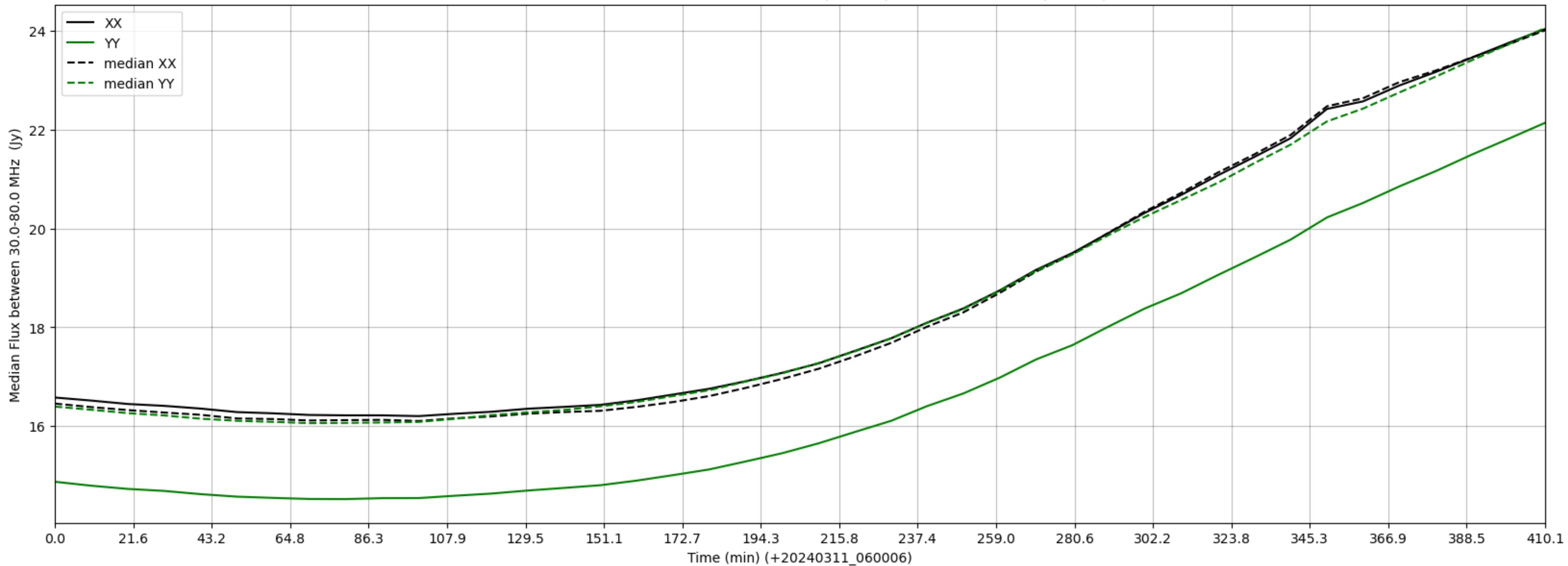
LWA160 - Correlator# 239 - XX FLAGS:BadSpecShape - YY FLAGS:BadSpecShape
