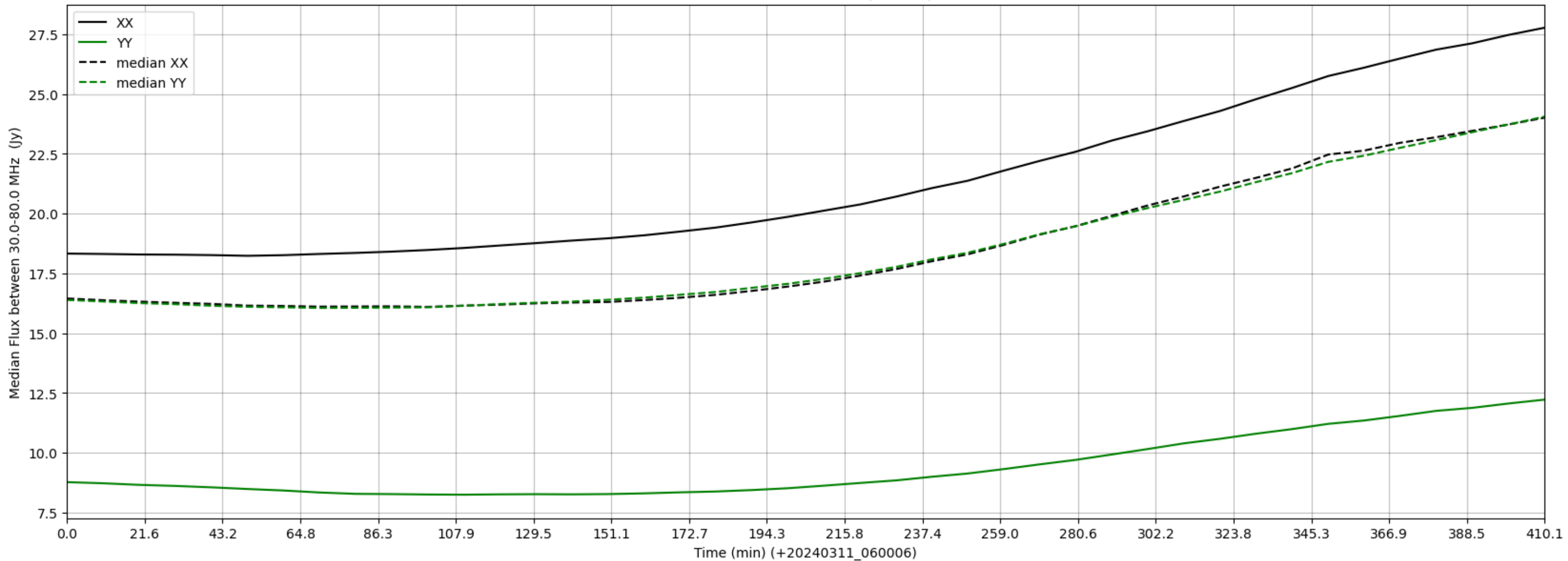
LWA319 - Correlator# 190 - XX FLAGS:BadSpecShape - YY FLAGS:Good
