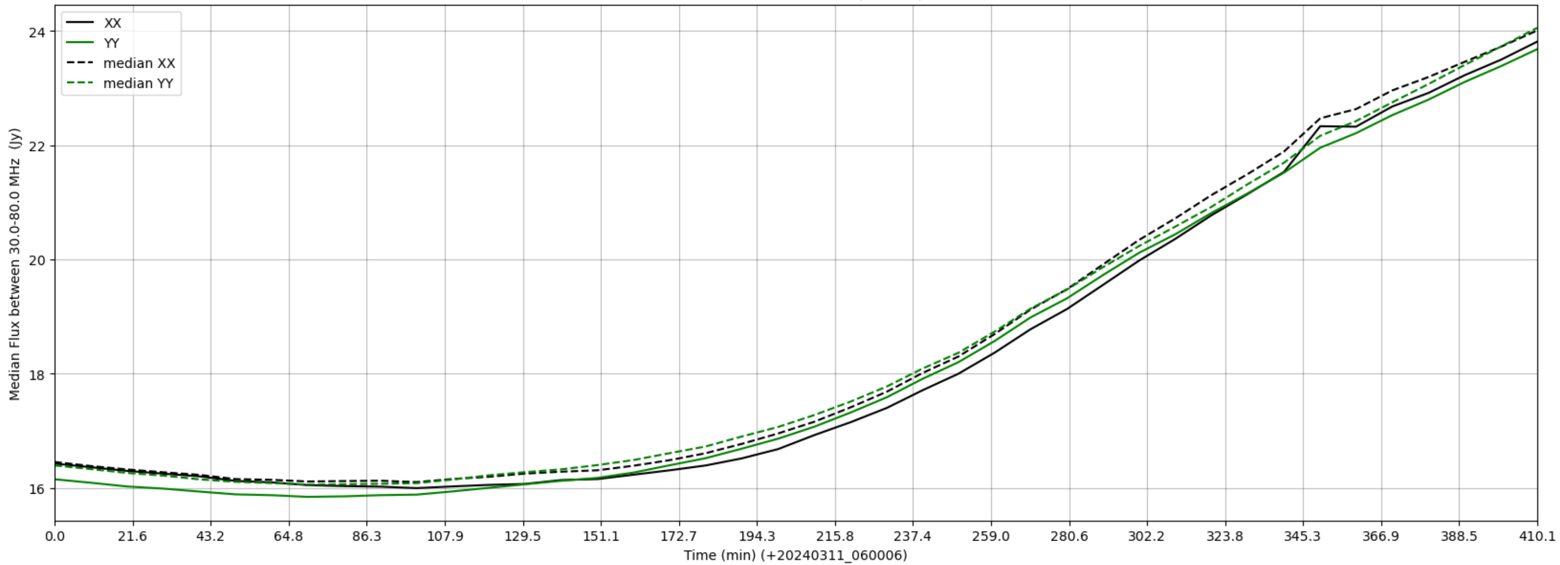
LWA183 - Correlator# 324 - XX FLAGS:BadSpecShape - YY FLAGS:Good
