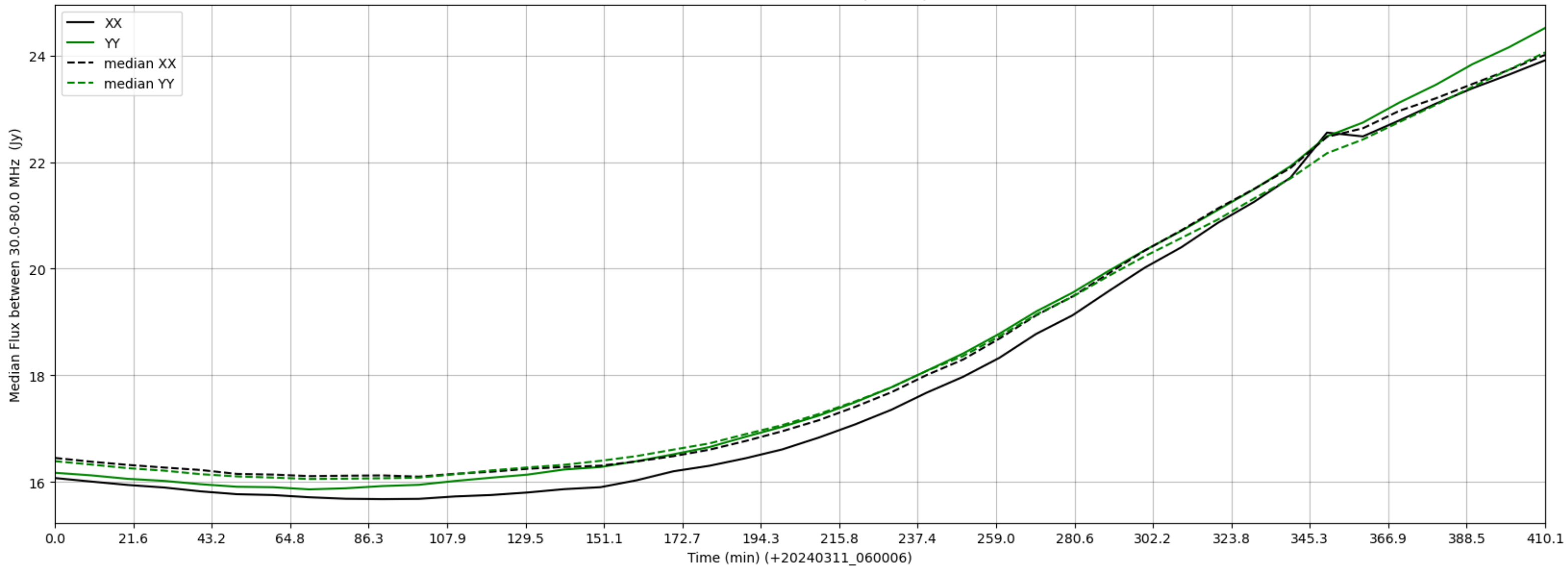
LWA087 - Correlator# 142 - XX FLAGS:BadSpecShape - YY FLAGS:Good
