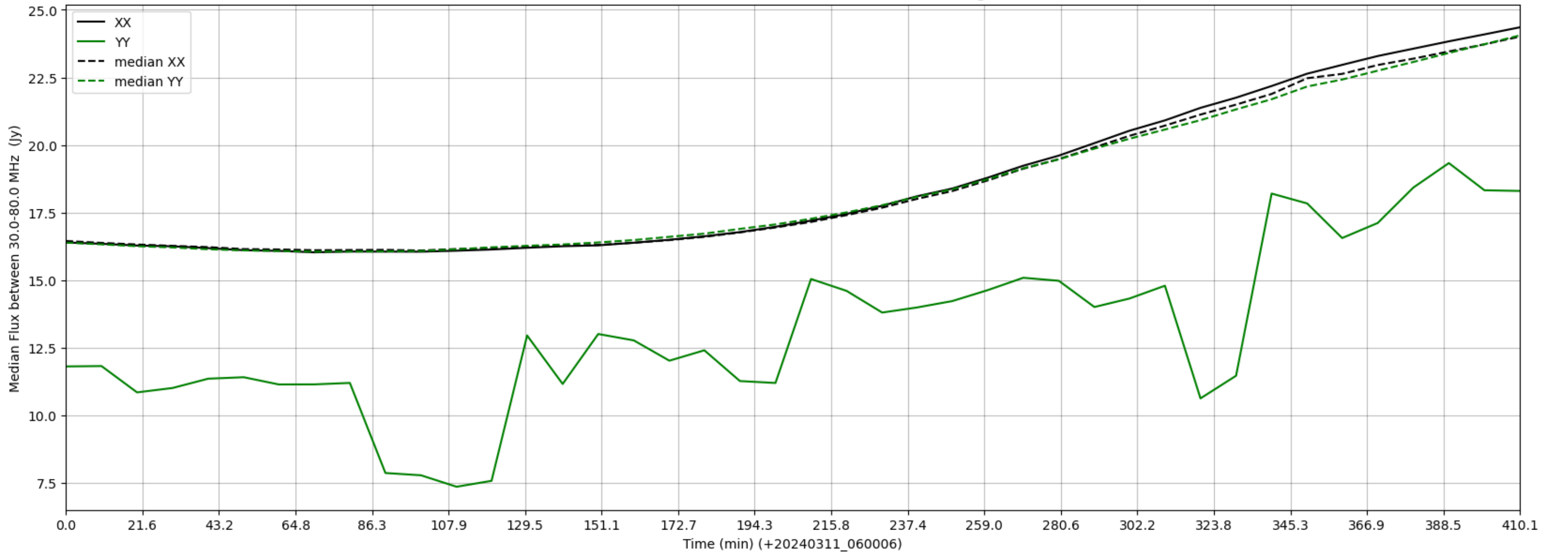
LWA044 - Correlator# 080 - XX FLAGS:Good - YY FLAGS:HighTimeVar
