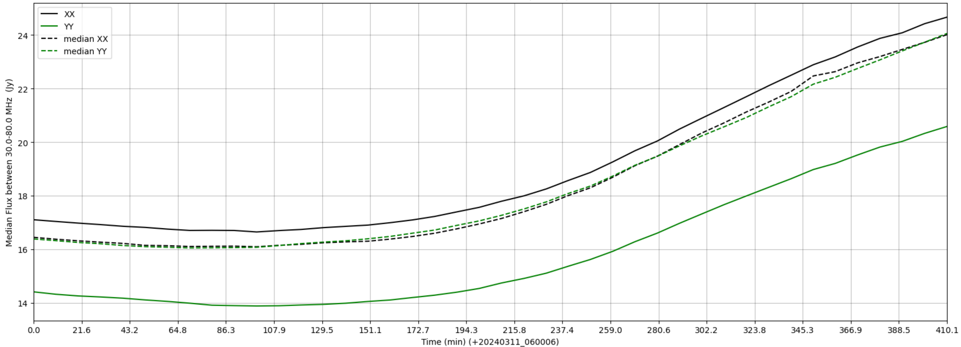
LWA350 - Correlator# 319 - XX FLAGS:BadSpecShape - YY FLAGS:Good
