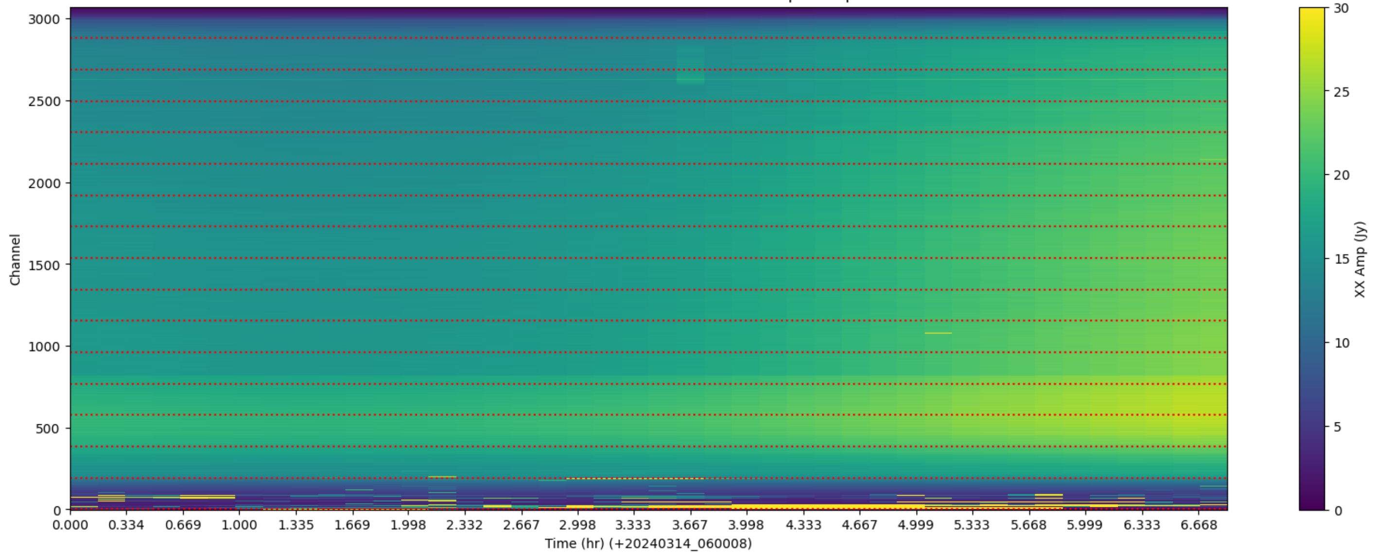
LWA062 - Correlator# 138 - XX - FLAGS: BadSpecShape
