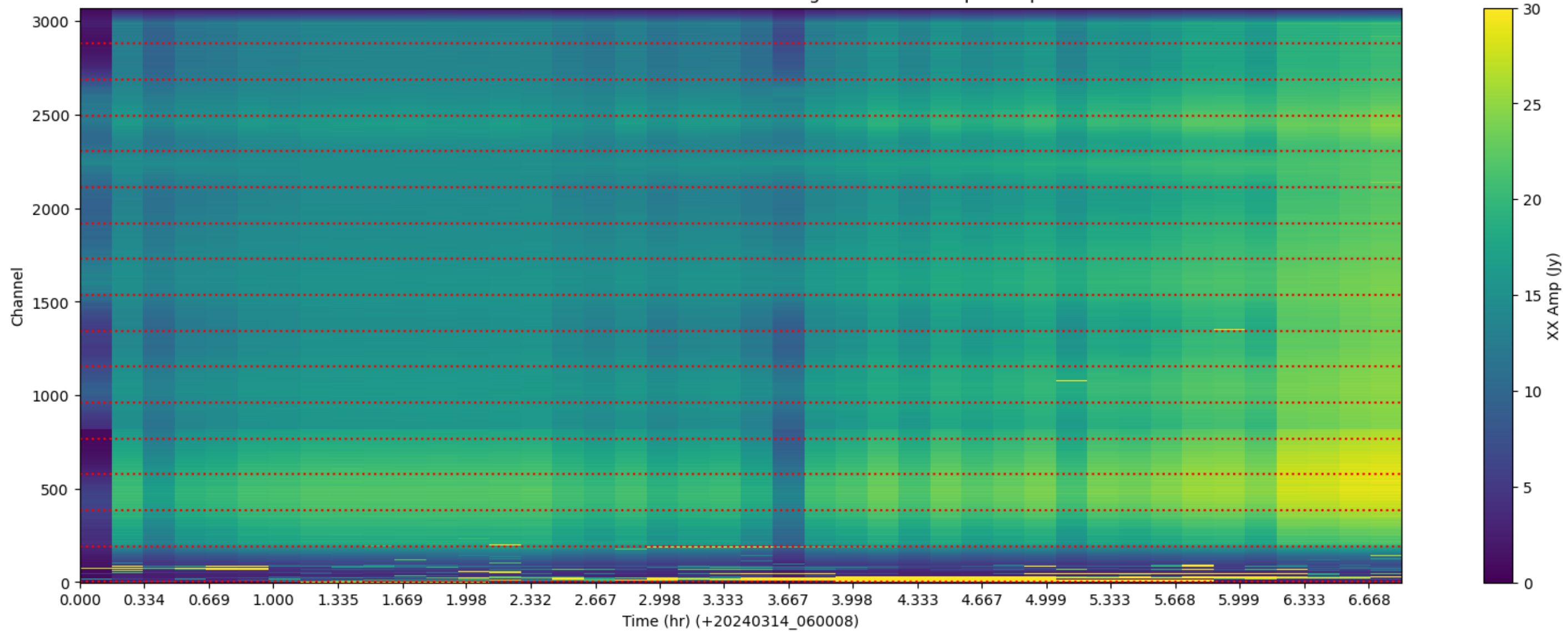
LWA120 - Correlator# 208 - XX - FLAGS: HighTimeVar+BadSpecShape
