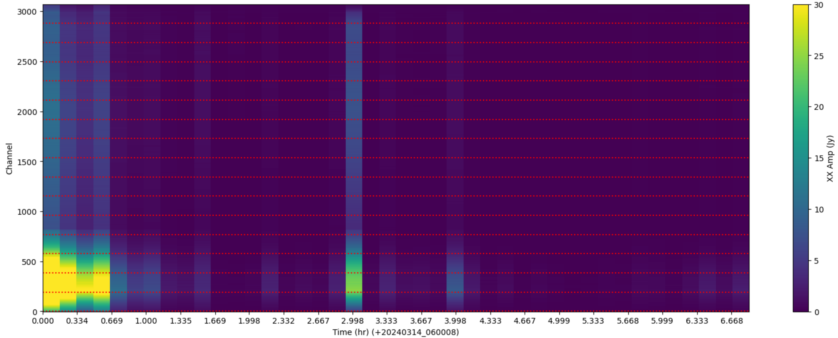
LWA353 - Correlator# 031 - XX - FLAGS: LowFlux
