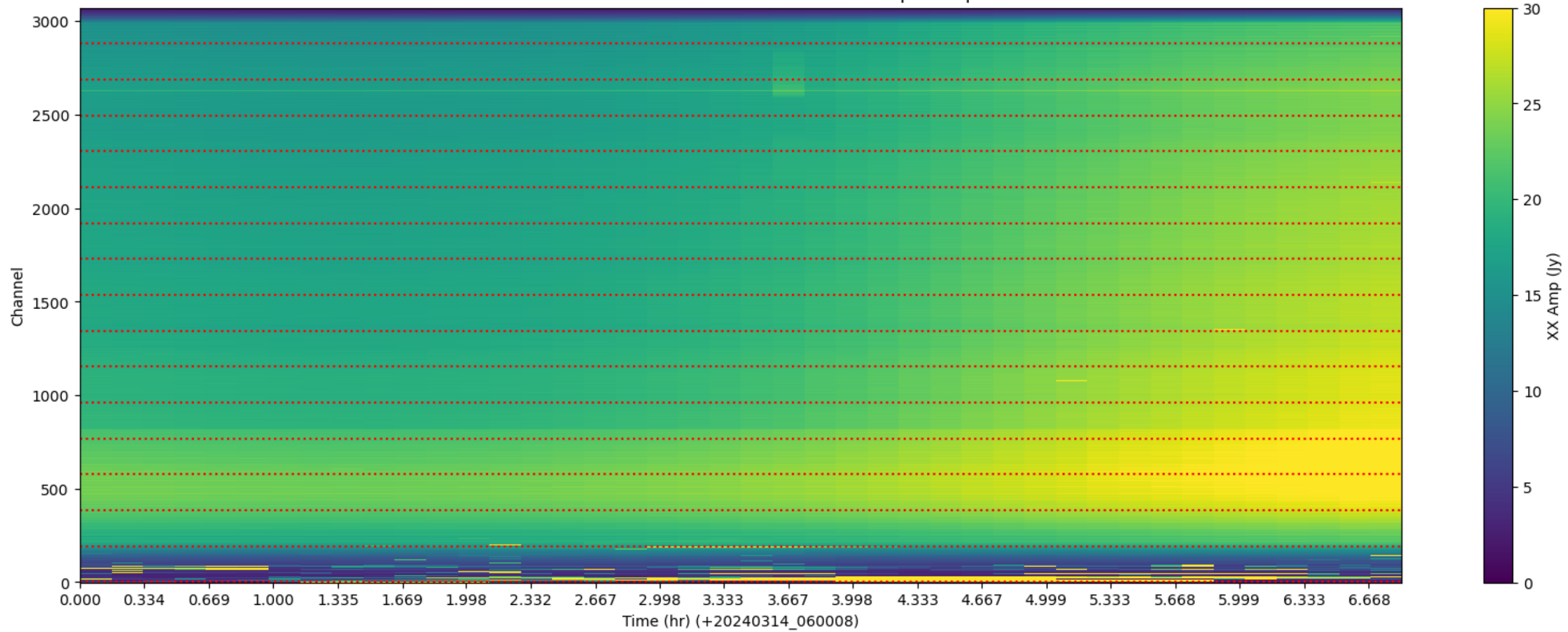
LWA024 - Correlator# 106 - XX - FLAGS: BadSpecShape
