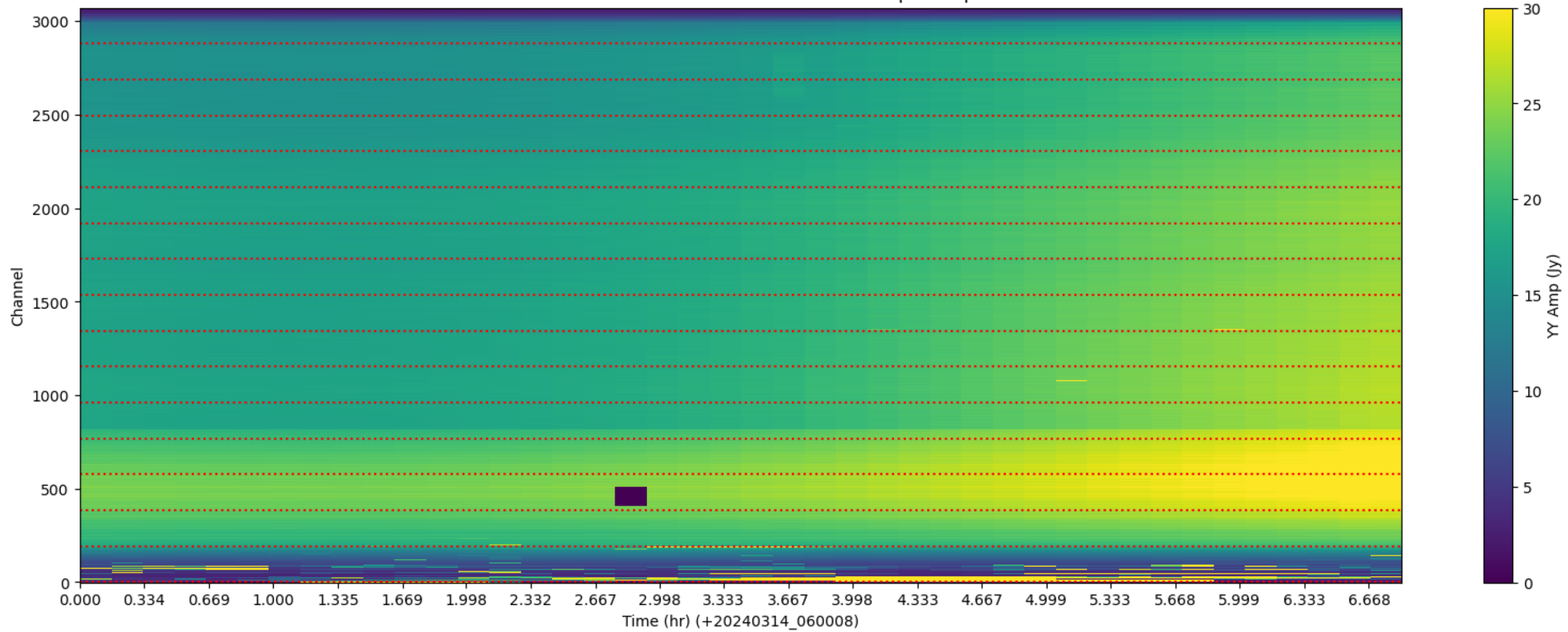
LWA122 - Correlator# 152 - YY - FLAGS: BadSpecShape
