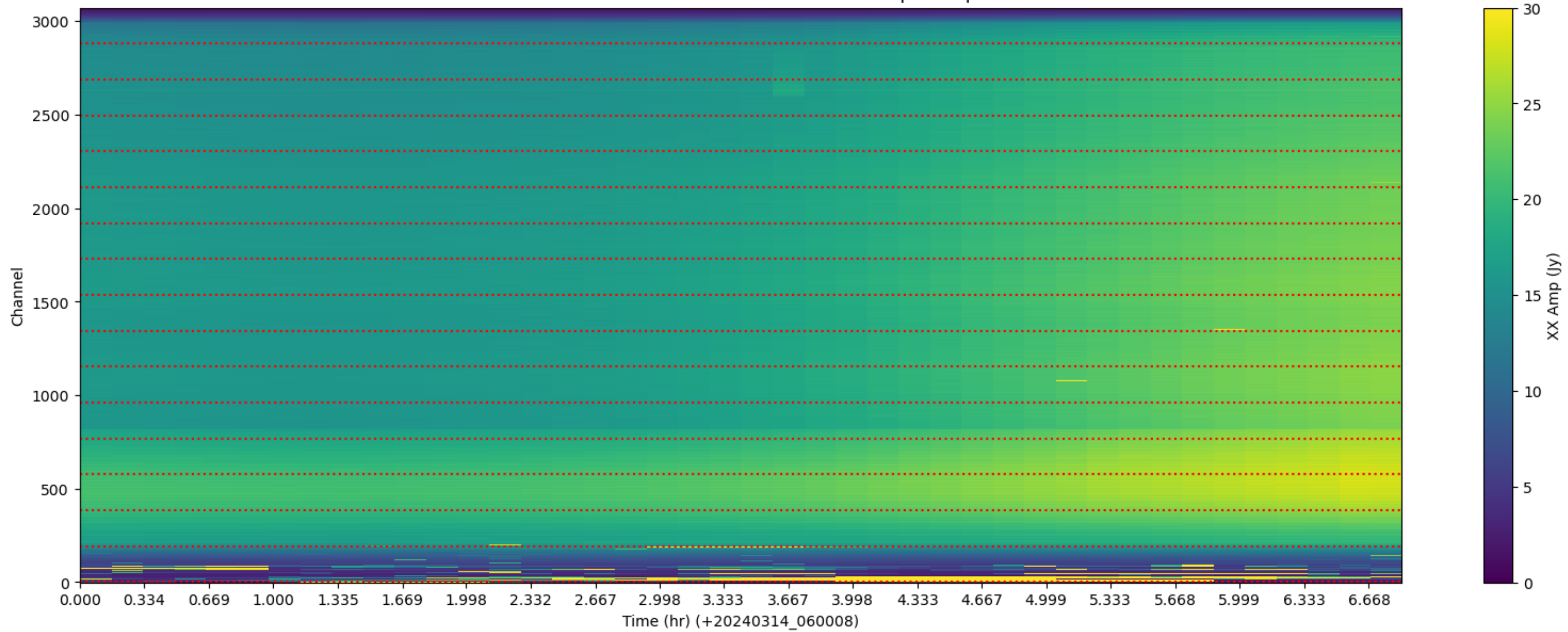
LWA053 - Correlator# 116 - XX - FLAGS: BadSpecShape
