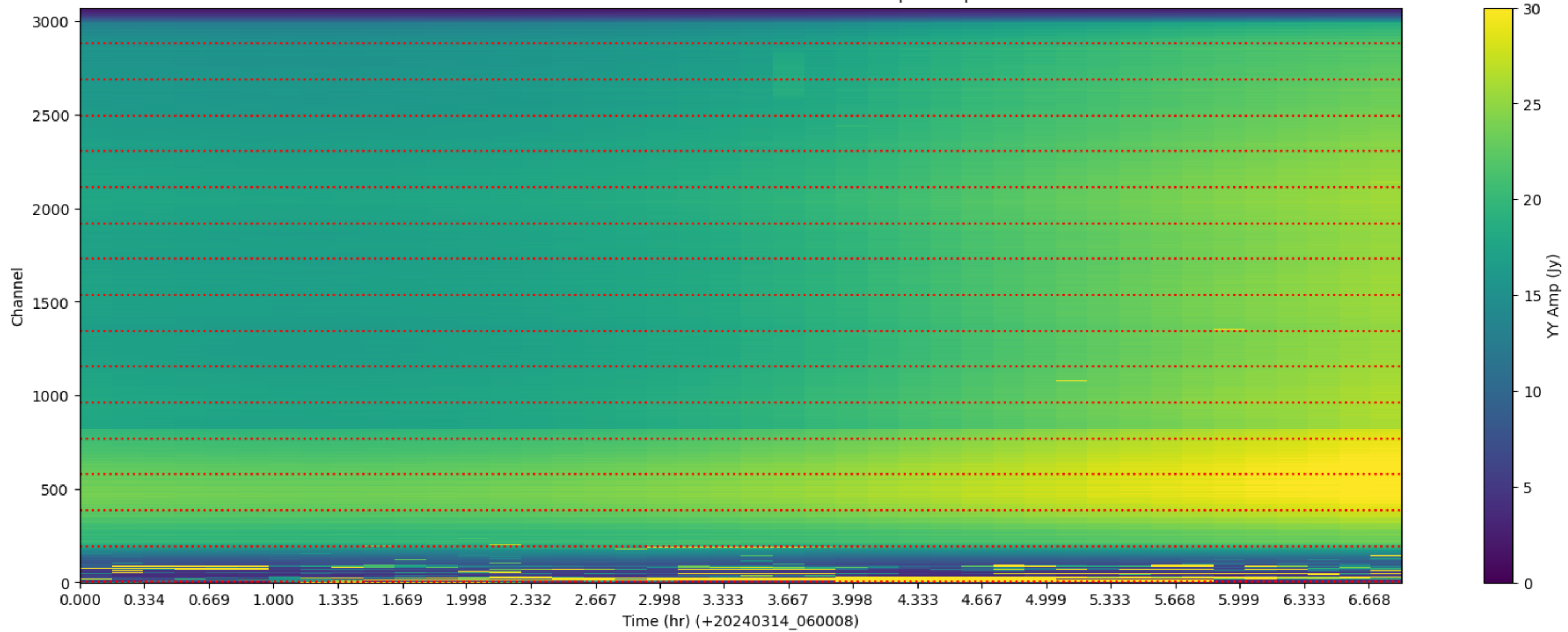
LWA076 - Correlator# 193 - YY - FLAGS: BadSpecShape
