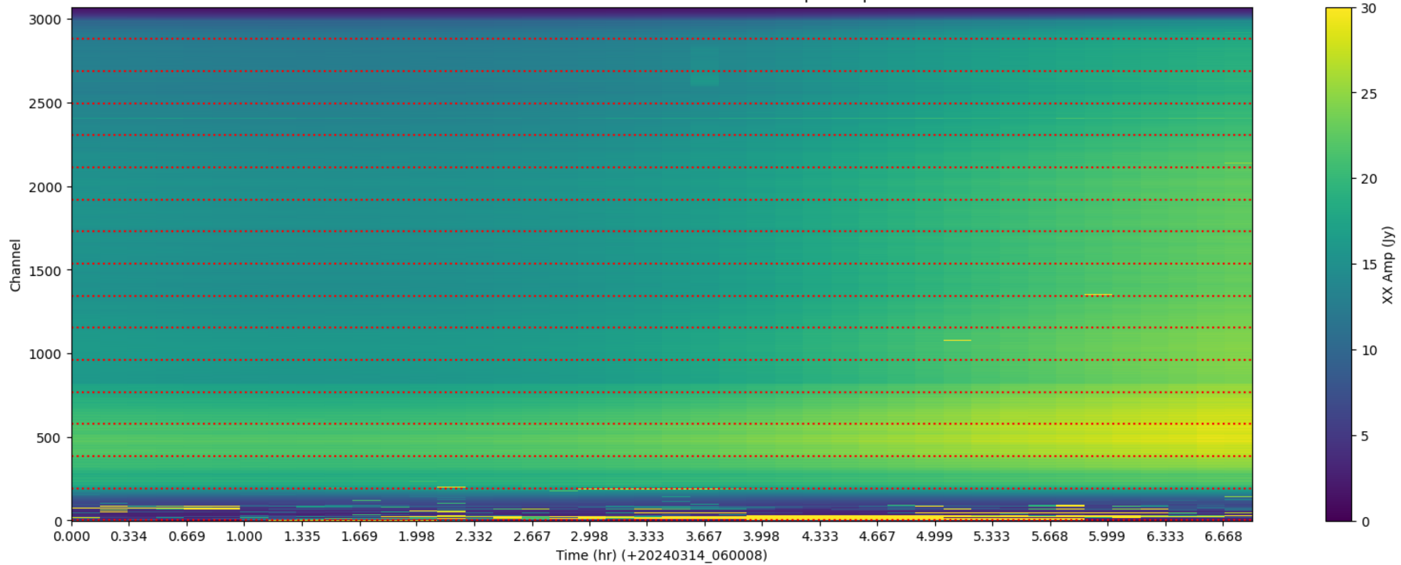
LWA093 - Correlator# 148 - XX - FLAGS: BadSpecShape
