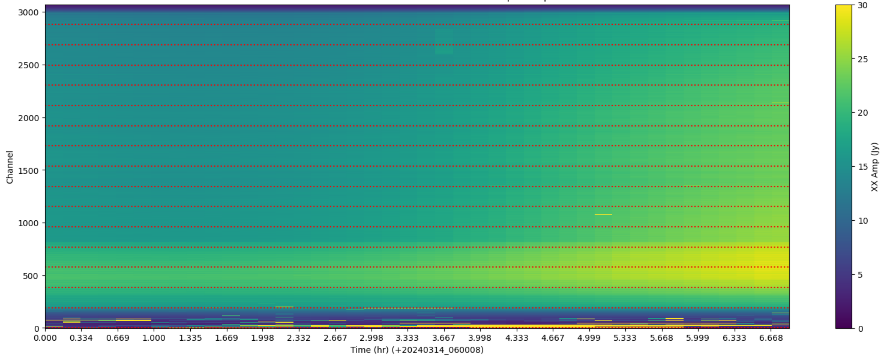
LWA064 - Correlator# 141 - XX - FLAGS: BadSpecShape
