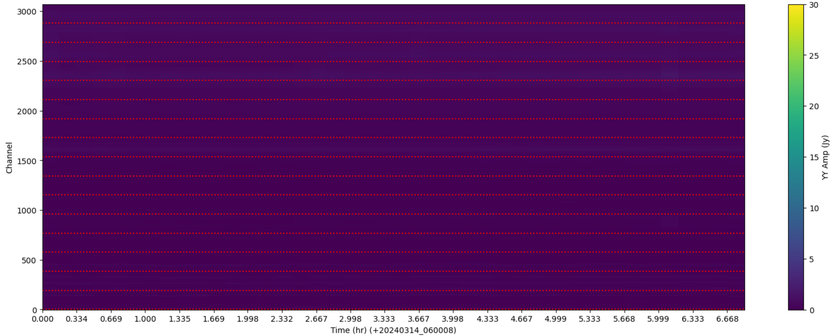
LWA105 - Correlator# 178 - YY - FLAGS: LowFlux
