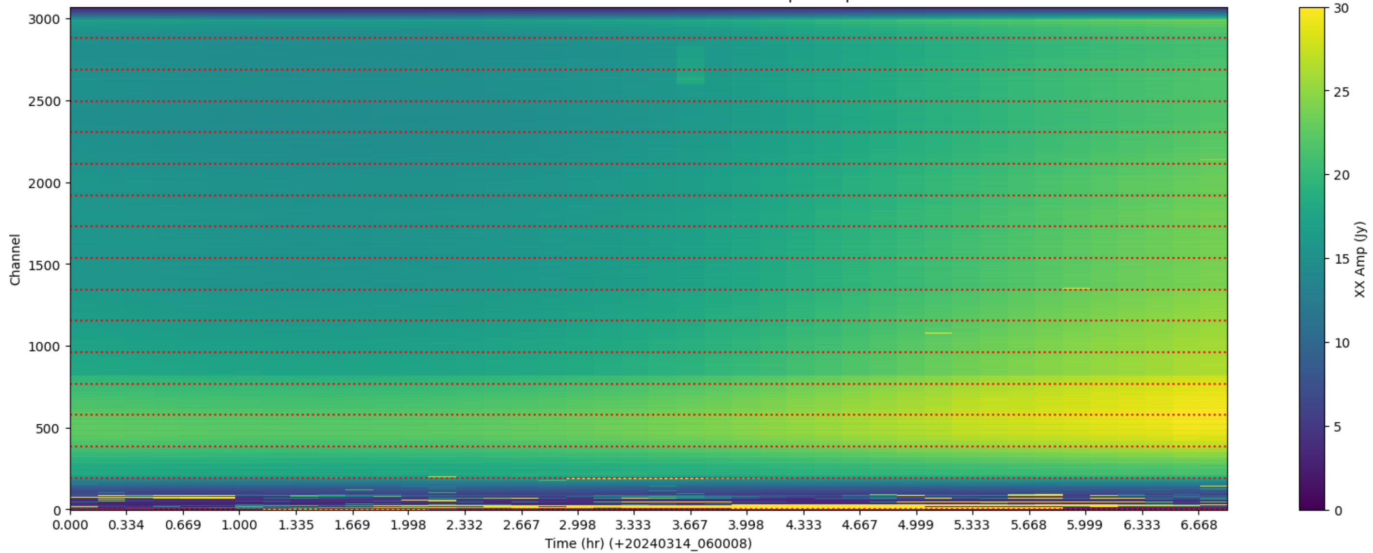
LWA049 - Correlator# 112 - XX - FLAGS: BadSpecShape
