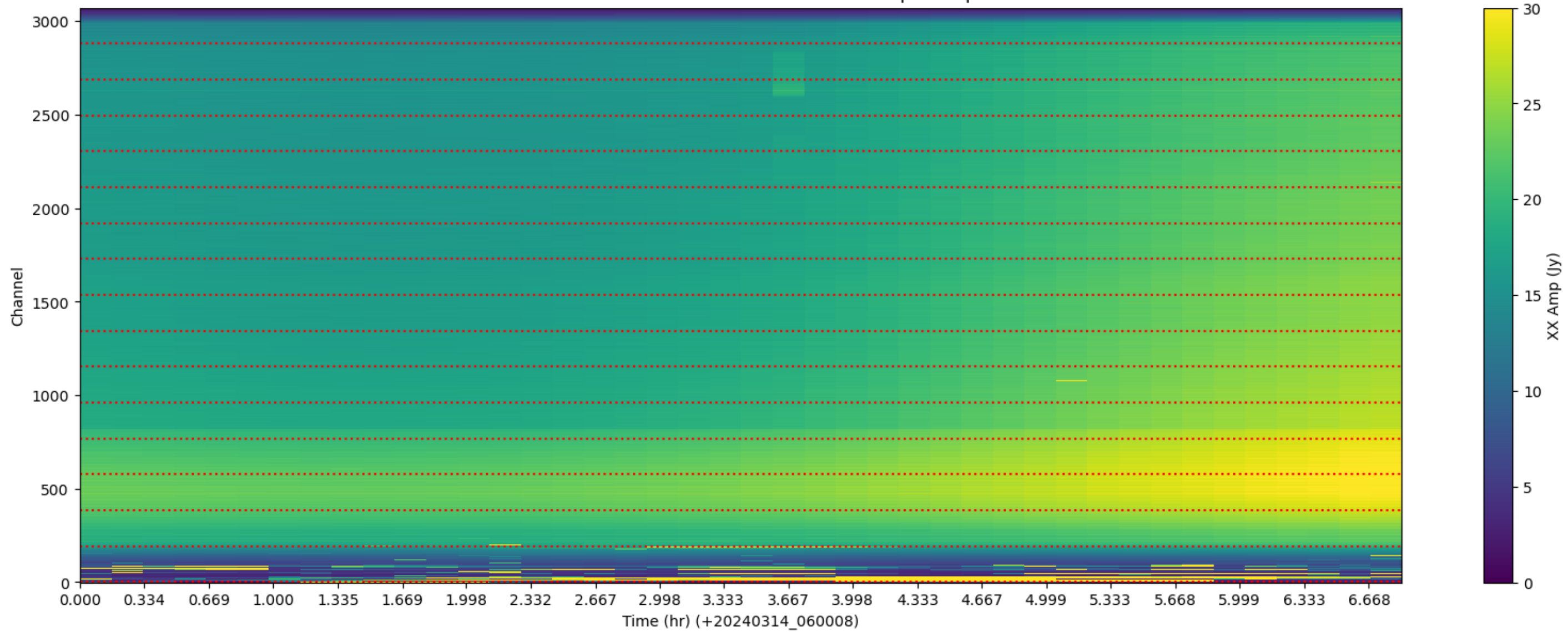
LWA023 - Correlator# 107 - XX - FLAGS: BadSpecShape
