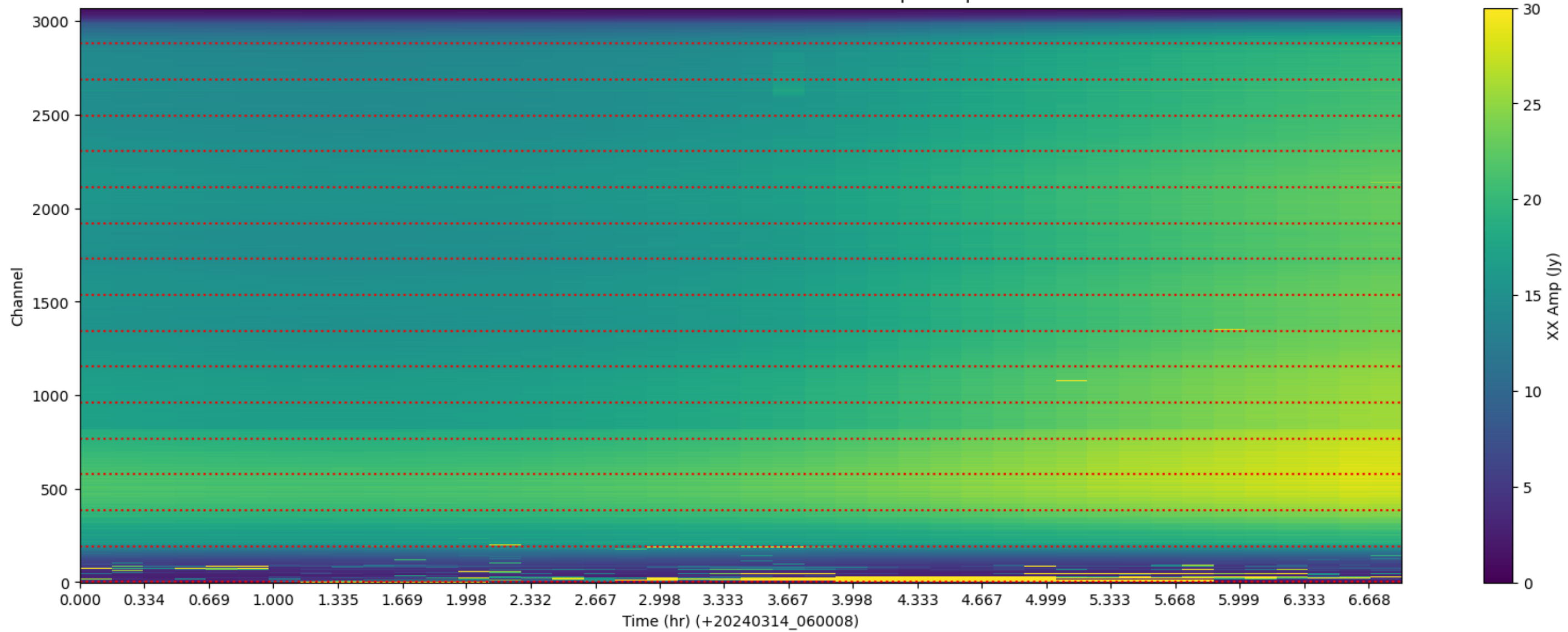
LWA213 - Correlator# 329 - XX - FLAGS: BadSpecShape
