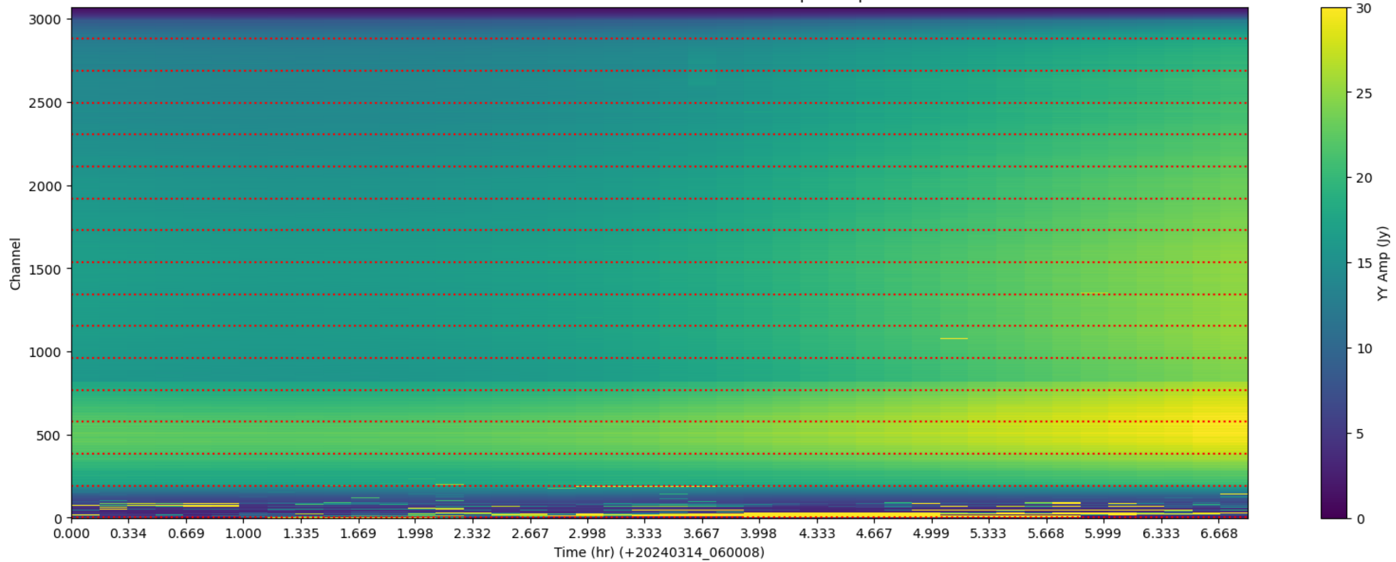
LWA059 - Correlator# 136 - YY - FLAGS: BadSpecShape
