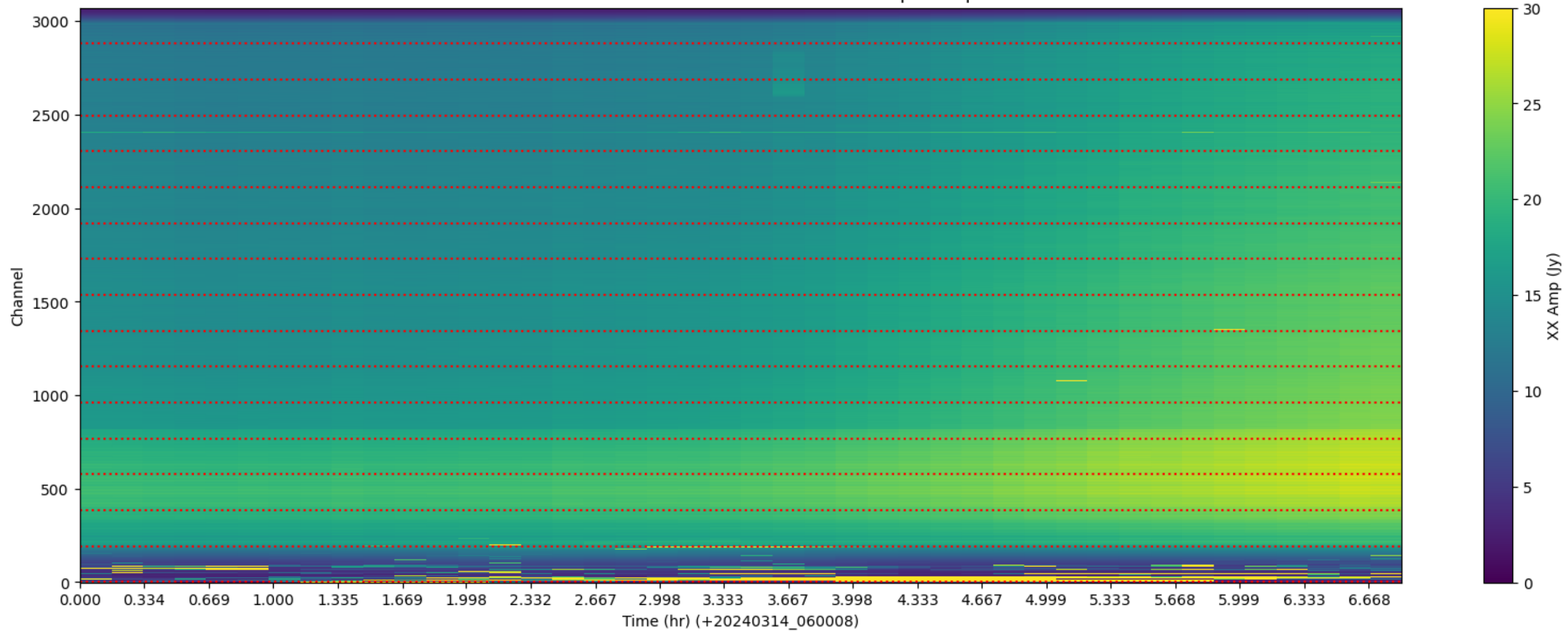
LWA224 - Correlator# 248 - XX - FLAGS: BadSpecShape
