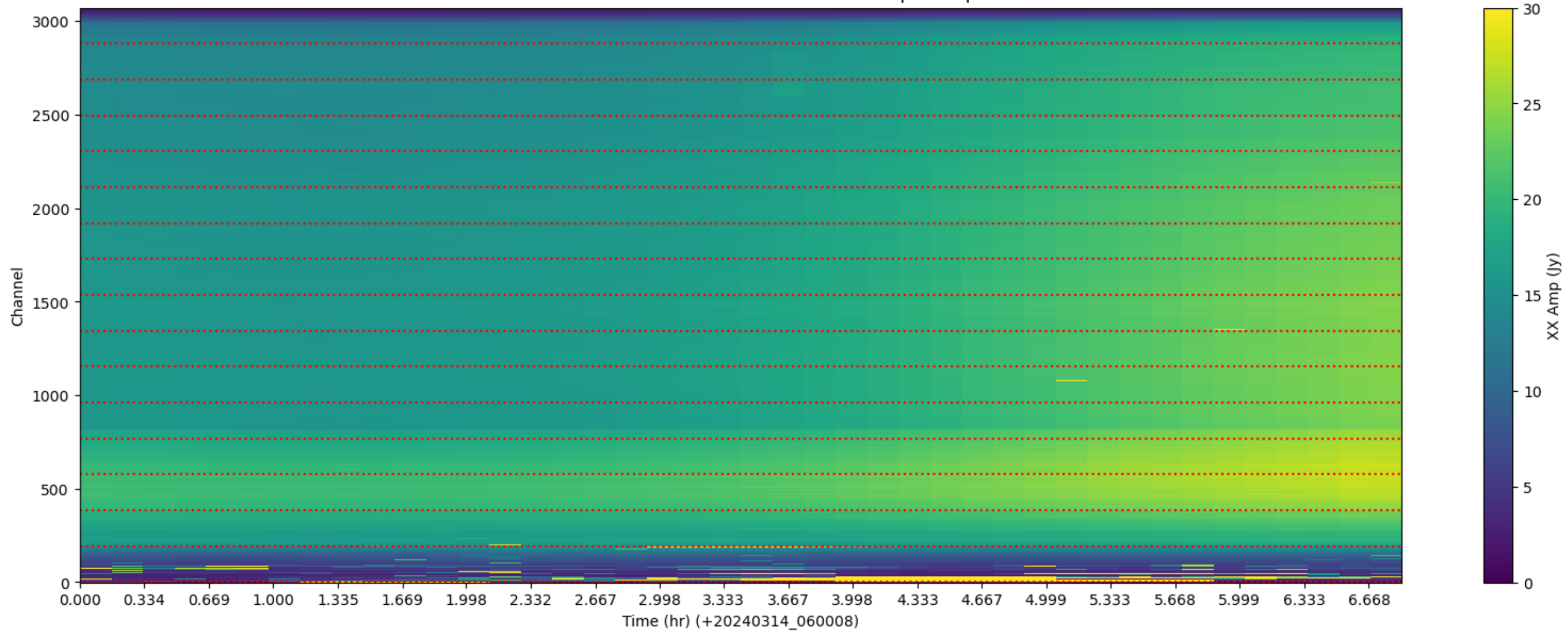
LWA089 - Correlator# 144 - XX - FLAGS: BadSpecShape
