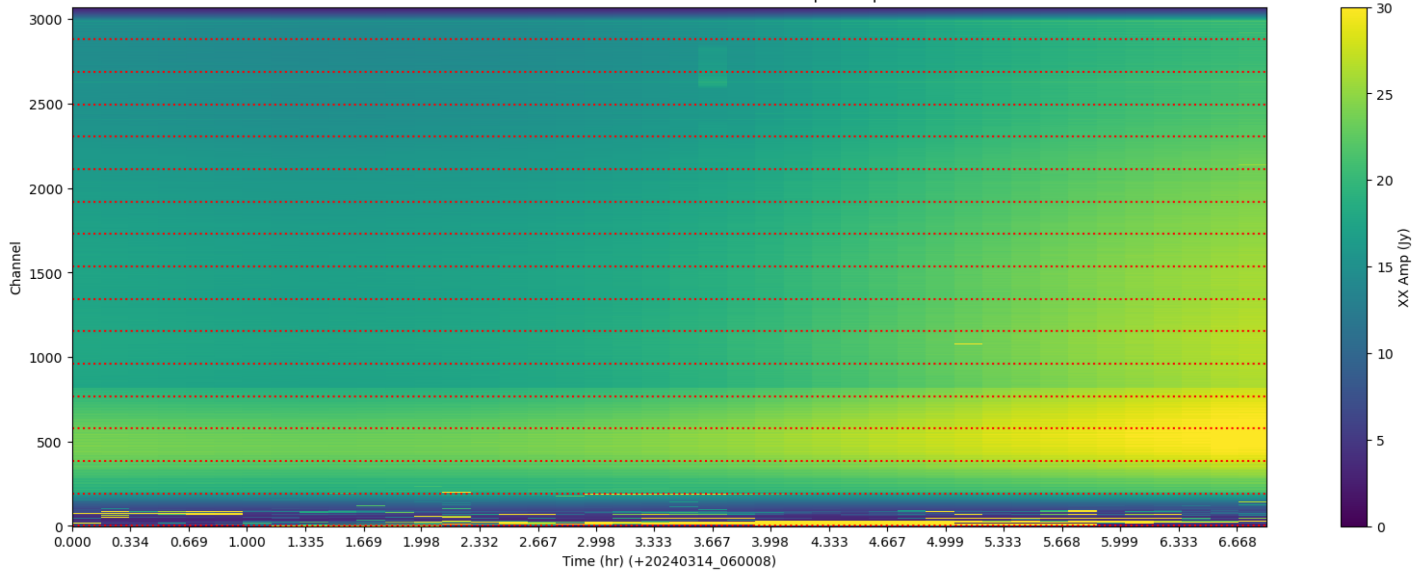
LWA057 - Correlator# 134 - XX - FLAGS: BadSpecShape
