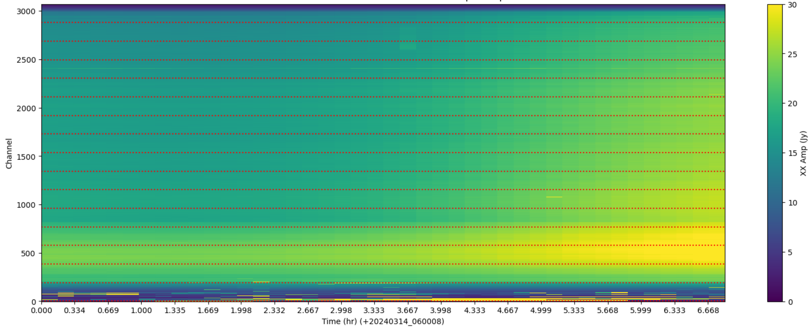
LWA126 - Correlator# 226 - XX - FLAGS: BadSpecShape
