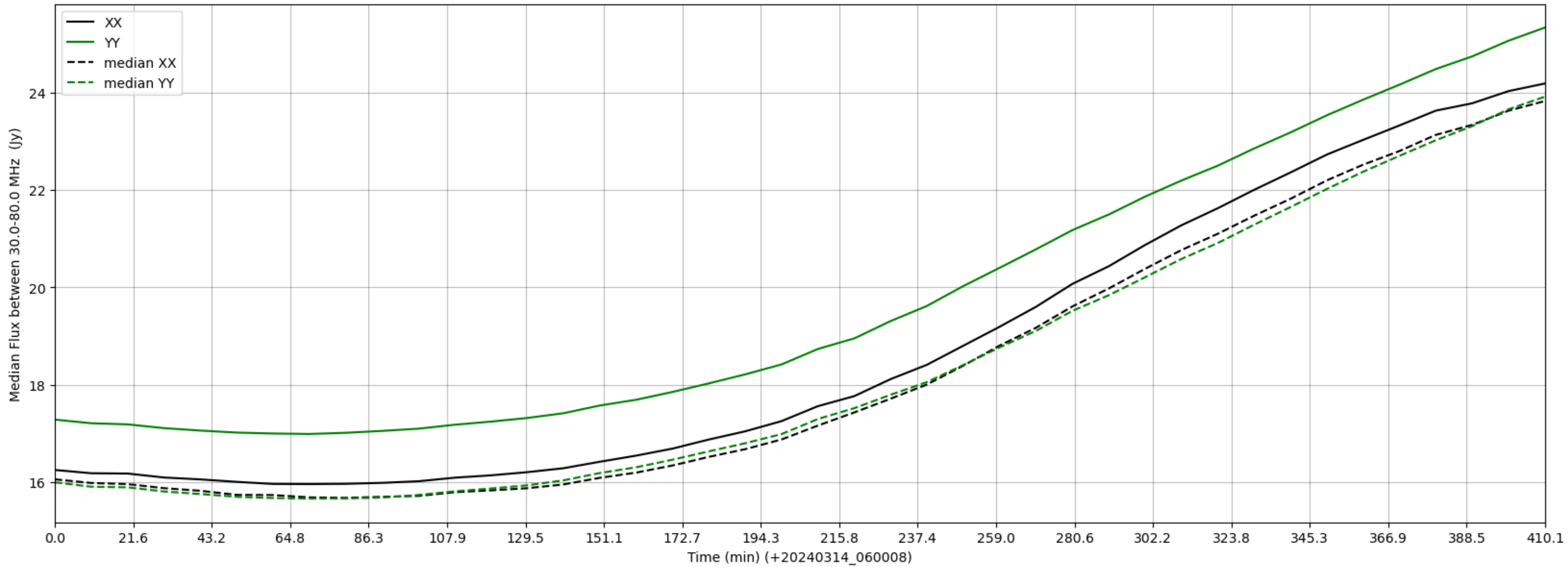
LWA122 - Correlator# 152 - XX FLAGS:BadSpecShape - YY FLAGS:BadSpecShape
