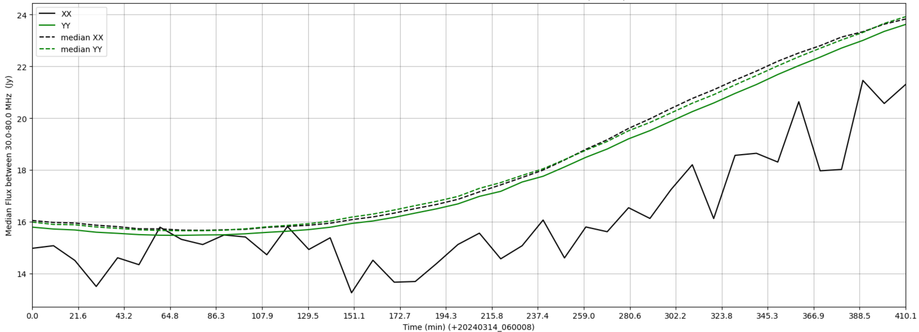
LWA052 - Correlator# 117 - XX FLAGS:Good - YY FLAGS:BadSpecShape
