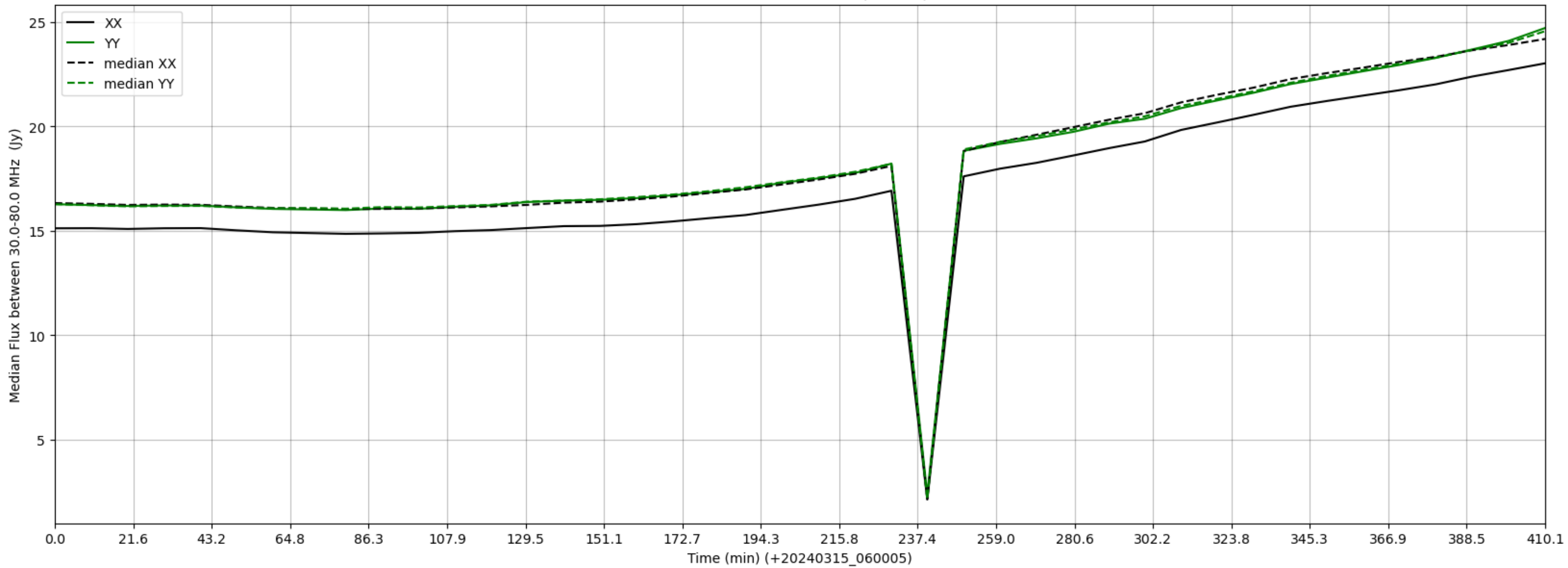
LWA233 - Correlator# 306 - XX FLAGS:BadSpecShape - YY FLAGS:Good
