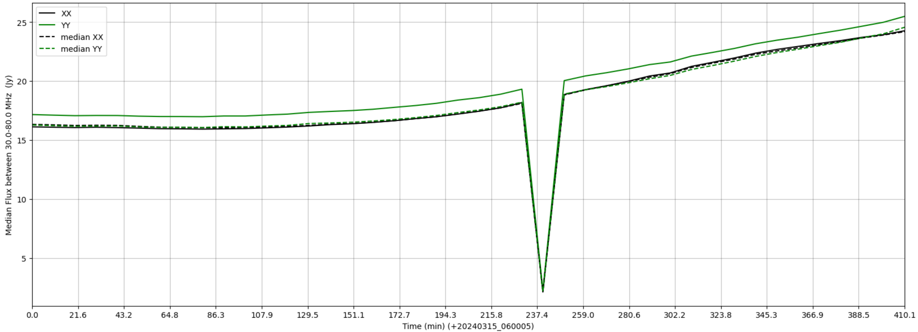
LWA122 - Correlator# 152 - XX FLAGS:Good - YY FLAGS:BadSpecShape
