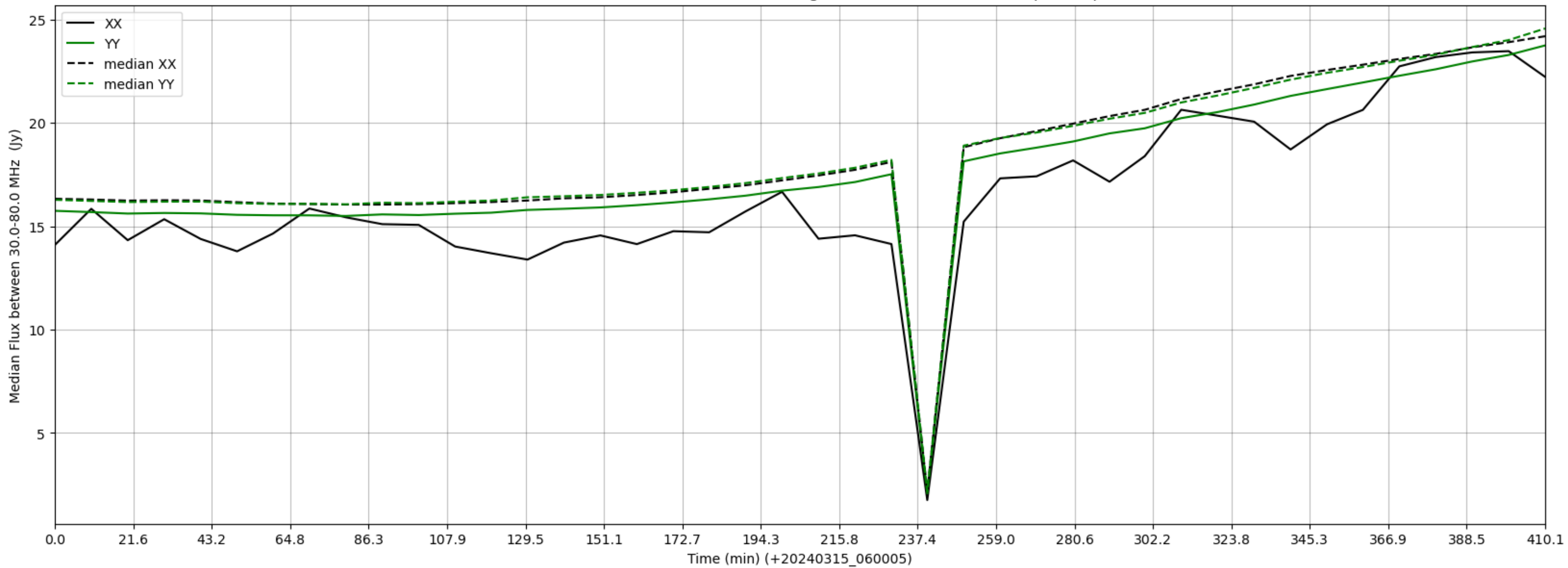
LWA052 - Correlator# 117 - XX FLAGS:HighTimeVar - YY FLAGS:BadSpecShape
