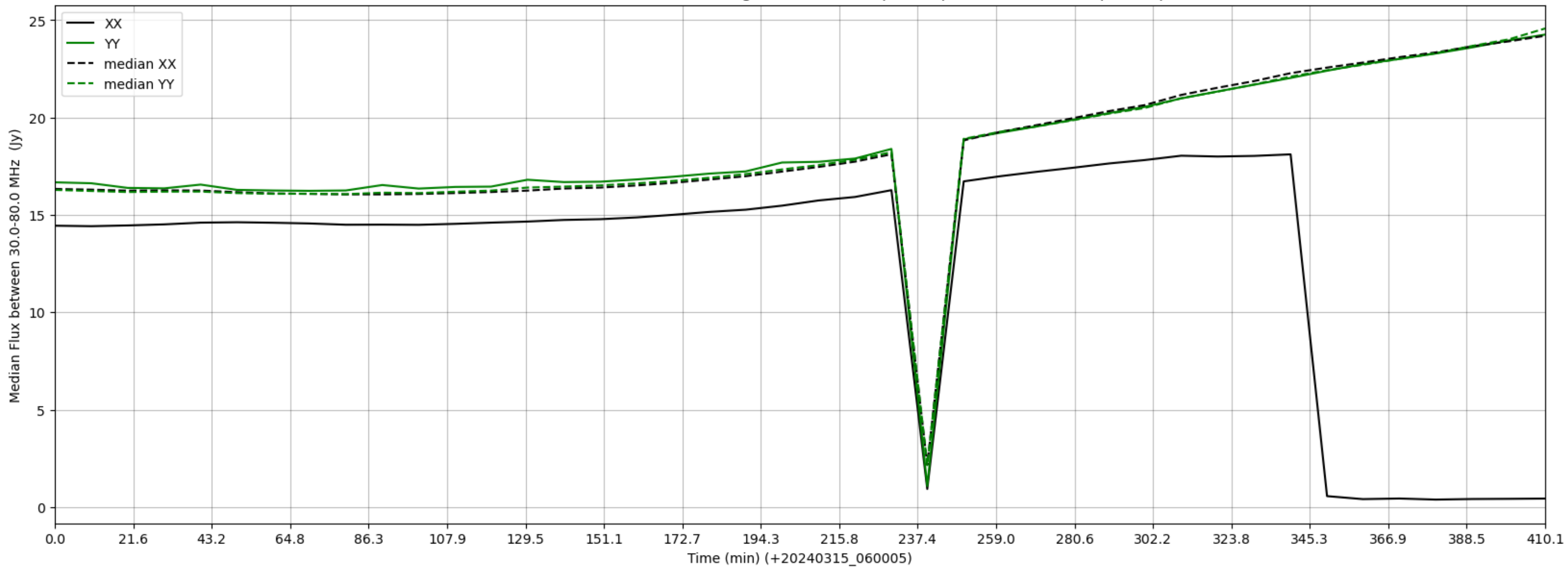
LWA353 - Correlator# 031 - XX FLAGS:HighTimeVar+BadSpecShape - YY FLAGS:BadSpecShape
