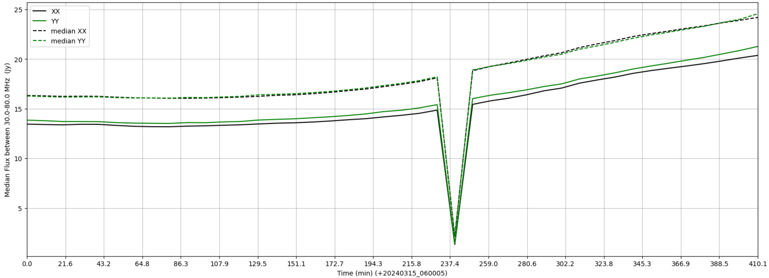
LWA337 - Correlator# 059 - XX FLAGS:BadSpecShape - YY FLAGS:BadSpecShape
