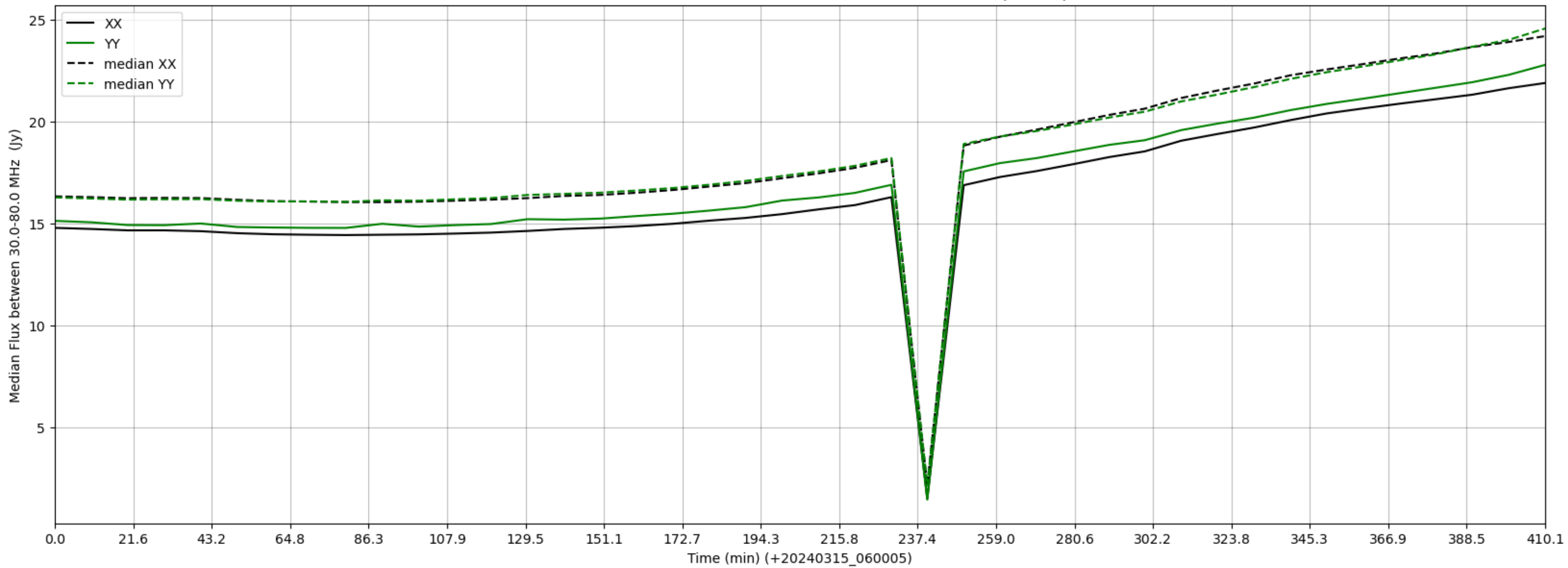
LWA320 - Correlator# 054 - XX FLAGS:Good - YY FLAGS:BadSpecShape
