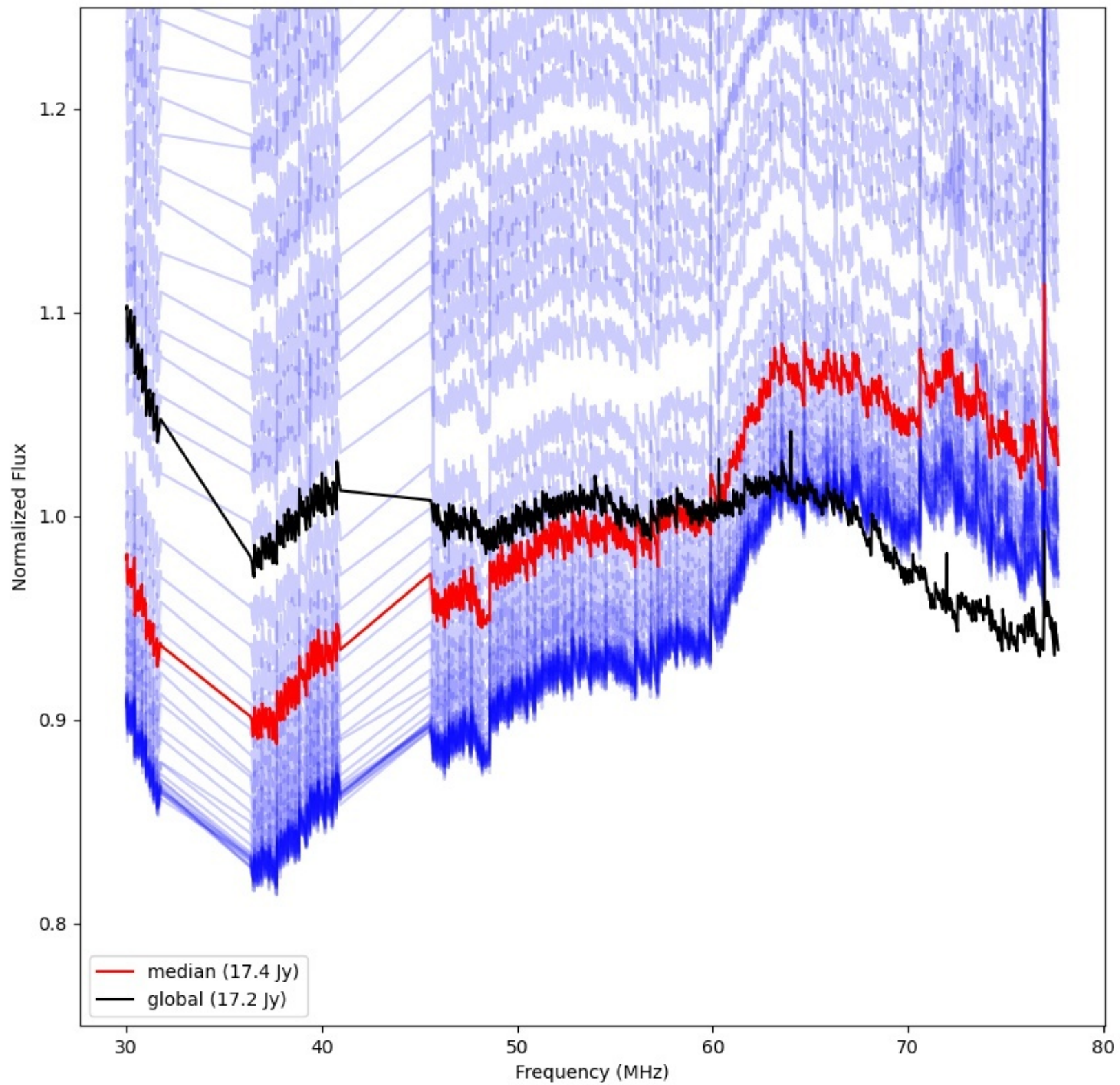
LWA130 - Correlator# 183 - YY - FLAGS:Good
