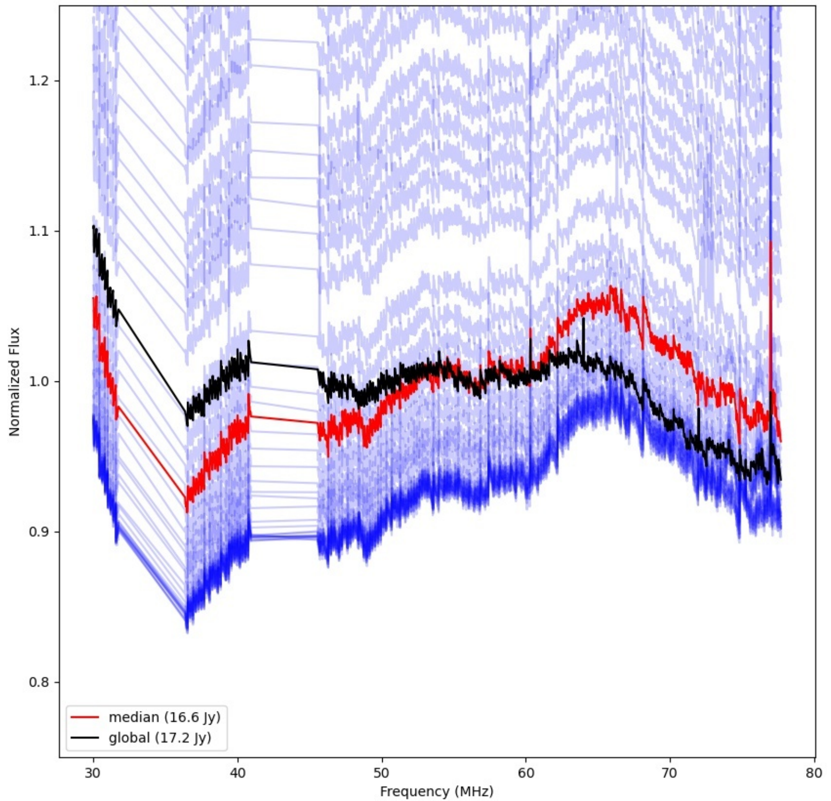
LWA210 - Correlator# 300 - YY - FLAGS:Good
