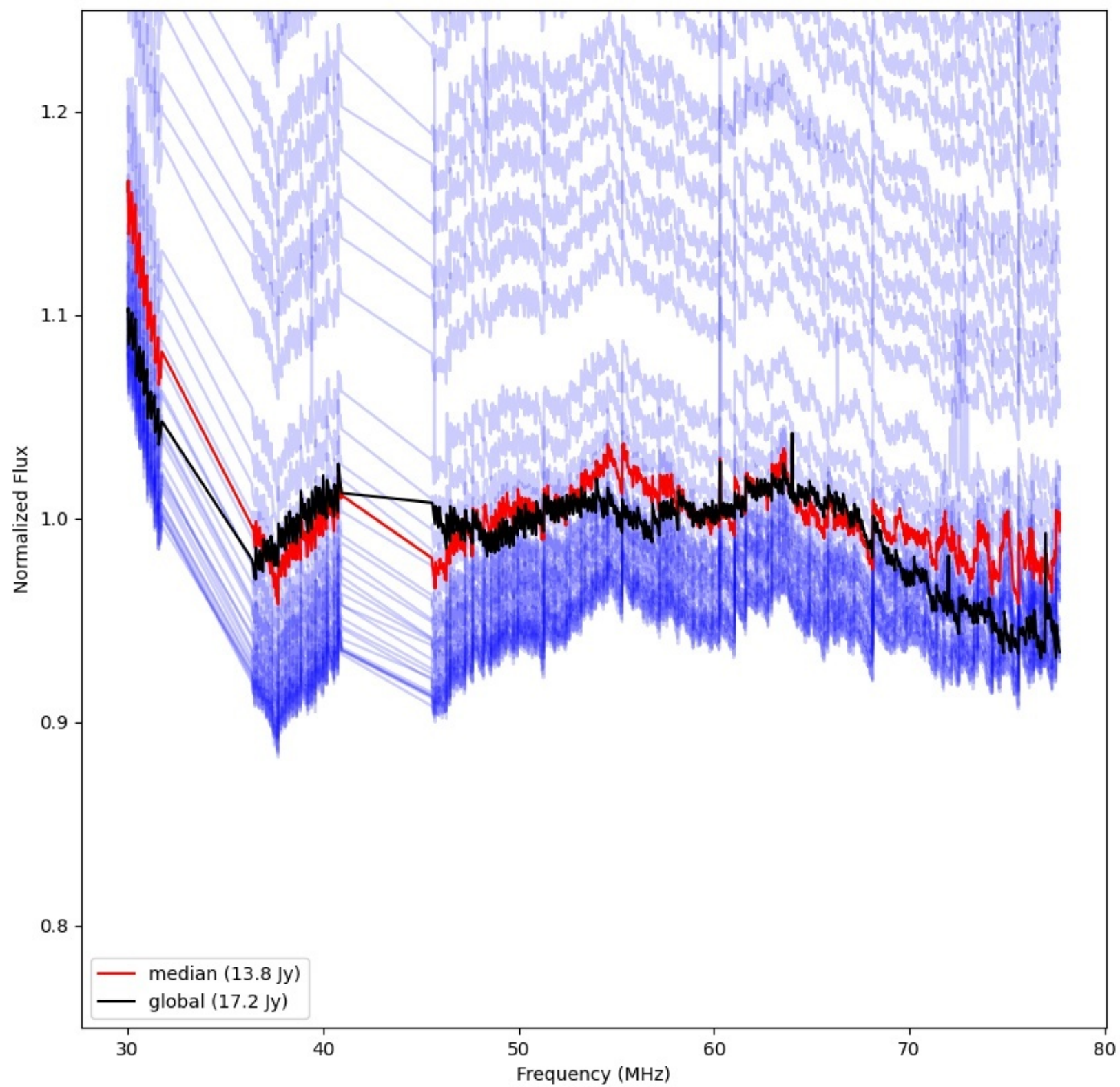
LWA294 - Correlator# 188 - YY - FLAGS:Good
