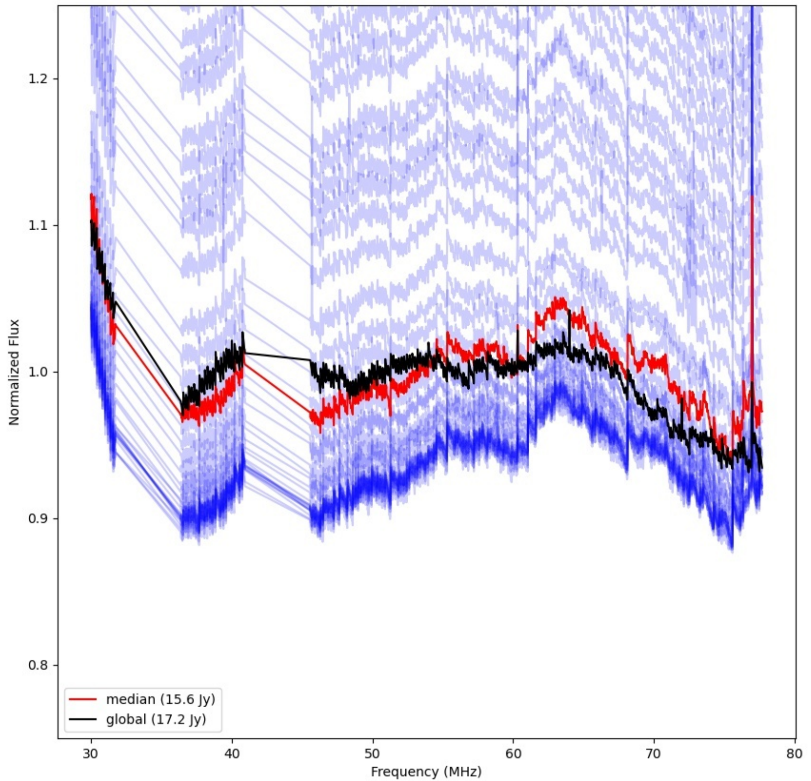
LWA310 - Correlator# 017 - YY - FLAGS:Good
