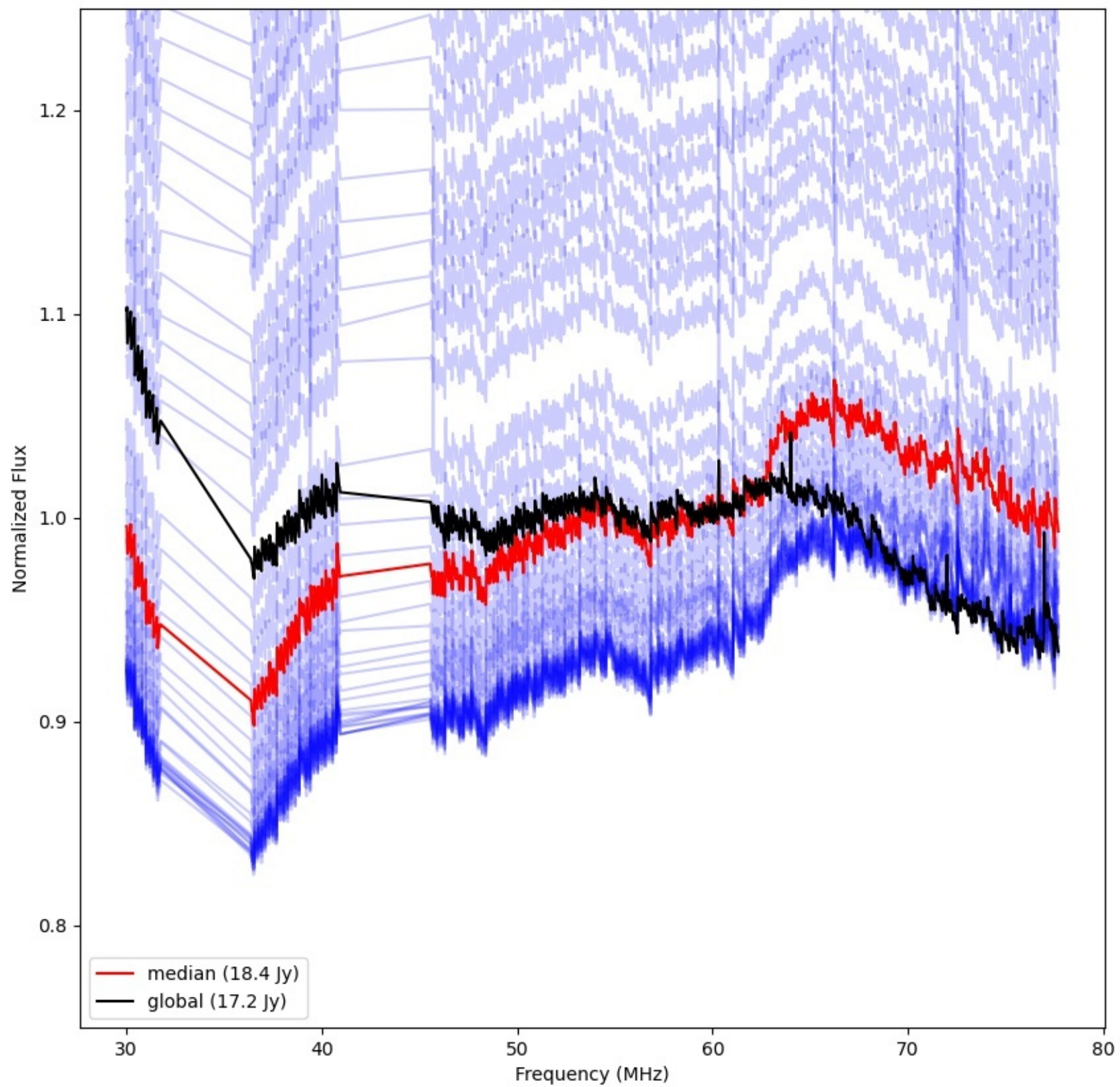
LWA134 - Correlator# 184 - YY - FLAGS:Good
