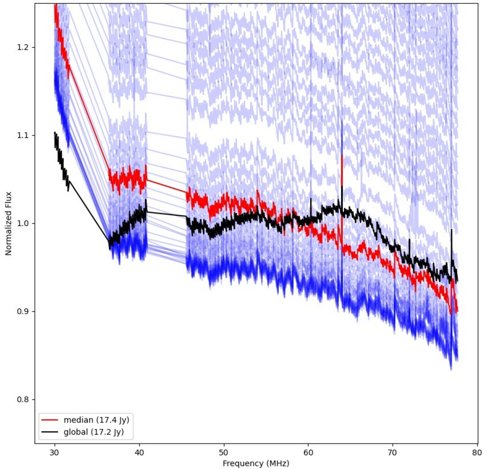
LWA026 - Correlator# 108 - YY - FLAGS:Good
