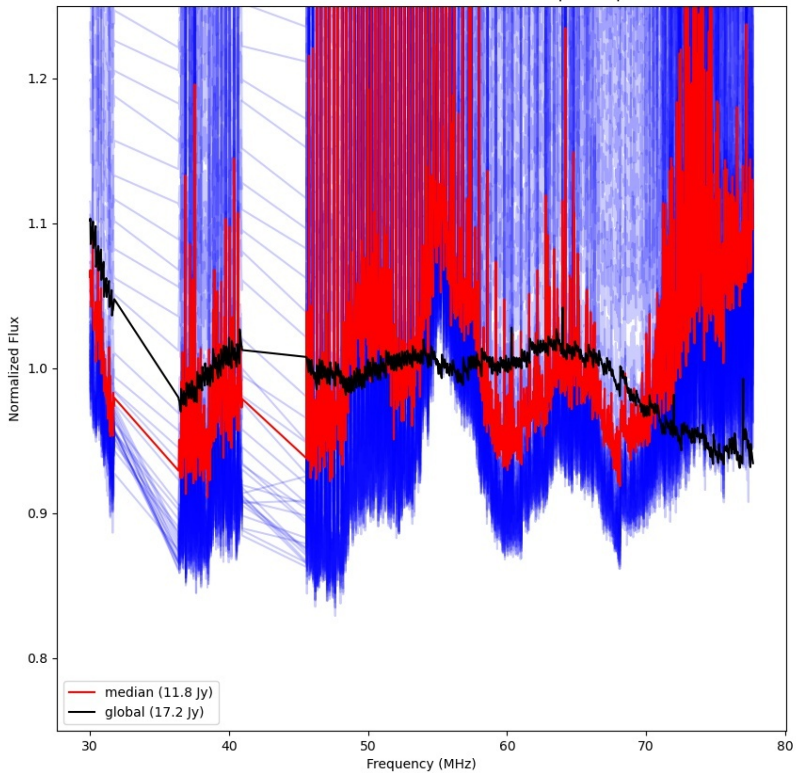
LWA302 - Correlator# 092 - YY - FLAGS:BadSpecShape
