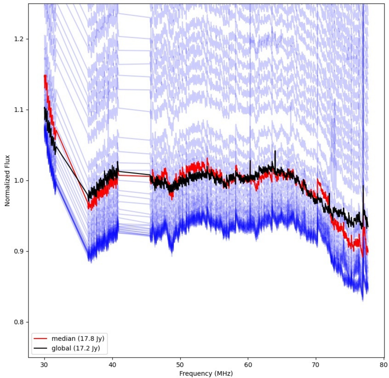
LWA211 - Correlator# 327 - YY - FLAGS:Good
