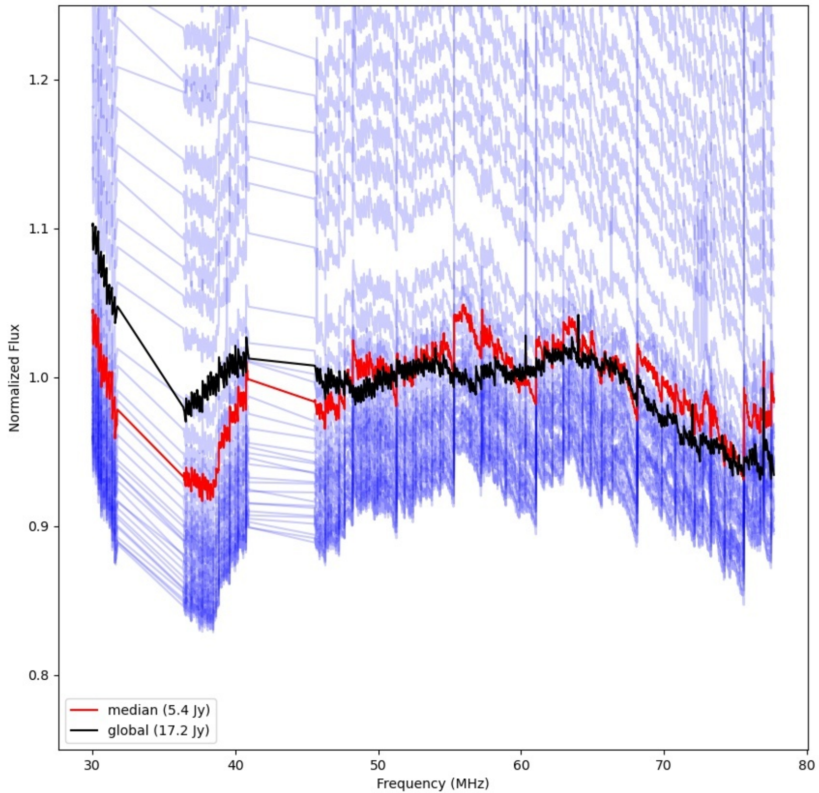
LWA303 - Correlator# 051 - YY - FLAGS:Good
