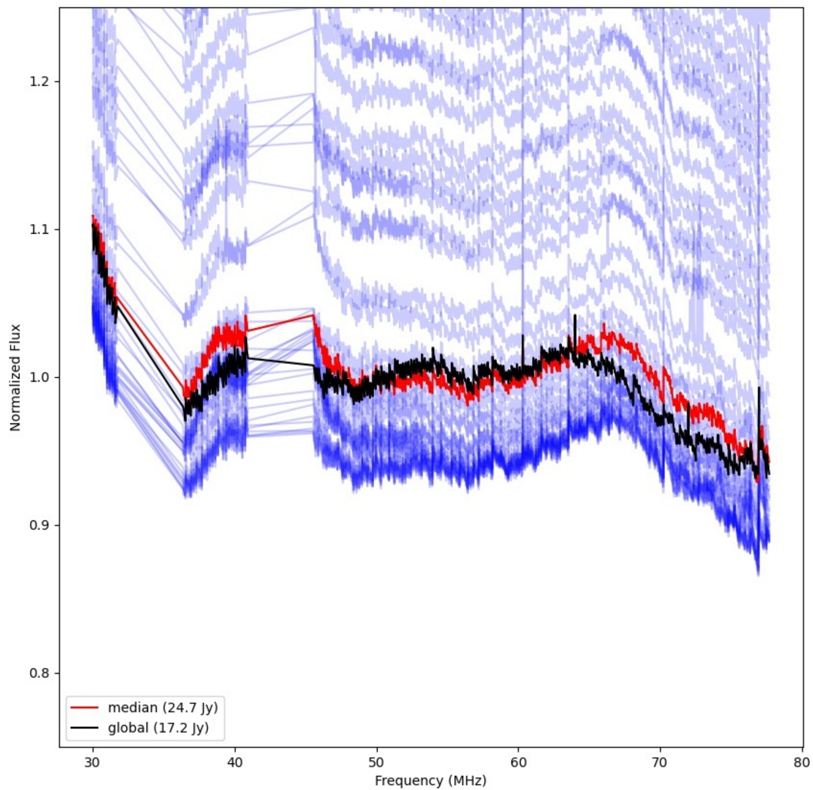
LWA178 - Correlator# 221 - YY - FLAGS:Good
