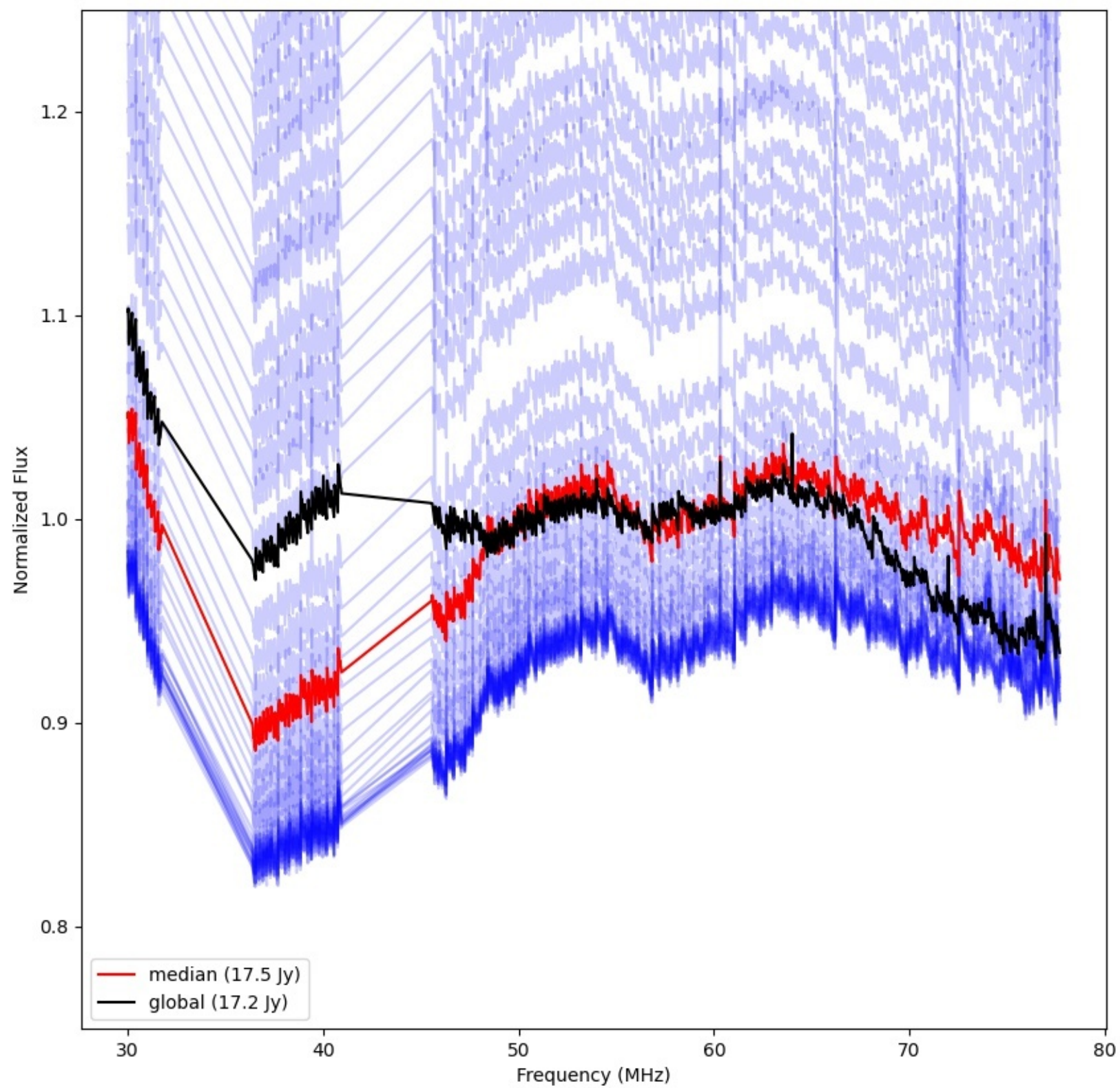
LWA135 - Correlator# 256 - YY - FLAGS:Good
