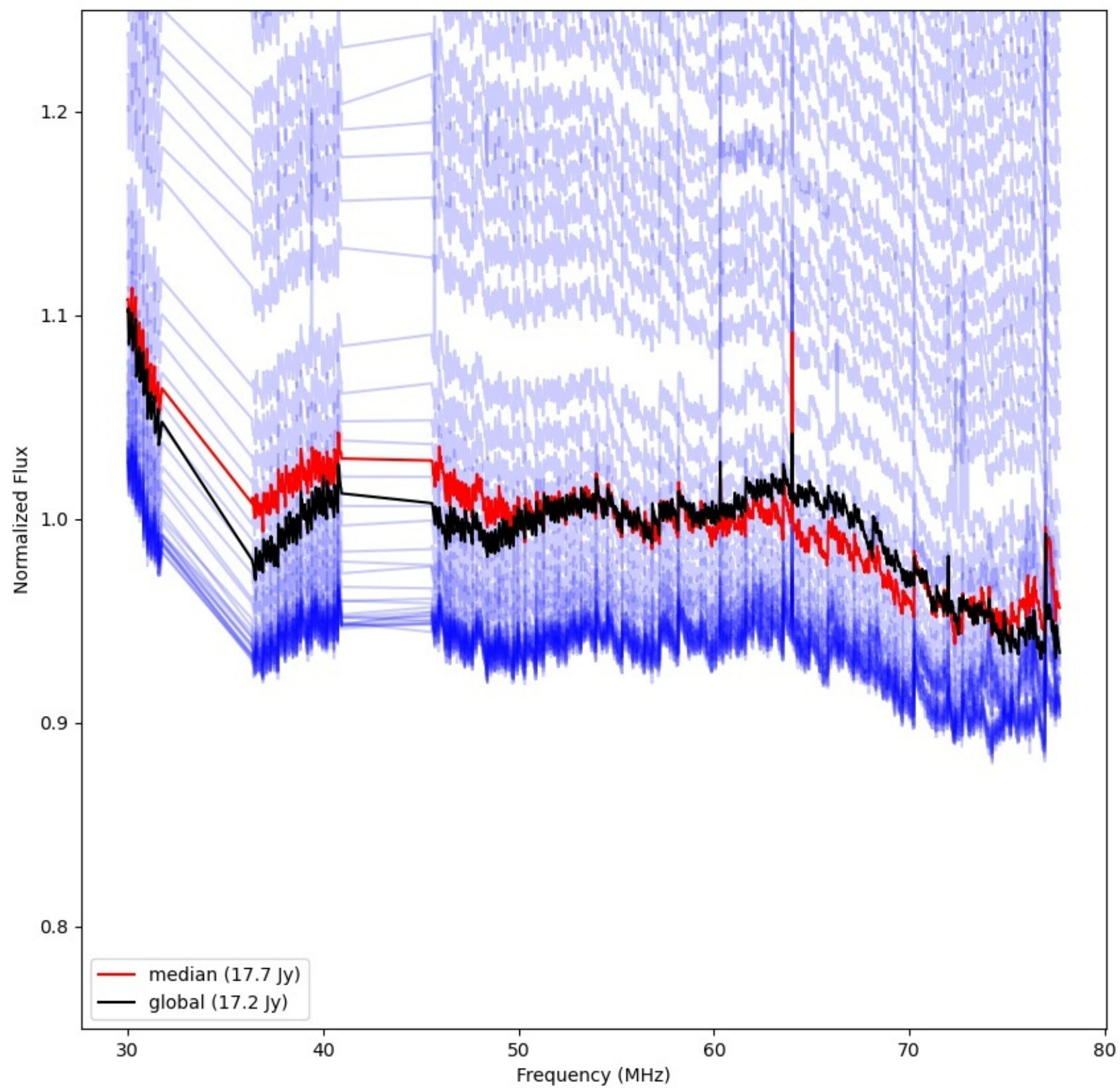
LWA055 - Correlator# 121 - YY - FLAGS:Good
