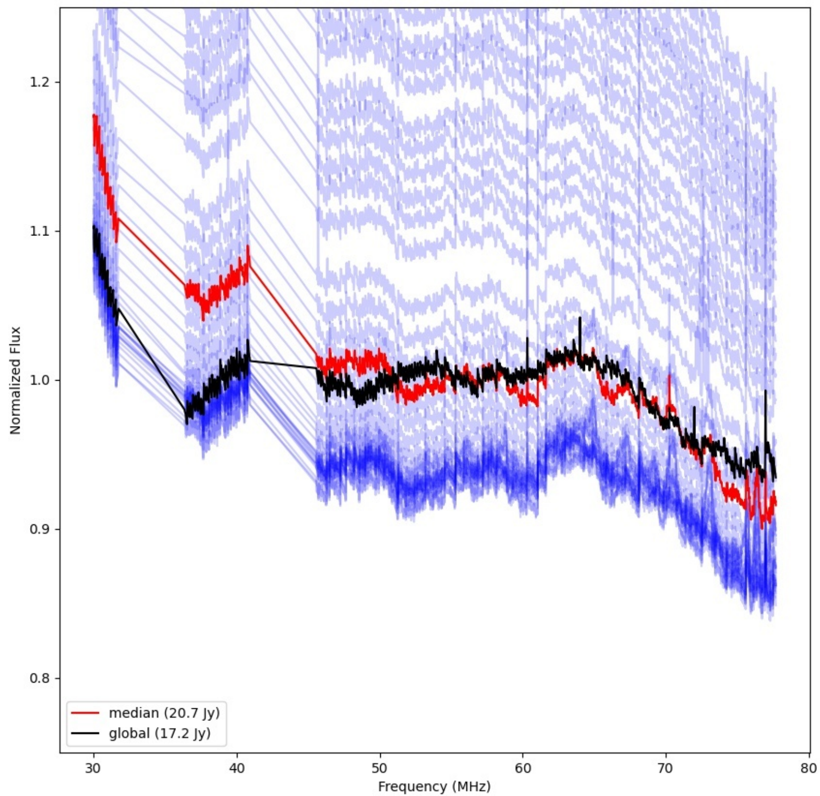
LWA316 - Correlator# 155 - YY - FLAGS:Good
