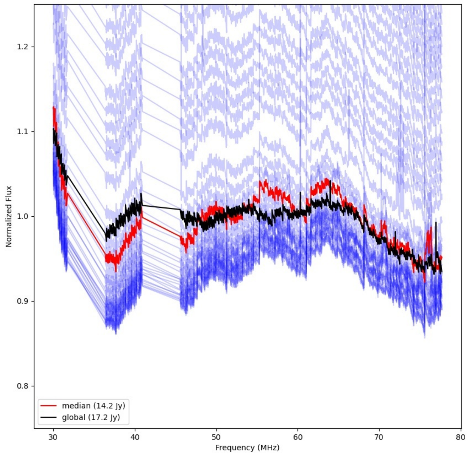
LWA335 - Correlator# 057 - YY - FLAGS:Good
