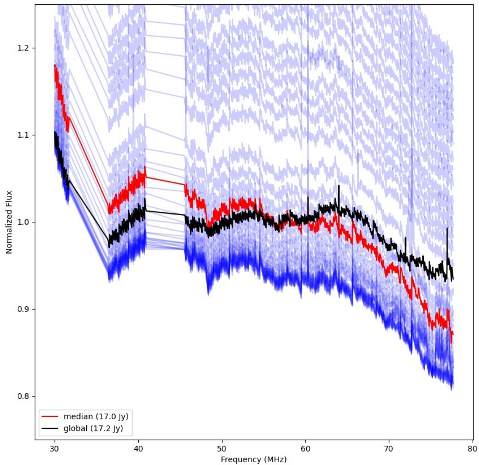
LWA183 - Correlator# 324 - YY - FLAGS:Good
