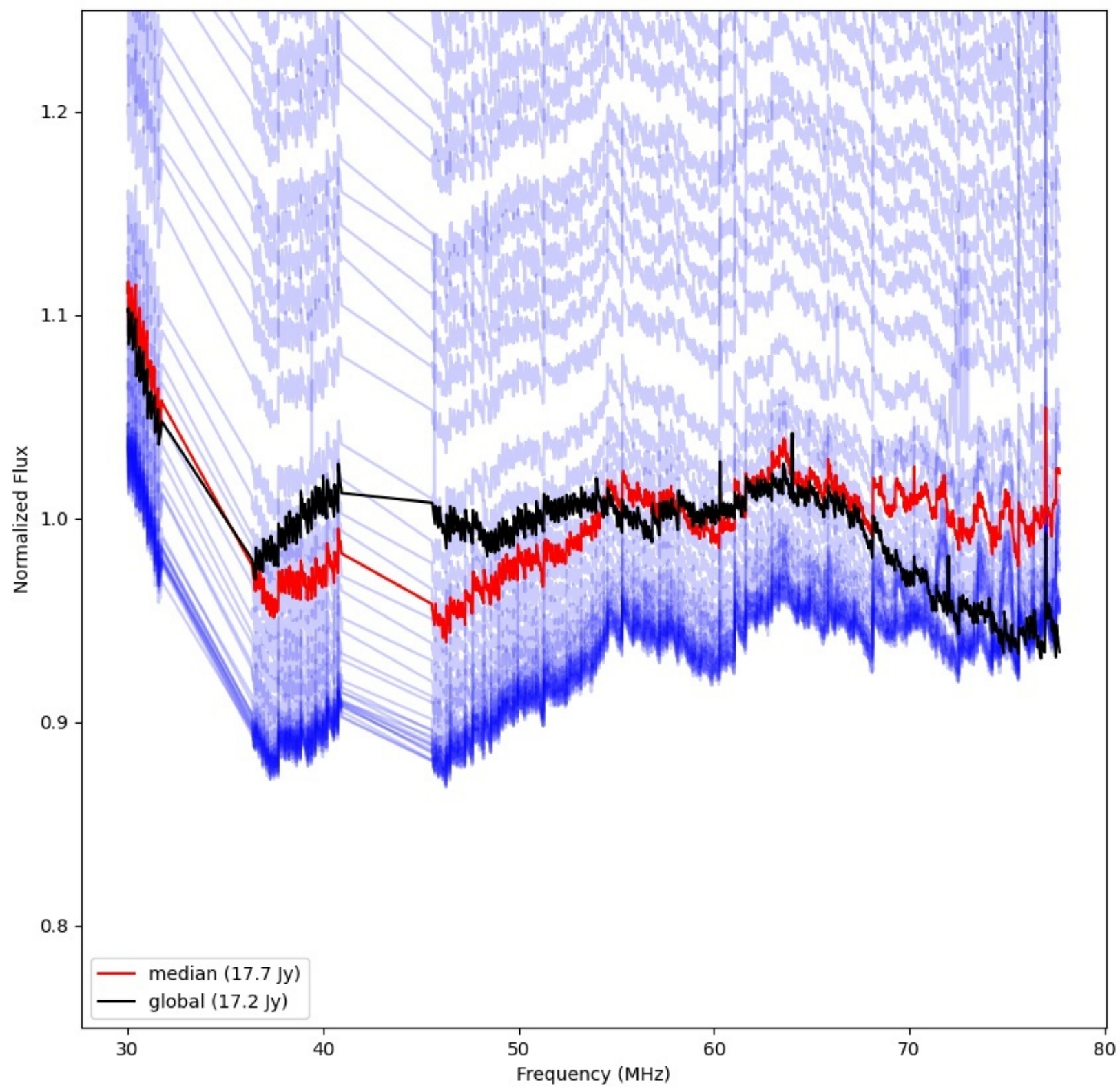
LWA327 - Correlator# 023 - YY - FLAGS:Good
