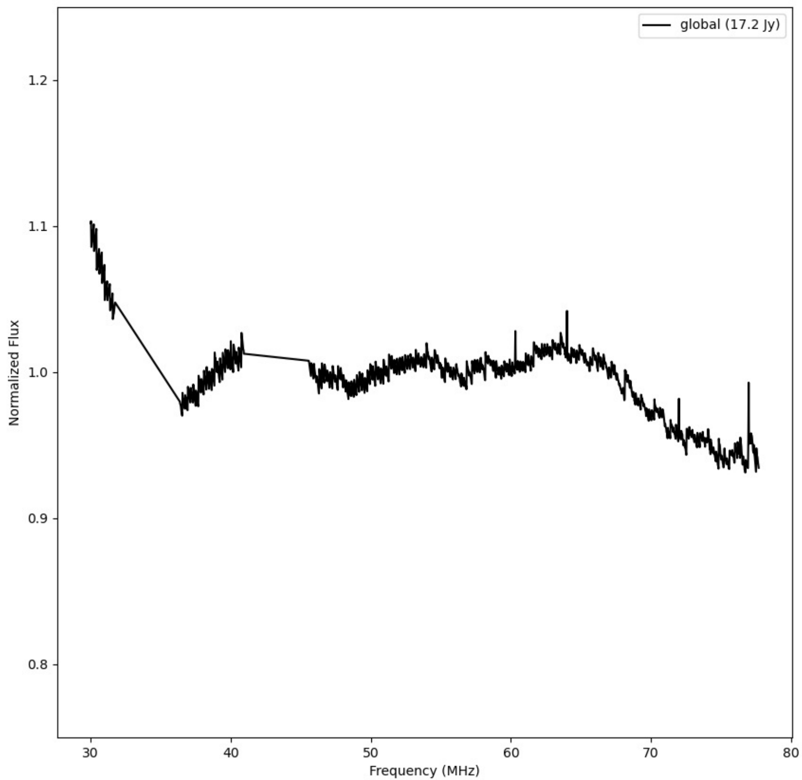
LWA150 - Correlator# 215 - YY - FLAGS:LowFlux
