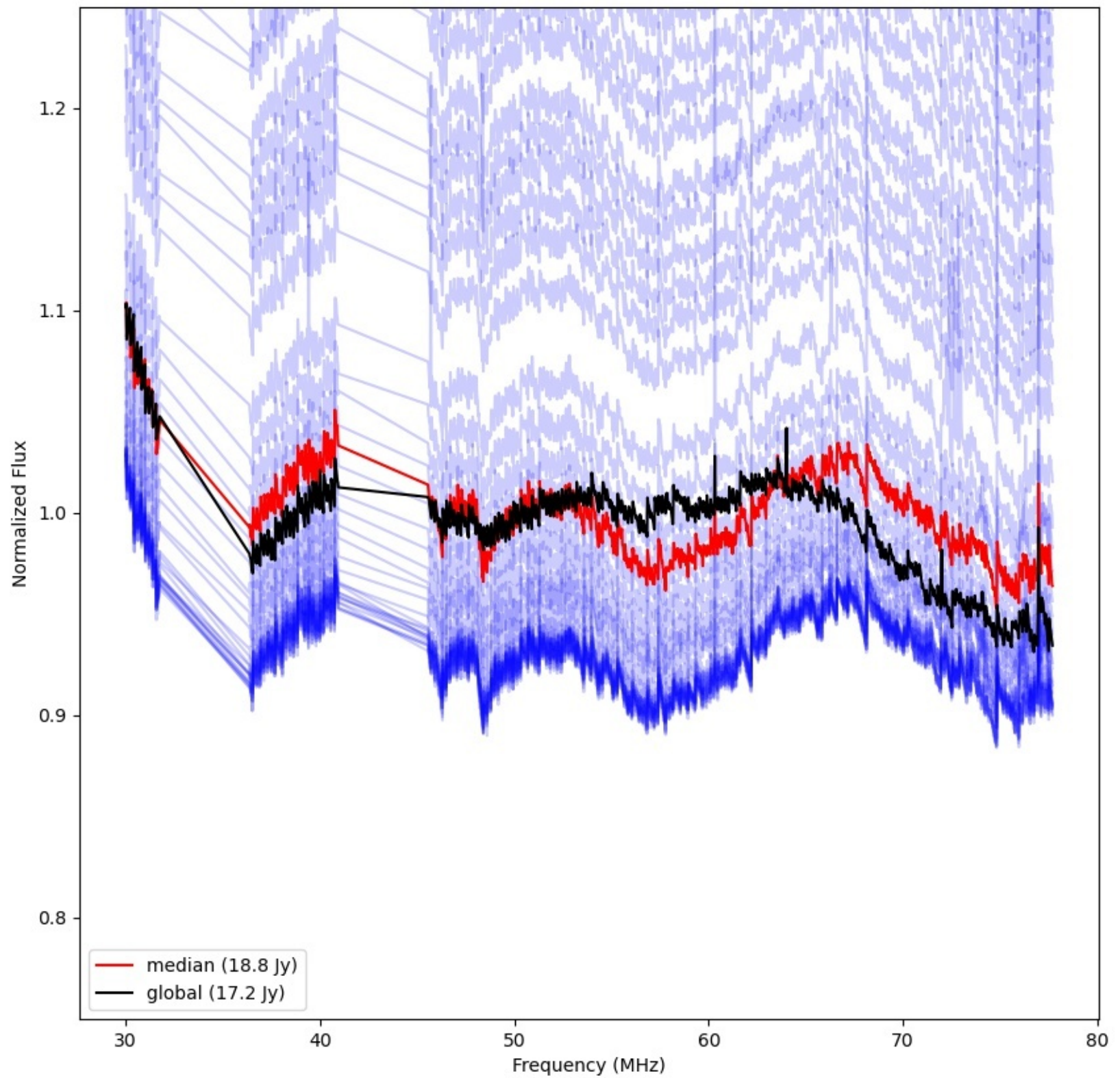
LWA167 - Correlator# 268 - YY - FLAGS:Good
