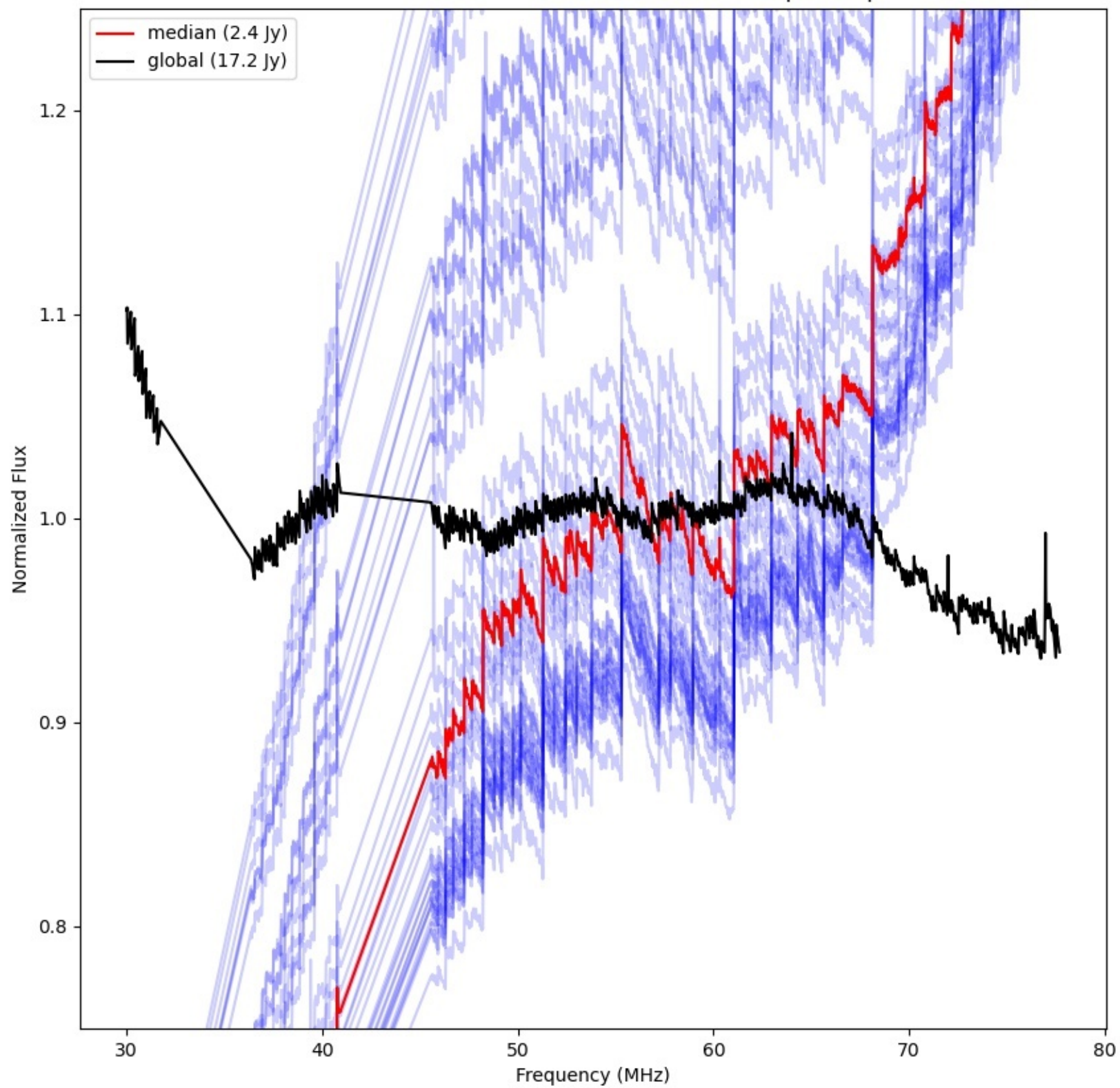
LWA307 - Correlator# 012 - YY - FLAGS:BadSpecShape
