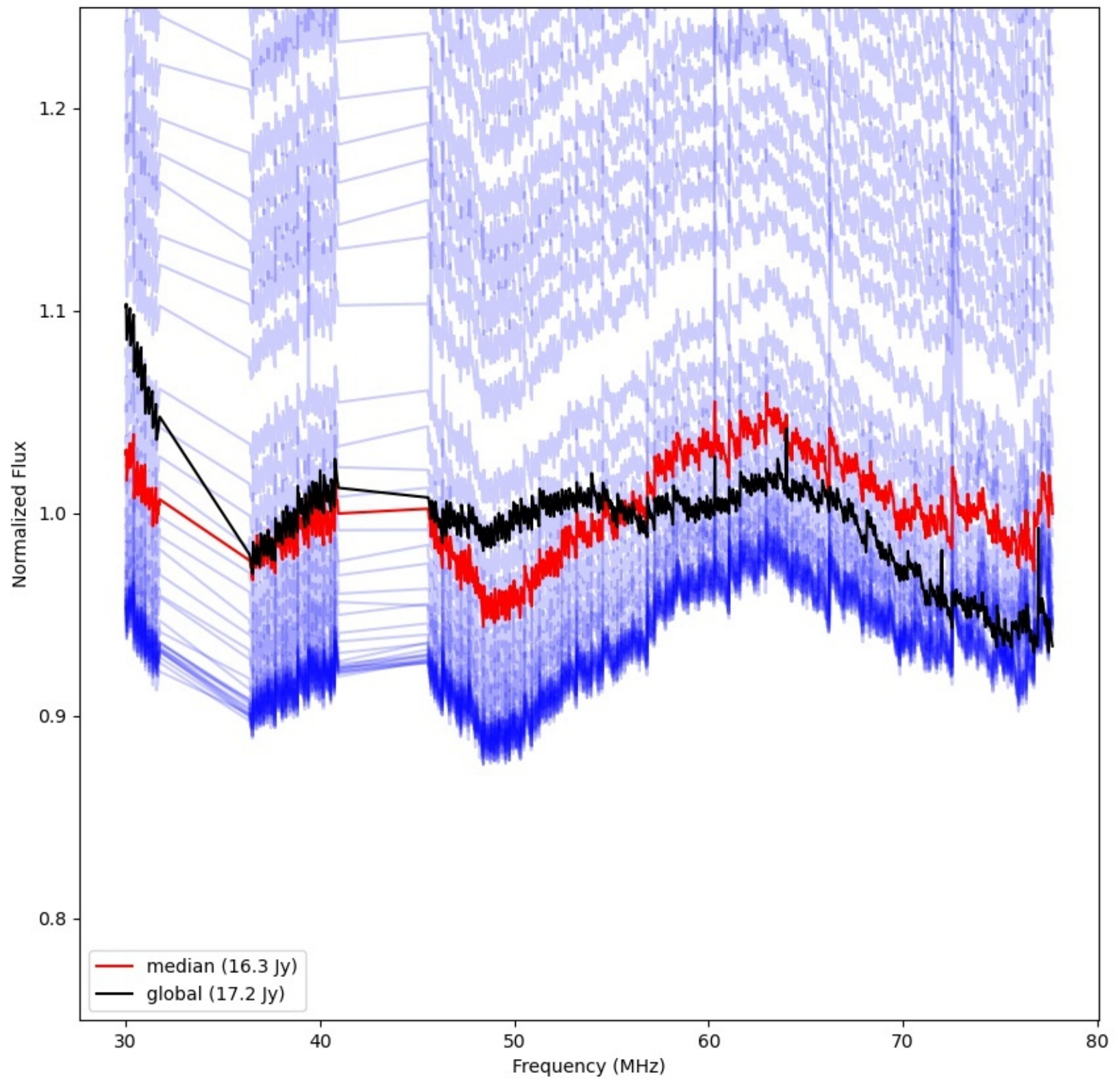
LWA010 - Correlator# 073 - YY - FLAGS:Good
