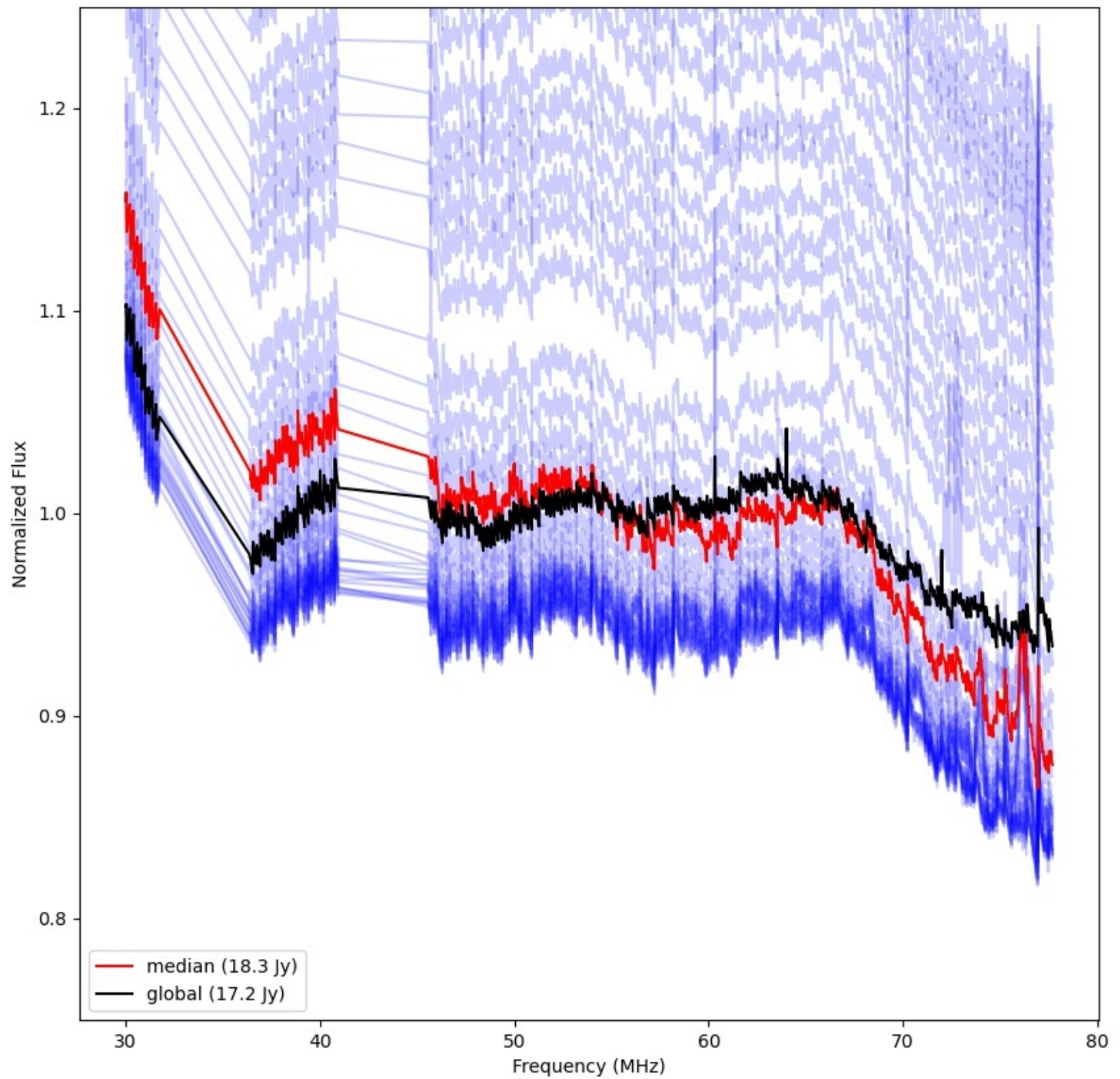
LWA256 - Correlator# 347 - YY - FLAGS:Good
