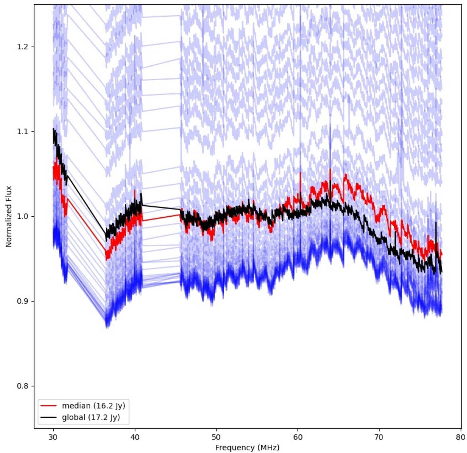
LWA157 - Correlator# 234 - YY - FLAGS:Good
