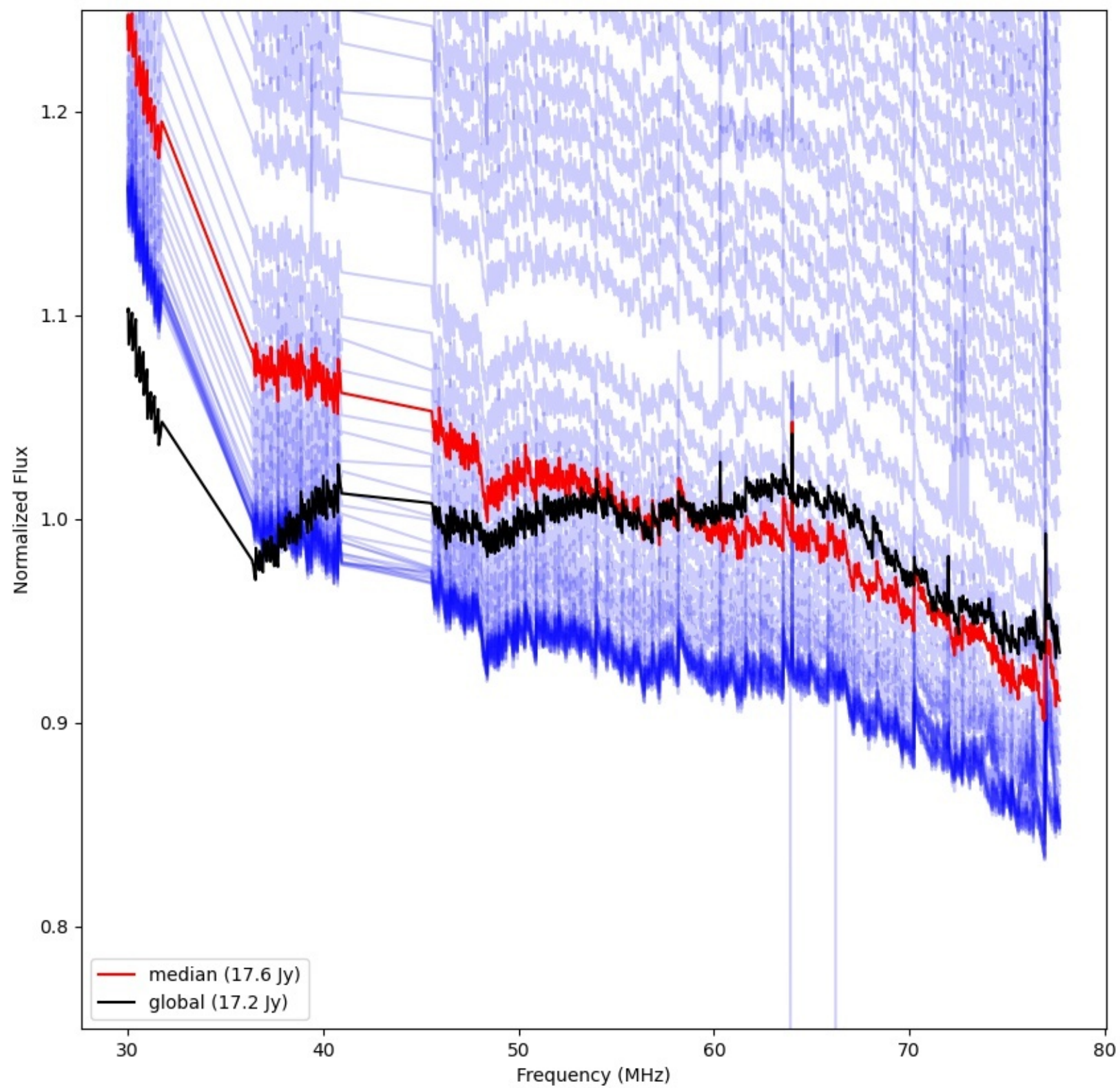
LWA024 - Correlator# 106 - YY - FLAGS:Good
