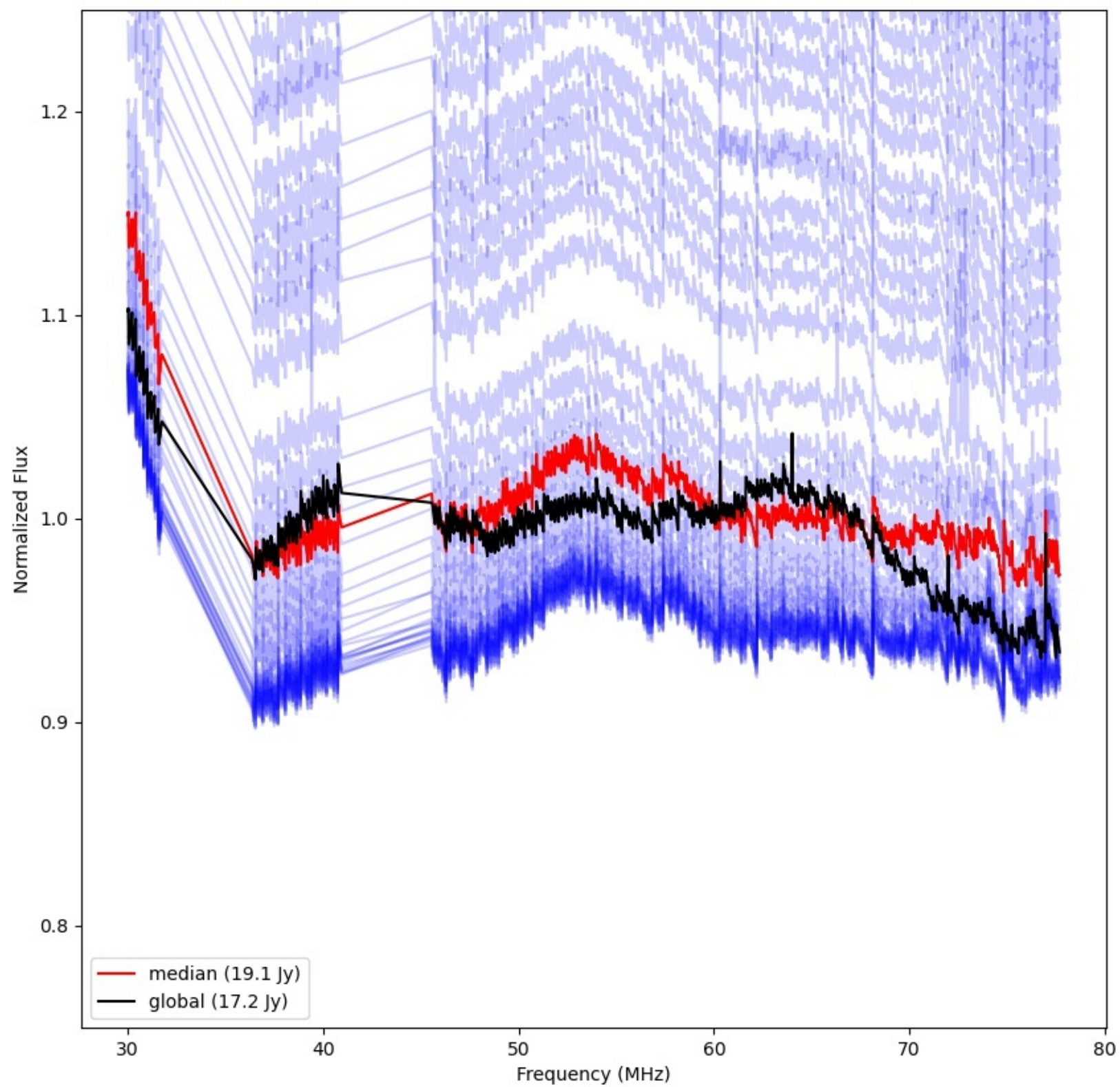
LWA140 - Correlator# 260 - YY - FLAGS:Good
