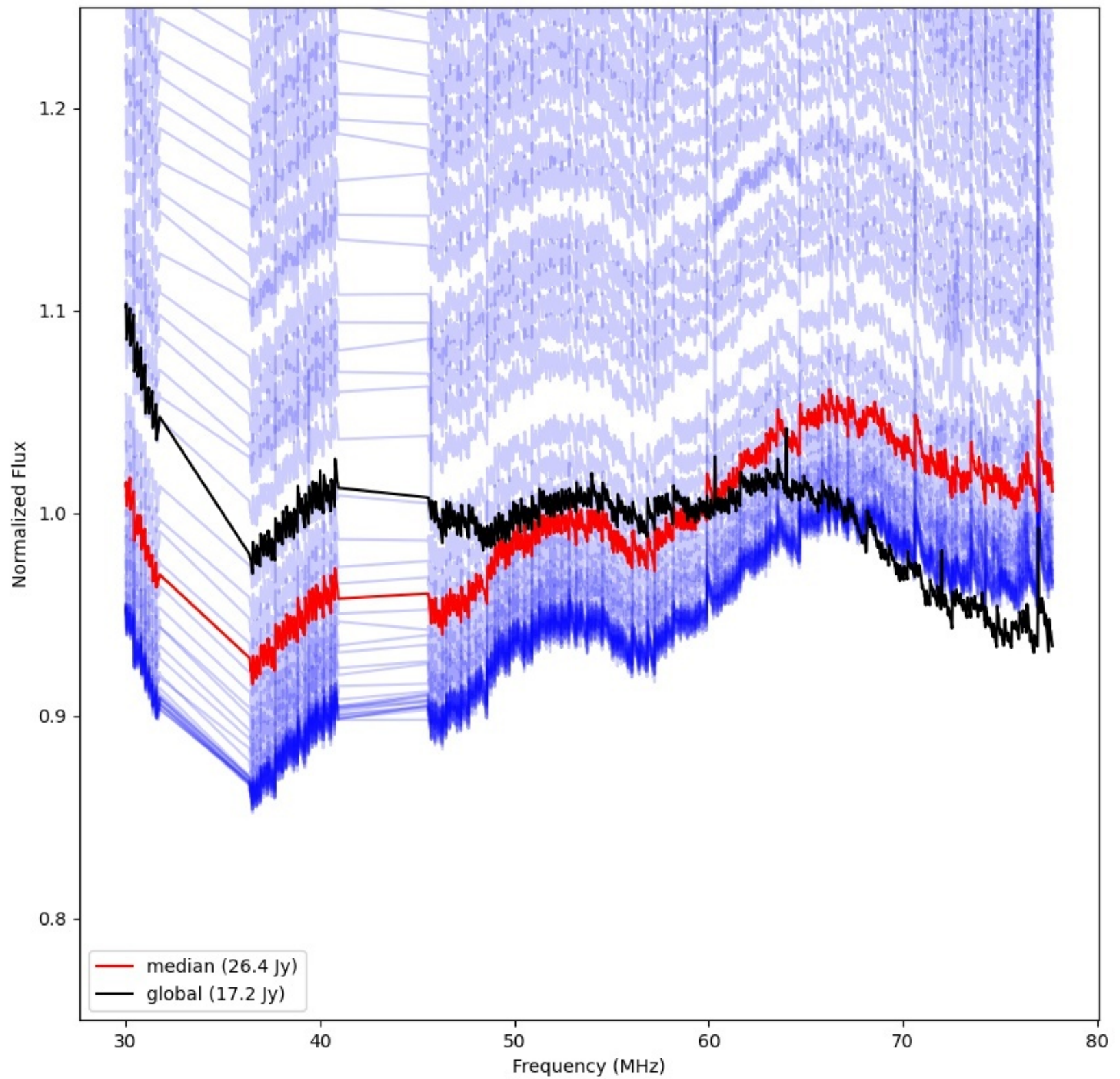
LWA195 - Correlator# 272 - YY - FLAGS:Good
