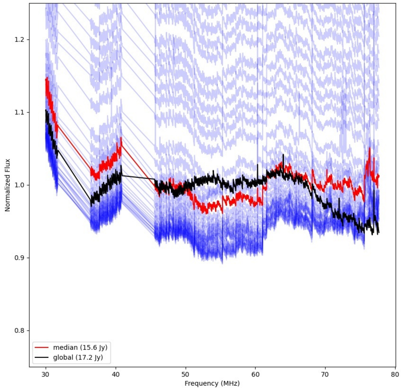
LWA306 - Correlator# 053 - YY - FLAGS:Good
