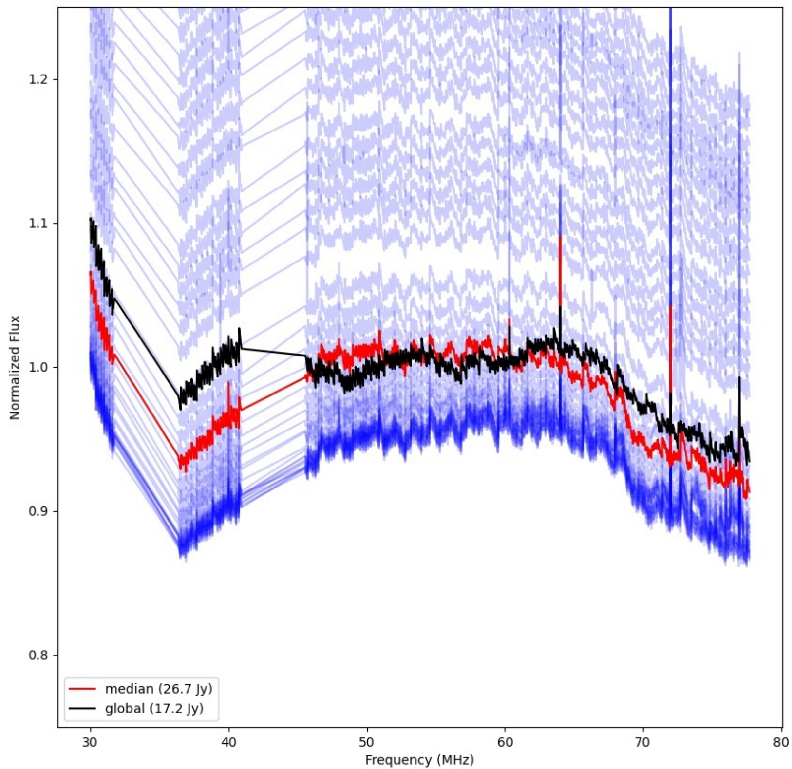
LWA222 - Correlator# 249 - YY - FLAGS:Good
