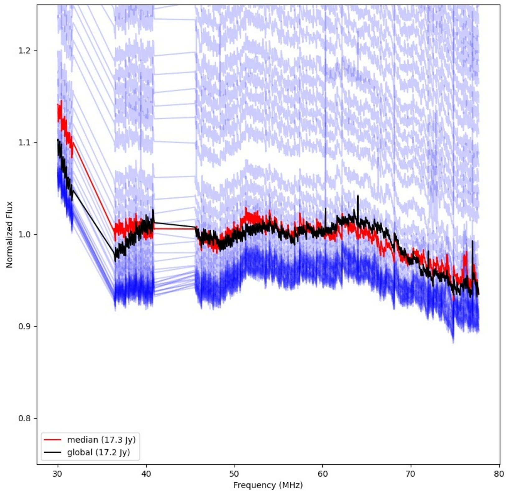
LWA018 - Correlator# 100 - YY - FLAGS:Good
