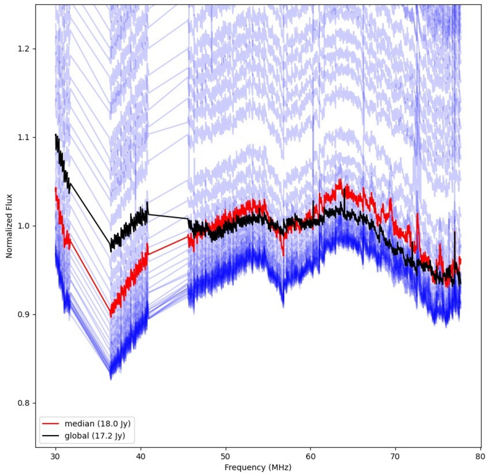
LWA252 - Correlator# 186 - YY - FLAGS:Good
