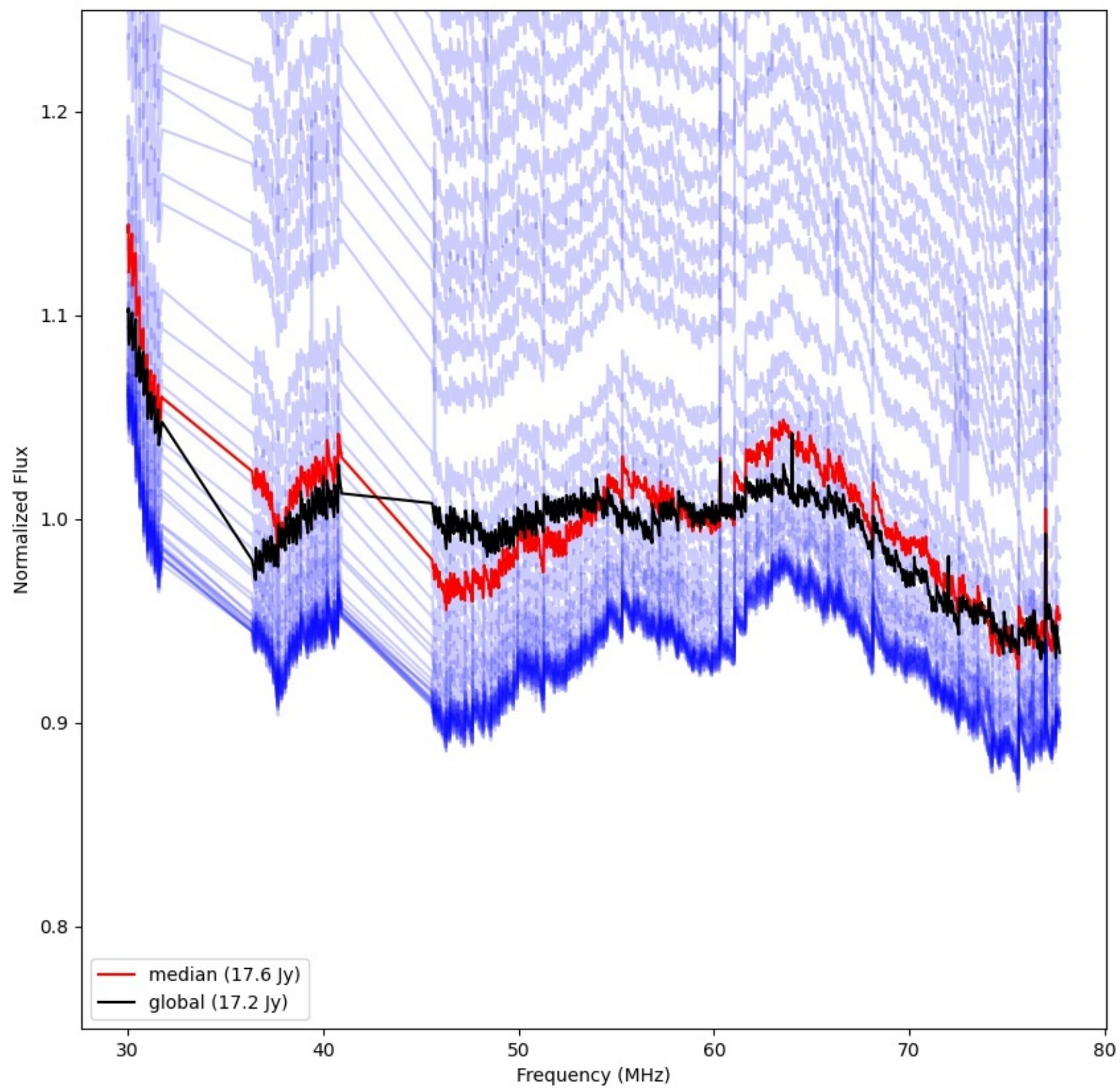
LWA300 - Correlator# 348 - YY - FLAGS:Good
