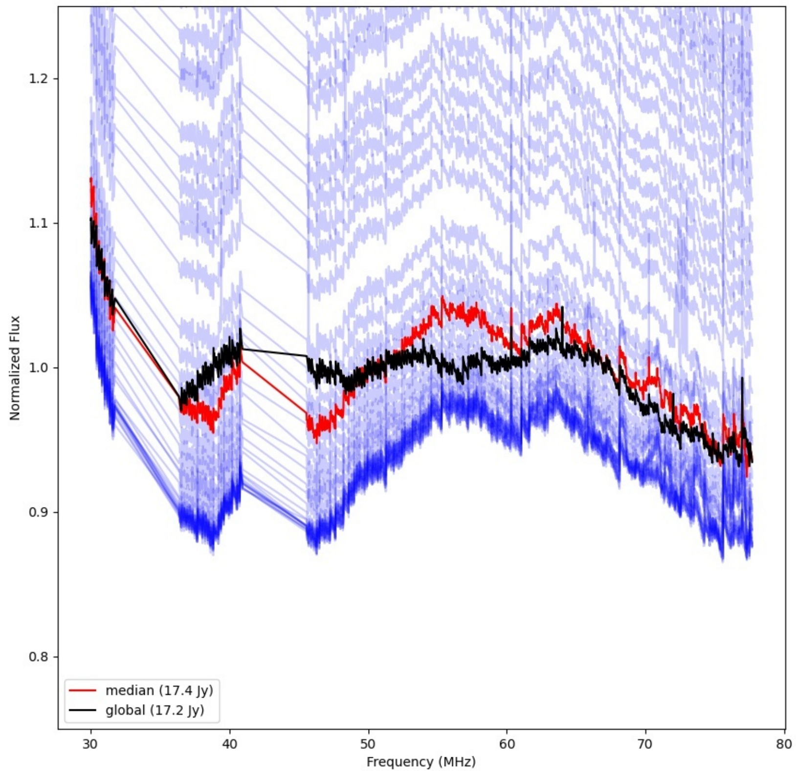
LWA344 - Correlator# 061 - YY - FLAGS:Good
