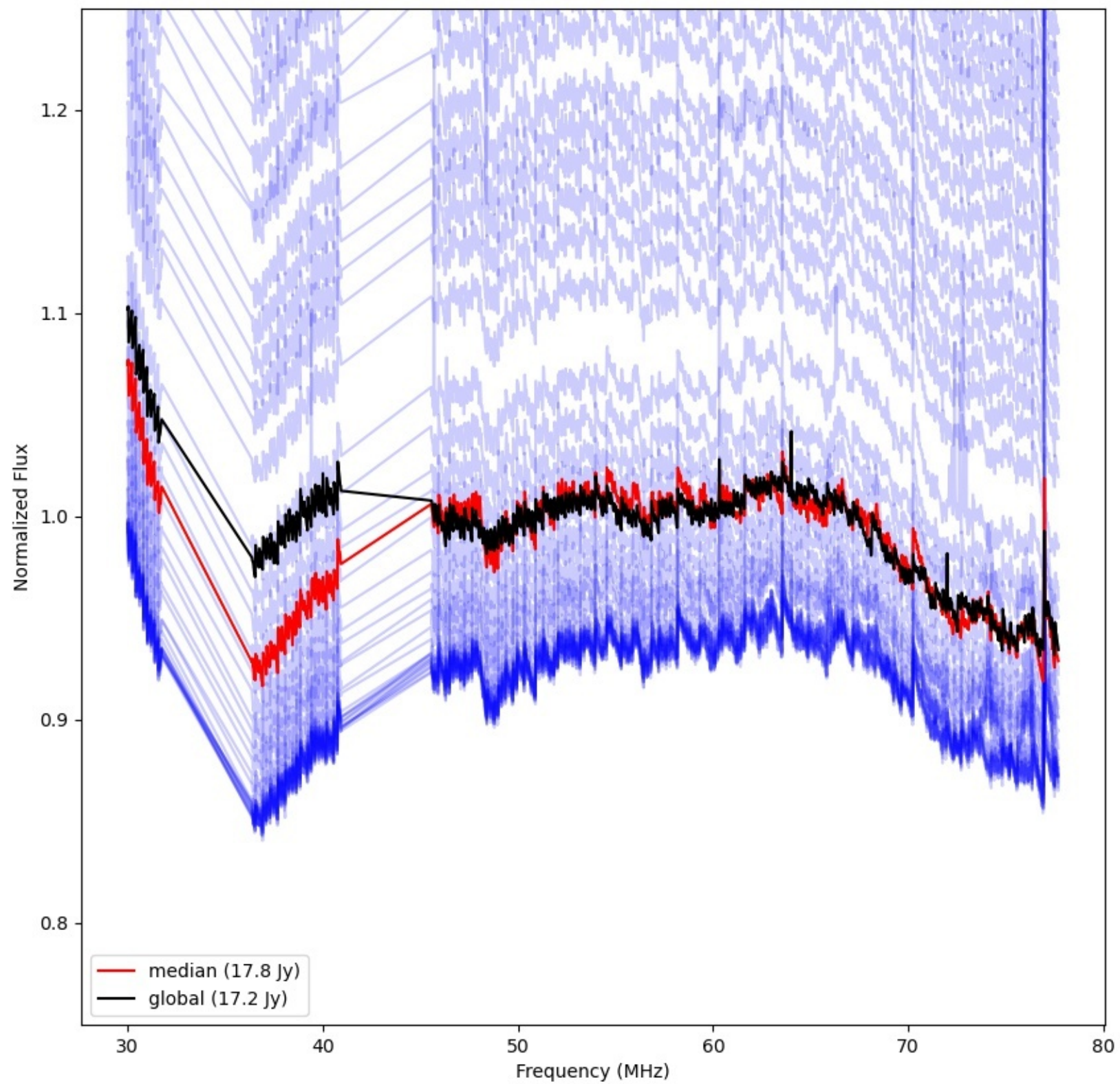
LWA080 - Correlator# 119 - YY - FLAGS:Good
