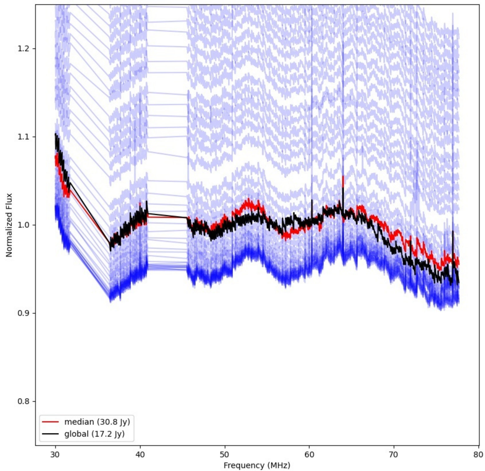
LWA187 - Correlator# 242 - YY - FLAGS:Good
