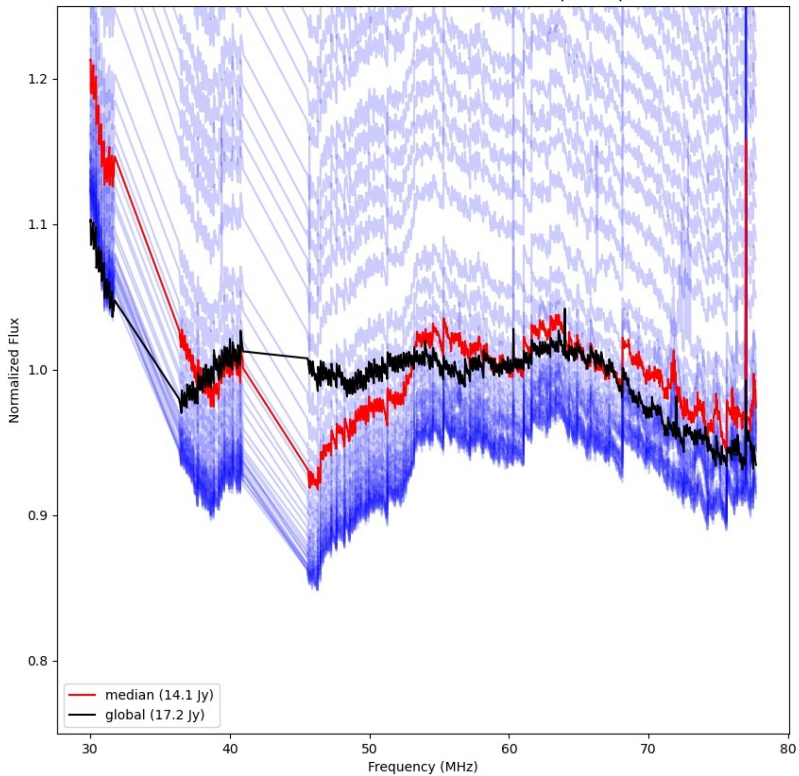
LWA330 - Correlator# 022 - YY - FLAGS:BadSpecShape
