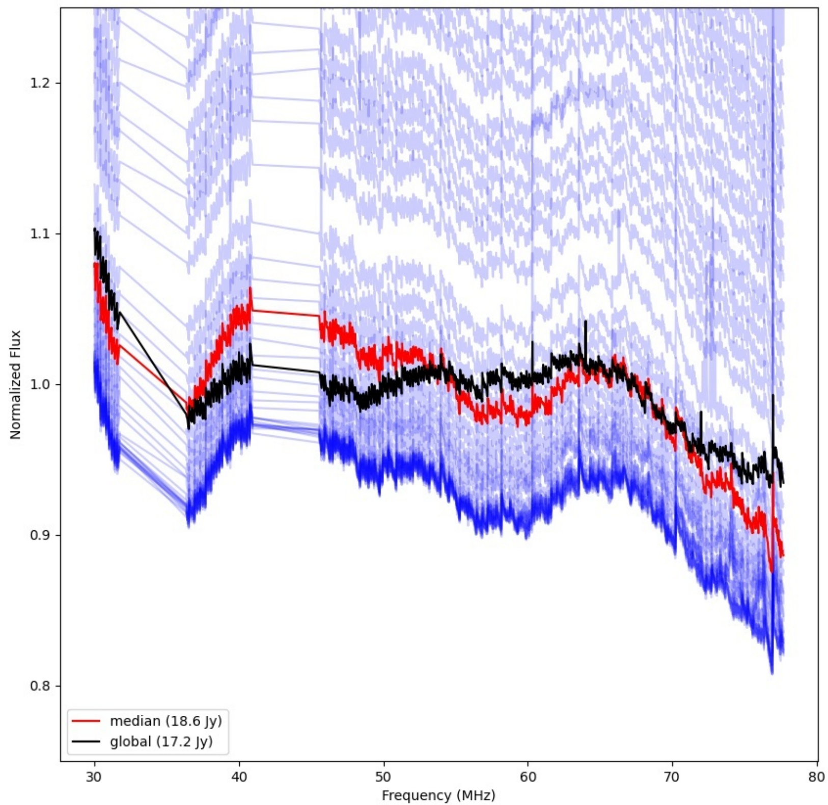
LWA078 - Correlator# 192 - YY - FLAGS:Good
