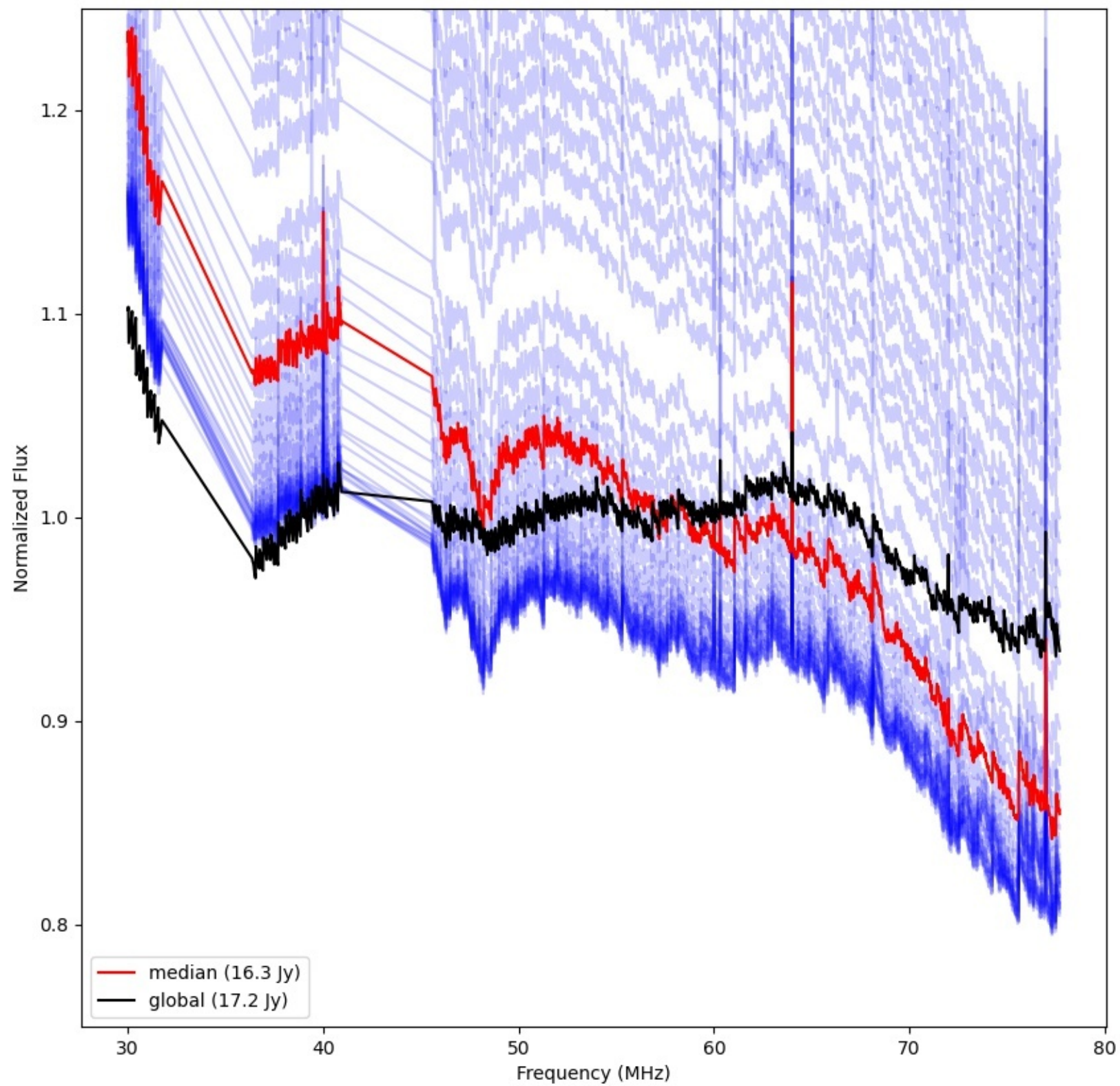
LWA188 - Correlator# 228 - YY - FLAGS:Good
