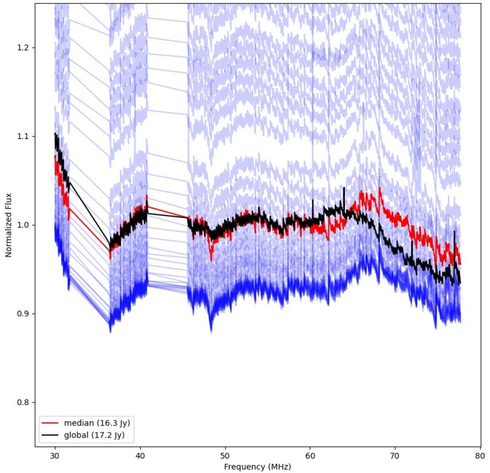
LWA171 - Correlator# 291 - YY - FLAGS:Good
