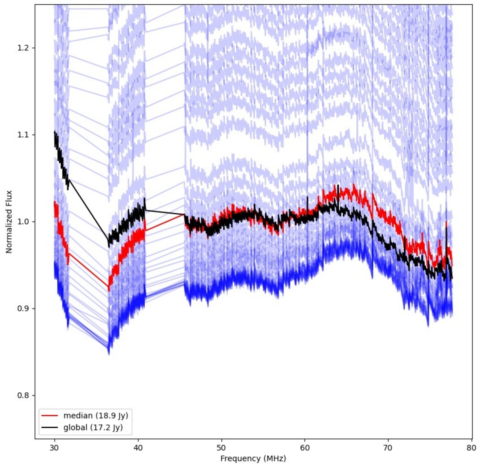
LWA107 - Correlator# 197 - YY - FLAGS:Good
