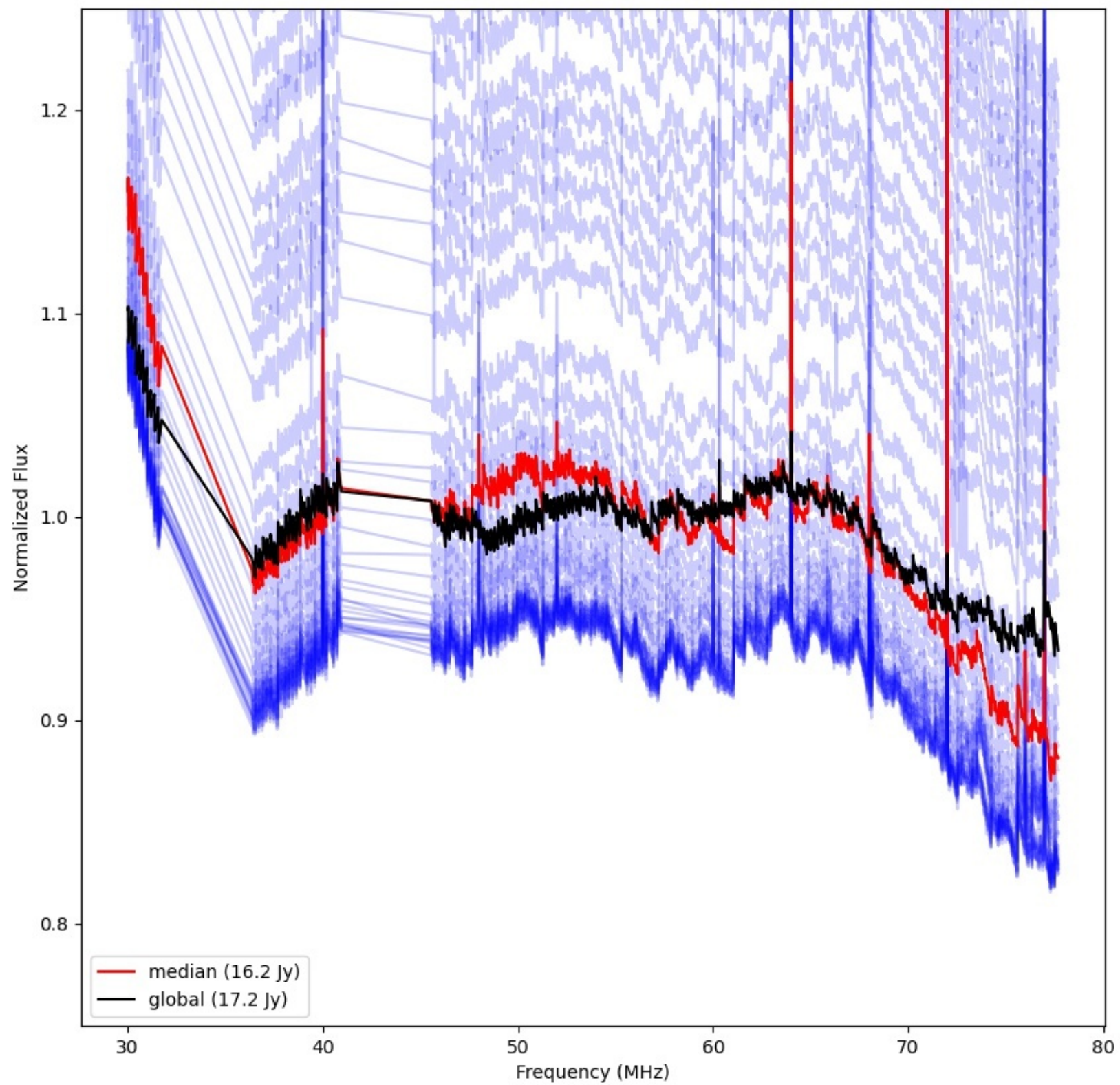
LWA191 - Correlator# 246 - YY - FLAGS:Good
