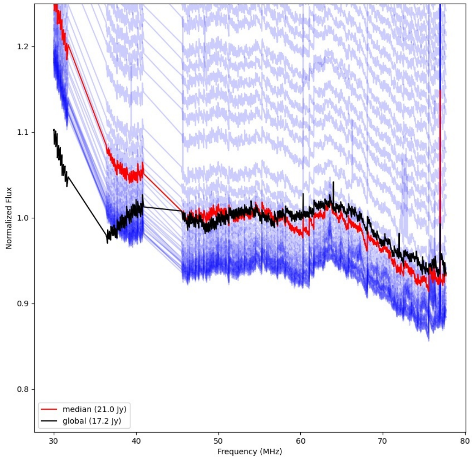
LWA298 - Correlator# 049 - YY - FLAGS:Good
