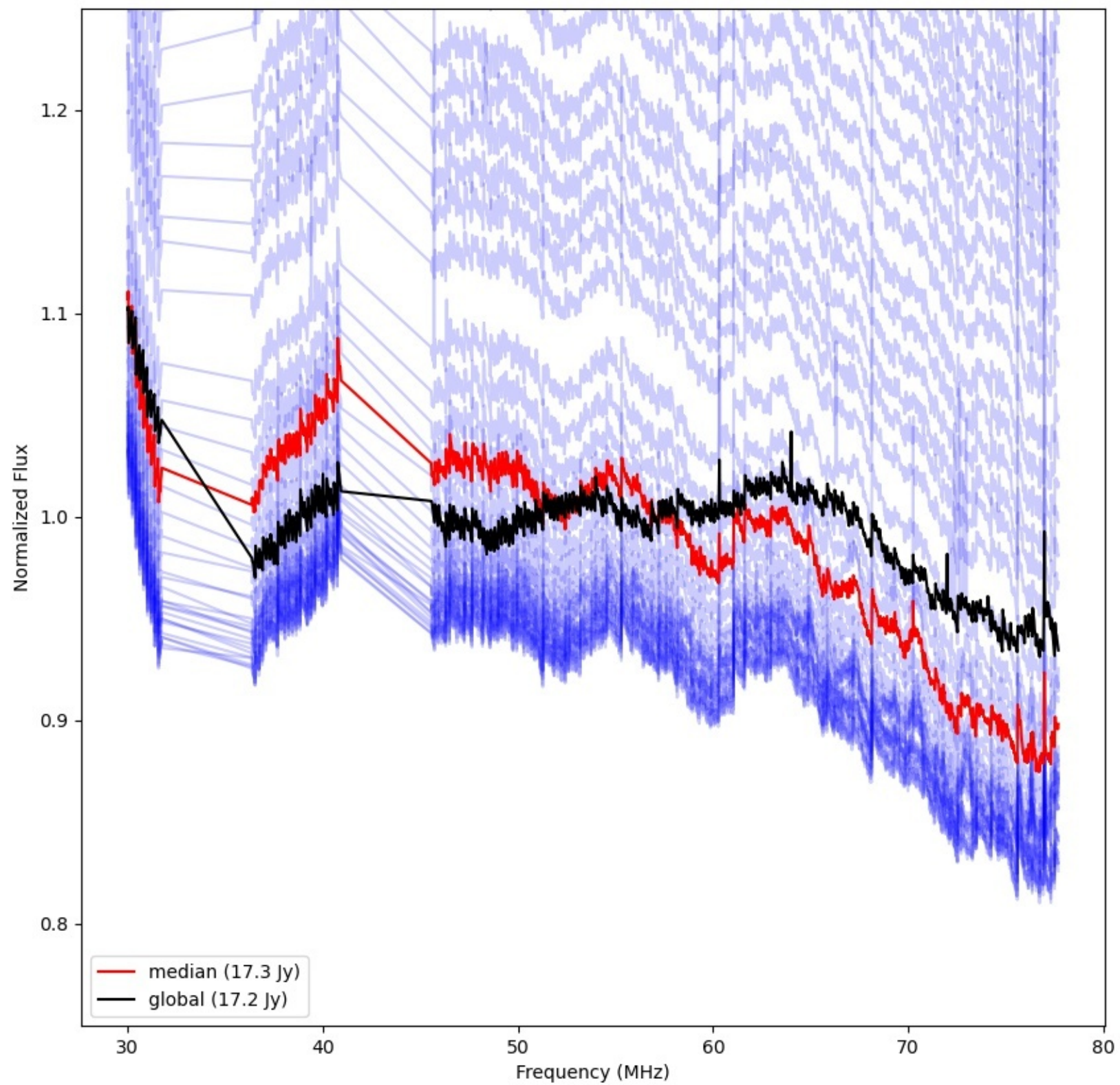
LWA283 - Correlator# 040 - YY - FLAGS:Good
