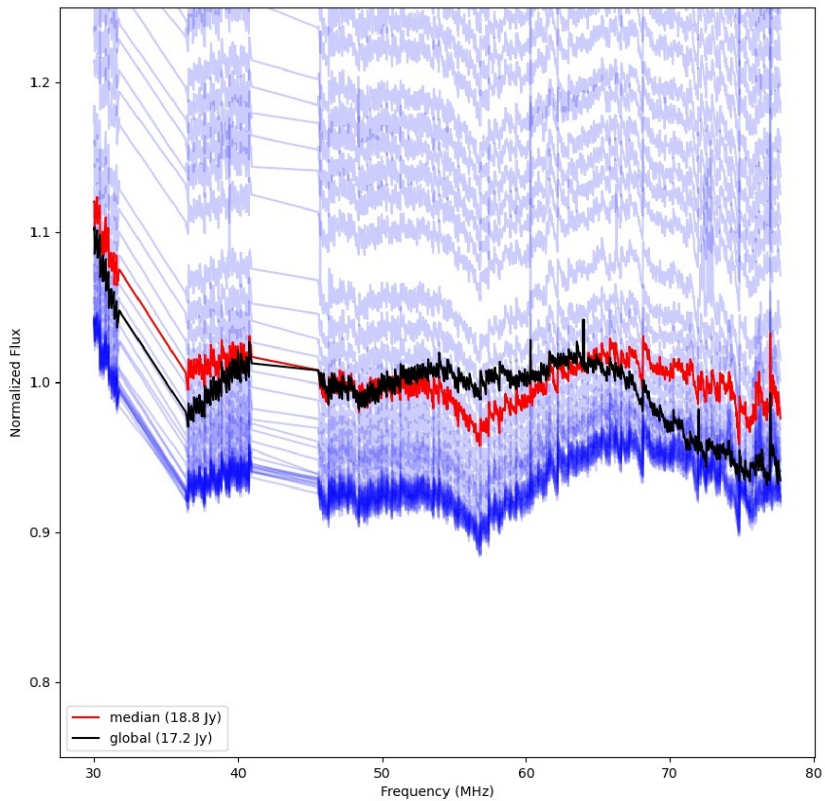
LWA173 - Correlator# 290 - YY - FLAGS:Good
