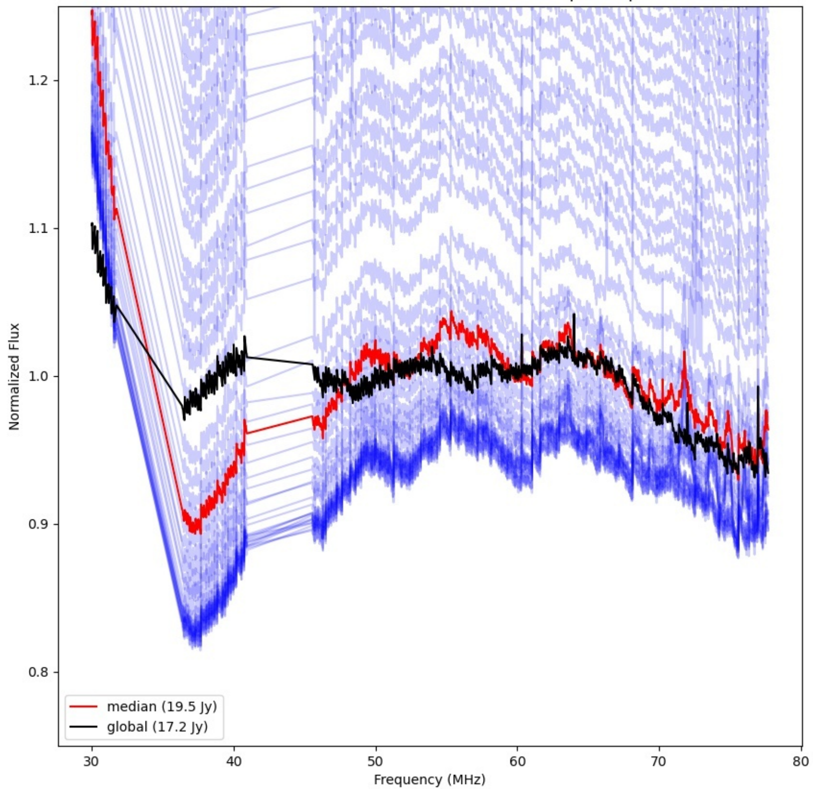
LWA291 - Correlator# 045 - YY - FLAGS:BadSpecShape
