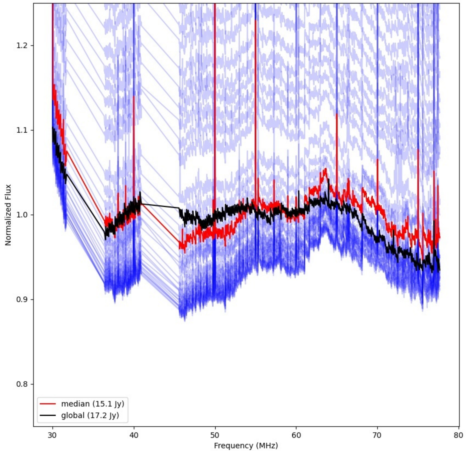
LWA360 - Correlator# 062 - YY - FLAGS:Good
