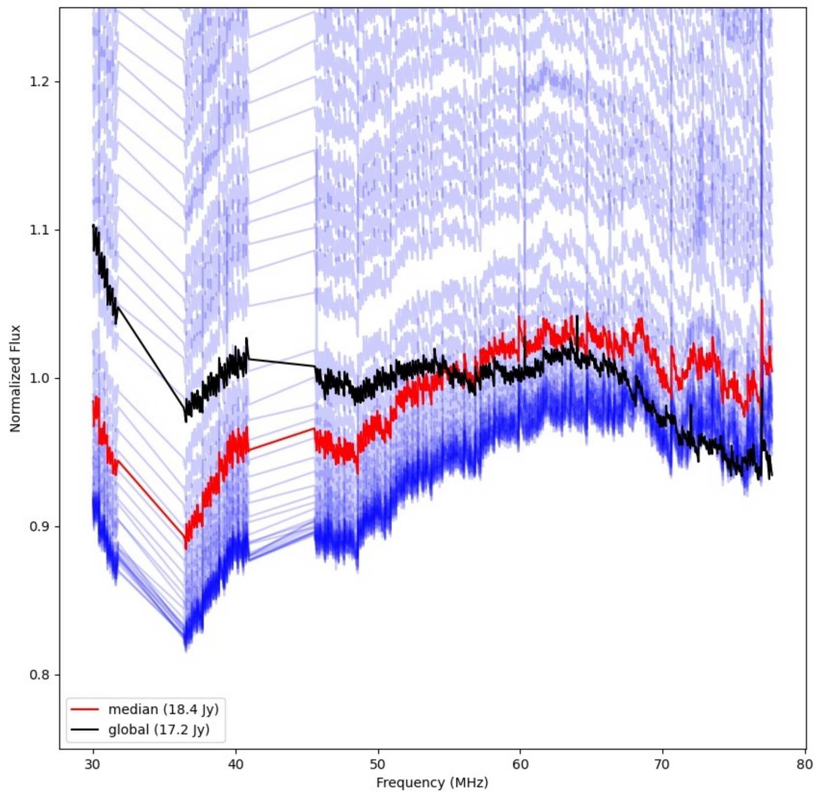
LWA097 - Correlator# 170 - YY - FLAGS:Good
