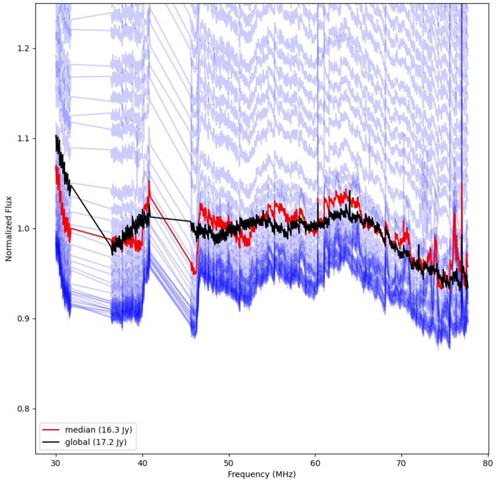
LWA349 - Correlator# 282 - YY - FLAGS:Good
