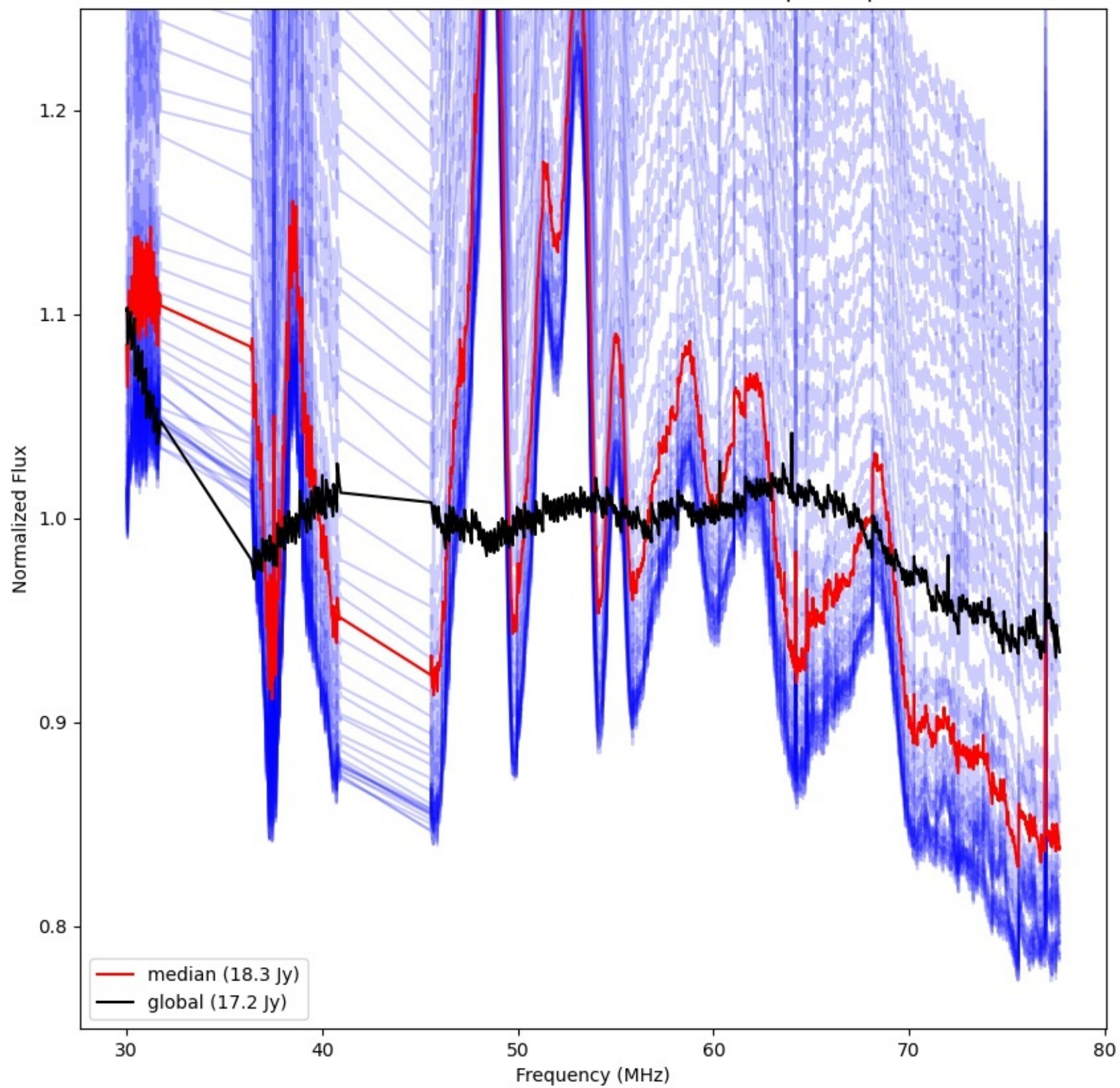
LWA336 - Correlator# 056 - YY - FLAGS:BadSpecShape
