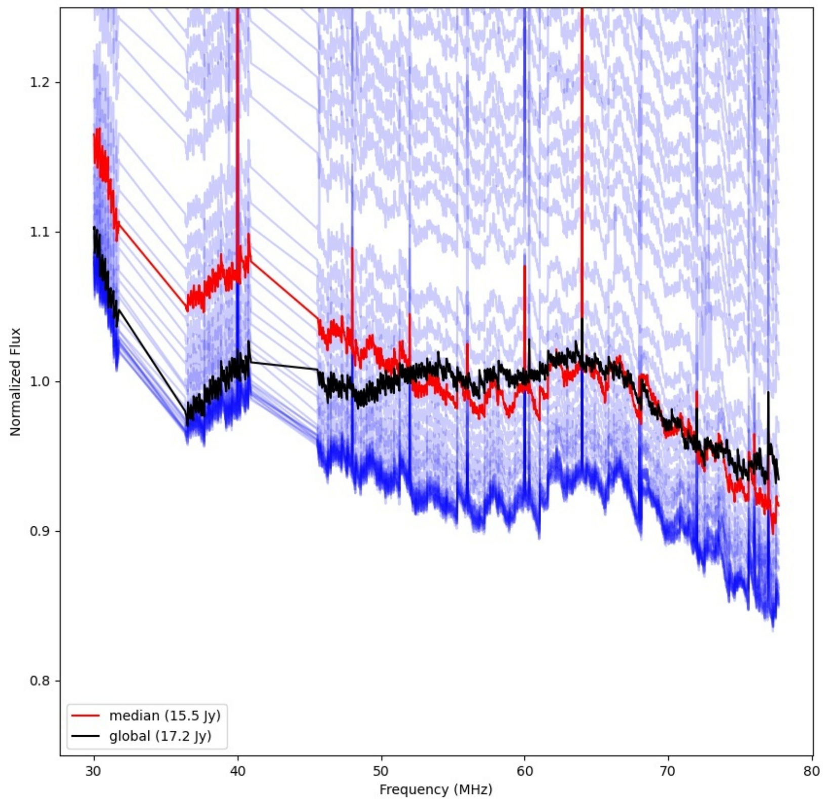
LWA159 - Correlator# 236 - YY - FLAGS:Good
