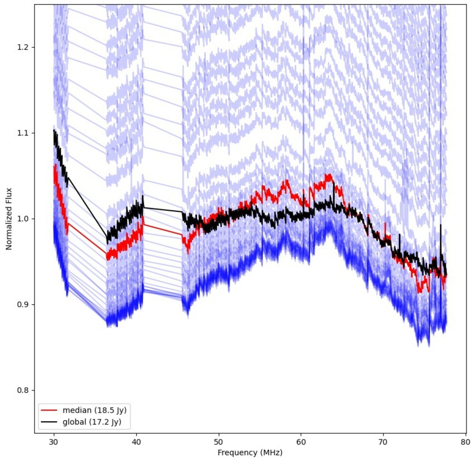
LWA285 - Correlator# 013 - YY - FLAGS:Good
