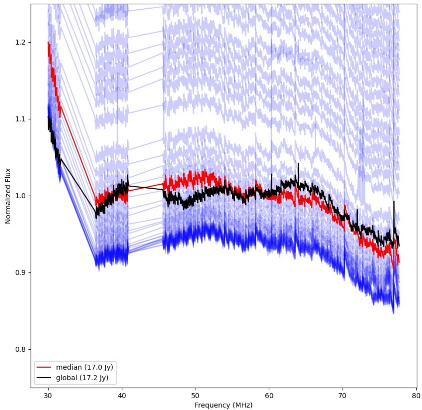
LWA051 - Correlator# 114 - YY - FLAGS:Good
