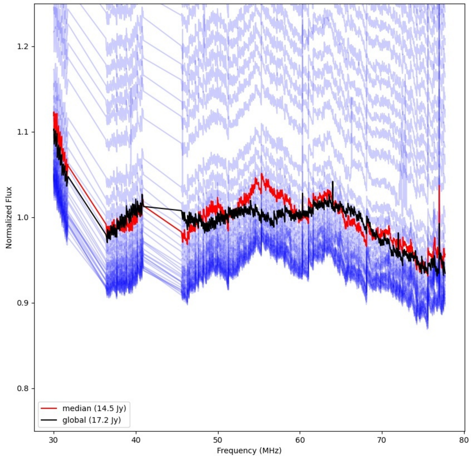
LWA269 - Correlator# 005 - YY - FLAGS:Good
