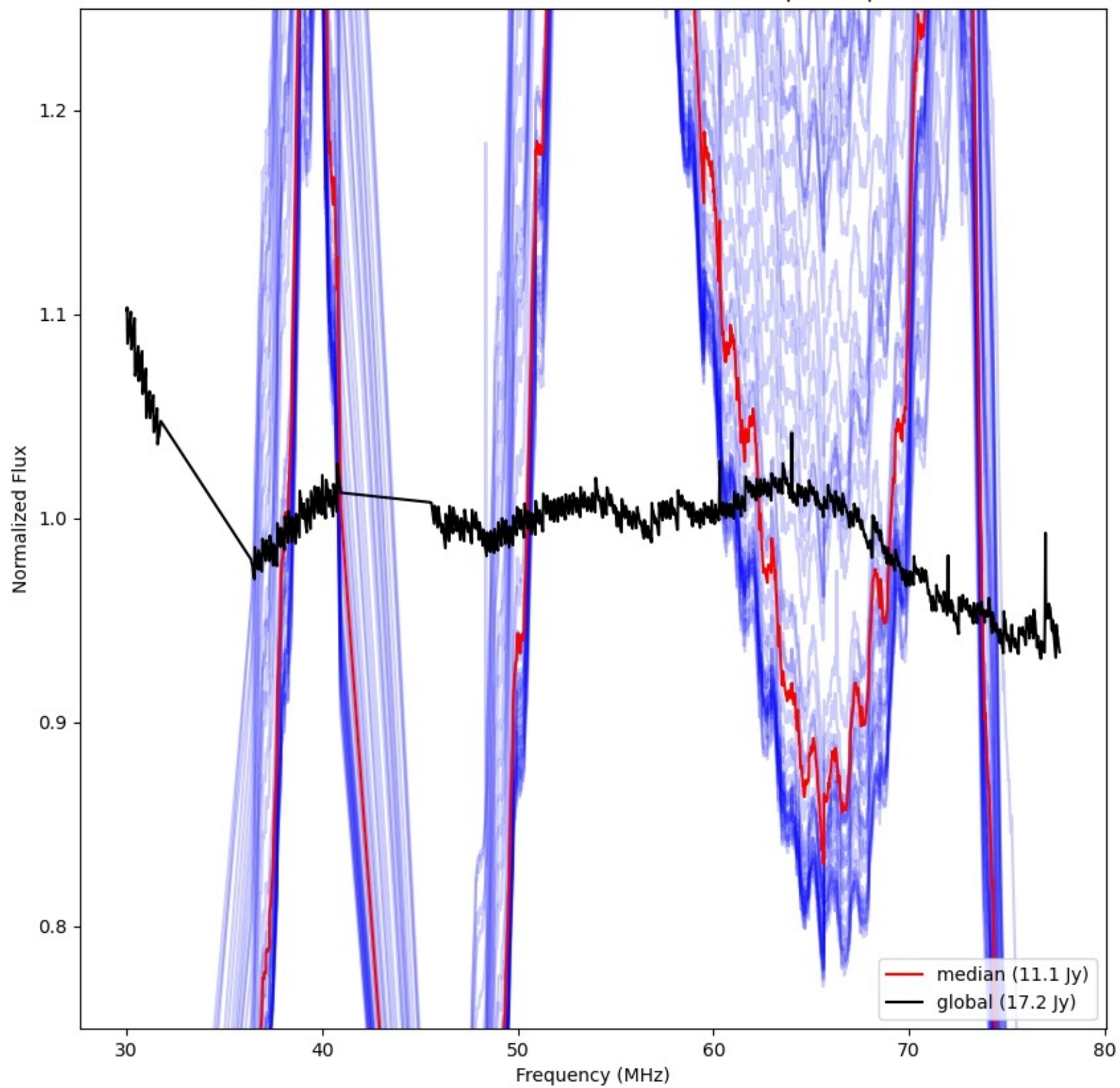
LWA120 - Correlator# 208 - YY - FLAGS:BadSpecShape
