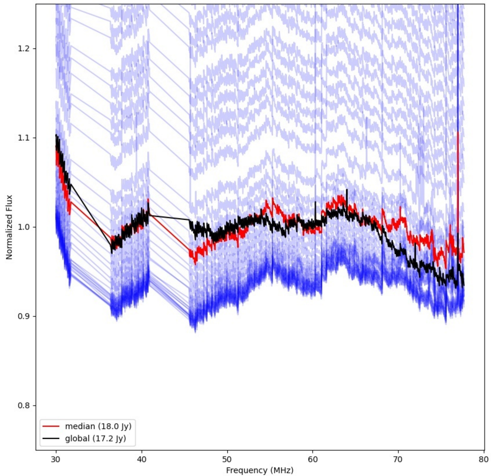
LWA273 - Correlator# 007 - YY - FLAGS:Good
