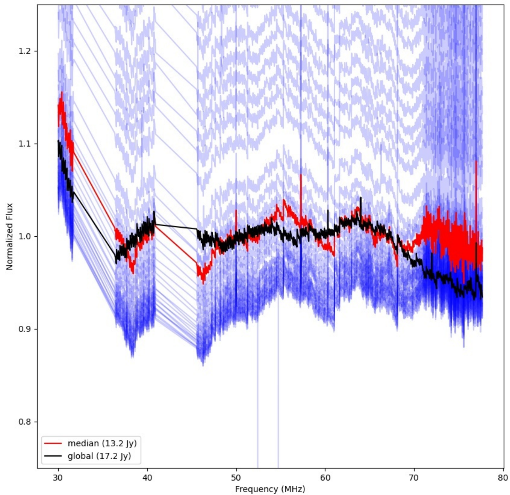
LWA263 - Correlator# 037 - YY - FLAGS:Good
