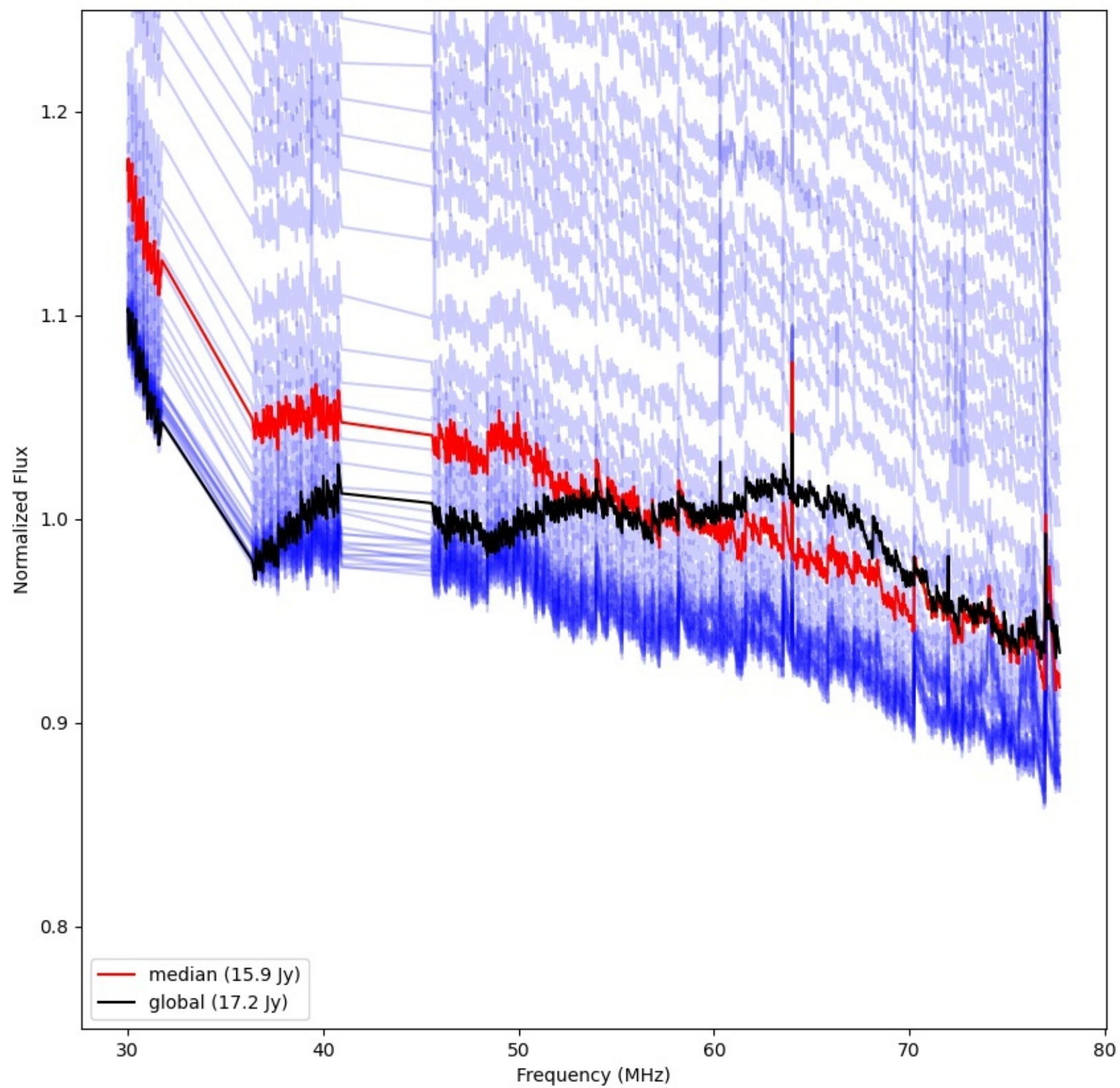
LWA027 - Correlator# 111 - YY - FLAGS:Good
