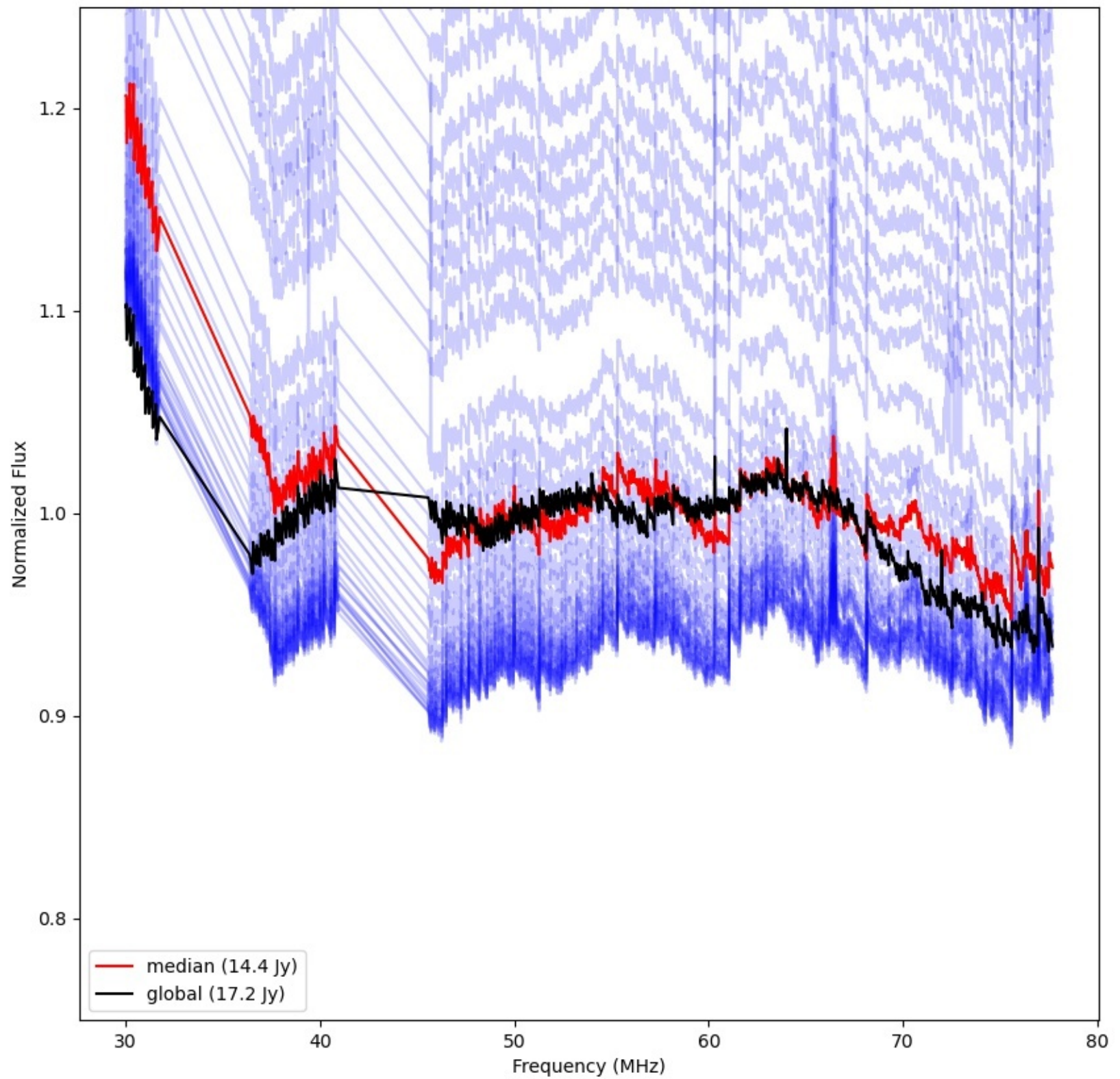
LWA299 - Correlator# 191 - YY - FLAGS:Good
