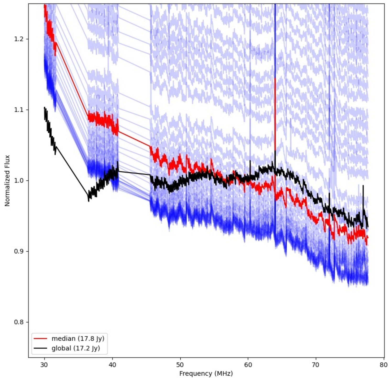
LWA032 - Correlator# 130 - YY - FLAGS:Good
