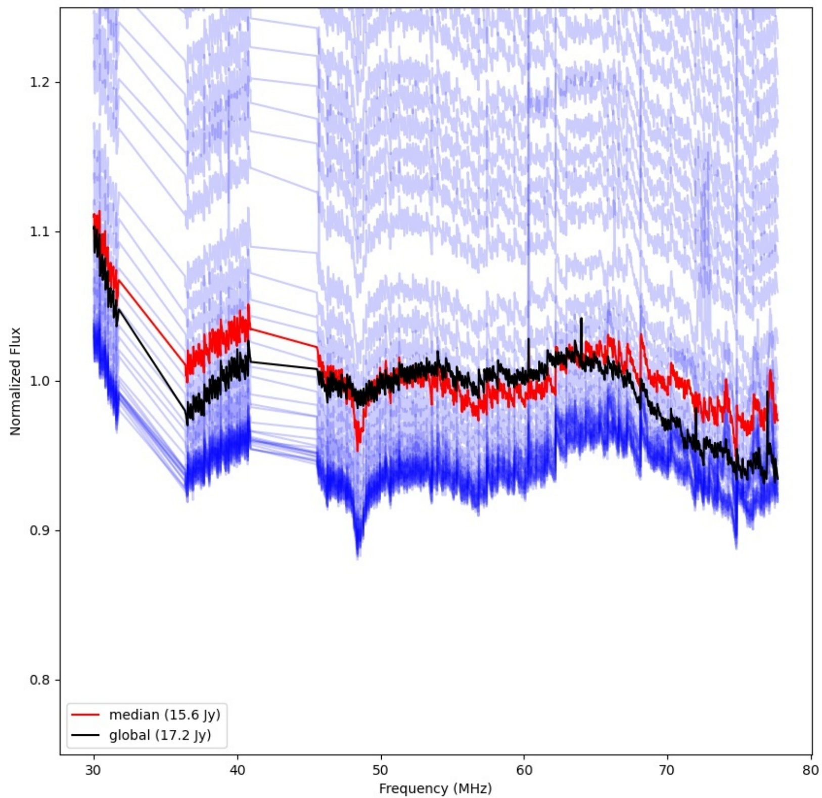
LWA238 - Correlator# 310 - YY - FLAGS:Good
