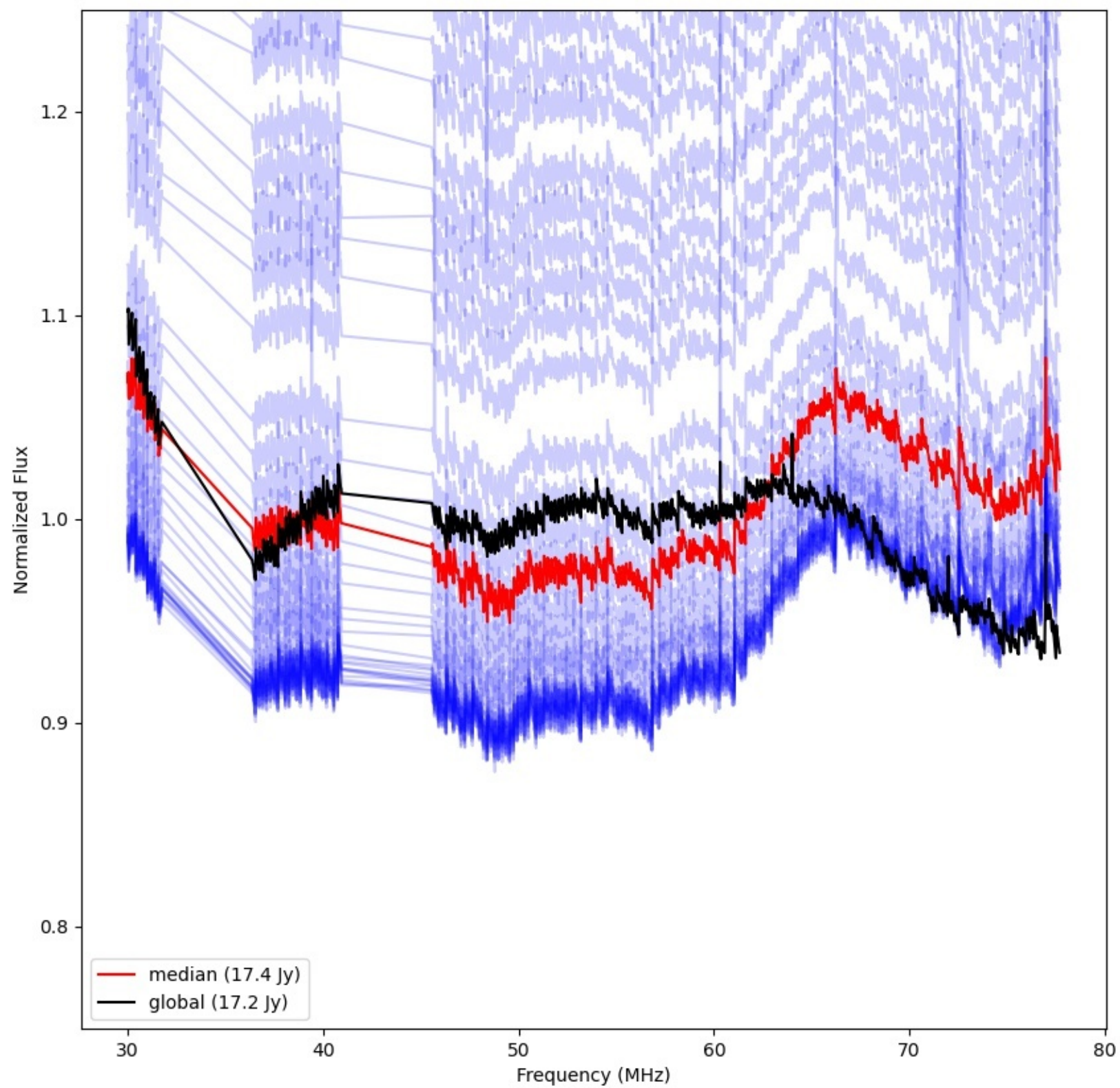
LWA228 - Correlator# 302 - YY - FLAGS:Good
