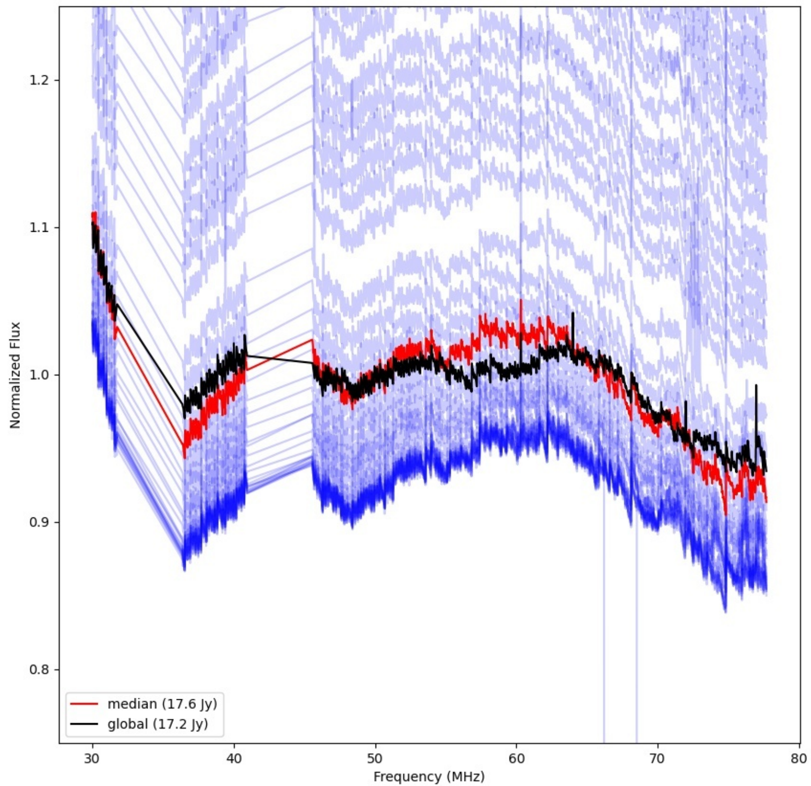
LWA072 - Correlator# 171 - YY - FLAGS:Good
