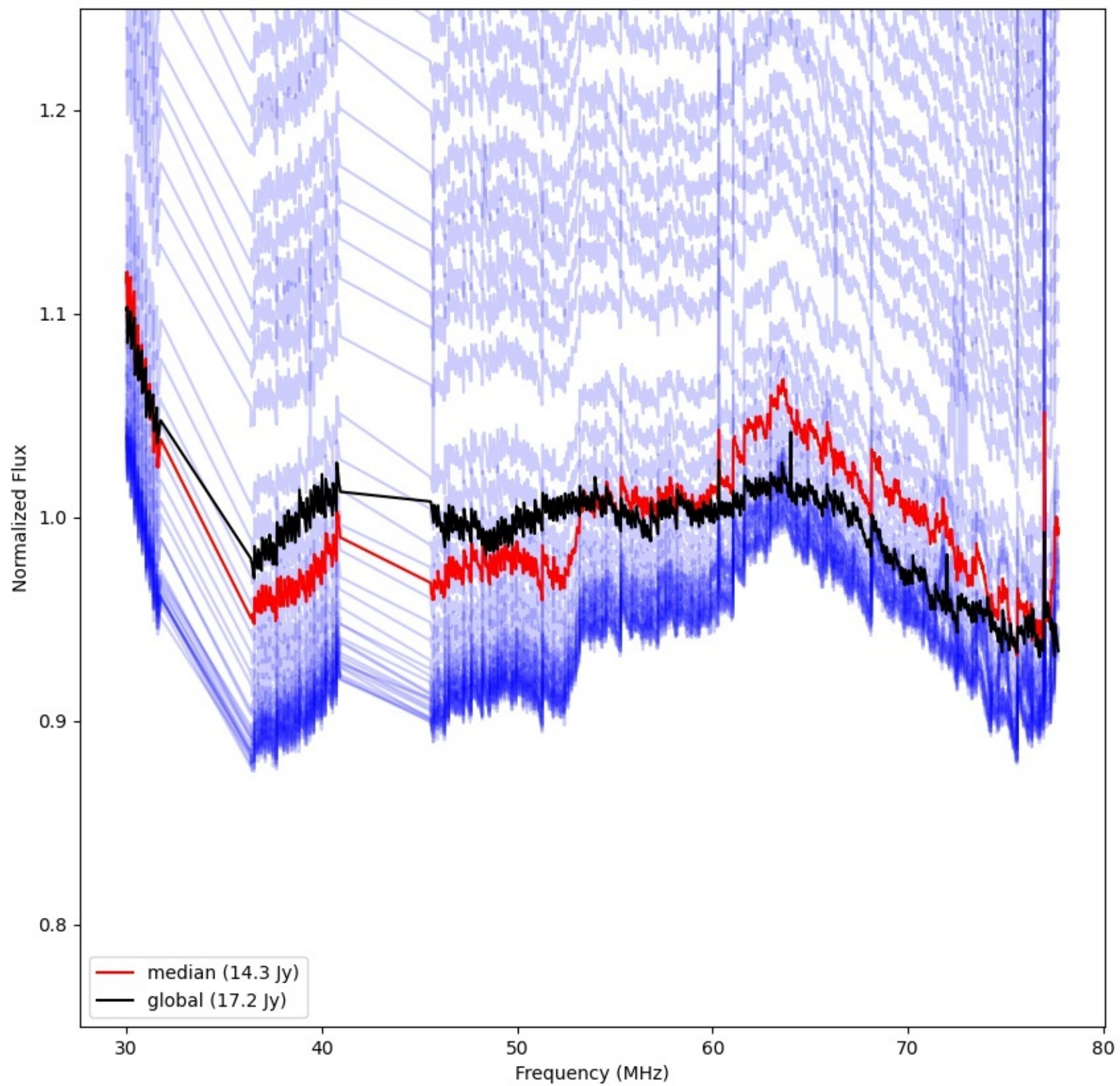
LWA274 - Correlator# 091 - YY - FLAGS:Good
