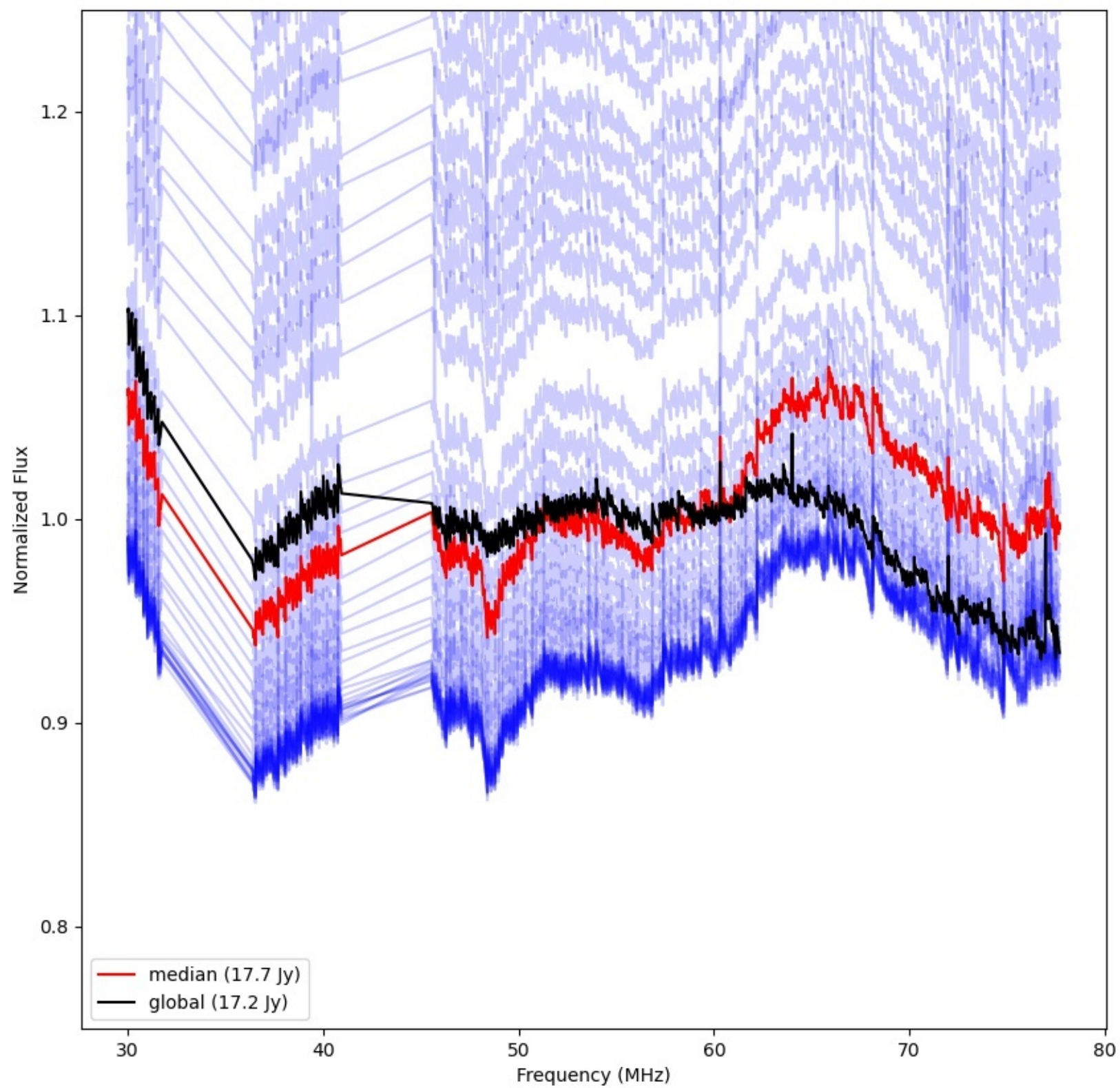
LWA245 - Correlator# 341 - YY - FLAGS:Good
