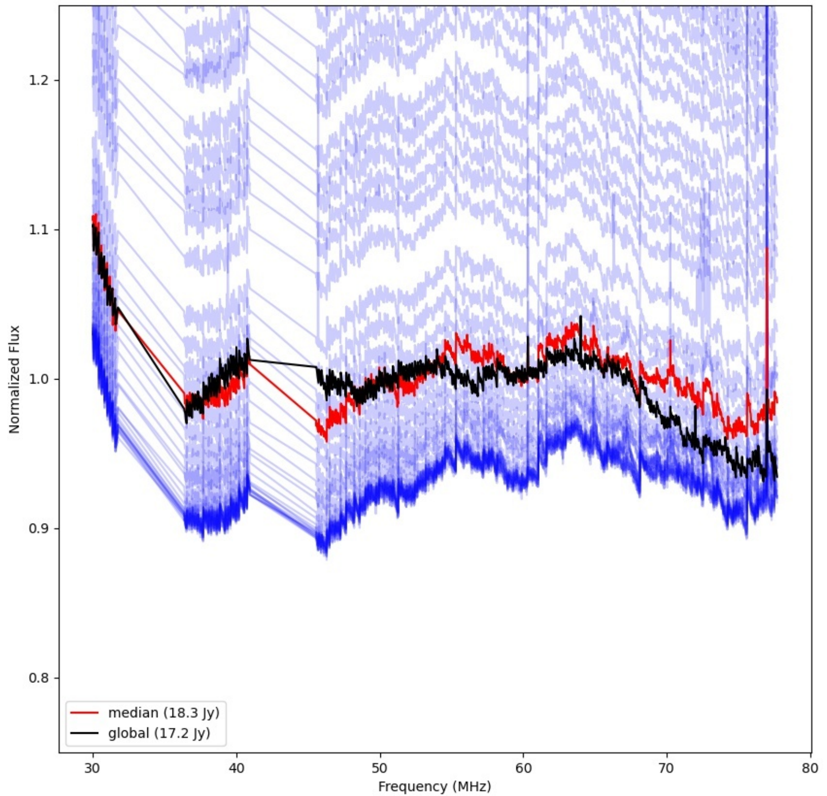
LWA257 - Correlator# 032 - YY - FLAGS:Good
