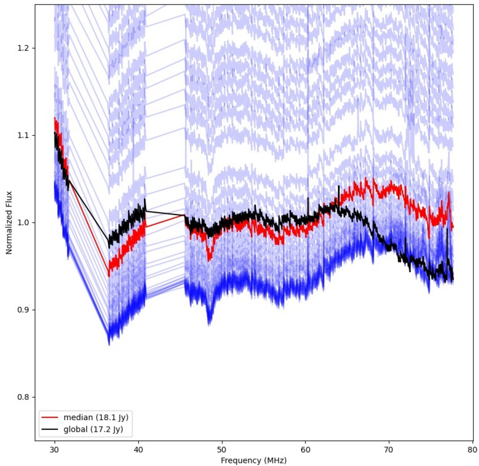
LWA240 - Correlator# 312 - YY - FLAGS:Good
