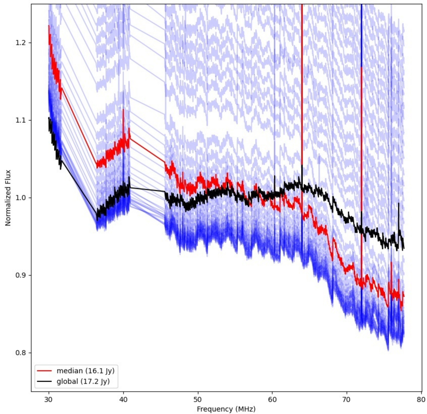
LWA093 - Correlator# 148 - YY - FLAGS:Good
