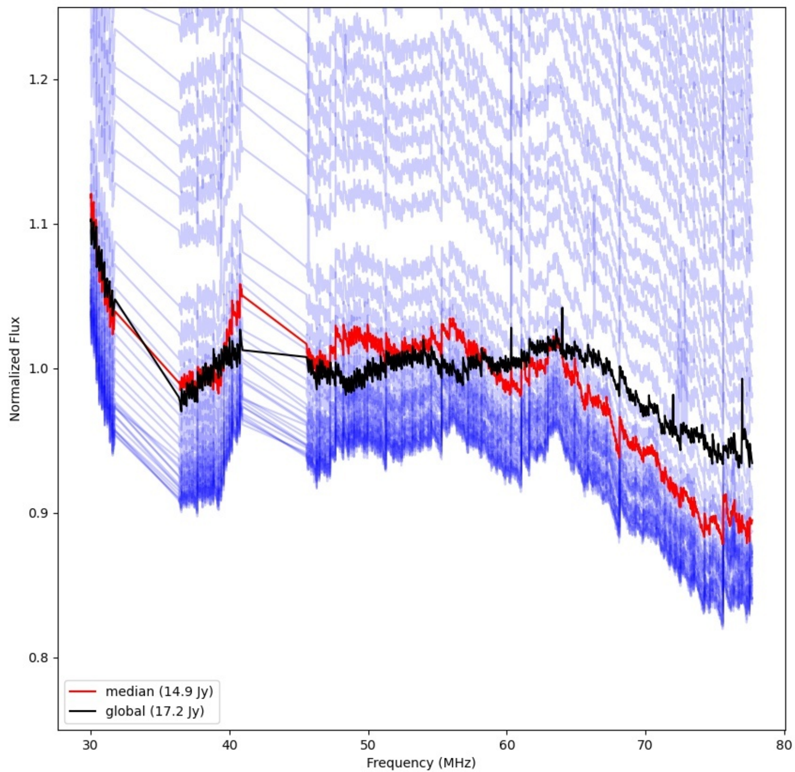
LWA313 - Correlator# 018 - YY - FLAGS:Good
