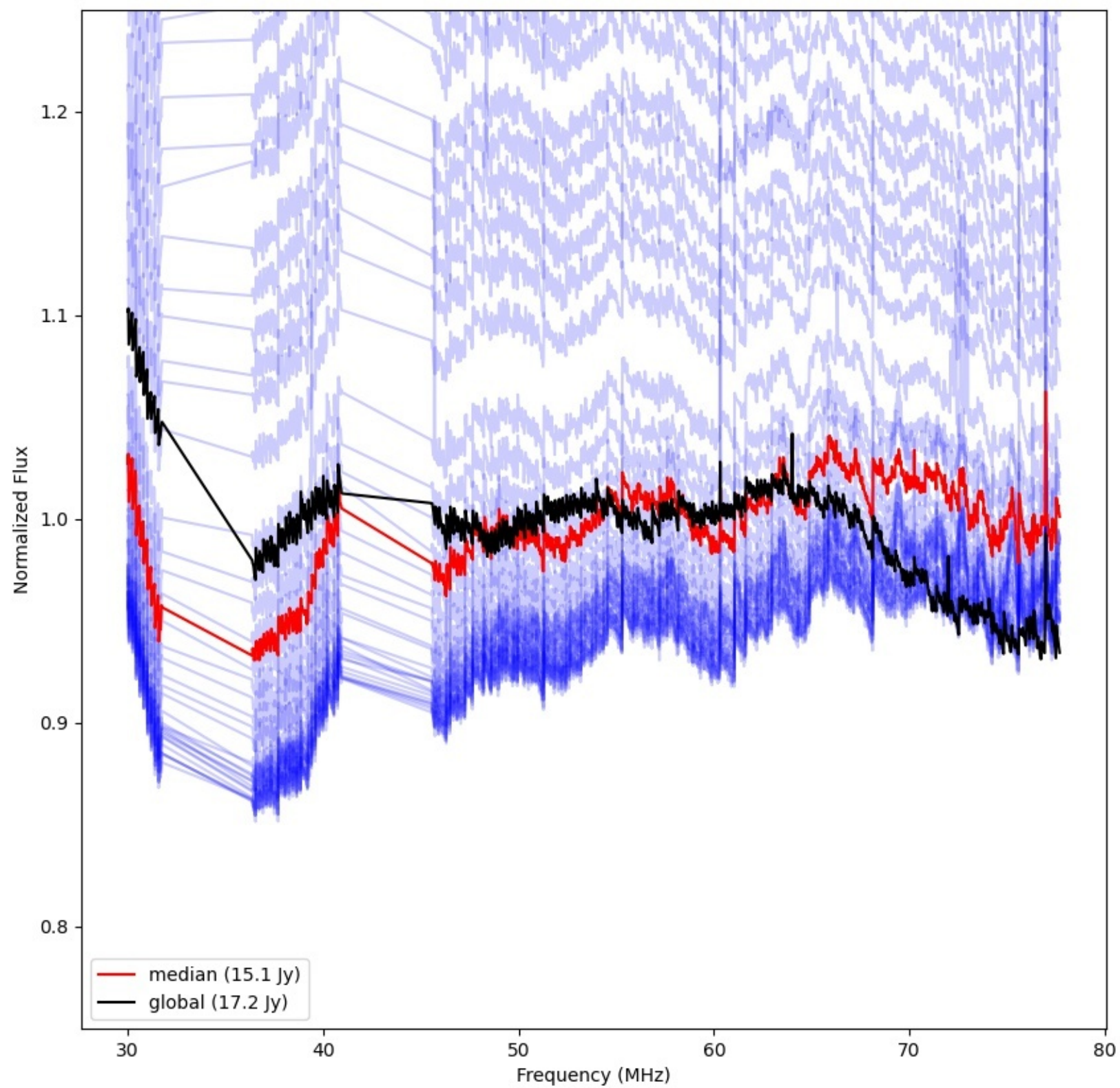
LWA266 - Correlator# 000 - YY - FLAGS:Good
