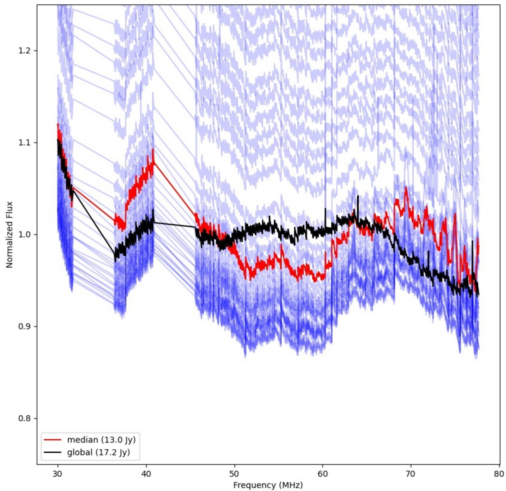
LWA347 - Correlator# 255 - YY - FLAGS:Good
