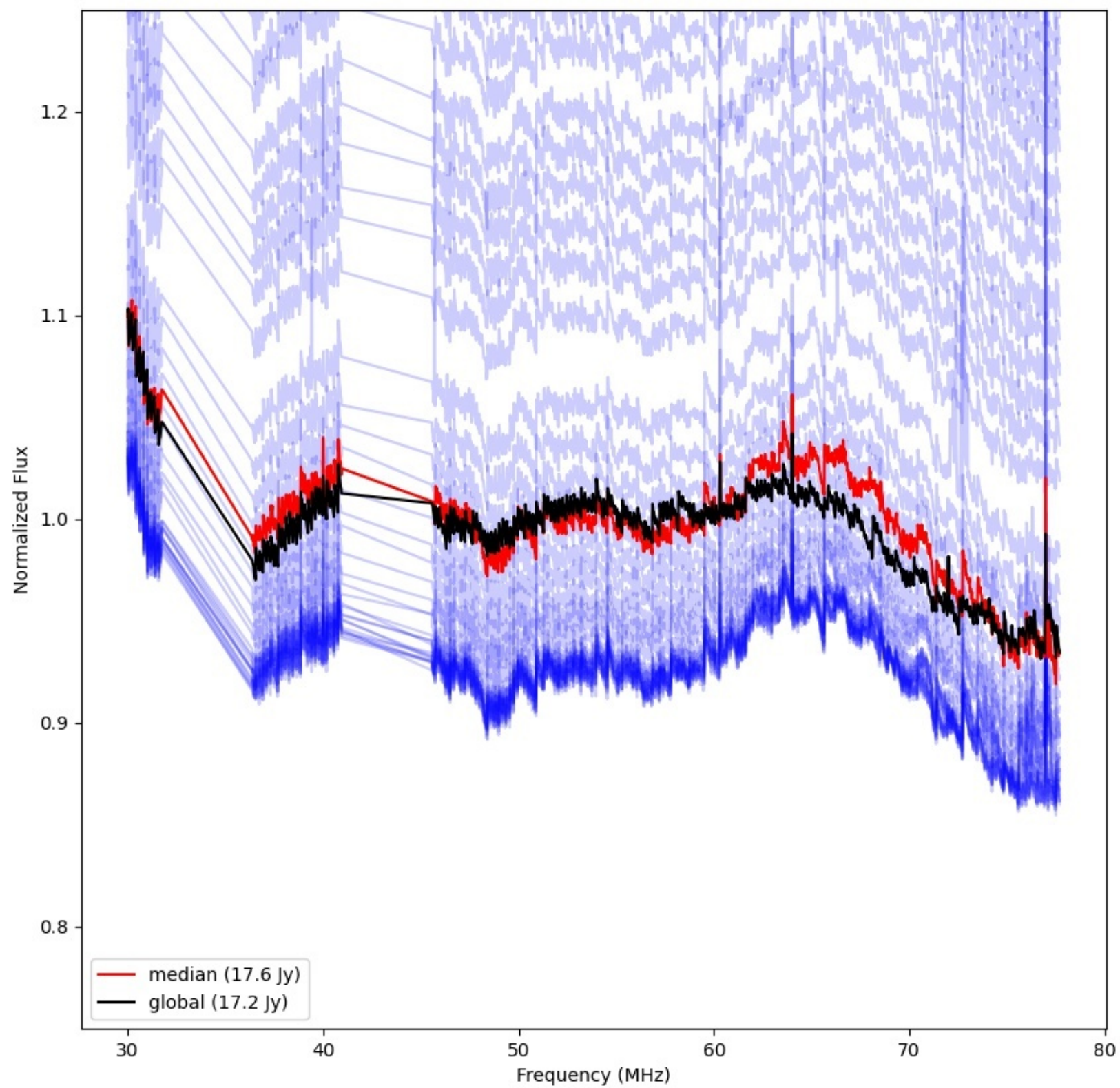
LWA156 - Correlator# 235 - YY - FLAGS:Good
