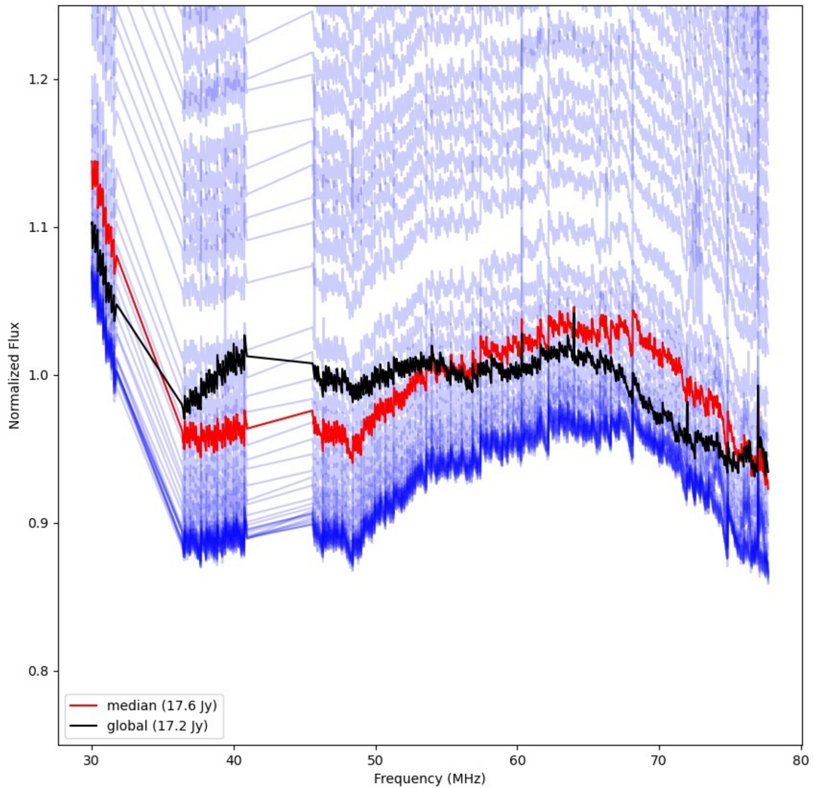
LWA048 - Correlator# 113 - YY - FLAGS:Good
