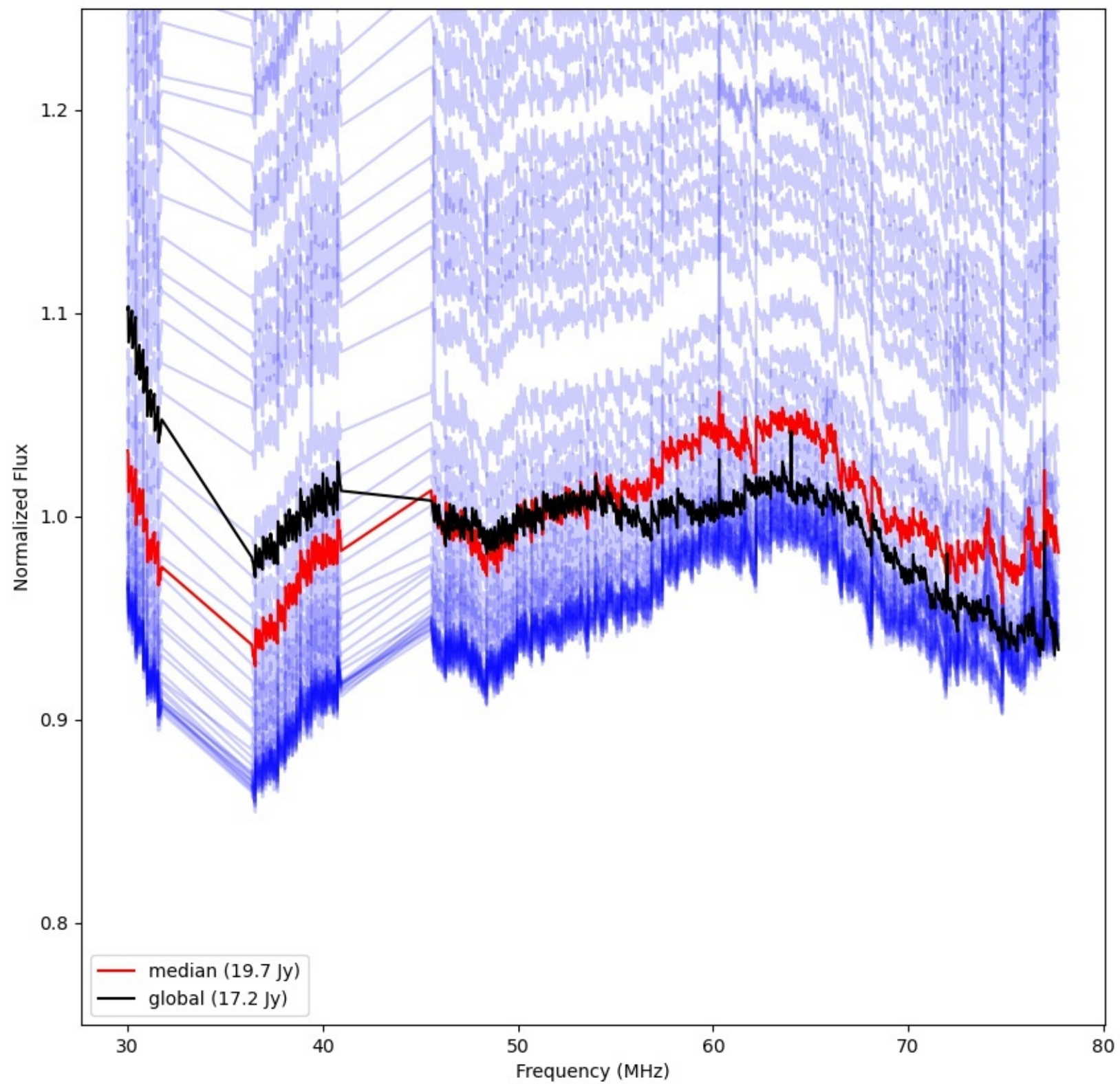
LWA108 - Correlator# 196 - YY - FLAGS:Good
