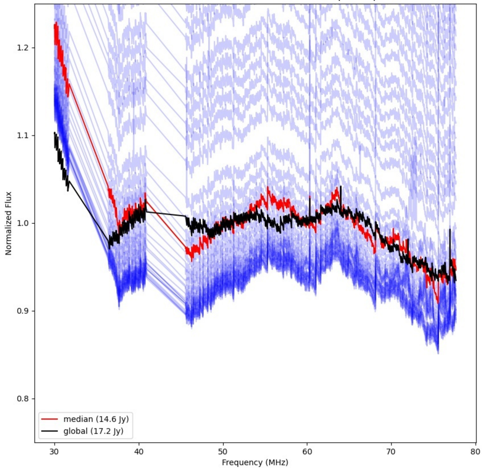
LWA337 - Correlator# 059 - YY - FLAGS:BadSpecShape
