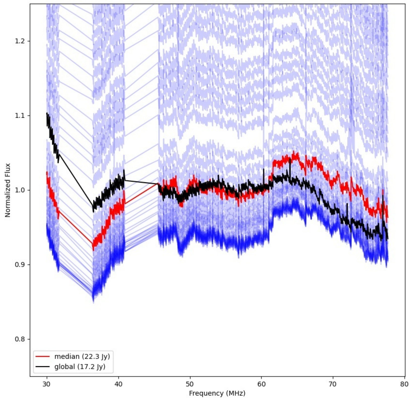
LWA197 - Correlator# 274 - YY - FLAGS:Good
