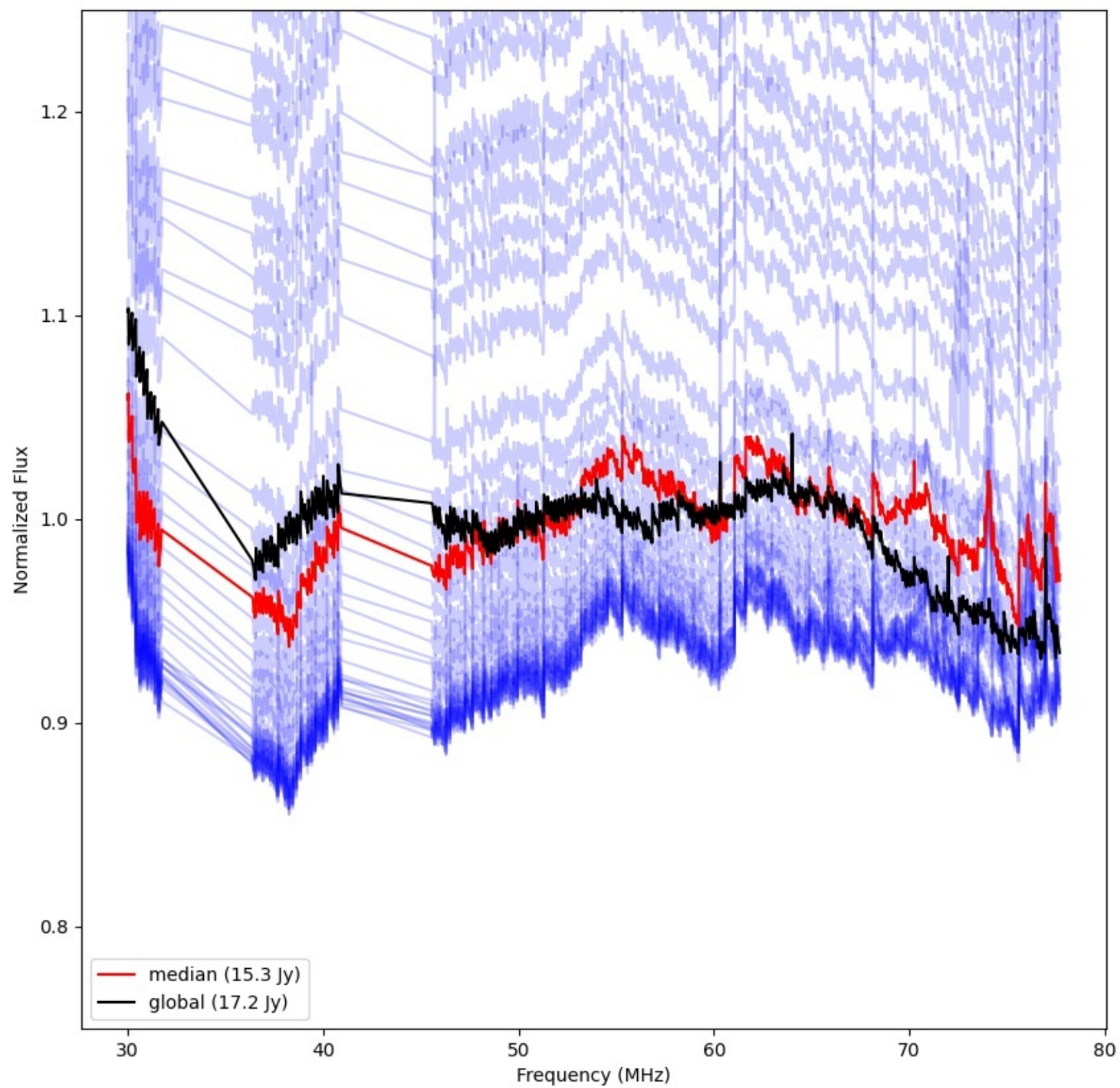
LWA321 - Correlator# 020 - YY - FLAGS:Good
