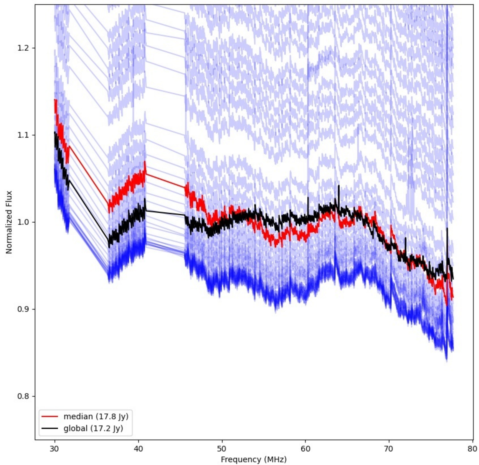
LWA177 - Correlator# 320 - YY - FLAGS:Good
