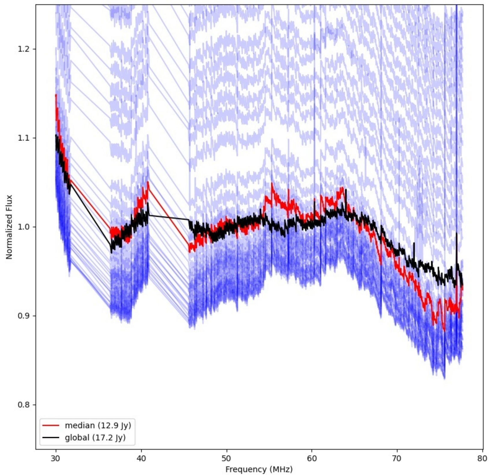
LWA290 - Correlator# 285 - YY - FLAGS:Good
