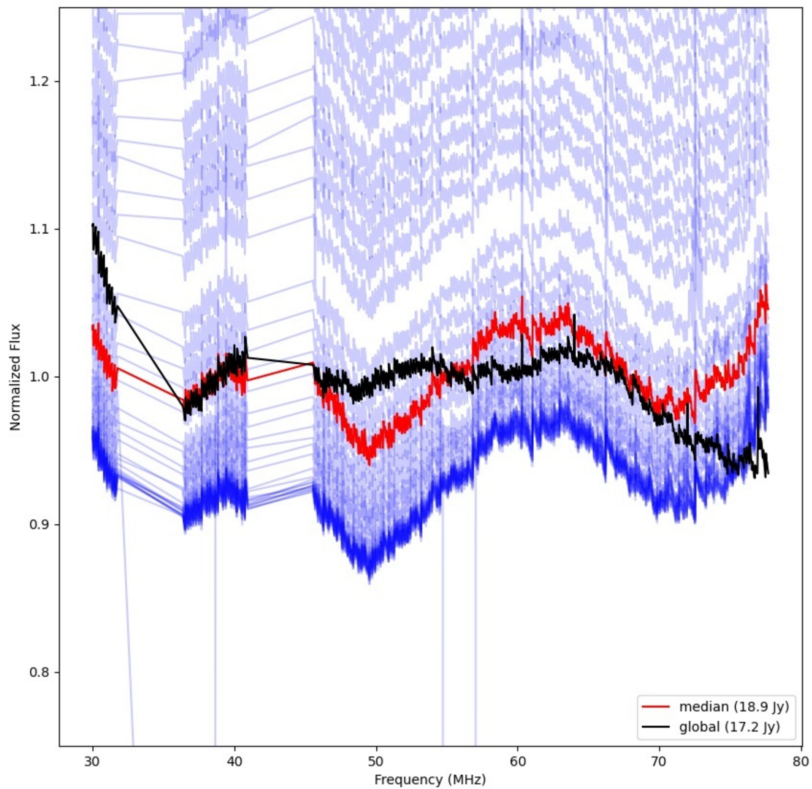
LWA006 - Correlator# 068 - YY - FLAGS:Good
