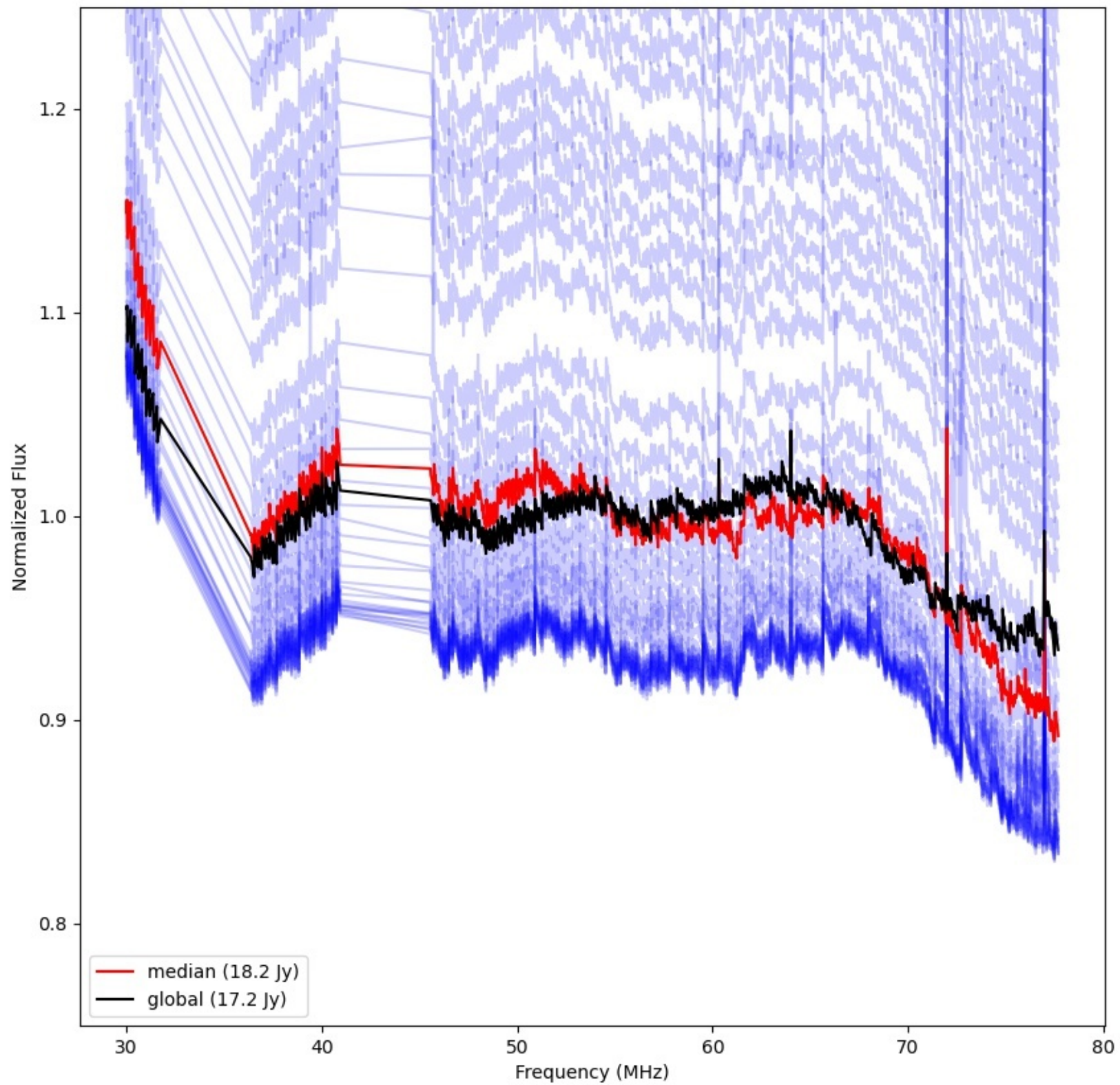
LWA221 - Correlator# 334 - YY - FLAGS:Good
