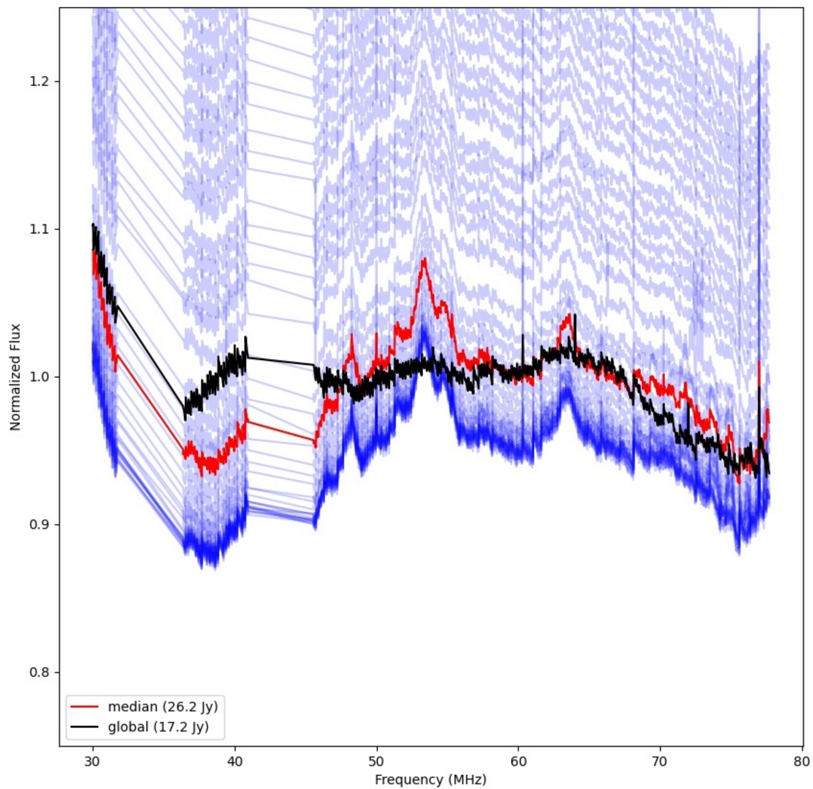
LWA296 - Correlator# 046 - YY - FLAGS:Good
