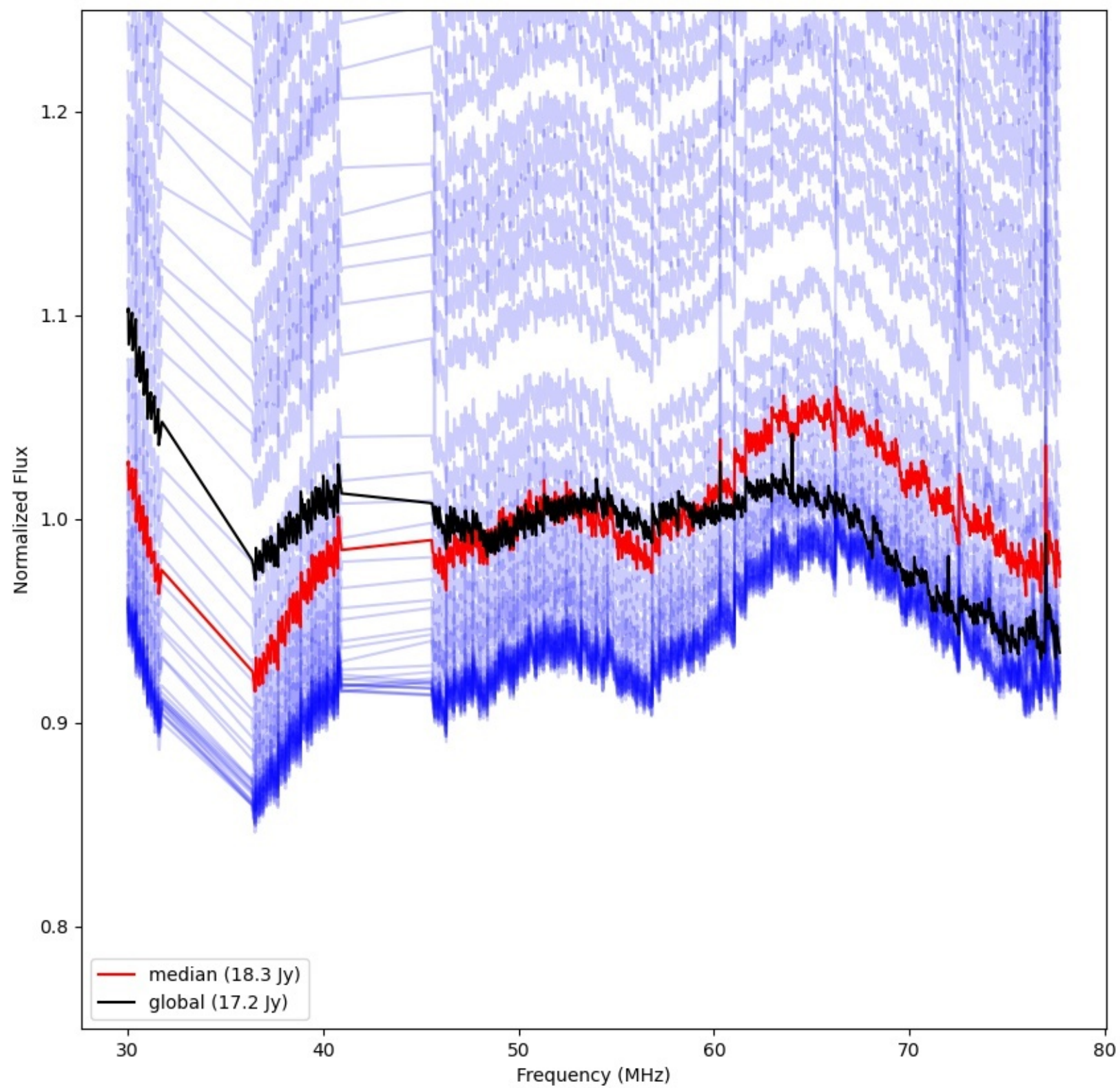
LWA200 - Correlator# 276 - YY - FLAGS:Good
