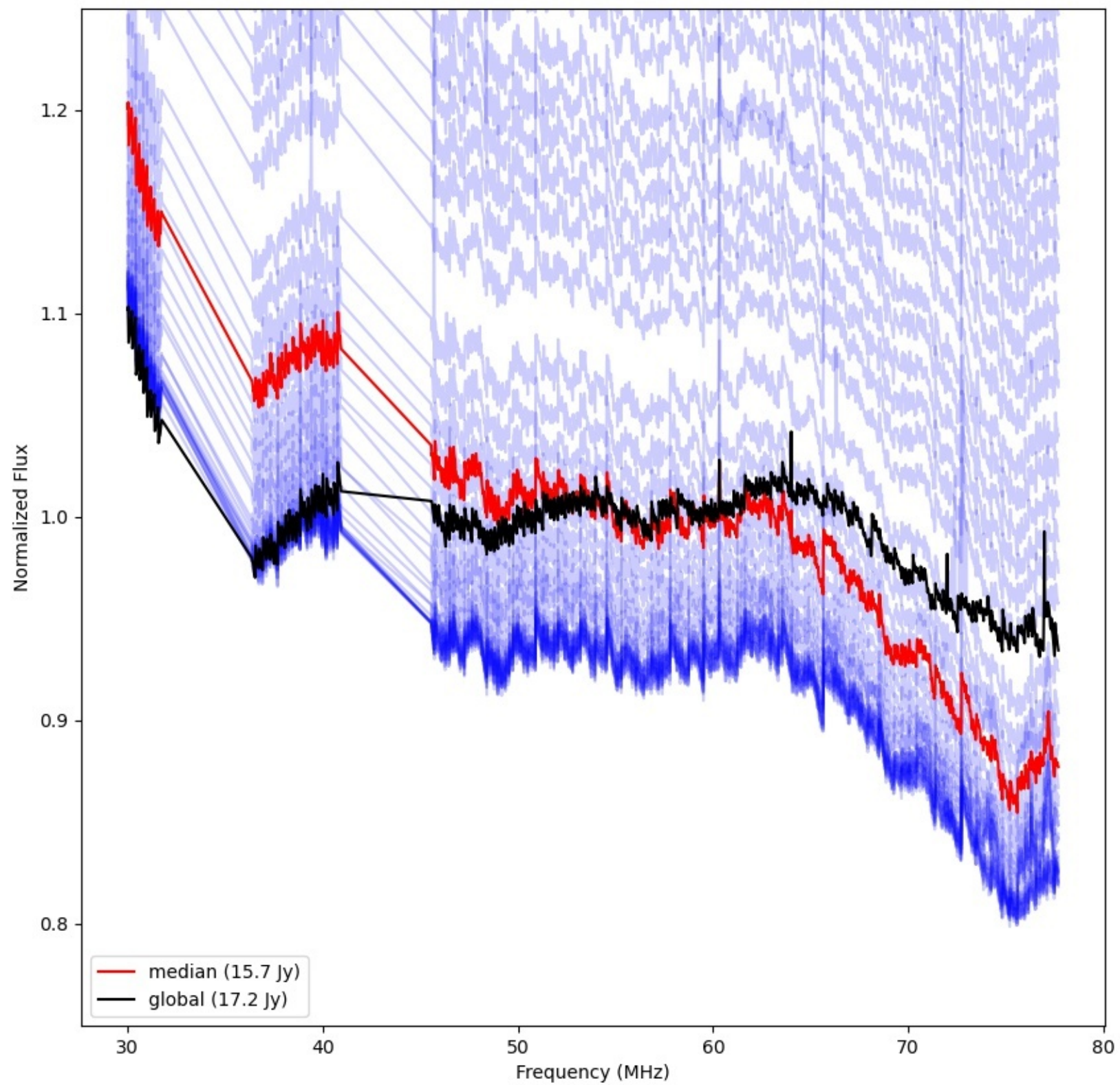
LWA121 - Correlator# 153 - YY - FLAGS:Good
