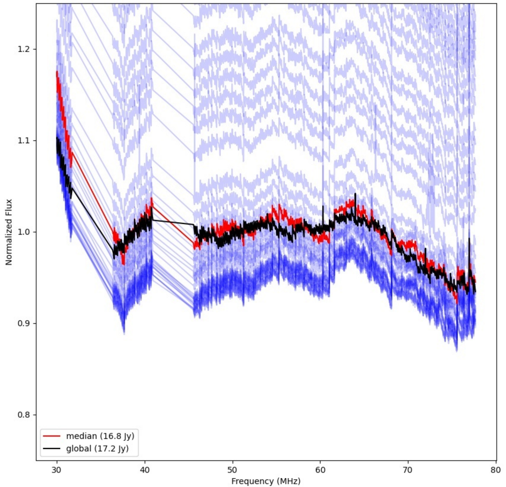
LWA275 - Correlator# 090 - YY - FLAGS:Good
