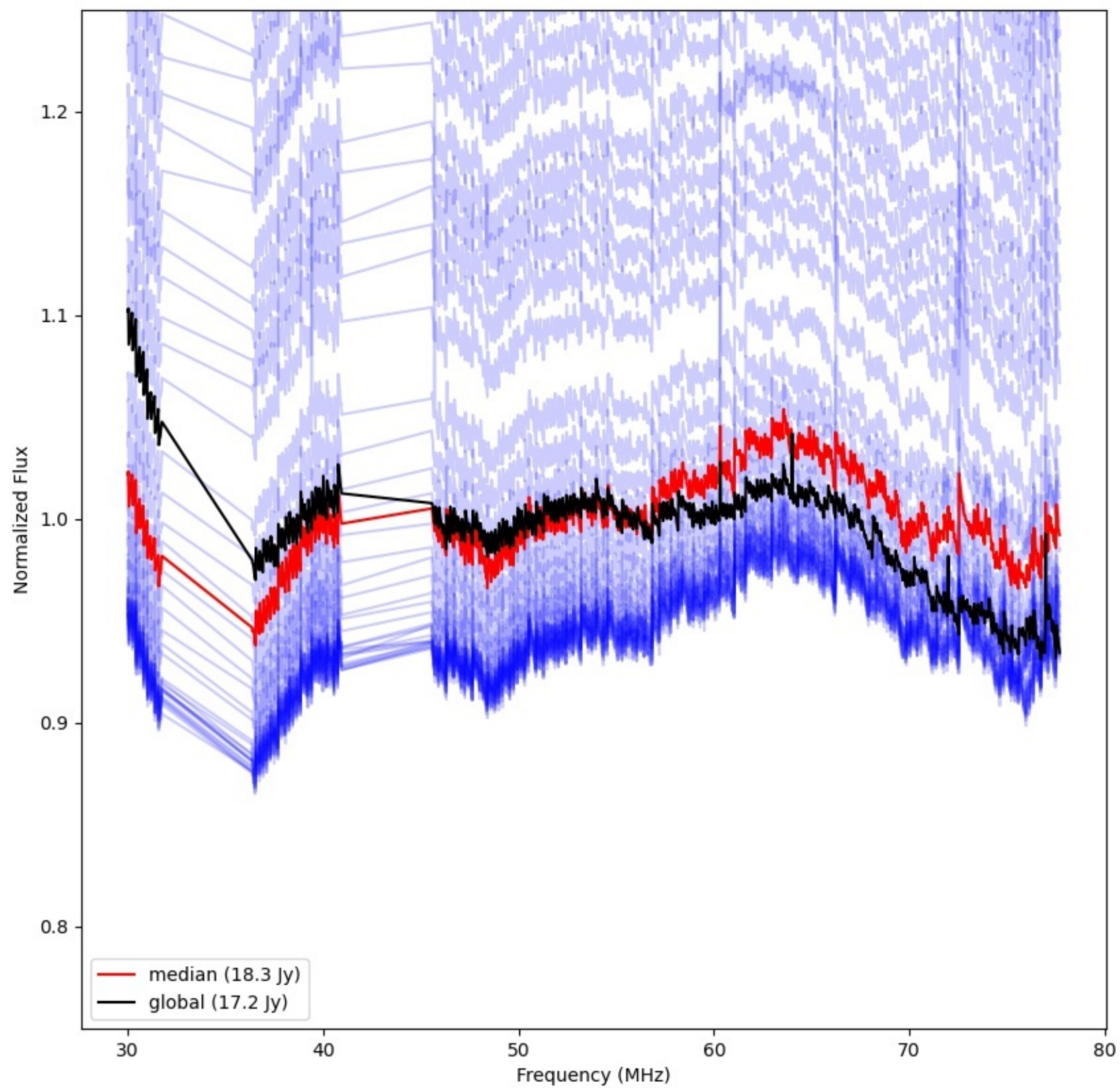
LWA069 - Correlator# 169 - YY - FLAGS:Good
