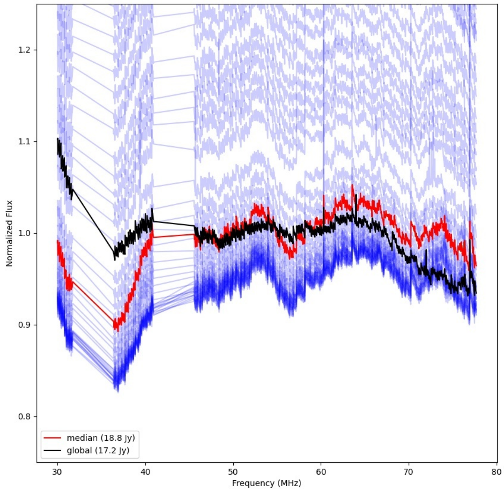
LWA118 - Correlator# 206 - YY - FLAGS:Good
