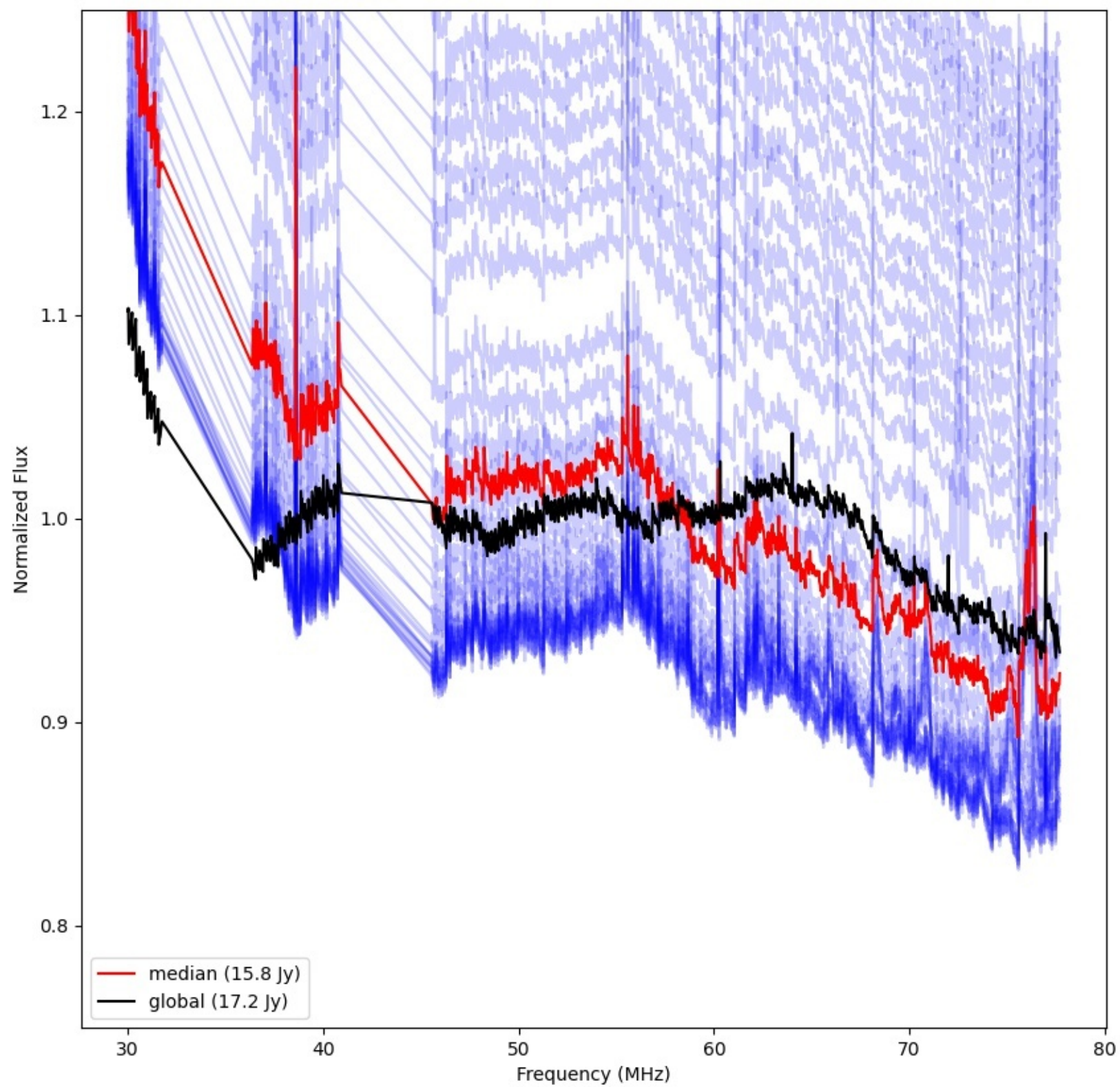
LWA341 - Correlator# 029 - YY - FLAGS:Good
