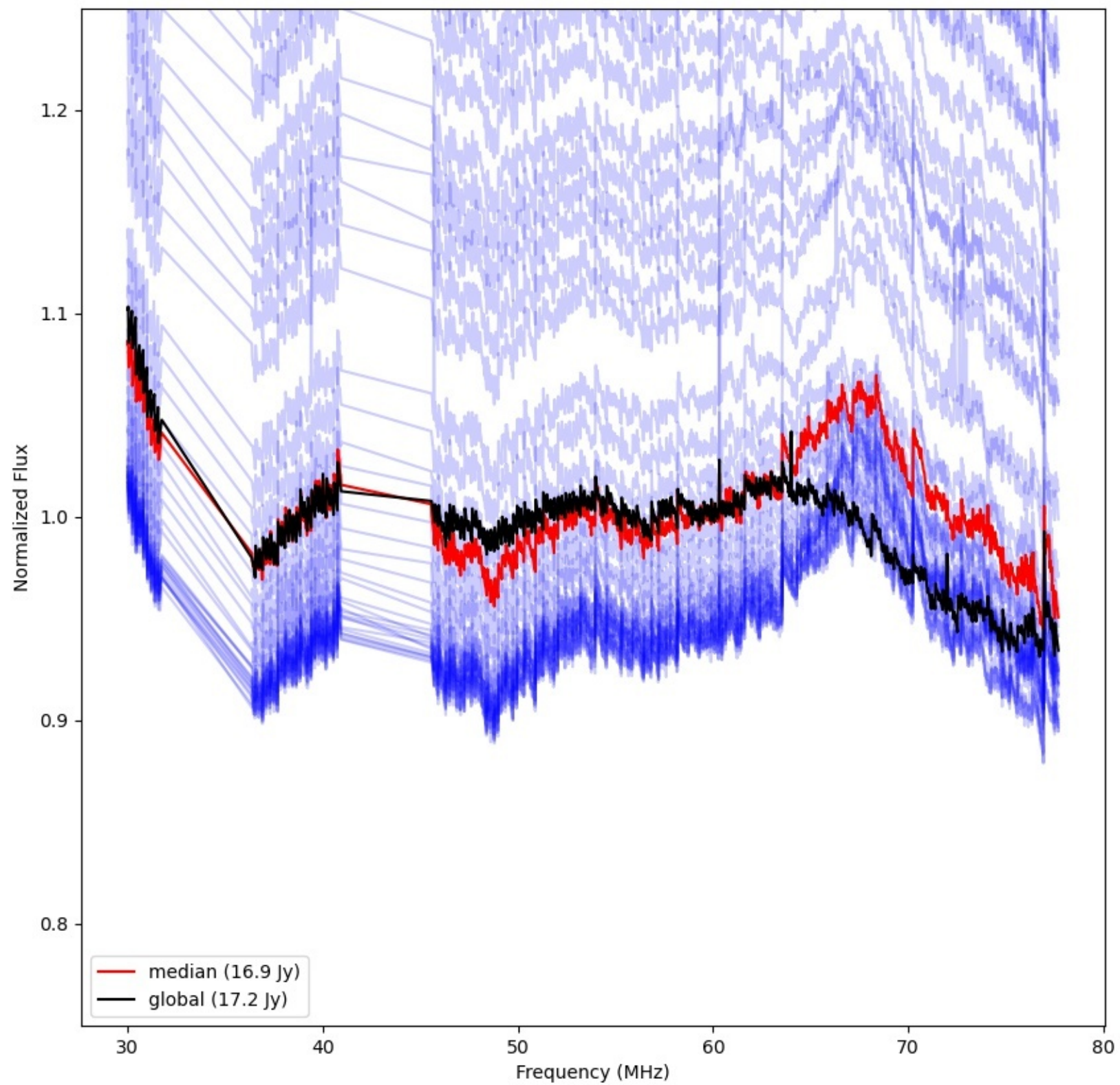
LWA149 - Correlator# 216 - YY - FLAGS:Good
