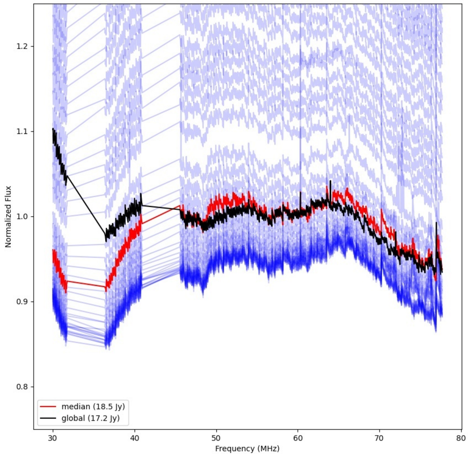
LWA114 - Correlator# 202 - YY - FLAGS:Good
