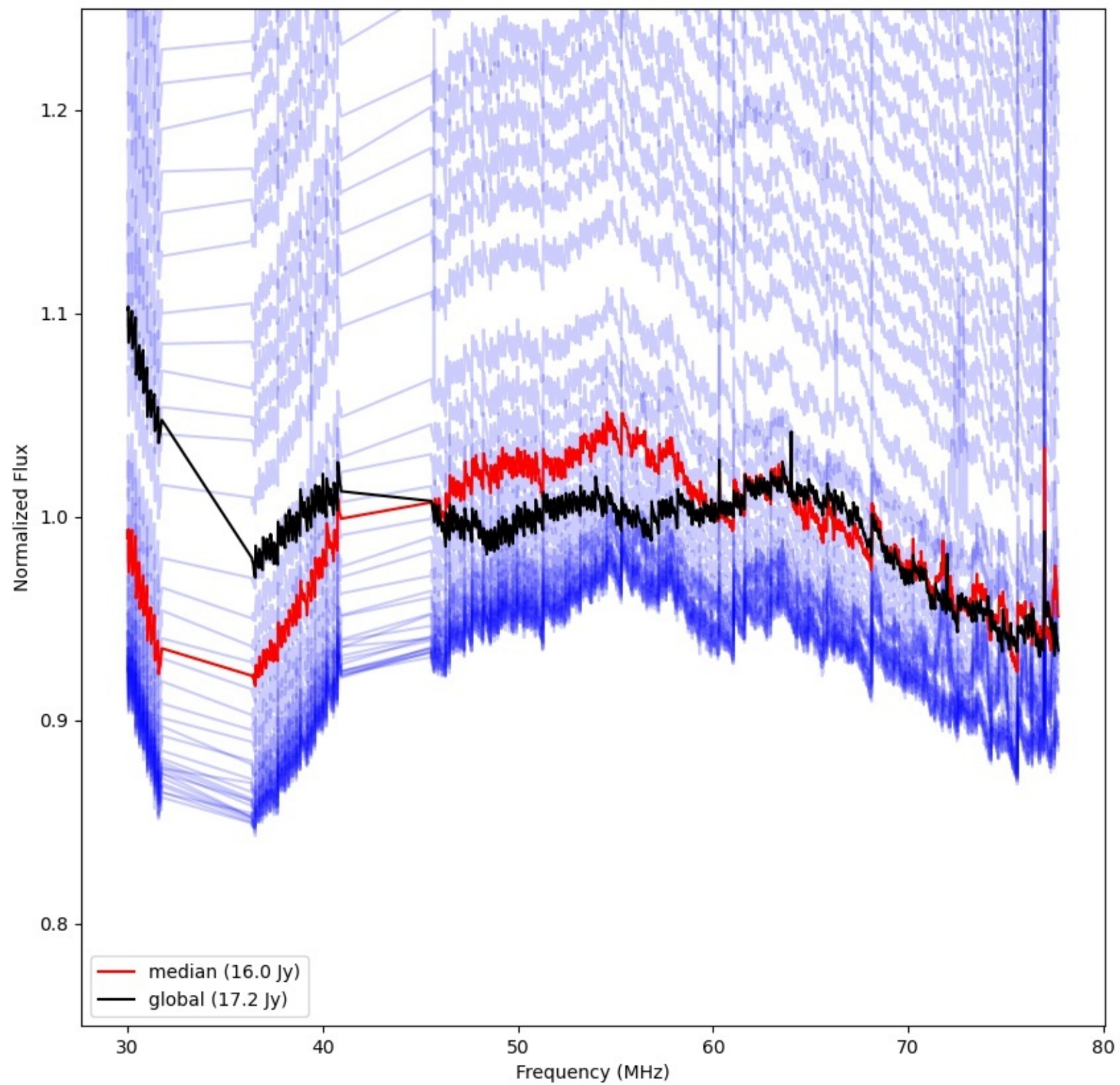
LWA339 - Correlator# 027 - YY - FLAGS:Good
