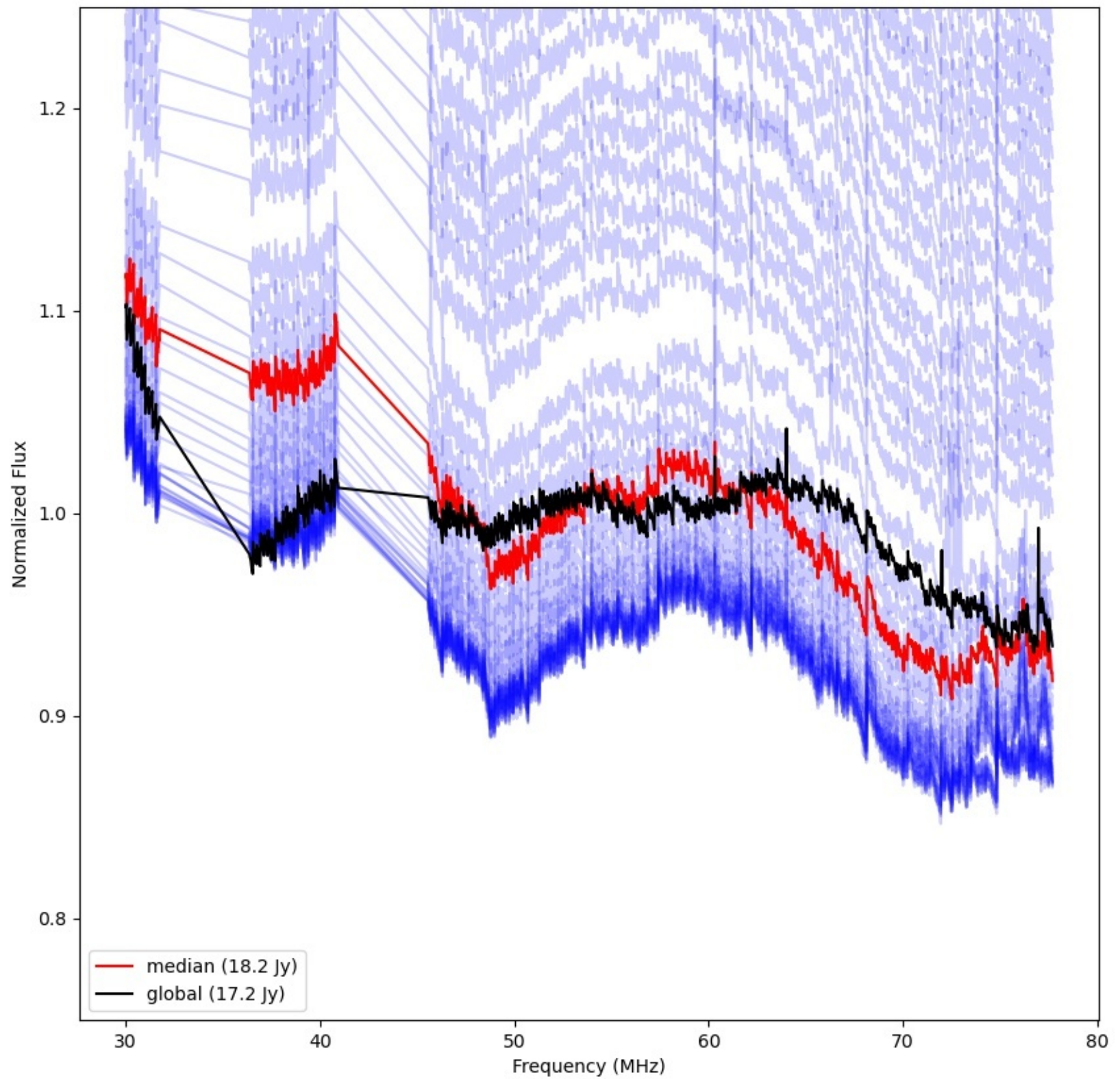
LWA012 - Correlator# 074 - YY - FLAGS:Good
