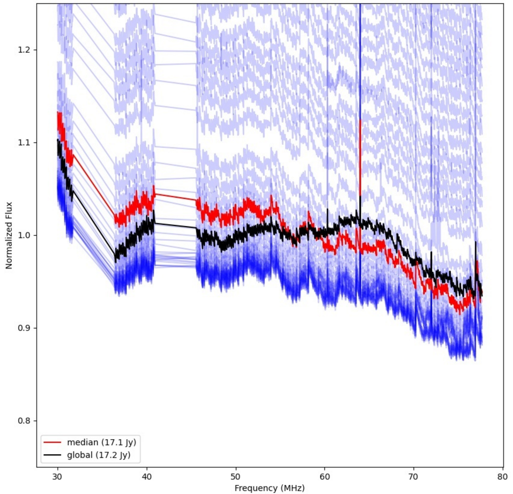
LWA031 - Correlator# 131 - YY - FLAGS:Good
