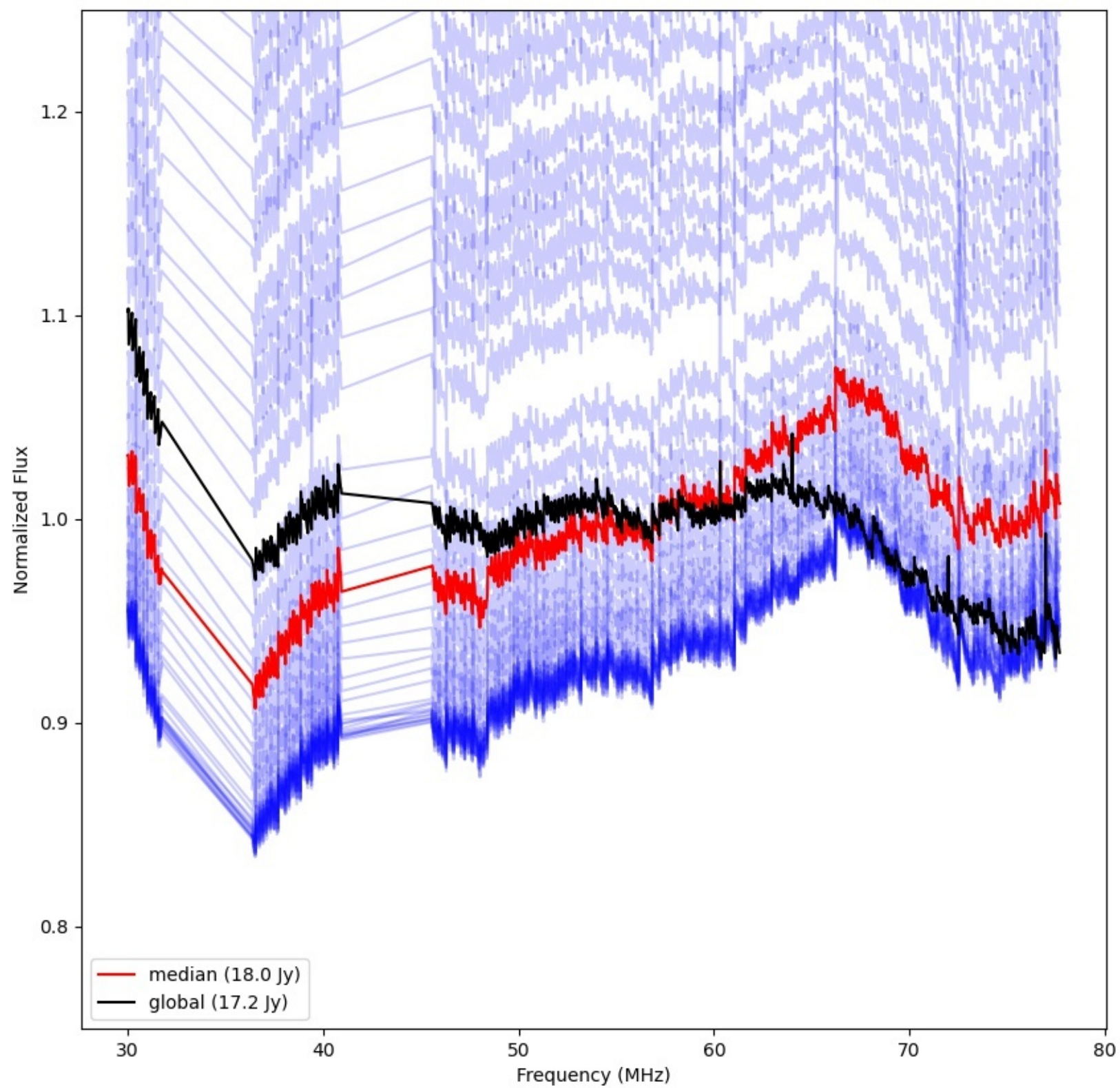
LWA164 - Correlator# 267 - YY - FLAGS:Good
