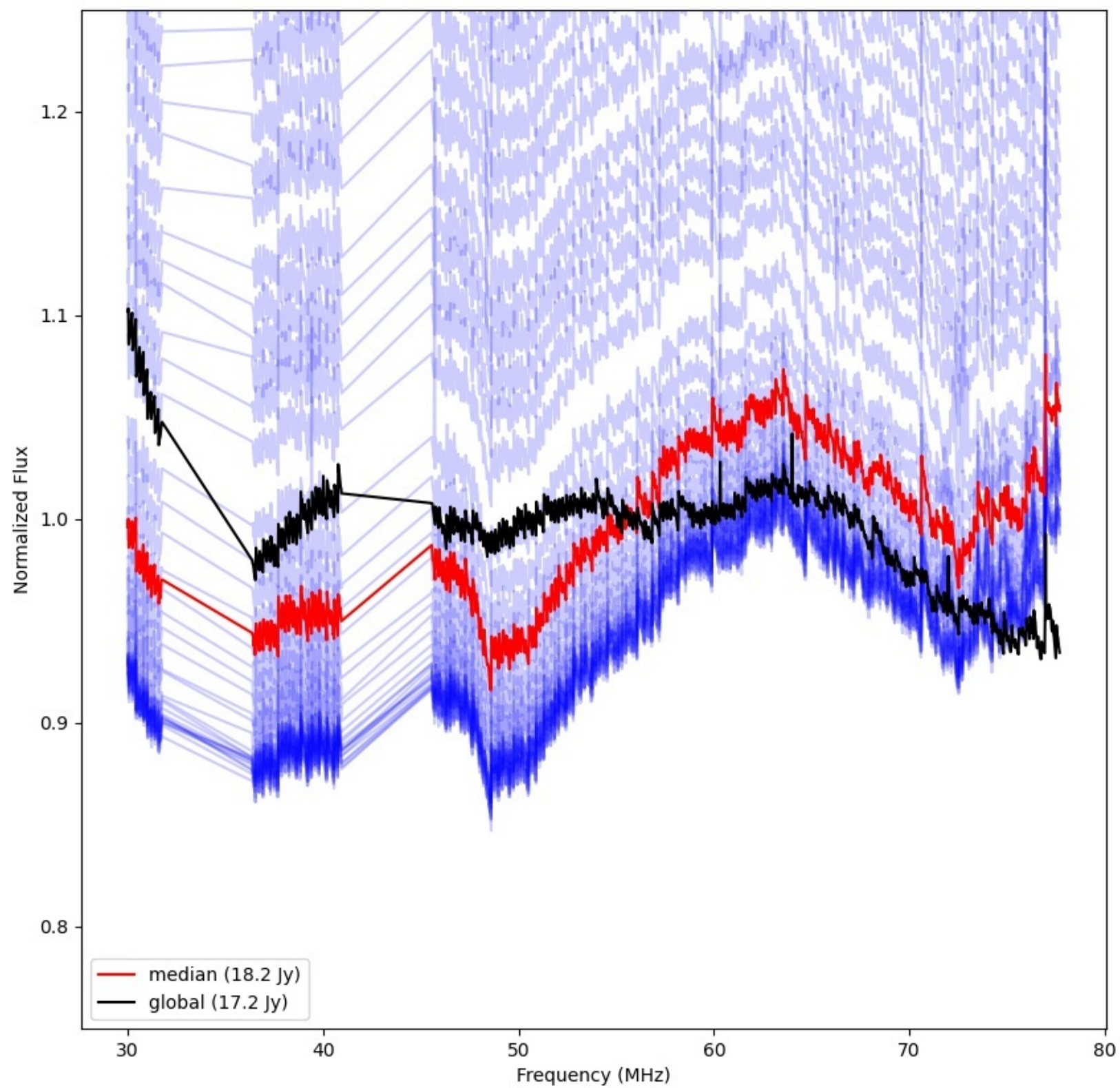
LWA001 - Correlator# 065 - YY - FLAGS:Good
