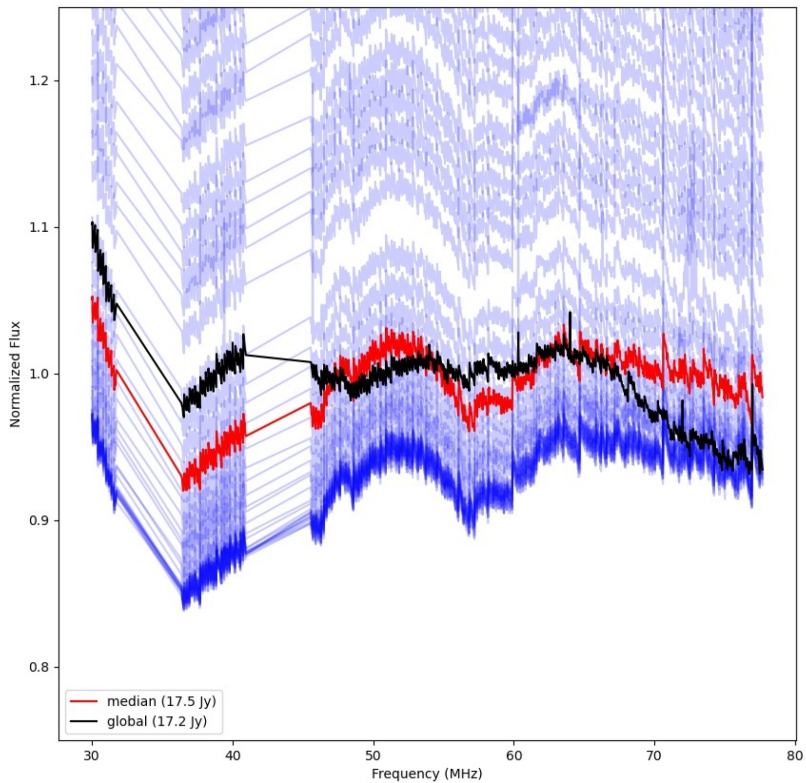
LWA193 - Correlator# 270 - YY - FLAGS:Good
