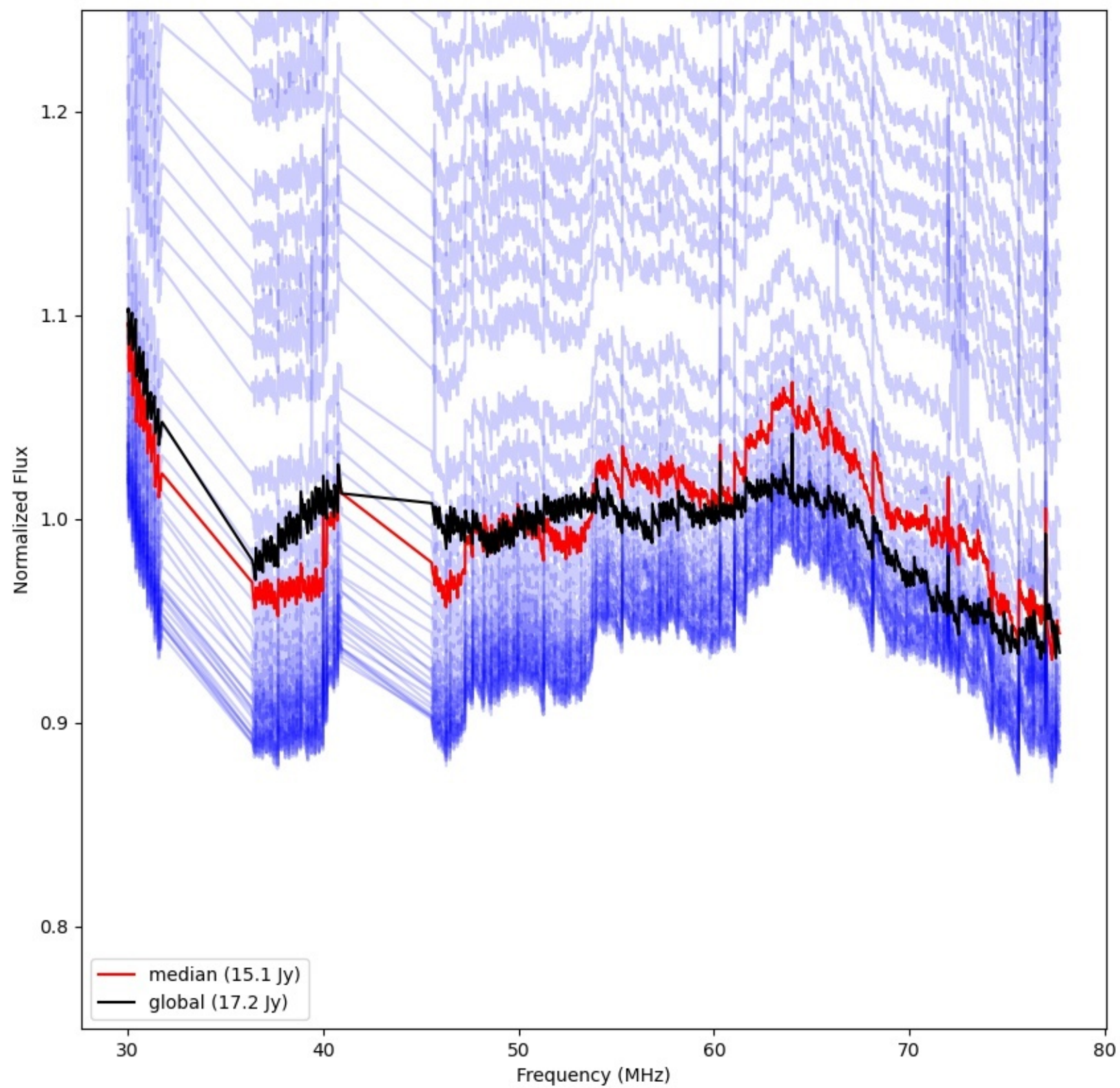
LWA361 - Correlator# 158 - YY - FLAGS:Good
