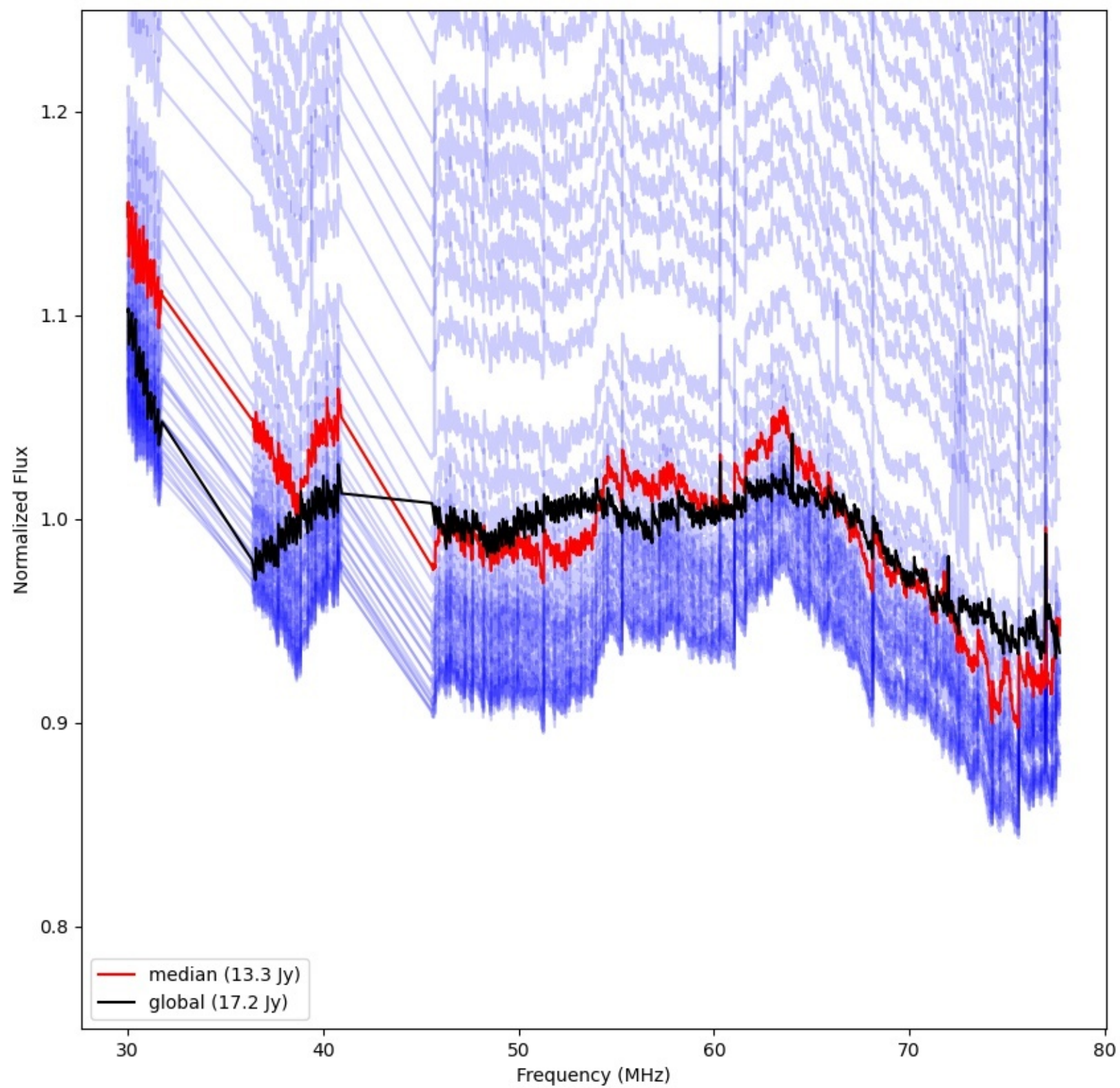
LWA293 - Correlator# 284 - YY - FLAGS:Good
