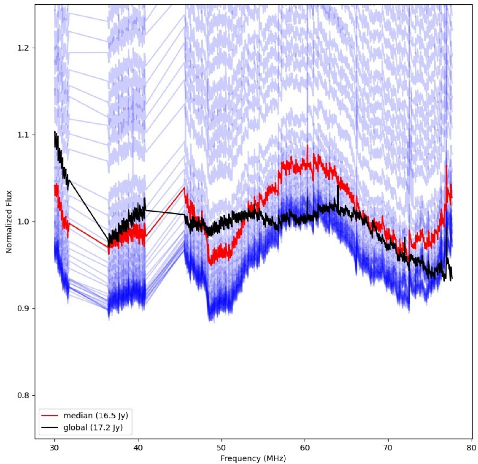
LWA005 - Correlator# 069 - YY - FLAGS:Good
