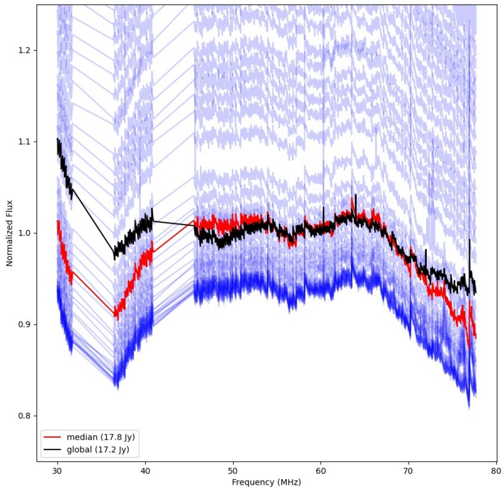
LWA079 - Correlator# 195 - YY - FLAGS:Good
