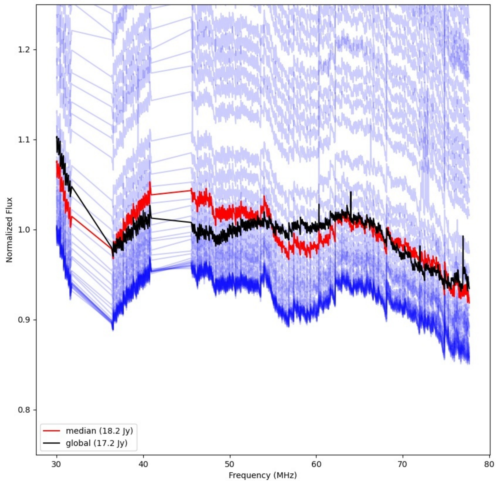
LWA103 - Correlator# 176 - YY - FLAGS:Good
