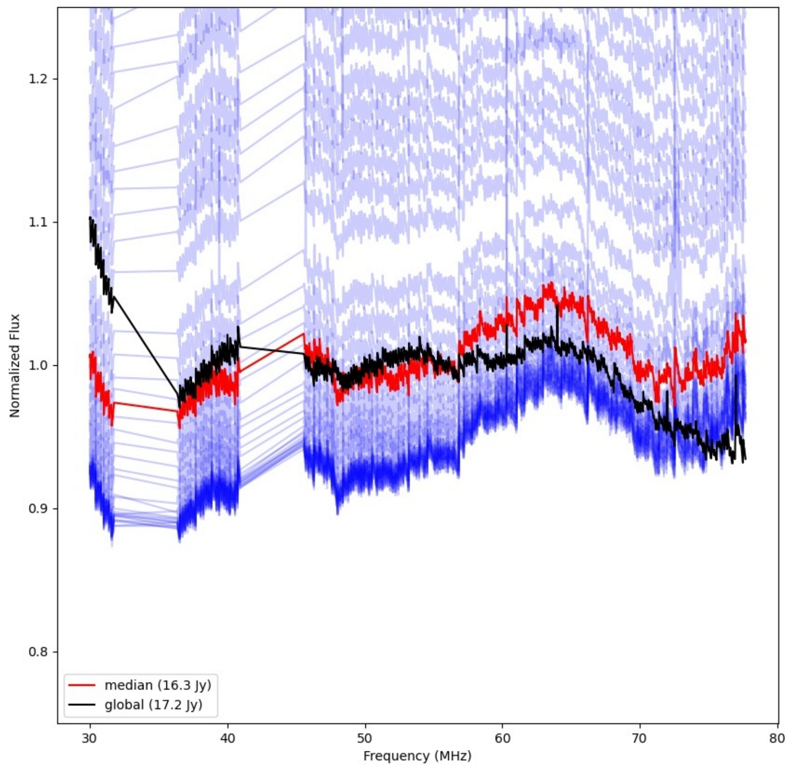
LWA099 - Correlator# 172 - YY - FLAGS:Good
