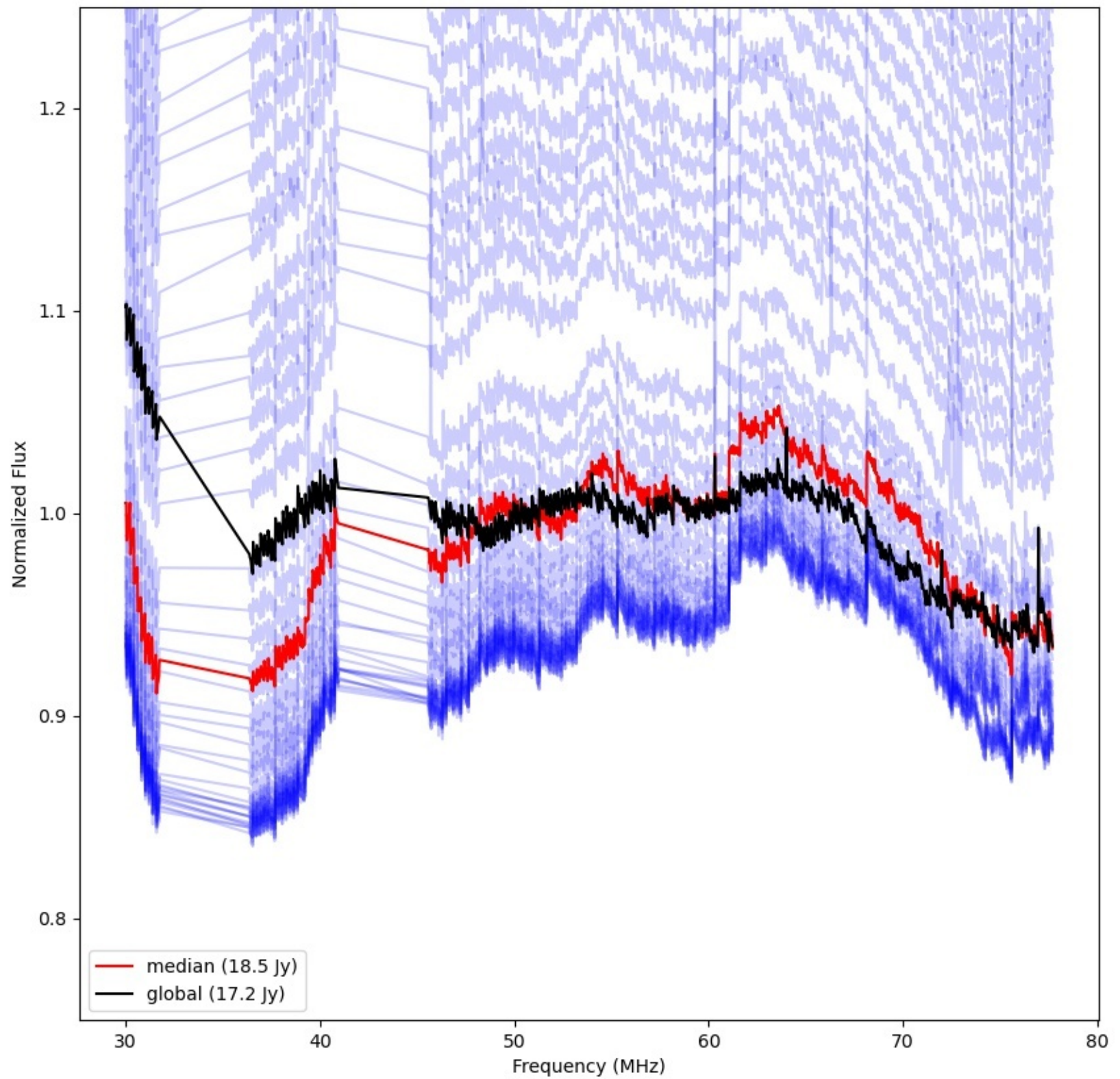
LWA324 - Correlator# 122 - YY - FLAGS:Good
