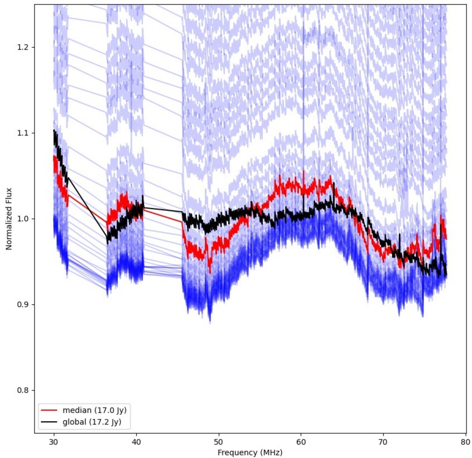
LWA074 - Correlator# 086 - YY - FLAGS:Good
