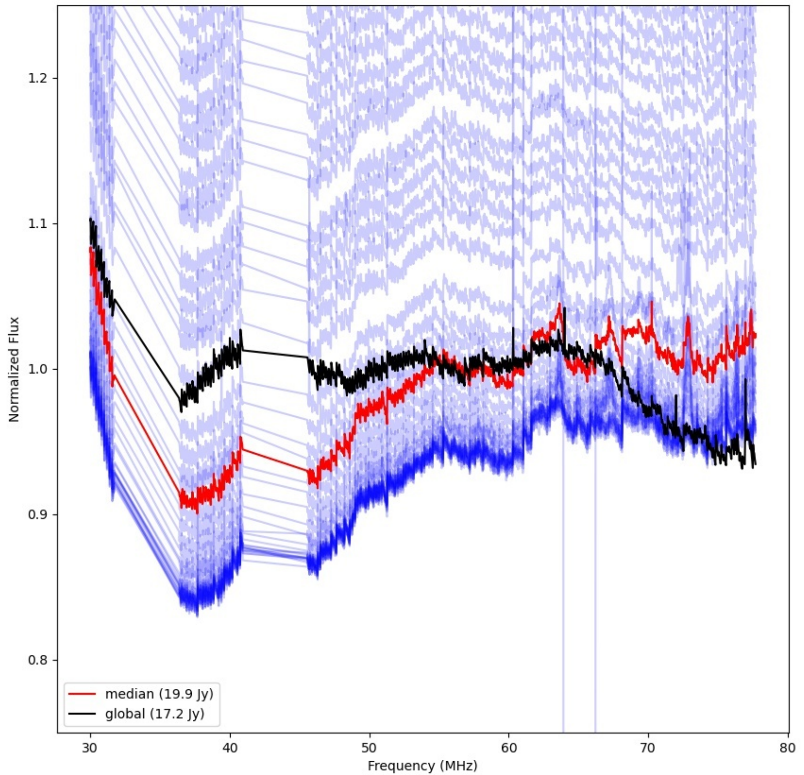
LWA352 - Correlator# 028 - YY - FLAGS:Good
