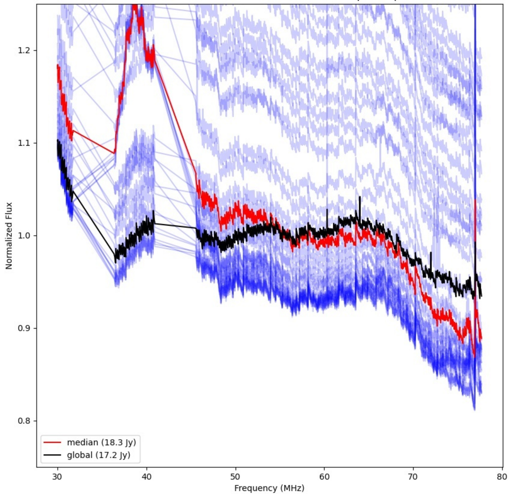
LWA172 - Correlator# 219 - YY - FLAGS:BadSpecShape
