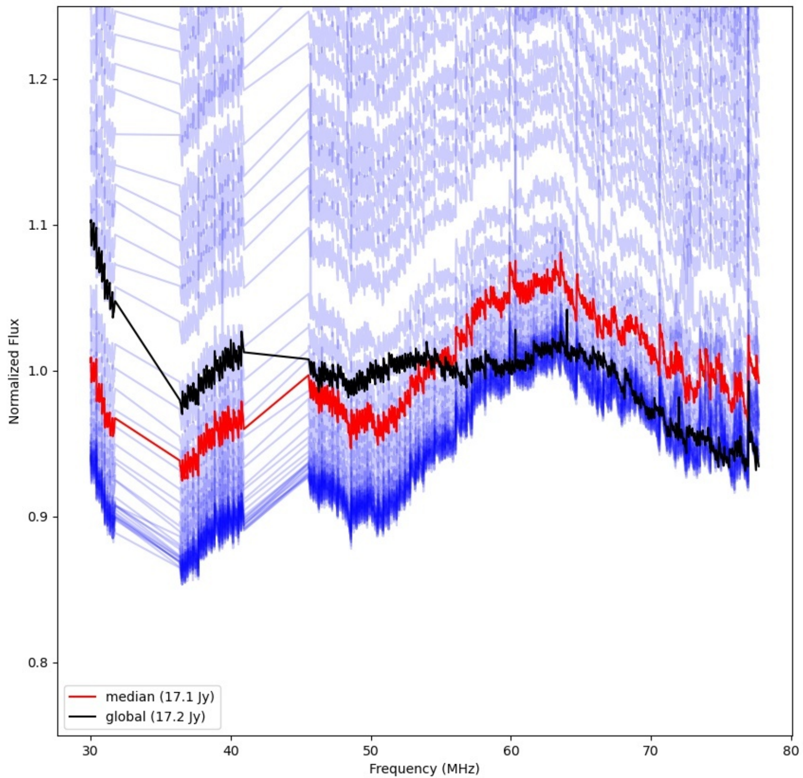
LWA066 - Correlator# 164 - YY - FLAGS:Good
