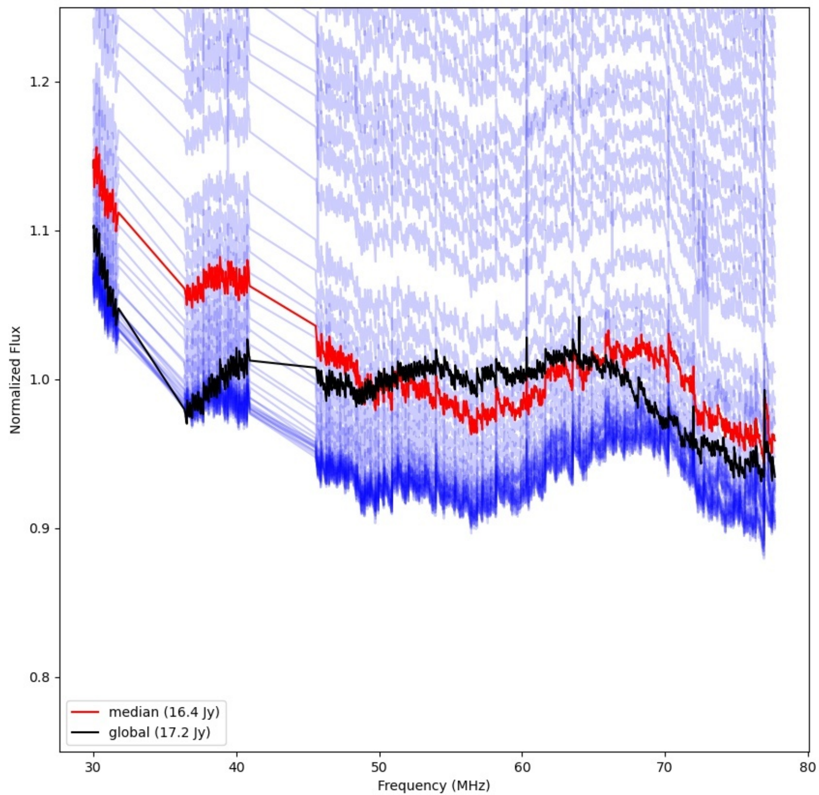
LWA219 - Correlator# 335 - YY - FLAGS:Good
