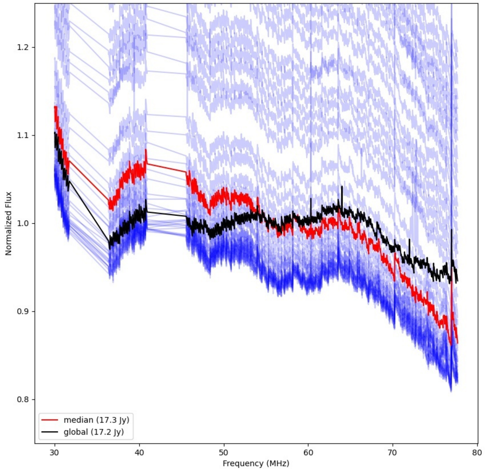
LWA145 - Correlator# 212 - YY - FLAGS:Good
