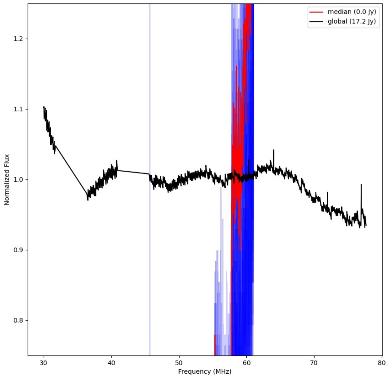
LWA314 - Correlator# 021 - YY - FLAGS:LowFlux
