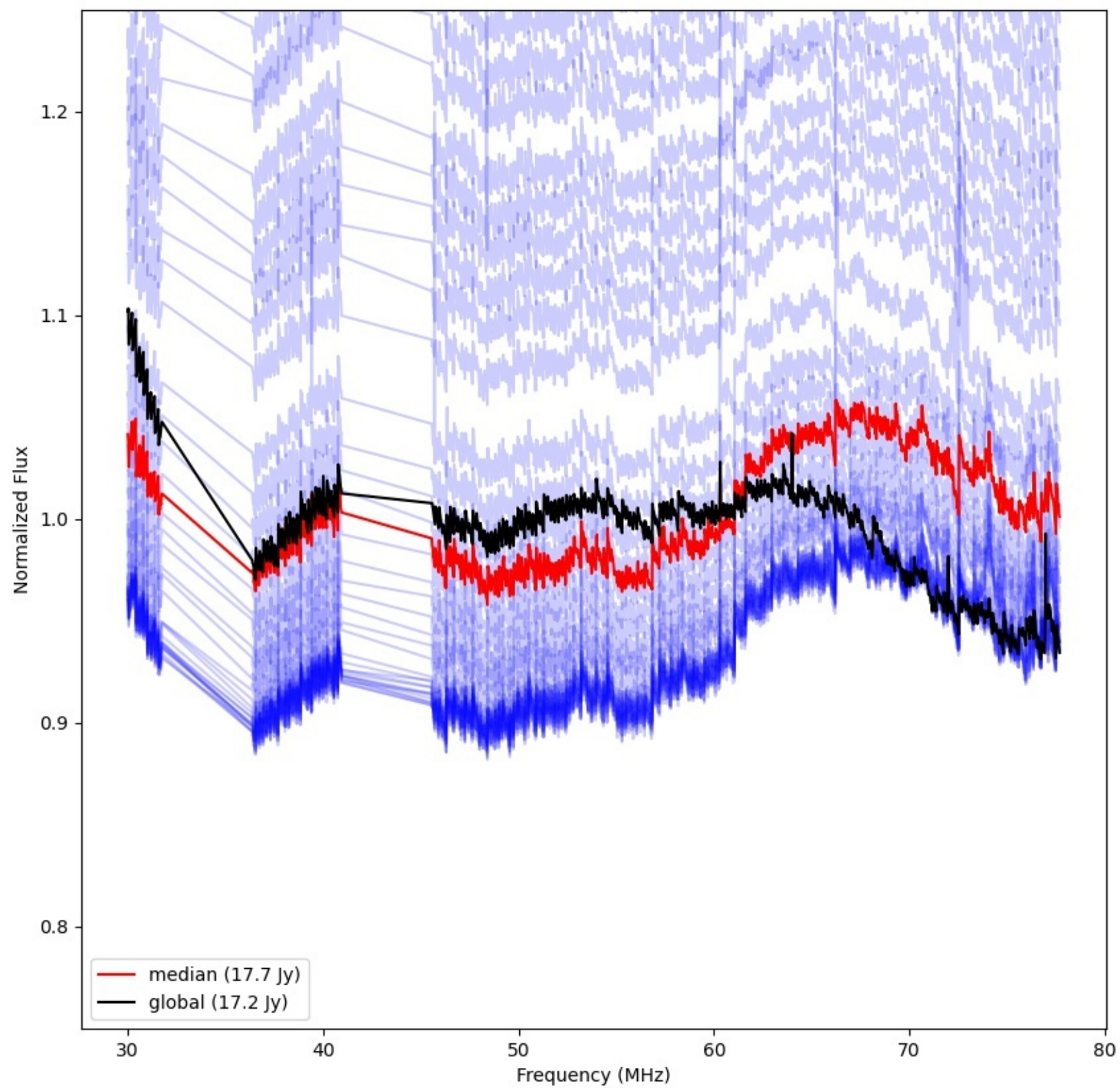
LWA229 - Correlator# 305 - YY - FLAGS:Good
