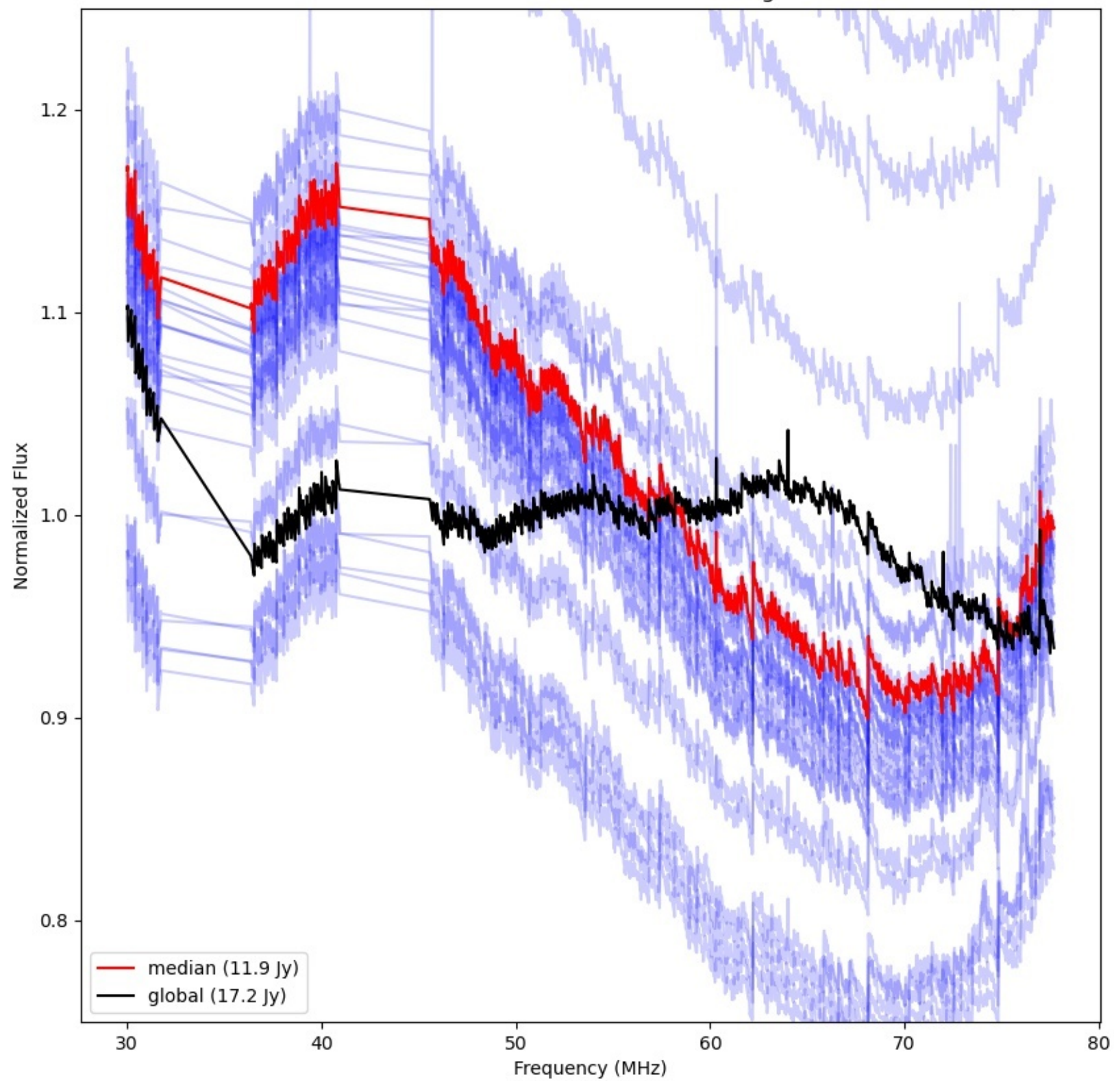
LWA044 - Correlator# 080 - YY - FLAGS:HighTimeVar
