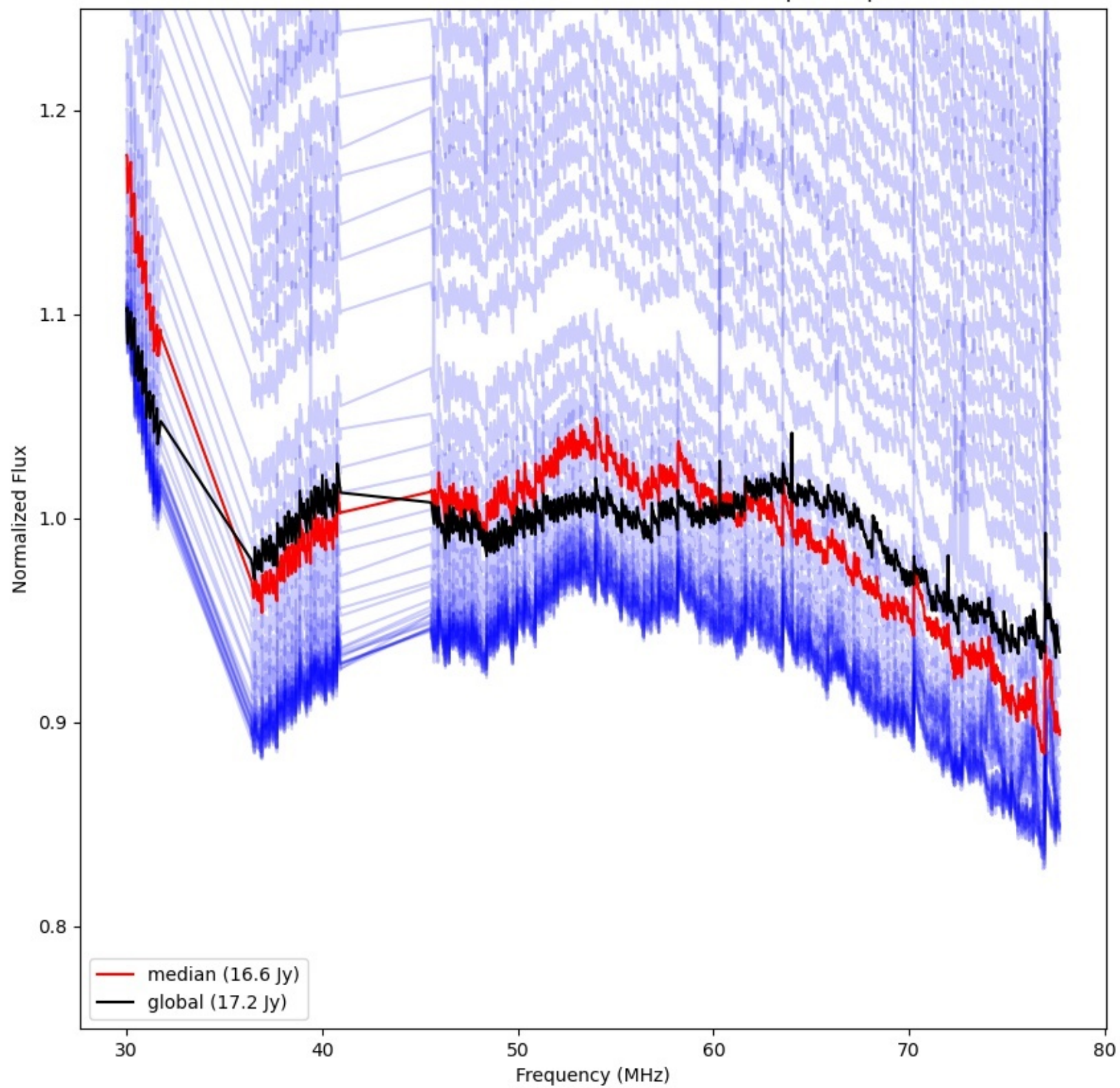
LWA052 - Correlator# 117 - YY - FLAGS:BadSpecShape
