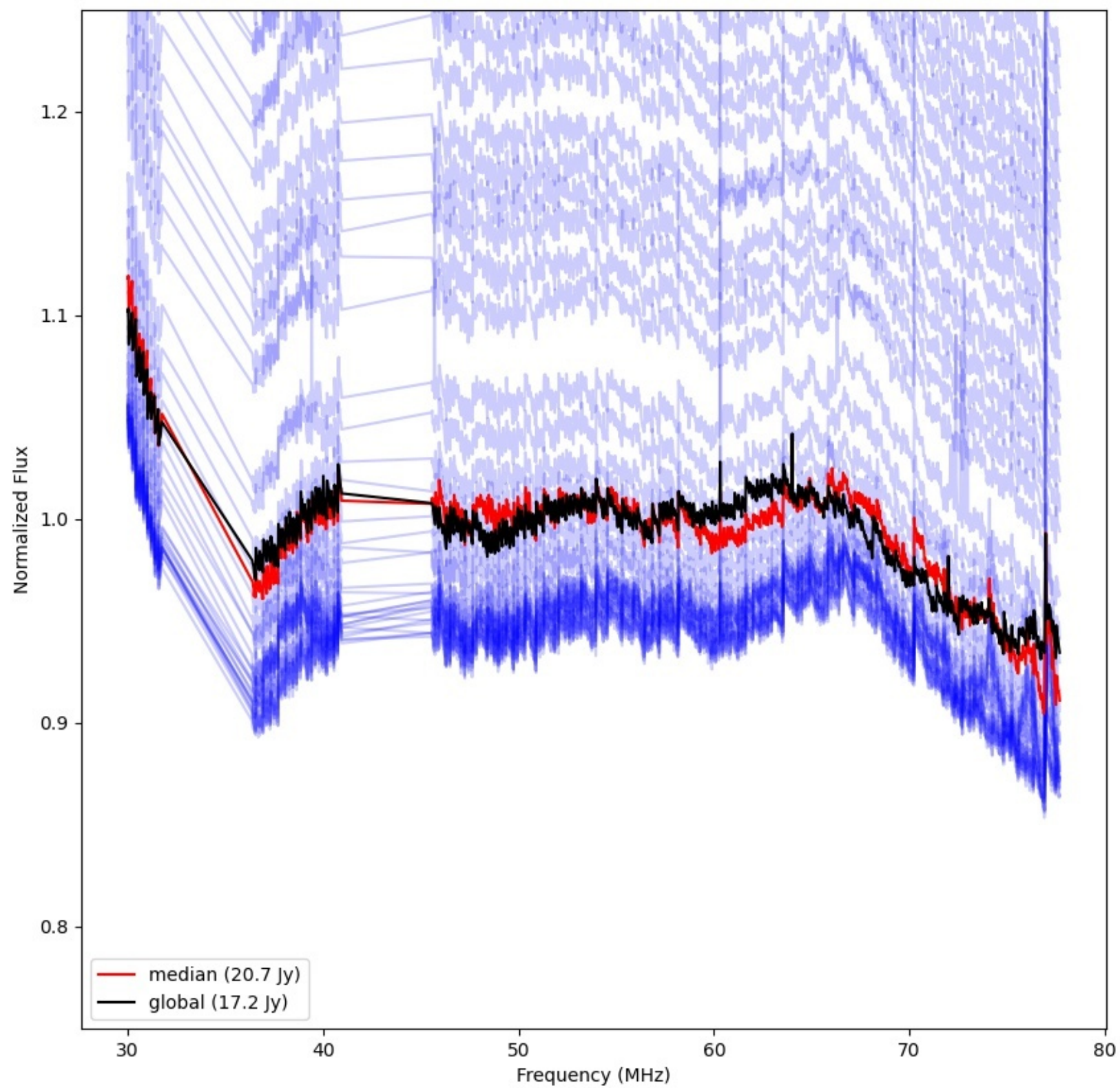
LWA148 - Correlator# 217 - YY - FLAGS:Good
