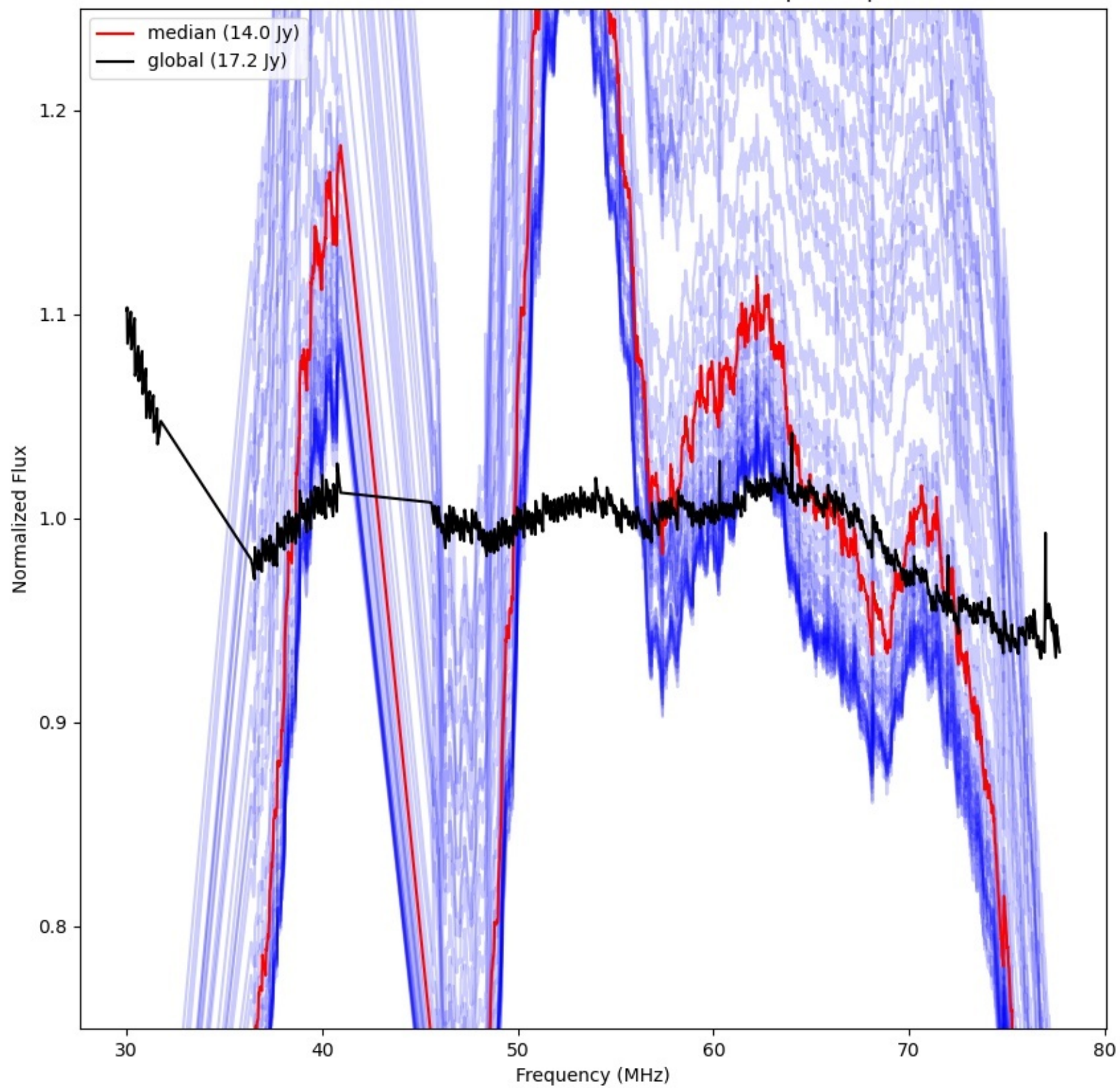
LWA142 - Correlator# 211 - YY - FLAGS:BadSpecShape
