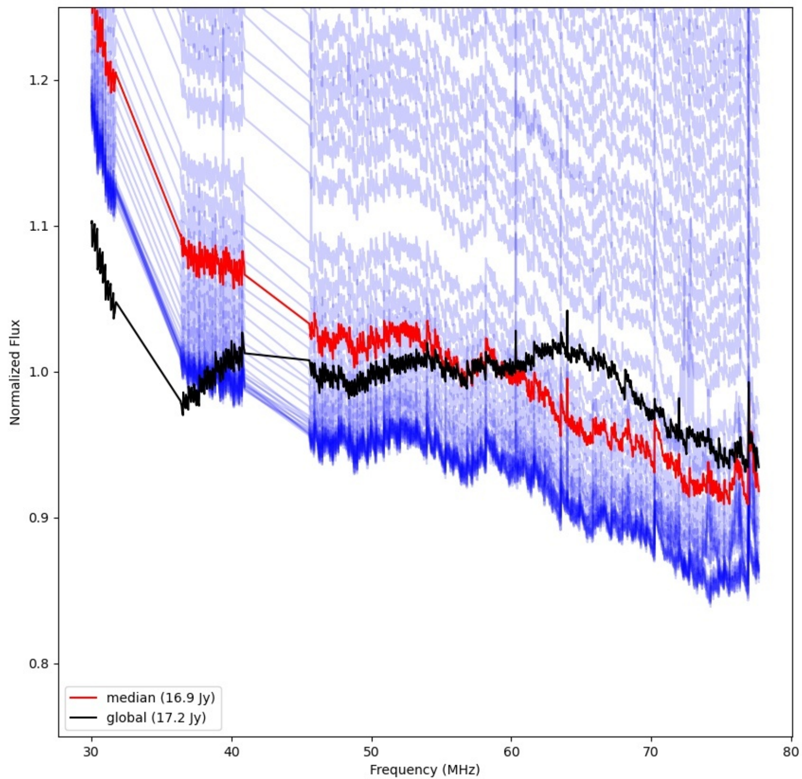
LWA050 - Correlator# 115 - YY - FLAGS:Good
