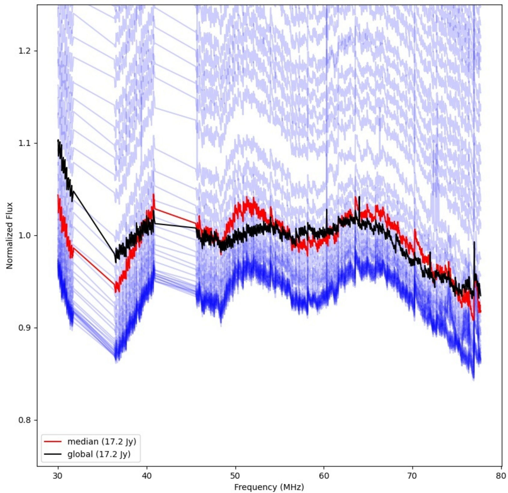
LWA117 - Correlator# 207 - YY - FLAGS:Good
