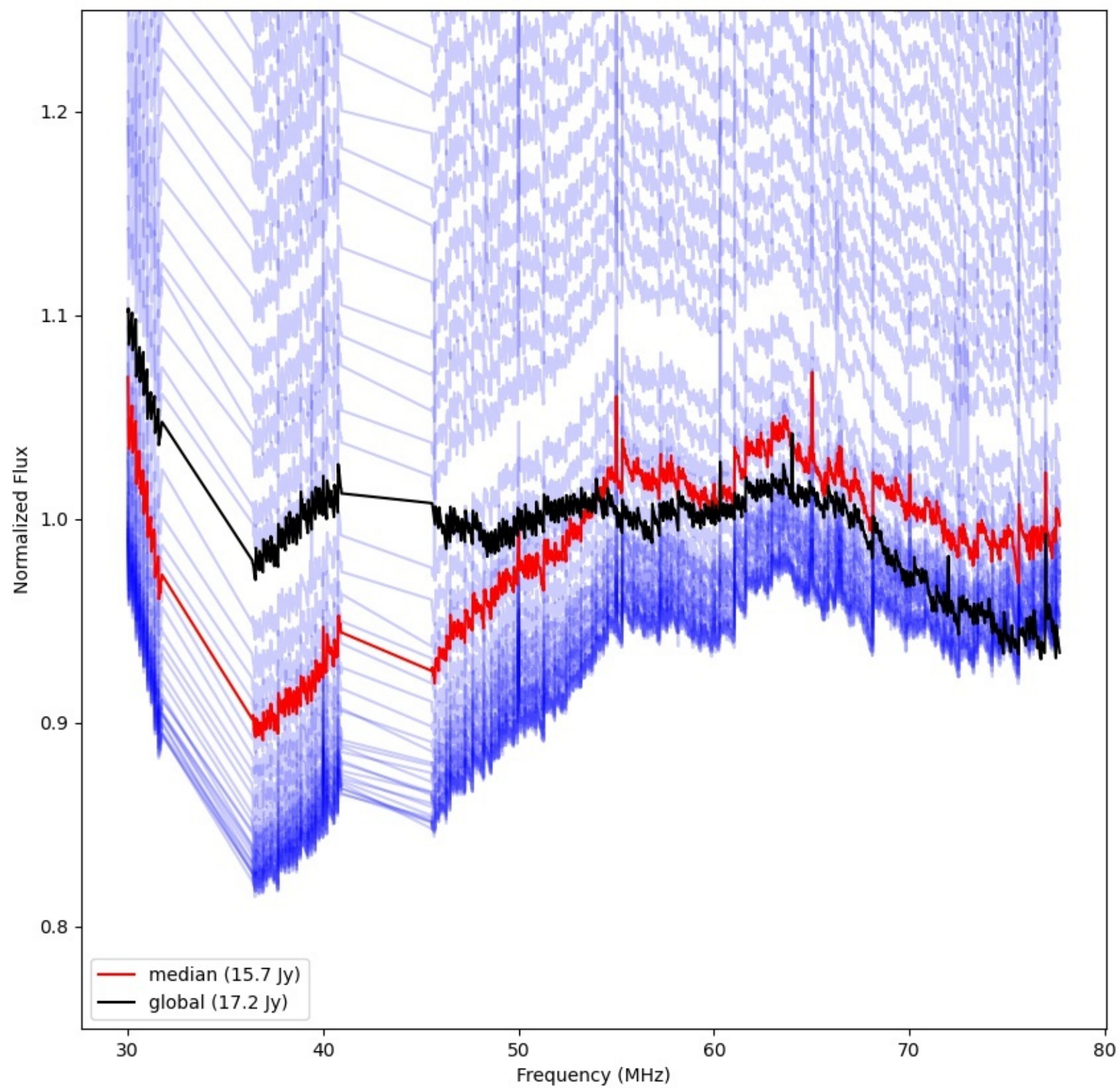
LWA362 - Correlator# 030 - YY - FLAGS:Good
