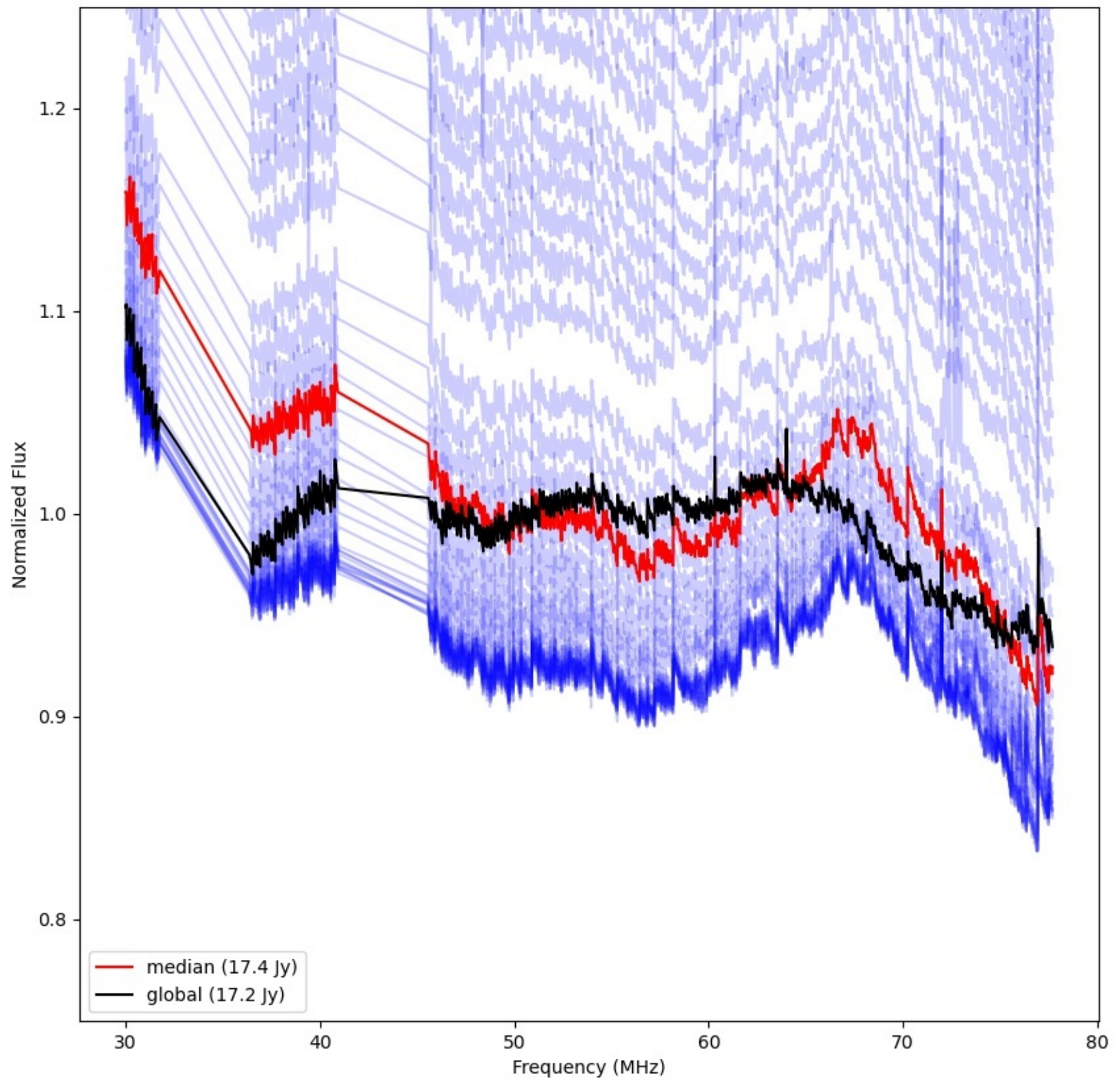
LWA248 - Correlator# 343 - YY - FLAGS:Good
