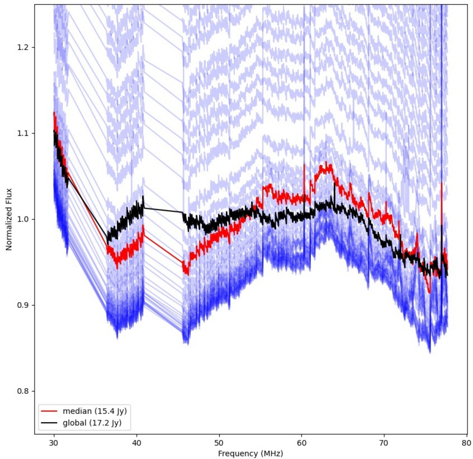
LWA350 - Correlator# 319 - YY - FLAGS:Good
