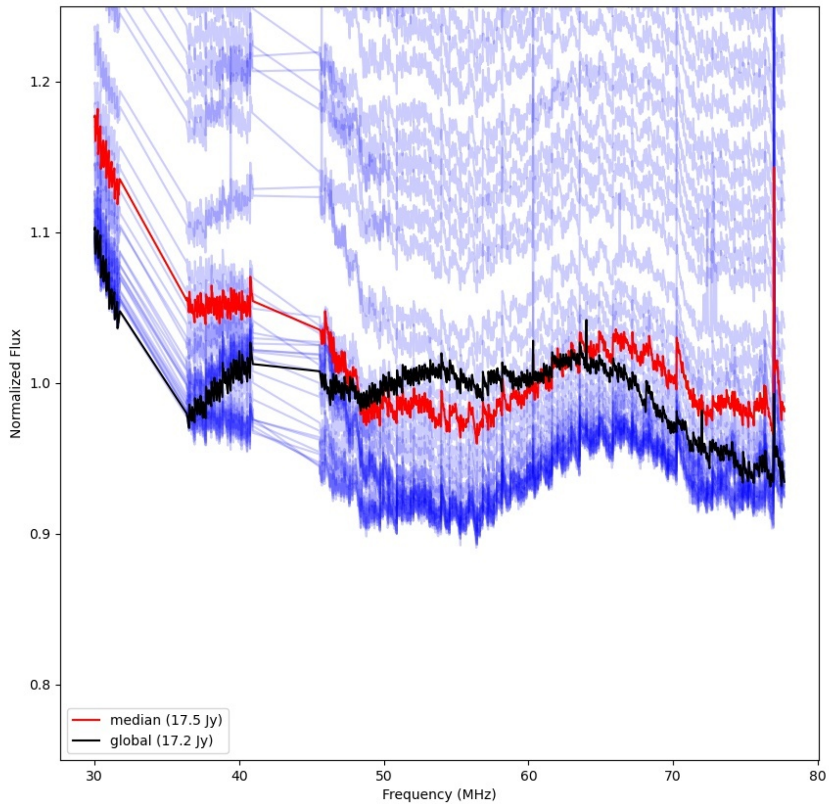
LWA151 - Correlator# 218 - YY - FLAGS:Good
