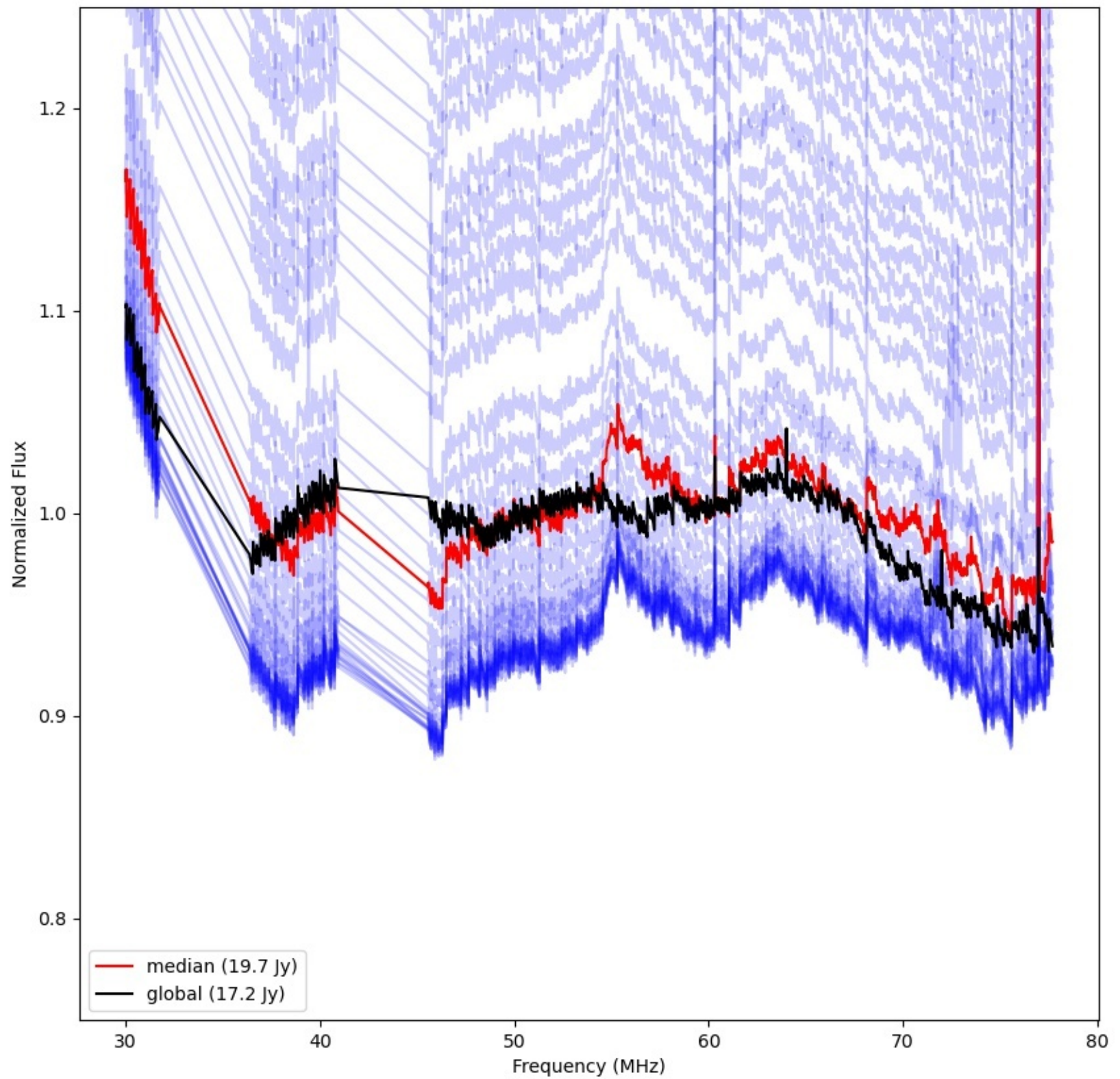
LWA332 - Correlator# 025 - YY - FLAGS:Good
