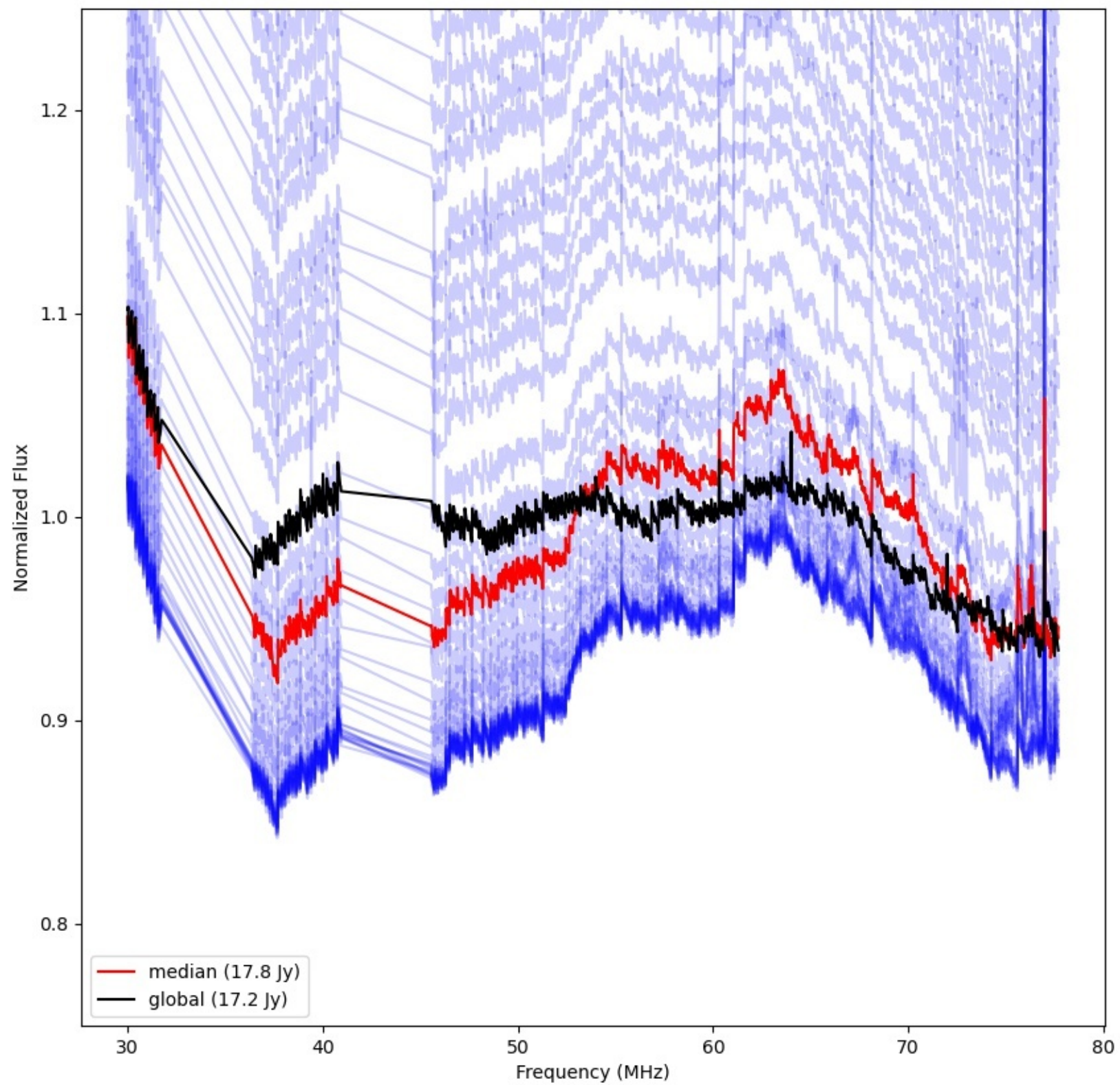
LWA328 - Correlator# 157 - YY - FLAGS:Good
