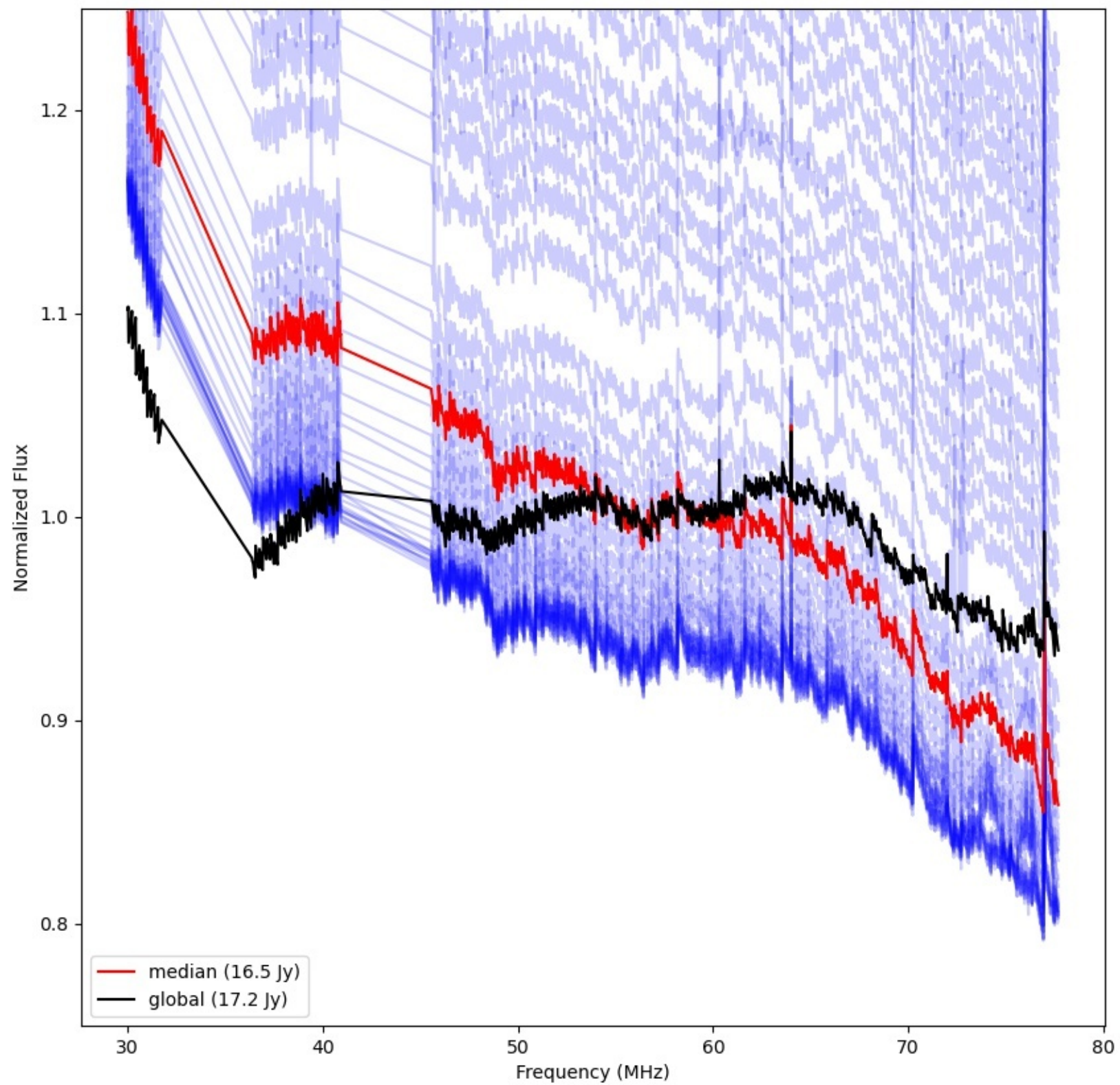
LWA022 - Correlator# 104 - YY - FLAGS:Good
