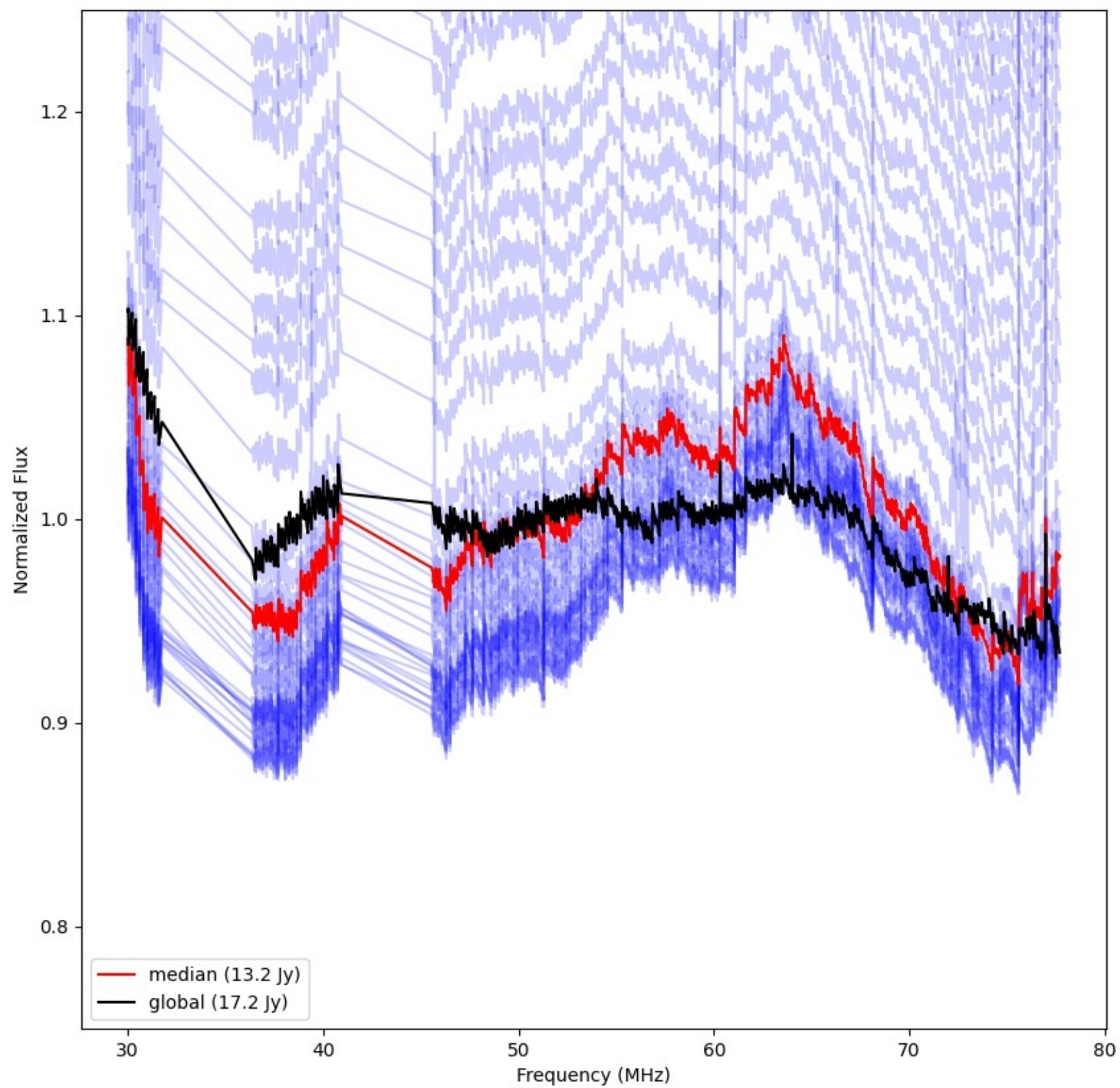
LWA297 - Correlator# 314 - YY - FLAGS:Good
