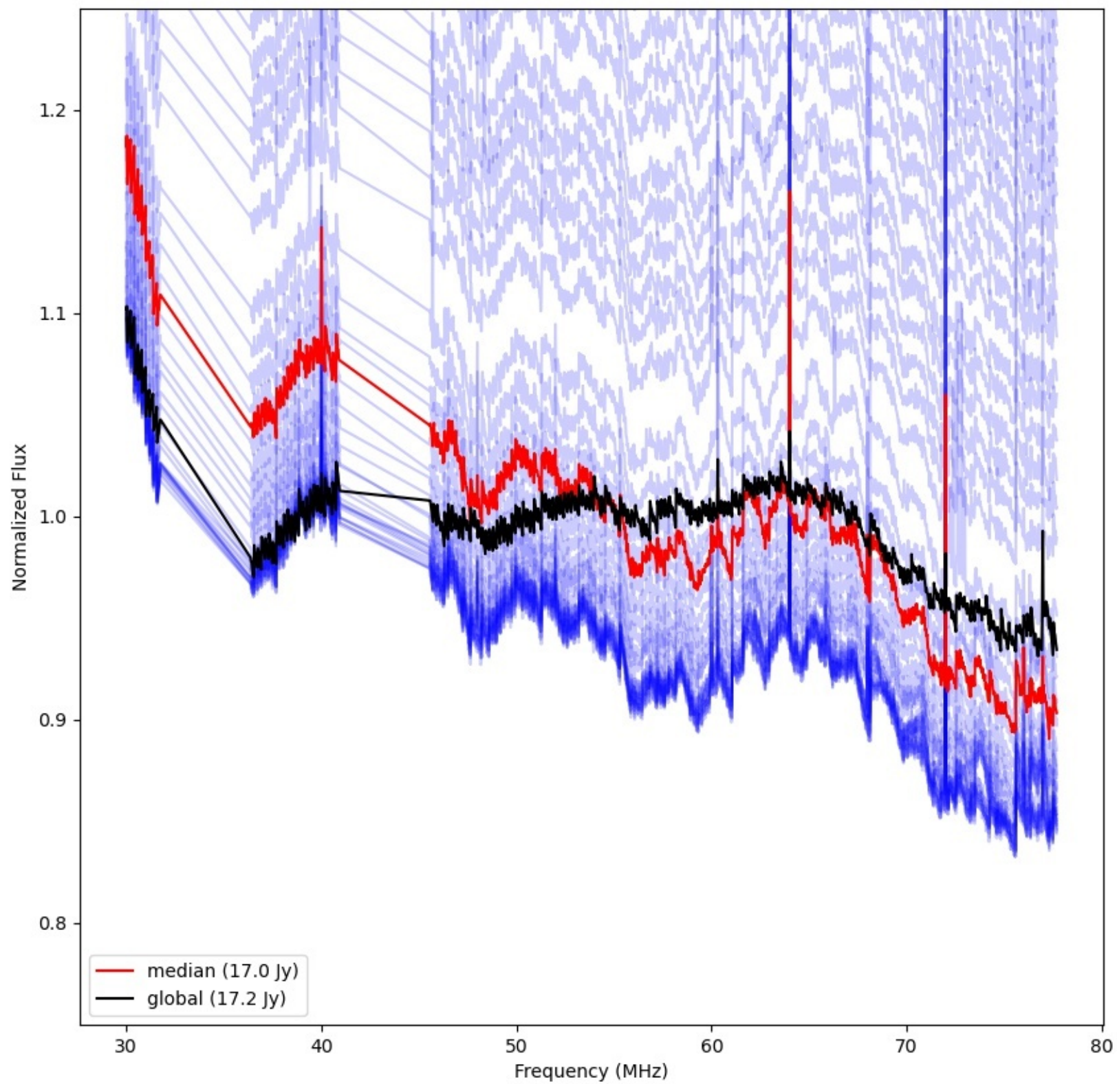
LWA189 - Correlator# 245 - YY - FLAGS:Good
