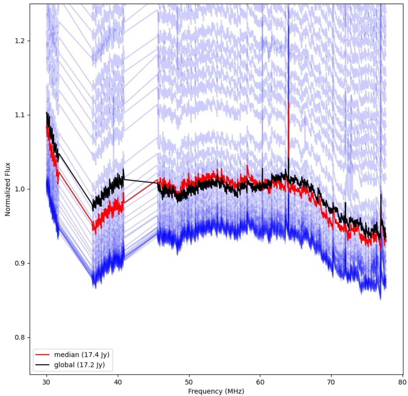
LWA028 - Correlator# 129 - YY - FLAGS:Good
