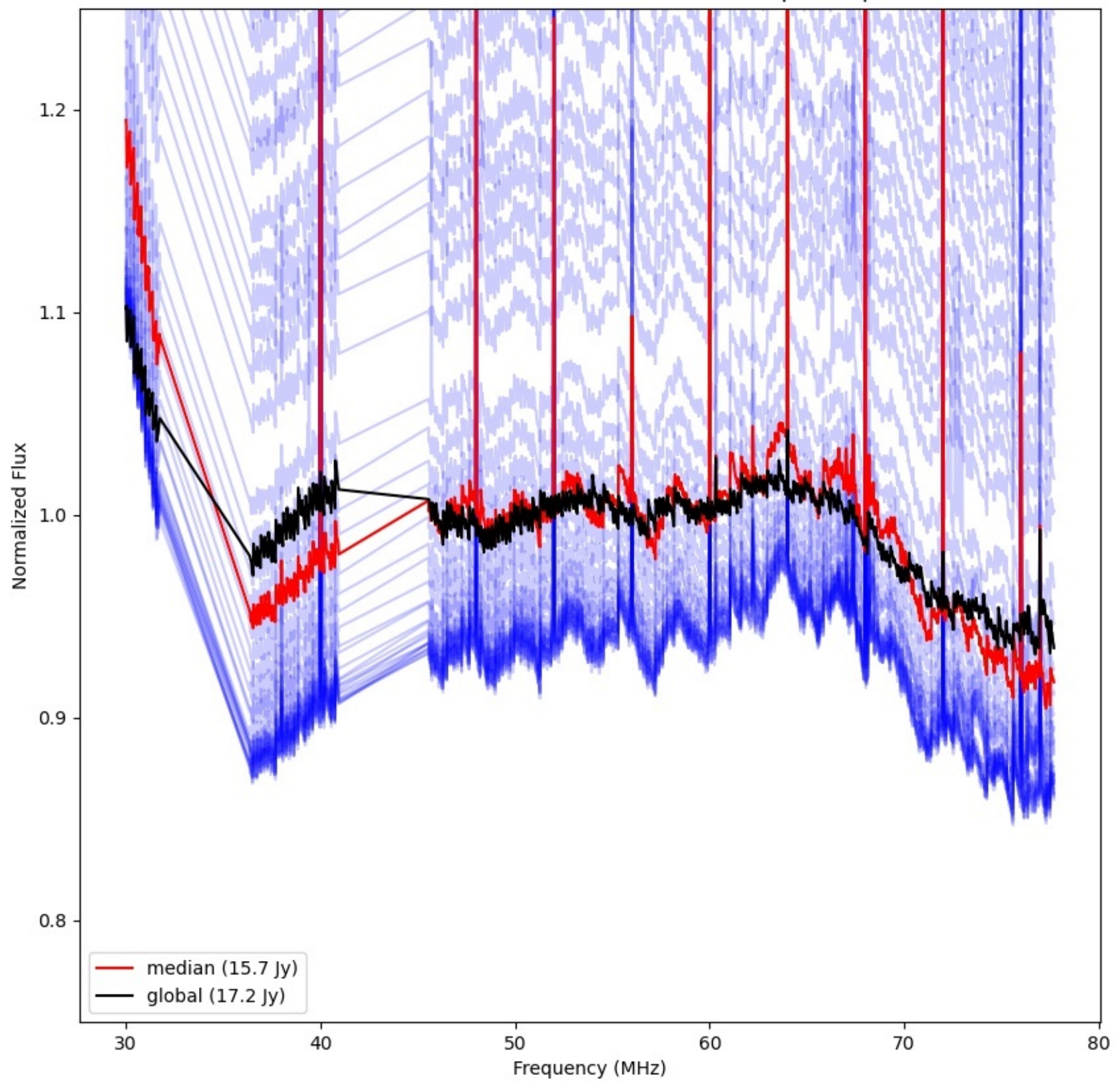
LWA160 - Correlator# 239 - YY - FLAGS:BadSpecShape
