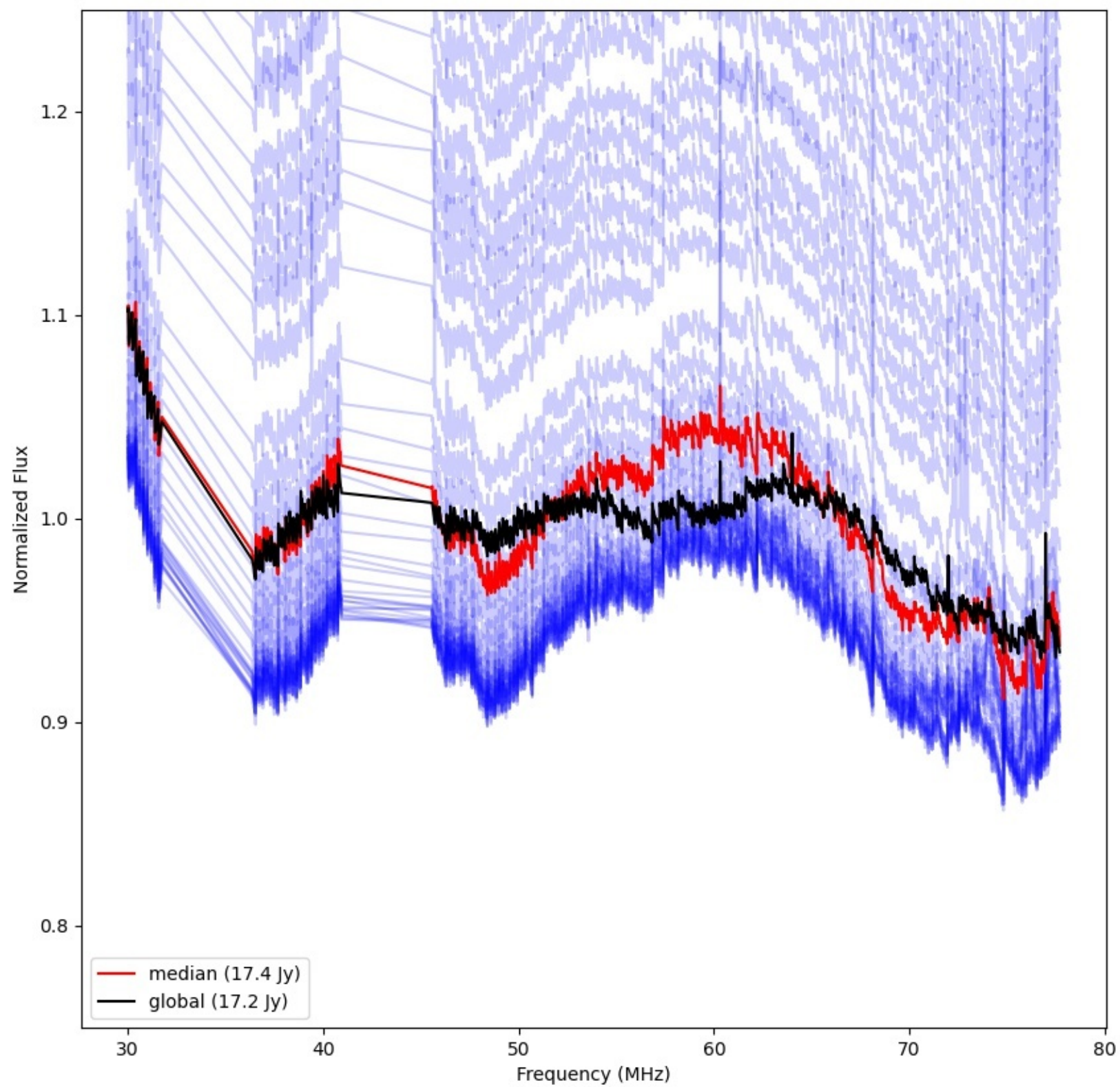
LWA073 - Correlator# 087 - YY - FLAGS:Good
