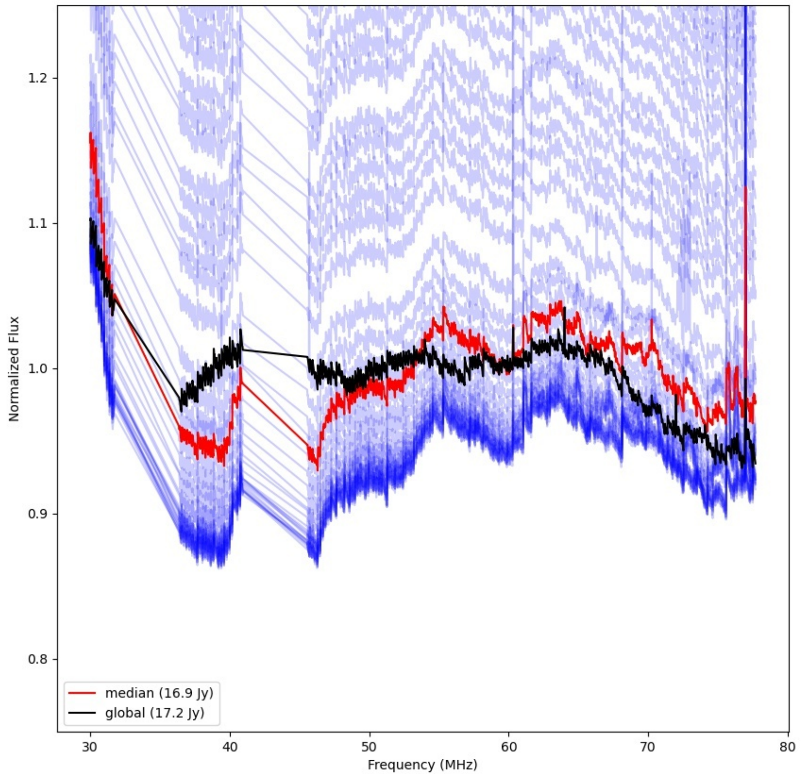
LWA312 - Correlator# 019 - YY - FLAGS:Good
