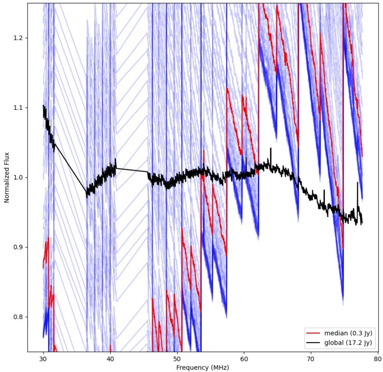
LWA204 - Correlator# 294 - YY - FLAGS:LowFlux
