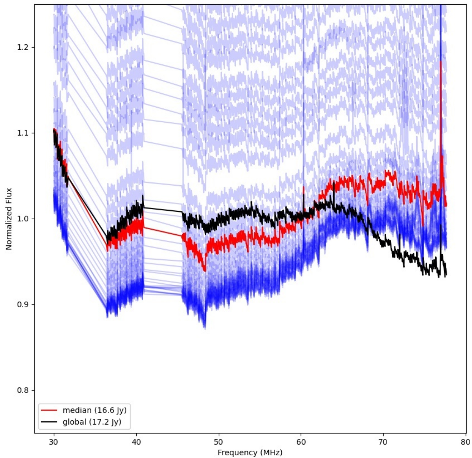
LWA239 - Correlator# 313 - YY - FLAGS:Good
