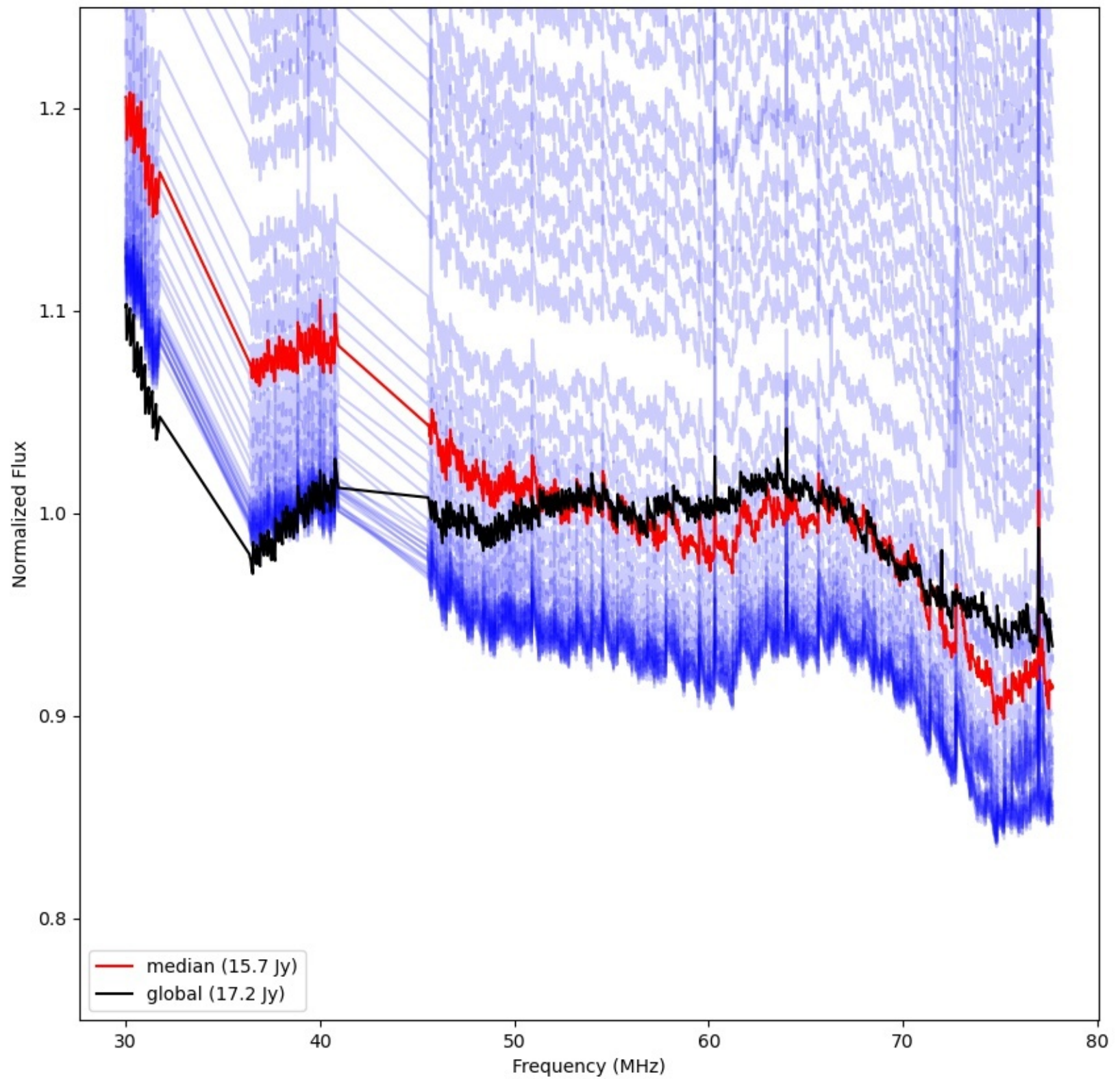
LWA185 - Correlator# 240 - YY - FLAGS:Good
