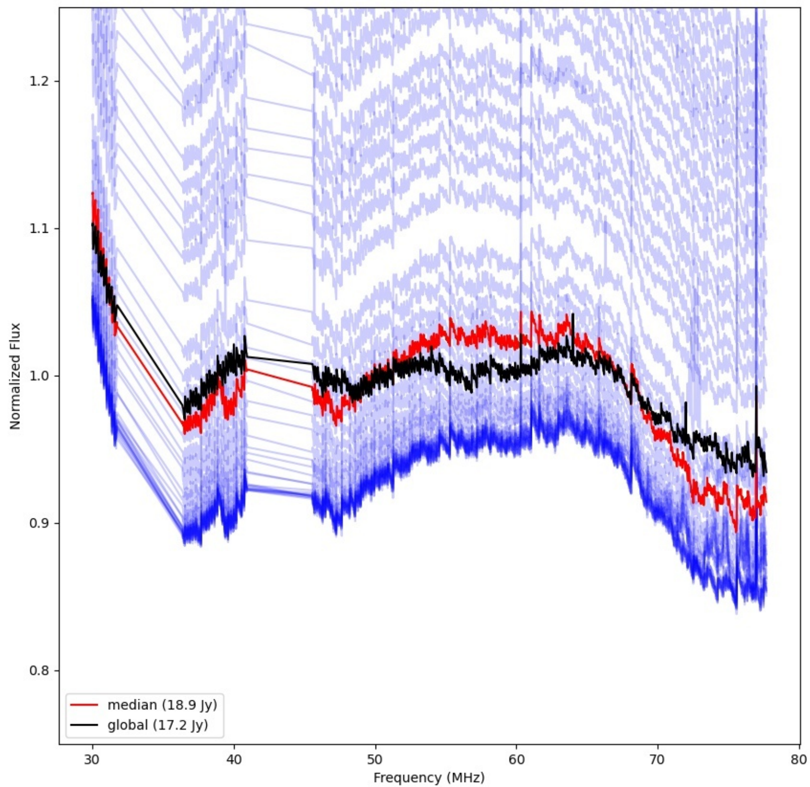
LWA346 - Correlator# 316 - YY - FLAGS:Good
