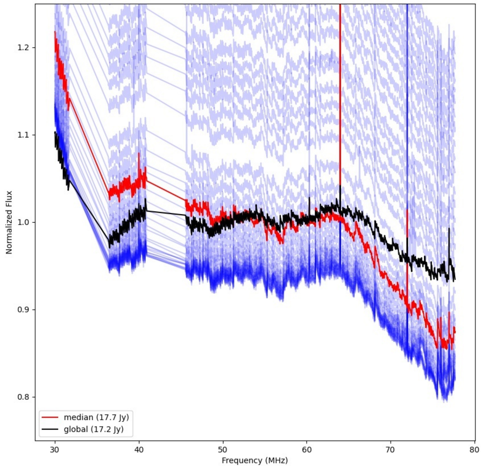
LWA092 - Correlator# 149 - YY - FLAGS:Good
