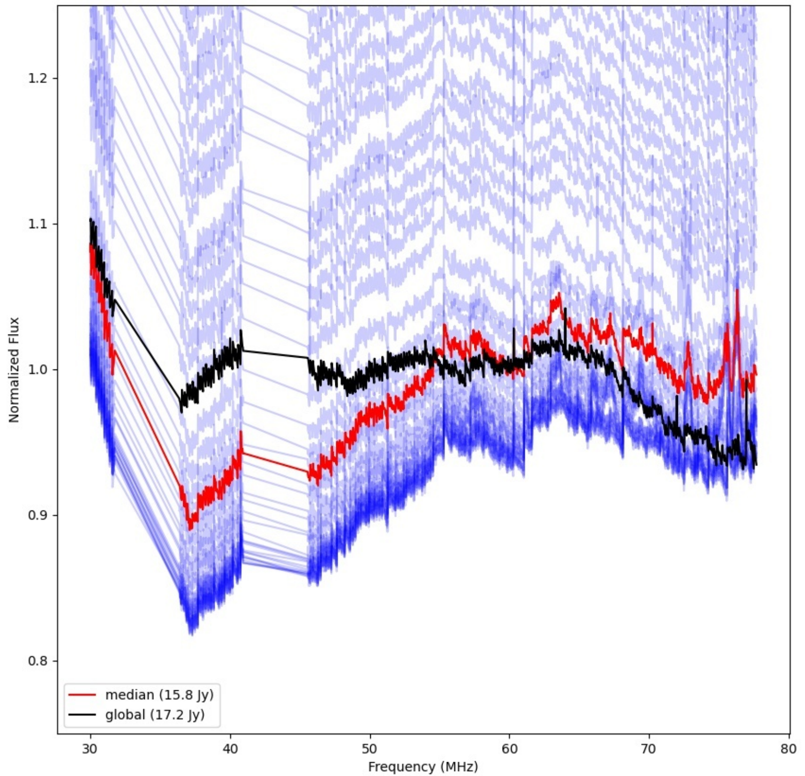
LWA354 - Correlator# 063 - YY - FLAGS:Good
