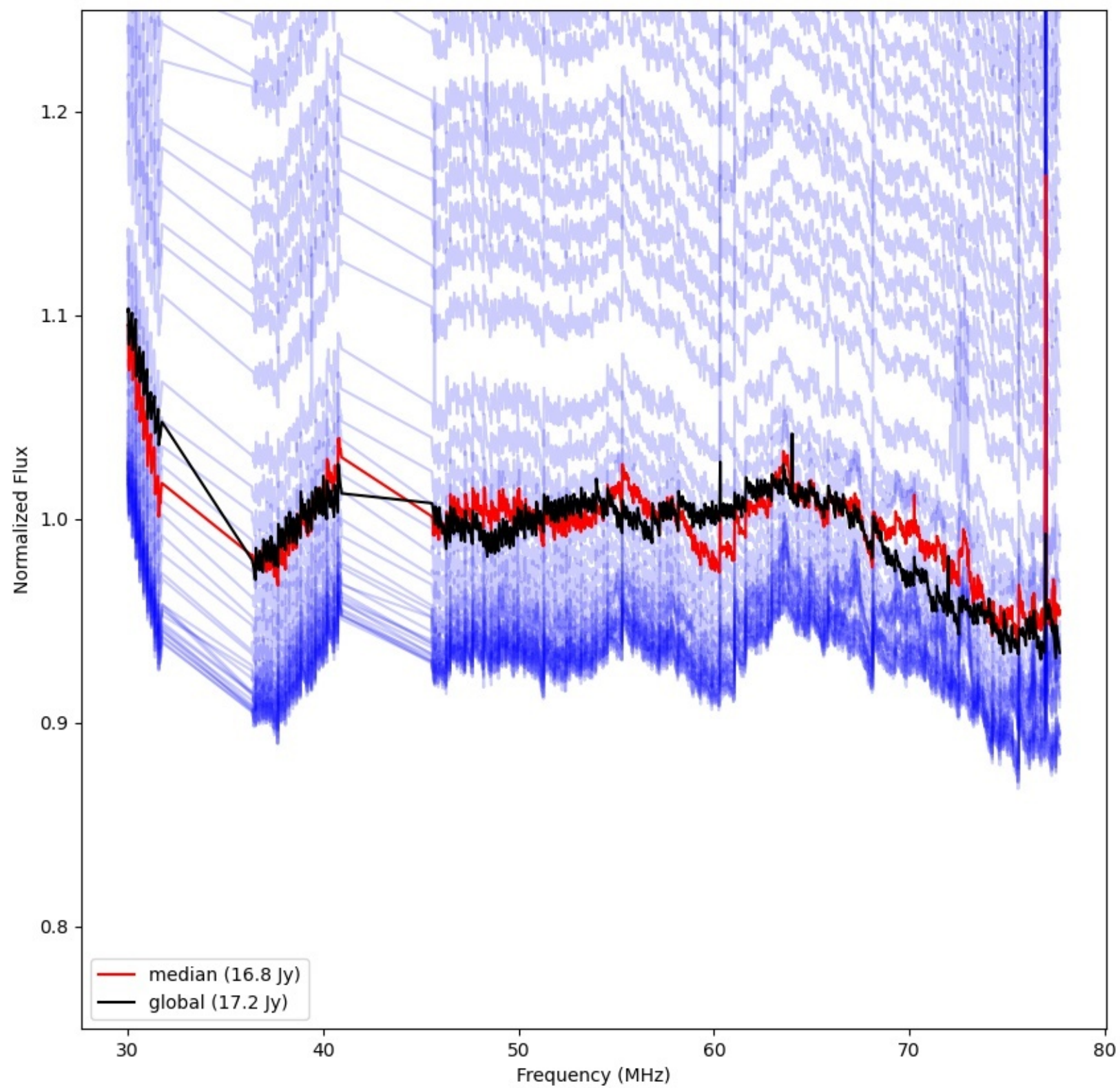
LWA268 - Correlator# 002 - YY - FLAGS:Good
