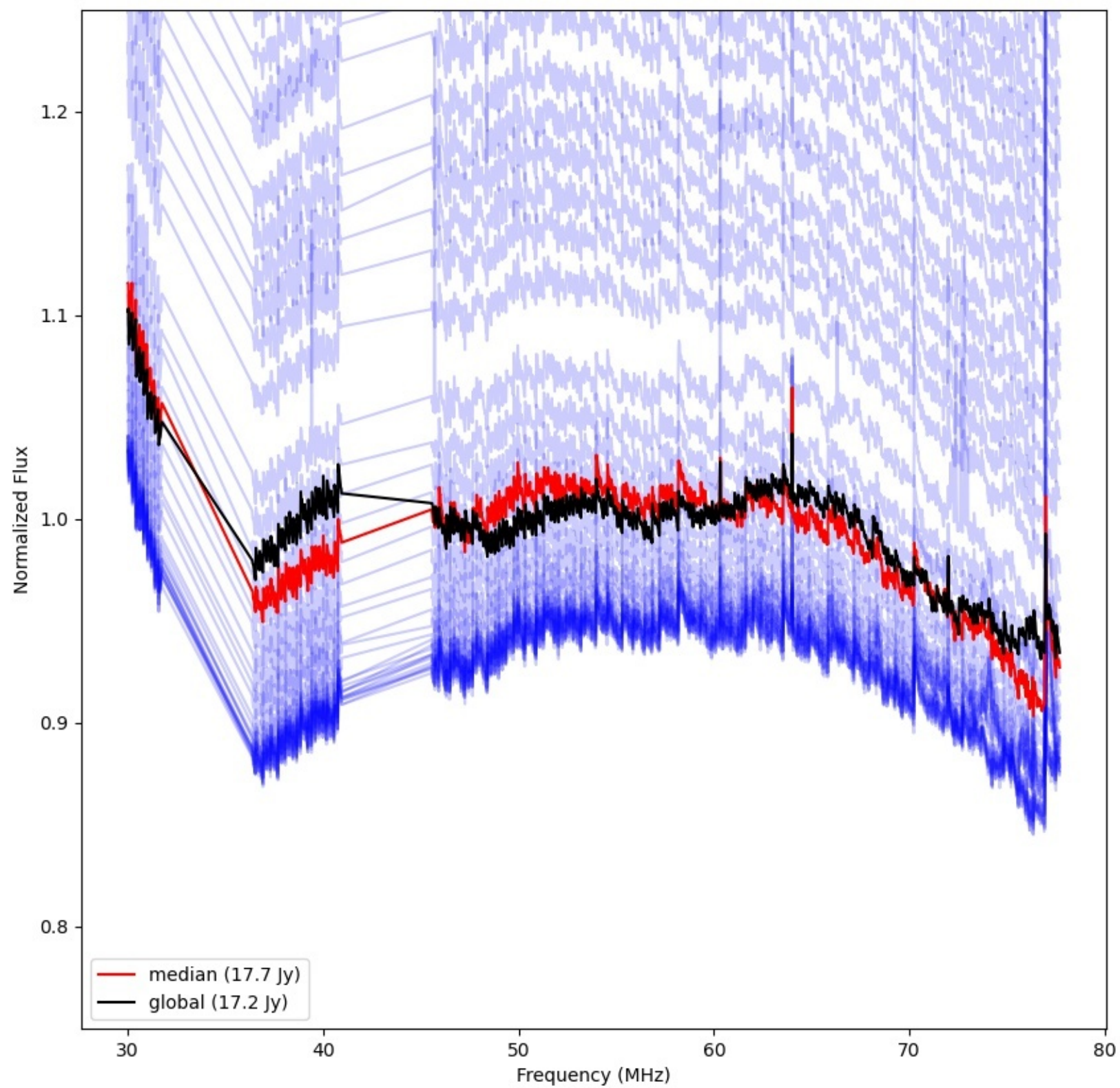
LWA056 - Correlator# 135 - YY - FLAGS:Good
