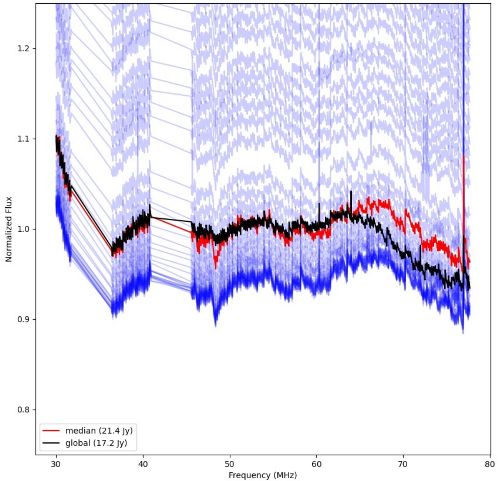
LWA180 - Correlator# 322 - YY - FLAGS:Good
