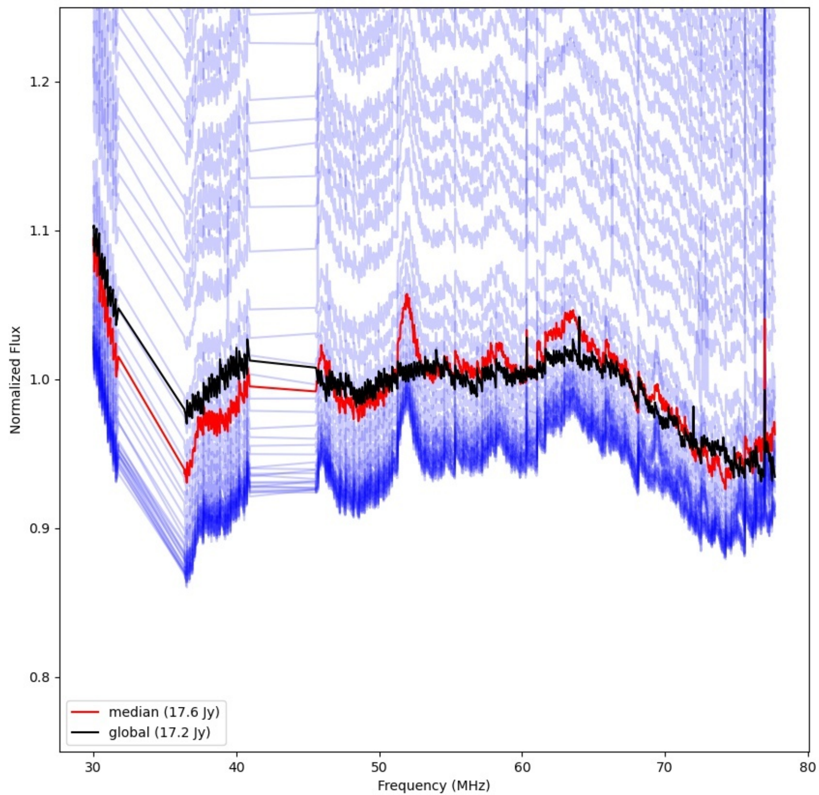
LWA261 - Correlator# 346 - YY - FLAGS:Good
