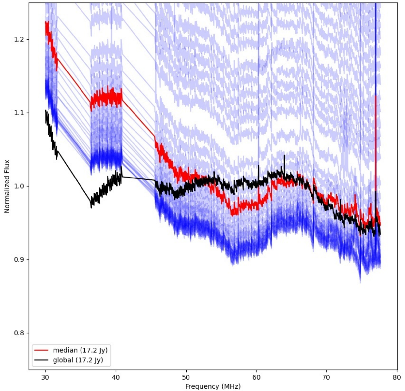
LWA233 - Correlator# 306 - YY - FLAGS:Good
