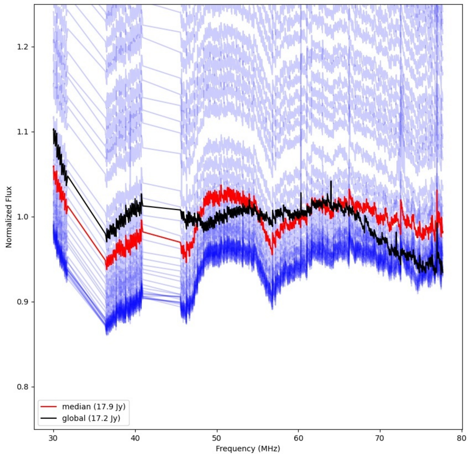
LWA198 - Correlator# 271 - YY - FLAGS:Good
