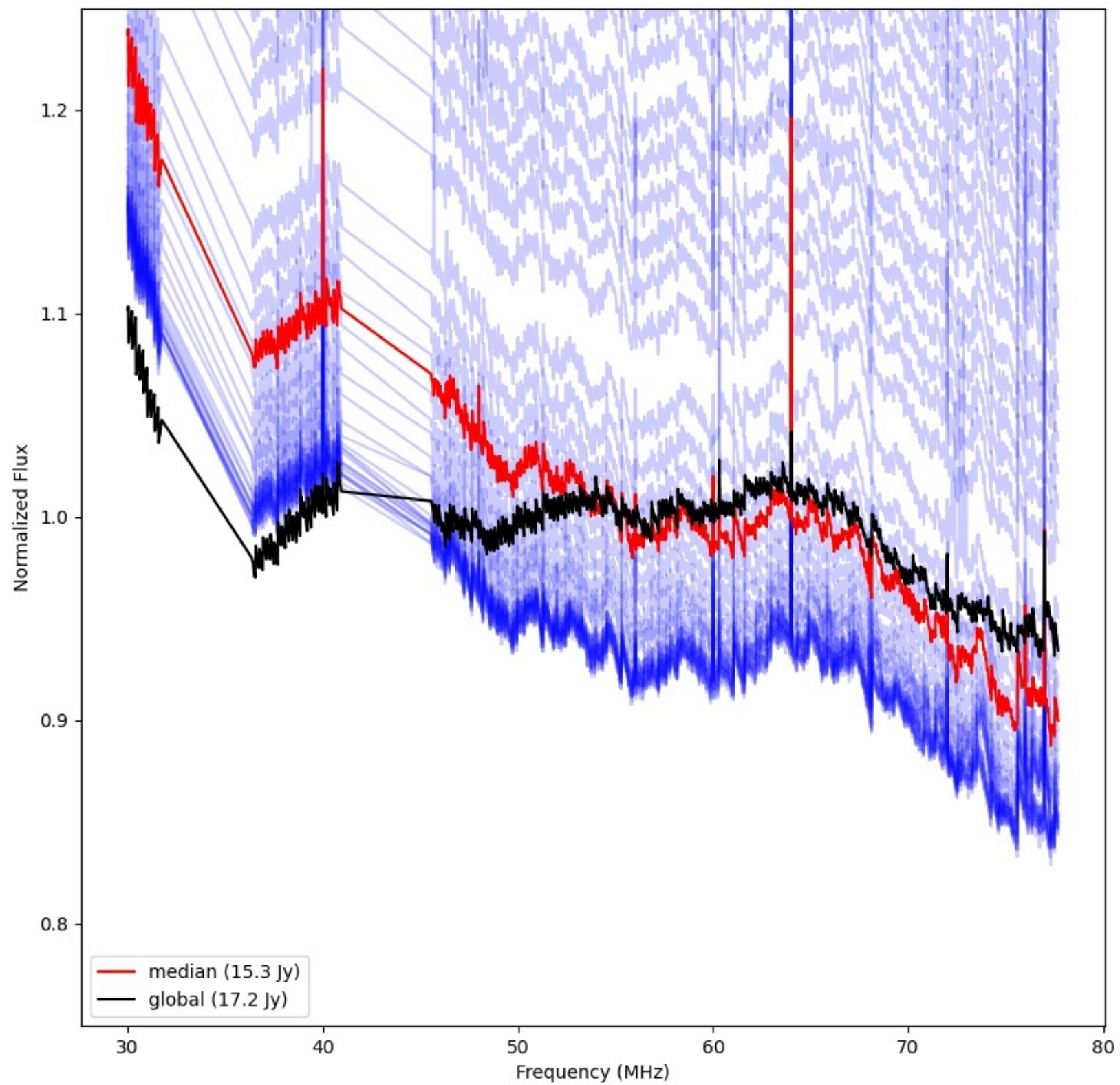
LWA158 - Correlator# 237 - YY - FLAGS:Good
