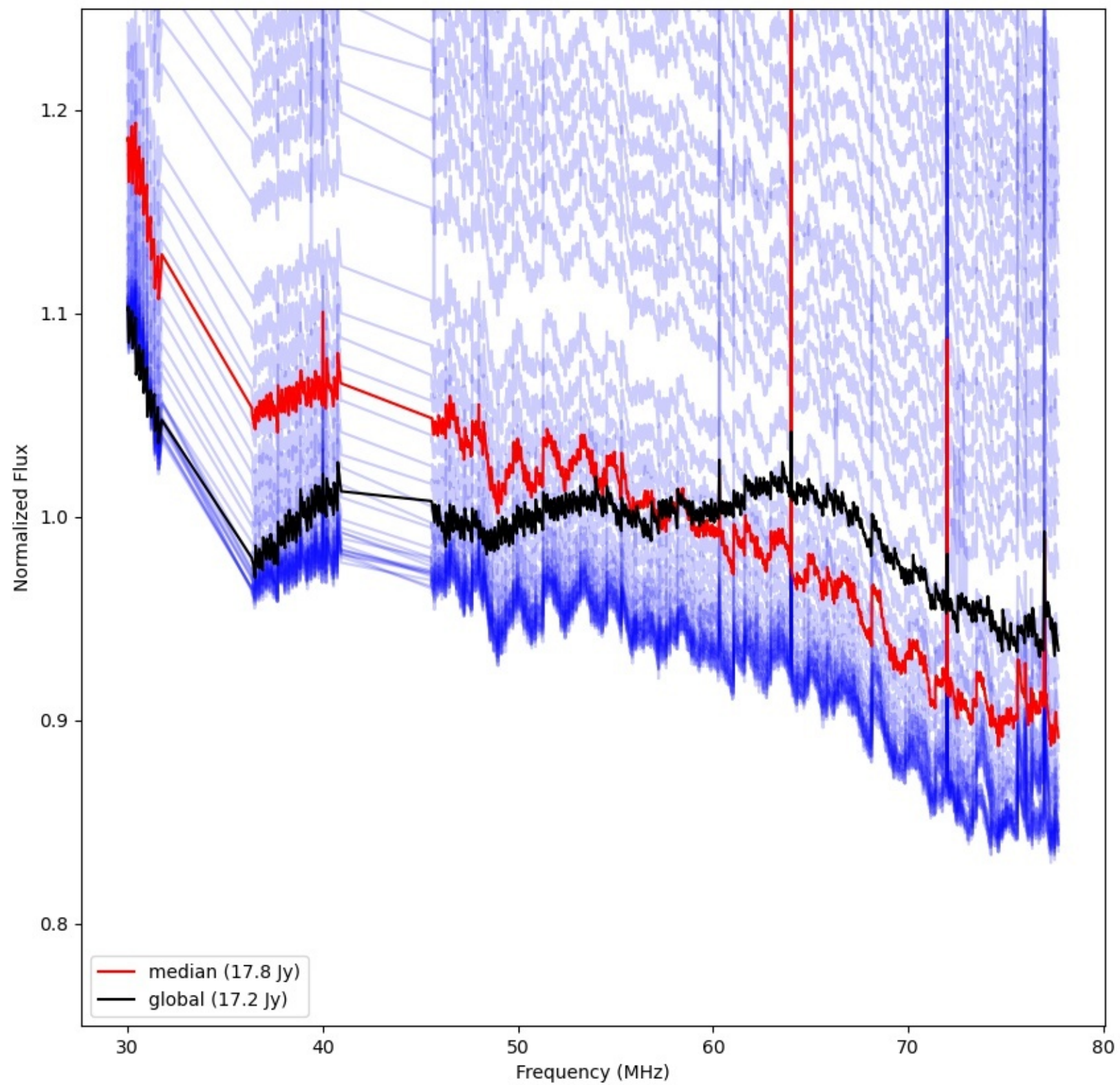
LWA064 - Correlator# 141 - YY - FLAGS:Good
