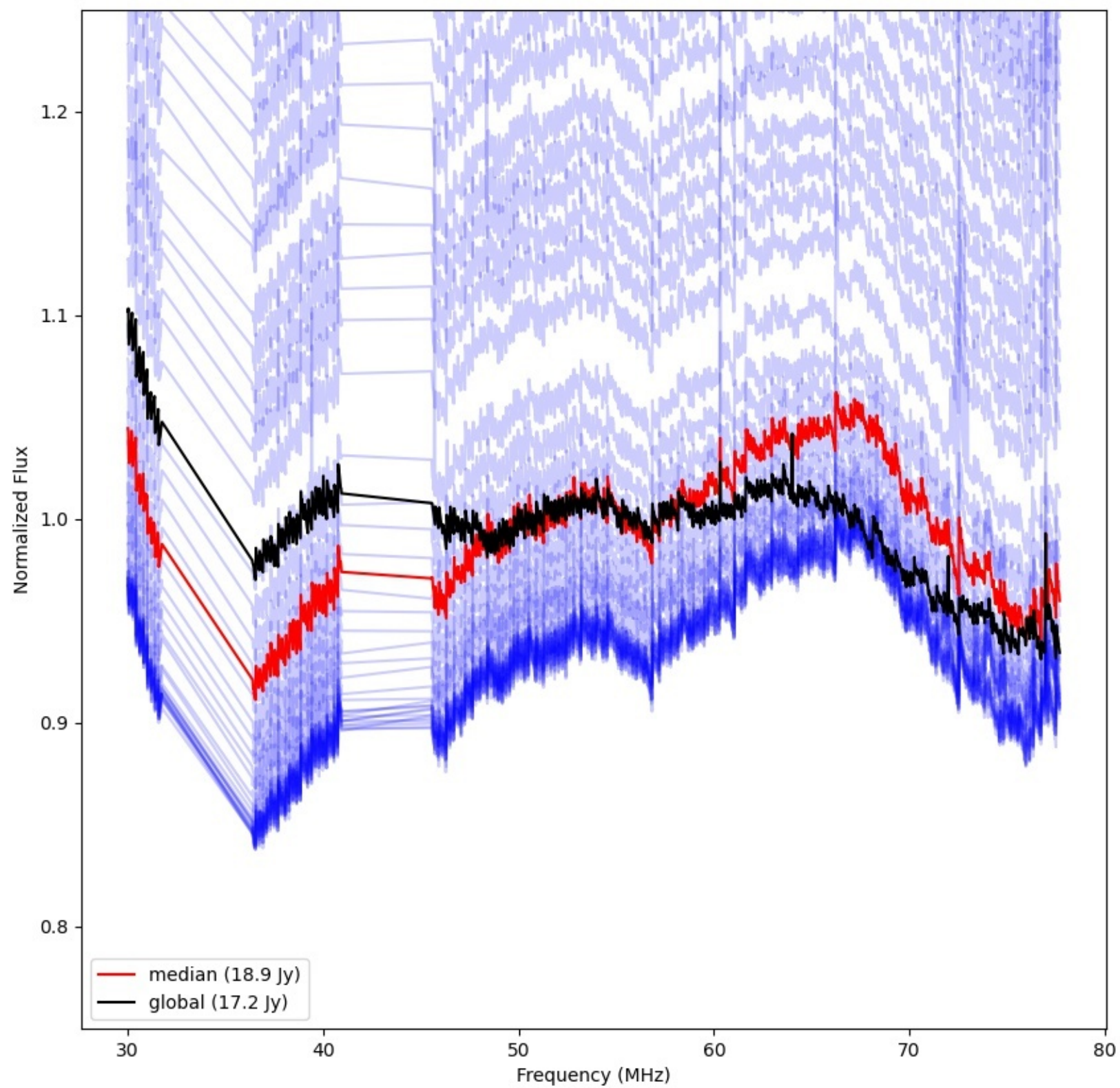
LWA196 - Correlator# 275 - YY - FLAGS:Good
