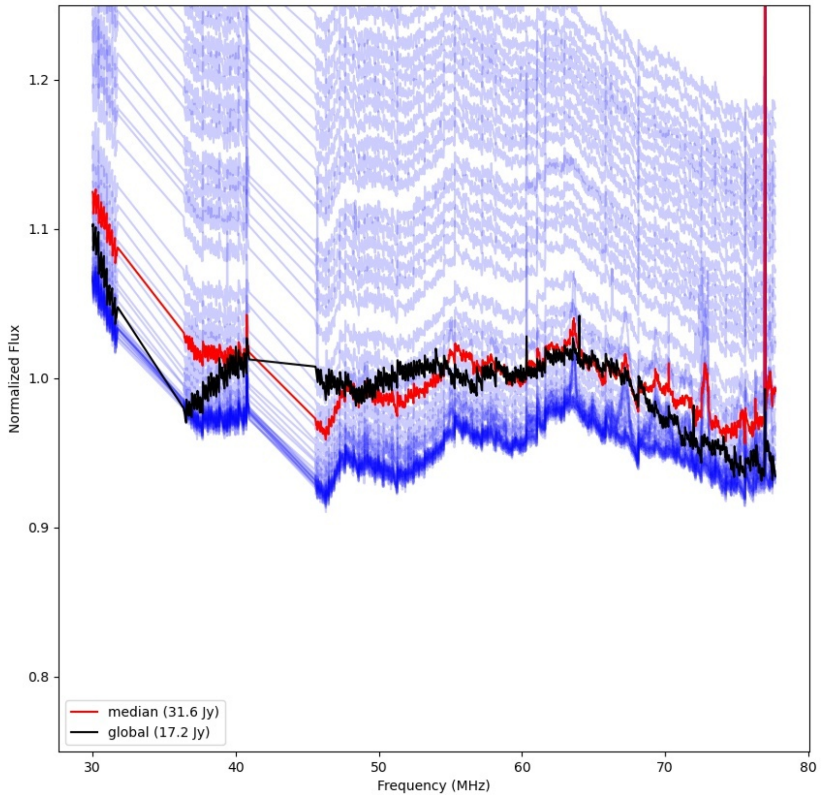
LWA272 - Correlator# 038 - YY - FLAGS:Good
