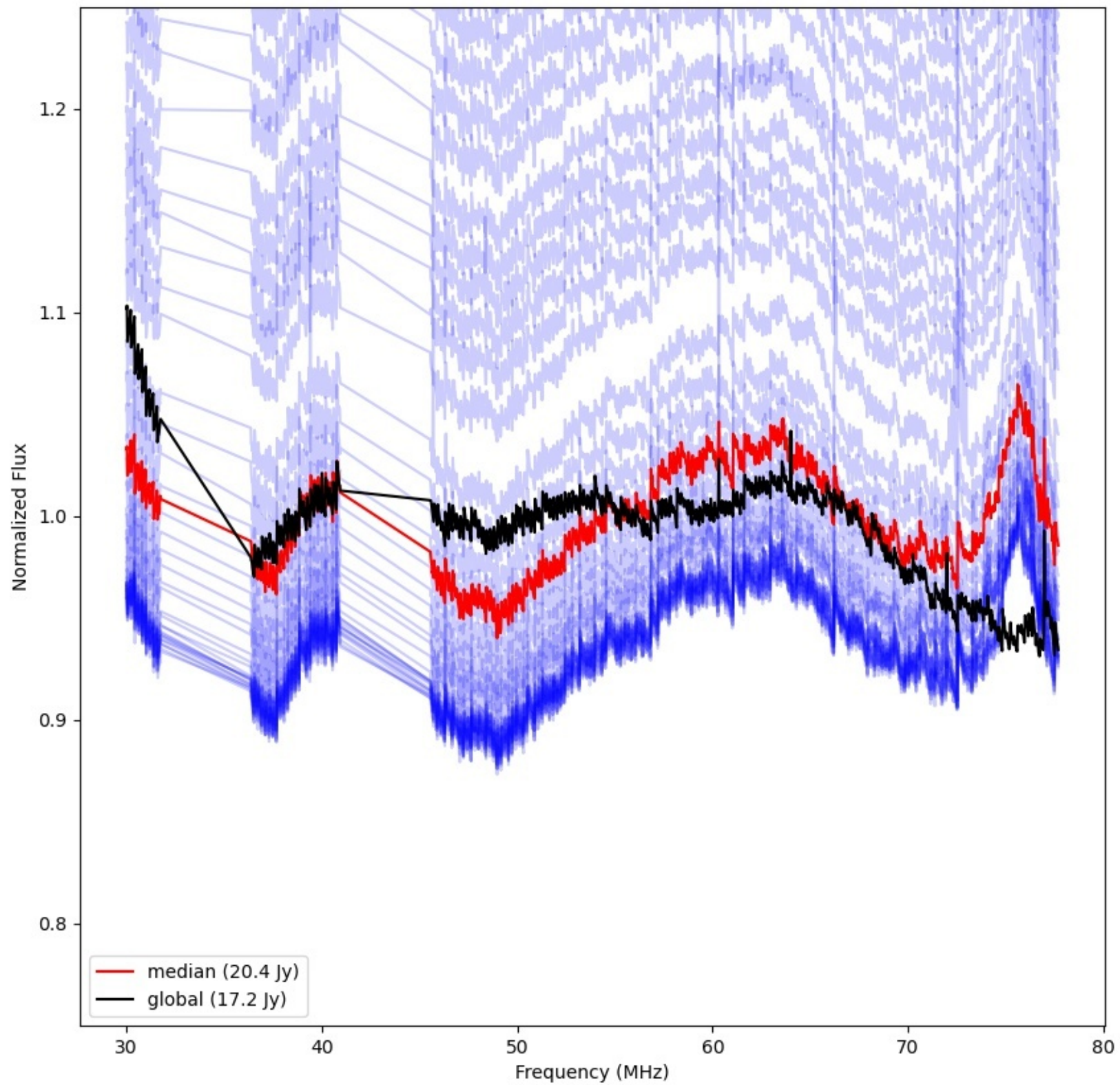
LWA009 - Correlator# 070 - YY - FLAGS:Good
