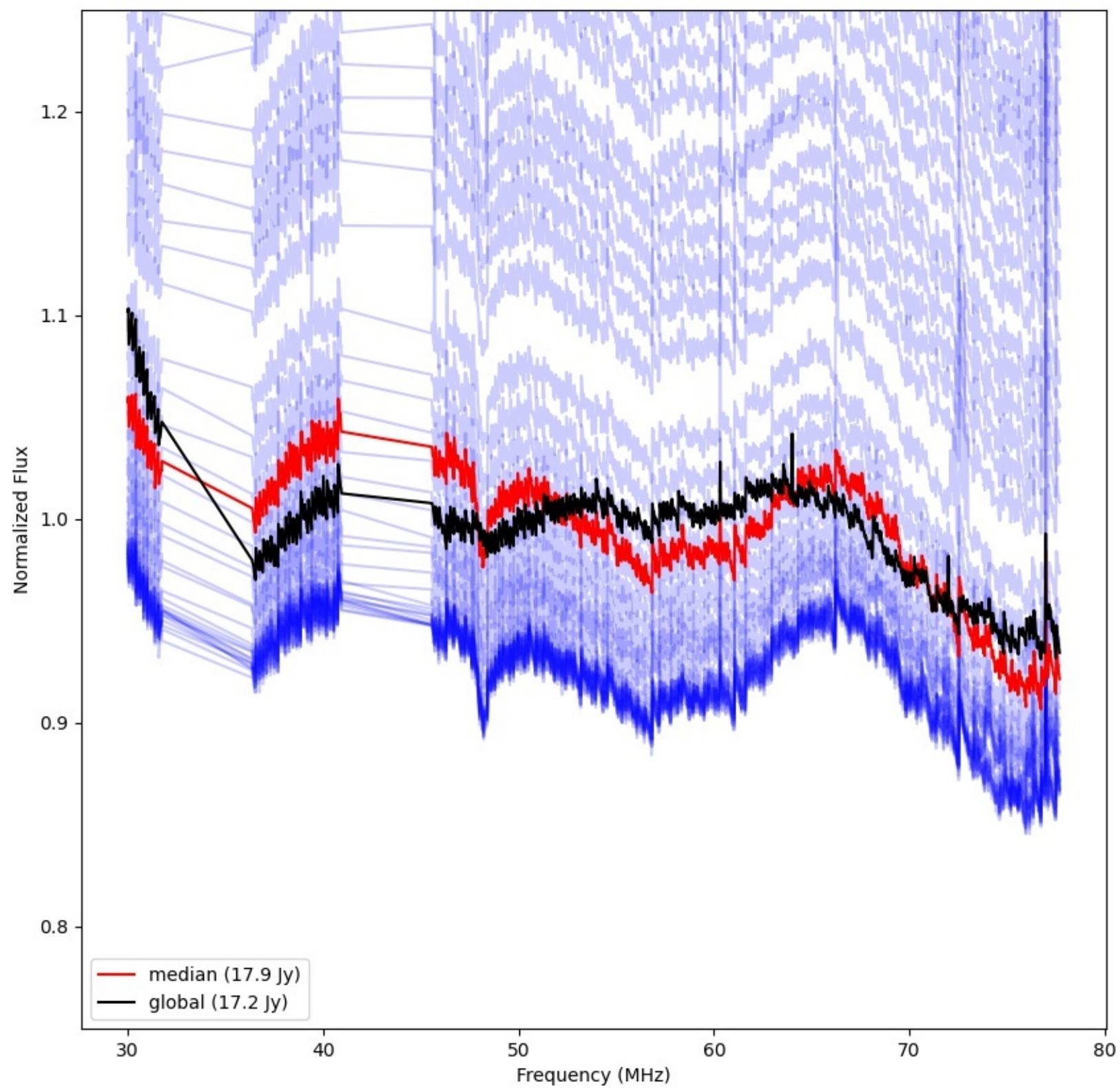
LWA227 - Correlator# 280 - YY - FLAGS:Good
