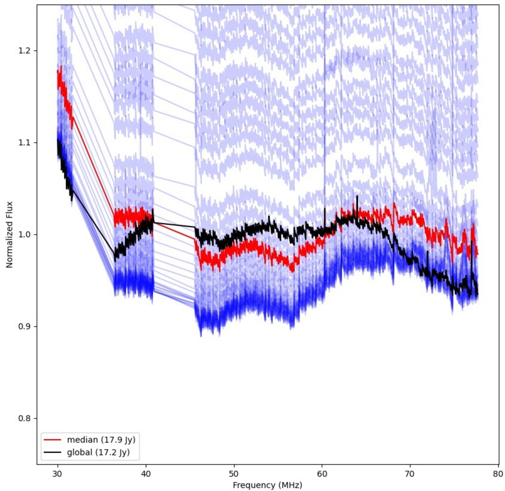
LWA235 - Correlator# 309 - YY - FLAGS:Good
