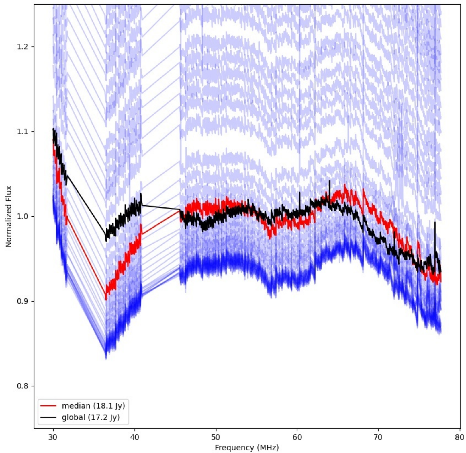
LWA254 - Correlator# 315 - YY - FLAGS:Good
