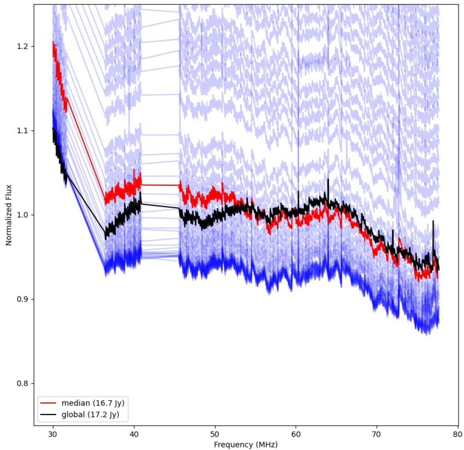
LWA089 - Correlator# 144 - YY - FLAGS:Good
