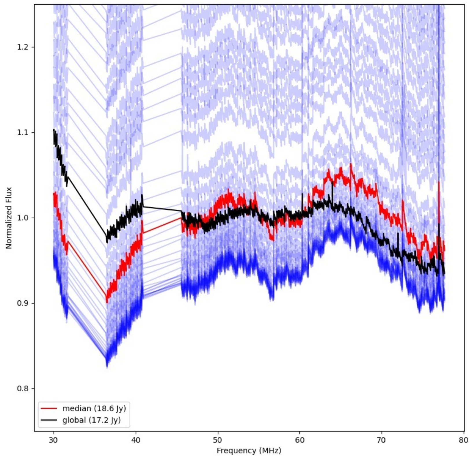
LWA253 - Correlator# 283 - YY - FLAGS:Good
