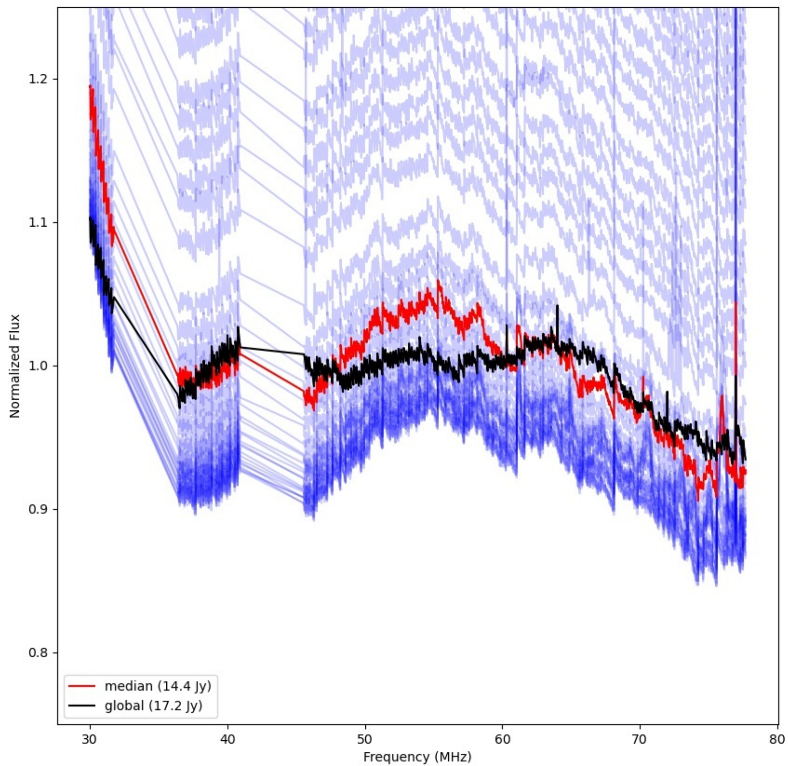
LWA287 - Correlator# 223 - YY - FLAGS:Good
