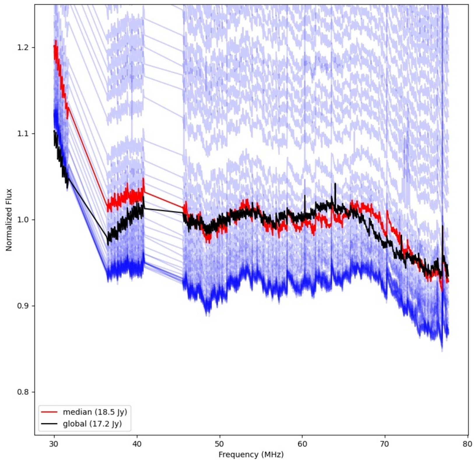
LWA176 - Correlator# 325 - YY - FLAGS:Good
