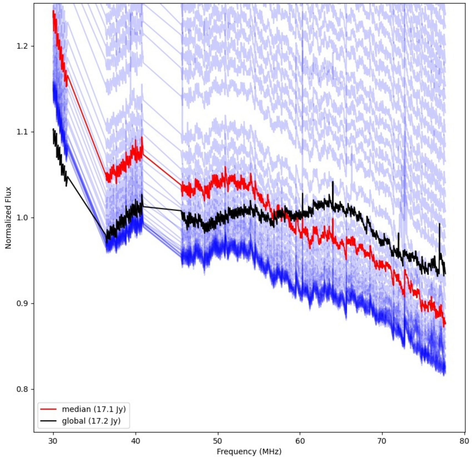
LWA087 - Correlator# 142 - YY - FLAGS:Good
