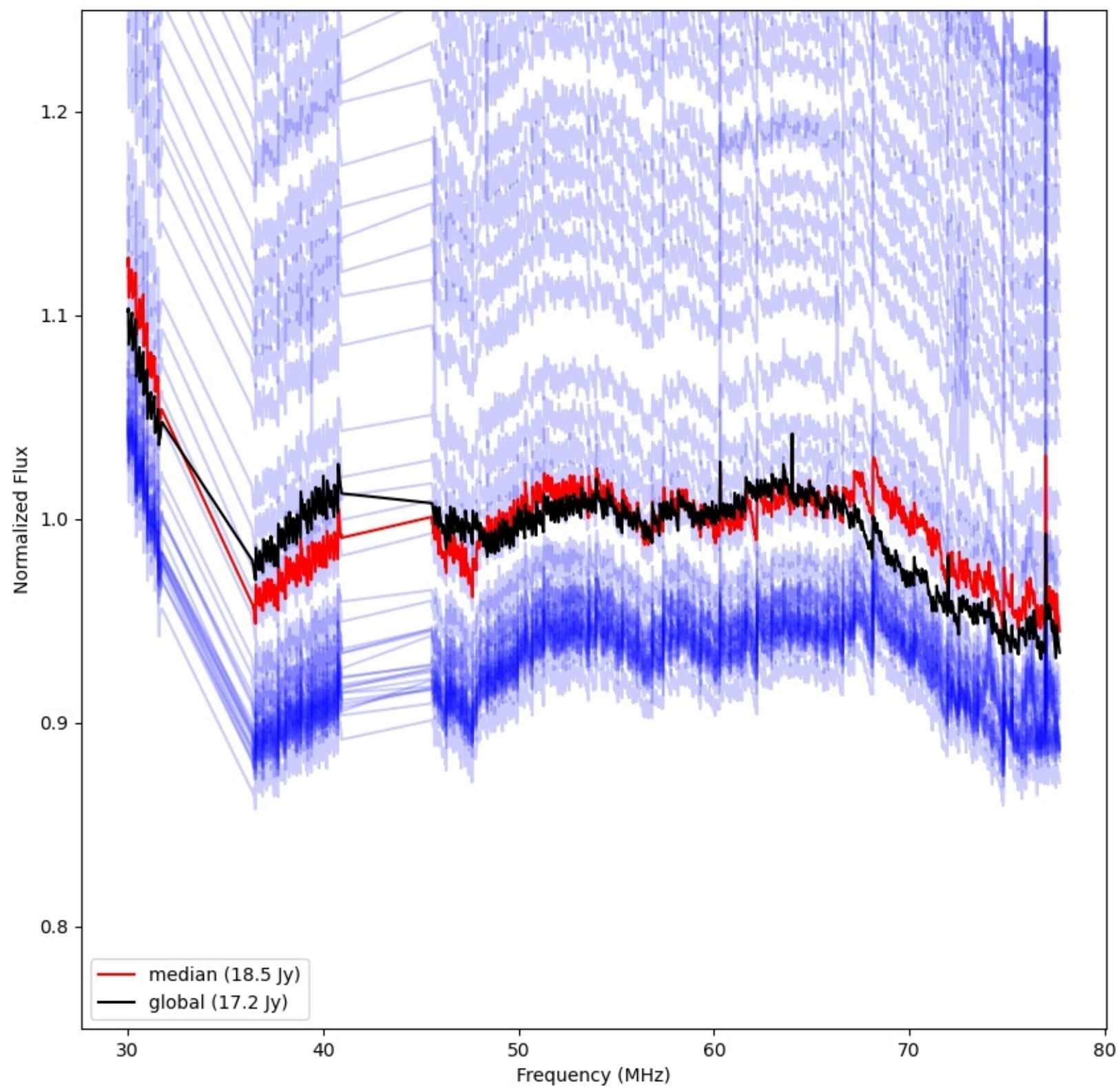
LWA205 - Correlator# 297 - YY - FLAGS:Good
