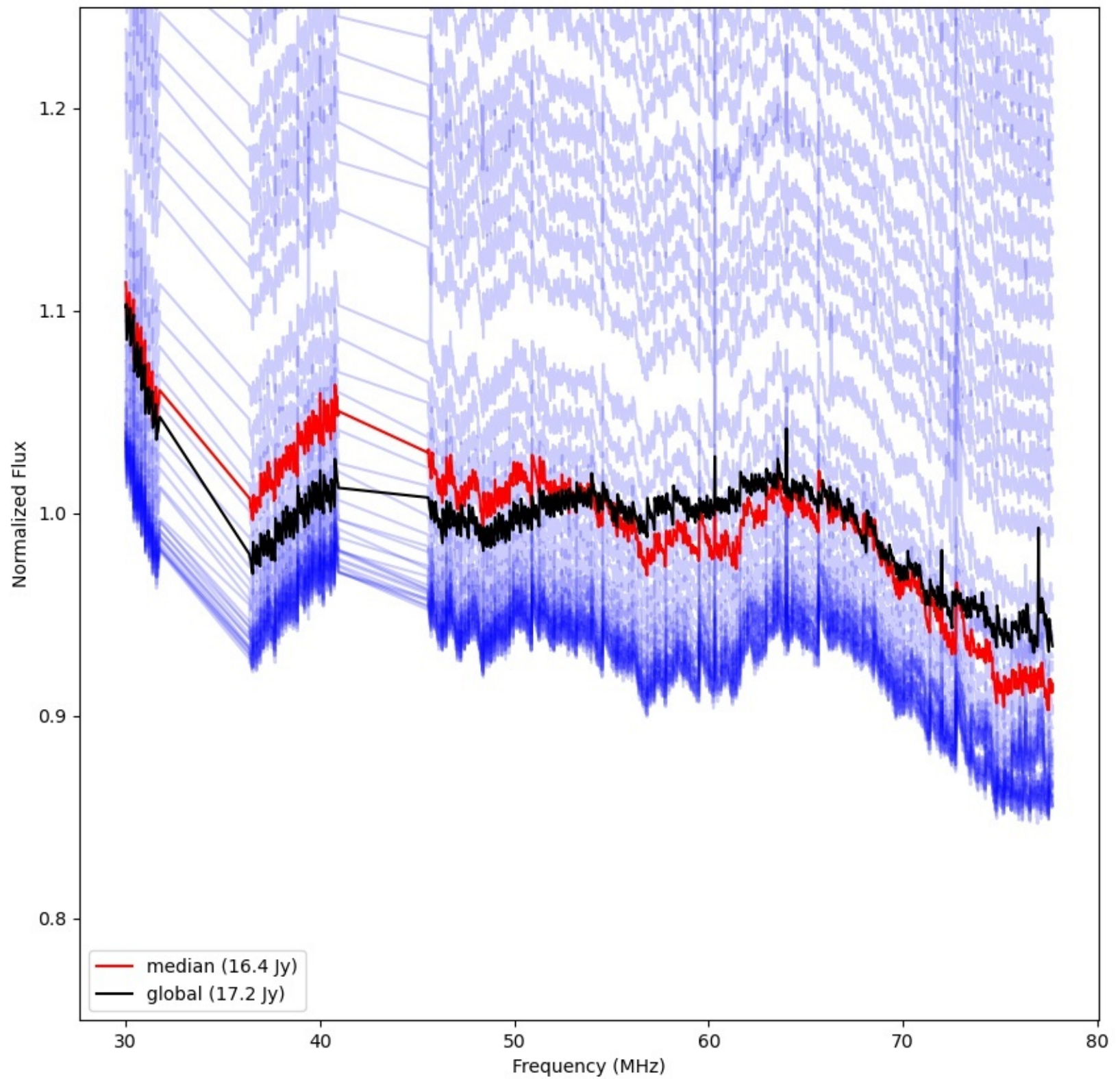
LWA186 - Correlator# 243 - YY - FLAGS:Good
