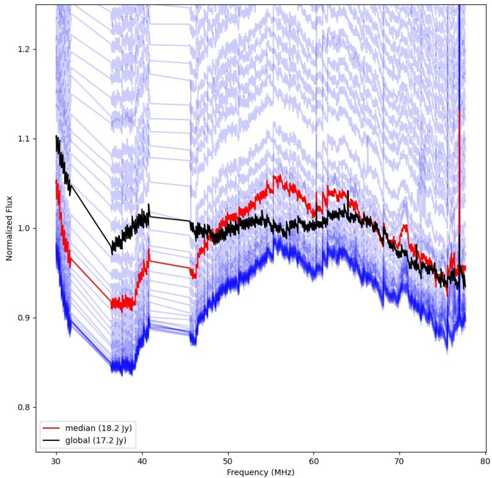
LWA317 - Correlator# 052 - YY - FLAGS:Good
