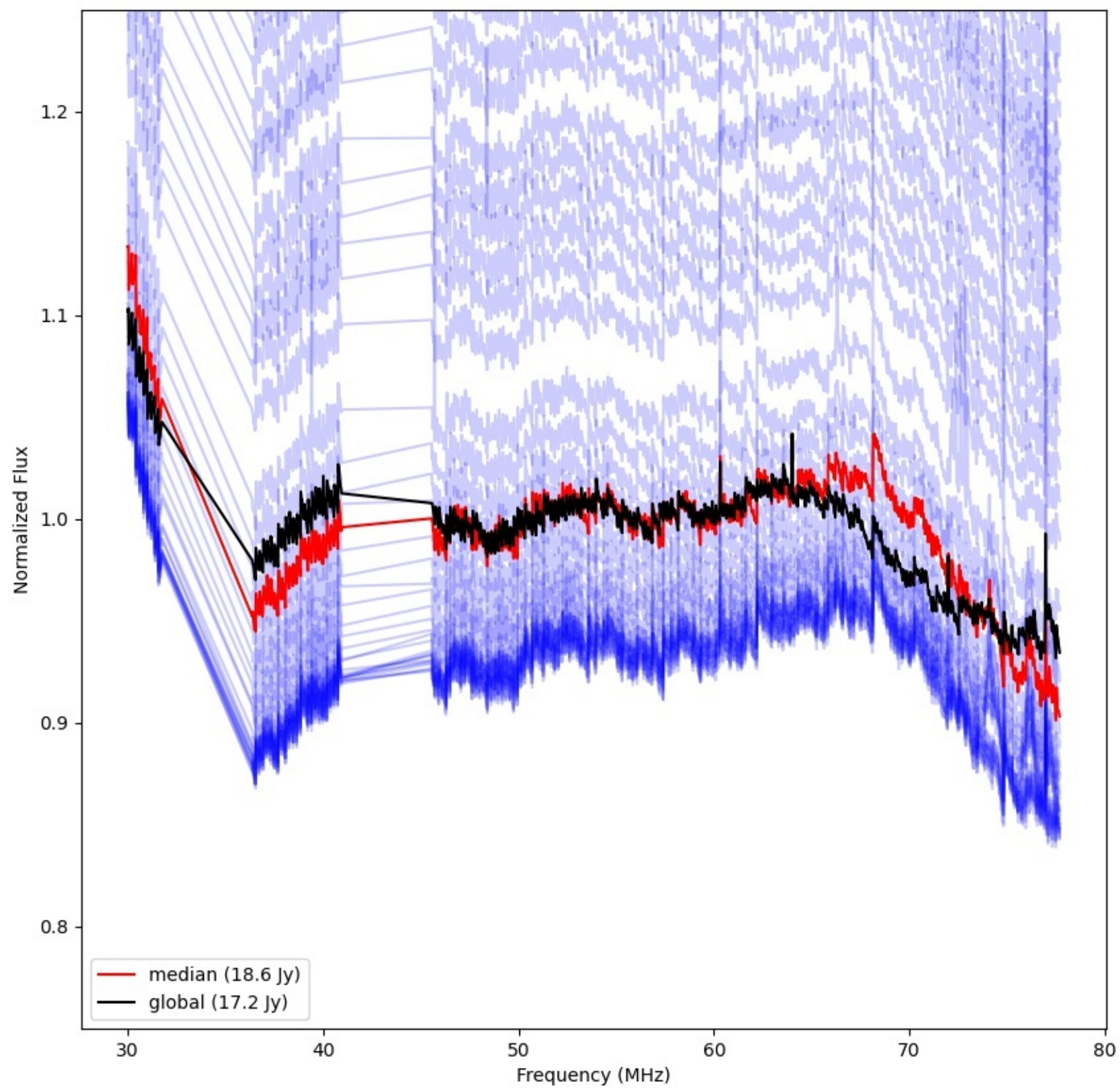
LWA206 - Correlator# 296 - YY - FLAGS:Good
