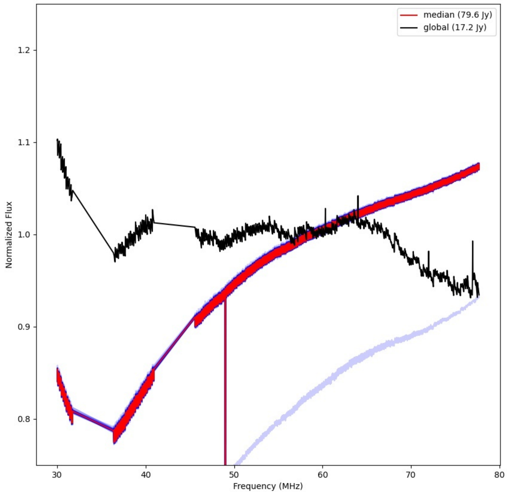
LWA280 - Correlator# 041 - YY - FLAGS:Good
