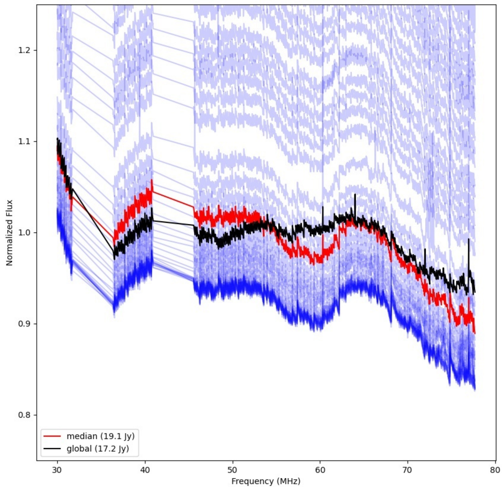
LWA166 - Correlator# 269 - YY - FLAGS:Good
