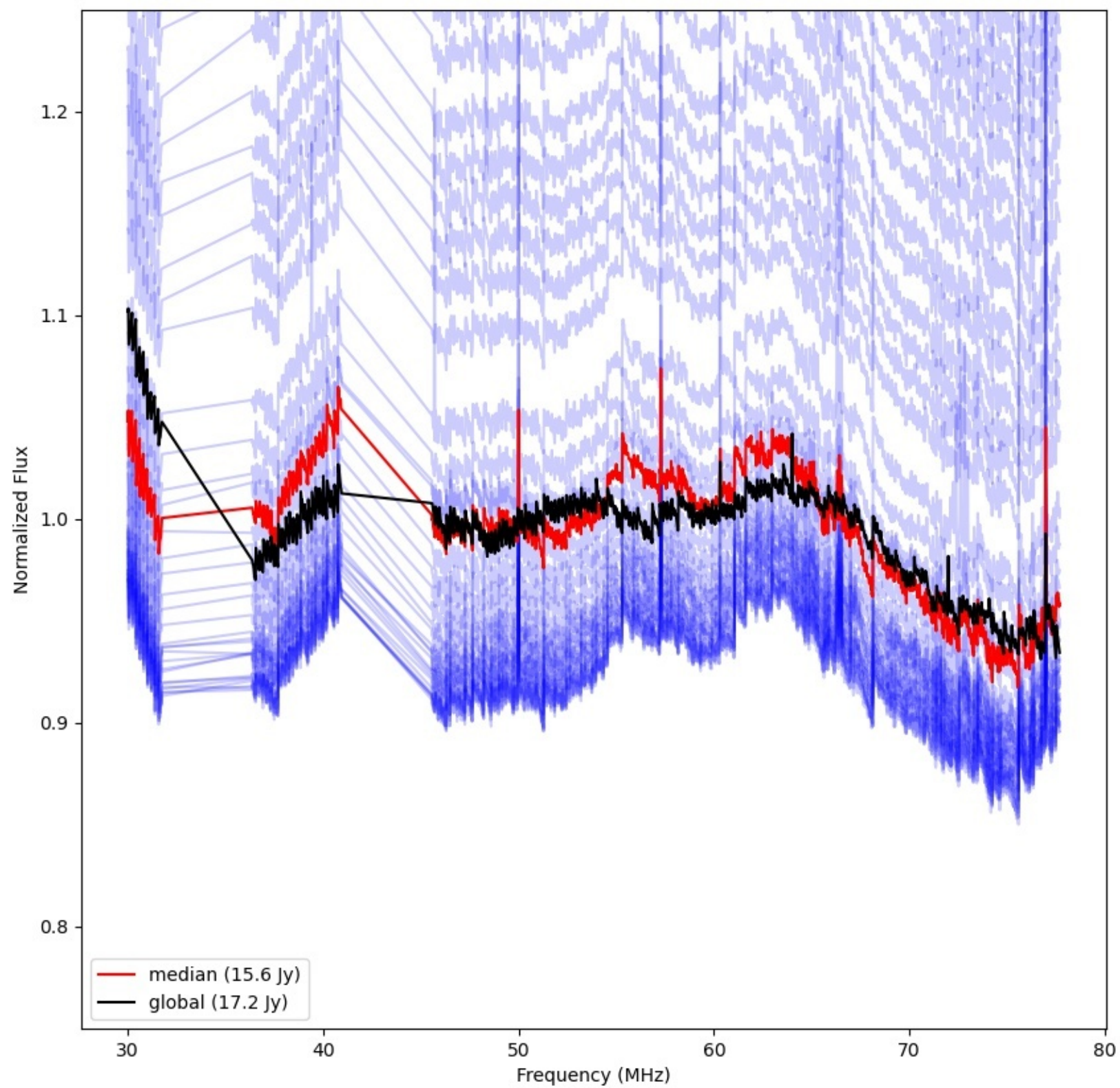
LWA355 - Correlator# 222 - YY - FLAGS:Good
