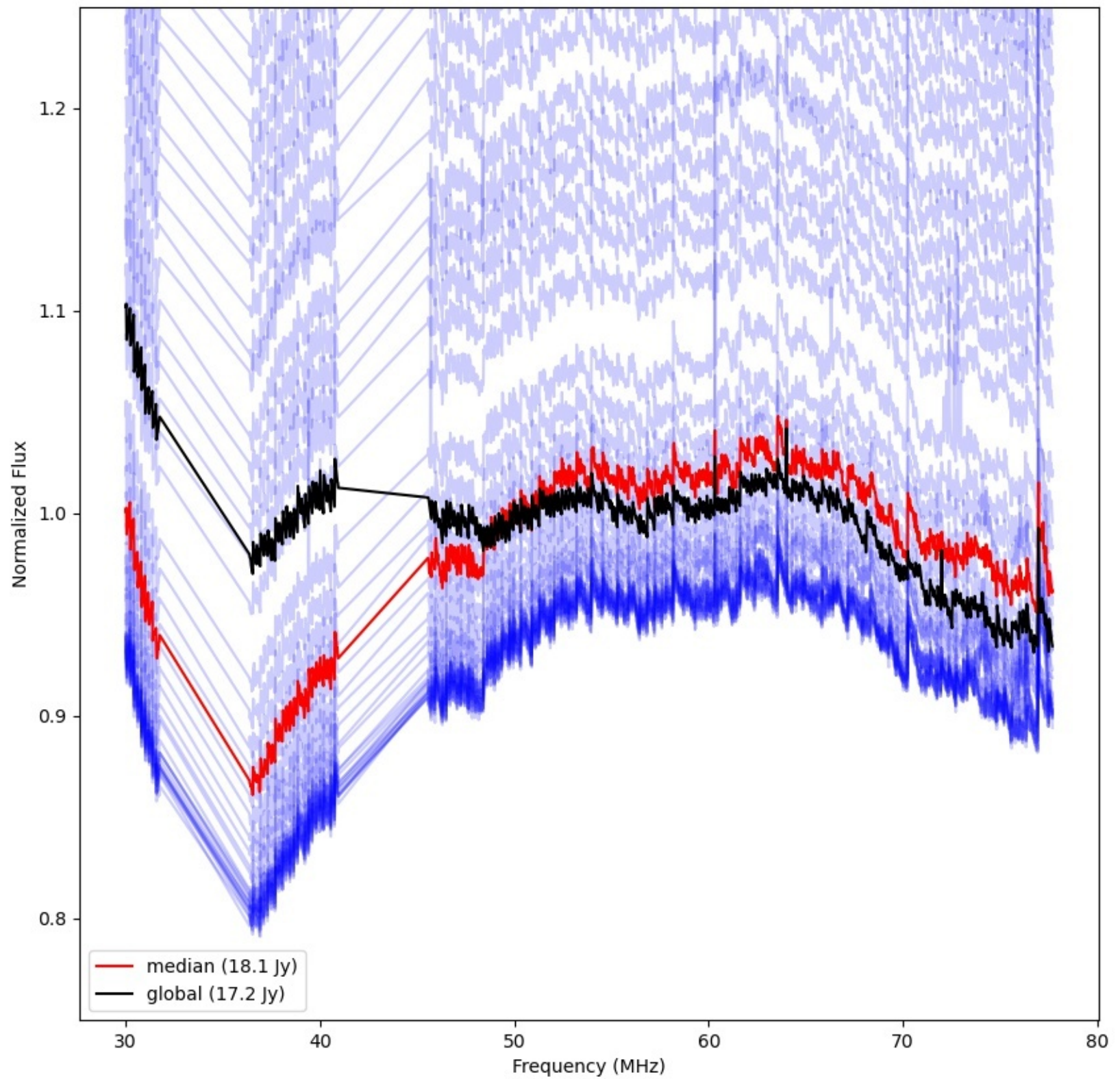
LWA084 - Correlator# 120 - YY - FLAGS:Good
