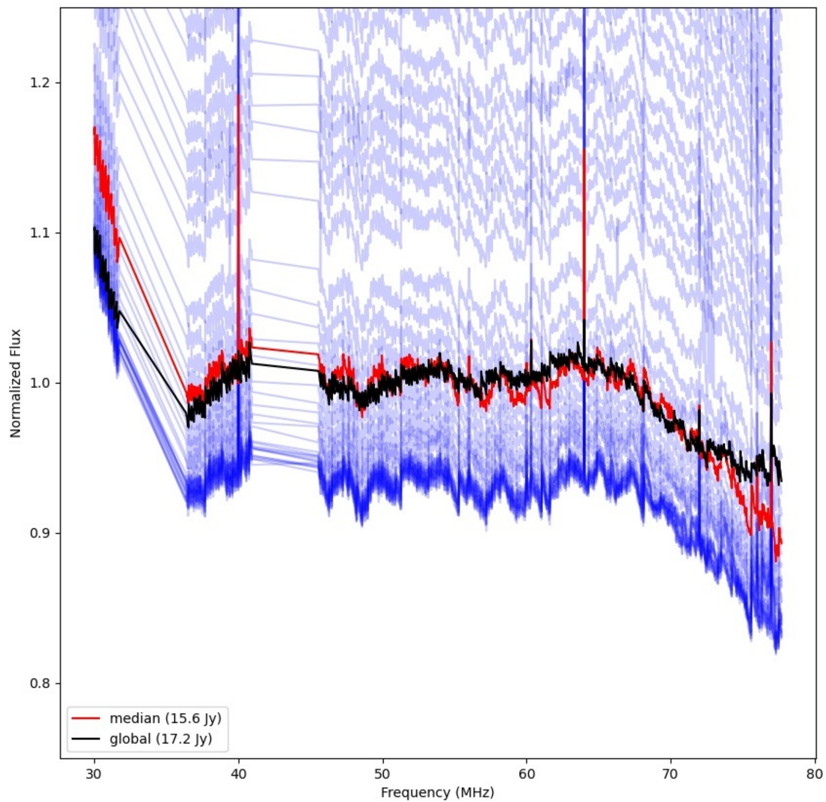
LWA127 - Correlator# 225 - YY - FLAGS:Good
