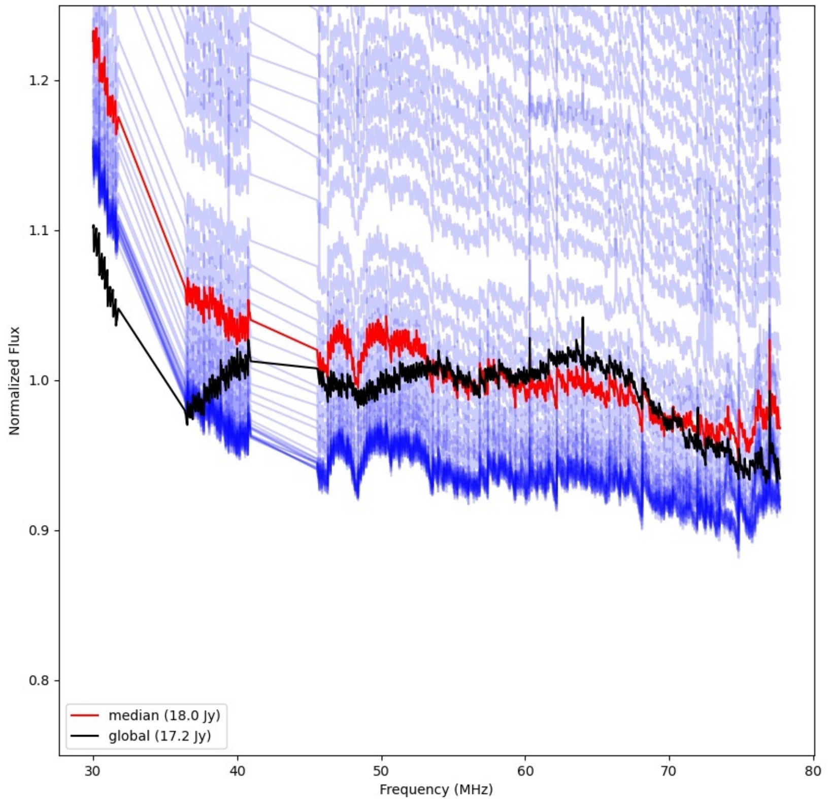
LWA014 - Correlator# 099 - YY - FLAGS:Good
