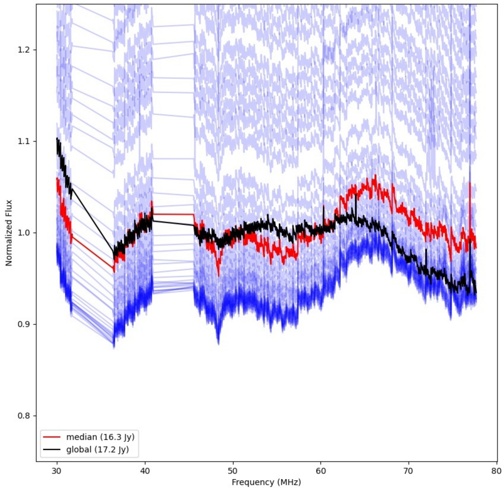
LWA208 - Correlator# 298 - YY - FLAGS:Good
