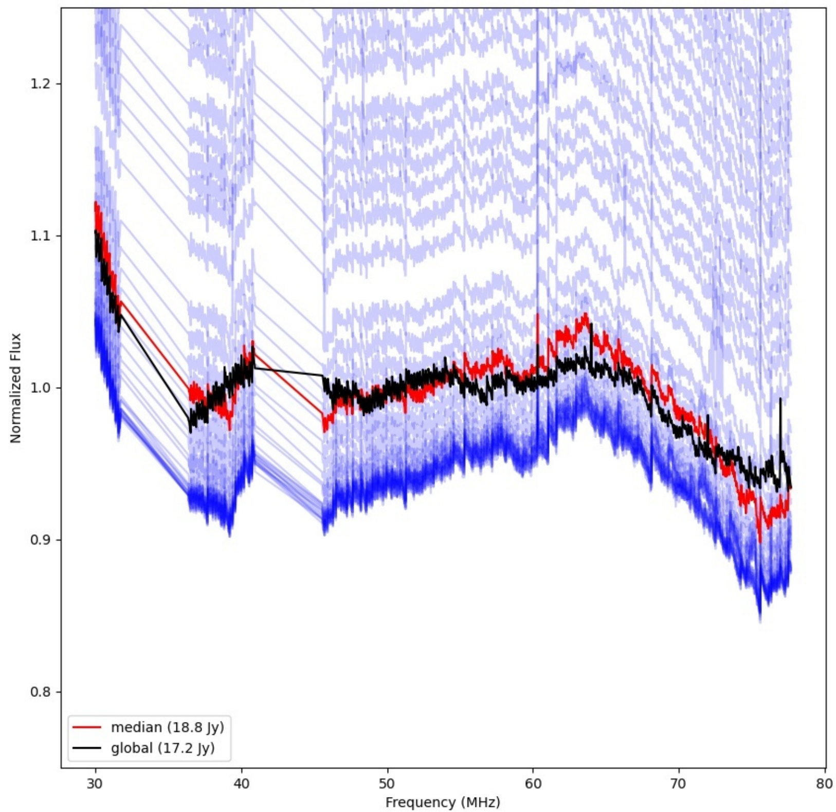
LWA329 - Correlator# 287 - YY - FLAGS:Good
