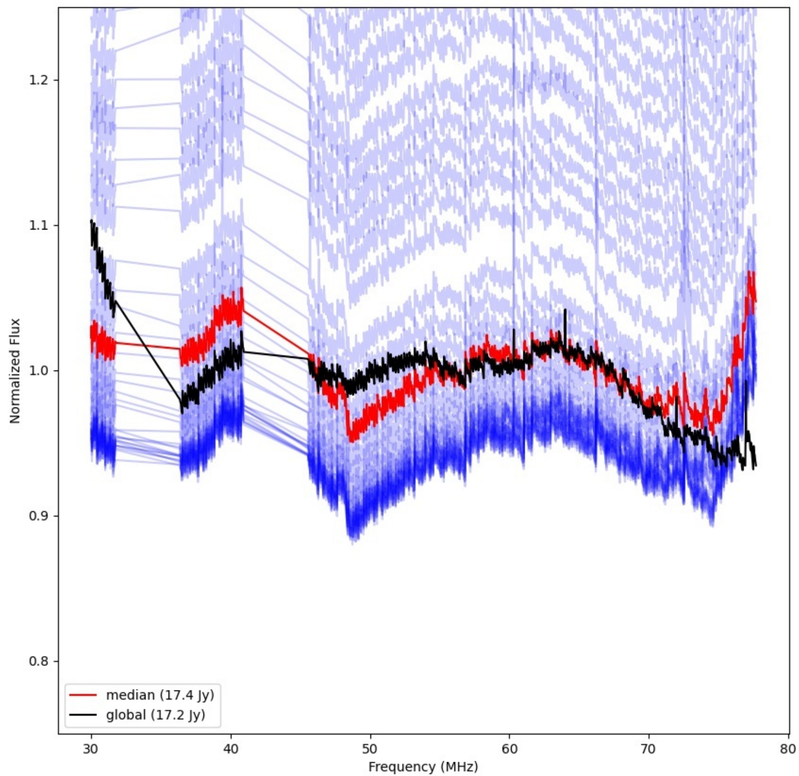
LWA011 - Correlator# 072 - YY - FLAGS:Good
