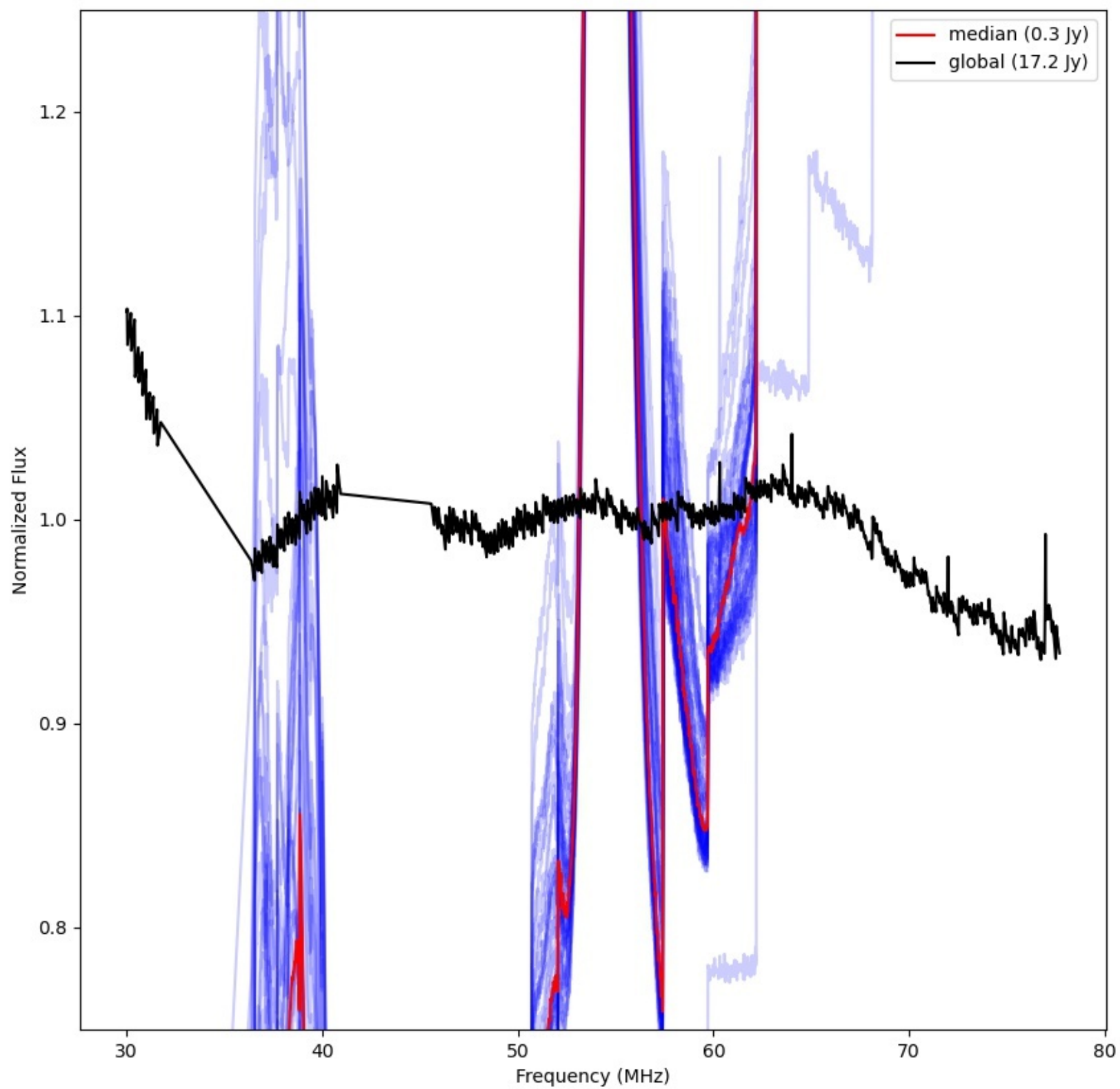
LWA105 - Correlator# 178 - YY - FLAGS:LowFlux
