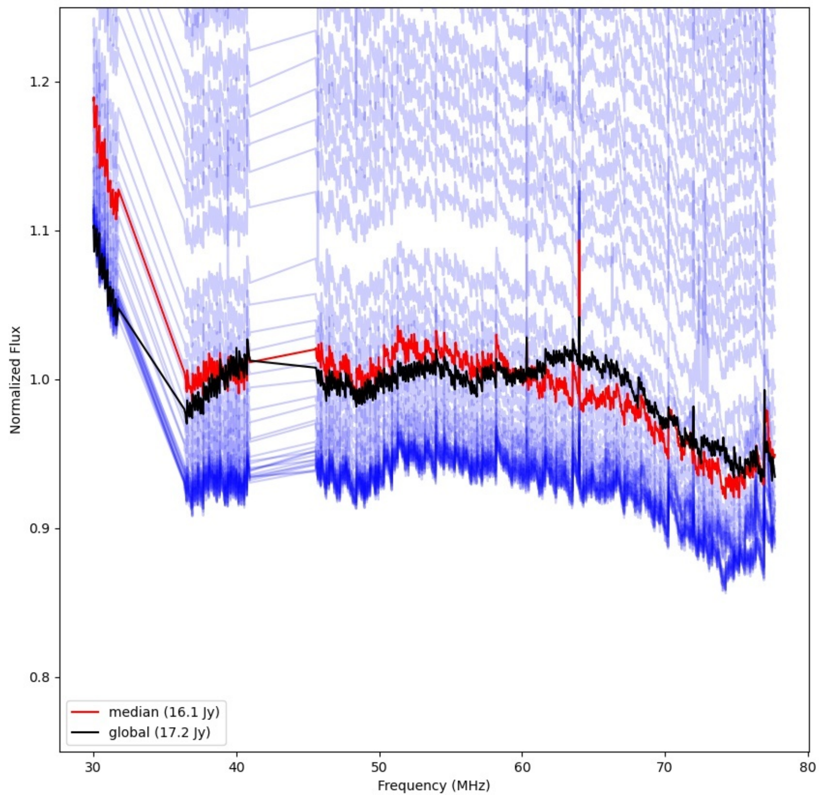
LWA030 - Correlator# 128 - YY - FLAGS:Good
