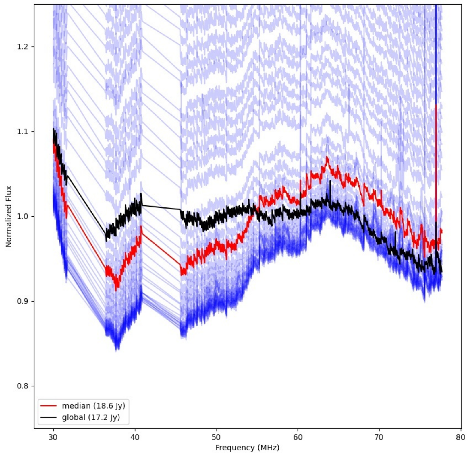
LWA342 - Correlator# 317 - YY - FLAGS:Good
