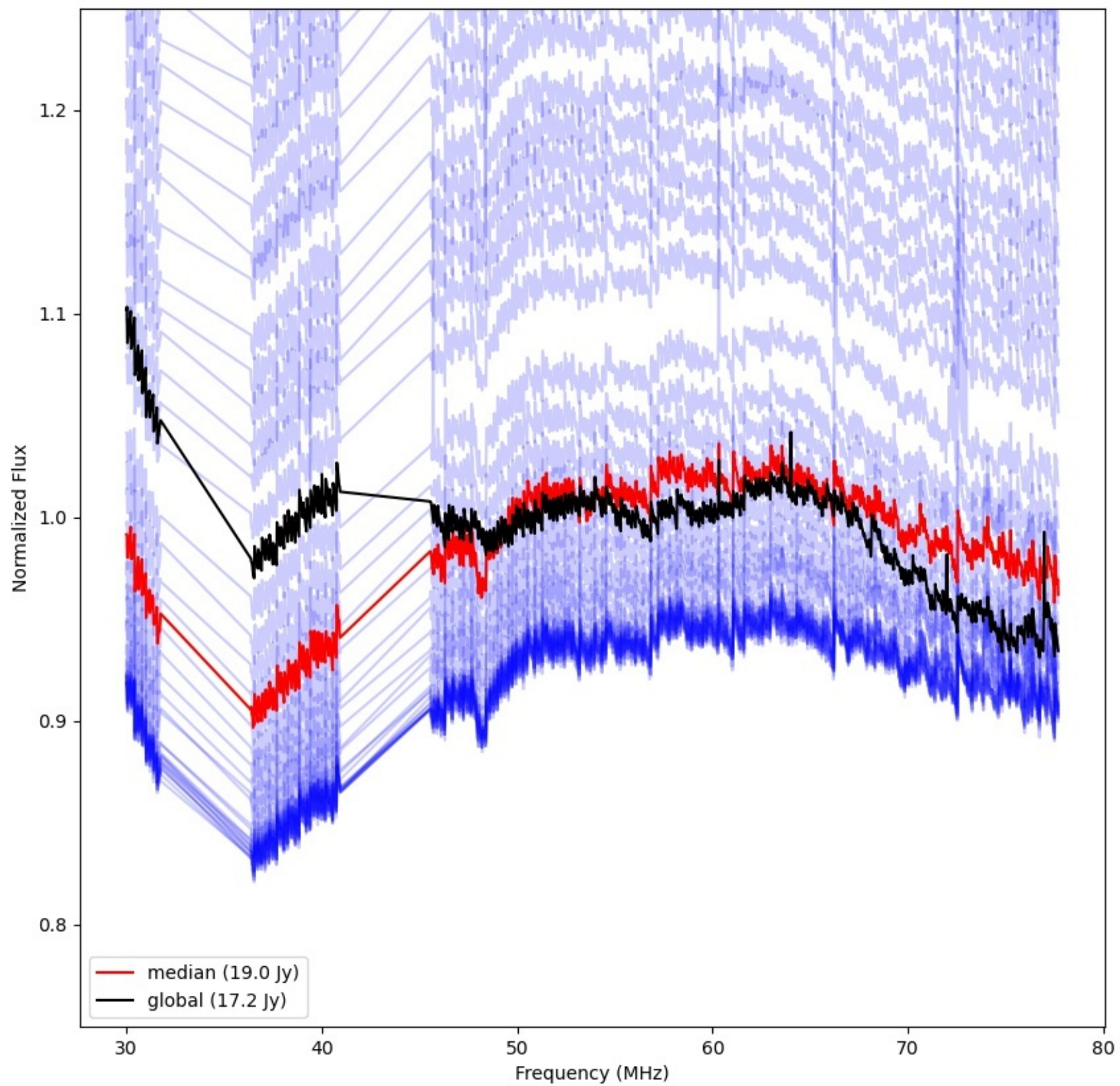
LWA137 - Correlator# 258 - YY - FLAGS:Good
