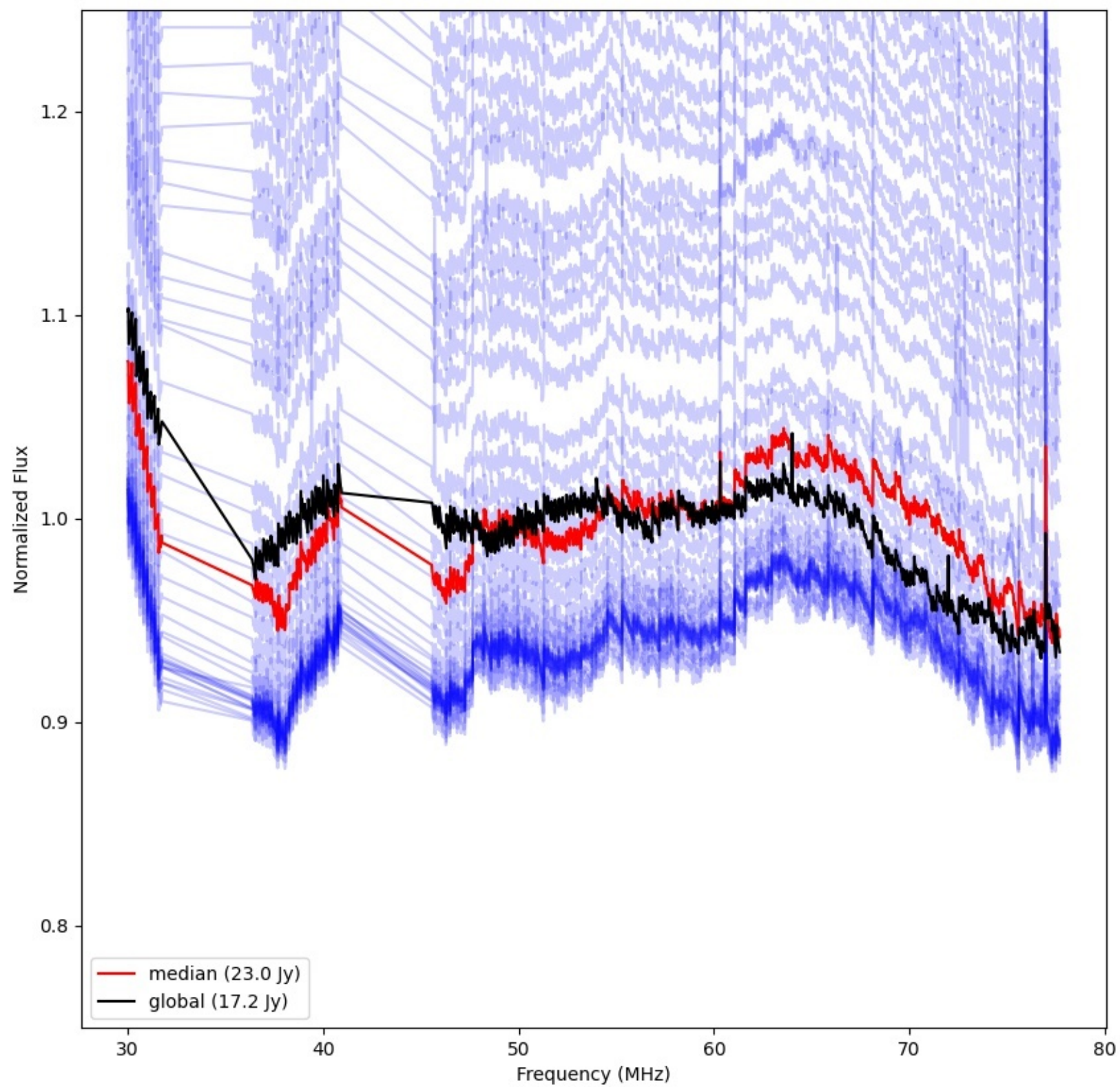
LWA331 - Correlator# 125 - YY - FLAGS:Good
