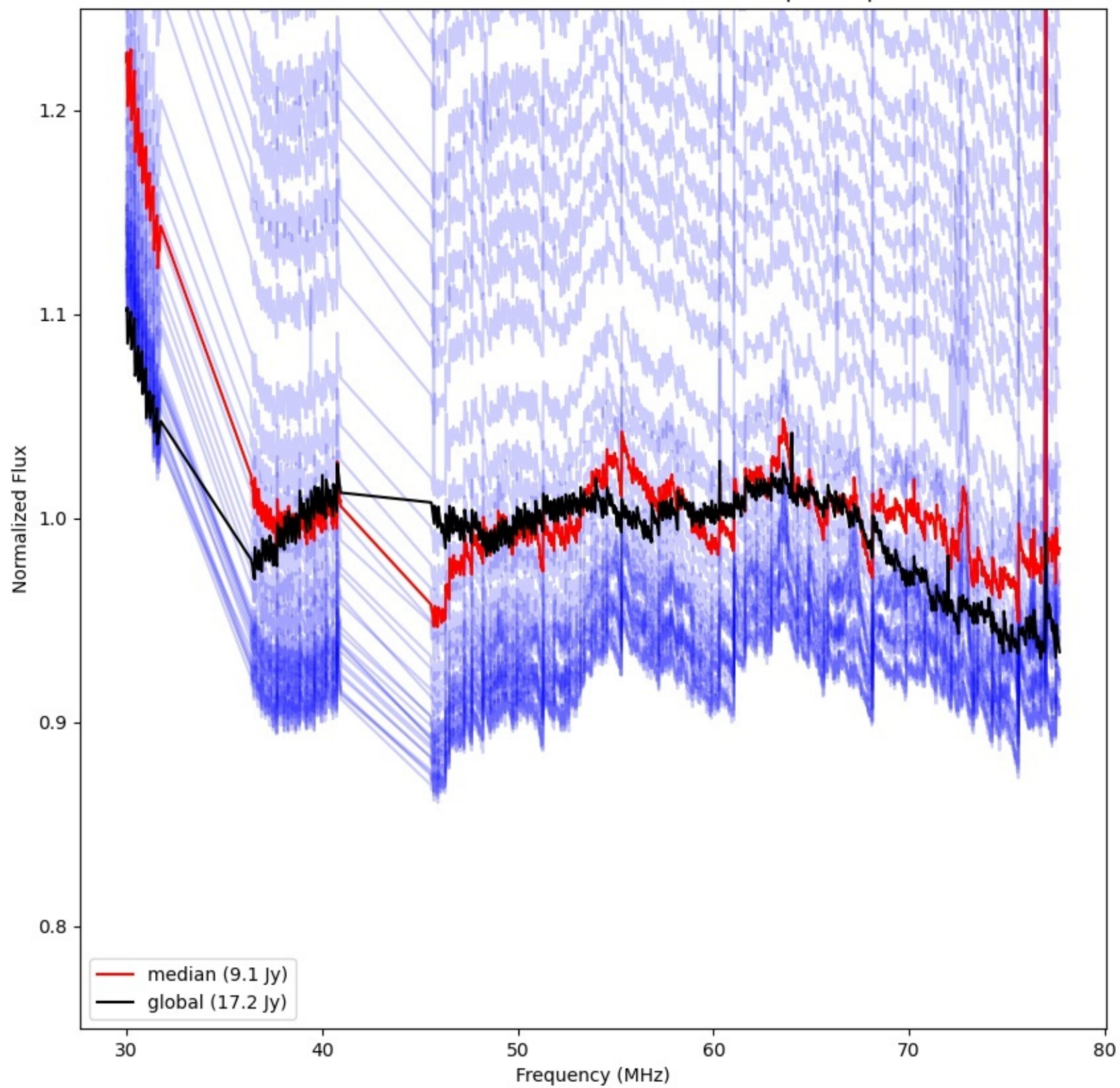
LWA319 - Correlator# 190 - YY - FLAGS:BadSpecShape
