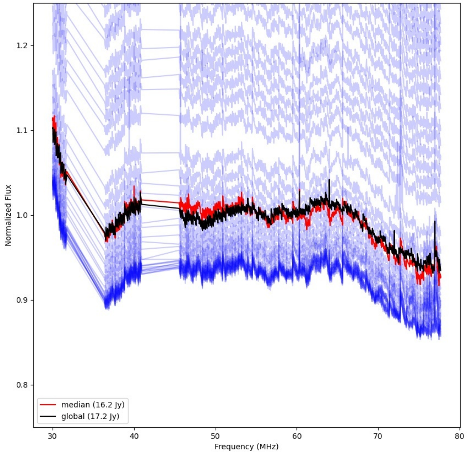
LWA155 - Correlator# 232 - YY - FLAGS:Good
