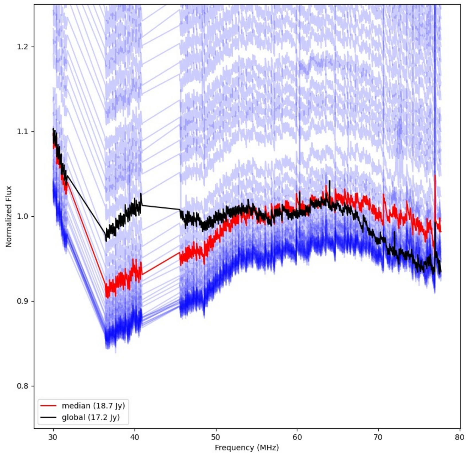
LWA161 - Correlator# 262 - YY - FLAGS:Good
