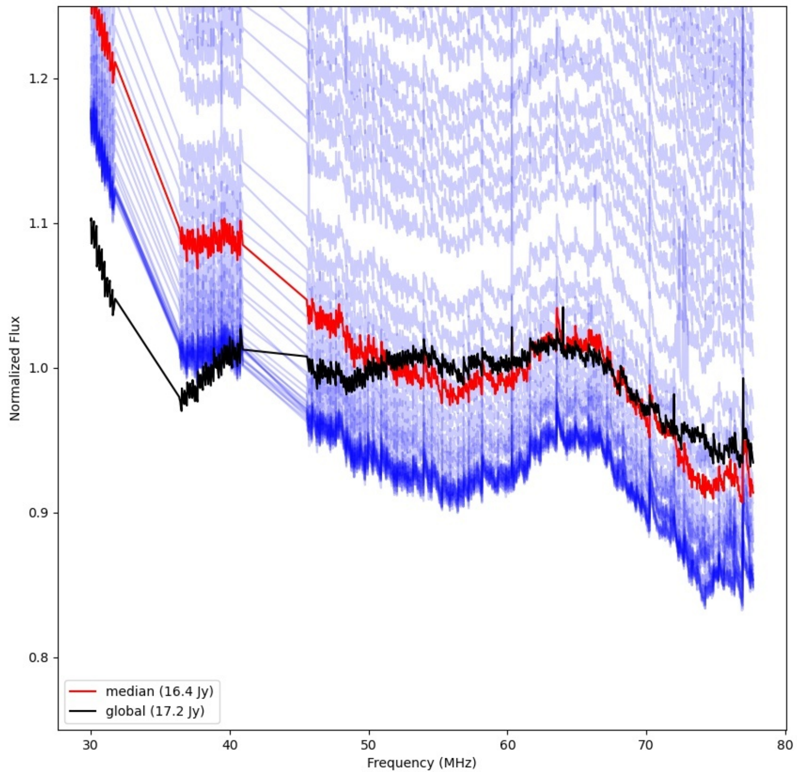
LWA241 - Correlator# 336 - YY - FLAGS:Good
