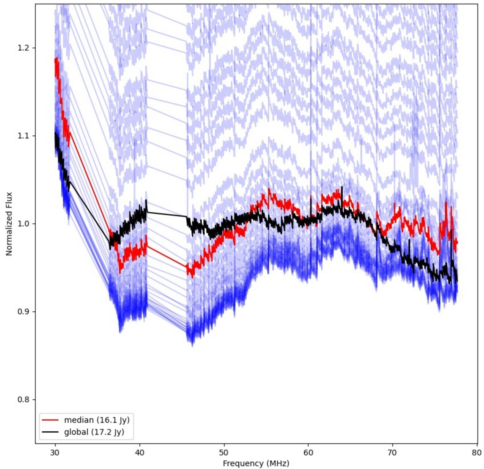
LWA340 - Correlator# 026 - YY - FLAGS:Good
