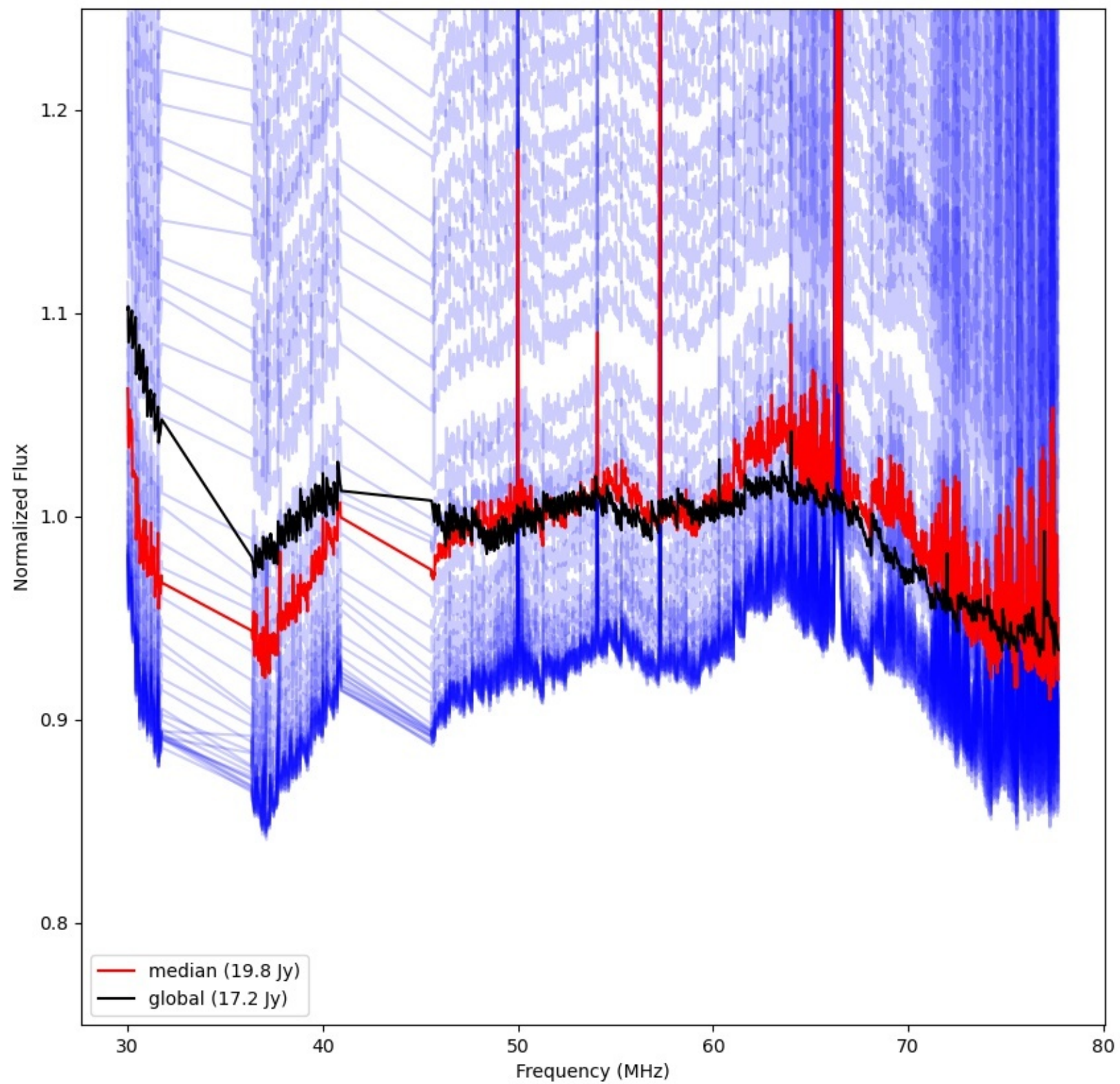
LWA364 - Correlator# 127 - YY - FLAGS:Good
