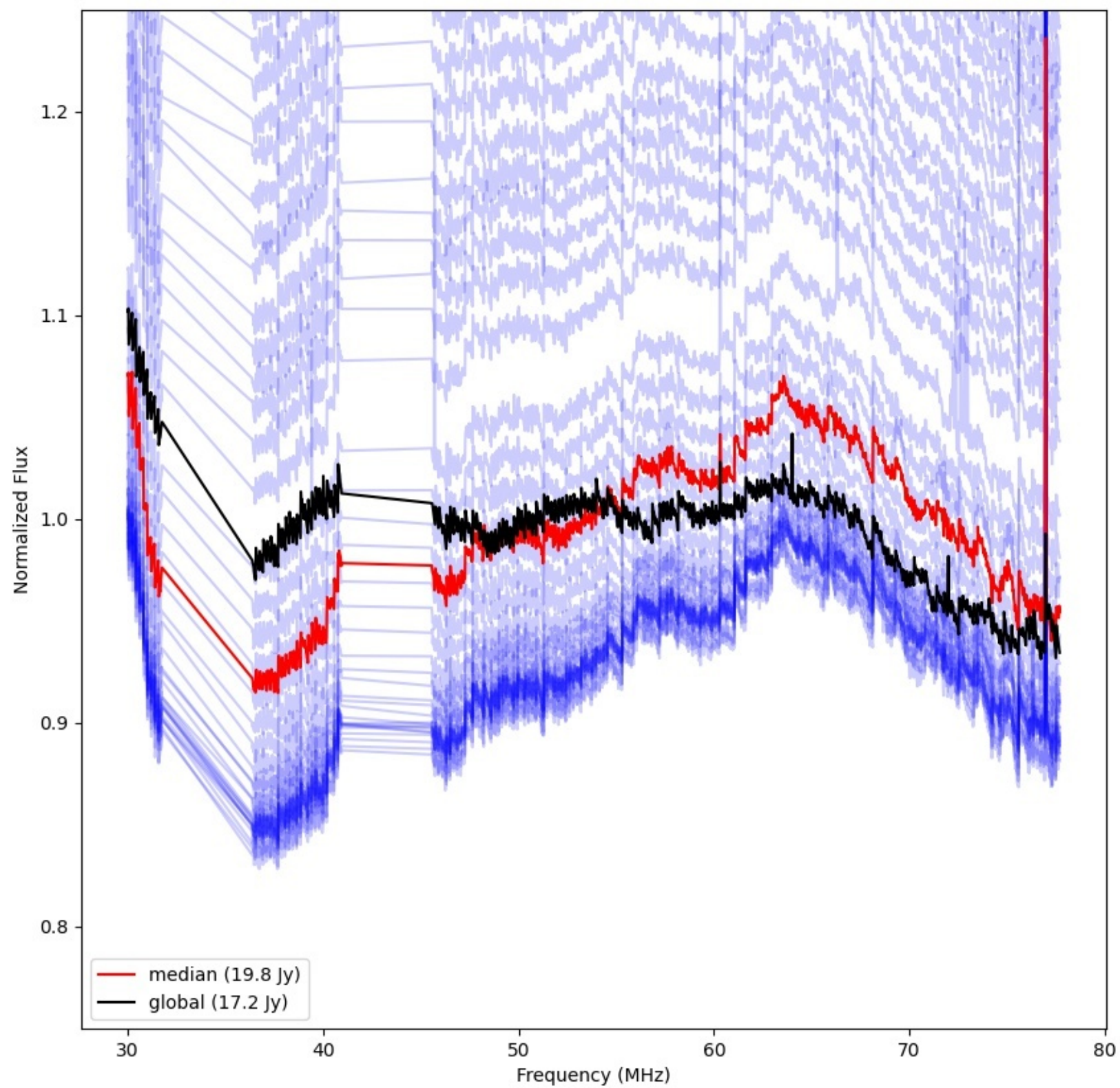
LWA333 - Correlator# 253 - YY - FLAGS:Good
