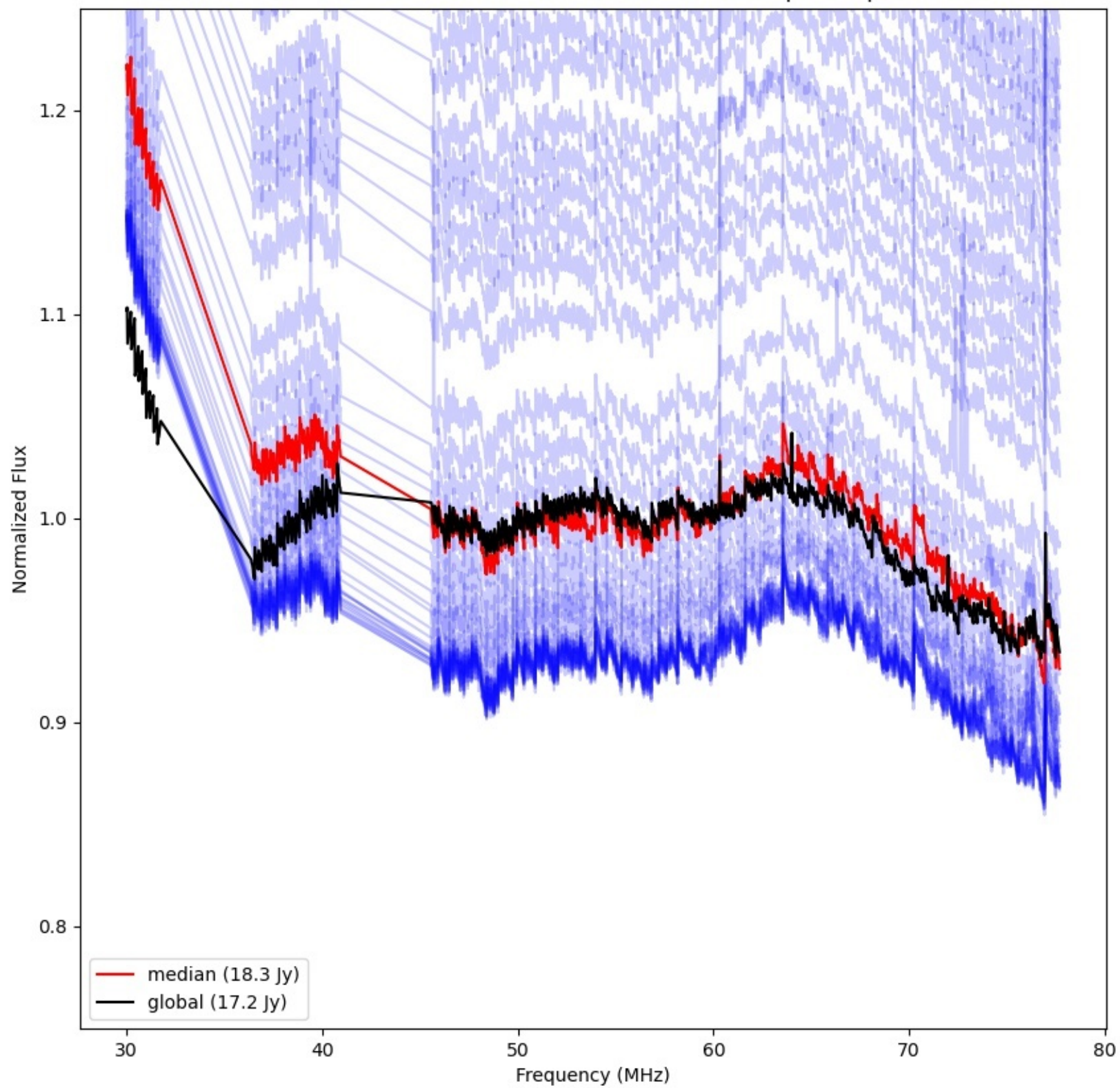
LWA076 - Correlator# 193 - YY - FLAGS:BadSpecShape
