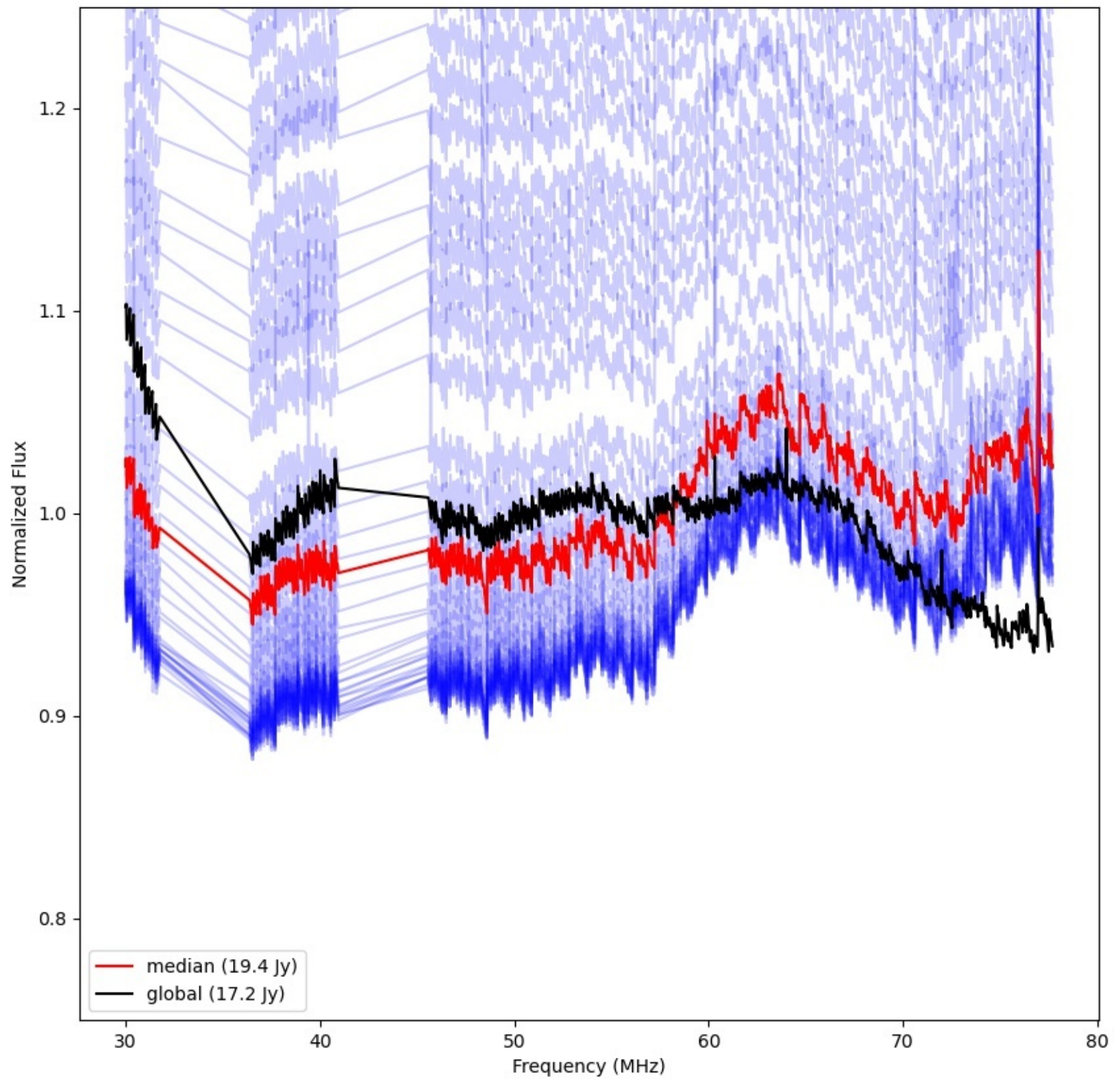
LWA033 - Correlator# 161 - YY - FLAGS:Good
