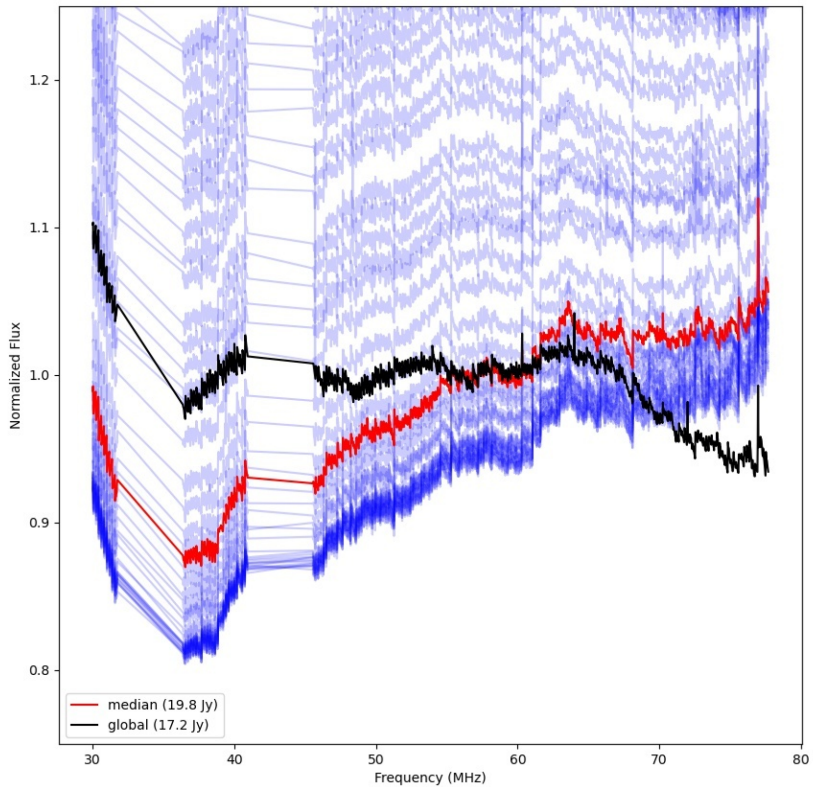
LWA288 - Correlator# 042 - YY - FLAGS:Good
