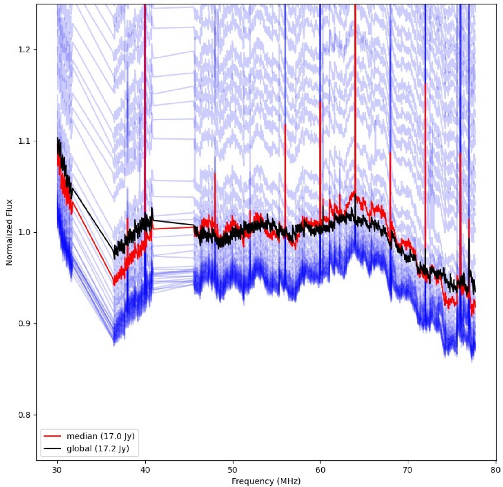
LWA128 - Correlator# 229 - YY - FLAGS:Good
