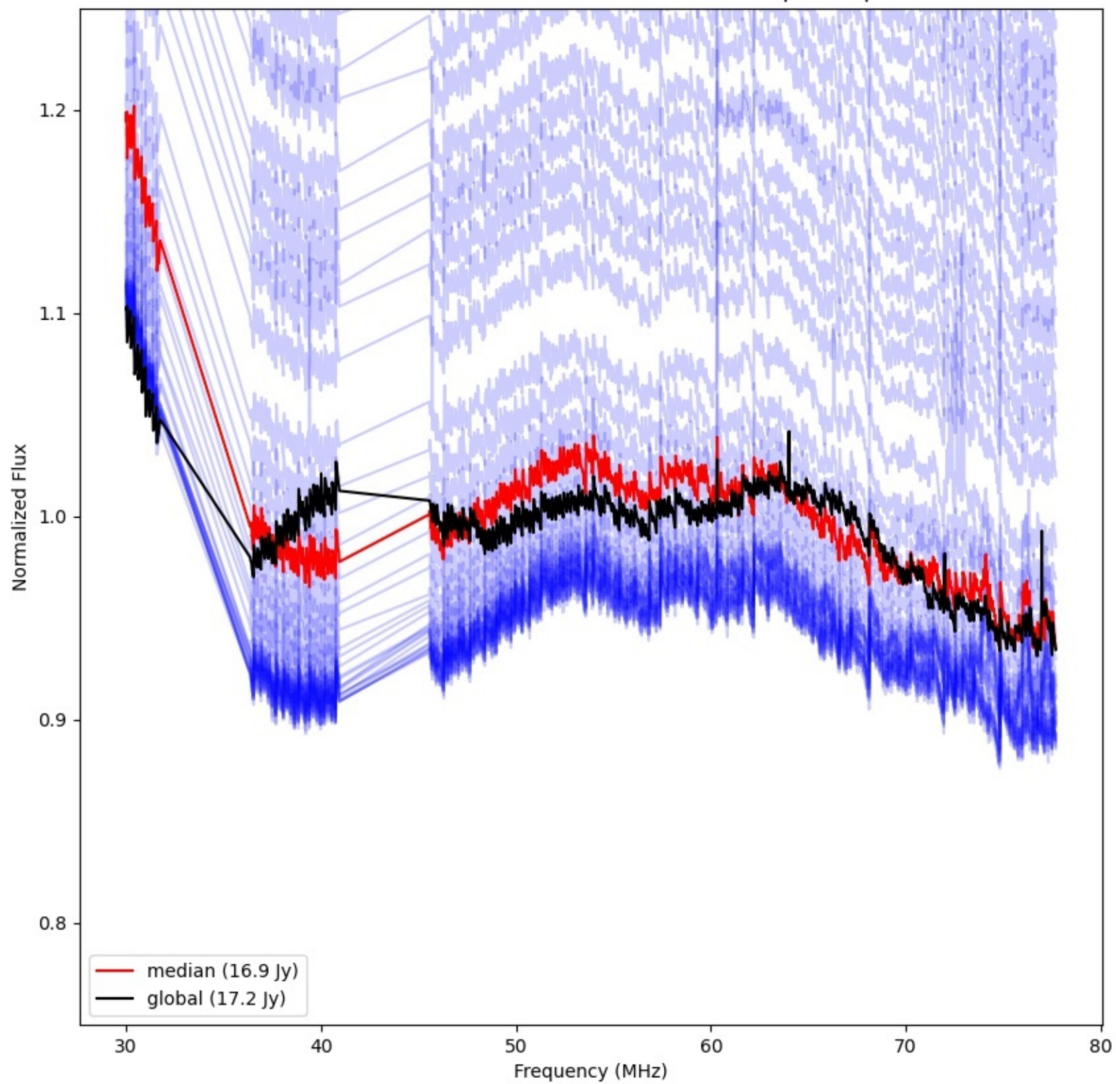
LWA075 - Correlator# 089 - YY - FLAGS:BadSpecShape
