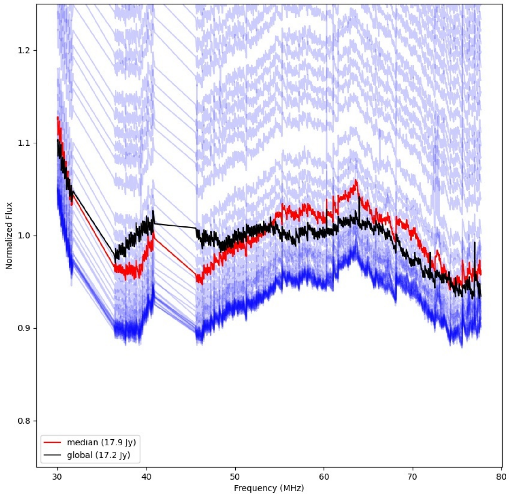
LWA338 - Correlator# 024 - YY - FLAGS:Good
