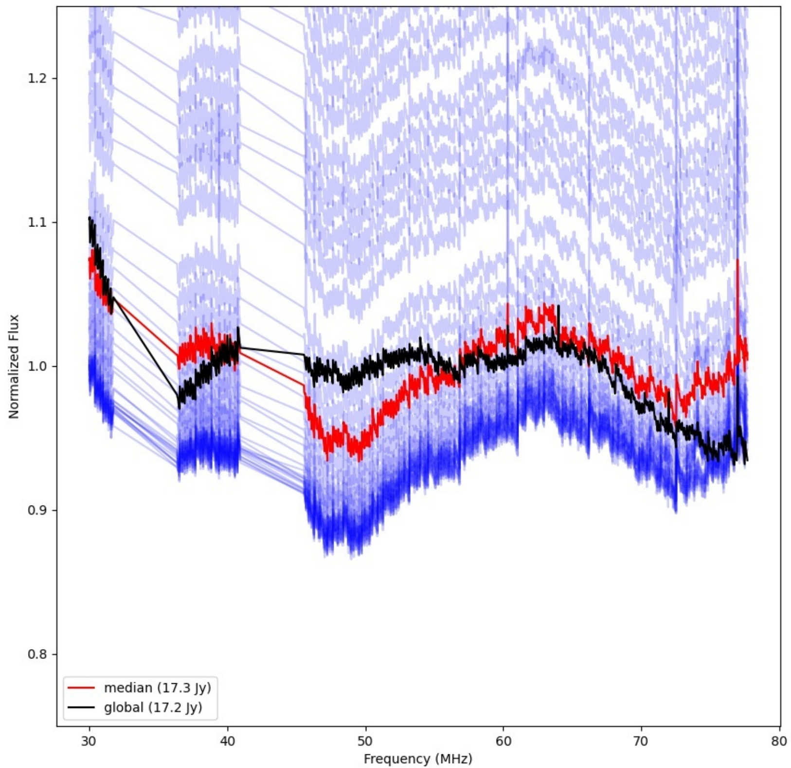
LWA042 - Correlator# 078 - YY - FLAGS:Good
