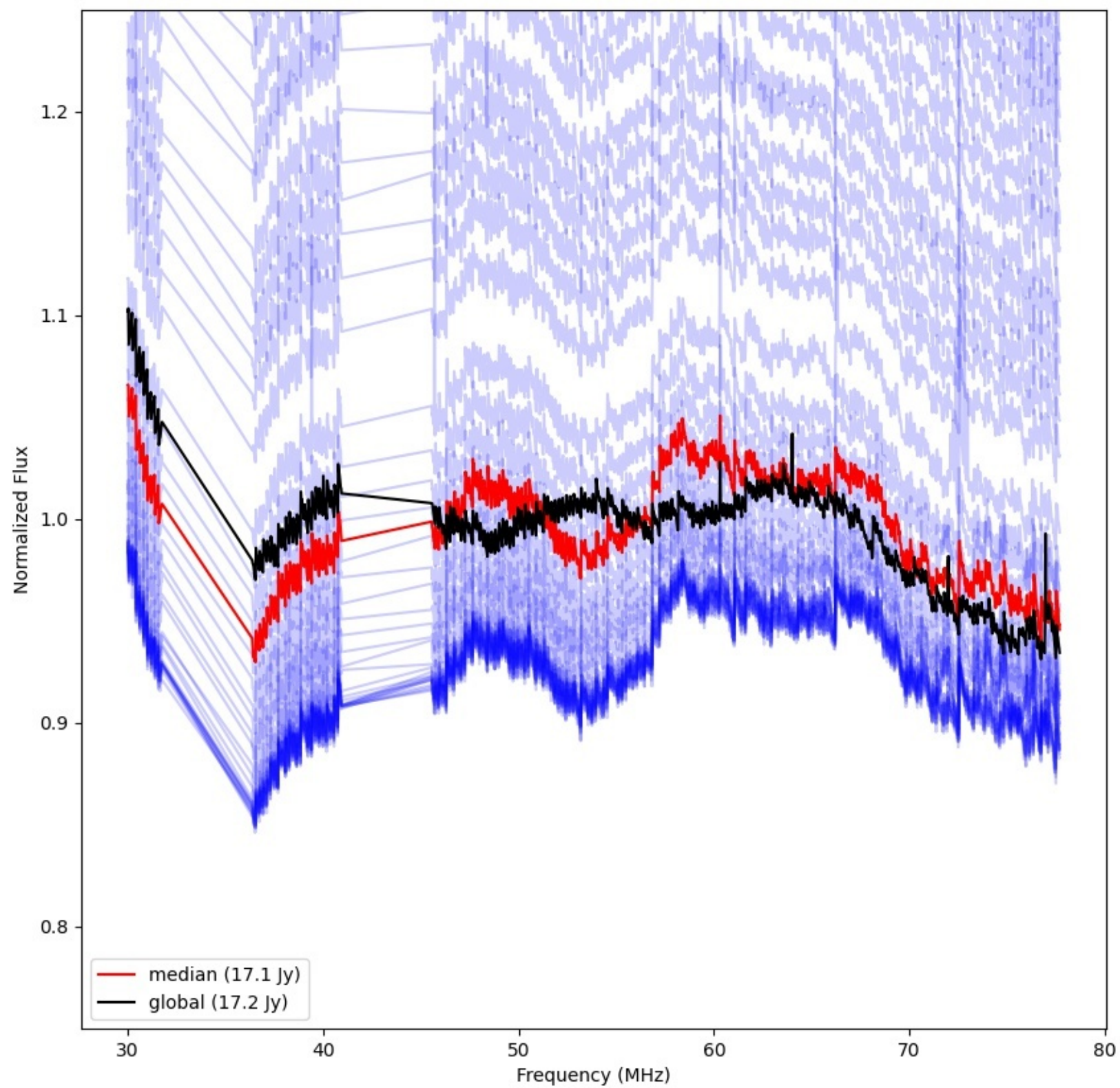
LWA133 - Correlator# 257 - YY - FLAGS:Good
