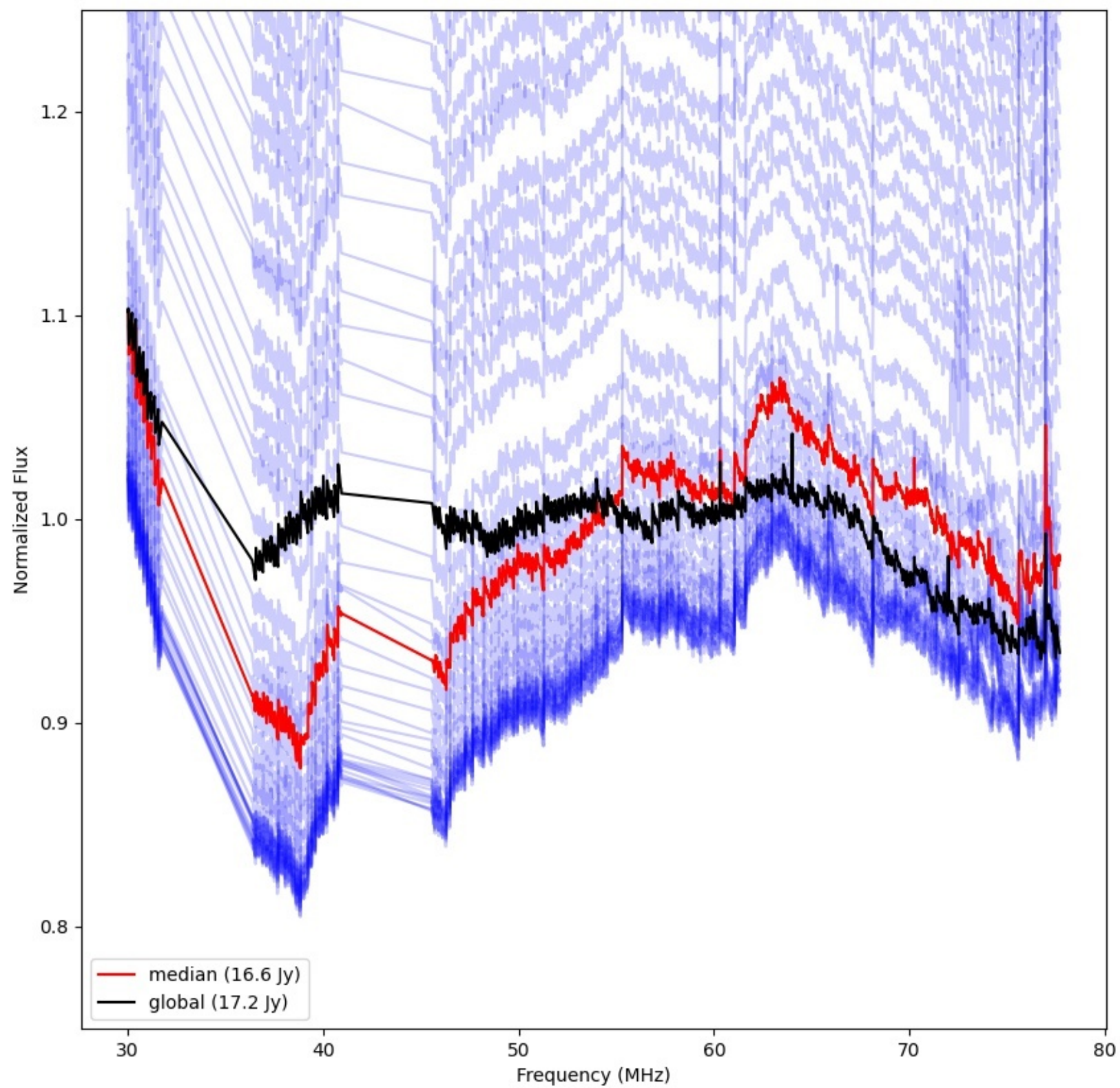
LWA305 - Correlator# 050 - YY - FLAGS:Good
