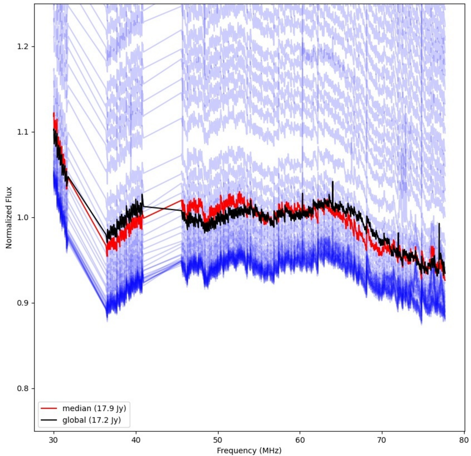
LWA013 - Correlator# 096 - YY - FLAGS:Good
