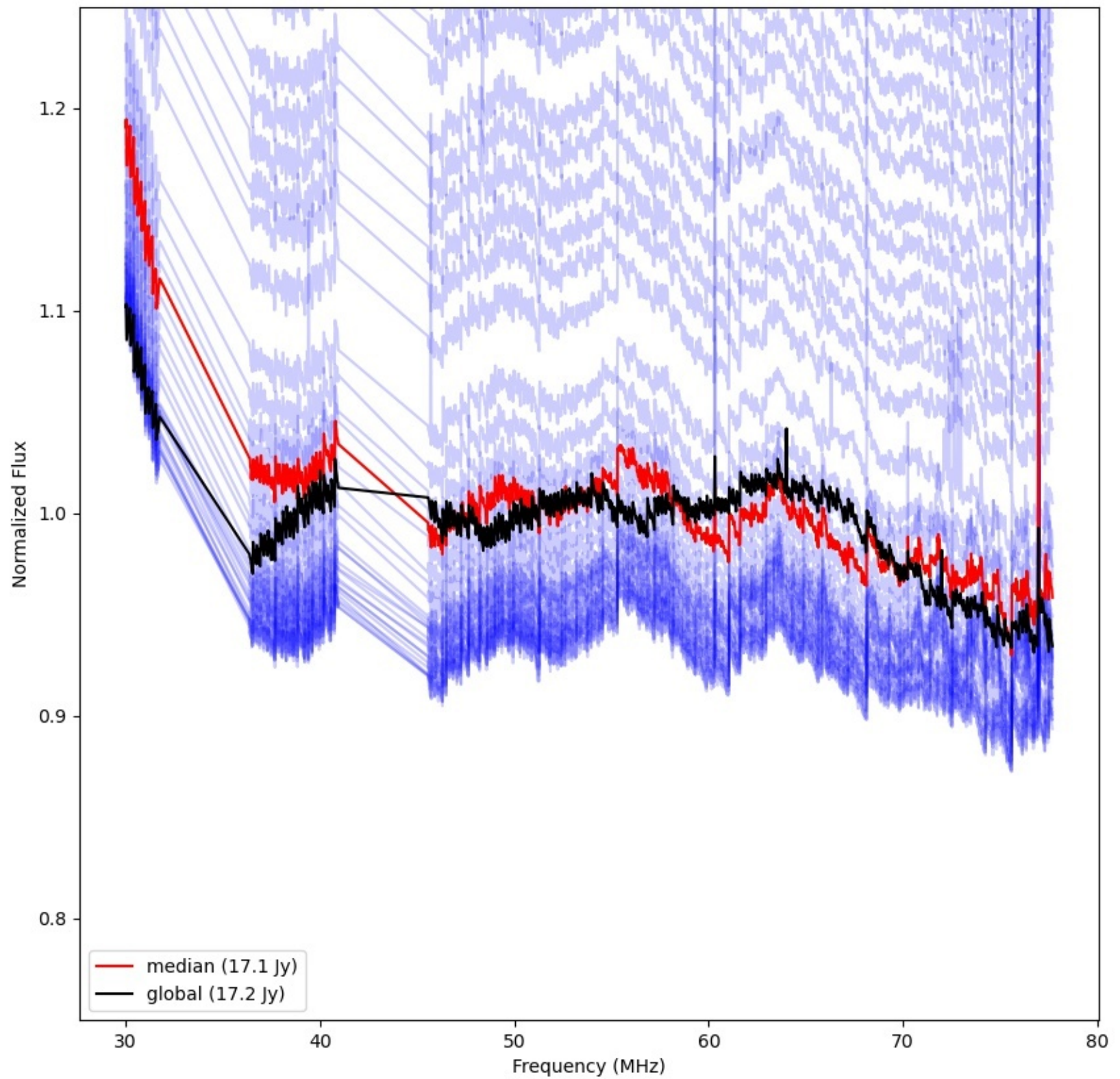
LWA284 - Correlator# 043 - YY - FLAGS:Good
