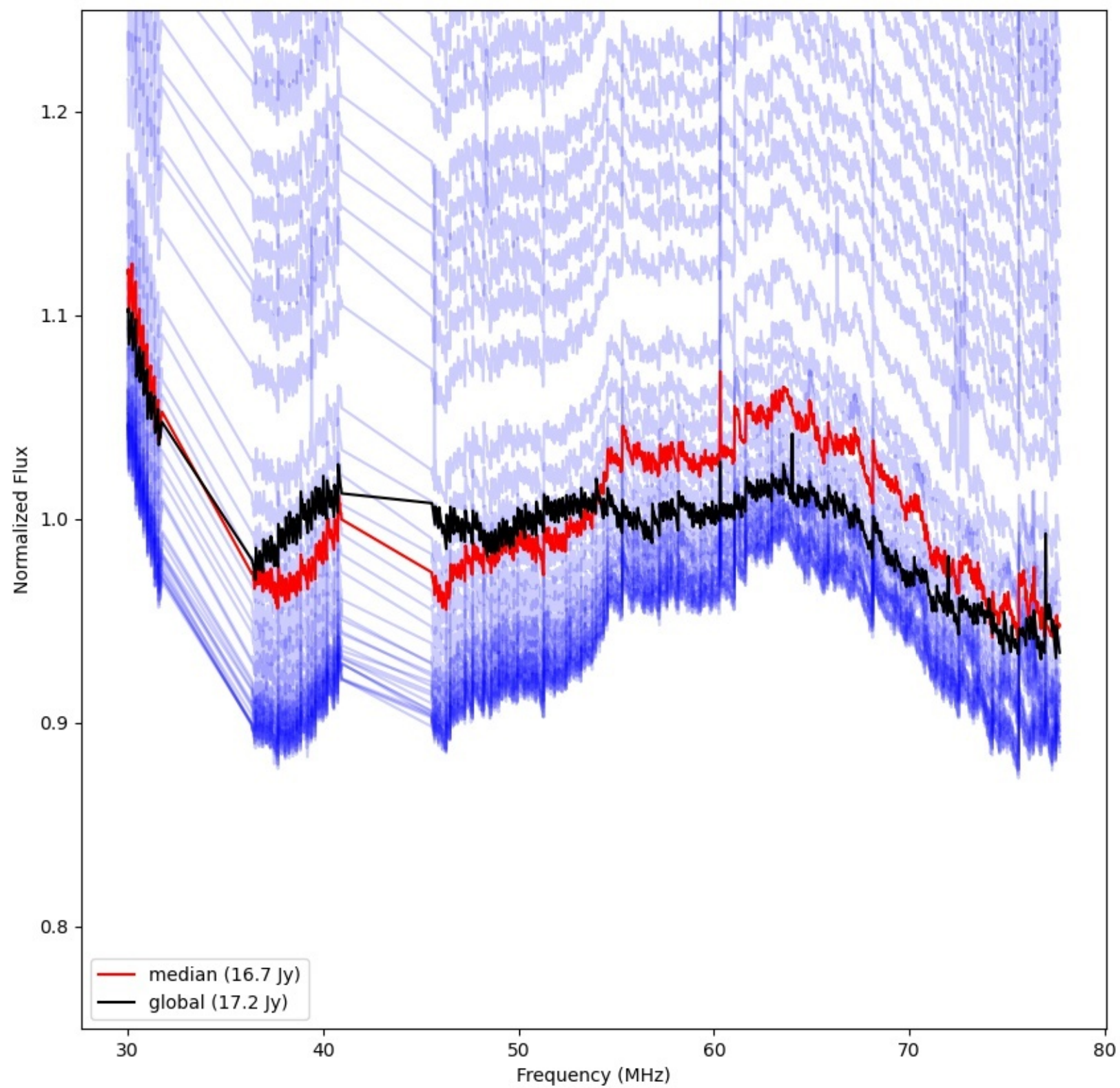
LWA267 - Correlator# 003 - YY - FLAGS:Good
