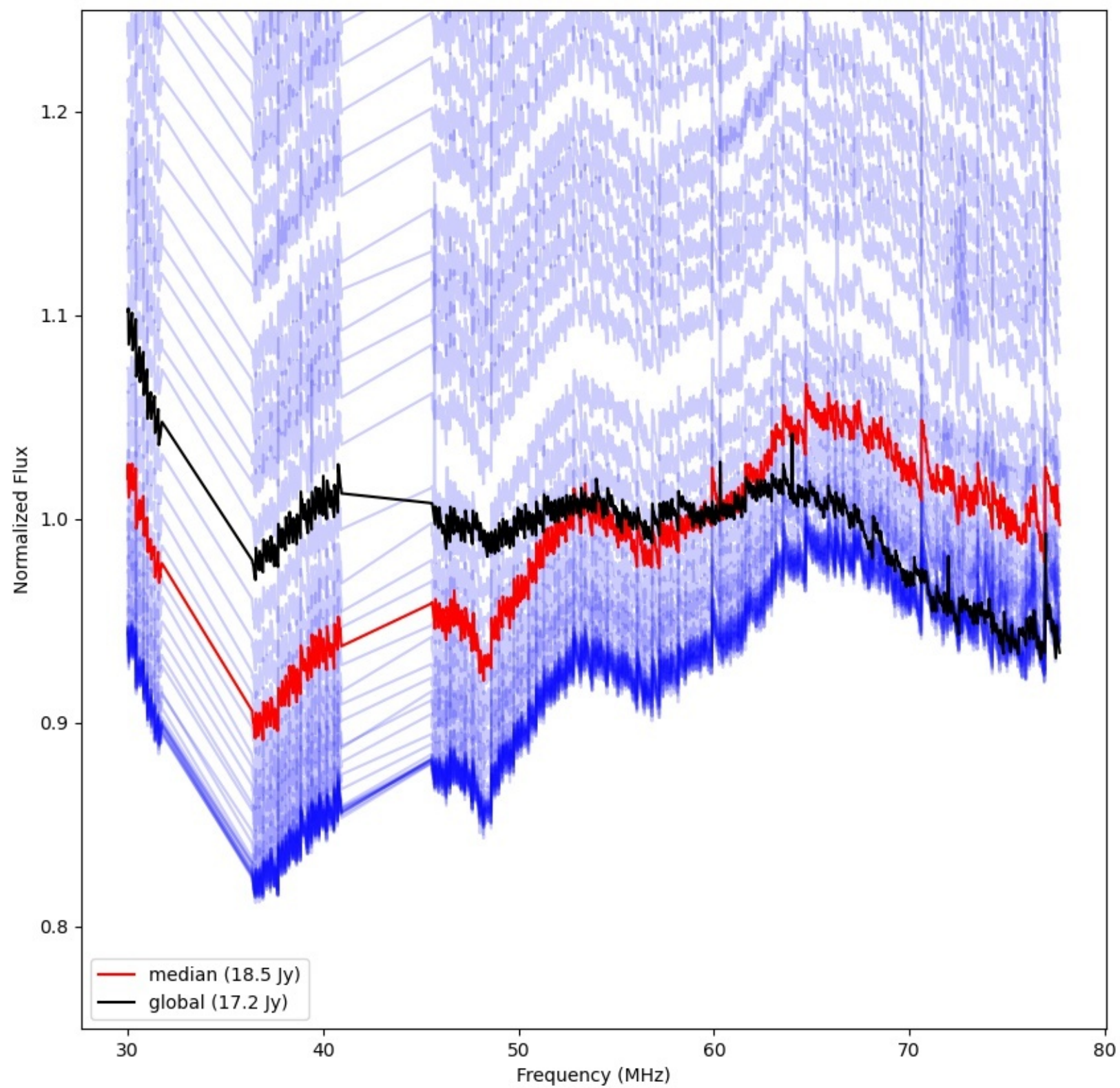
LWA225 - Correlator# 281 - YY - FLAGS:Good
