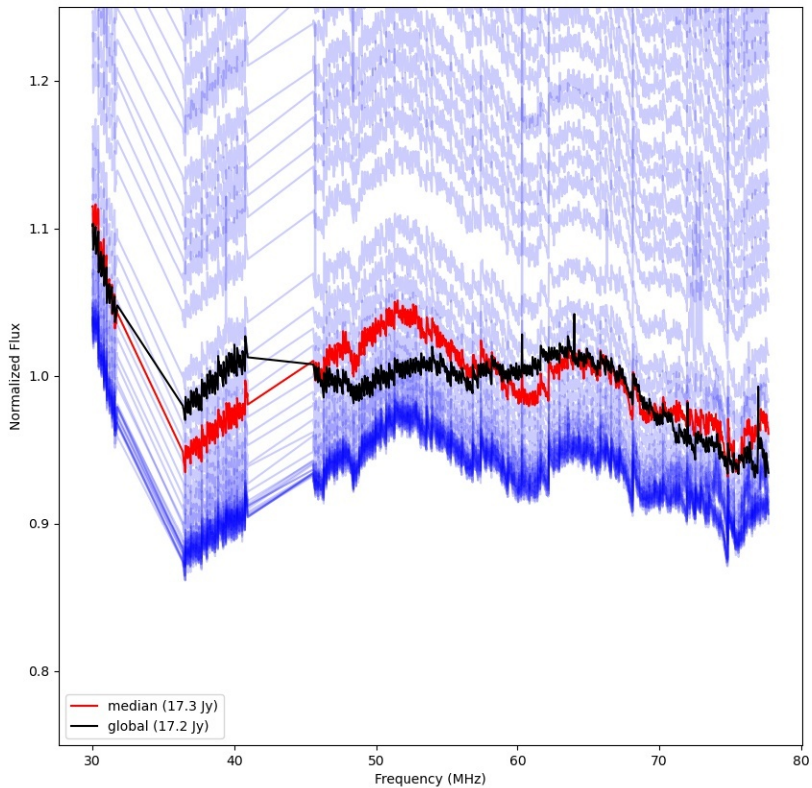
LWA138 - Correlator# 261 - YY - FLAGS:Good
