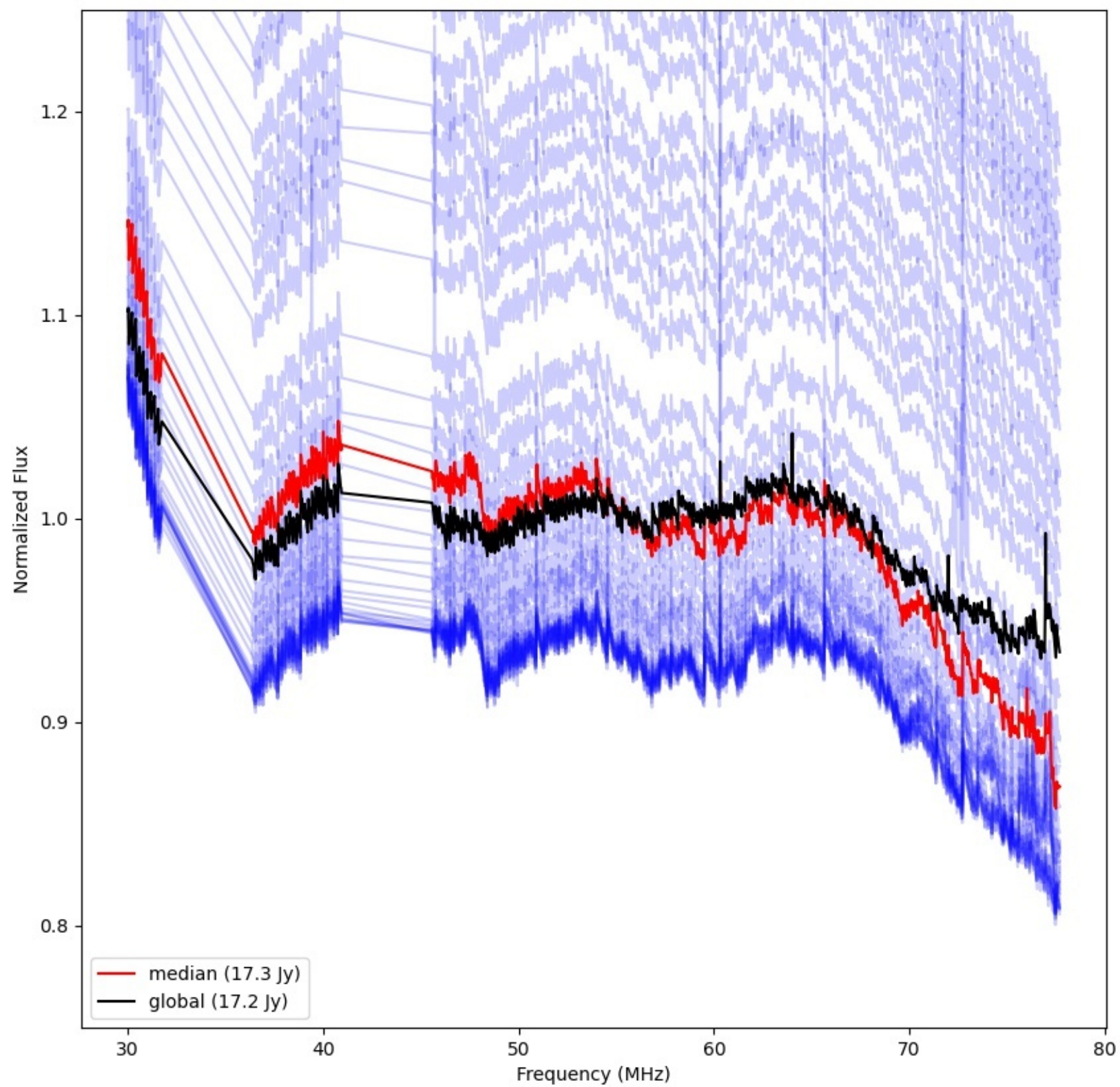
LWA184 - Correlator# 241 - YY - FLAGS:Good
