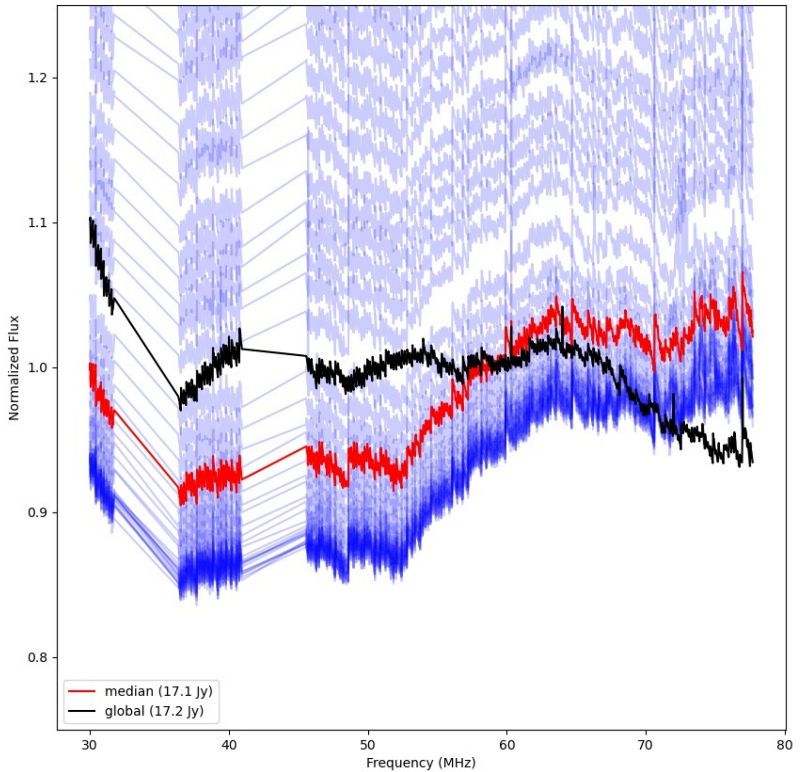
LWA034 - Correlator# 162 - YY - FLAGS:Good
