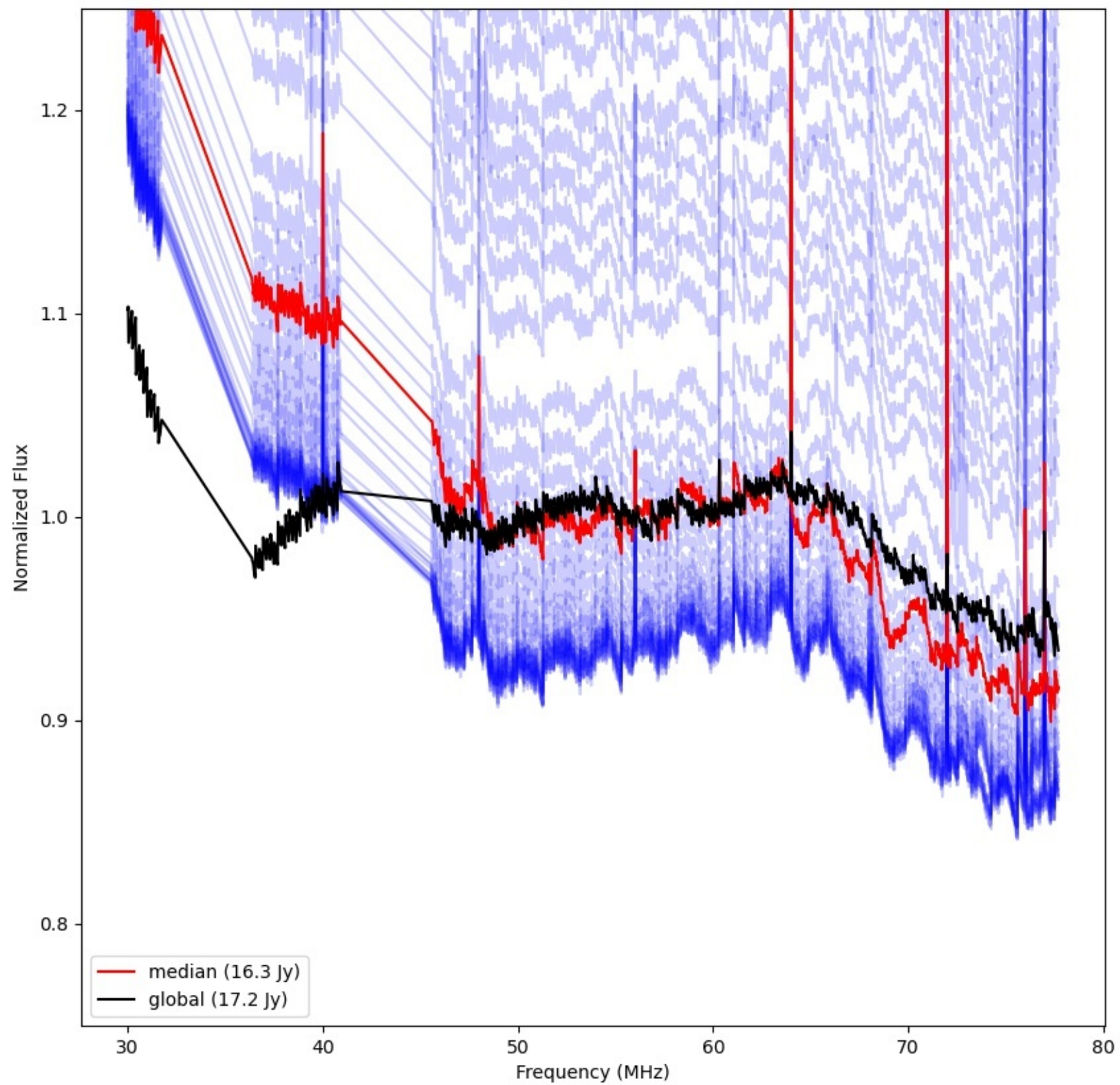
LWA095 - Correlator# 150 - YY - FLAGS:Good
