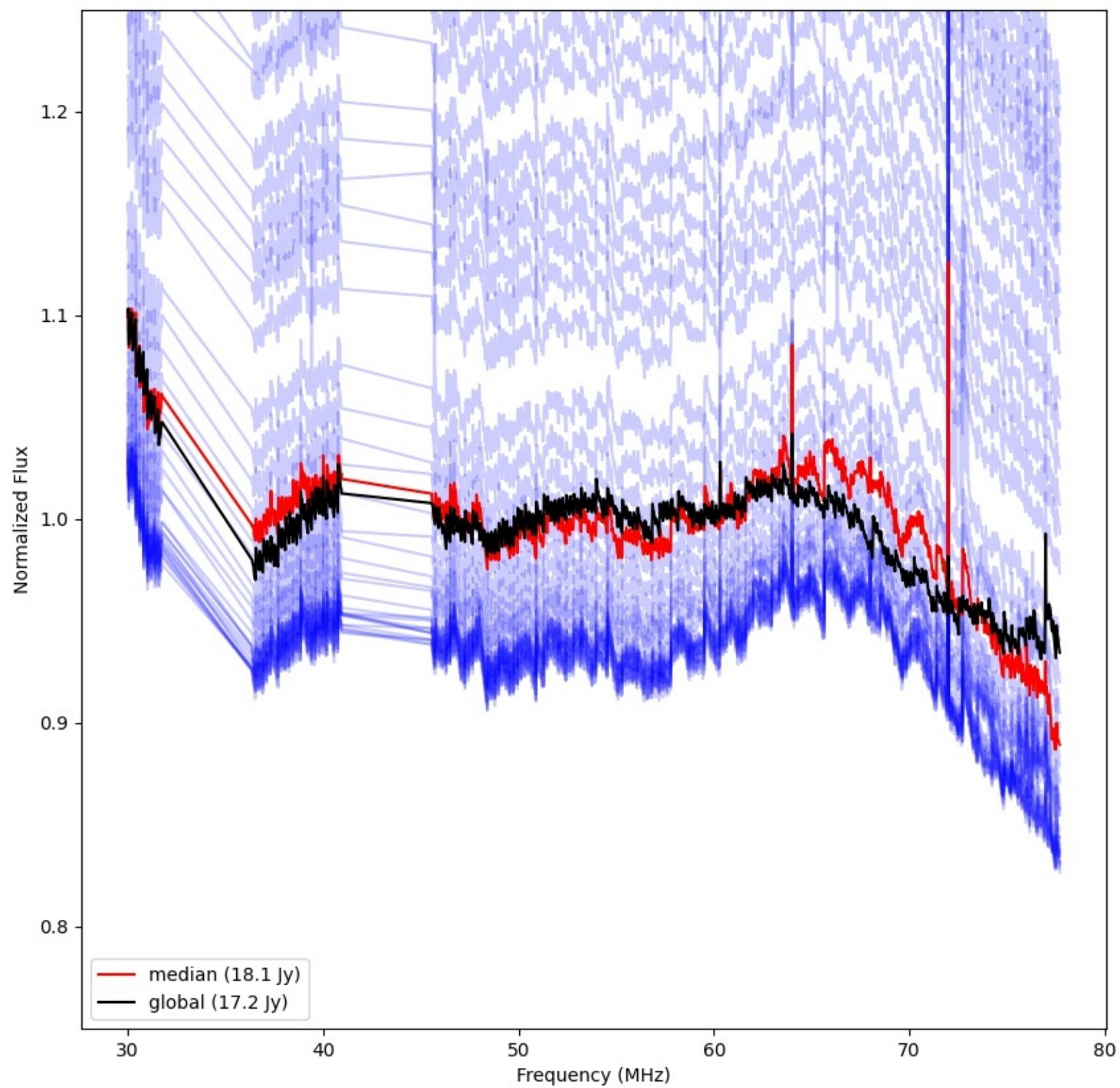
LWA223 - Correlator# 337 - YY - FLAGS:Good
