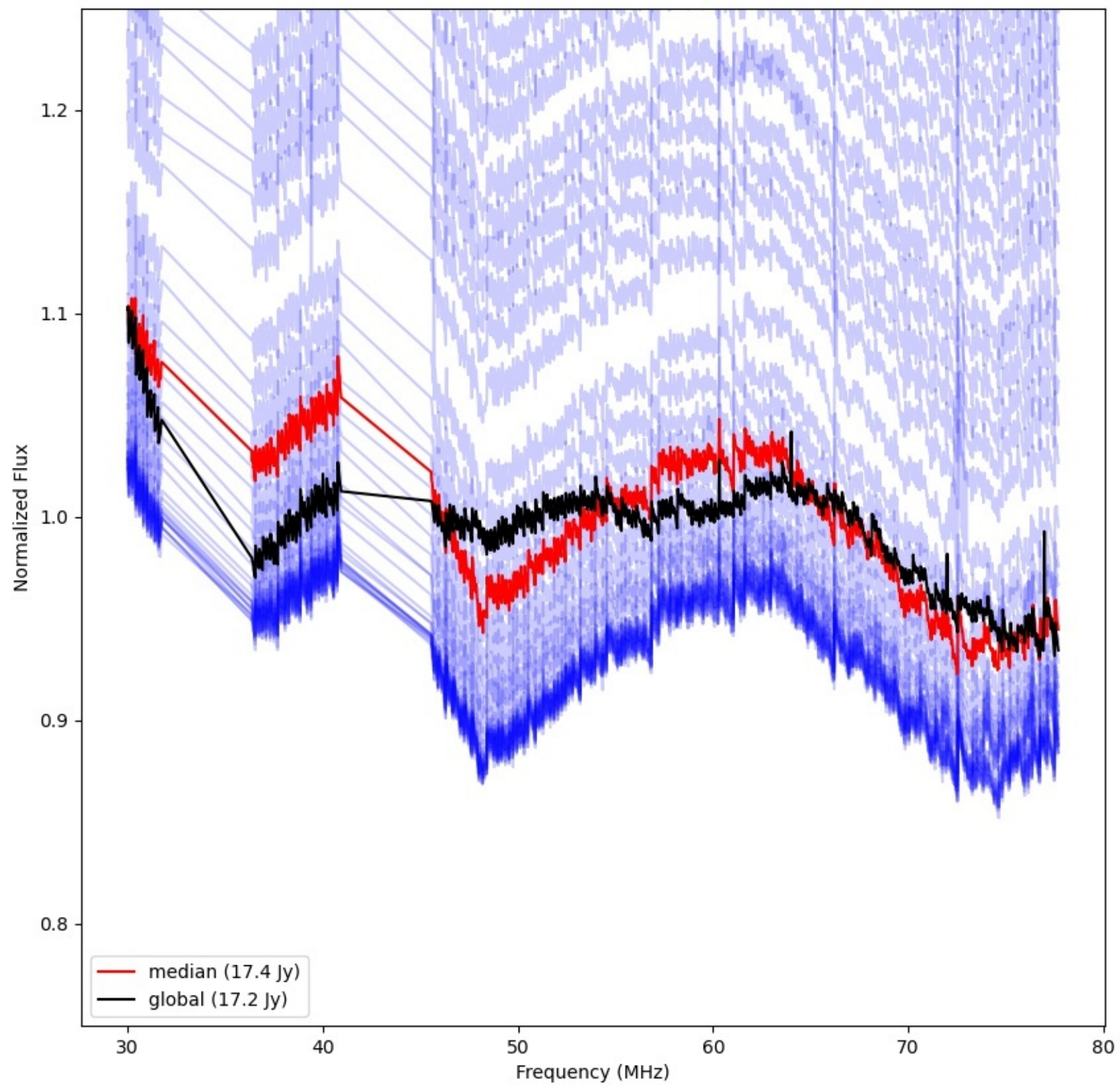
LWA040 - Correlator# 076 - YY - FLAGS:Good
