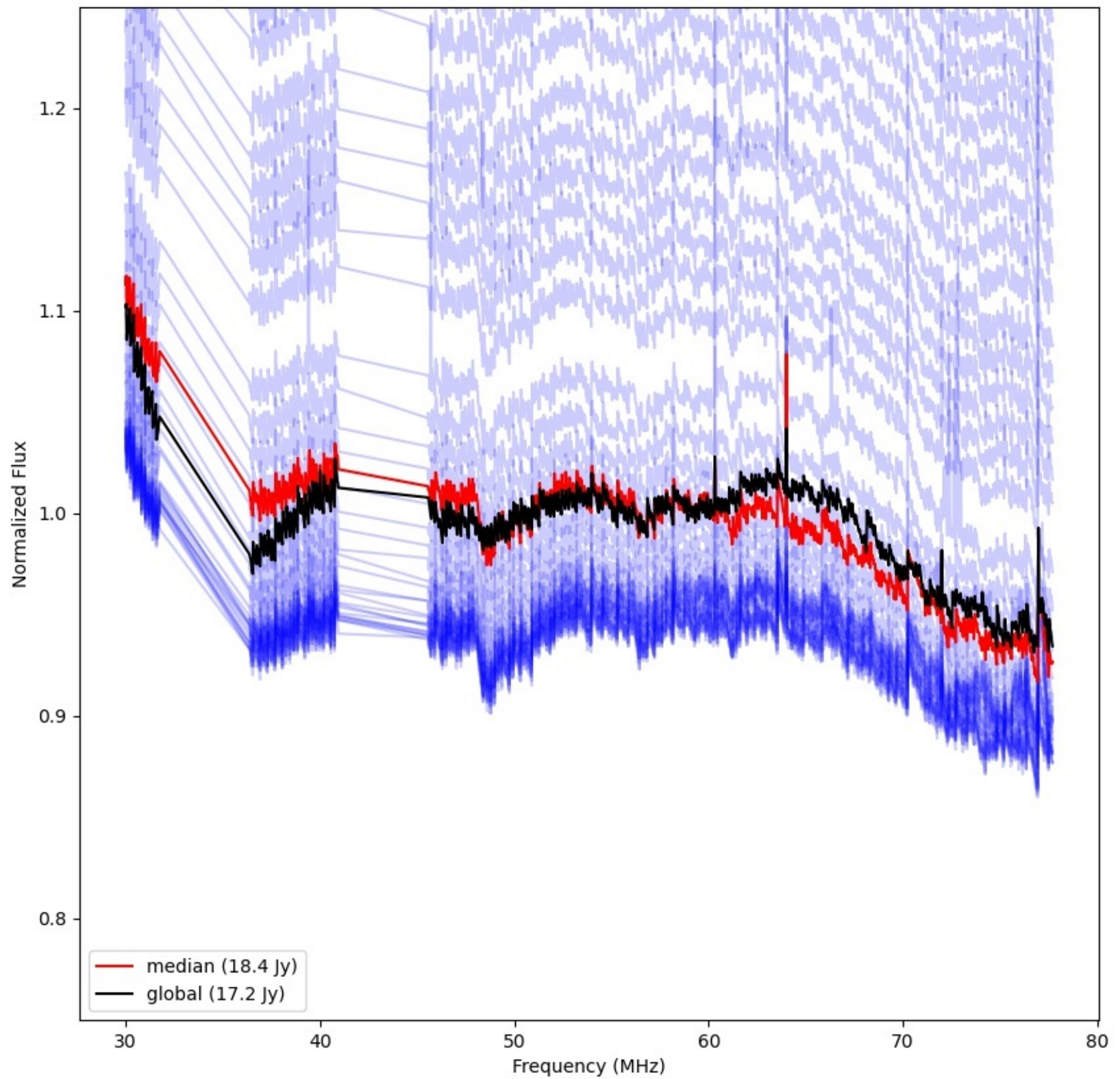
LWA029 - Correlator# 110 - YY - FLAGS:Good
