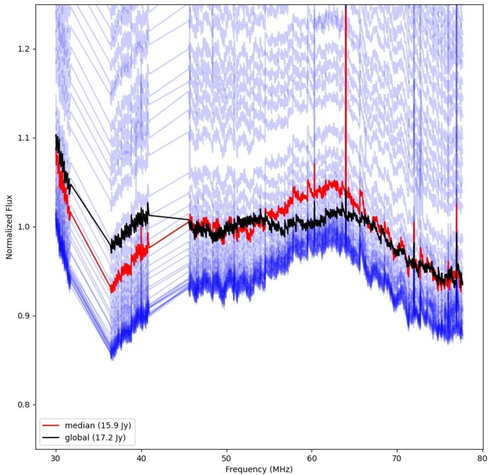
LWA091 - Correlator# 146 - YY - FLAGS:Good
