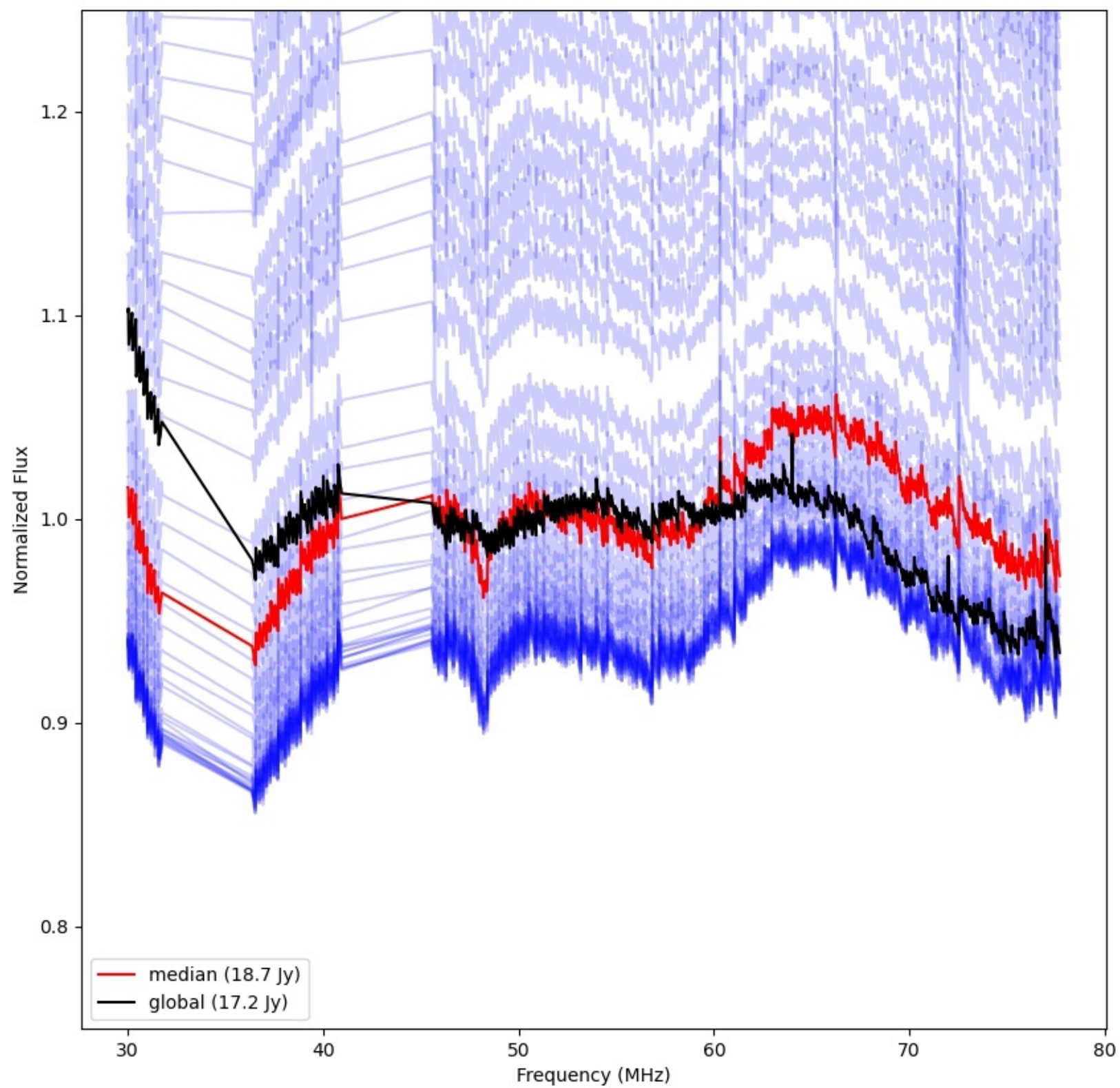
LWA199 - Correlator# 277 - YY - FLAGS:Good
