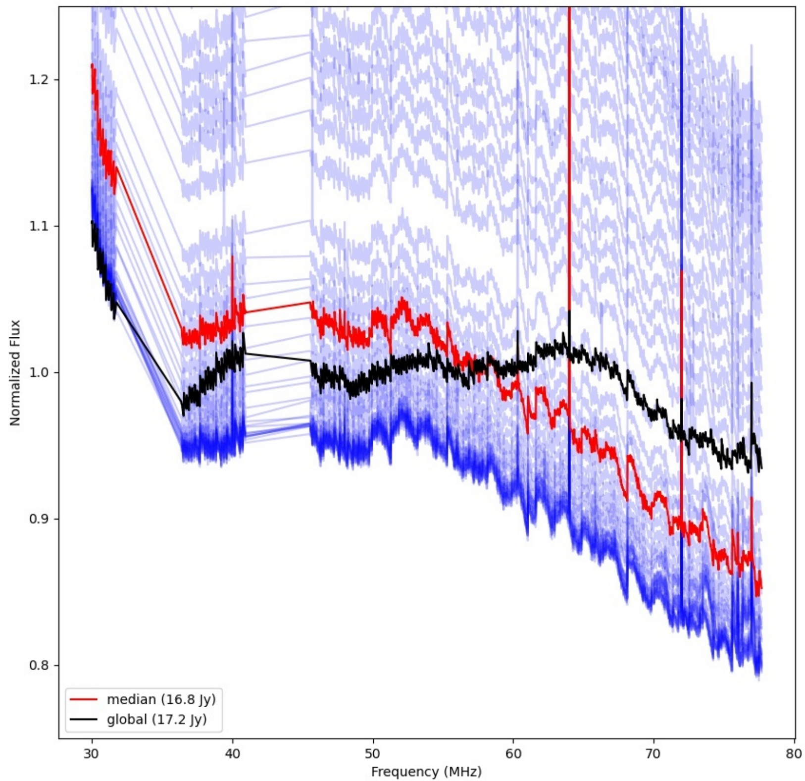
LWA063 - Correlator# 132 - YY - FLAGS:Good
