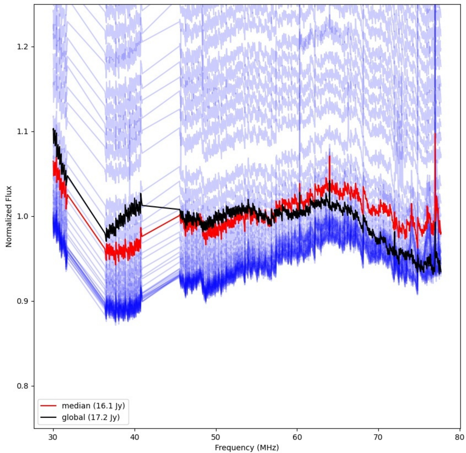
LWA021 - Correlator# 105 - YY - FLAGS:Good
