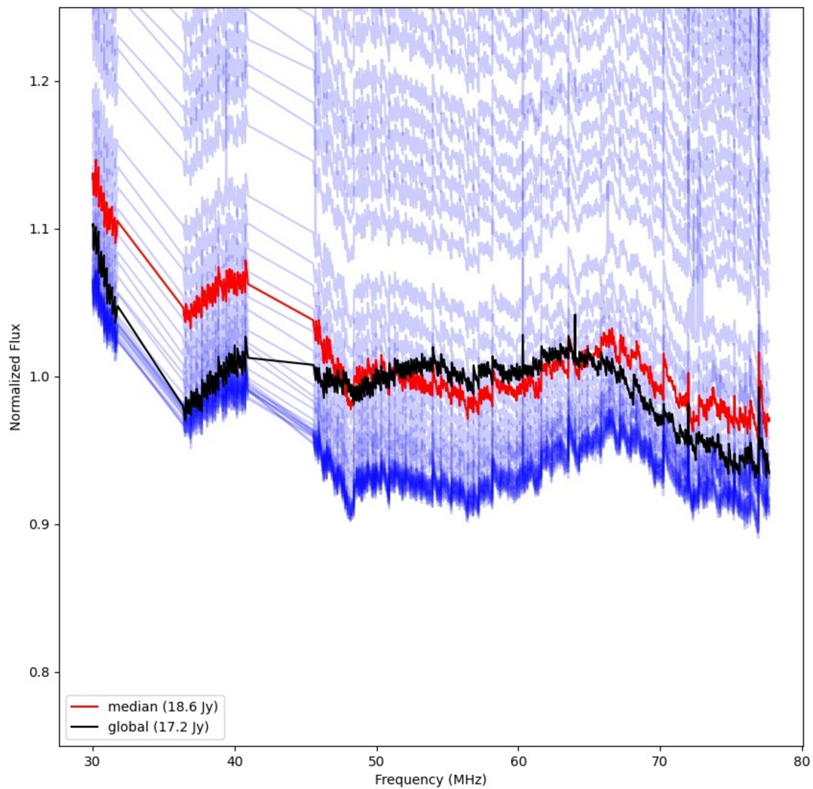
LWA247 - Correlator# 321 - YY - FLAGS:Good
