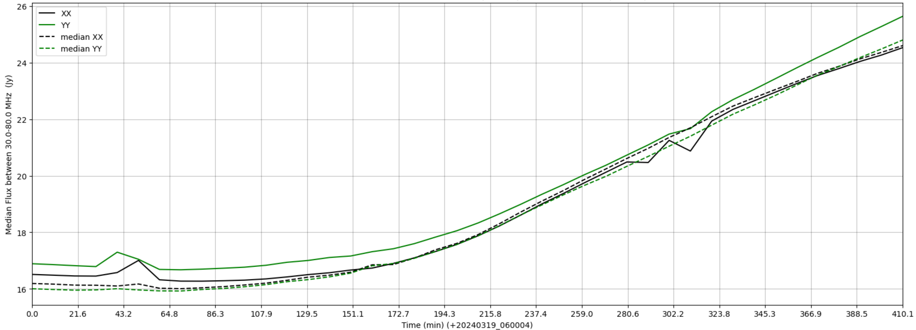
LWA003 - Correlator# 067 - XX FLAGS:BadSpecShape - YY FLAGS:BadSpecShape
