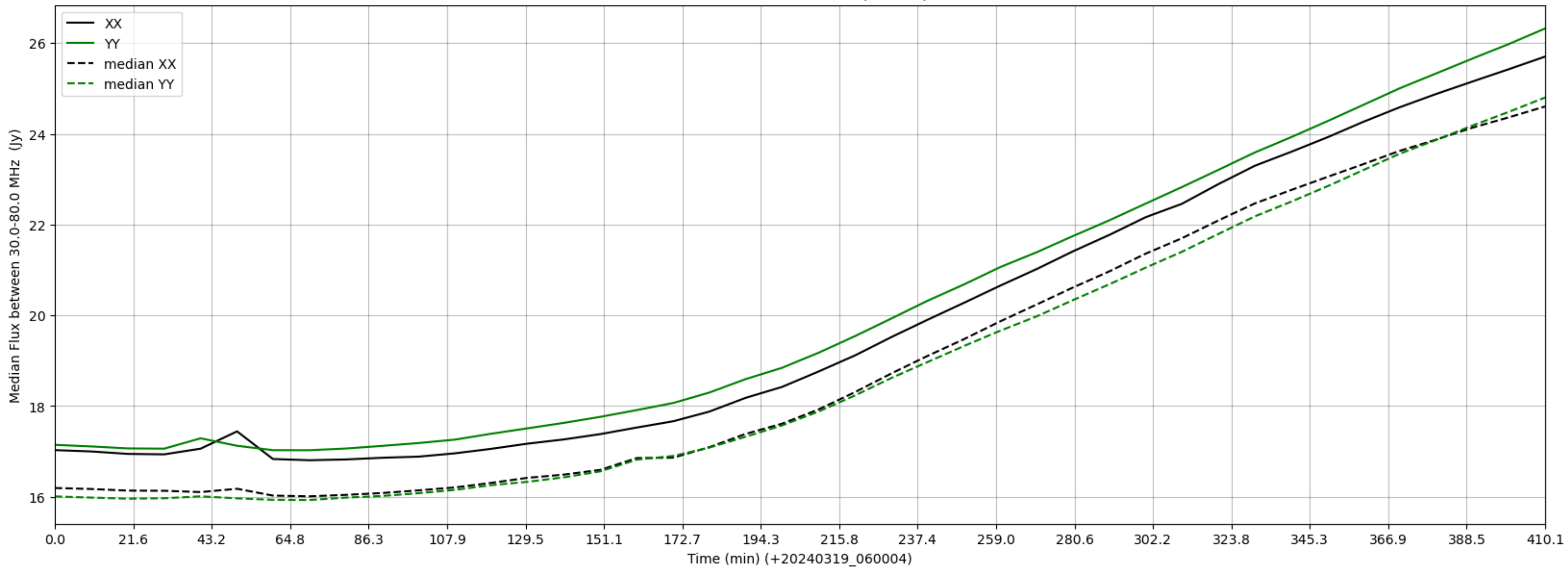
LWA114 - Correlator# 202 - XX FLAGS:BadSpecShape - YY FLAGS:Good
