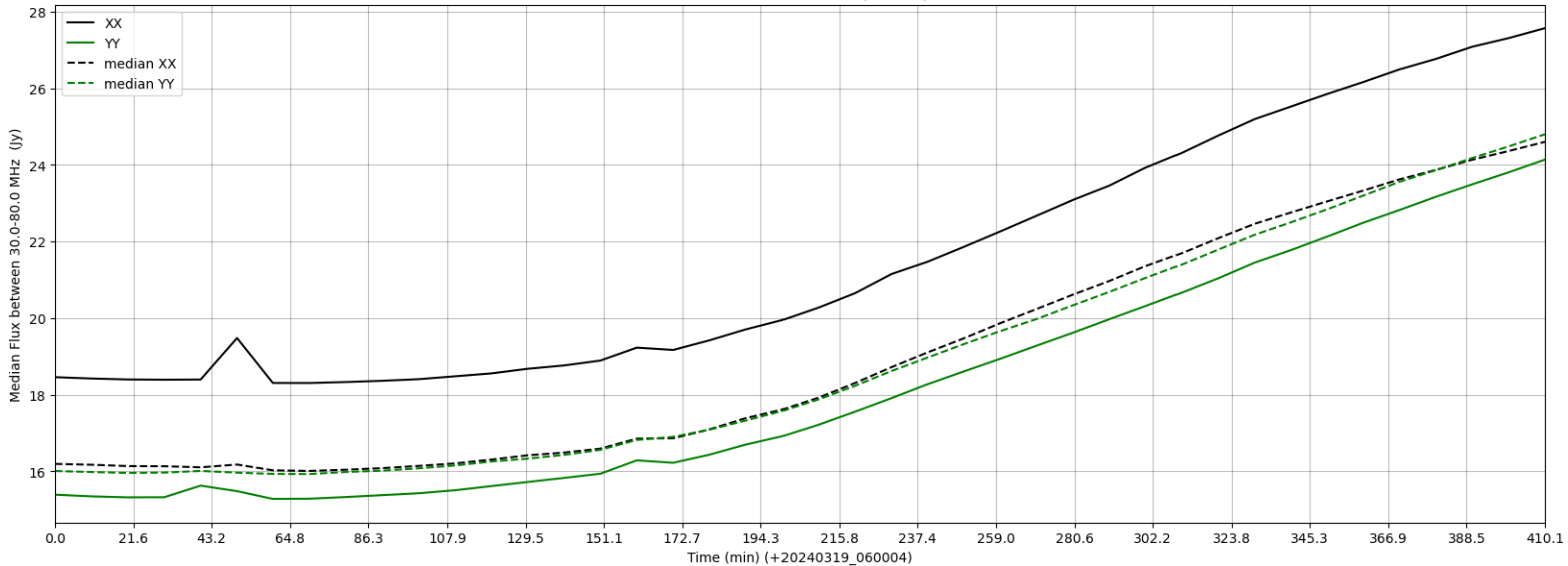
LWA025 - Correlator# 109 - XX FLAGS:BadSpecShape - YY FLAGS:Good
