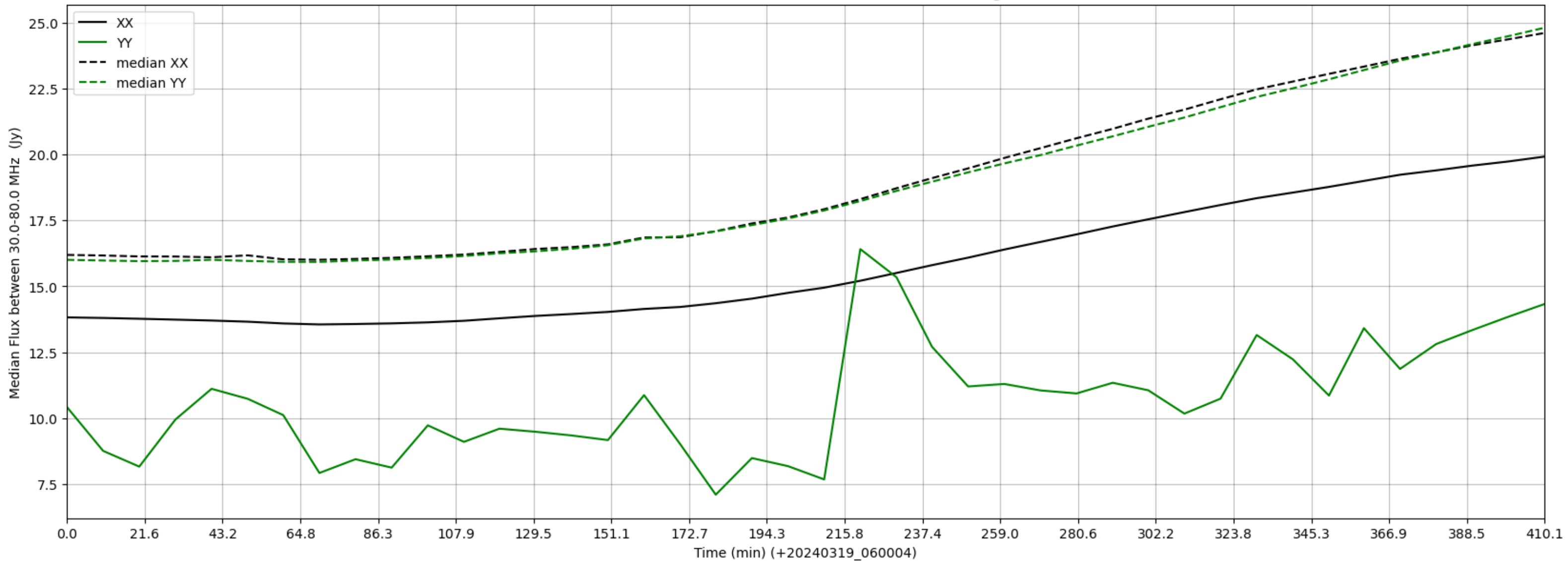
LWA314 - Correlator# 021 - XX FLAGS:Good - YY FLAGS:HighTimeVar
