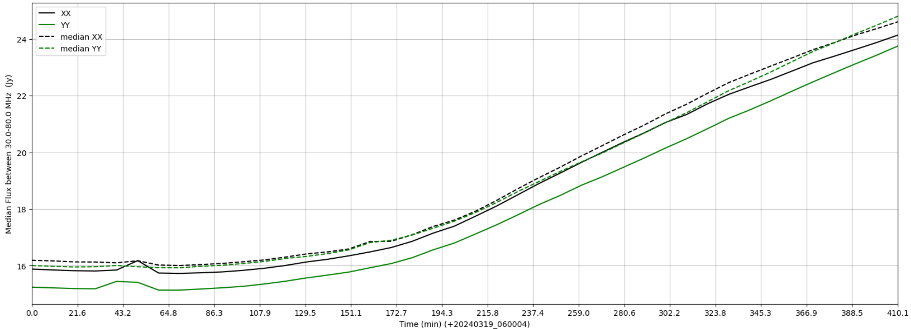
LWA082 - Correlator# 209 - XX FLAGS:BadSpecShape - YY FLAGS:Good
