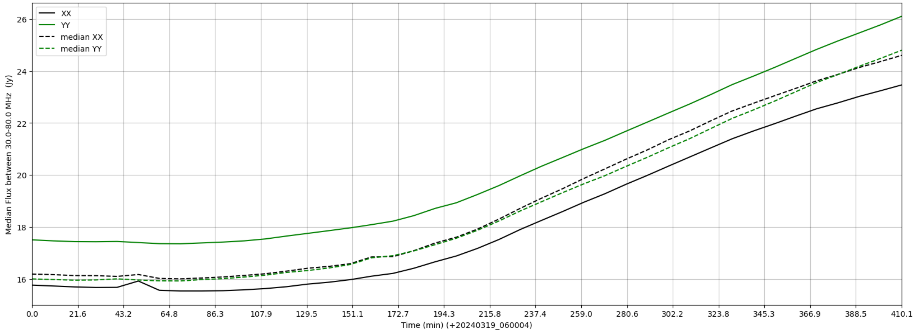
LWA110 - Correlator# 198 - XX FLAGS:BadSpecShape - YY FLAGS:Good
