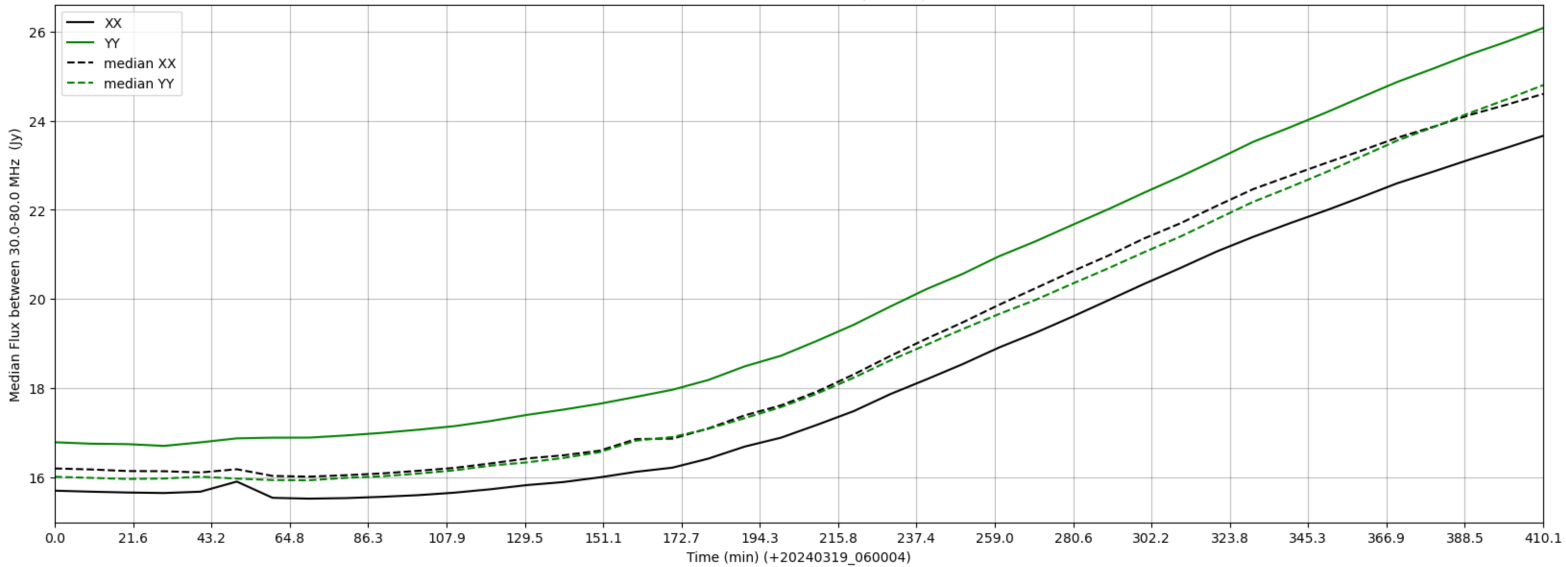
LWA113 - Correlator# 203 - XX FLAGS:BadSpecShape - YY FLAGS:Good
