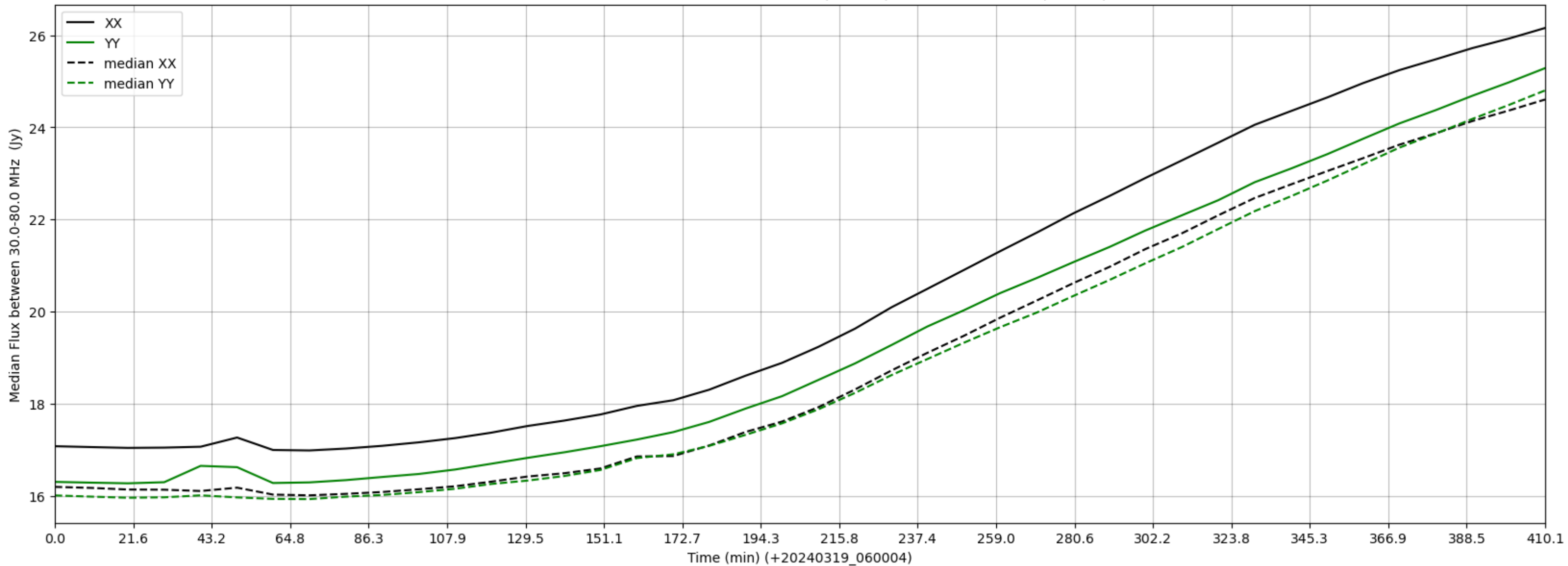
LWA080 - Correlator# 119 - XX FLAGS:BadSpecShape - YY FLAGS:BadSpecShape
