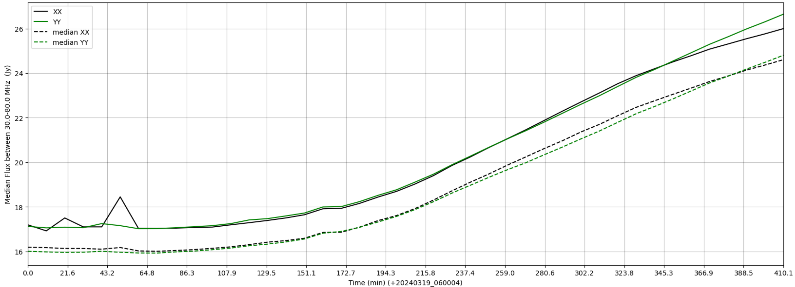
LWA012 - Correlator# 074 - XX FLAGS:BadSpecShape - YY FLAGS:Good
