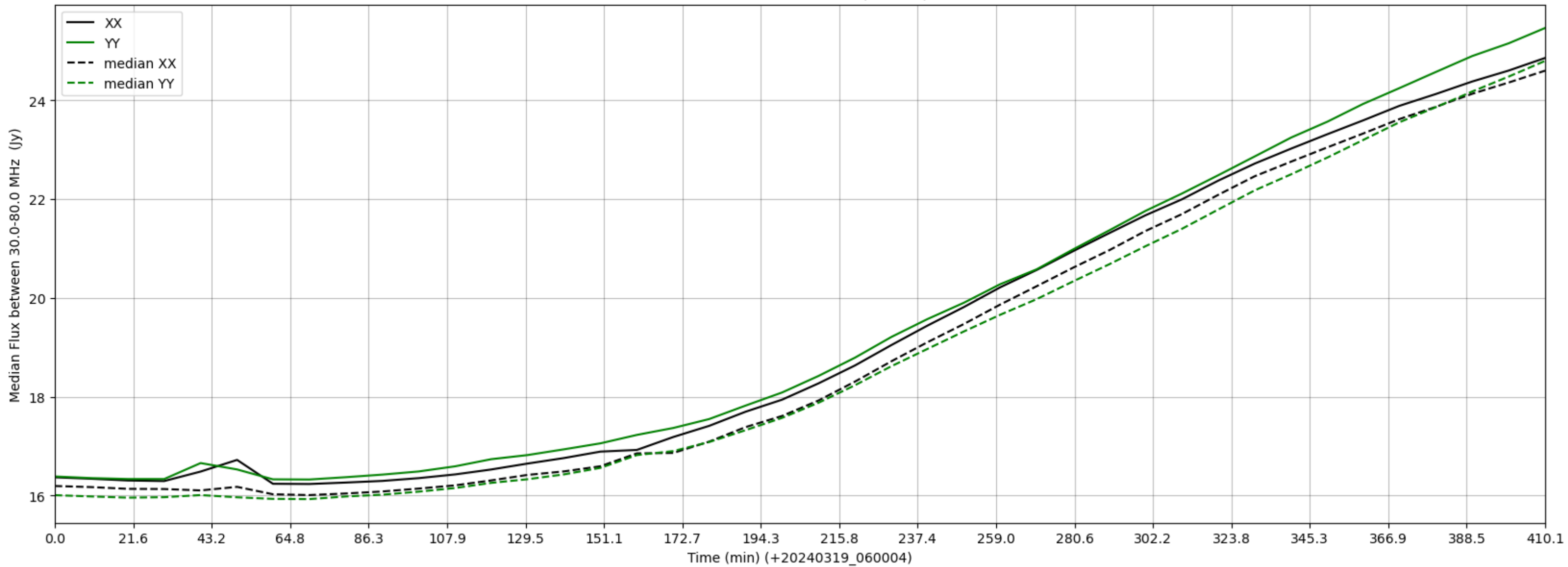
LWA079 - Correlator# 195 - XX FLAGS:BadSpecShape - YY FLAGS:Good
