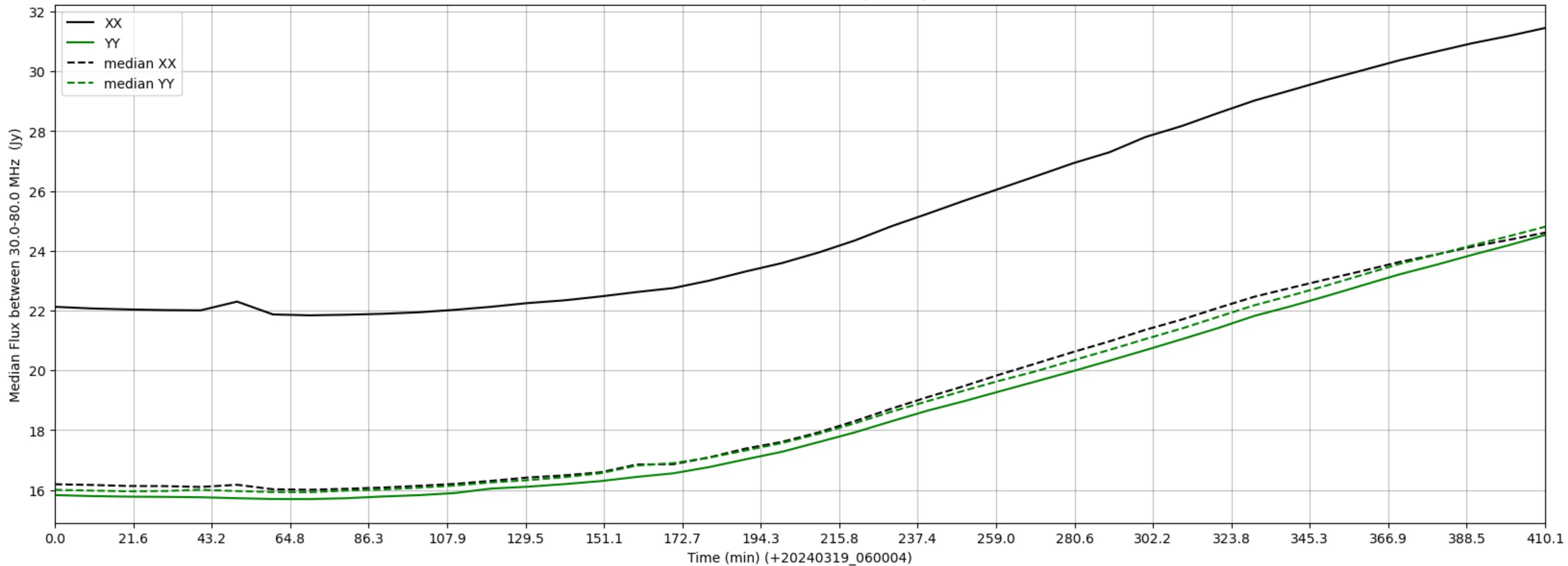
LWA075 - Correlator# 089 - XX FLAGS:BadSpecShape - YY FLAGS:Good
