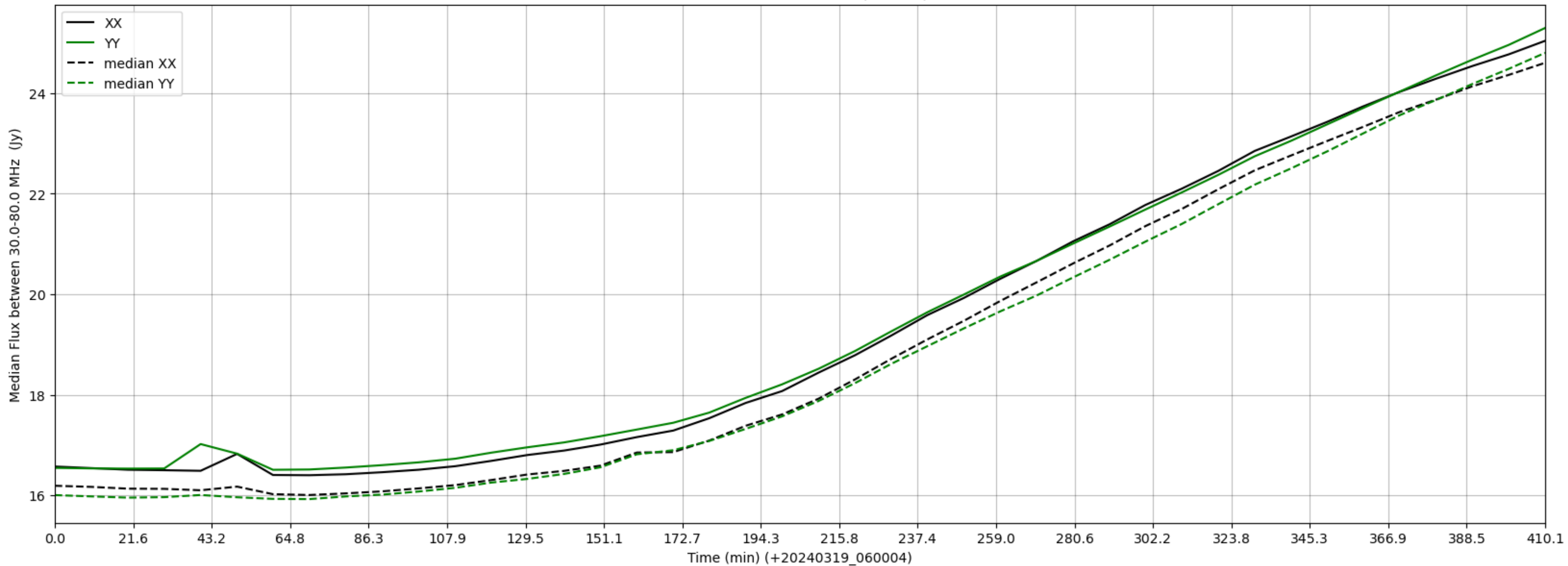
LWA084 - Correlator# 120 - XX FLAGS:BadSpecShape - YY FLAGS:Good
