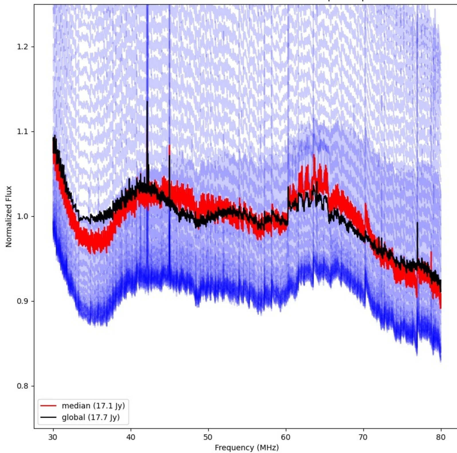
LWA110 - Correlator# 198 - XX - FLAGS:BadSpecShape
