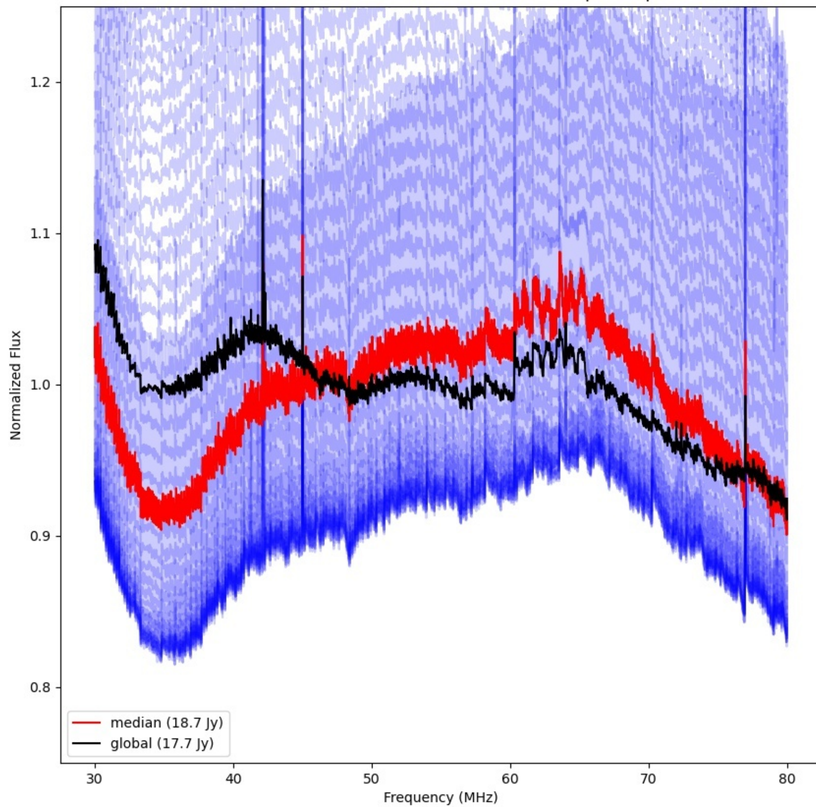
LWA114 - Correlator# 202 - XX - FLAGS:BadSpecShape
