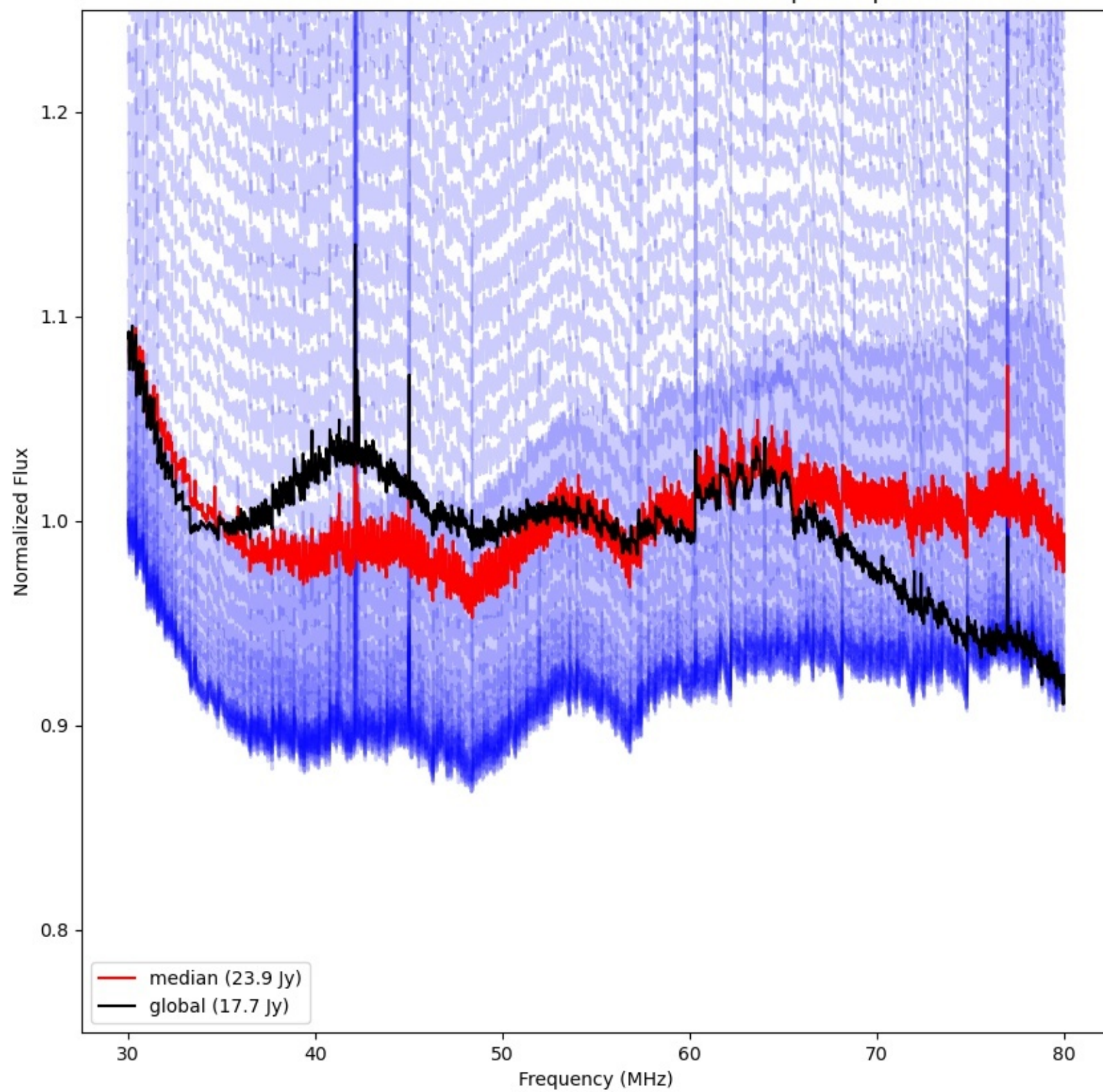
LWA075 - Correlator# 089 - XX - FLAGS:BadSpecShape
