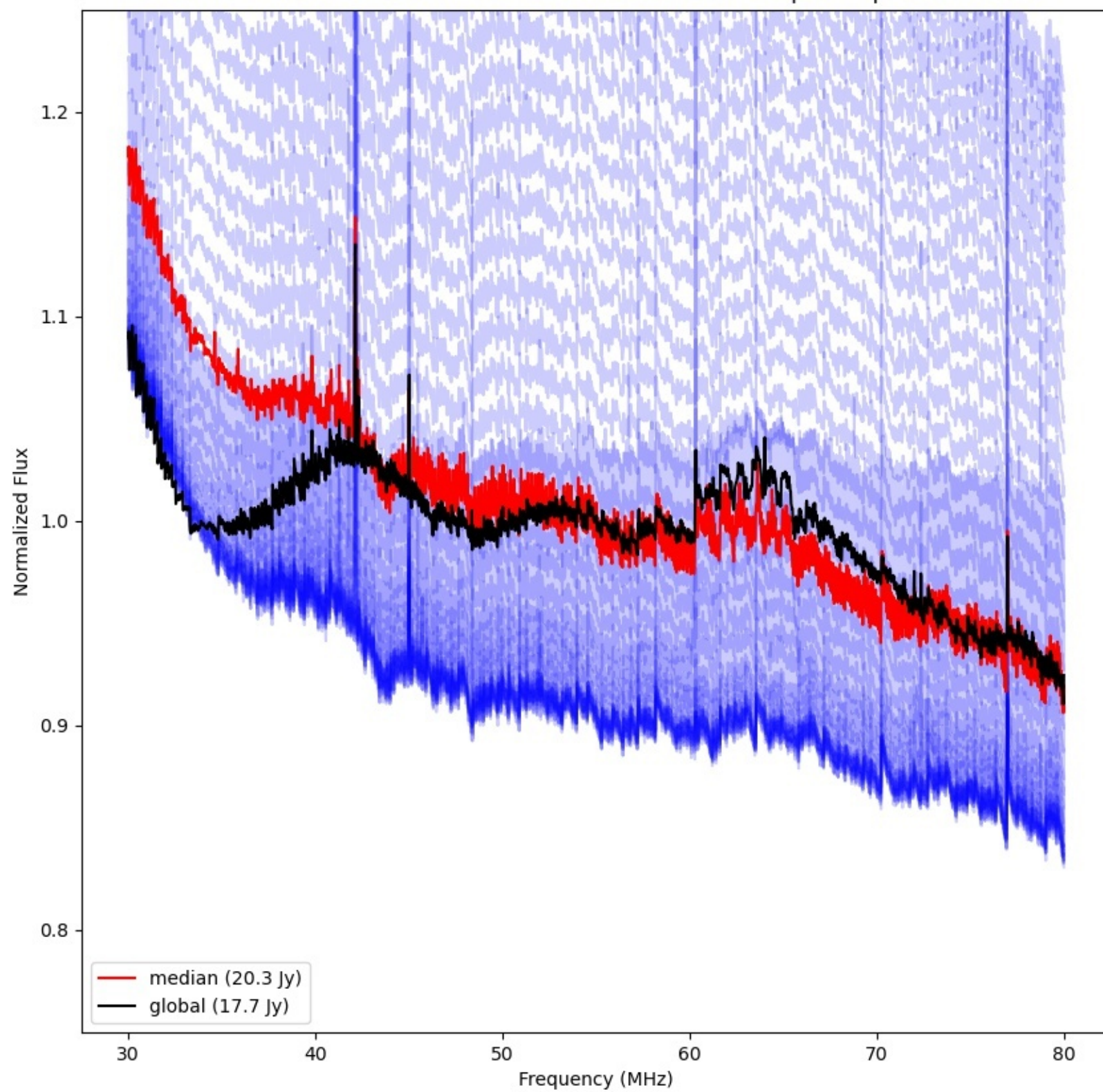
LWA025 - Correlator# 109 - XX - FLAGS:BadSpecShape
