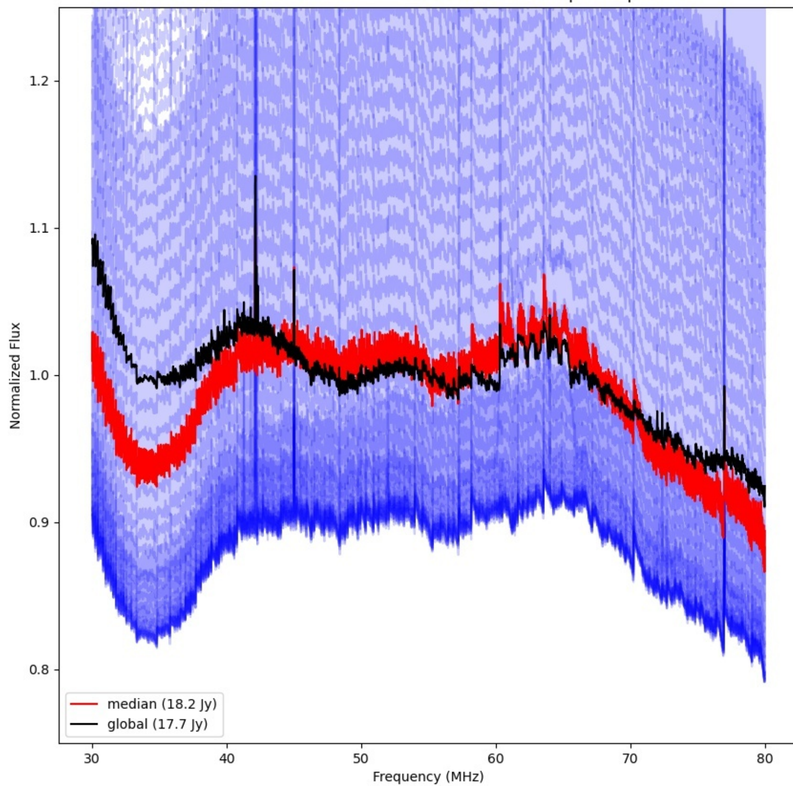
LWA079 - Correlator# 195 - XX - FLAGS:BadSpecShape
