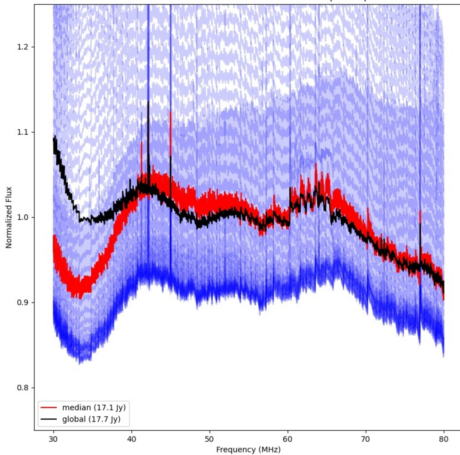
LWA113 - Correlator# 203 - XX - FLAGS:BadSpecShape
