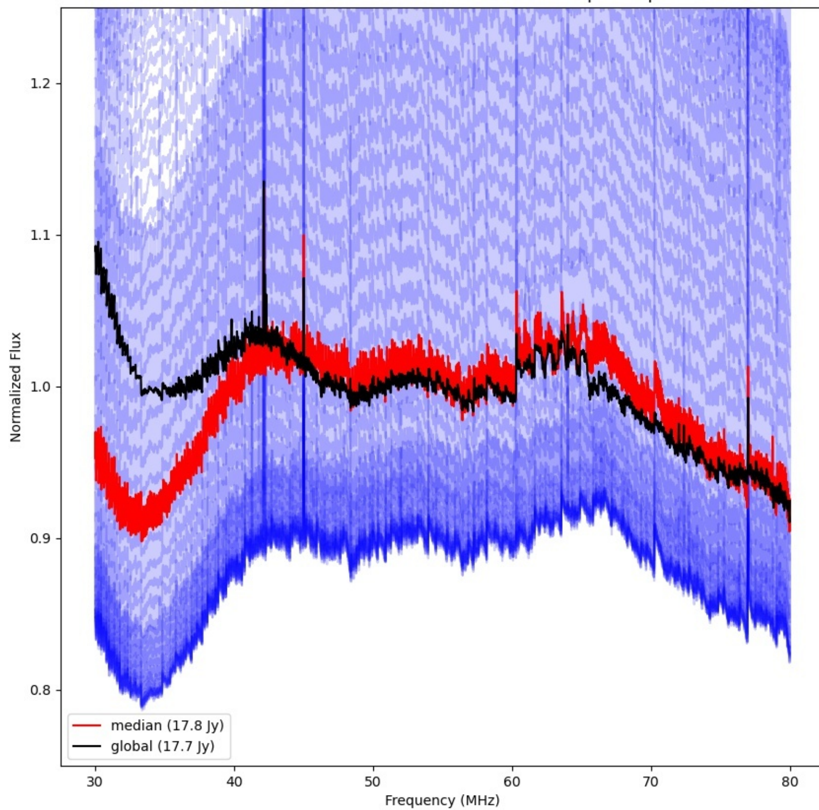
LWA081 - Correlator# 194 - XX - FLAGS:BadSpecShape
