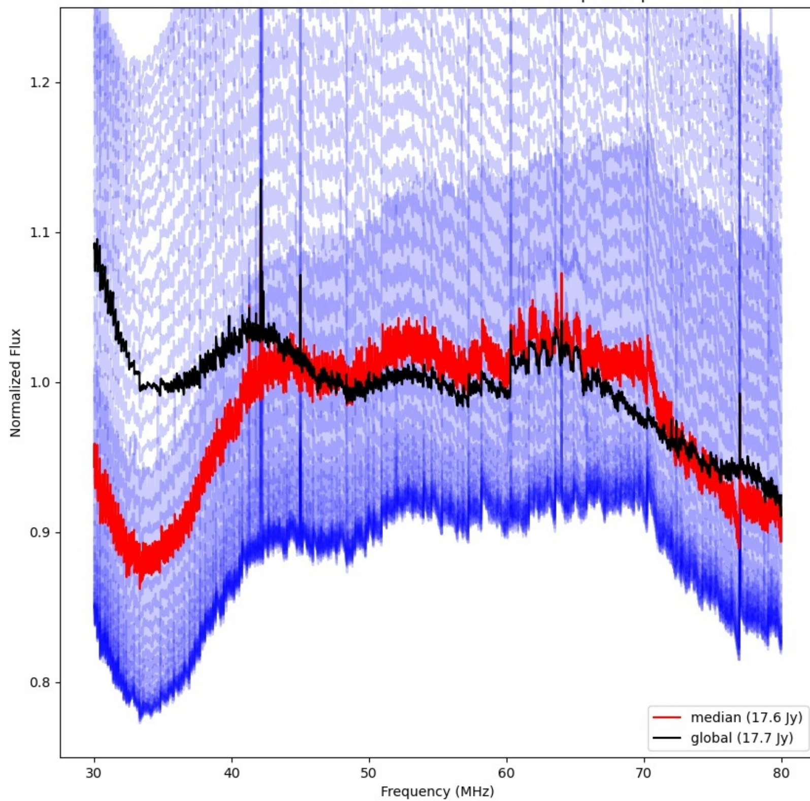
LWA082 - Correlator# 209 - XX - FLAGS:BadSpecShape
