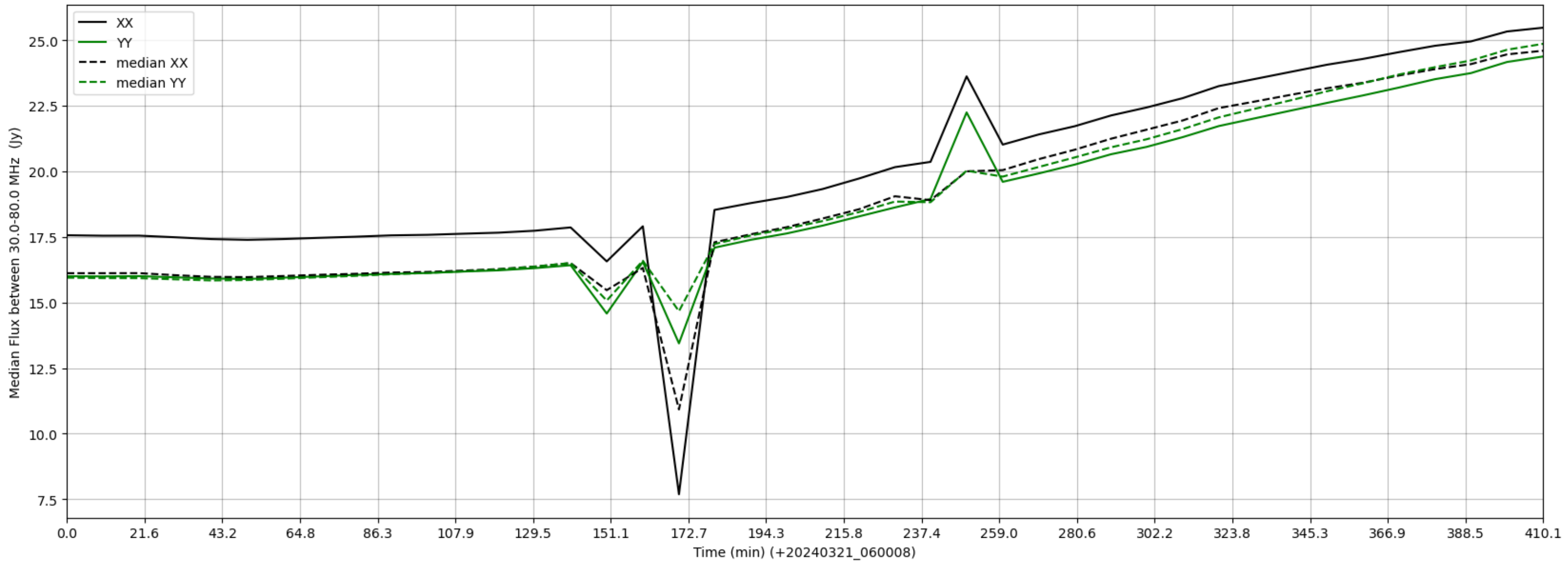
LWA066 - Correlator# 164 - XX FLAGS:Good - YY FLAGS:Good
