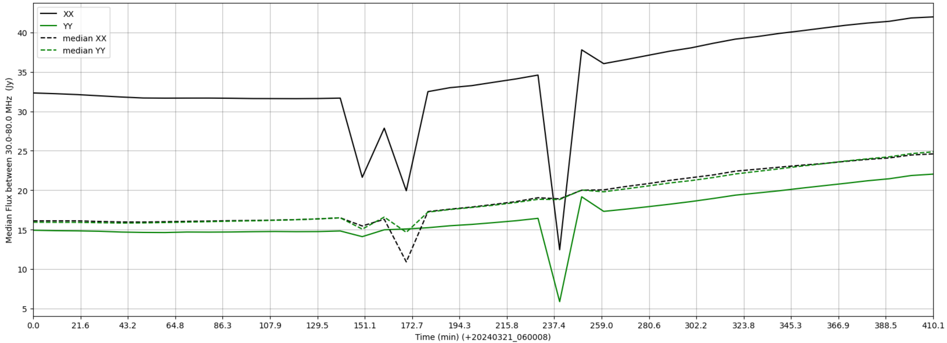
LWA362 - Correlator# 030 - XX FLAGS:Good - YY FLAGS:Good
