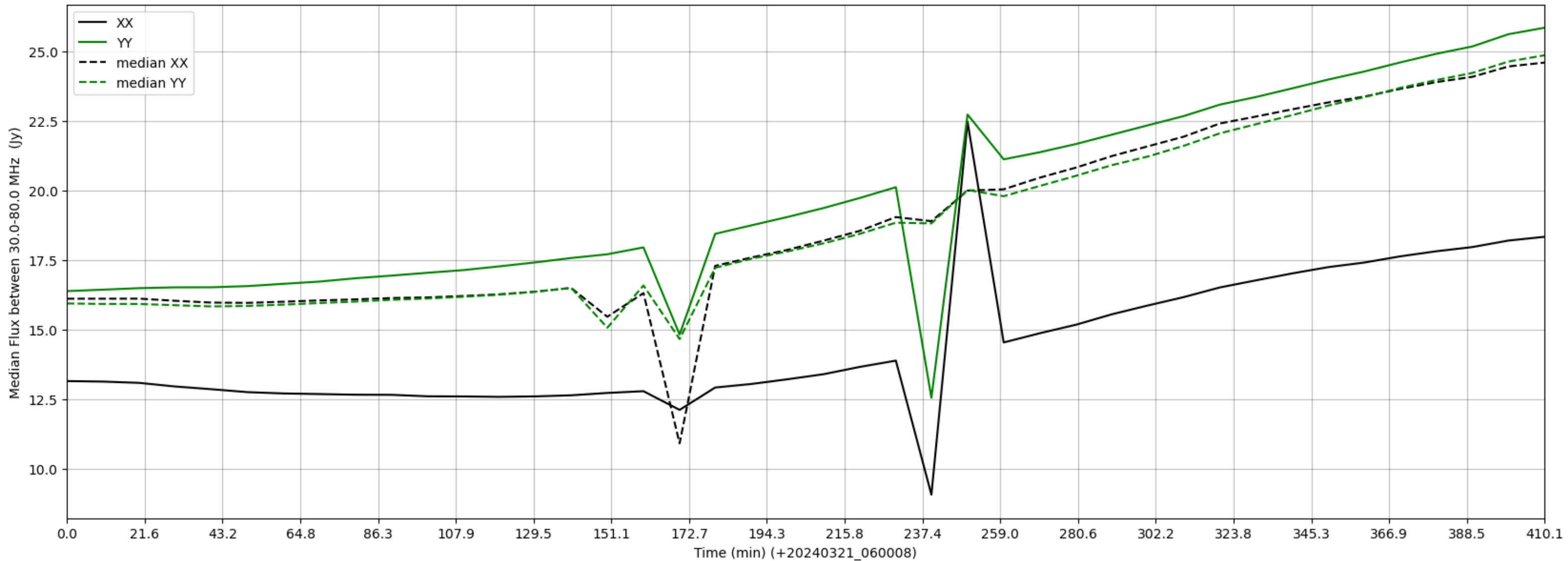
LWA317 - Correlator# 052 - XX FLAGS:Good - YY FLAGS:Good
