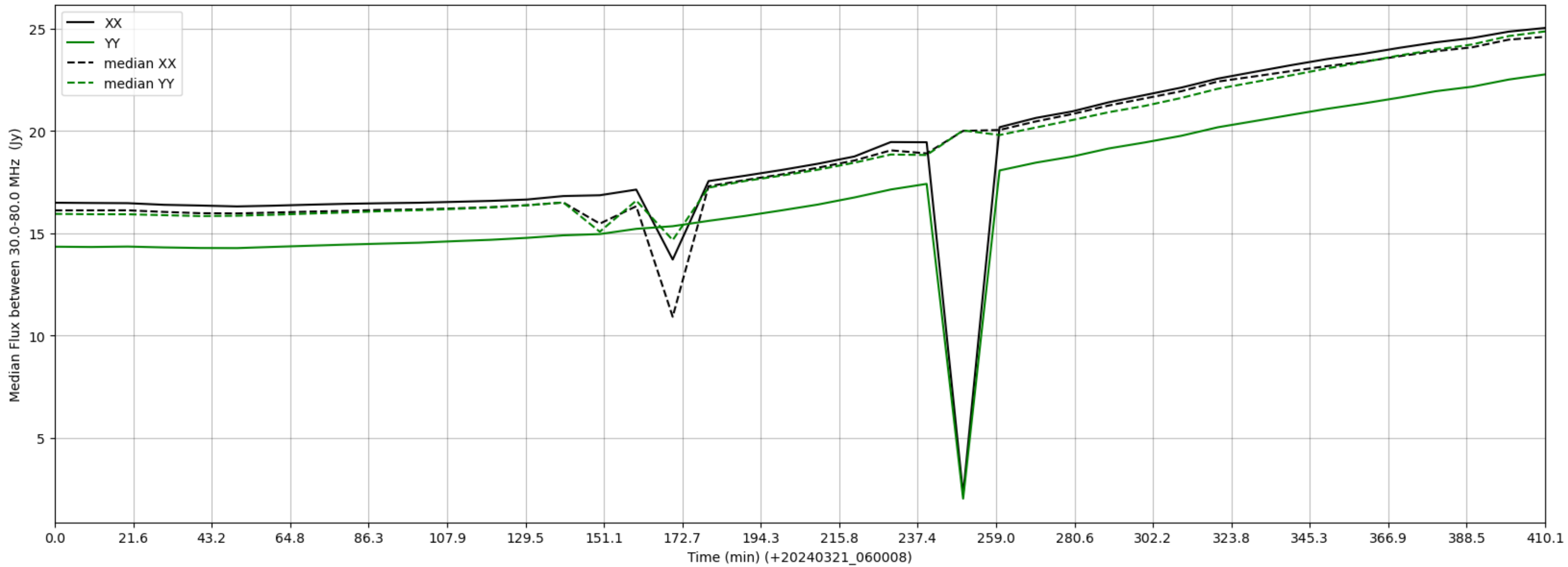
LWA158 - Correlator# 237 - XX FLAGS:Good - YY FLAGS:Good
