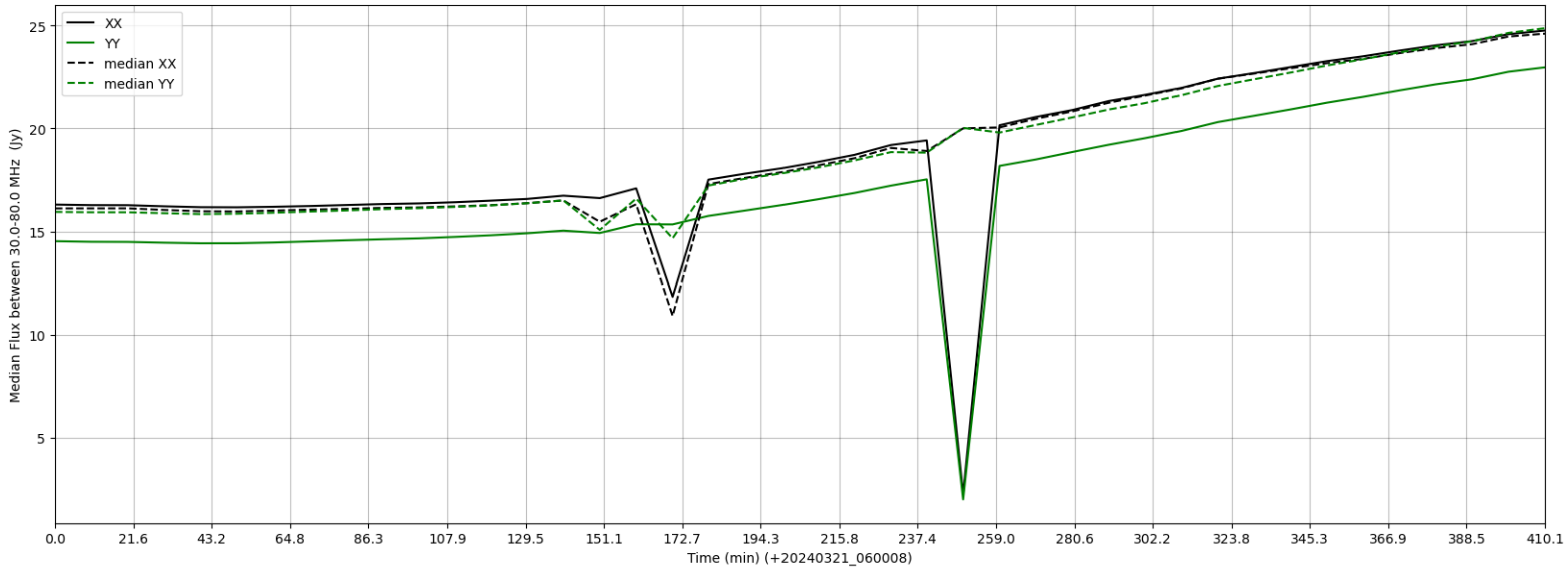
LWA160 - Correlator# 239 - XX FLAGS:Good - YY FLAGS:Good
