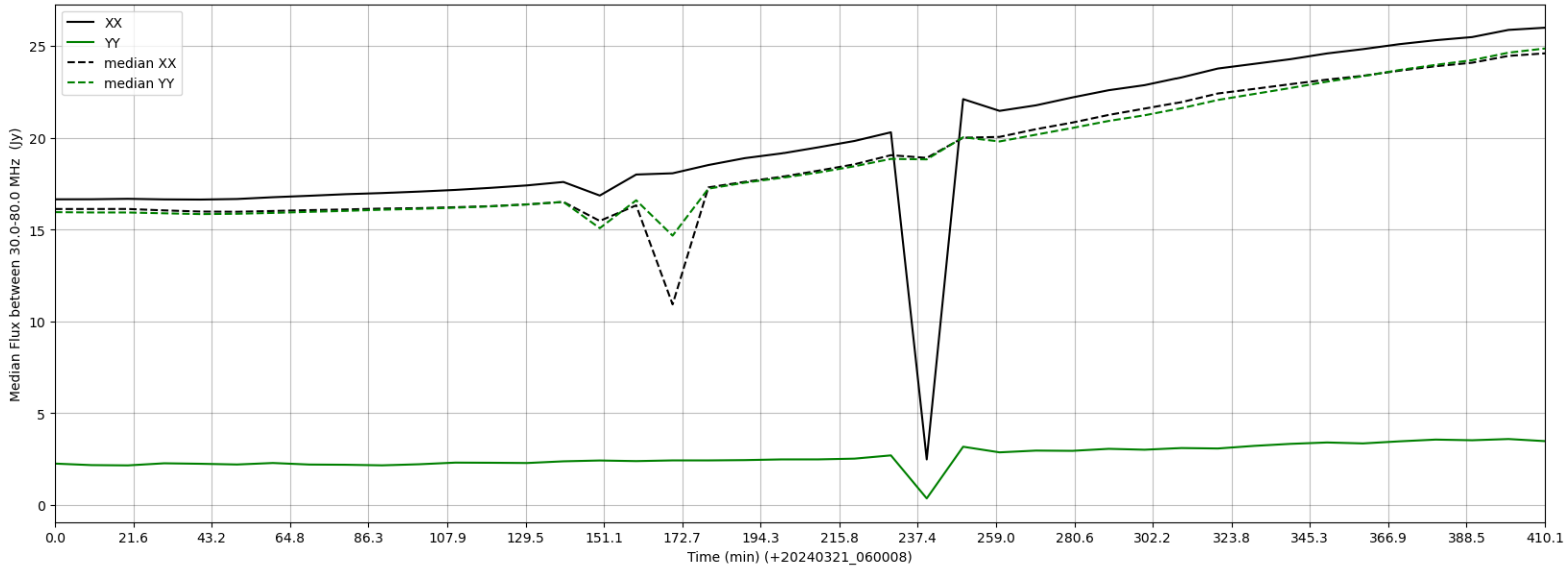
LWA307 - Correlator# 012 - XX FLAGS:Good - YY FLAGS:BadSpecShape
