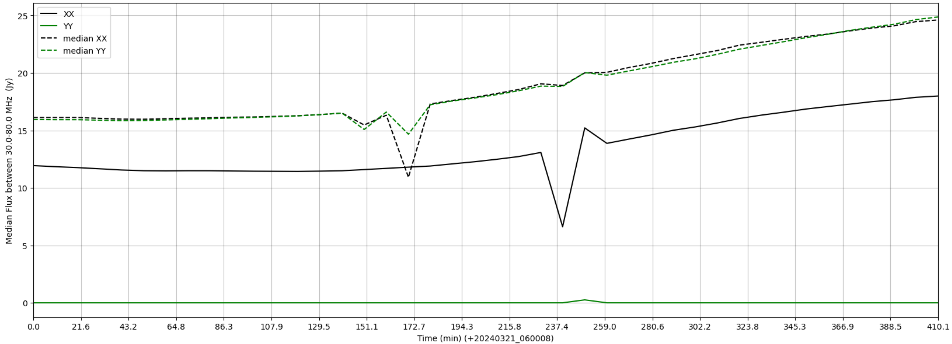
LWA292 - Correlator# 044 - XX FLAGS:Good - YY FLAGS:LowFlux
