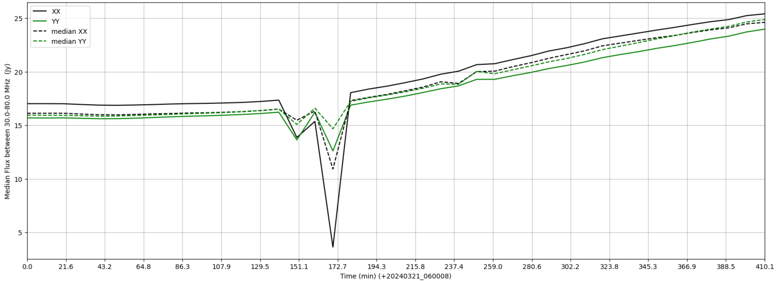
LWA109 - Correlator# 199 - XX FLAGS:Good - YY FLAGS:Good
