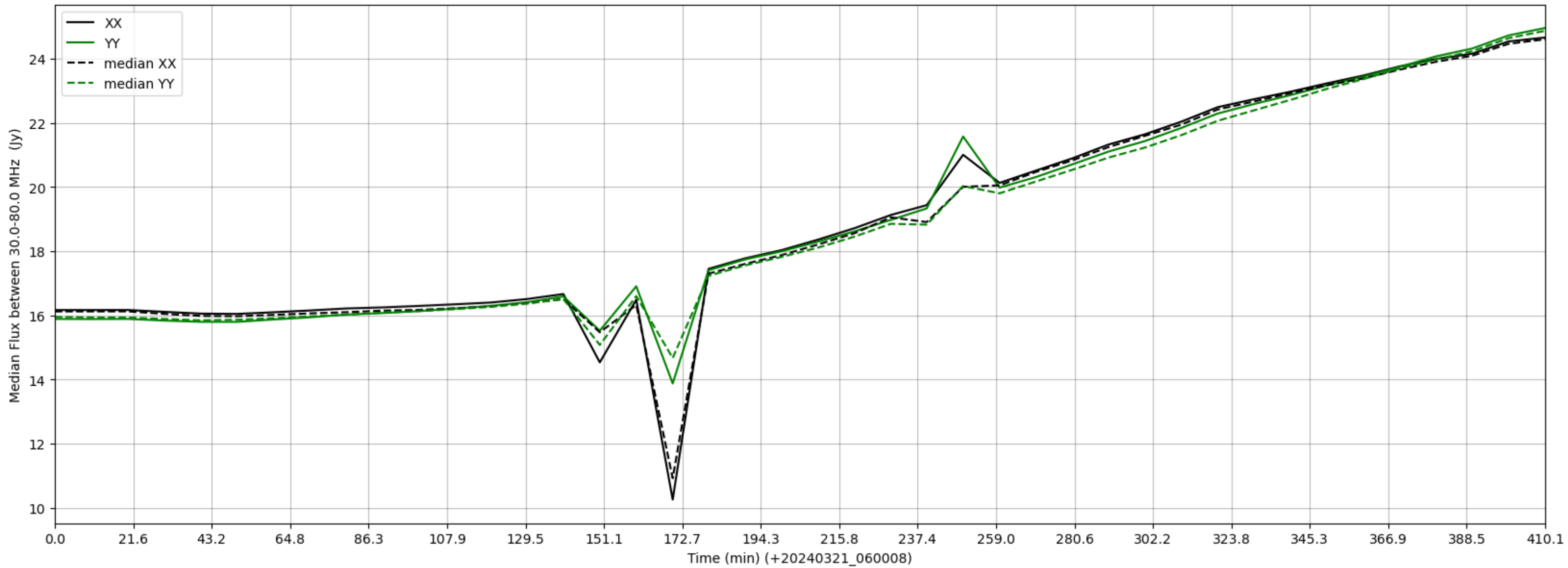
LWA228 - Correlator# 302 - XX FLAGS:Good - YY FLAGS:Good
