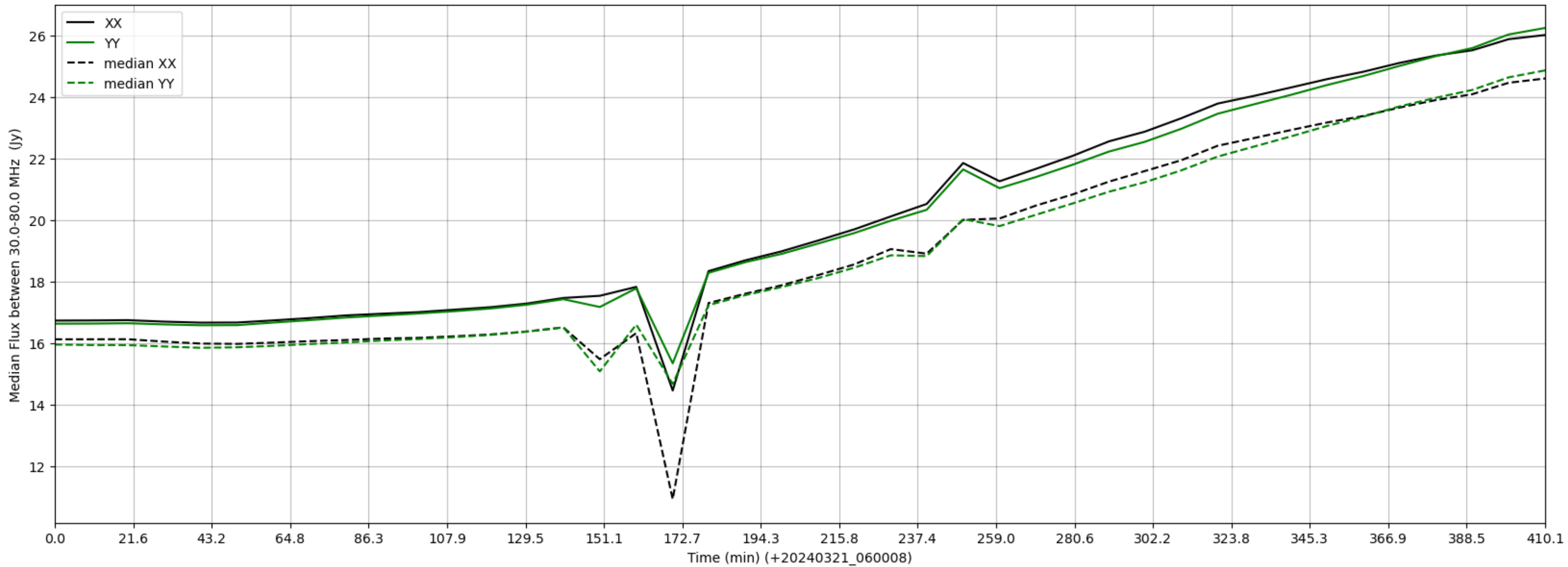
LWA236 - Correlator# 308 - XX FLAGS:Good - YY FLAGS:Good
