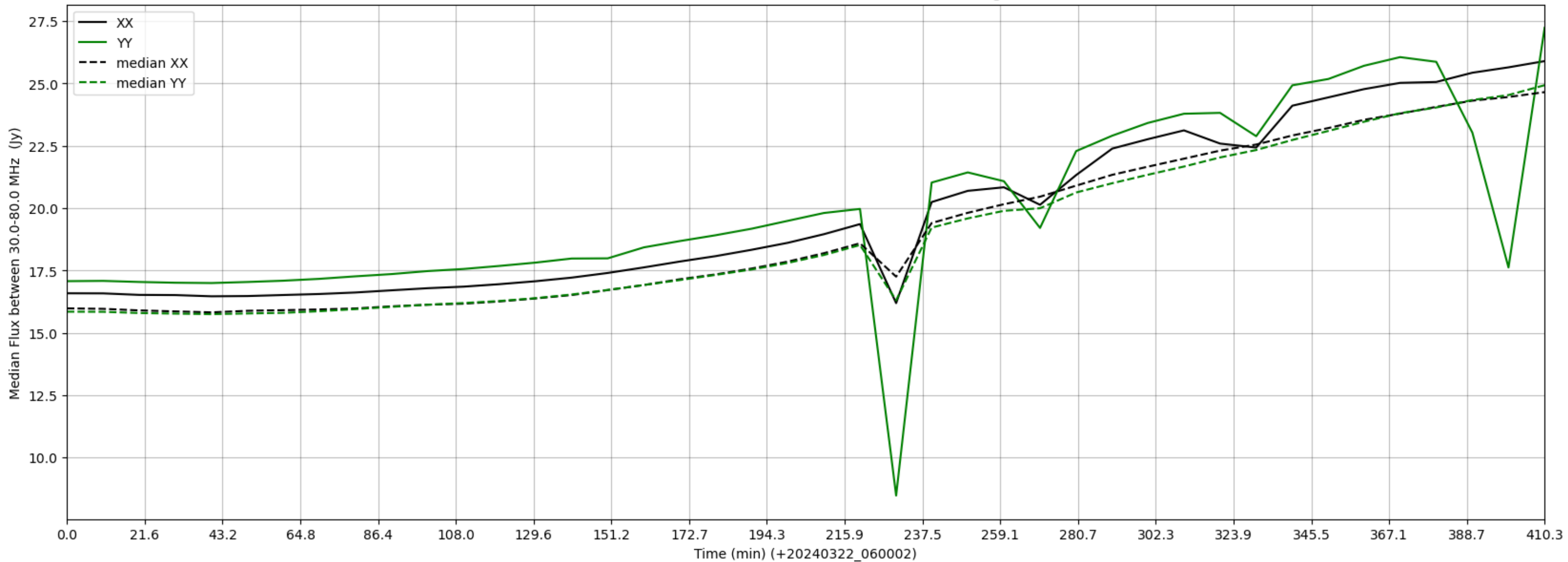
LWA006 - Correlator# 068 - XX FLAGS:Good - YY FLAGS:HighTimeVar
