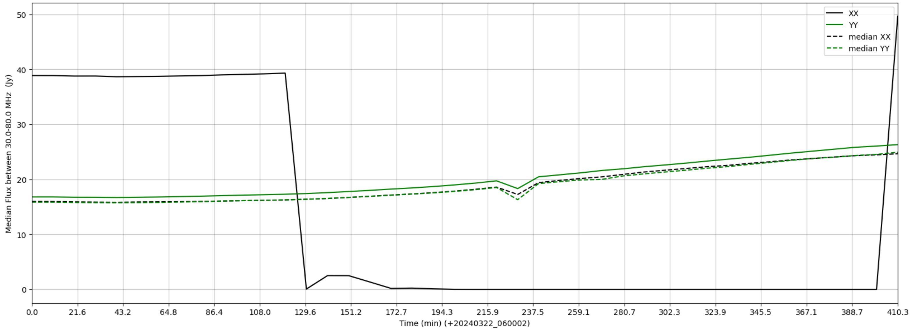
LWA221 - Correlator# 334 - XX FLAGS:LowFlux - YY FLAGS:Good
