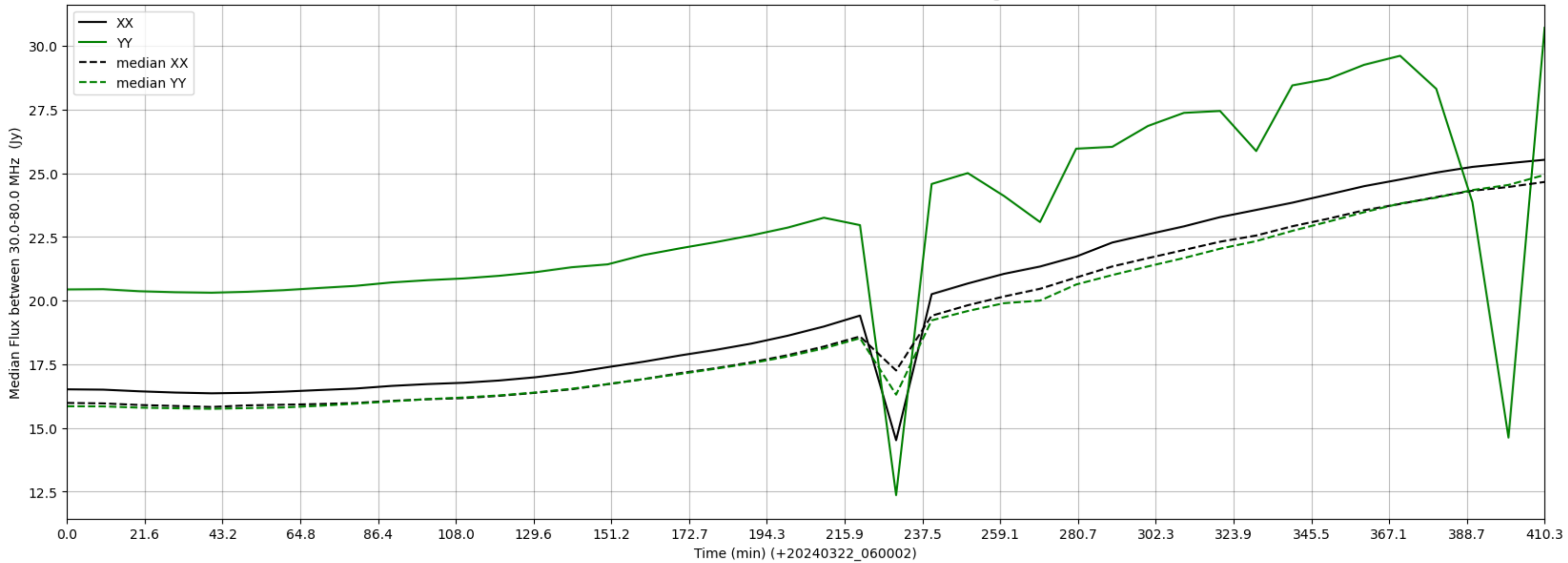
LWA197 - Correlator# 274 - XX FLAGS:Good - YY FLAGS:HighTimeVar
