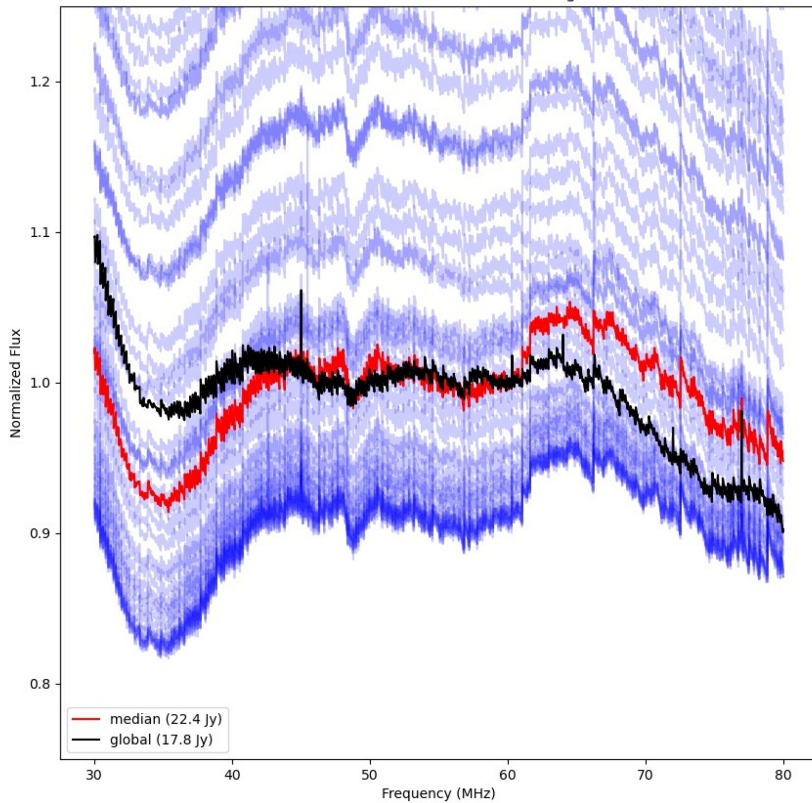
LWA197 - Correlator# 274 - YY - FLAGS:HighTimeVar
