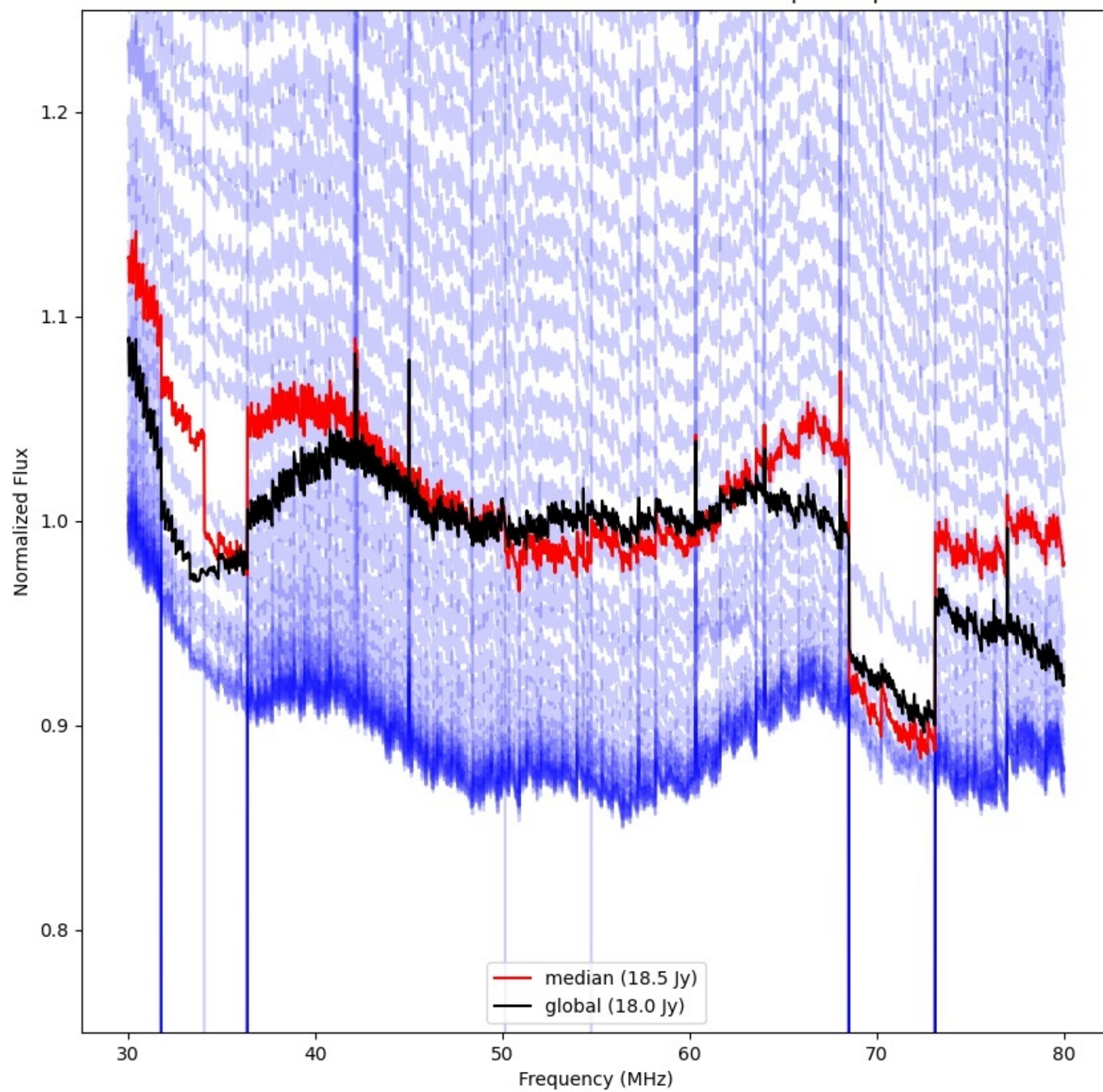
LWA217 - Correlator# 333 - XX - FLAGS:BadSpecShape
