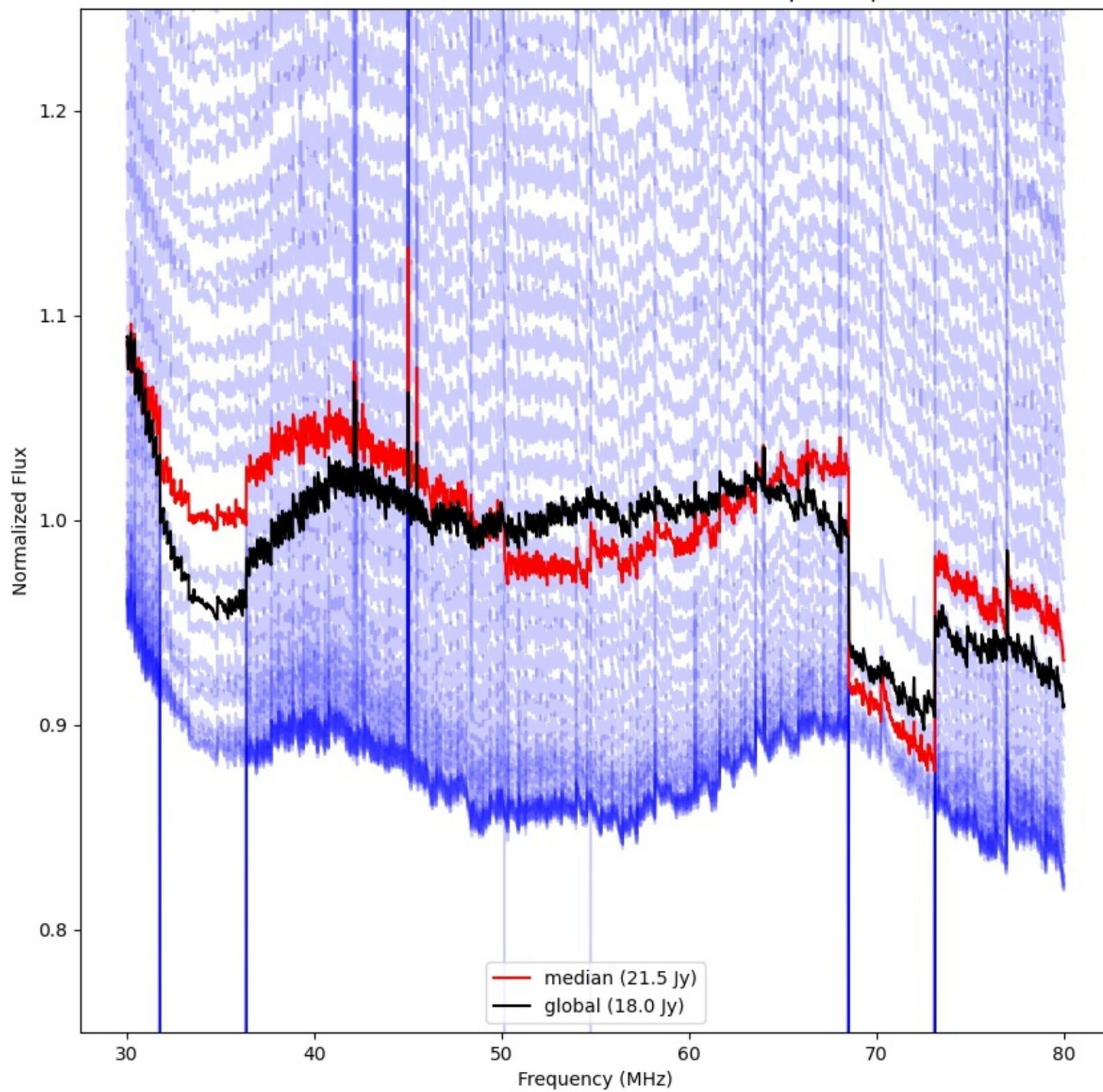
LWA218 - Correlator# 332 - YY - FLAGS:BadSpecShape
