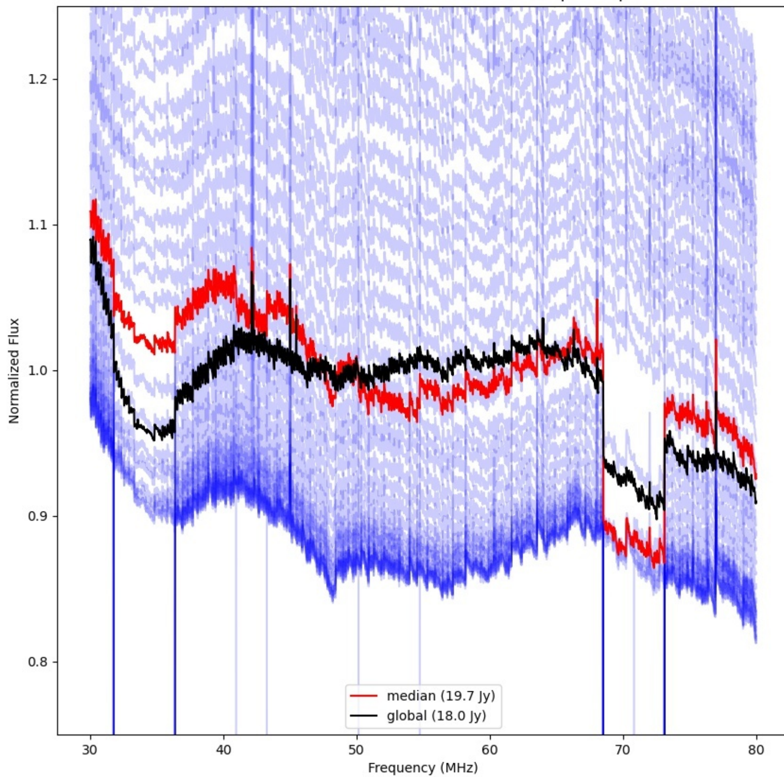
LWA247 - Correlator# 321 - YY - FLAGS:BadSpecShape
