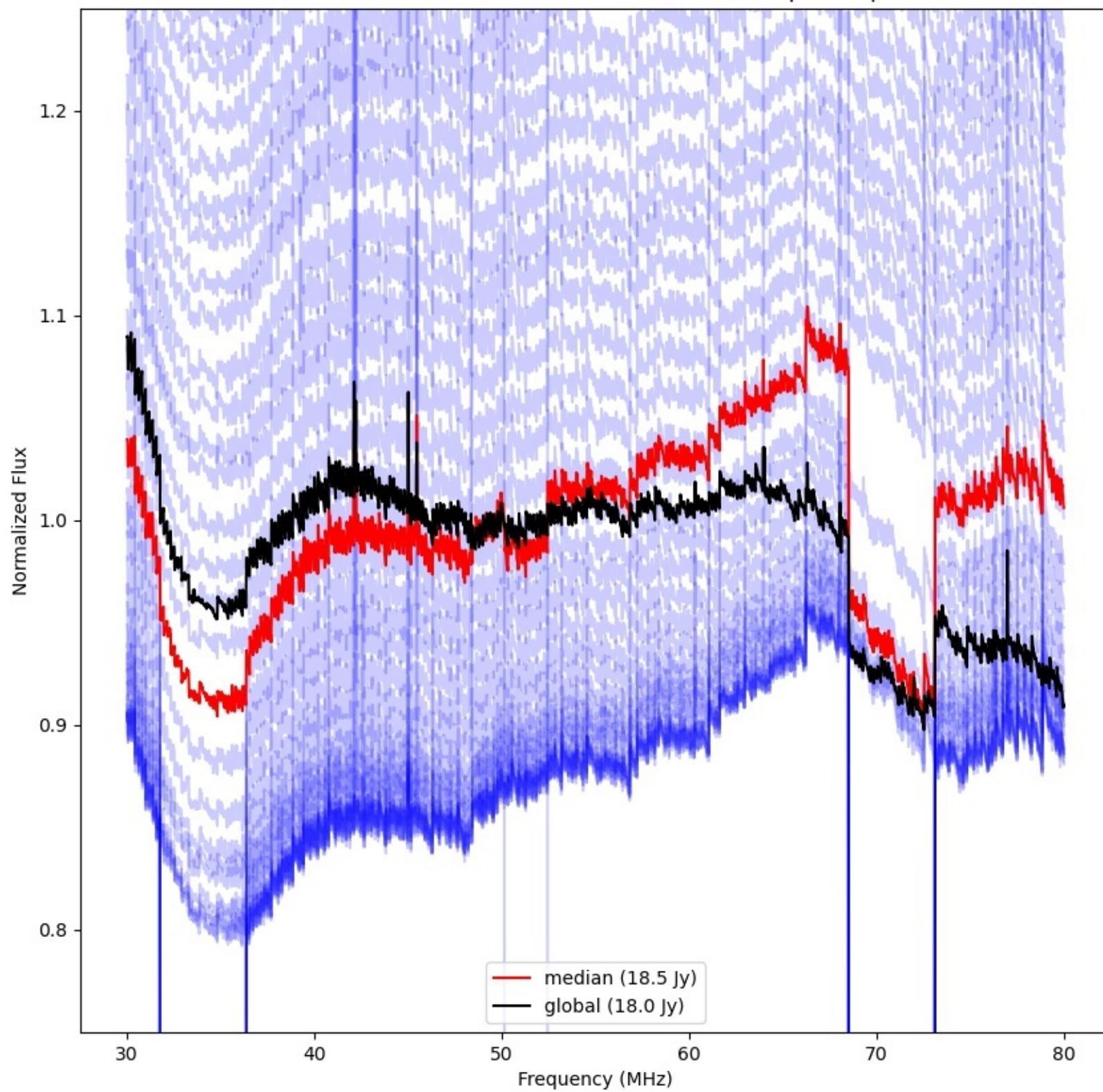
LWA164 - Correlator# 267 - YY - FLAGS:BadSpecShape
