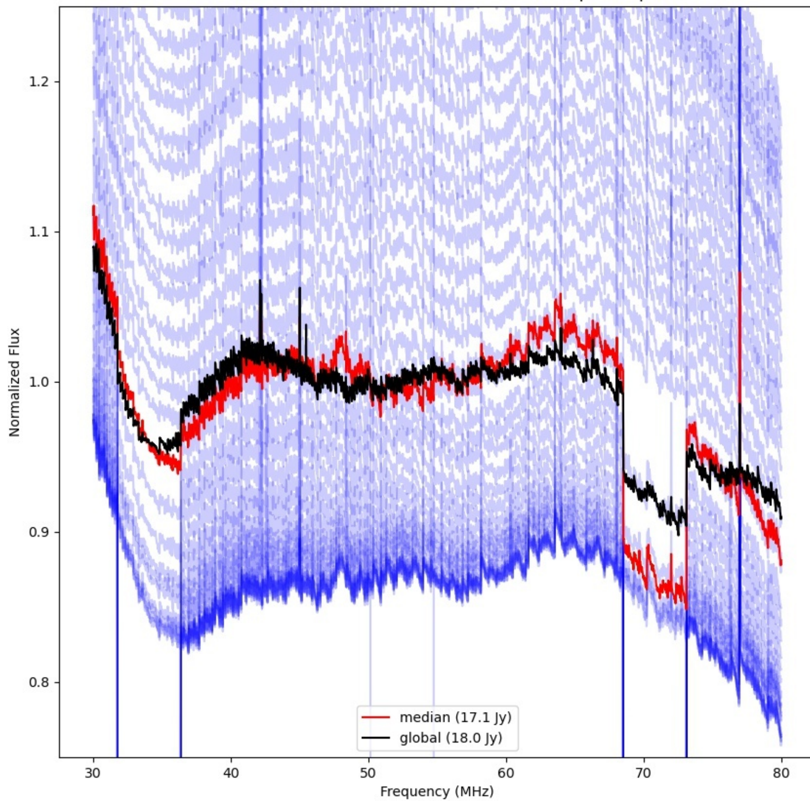
LWA249 - Correlator# 342 - YY - FLAGS:BadSpecShape
