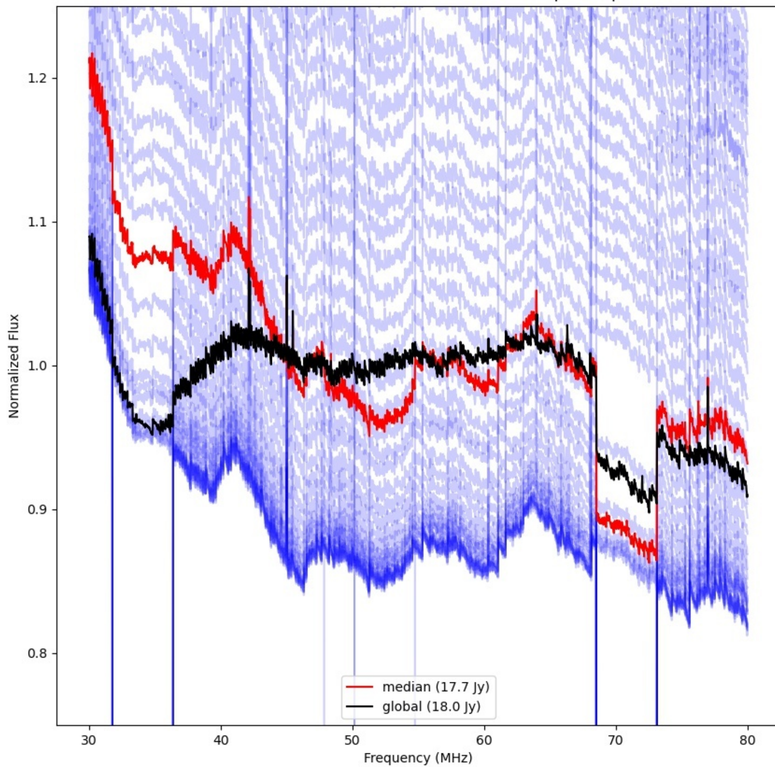
LWA357 - Correlator# 286 - YY - FLAGS:BadSpecShape
