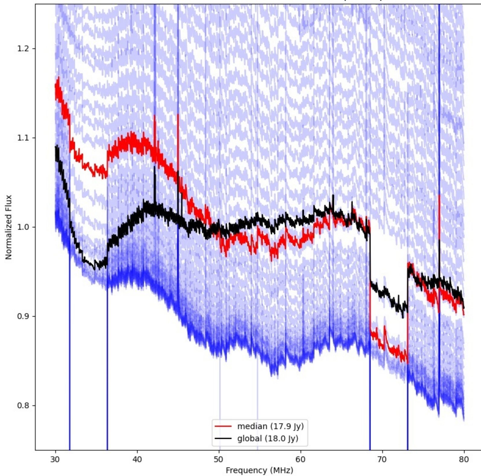
LWA215 - Correlator# 331 - YY - FLAGS:BadSpecShape
