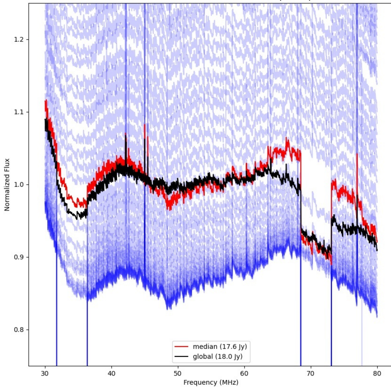
LWA181 - Correlator# 231 - YY - FLAGS:BadSpecShape
