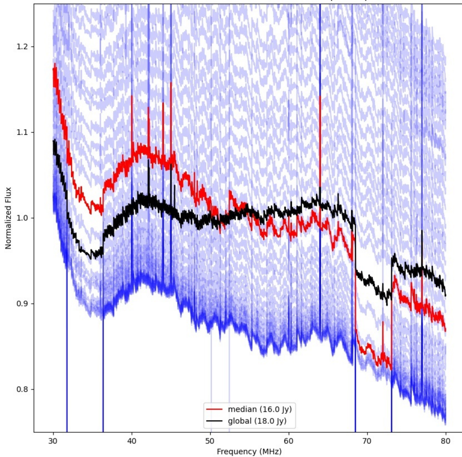
LWA190 - Correlator# 244 - YY - FLAGS:BadSpecShape
