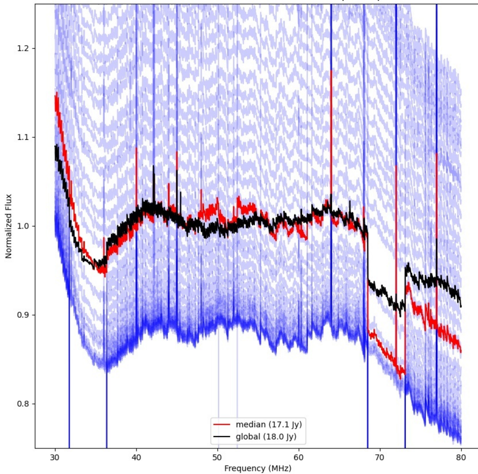
LWA191 - Correlator# 246 - YY - FLAGS:BadSpecShape
