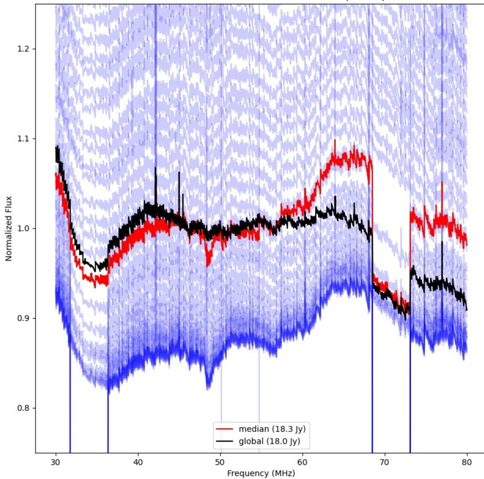
LWA245 - Correlator# 341 - YY - FLAGS:BadSpecShape
