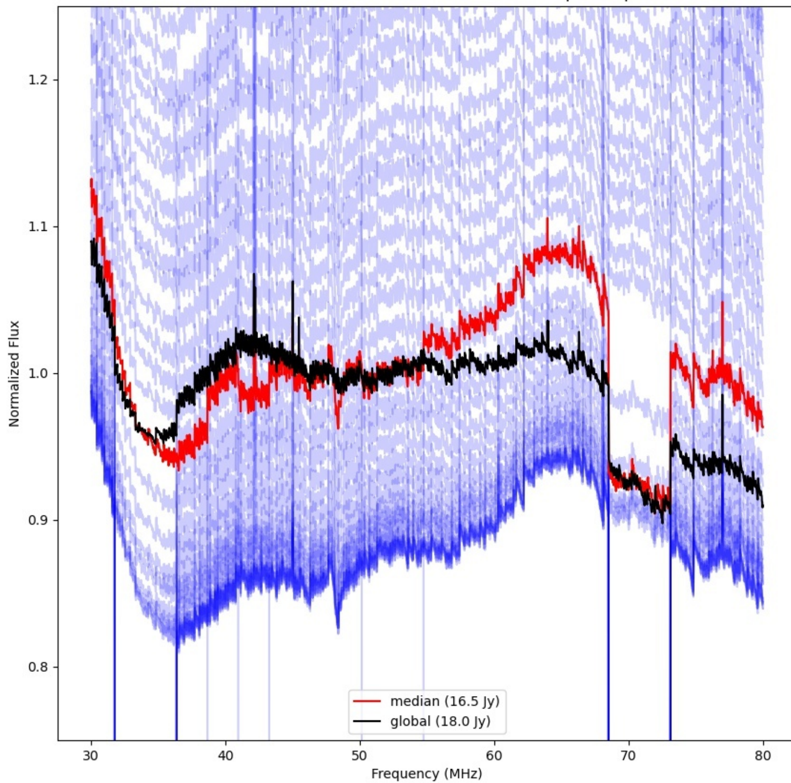
LWA207 - Correlator# 299 - YY - FLAGS:BadSpecShape
