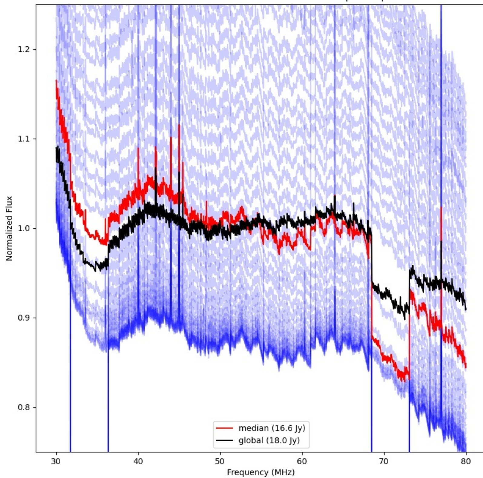
LWA125 - Correlator# 227 - YY - FLAGS:BadSpecShape
