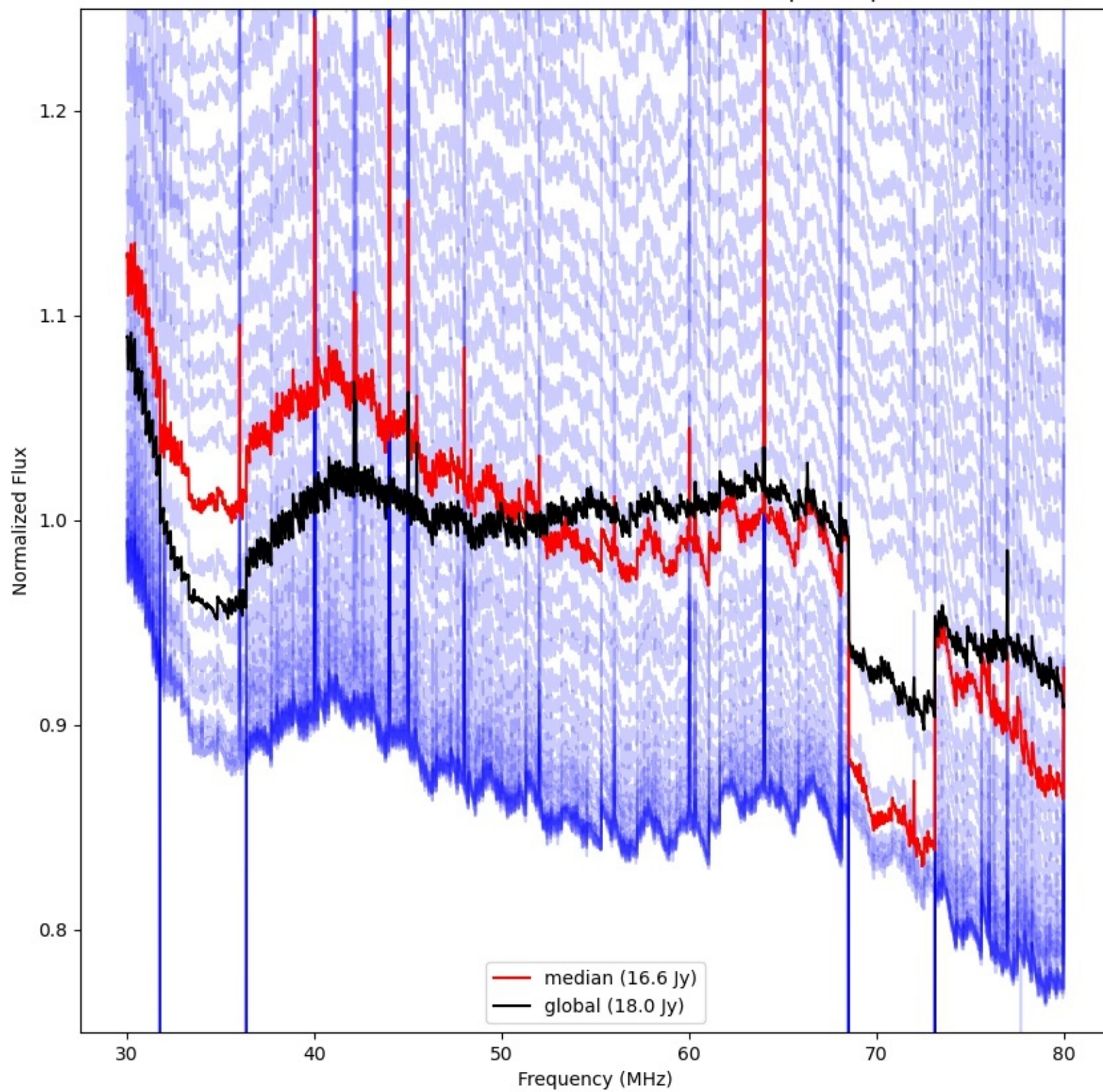
LWA159 - Correlator# 236 - YY - FLAGS:BadSpecShape
