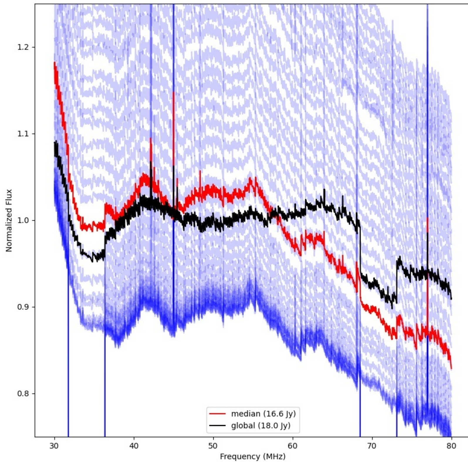
LWA307 - Correlator# 012 - YY - FLAGS:Good
