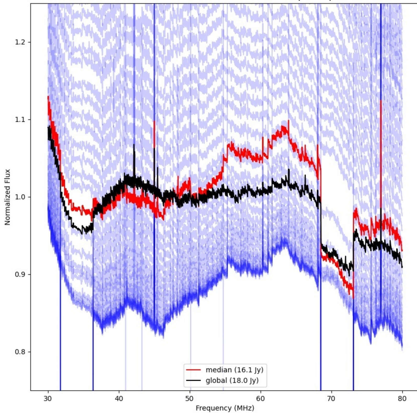
LWA350 - Correlator# 319 - YY - FLAGS:BadSpecShape
