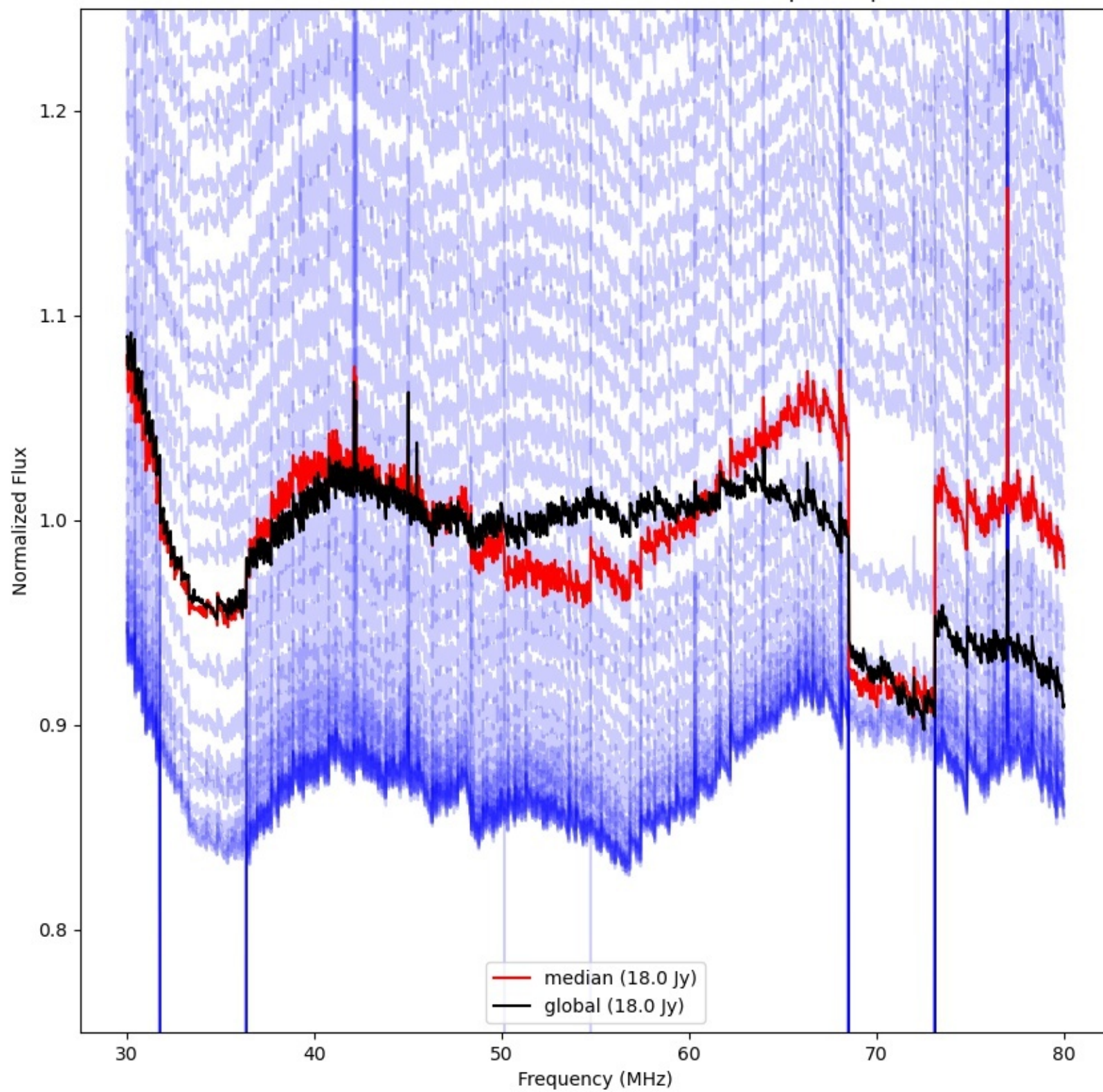
LWA243 - Correlator# 330 - YY - FLAGS:BadSpecShape
