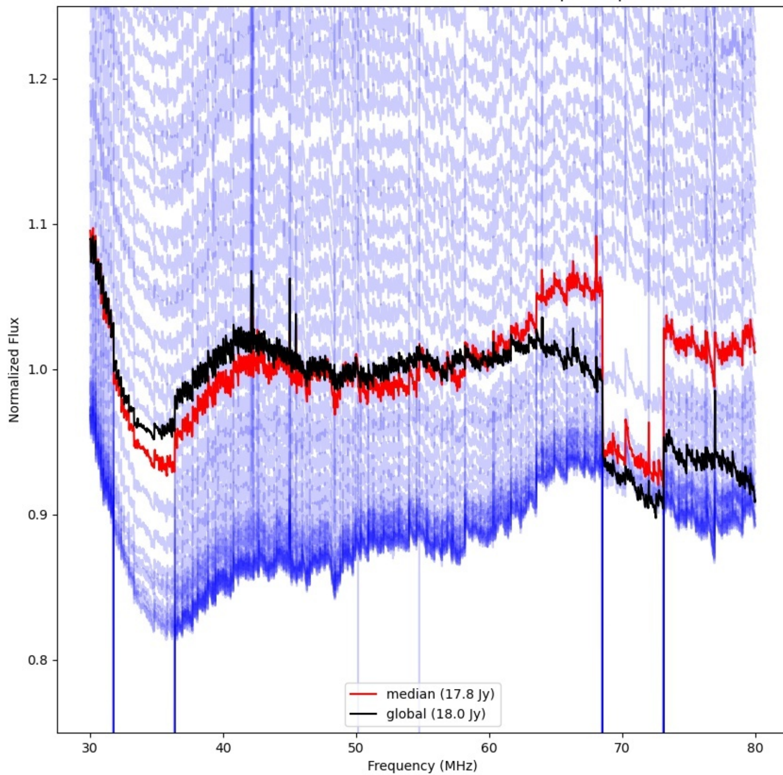
LWA250 - Correlator# 345 - YY - FLAGS:BadSpecShape
