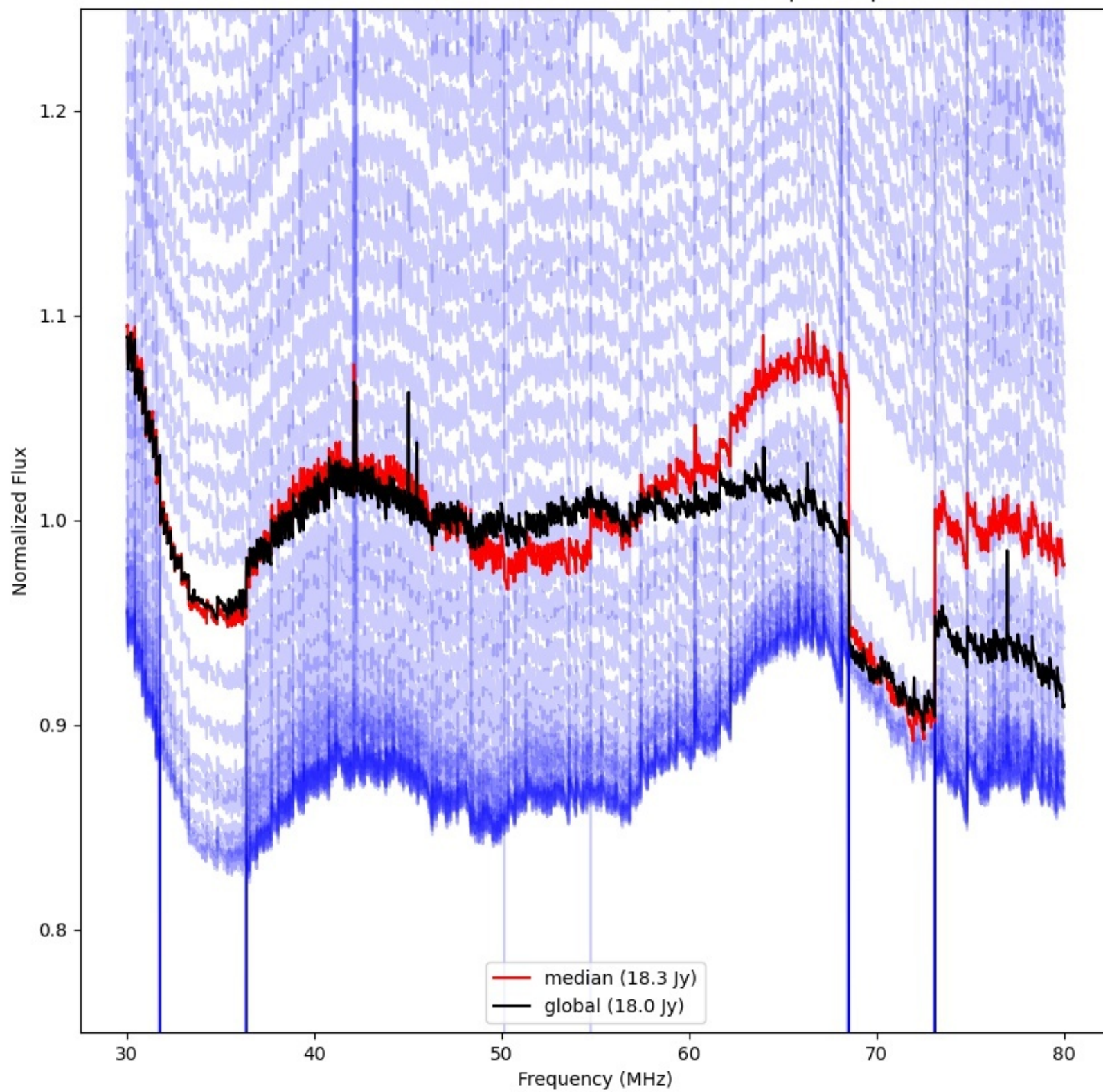
LWA242 - Correlator# 339 - YY - FLAGS:BadSpecShape
