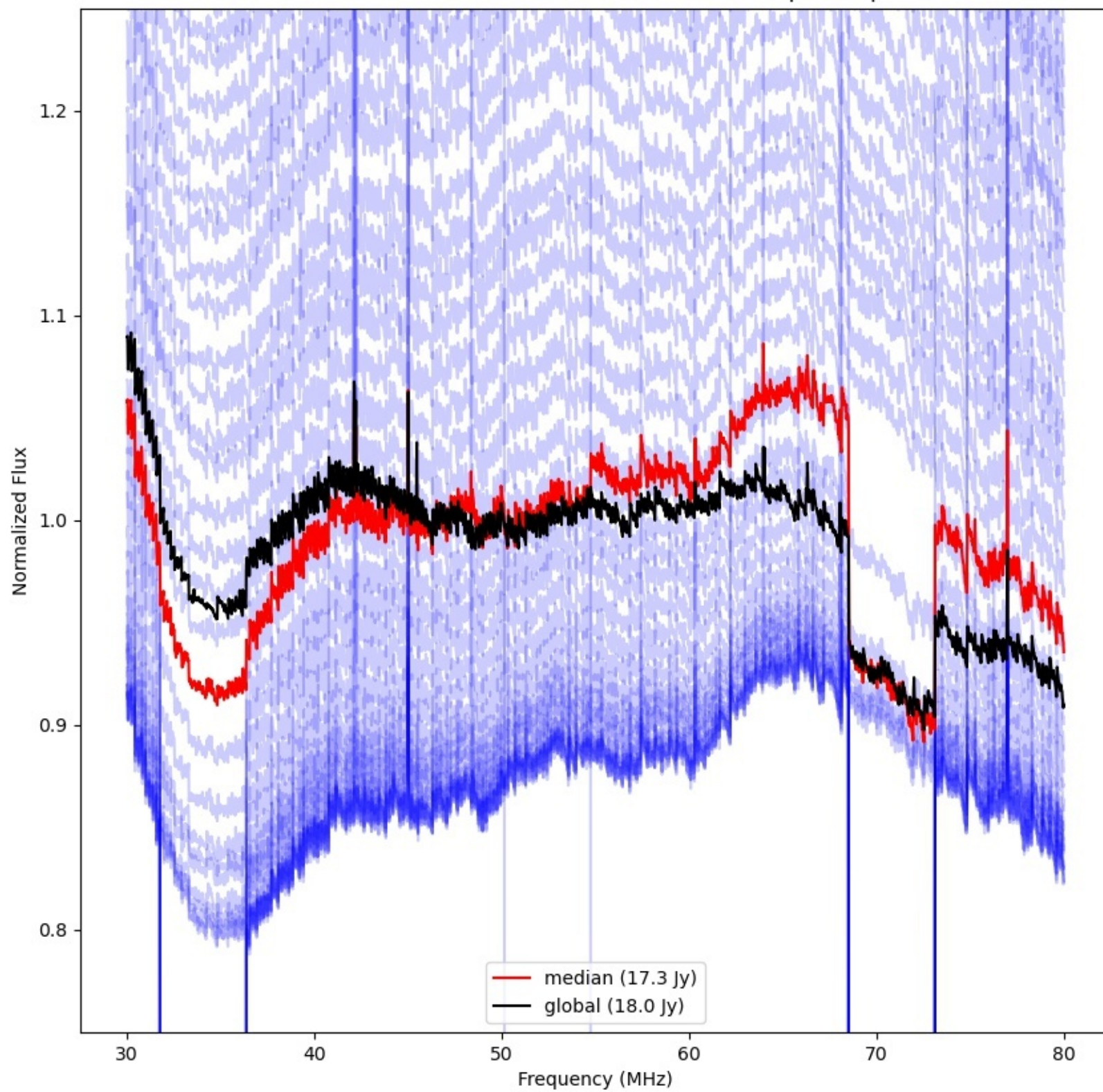
LWA210 - Correlator# 300 - YY - FLAGS:BadSpecShape
