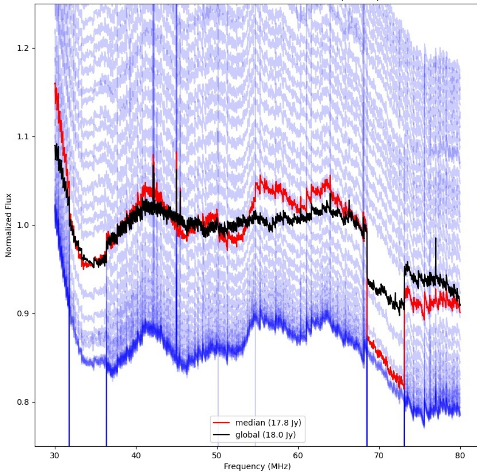
LWA315 - Correlator# 350 - YY - FLAGS:BadSpecShape
