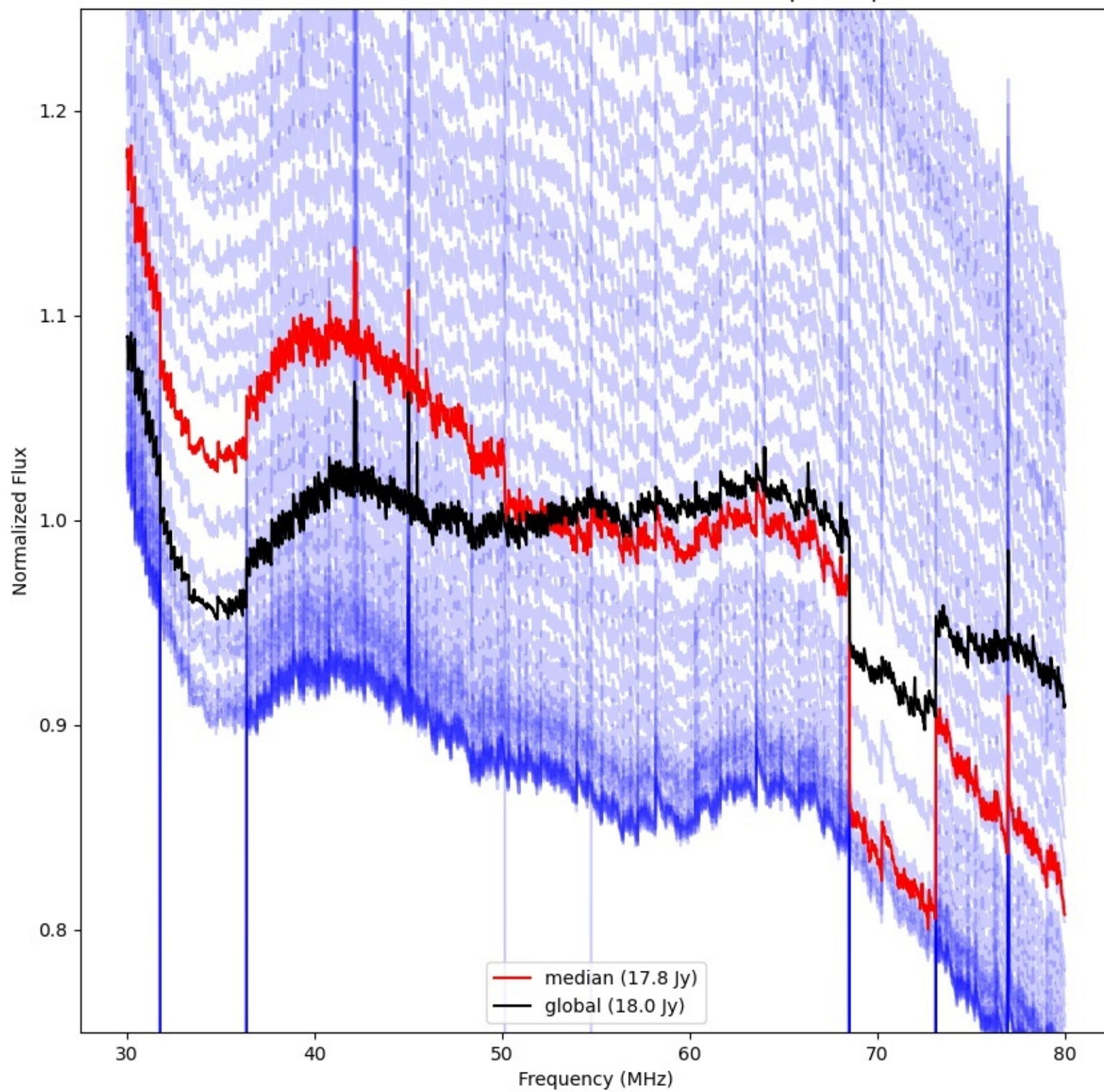
LWA175 - Correlator# 293 - YY - FLAGS:BadSpecShape
