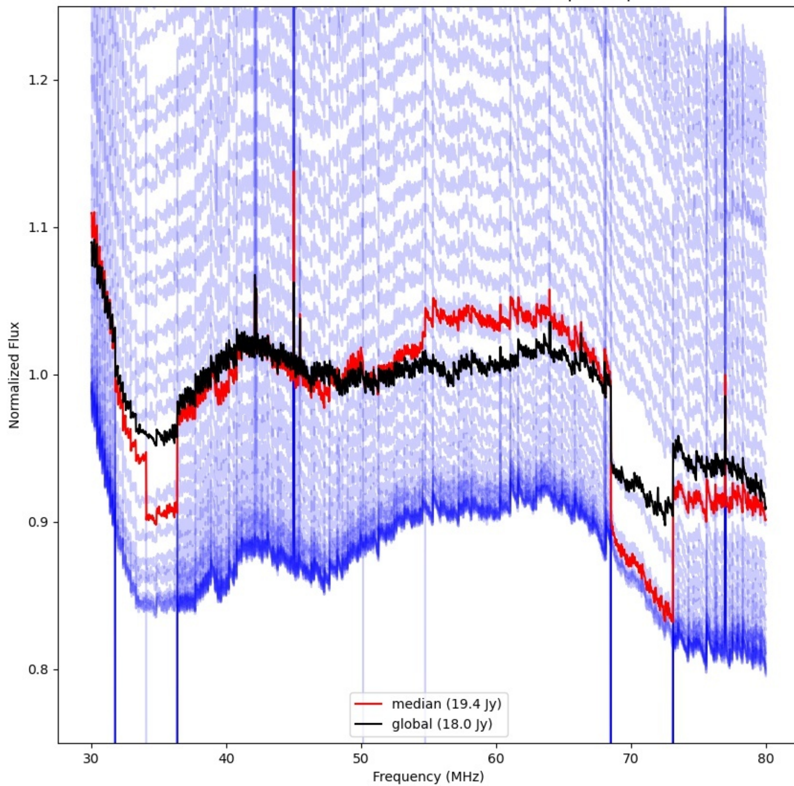
LWA346 - Correlator# 316 - YY - FLAGS:BadSpecShape
