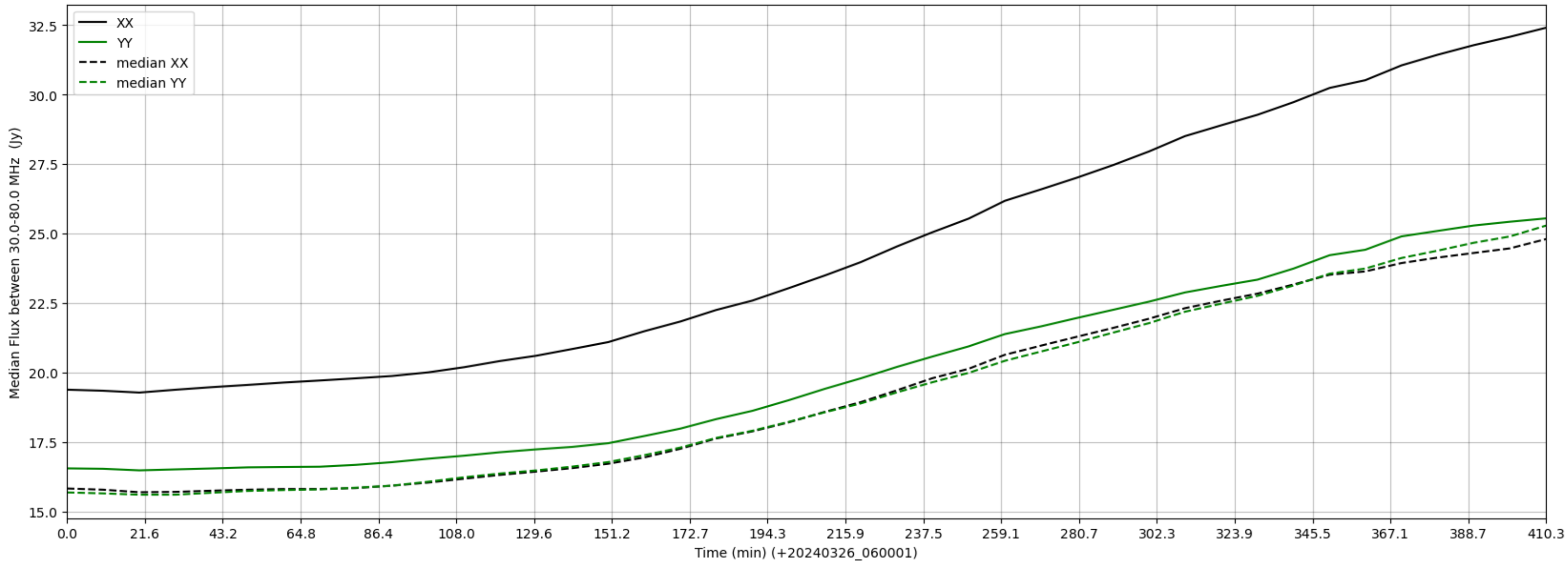
LWA308 - Correlator# 015 - XX FLAGS:Good - YY FLAGS:Good
