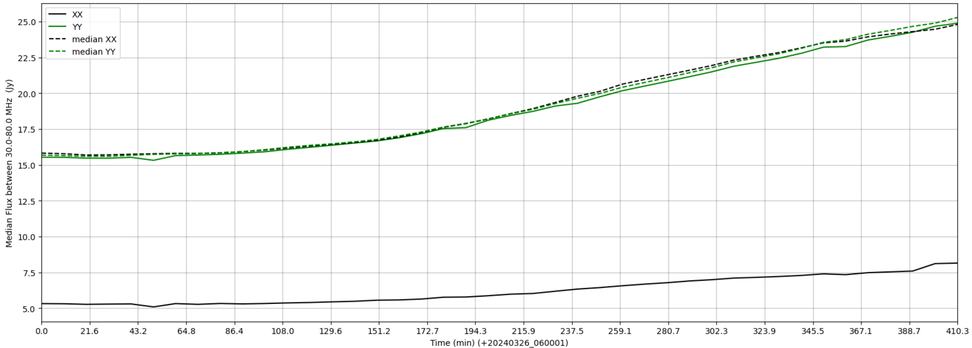
LWA130 - Correlator# 183 - XX FLAGS:Good - YY FLAGS:Good
