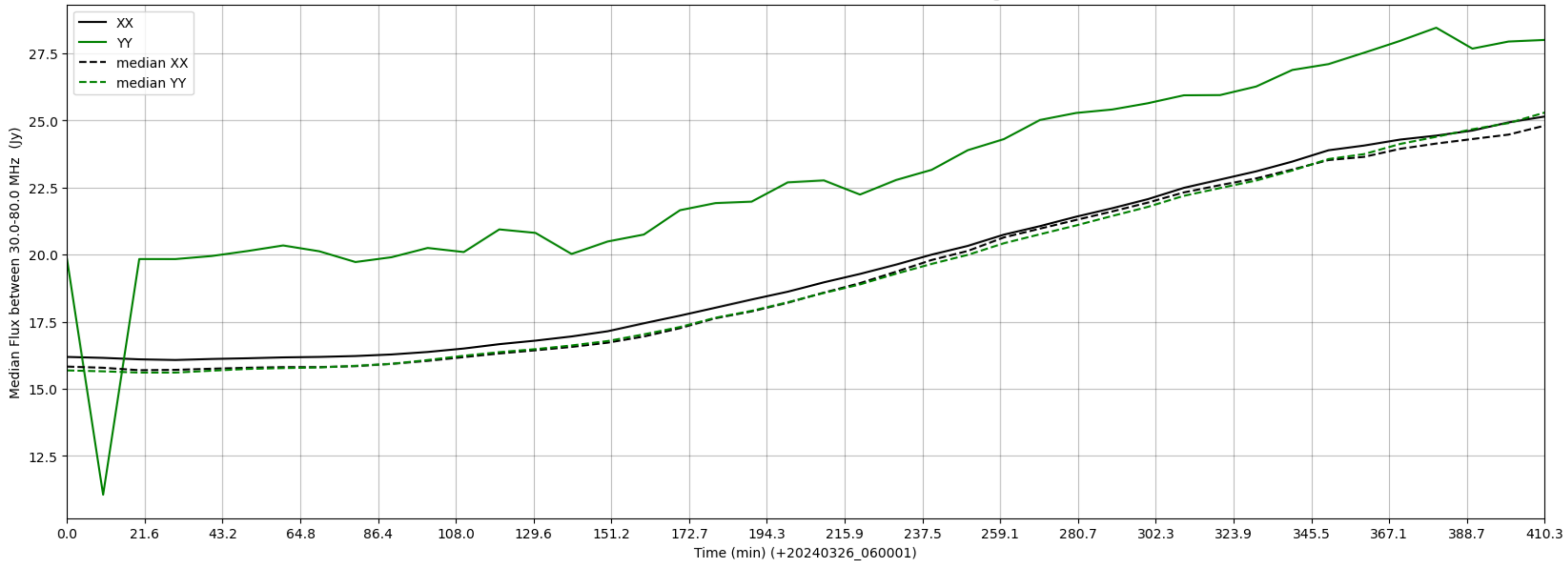
LWA358 - Correlator# 159 - XX FLAGS:Good - YY FLAGS:HighTimeVar
