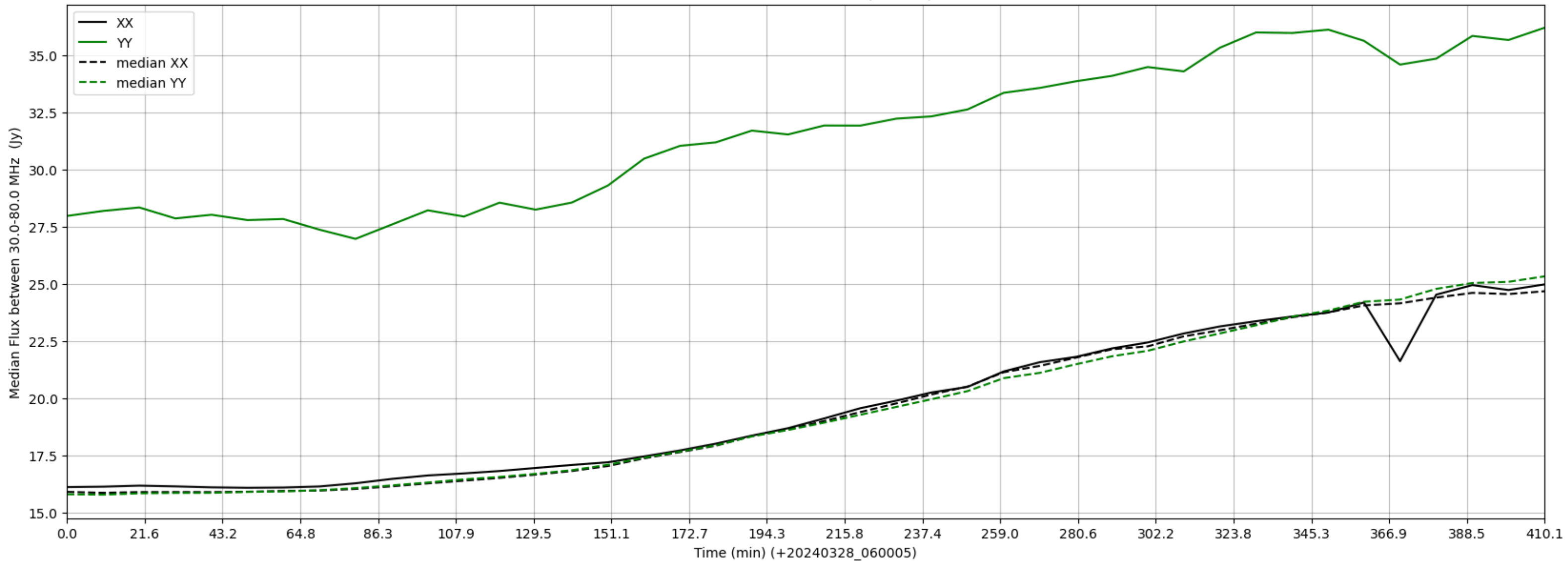
LWA358 - Correlator# 159 - XX FLAGS:BadSpecShape - YY FLAGS:Good
