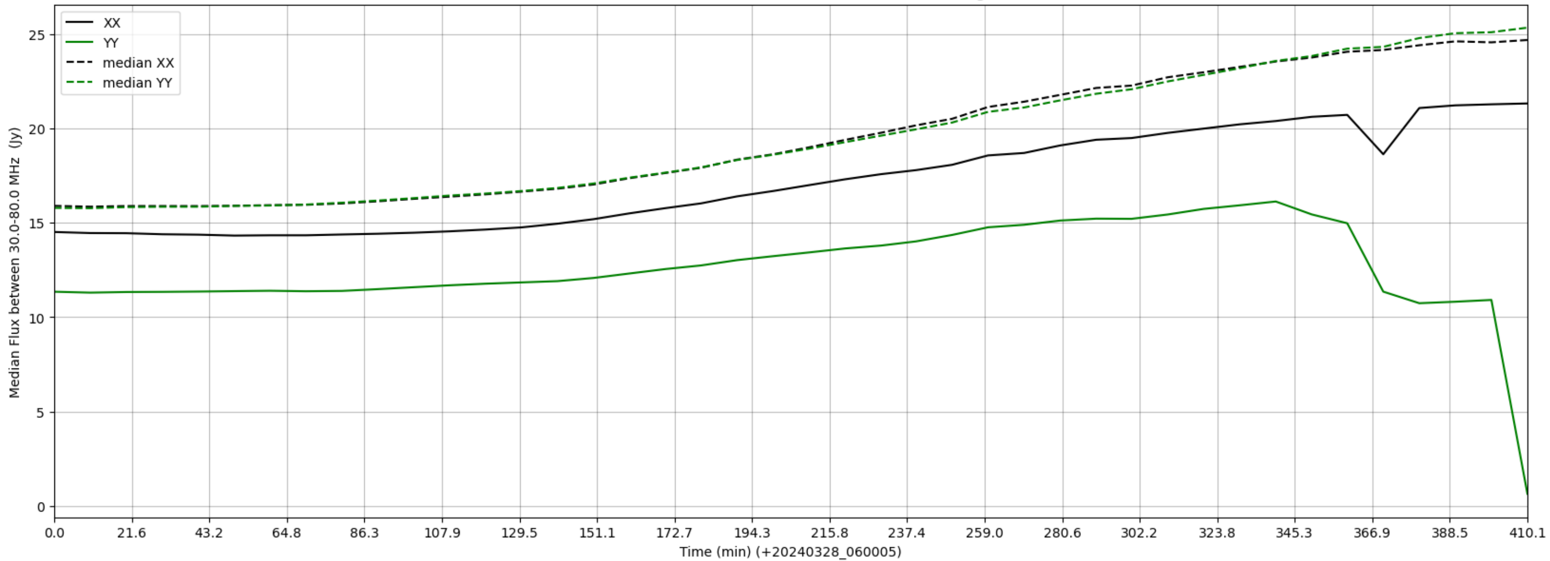
LWA314 - Correlator# 021 - XX FLAGS:Good - YY FLAGS:HighTimeVar
