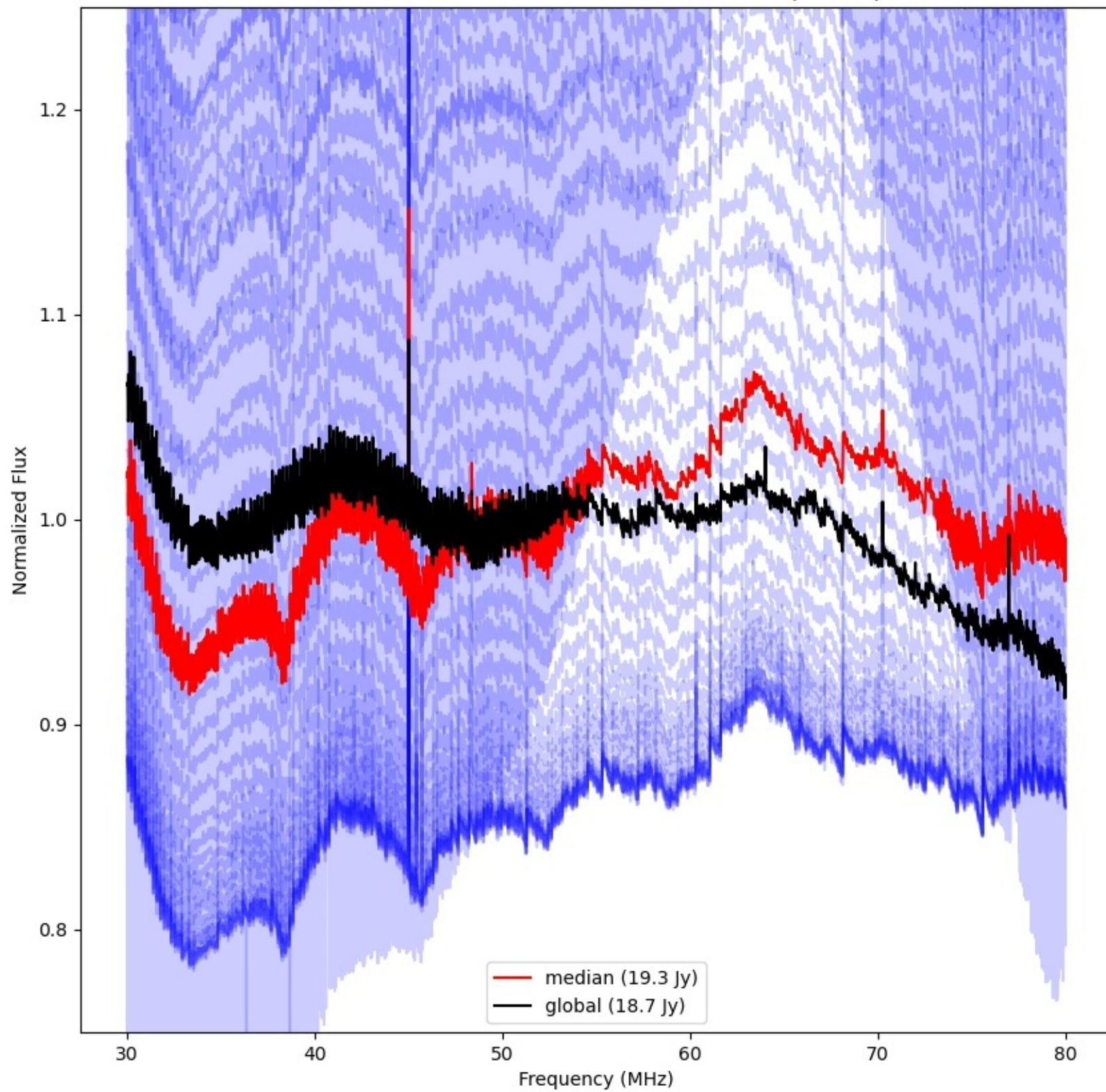
LWA326 - Correlator# 250 - XX - FLAGS:BadSpecShape
