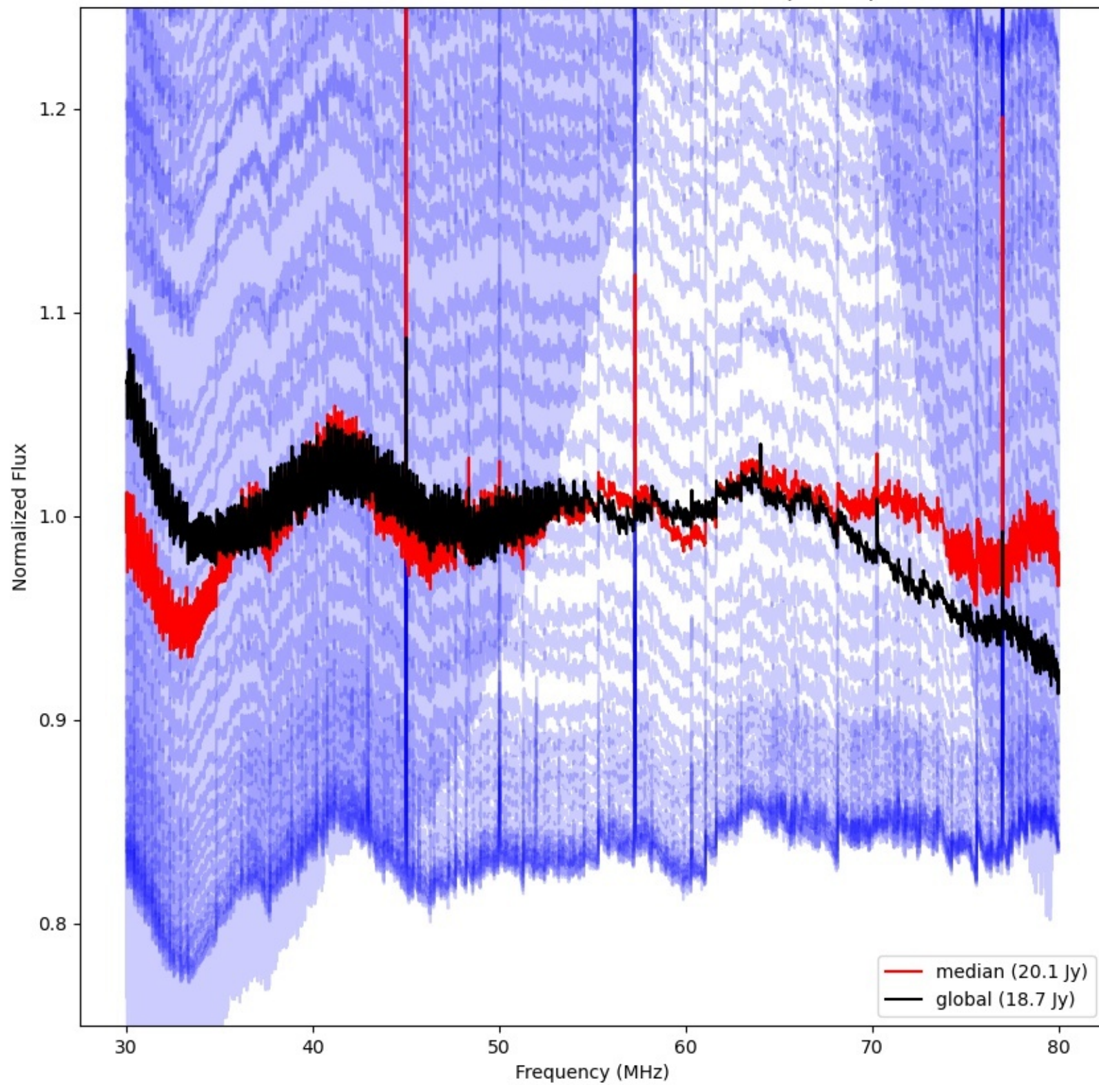
LWA355 - Correlator# 222 - XX - FLAGS:BadSpecShape
