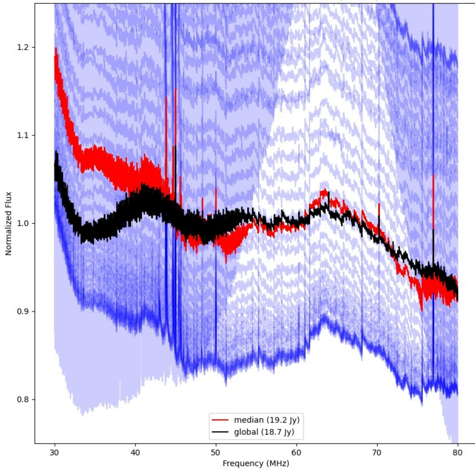
LWA325 - Correlator# 154 - XX - FLAGS:BadSpecShape
