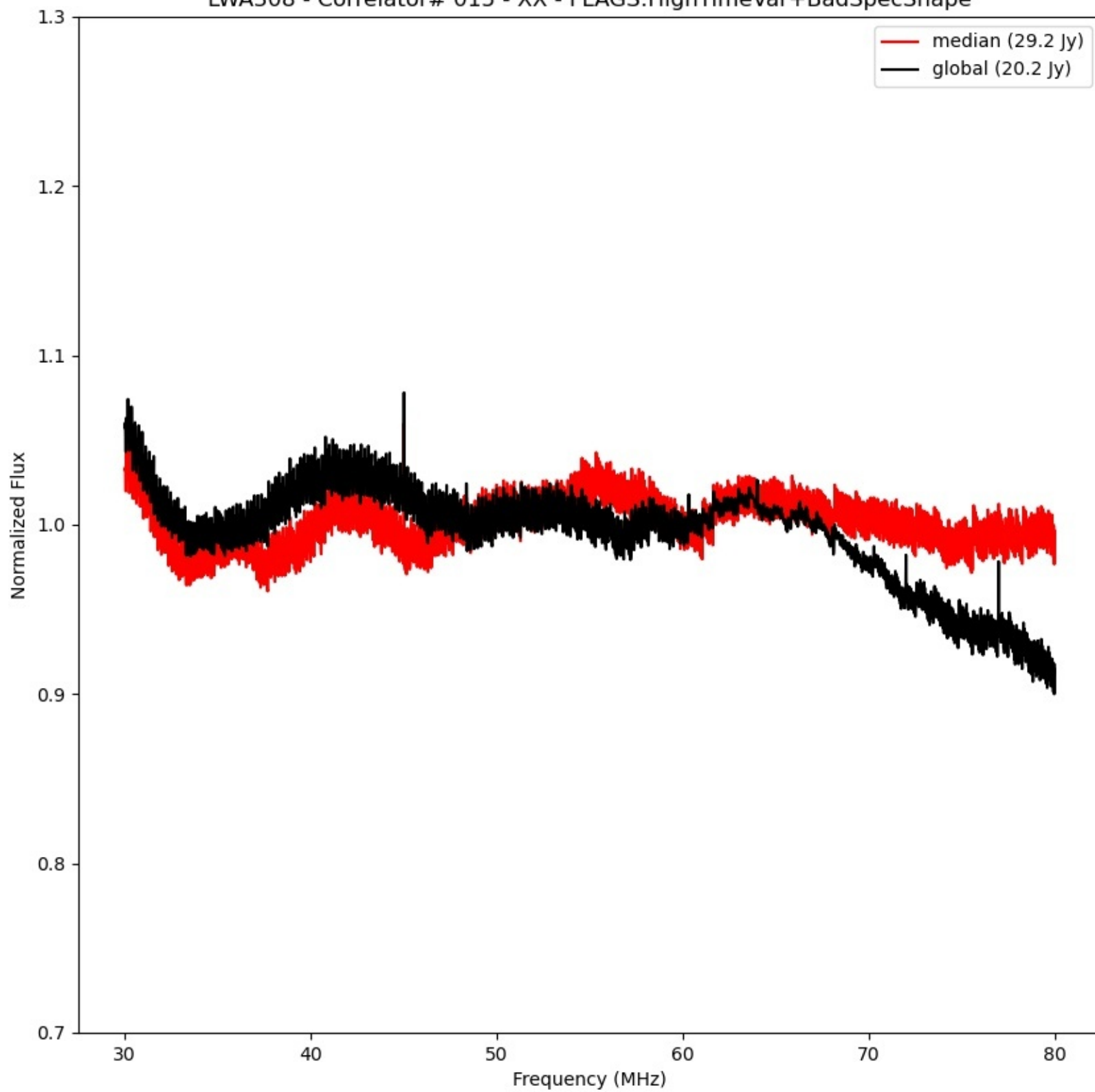
LWA308 - Correlator# 015 - XX - FLAGS:HighTimeVar+BadSpecShape
