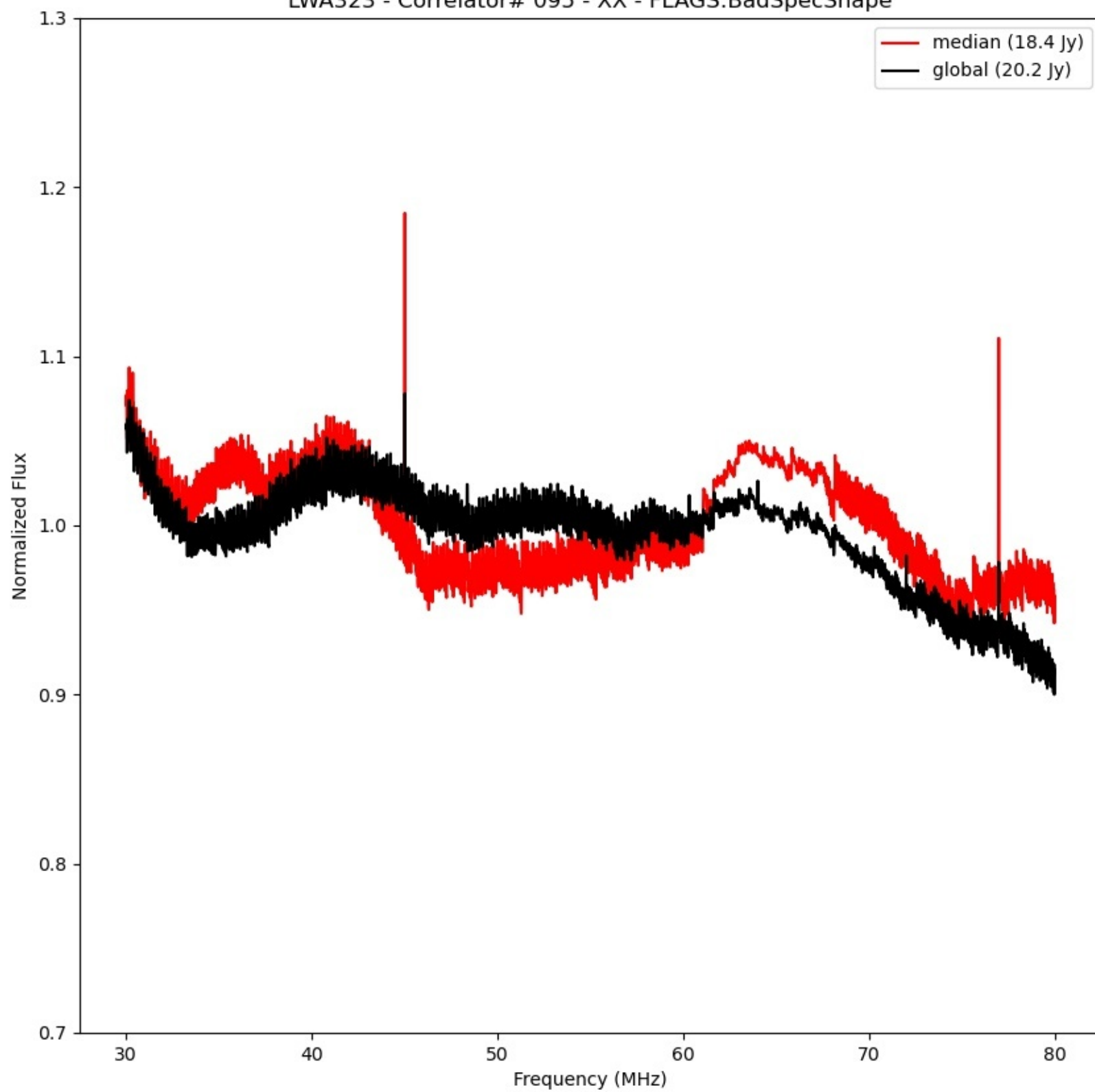
LWA323 - Correlator# 095 - XX - FLAGS:BadSpecShape
