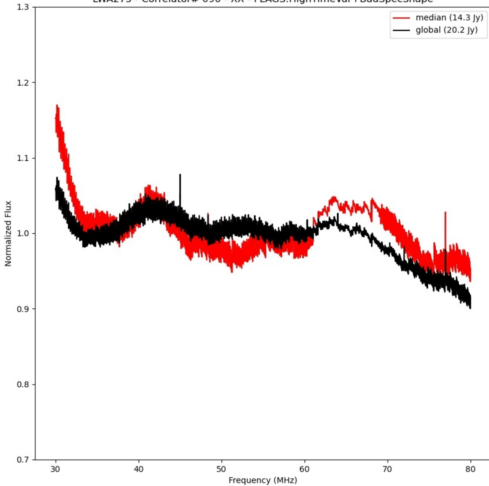
LWA275 - Correlator# 090 - XX - FLAGS:HighTimeVar+BadSpecShape
