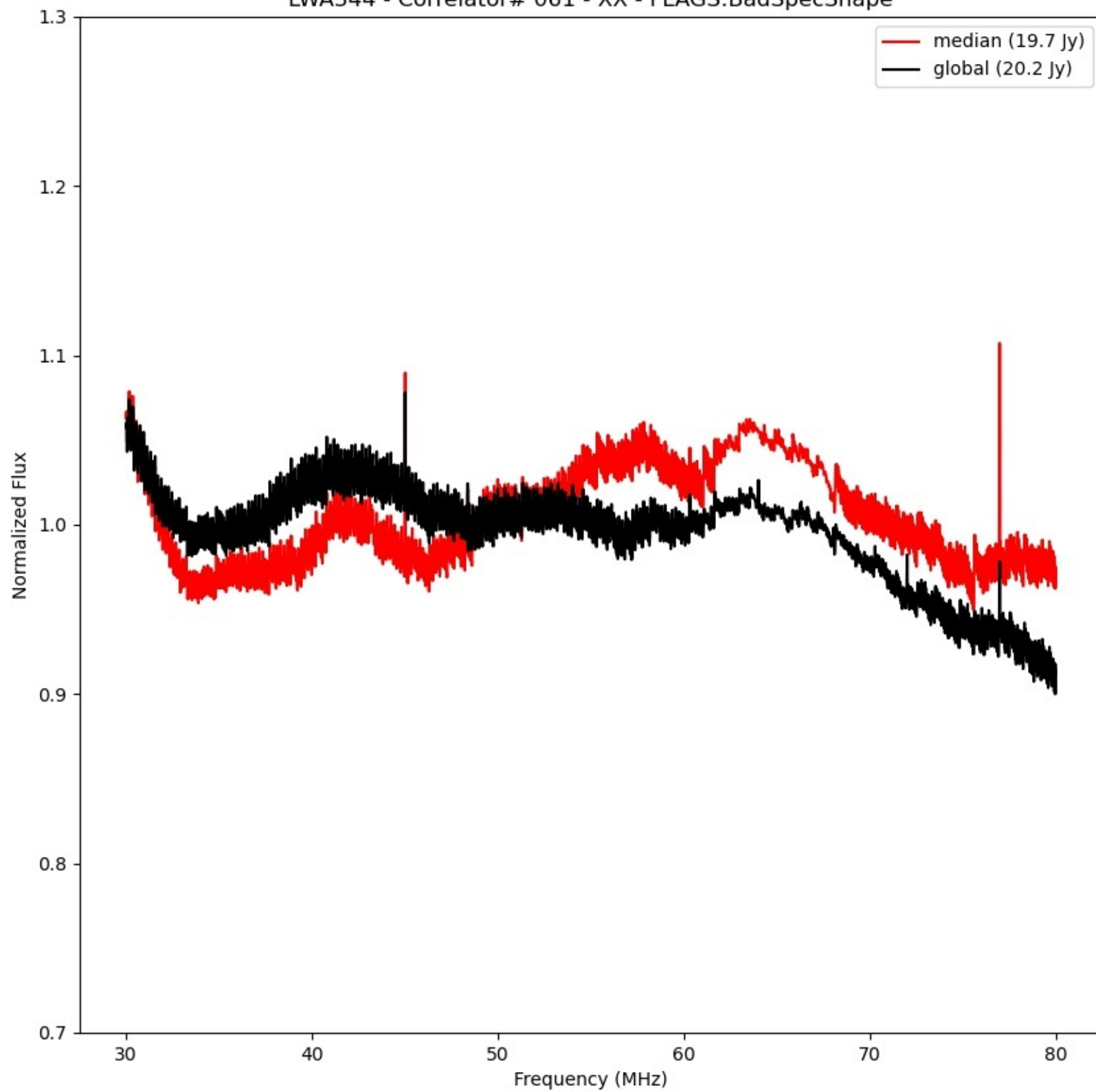
LWA344 - Correlator# 061 - XX - FLAGS:BadSpecShape
