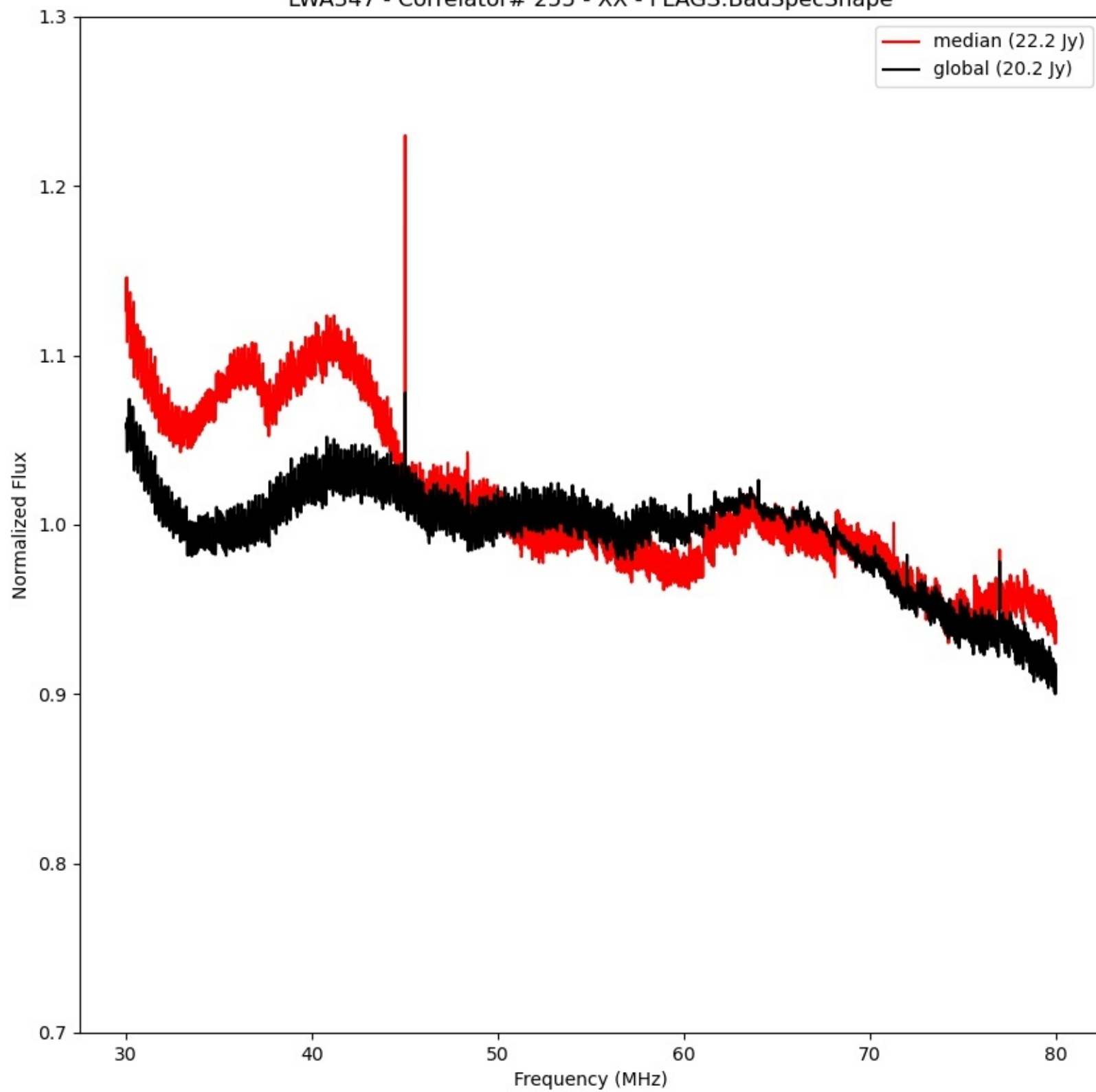
LWA347 - Correlator# 255 - XX - FLAGS:BadSpecShape
