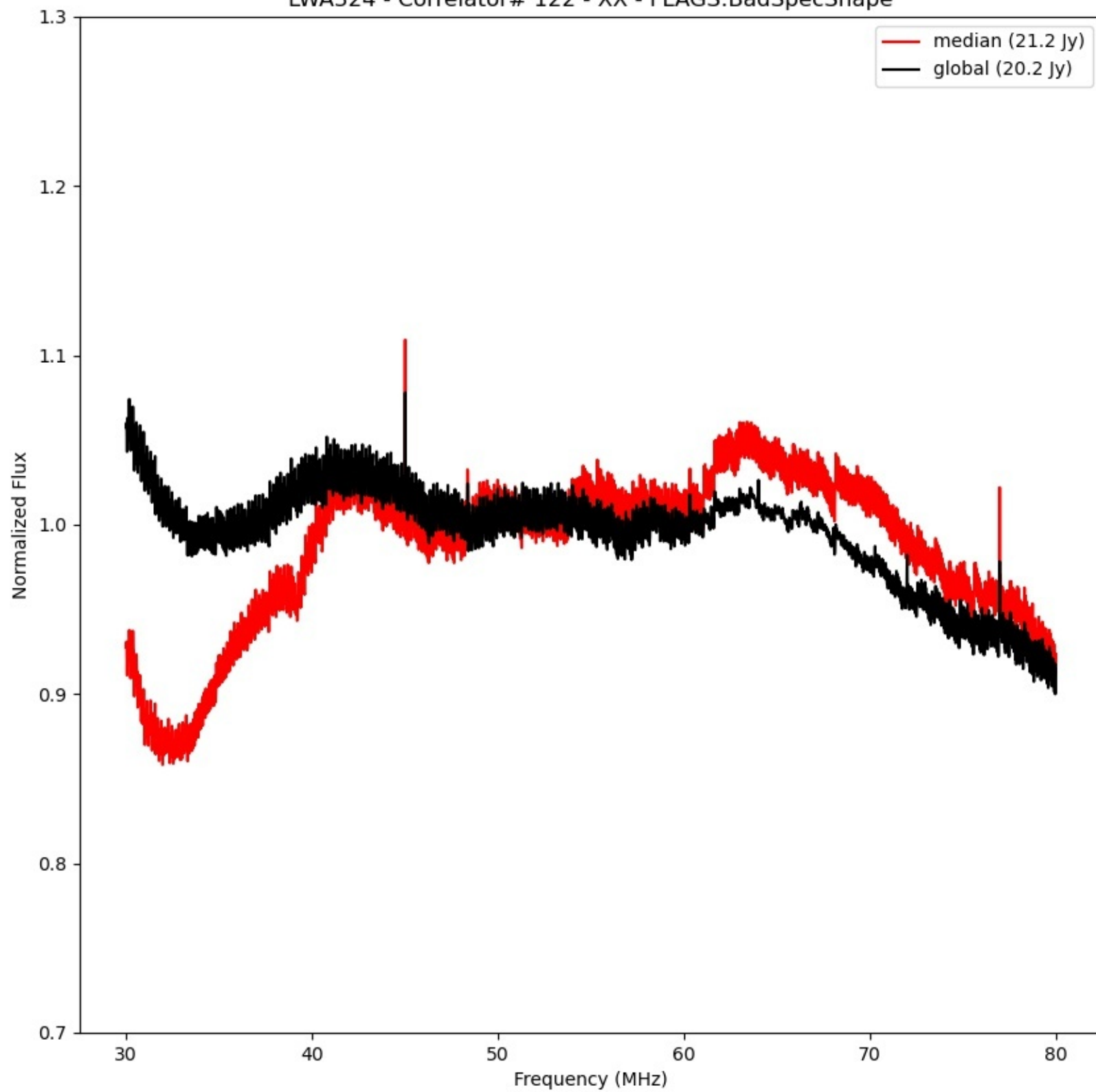
LWA324 - Correlator# 122 - XX - FLAGS:BadSpecShape
