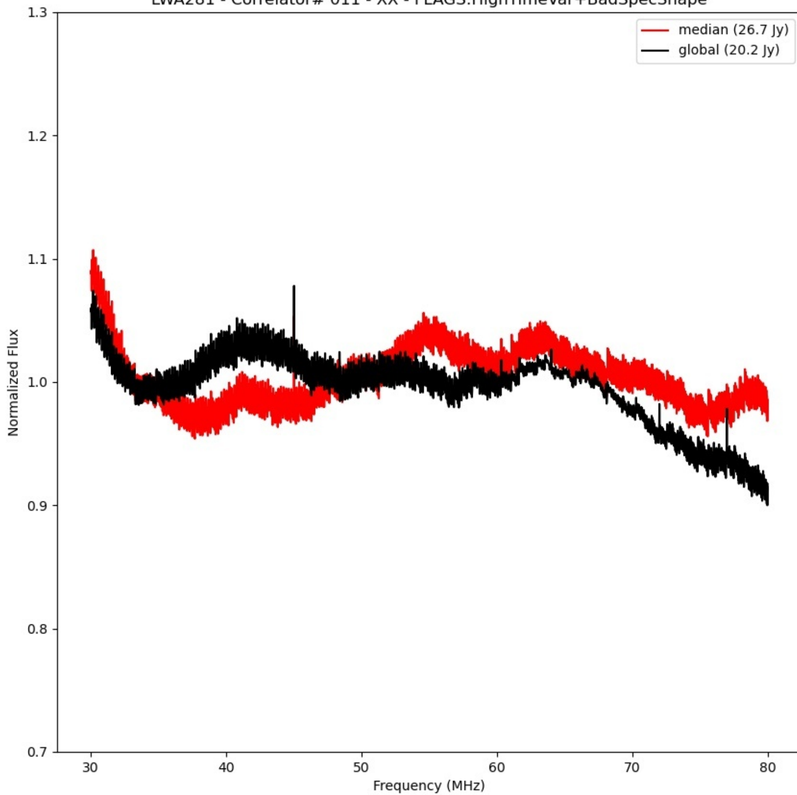
LWA281 - Correlator# 011 - XX - FLAGS:HighTimeVar+BadSpecShape
