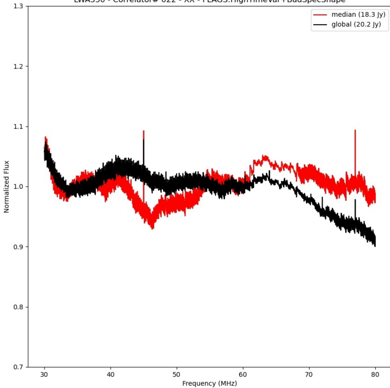
LWA330 - Correlator# 022 - XX - FLAGS:HighTimeVar+BadSpecShape
