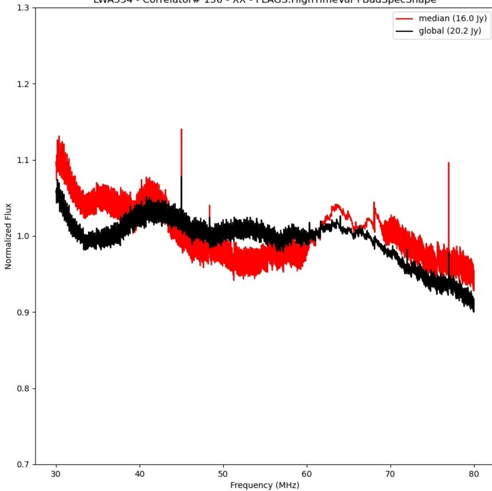
LWA334 - Correlator# 156 - XX - FLAGS:HighTimeVar+BadSpecShape
