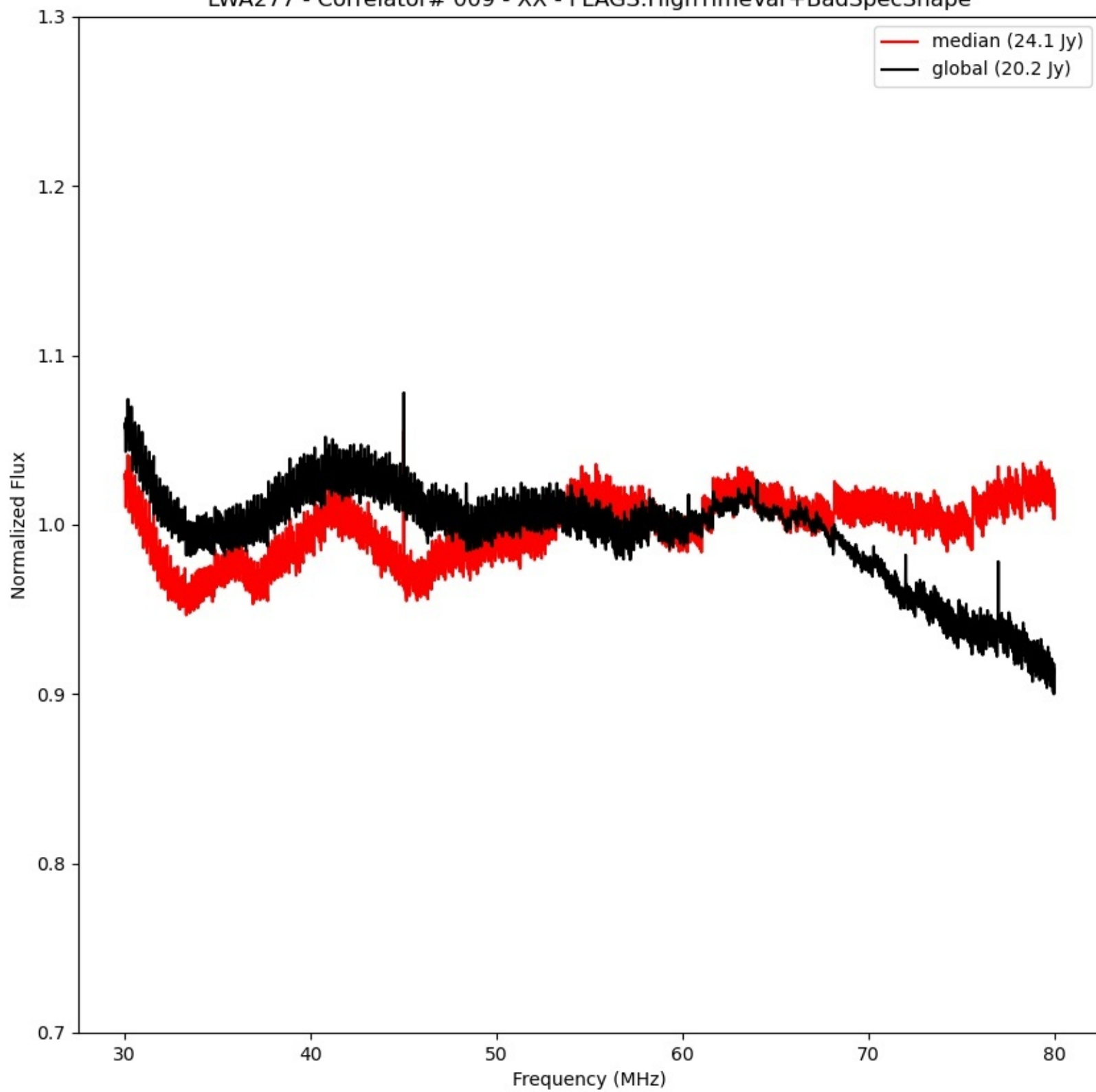
LWA277 - Correlator# 009 - XX - FLAGS:HighTimeVar+BadSpecShape
