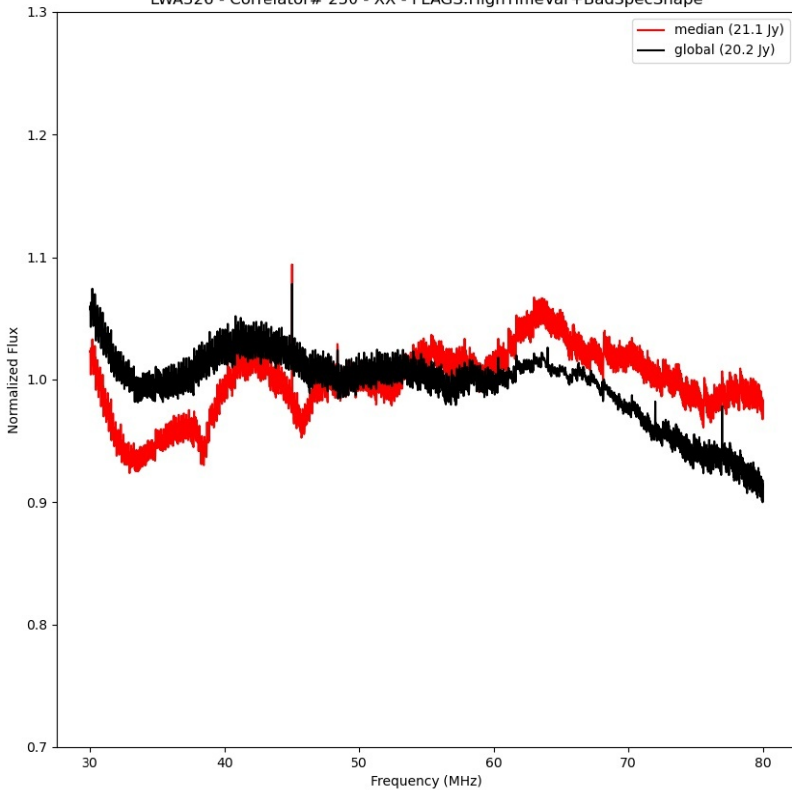
LWA326 - Correlator# 250 - XX - FLAGS:HighTimeVar+BadSpecShape
