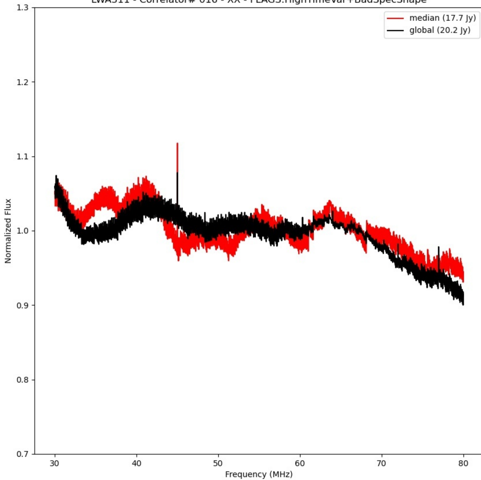
LWA311 - Correlator# 016 - XX - FLAGS:HighTimeVar+BadSpecShape
