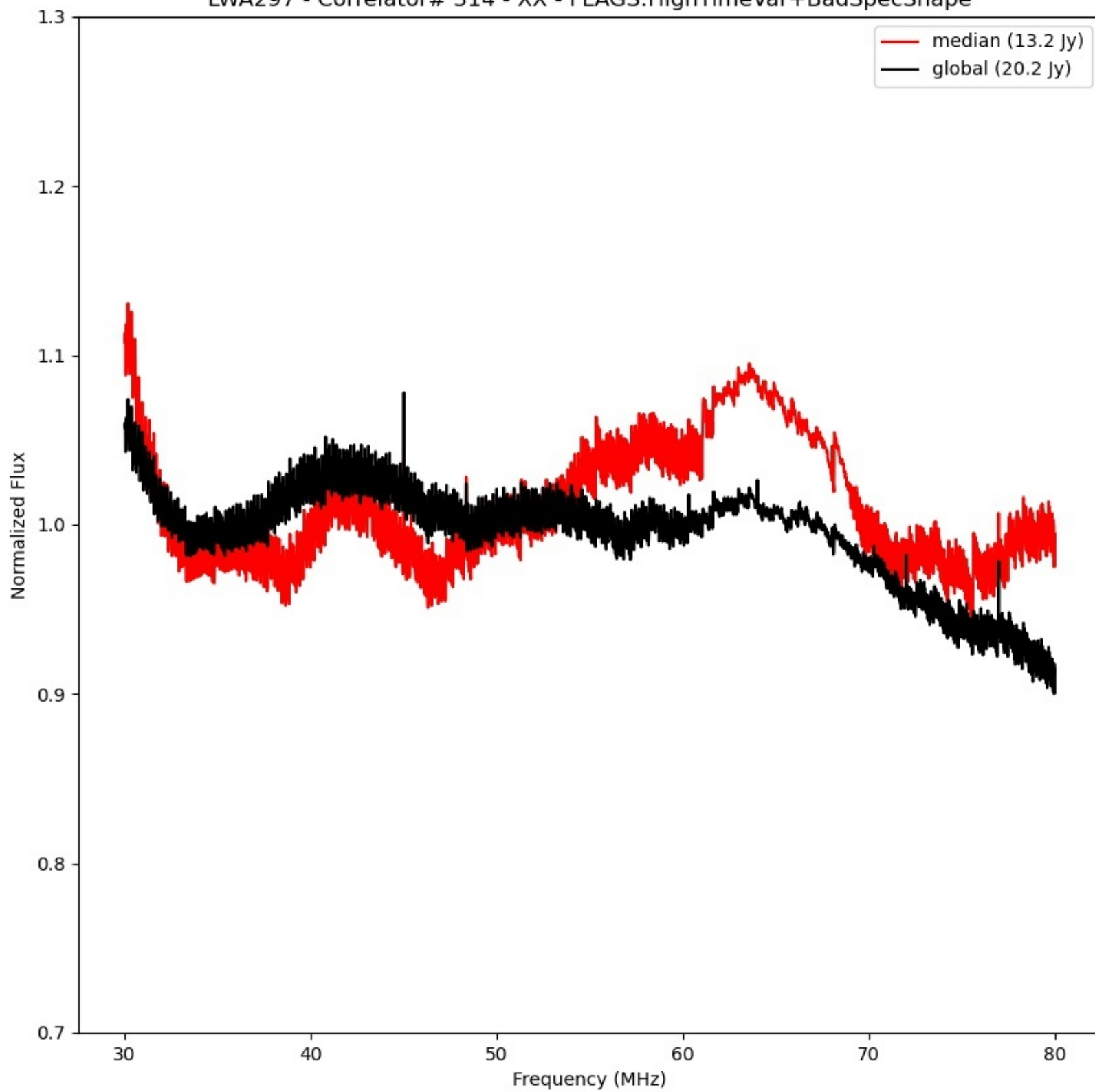
LWA297 - Correlator# 314 - XX - FLAGS:HighTimeVar+BadSpecShape
