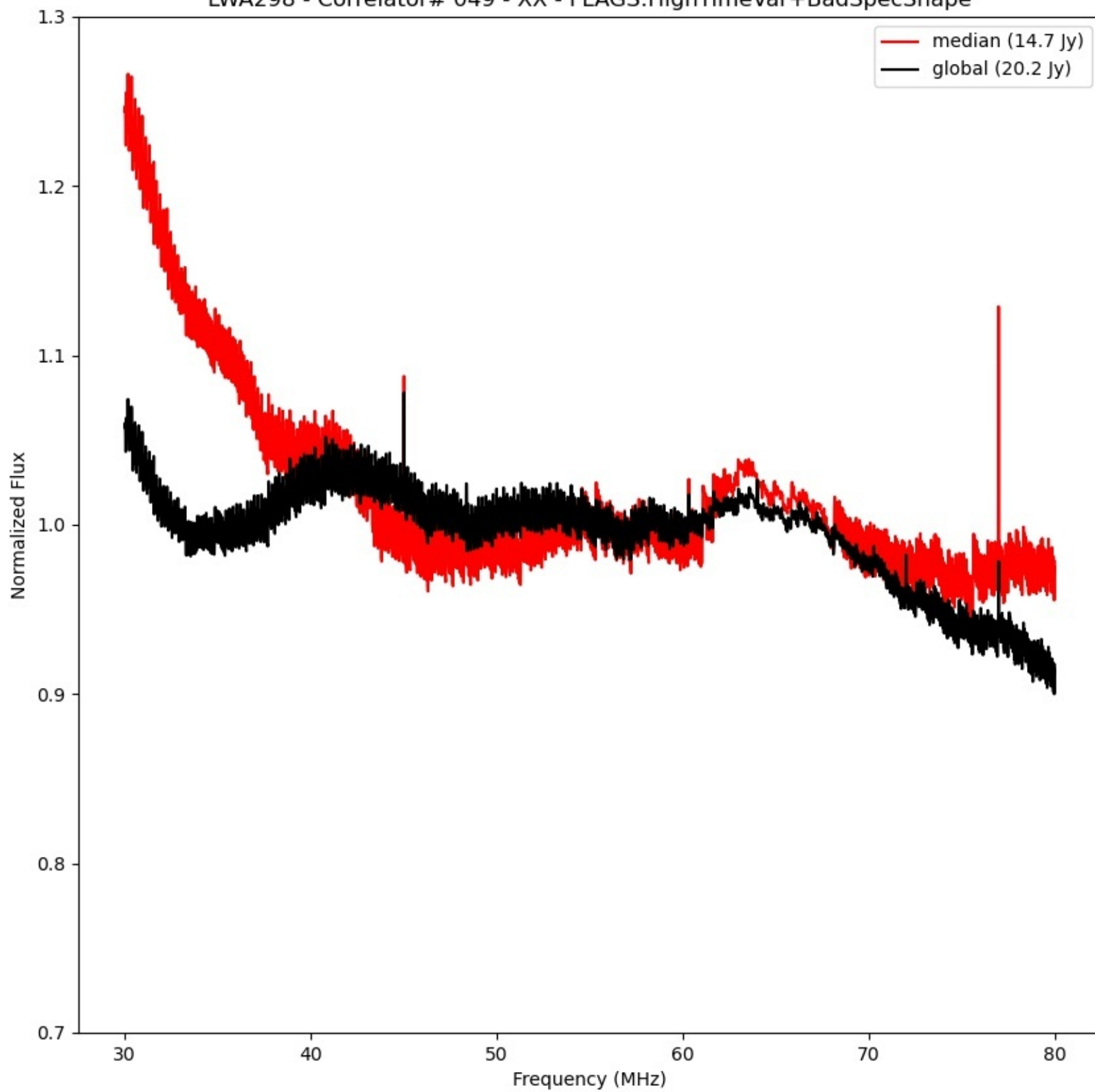
LWA298 - Correlator# 049 - XX - FLAGS:HighTimeVar+BadSpecShape
