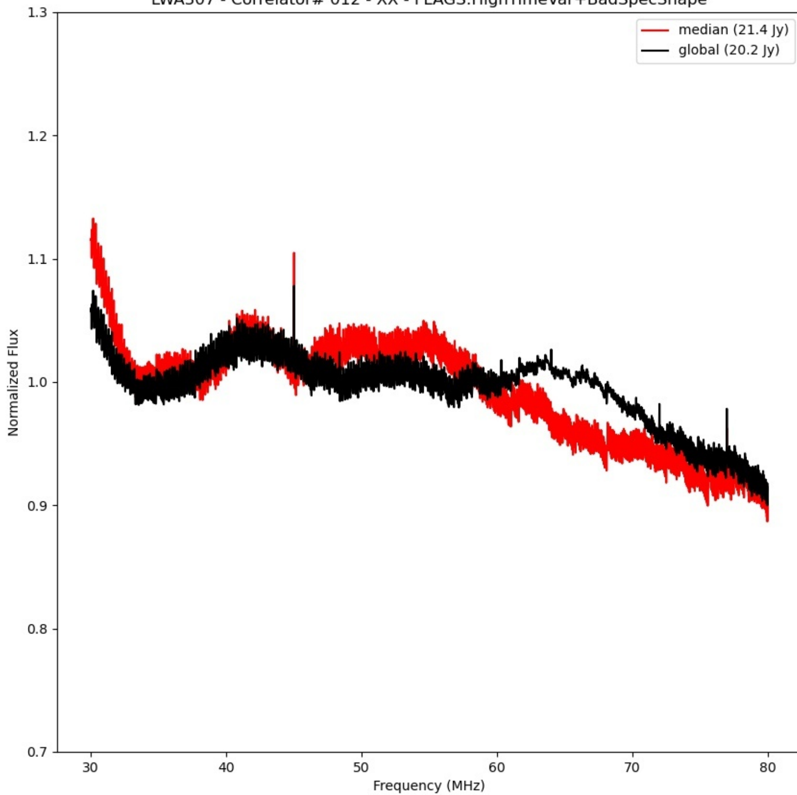
LWA307 - Correlator# 012 - XX - FLAGS:HighTimeVar+BadSpecShape
