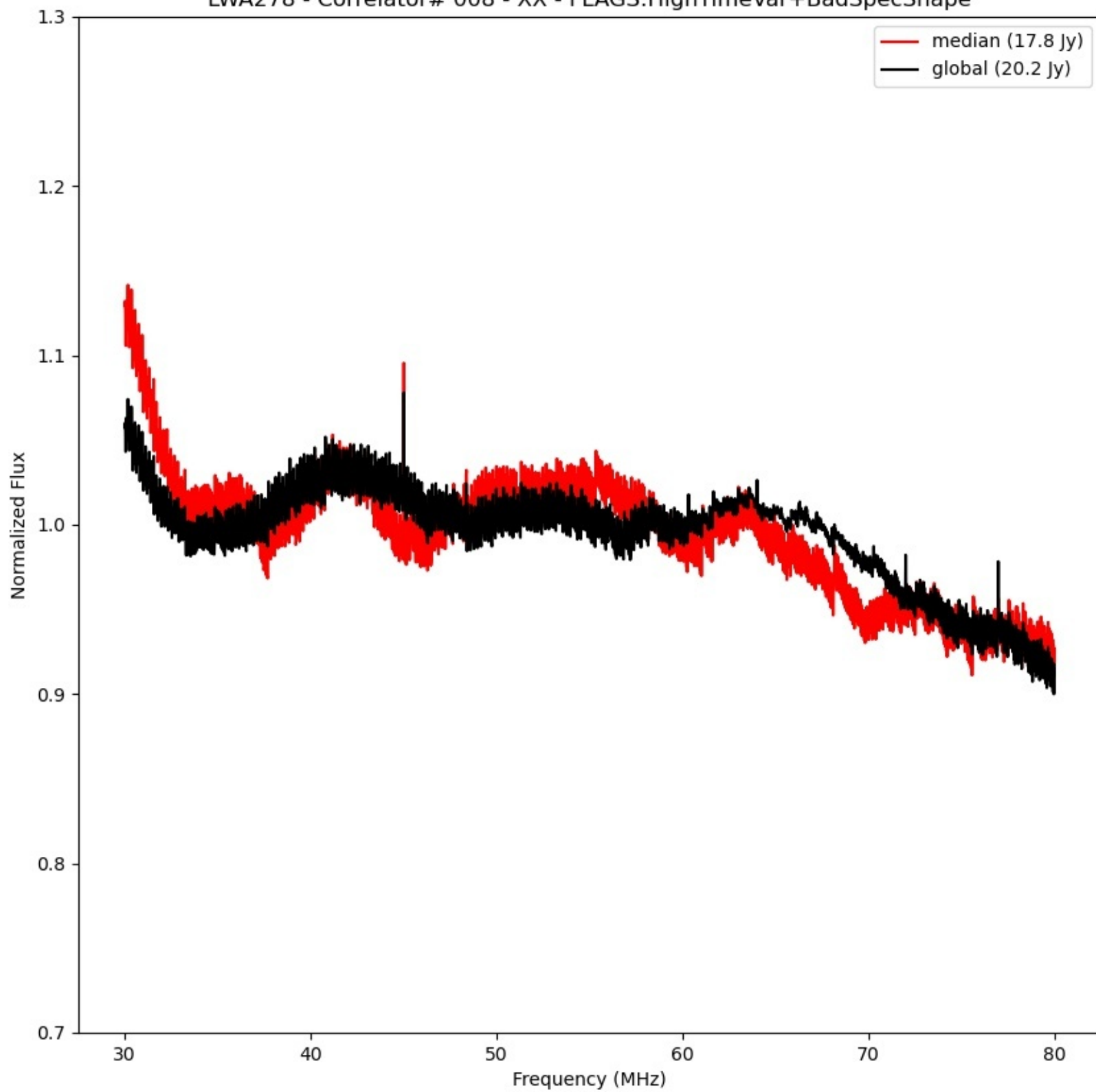
LWA278 - Correlator# 008 - XX - FLAGS:HighTimeVar+BadSpecShape
