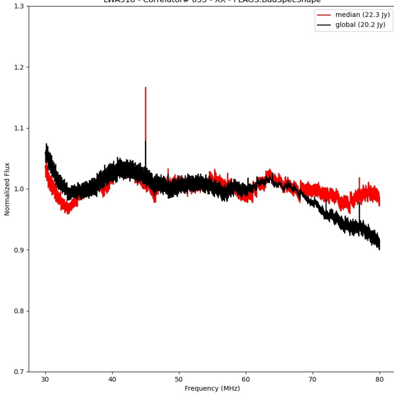
LWA318 - Correlator# 055 - XX - FLAGS:BadSpecShape
