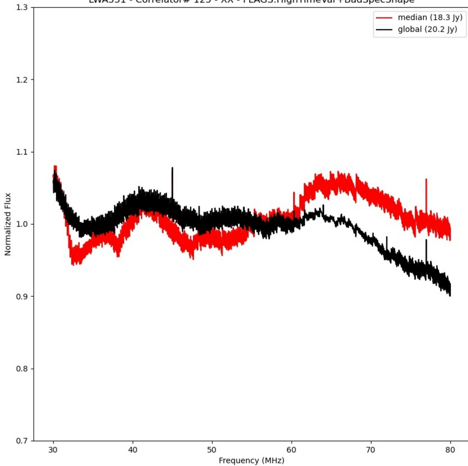
LWA331 - Correlator# 125 - XX - FLAGS:HighTimeVar+BadSpecShape
