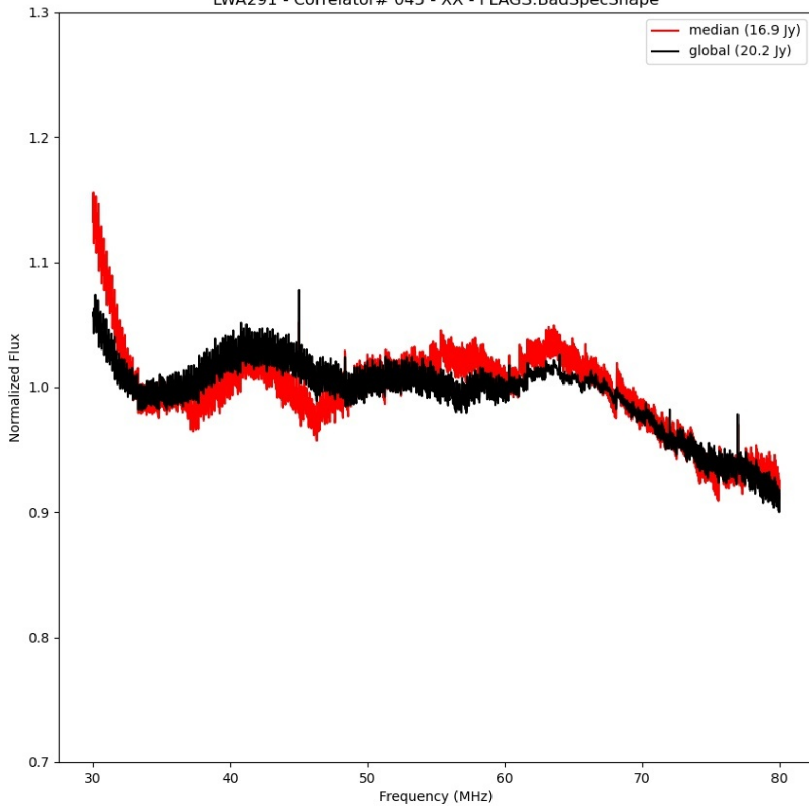
LWA291 - Correlator# 045 - XX - FLAGS:BadSpecShape
