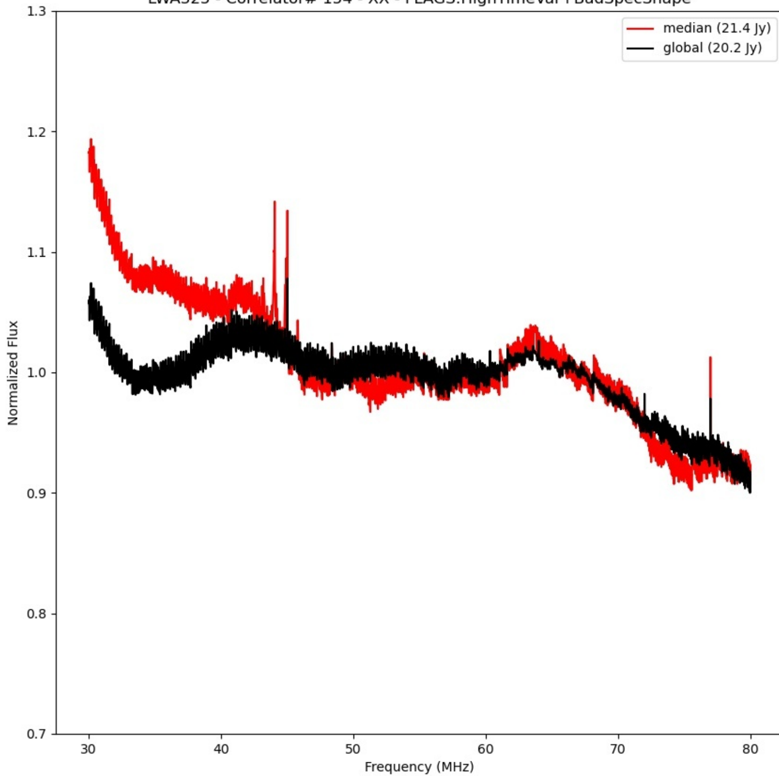
LWA325 - Correlator# 154 - XX - FLAGS:HighTimeVar+BadSpecShape
