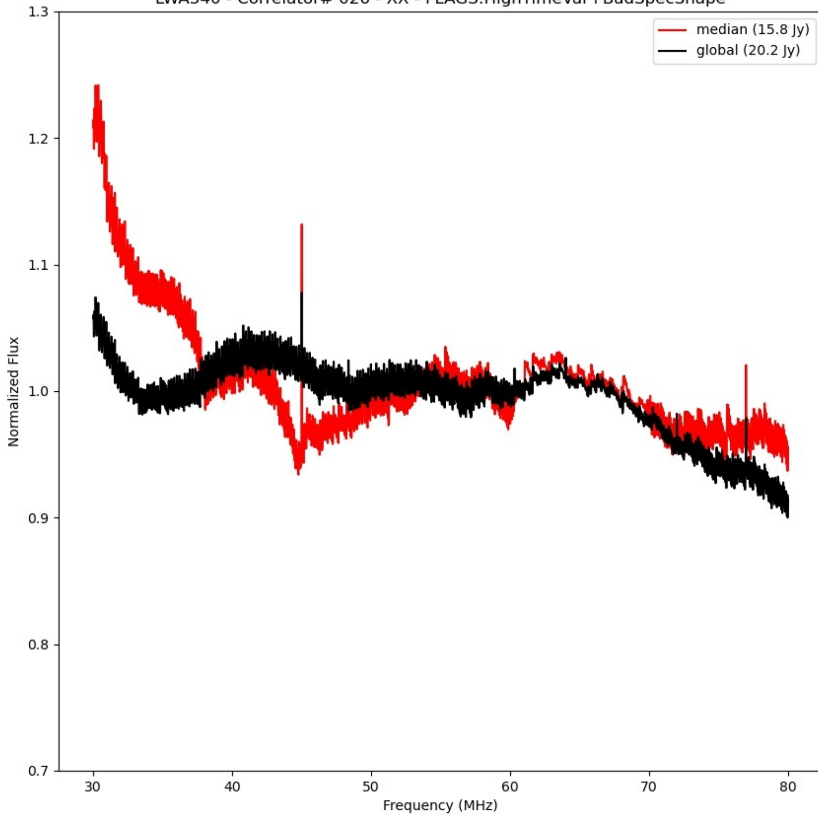
LWA340 - Correlator# 026 - XX - FLAGS:HighTimeVar+BadSpecShape
