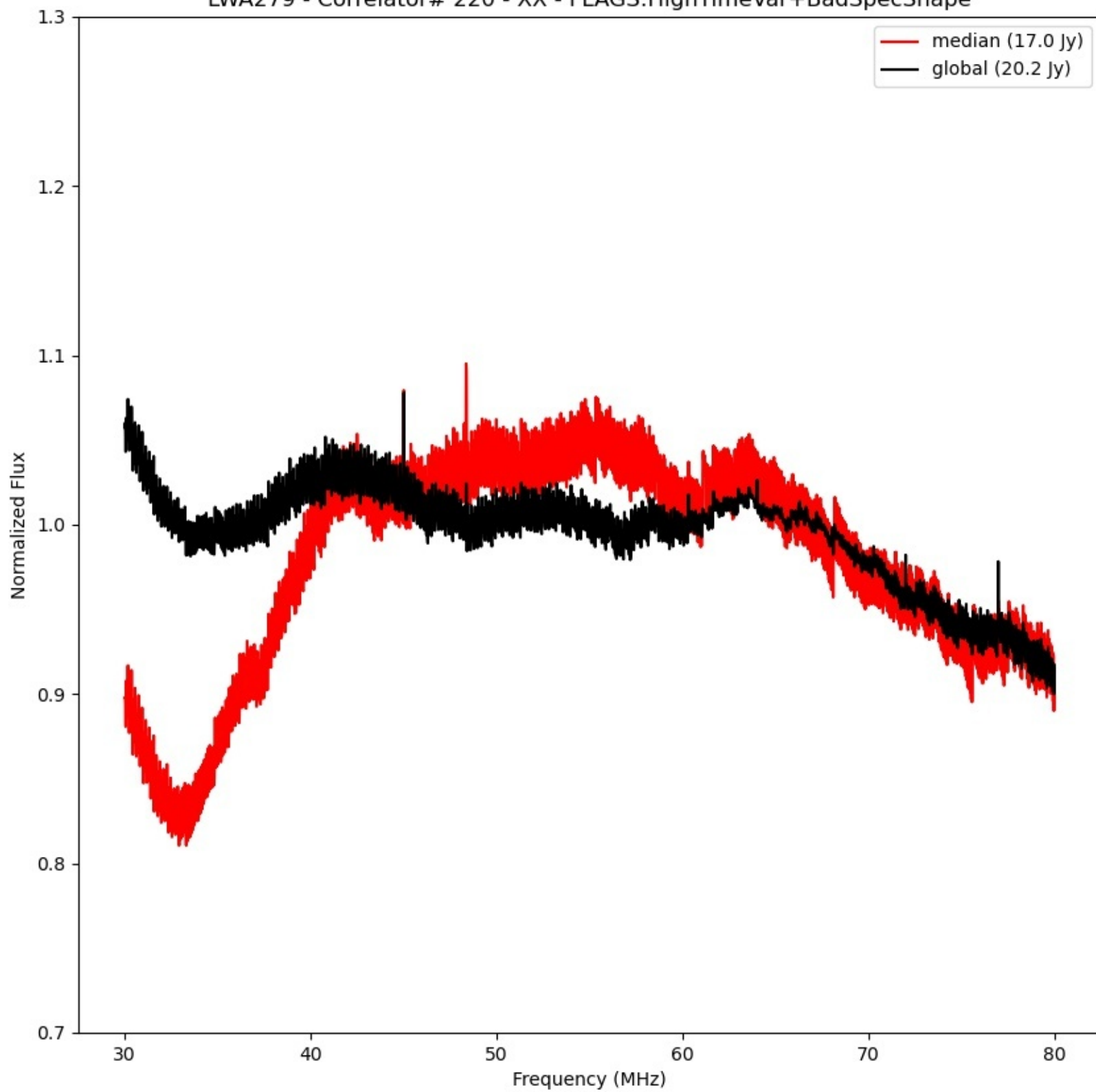
LWA279 - Correlator# 220 - XX - FLAGS:HighTimeVar+BadSpecShape
