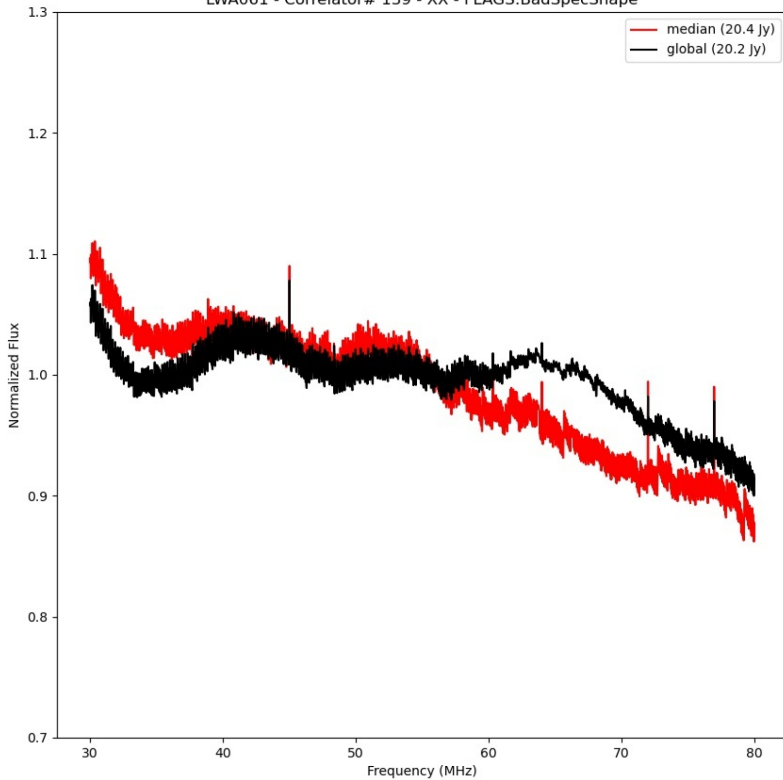
LWA061 - Correlator# 139 - XX - FLAGS:BadSpecShape
