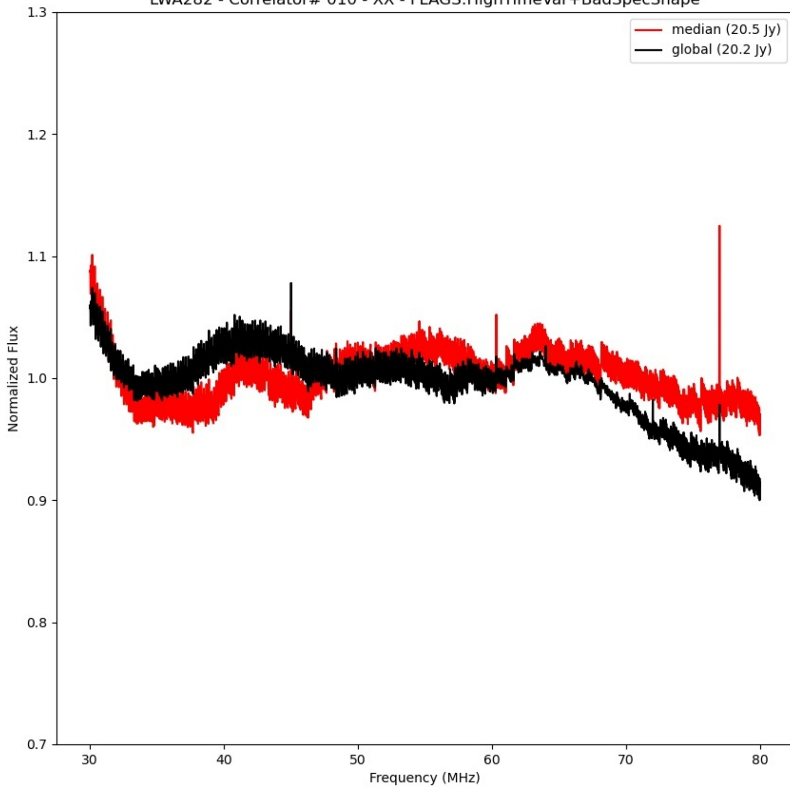
LWA282 - Correlator# 010 - XX - FLAGS:HighTimeVar+BadSpecShape
