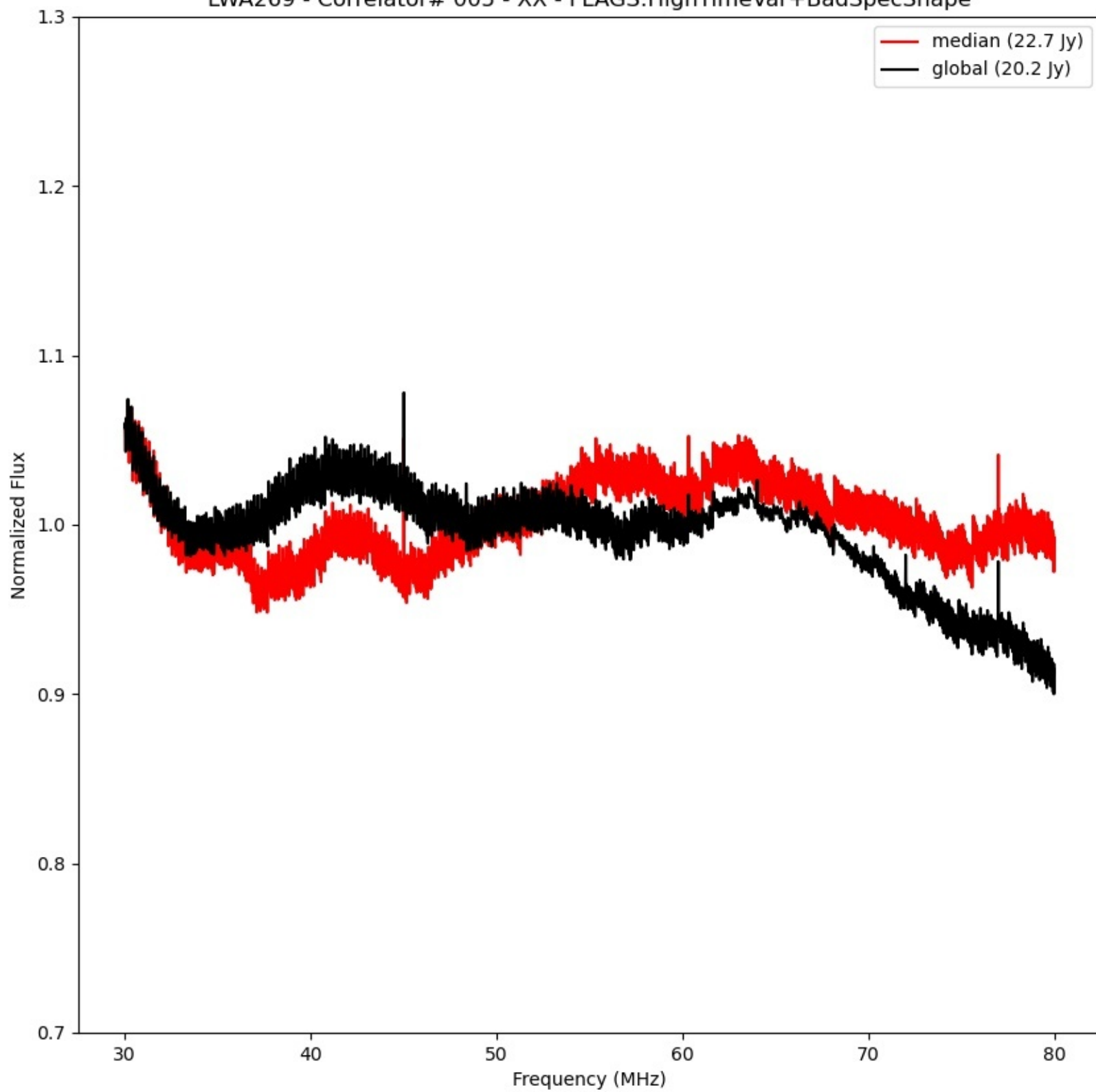
LWA269 - Correlator# 005 - XX - FLAGS:HighTimeVar+BadSpecShape
