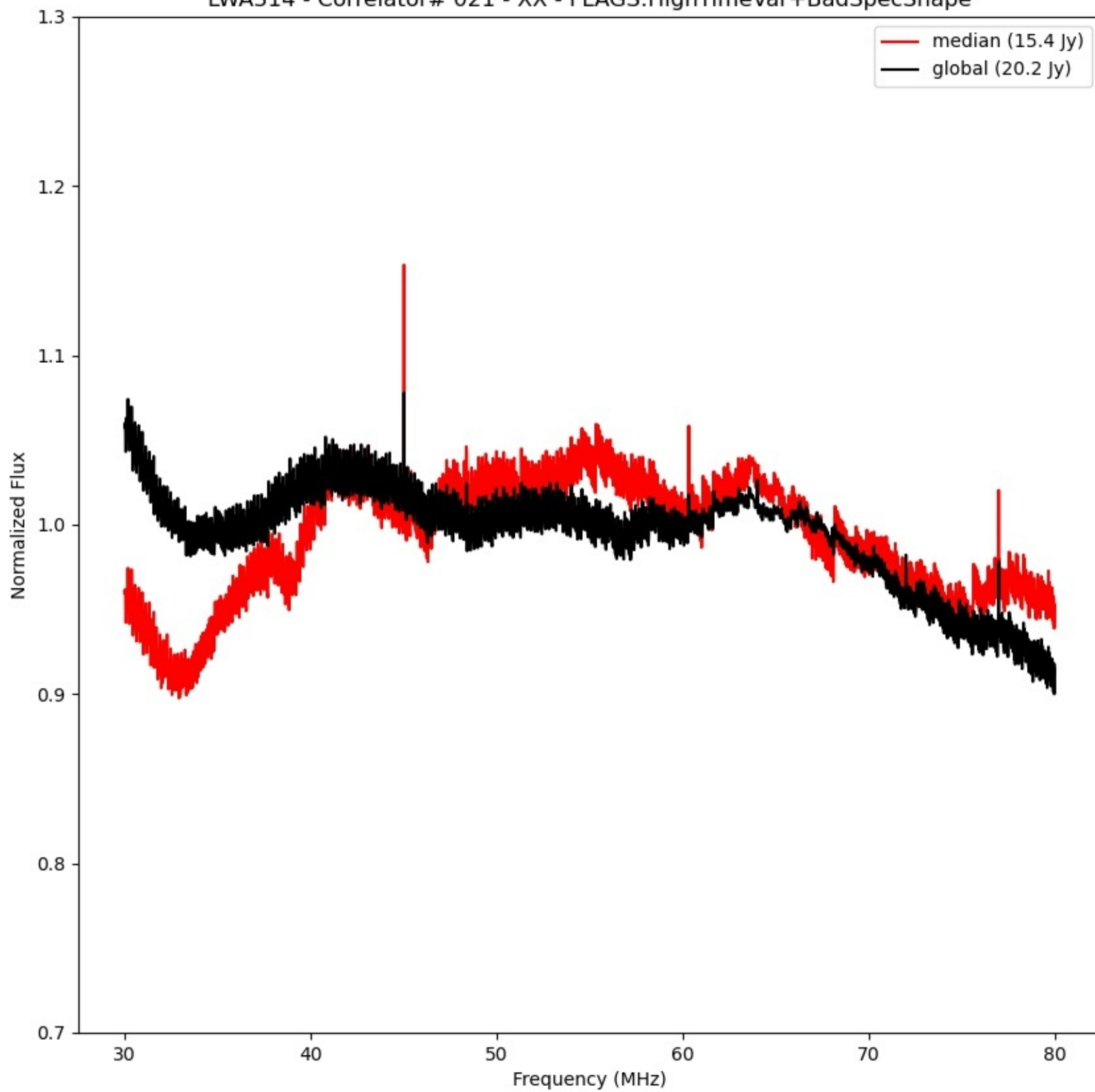
LWA314 - Correlator# 021 - XX - FLAGS:HighTimeVar+BadSpecShape
