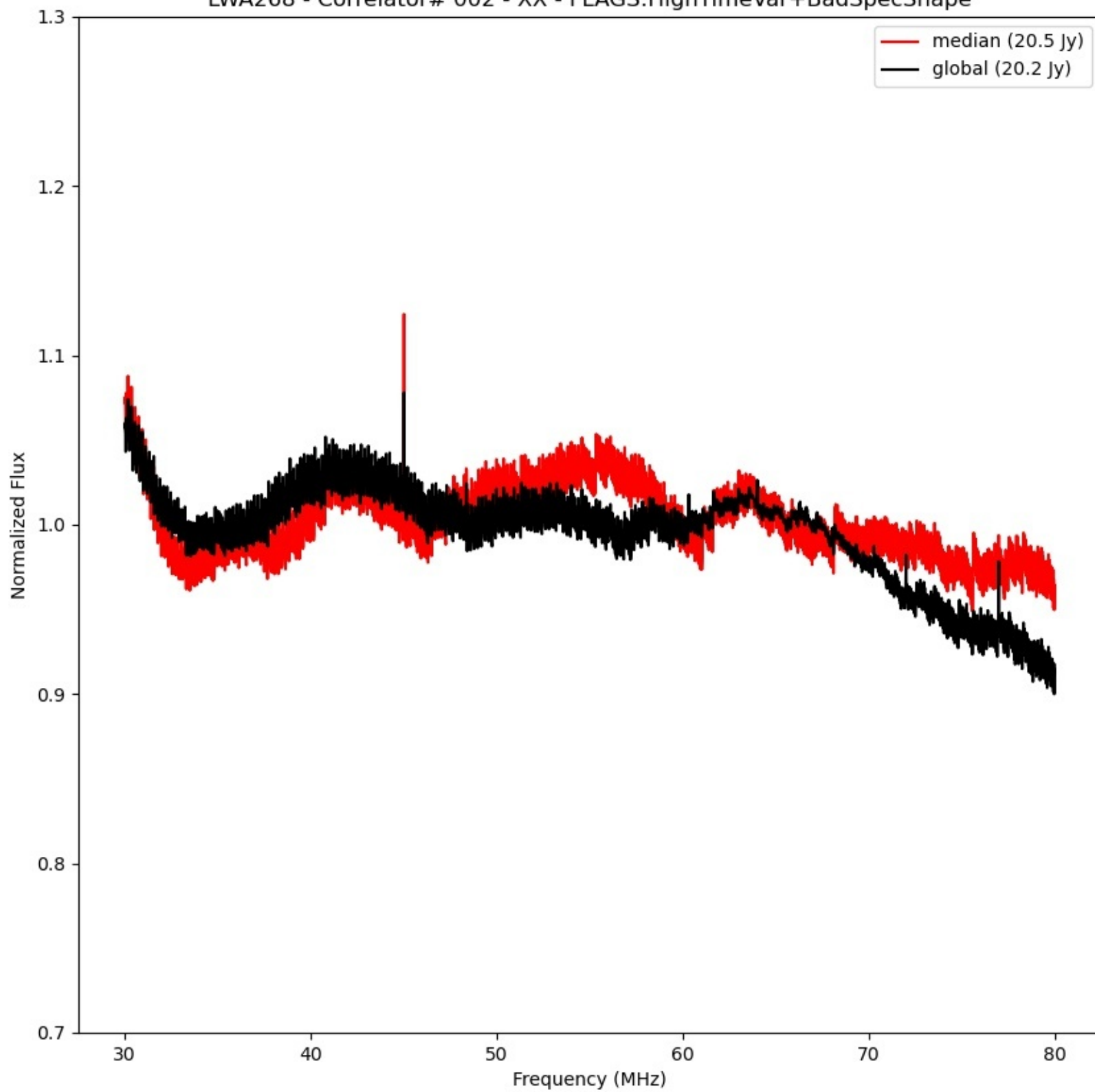
LWA268 - Correlator# 002 - XX - FLAGS:HighTimeVar+BadSpecShape
