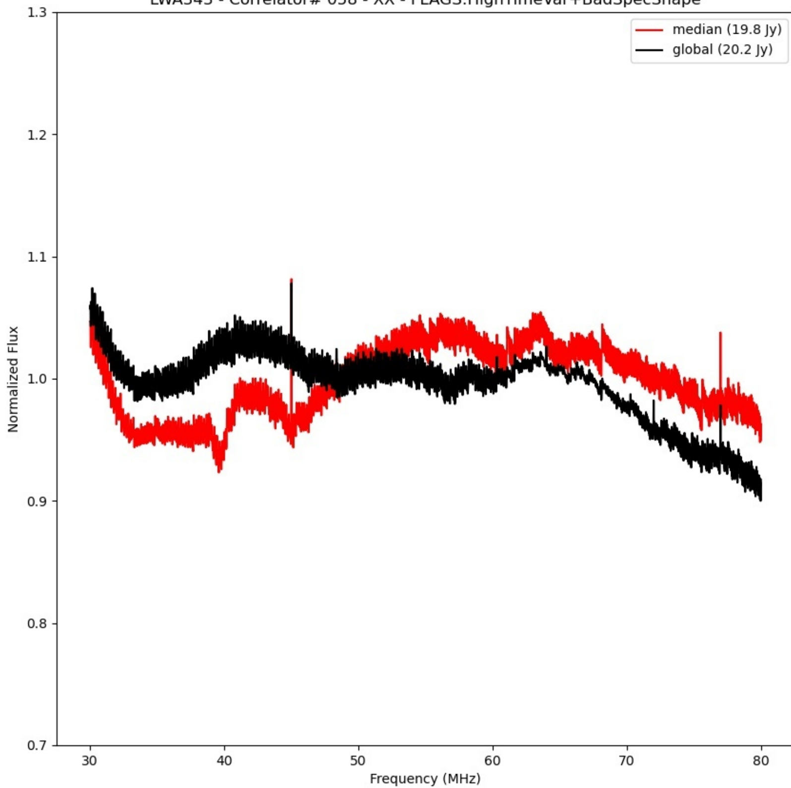
LWA343 - Correlator# 058 - XX - FLAGS:HighTimeVar+BadSpecShape
