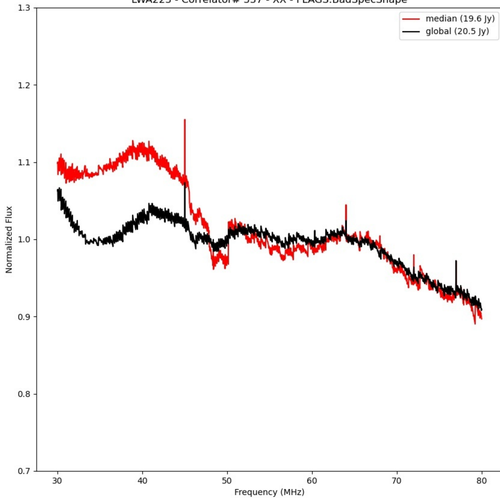
LWA223 - Correlator# 337 - XX - FLAGS:BadSpecShape
