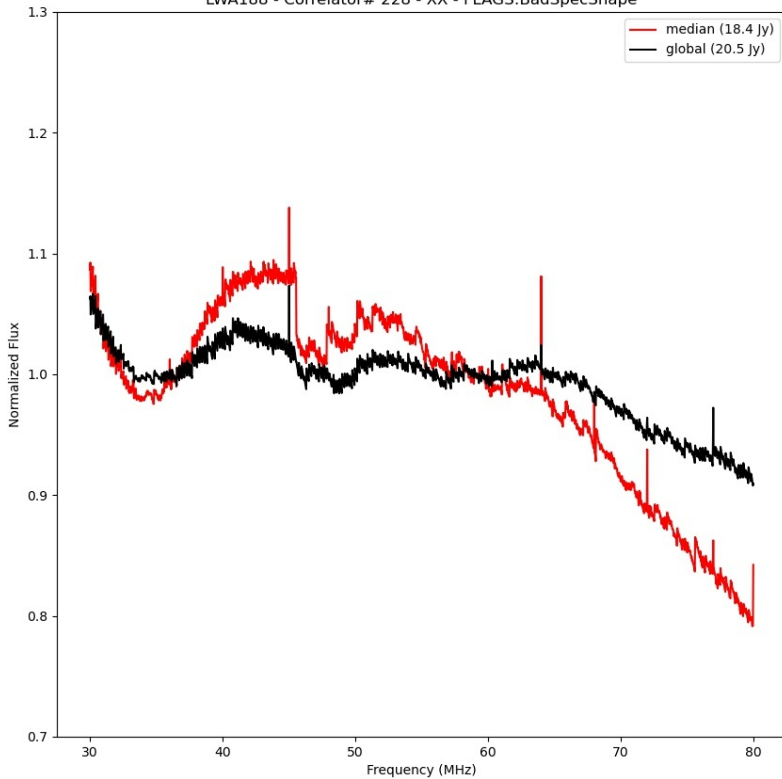
LWA188 - Correlator# 228 - XX - FLAGS:BadSpecShape
