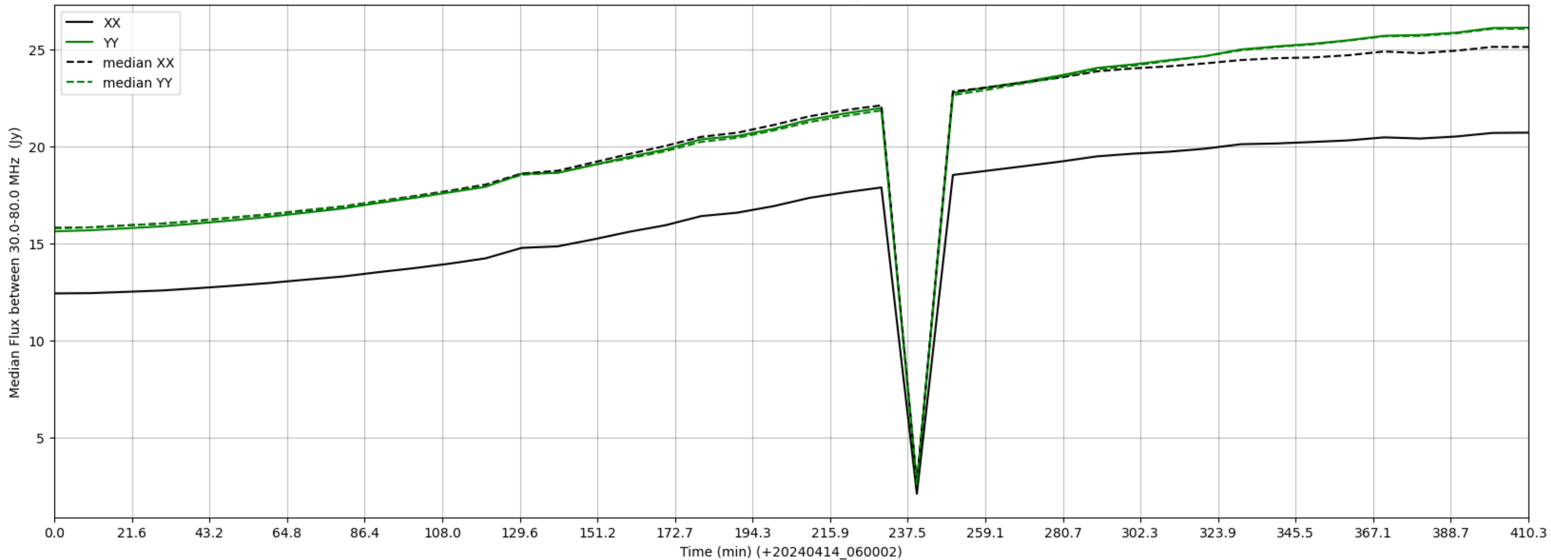
LWA215 - Correlator# 331 - XX FLAGS:BadSpecShape - YY FLAGS:Good
