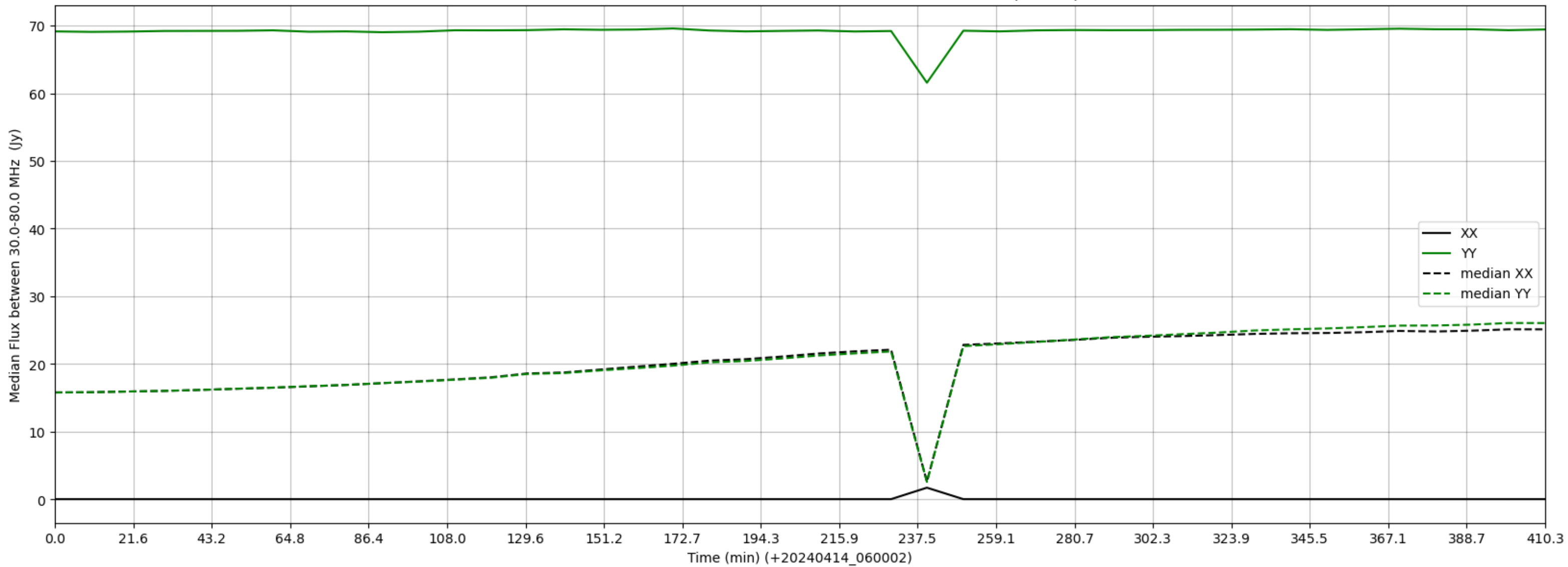
LWA280 - Correlator# 041 - XX FLAGS:LowFlux - YY FLAGS:BadSpecShape
