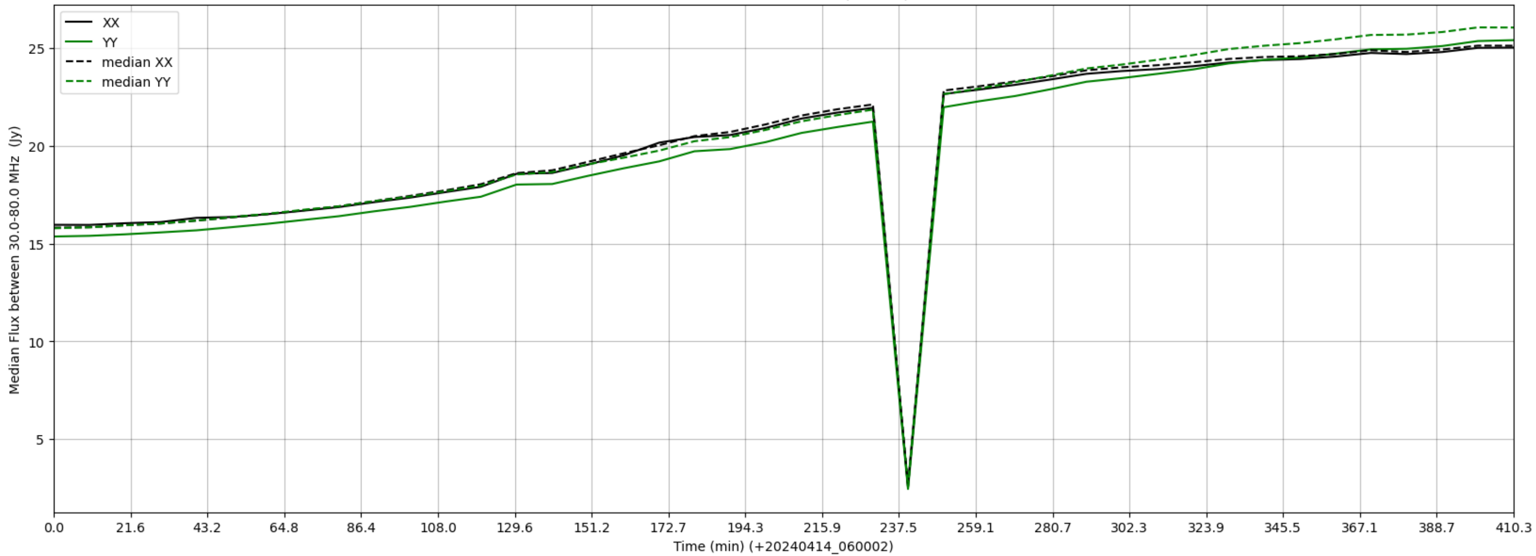
LWA004 - Correlator# 066 - XX FLAGS:BadSpecShape - YY FLAGS:Good
