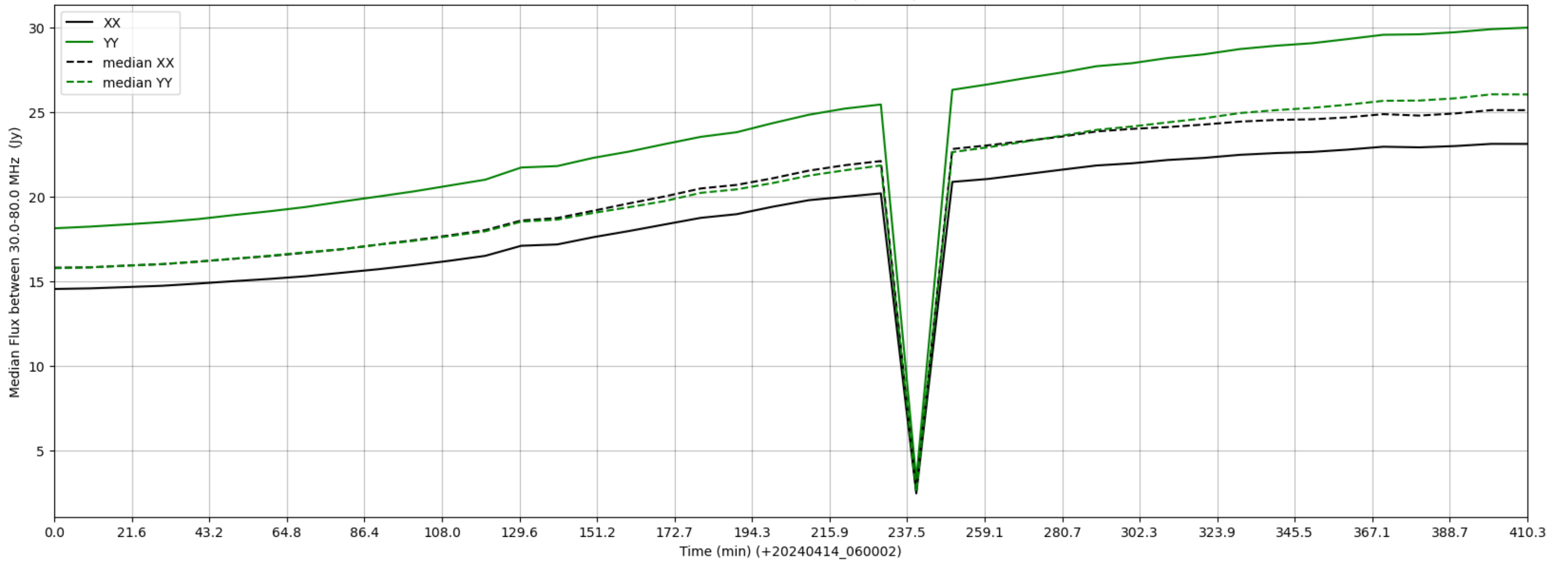
LWA364 - Correlator# 127 - XX FLAGS:BadSpecShape - YY FLAGS:Good
