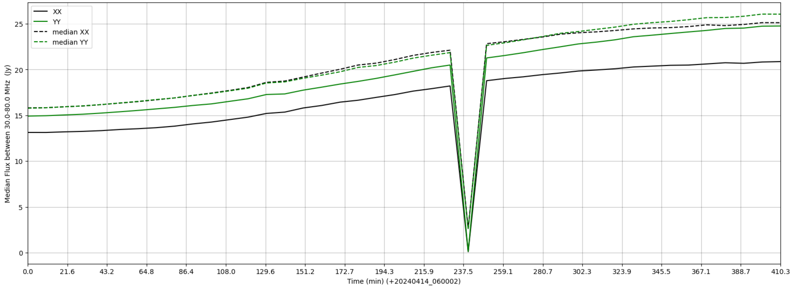
LWA340 - Correlator# 026 - XX FLAGS:BadSpecShape - YY FLAGS:Good
