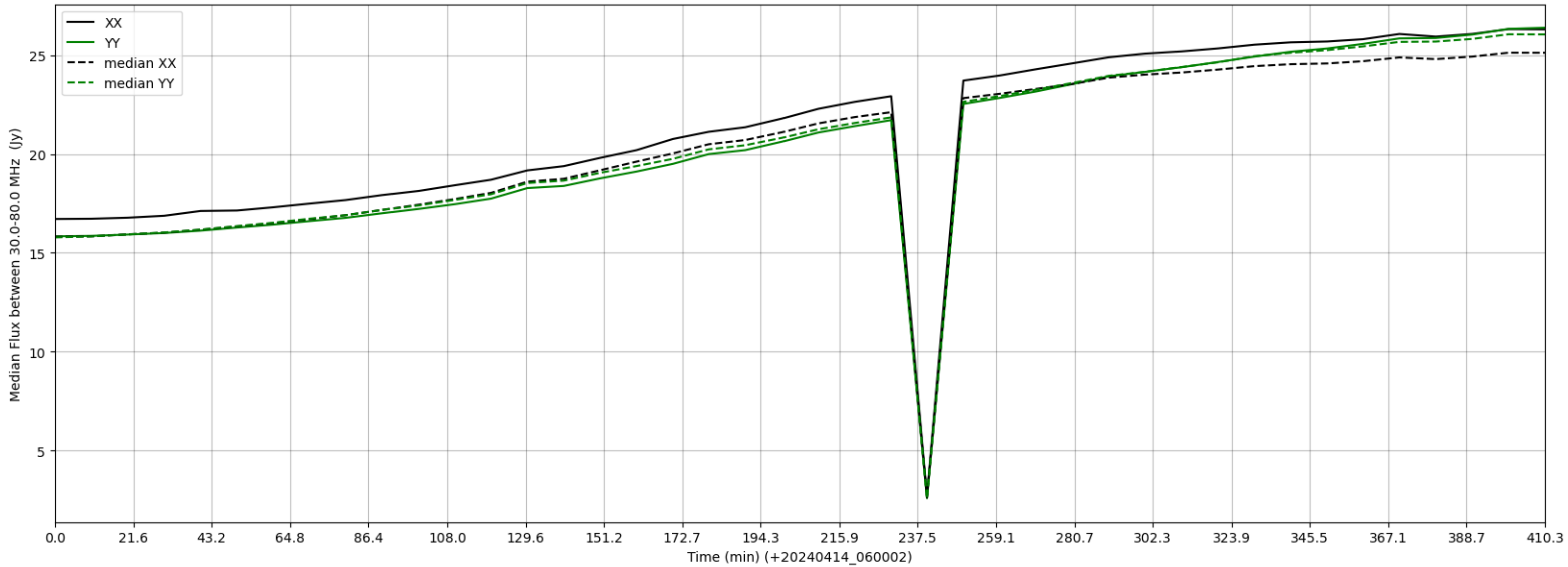
LWA002 - Correlator# 064 - XX FLAGS:BadSpecShape - YY FLAGS:Good
