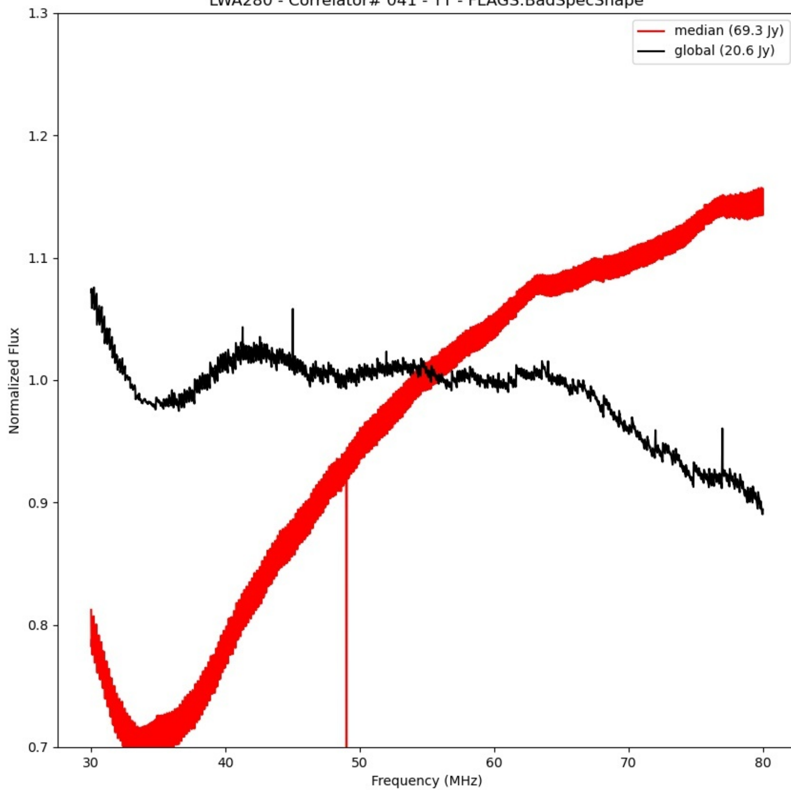
LWA280 - Correlator# 041 - YY - FLAGS:BadSpecShape
