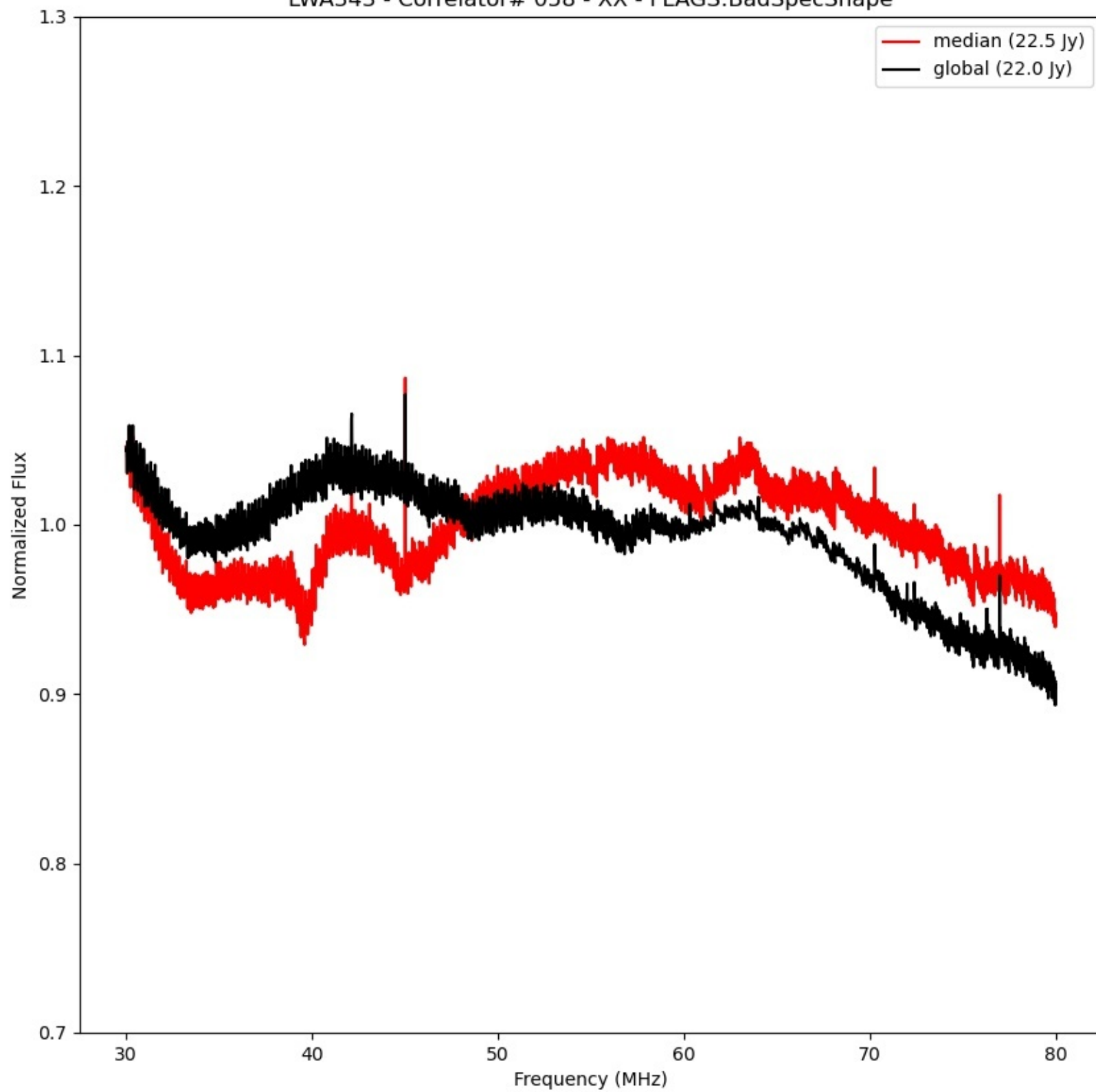
LWA343 - Correlator# 058 - XX - FLAGS:BadSpecShape
