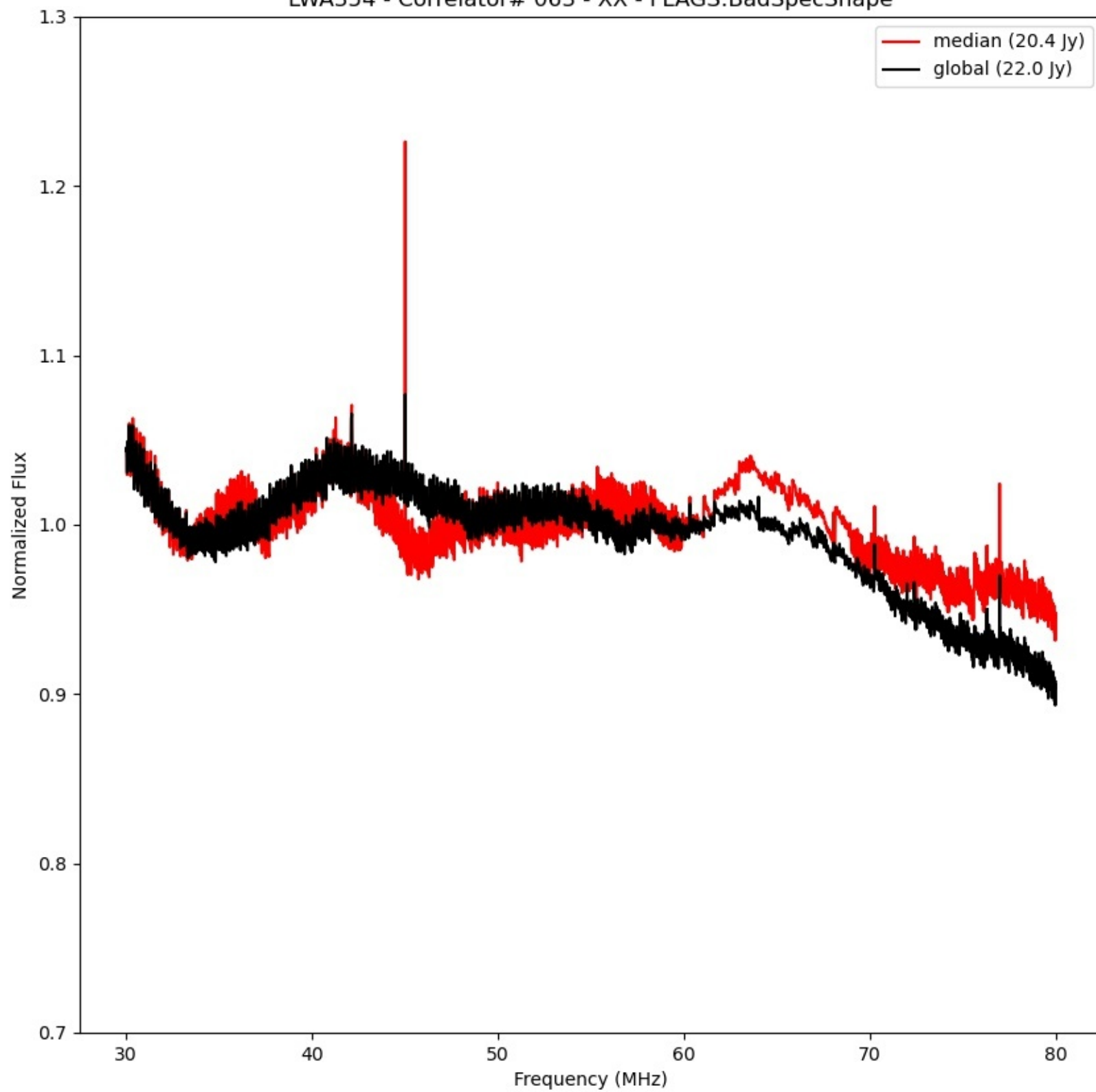
LWA354 - Correlator# 063 - XX - FLAGS:BadSpecShape
