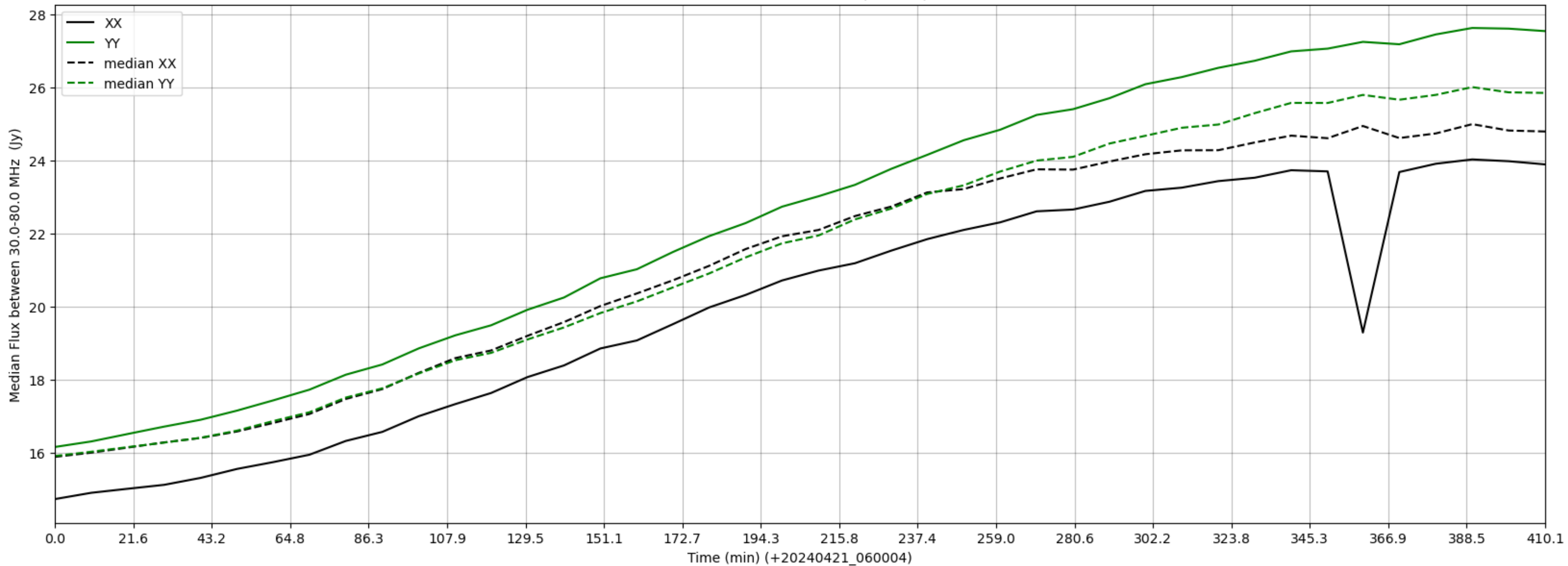
LWA278 - Correlator# 008 - XX FLAGS:BadSpecShape - YY FLAGS:Good
