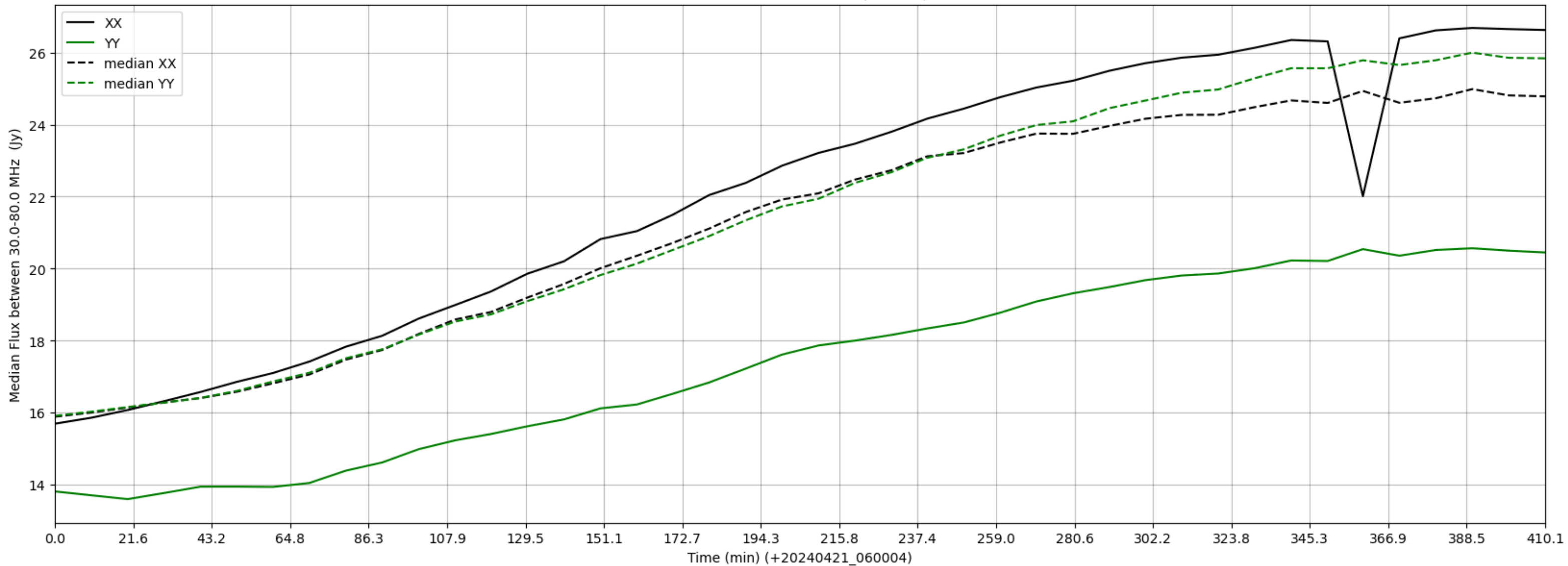
LWA271 - Correlator# 004 - XX FLAGS:BadSpecShape - YY FLAGS:Good
