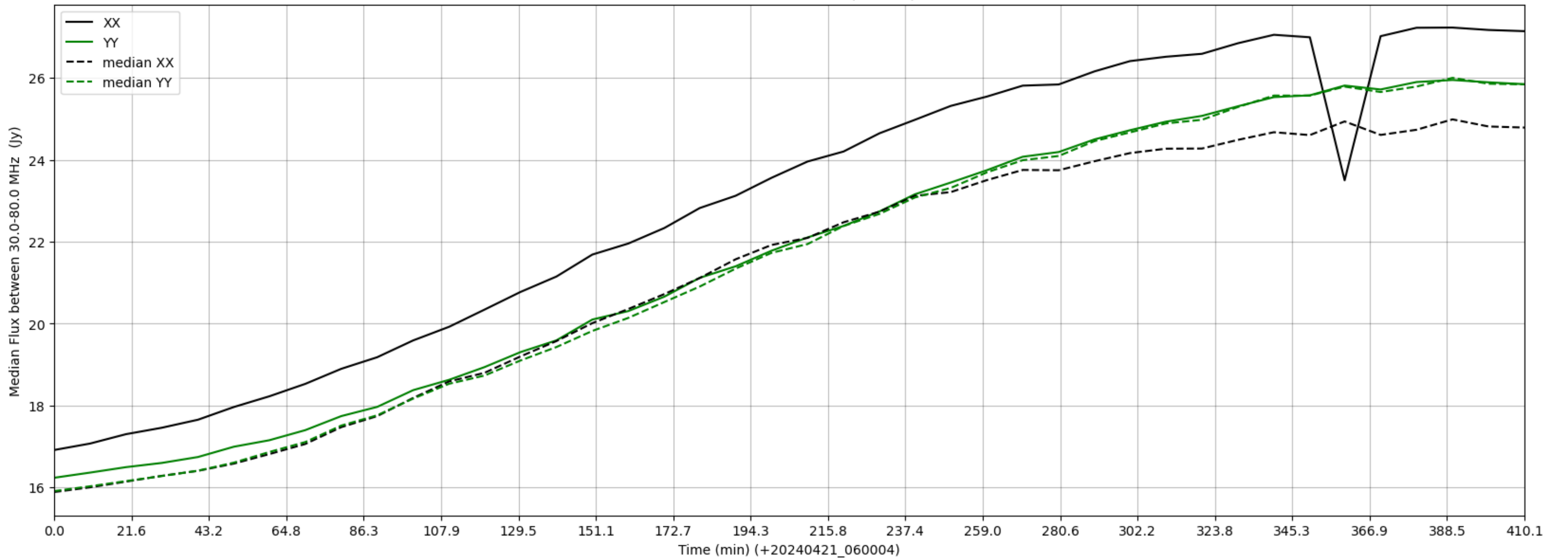
LWA327 - Correlator# 023 - XX FLAGS:BadSpecShape - YY FLAGS:Good
