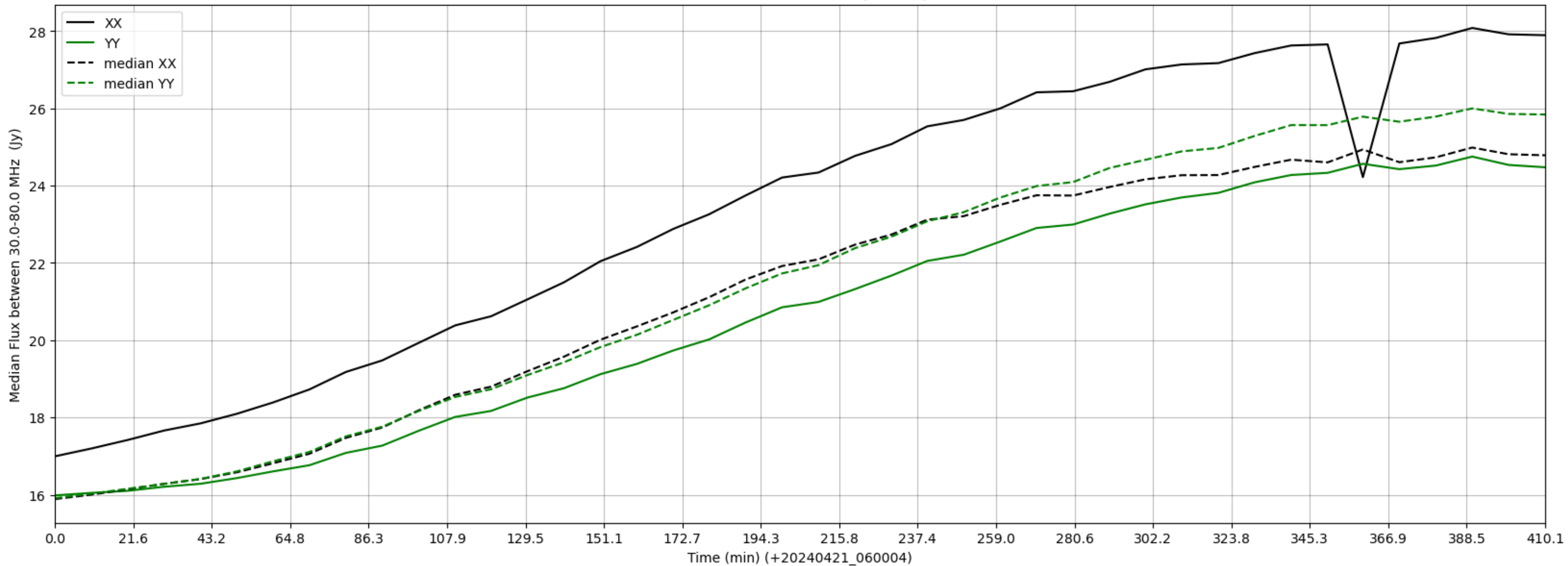
LWA304 - Correlator# 351 - XX FLAGS:BadSpecShape - YY FLAGS:Good
