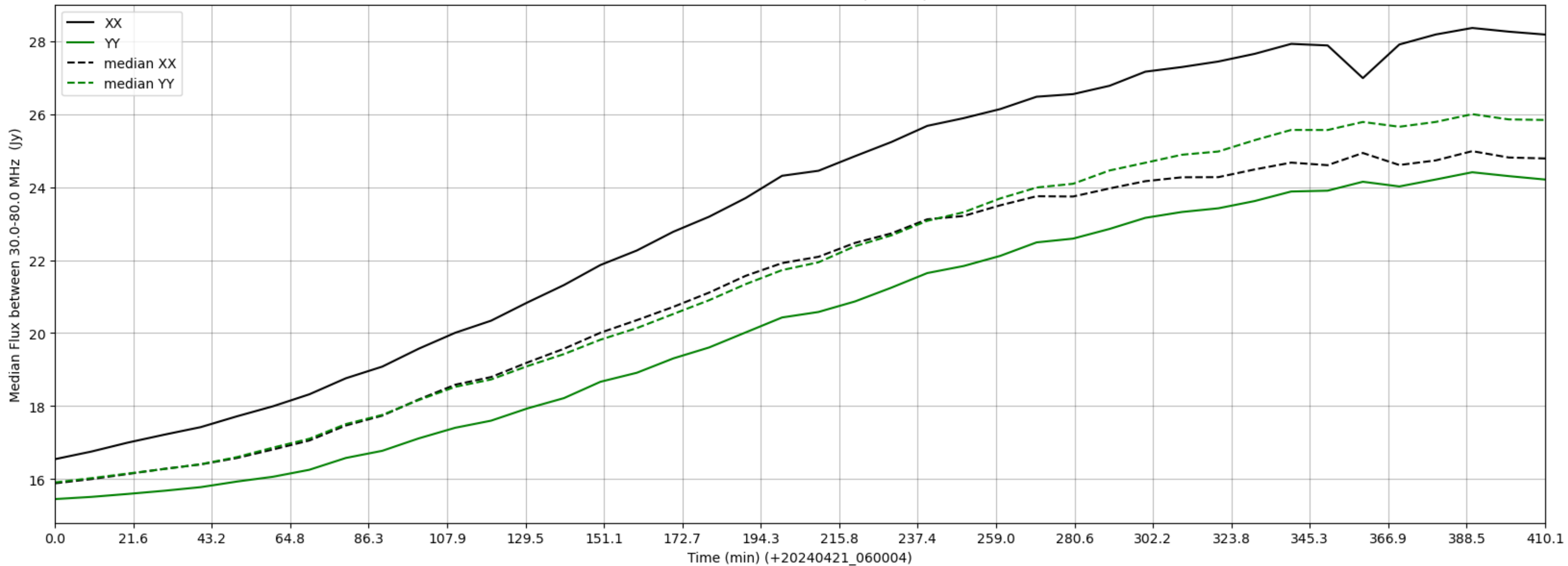
LWA306 - Correlator# 053 - XX FLAGS:BadSpecShape - YY FLAGS:Good
