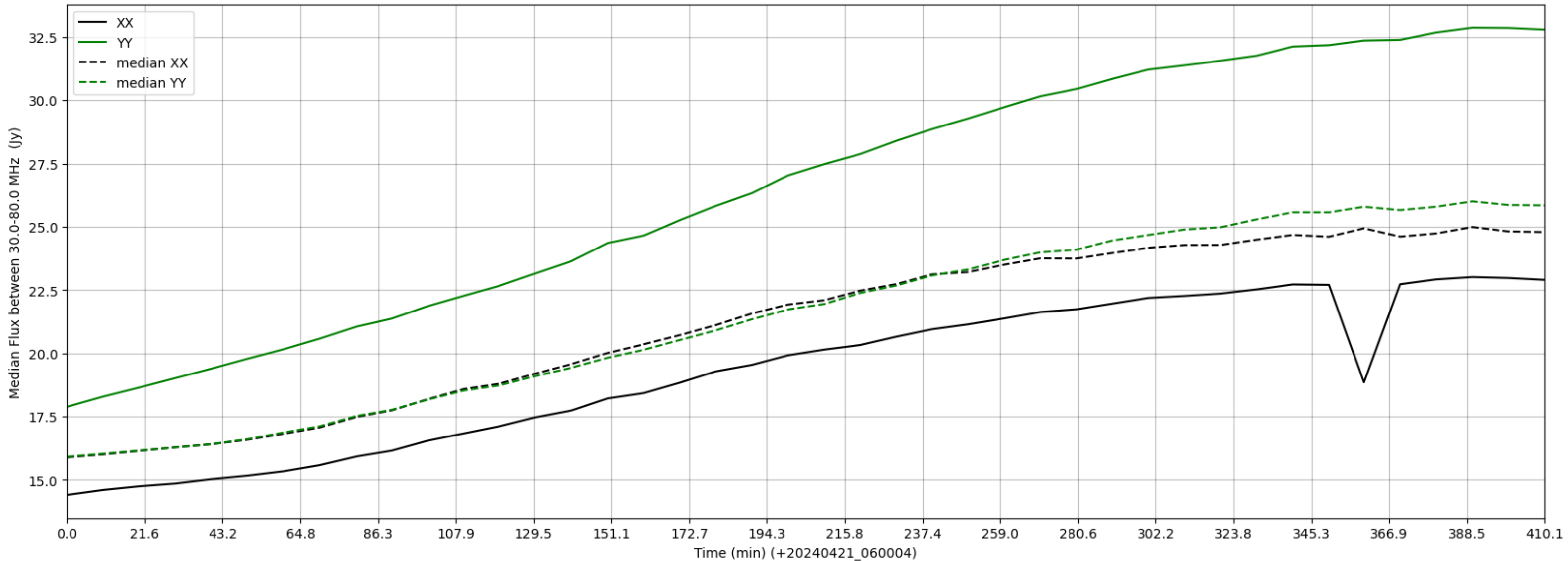
LWA331 - Correlator# 125 - XX FLAGS:BadSpecShape - YY FLAGS:Good
