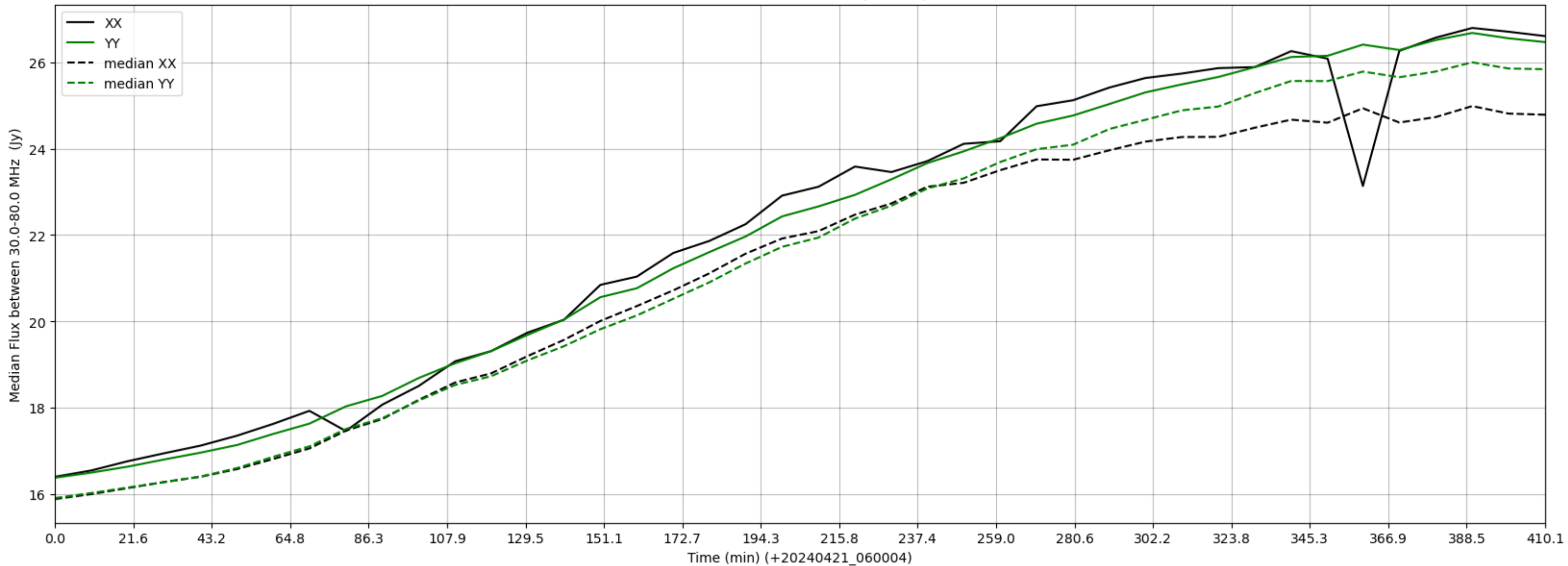
LWA261 - Correlator# 346 - XX FLAGS:BadSpecShape - YY FLAGS:Good
