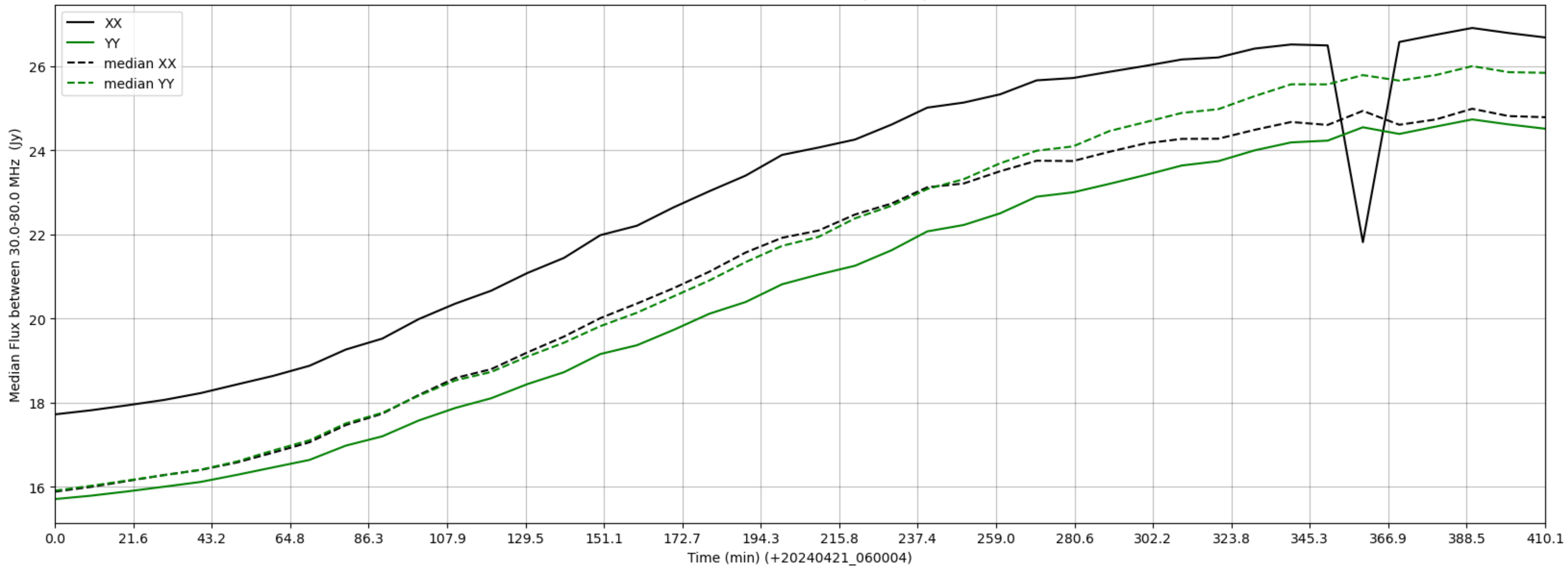
LWA268 - Correlator# 002 - XX FLAGS:BadSpecShape - YY FLAGS:Good
