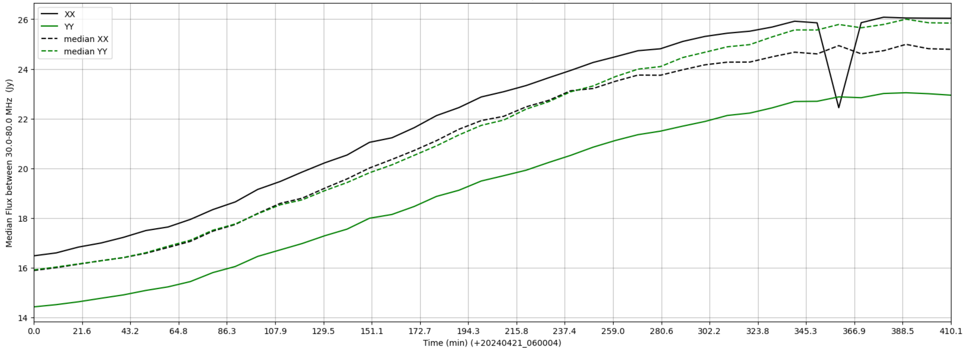
LWA321 - Correlator# 020 - XX FLAGS:BadSpecShape - YY FLAGS:Good
