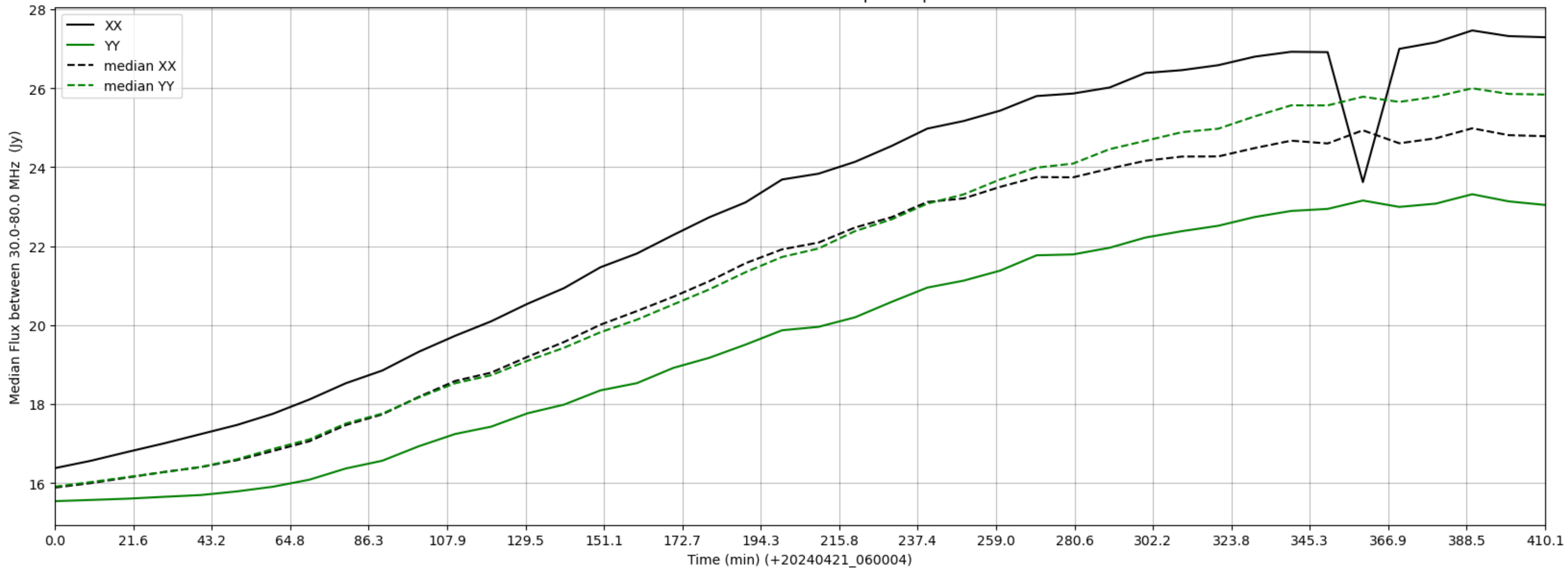
LWA269 - Correlator# 005 - XX FLAGS:BadSpecShape - YY FLAGS:Good
