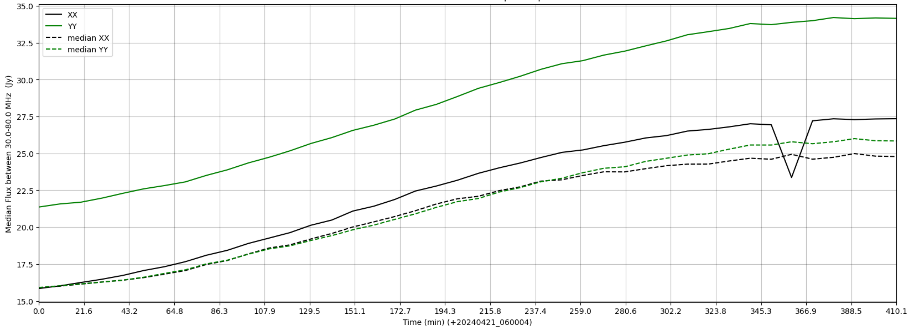
LWA322 - Correlator# 251 - XX FLAGS:BadSpecShape - YY FLAGS:Good
