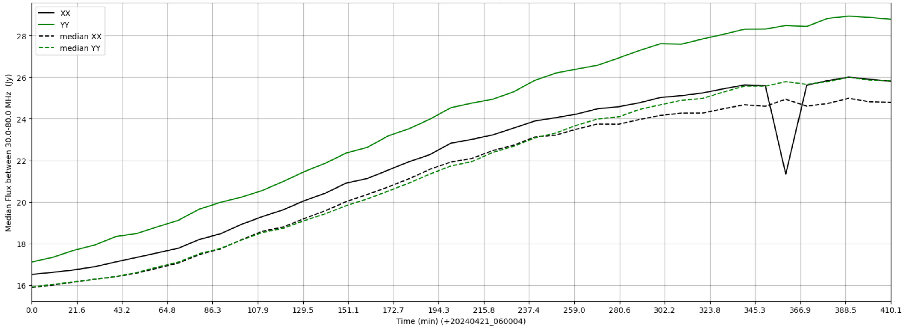
LWA282 - Correlator# 010 - XX FLAGS:BadSpecShape - YY FLAGS:Good
