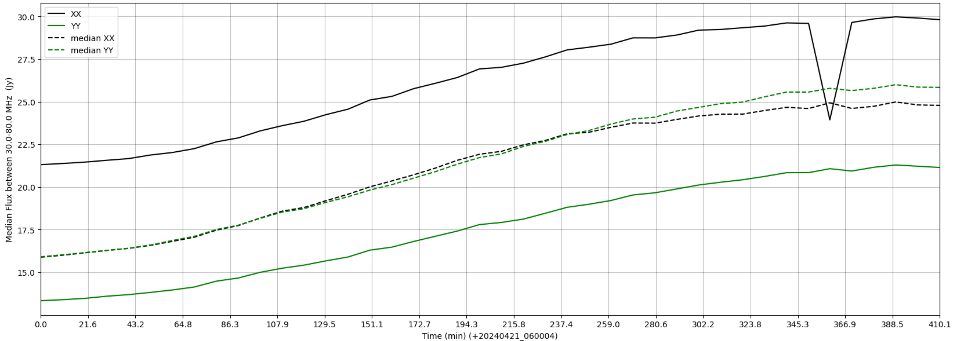
LWA295 - Correlator# 047 - XX FLAGS:BadSpecShape - YY FLAGS:Good
