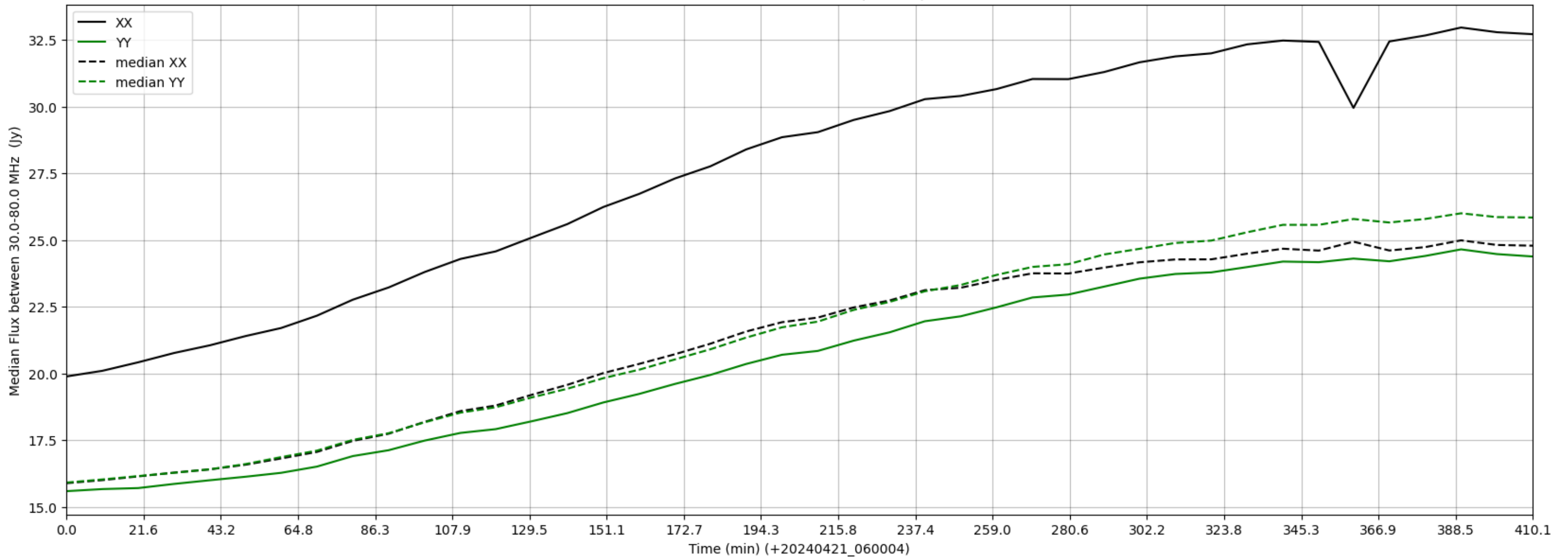
LWA301 - Correlator# 048 - XX FLAGS:BadSpecShape - YY FLAGS:Good
