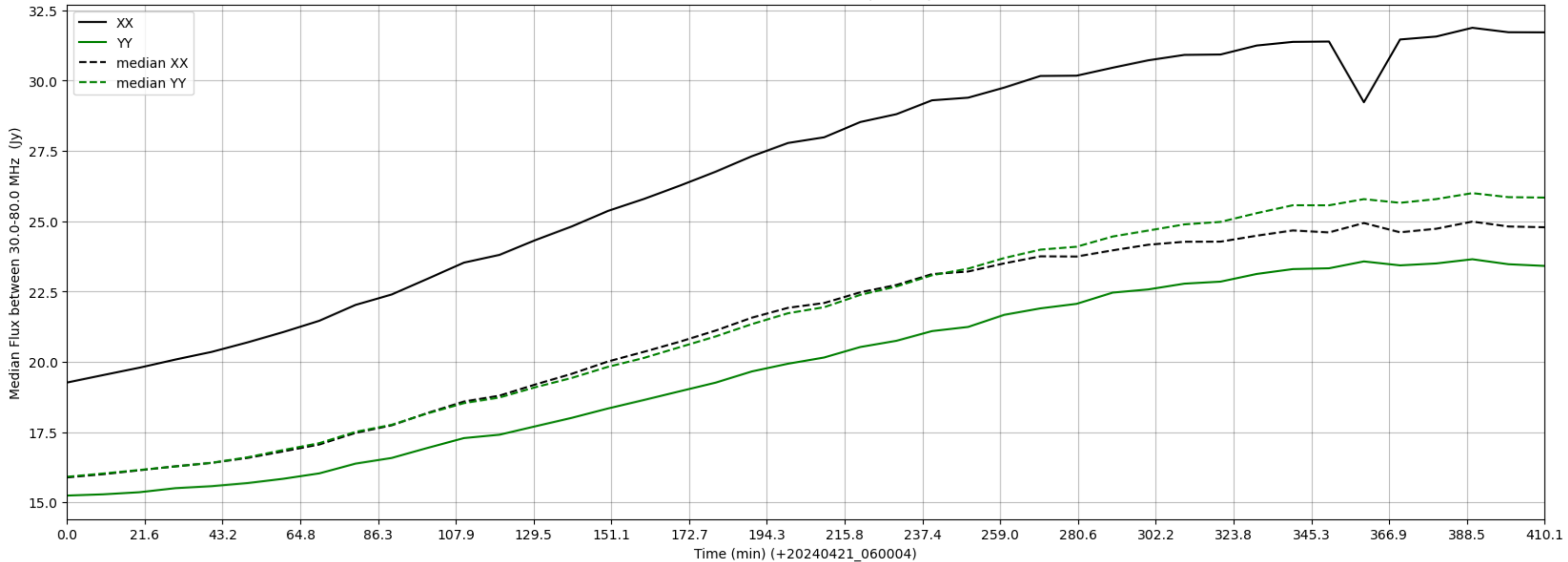
LWA345 - Correlator# 252 - XX FLAGS:BadSpecShape - YY FLAGS:Good
