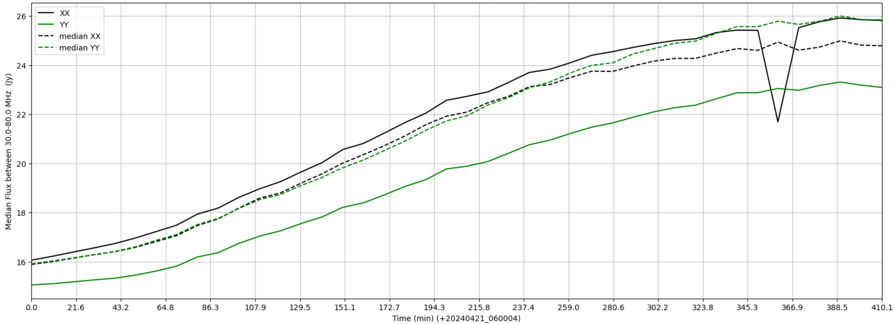
LWA266 - Correlator# 000 - XX FLAGS:BadSpecShape - YY FLAGS:Good
