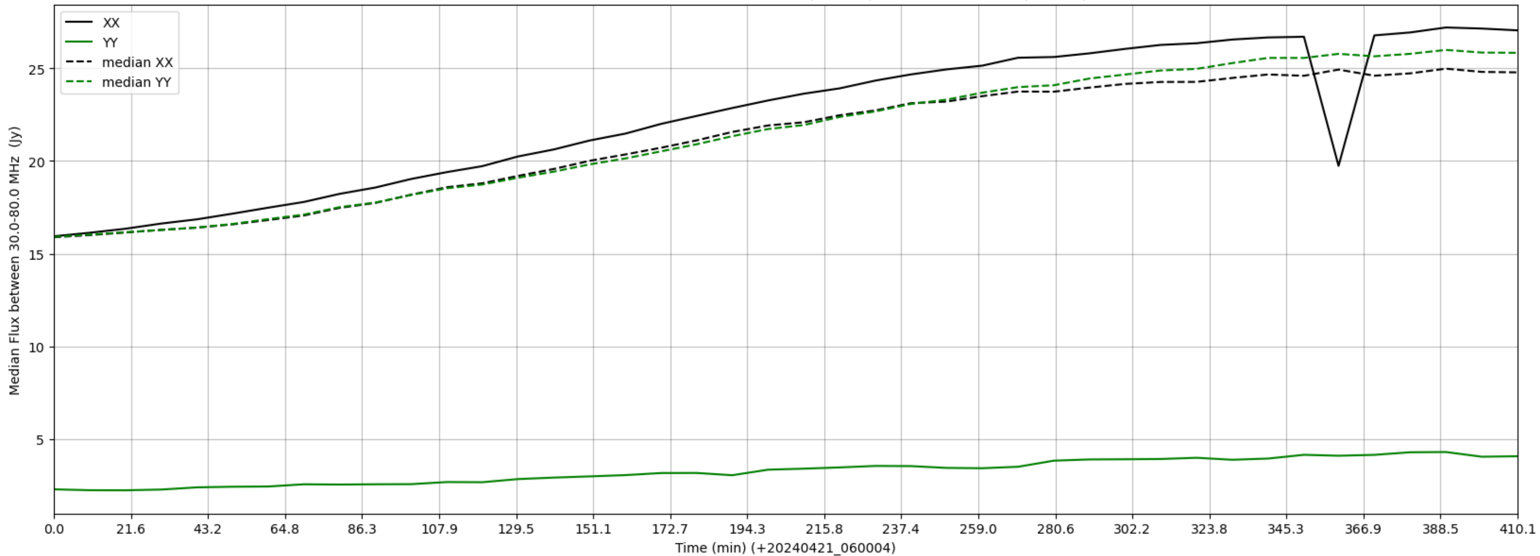
LWA307 - Correlator# 012 - XX FLAGS:BadSpecShape - YY FLAGS:BadSpecShape
