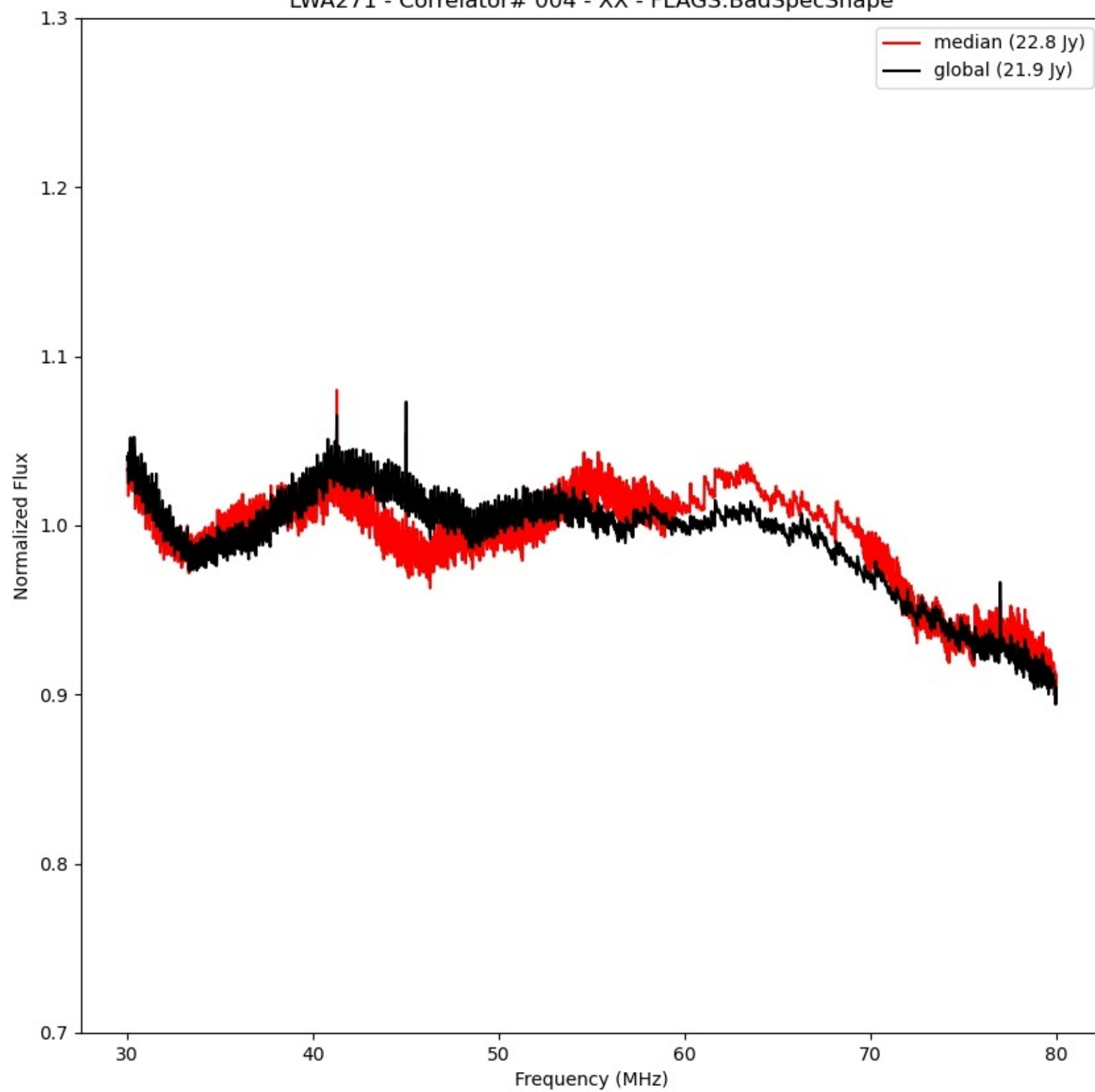
LWA271 - Correlator# 004 - XX - FLAGS:BadSpecShape
