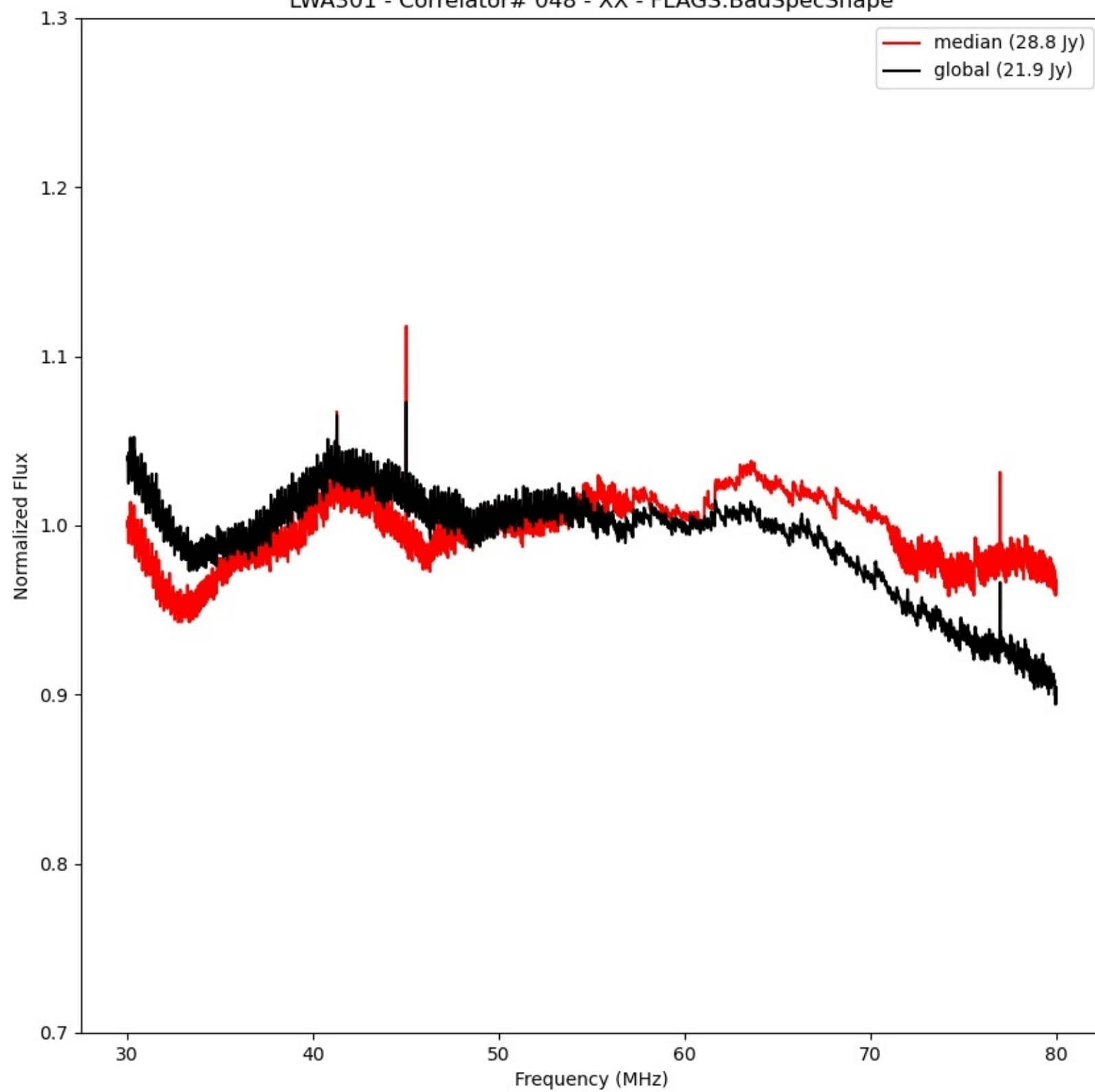
LWA301 - Correlator# 048 - XX - FLAGS:BadSpecShape
