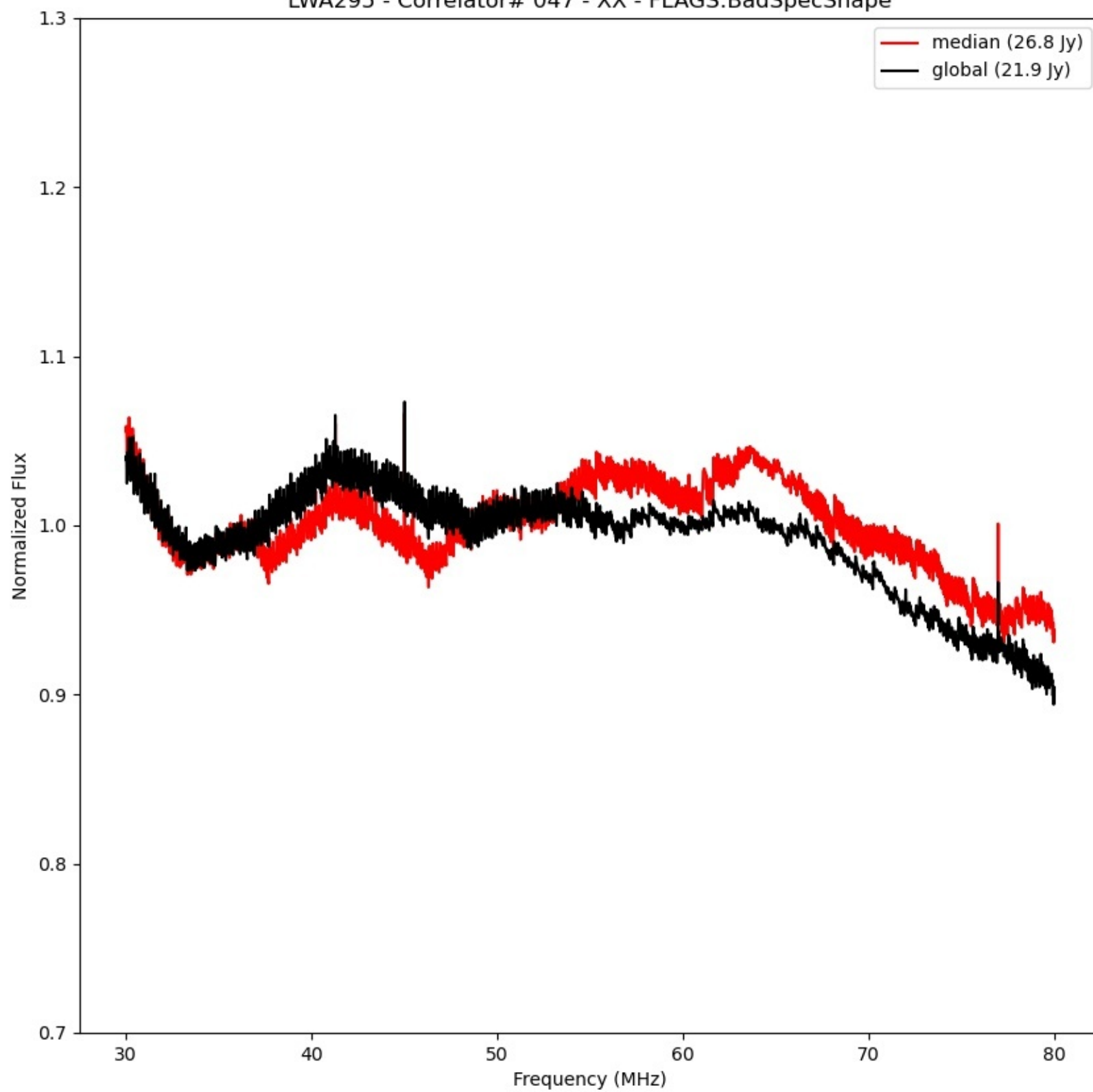
LWA295 - Correlator# 047 - XX - FLAGS:BadSpecShape
