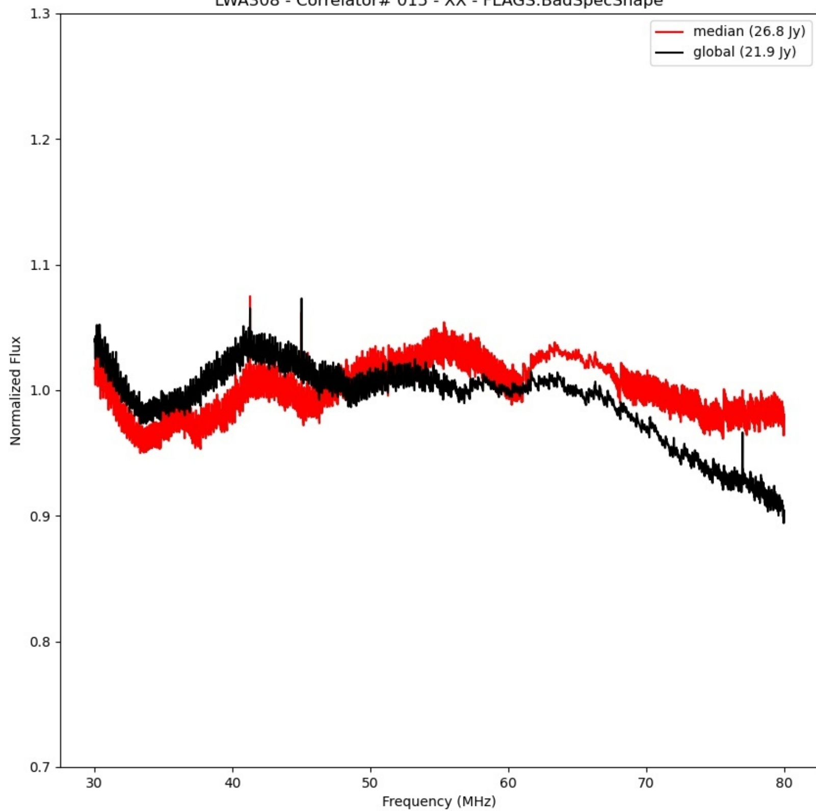
LWA308 - Correlator# 015 - XX - FLAGS:BadSpecShape
