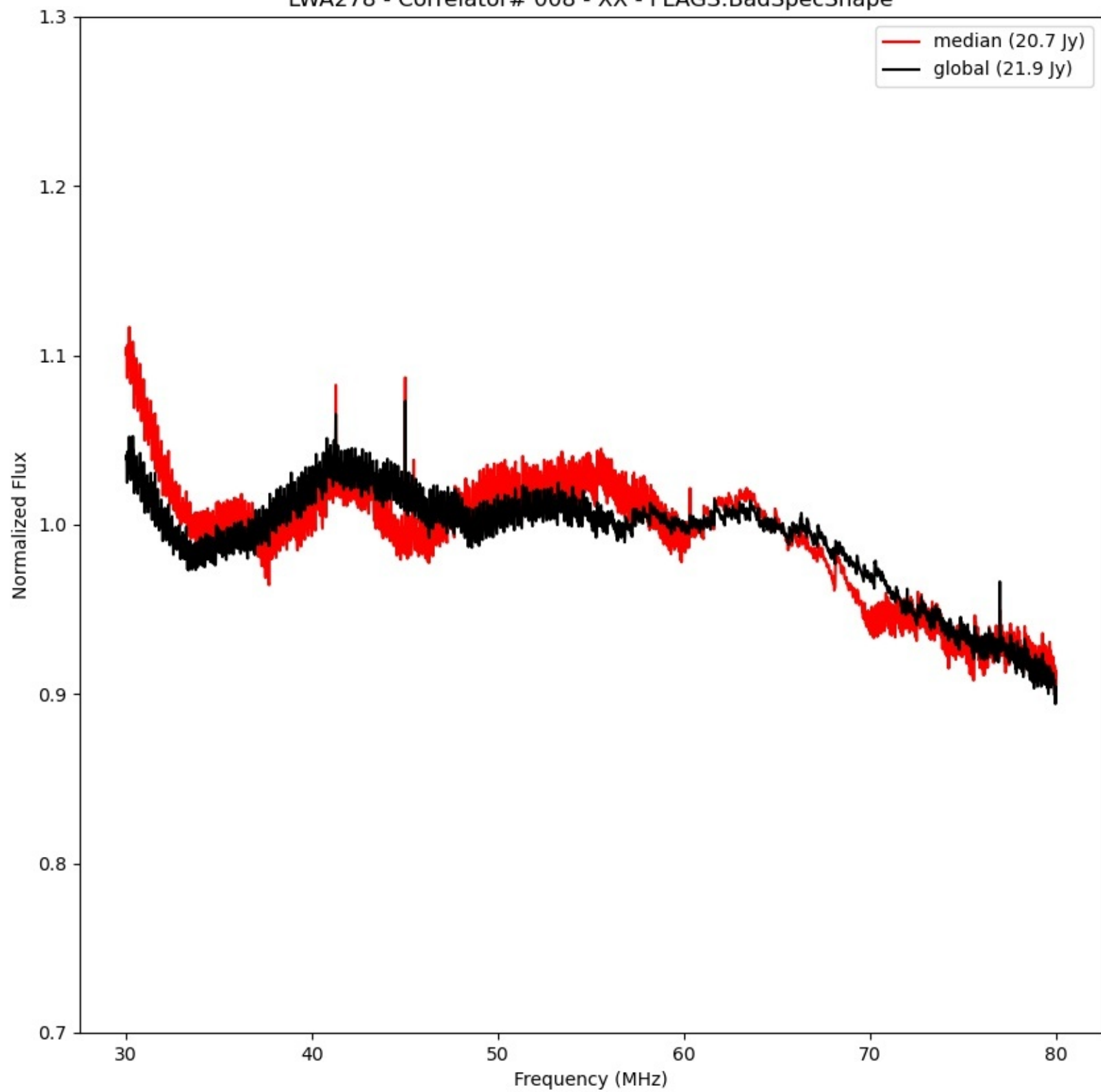
LWA278 - Correlator# 008 - XX - FLAGS:BadSpecShape
