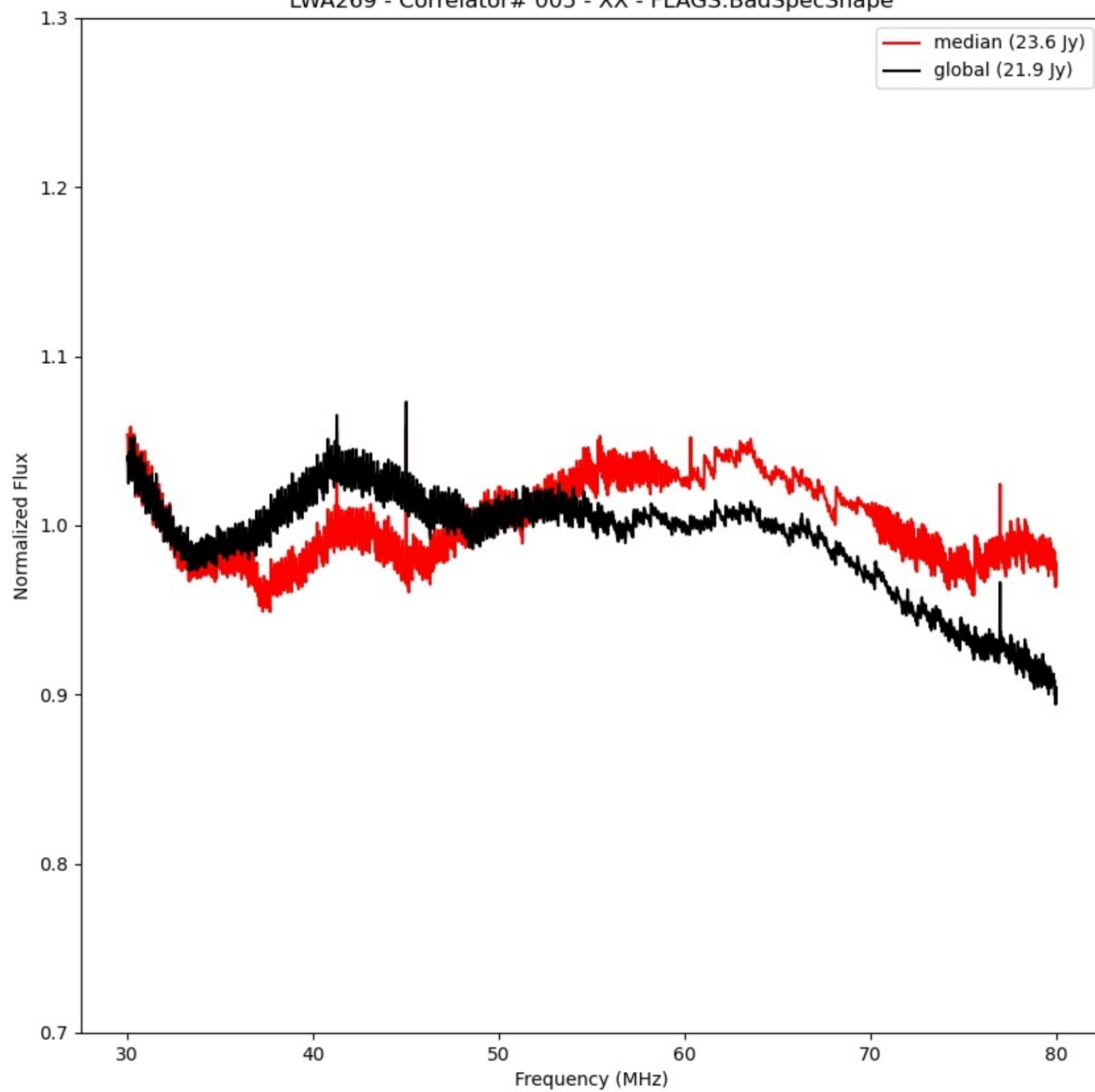
LWA269 - Correlator# 005 - XX - FLAGS:BadSpecShape
