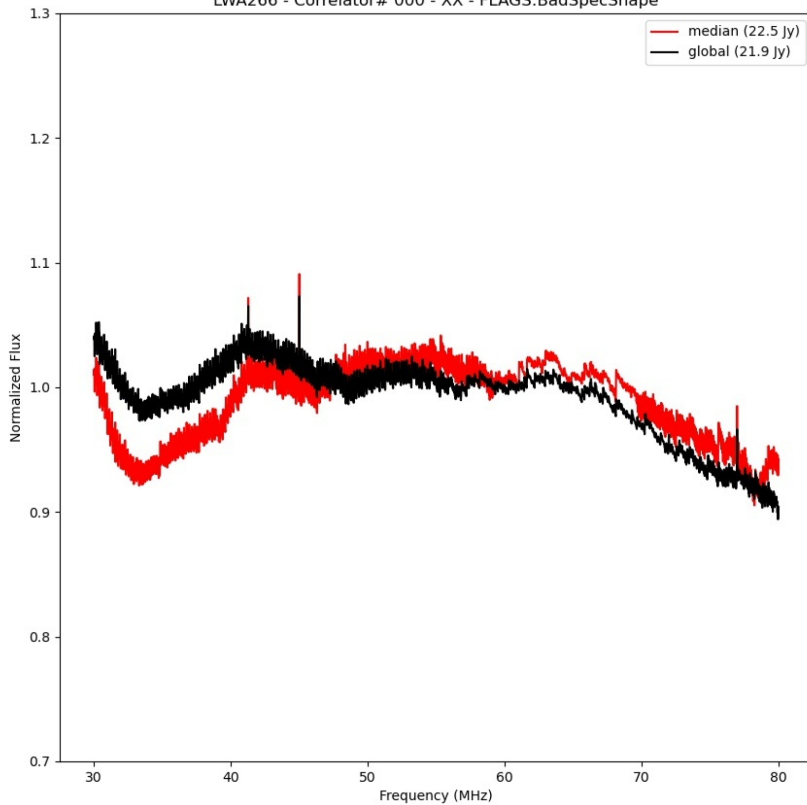
LWA266 - Correlator# 000 - XX - FLAGS:BadSpecShape
