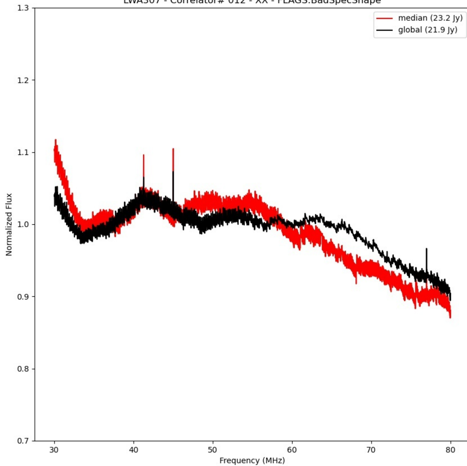
LWA307 - Correlator# 012 - XX - FLAGS:BadSpecShape
