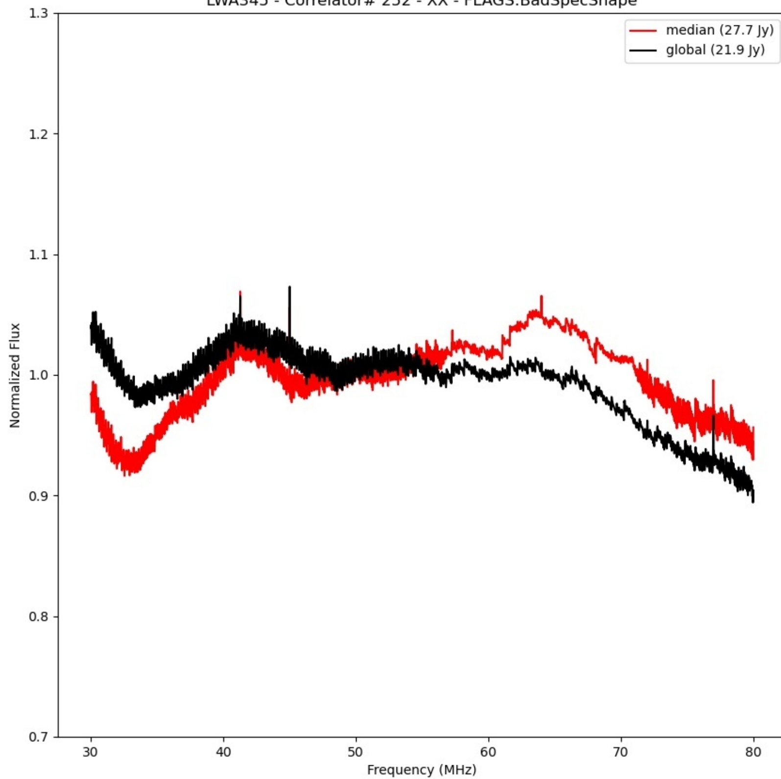
LWA345 - Correlator# 252 - XX - FLAGS:BadSpecShape
