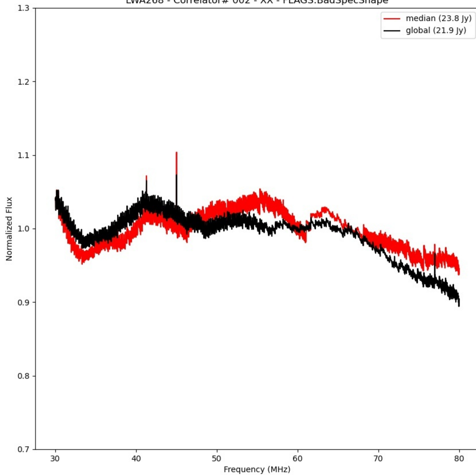
LWA268 - Correlator# 002 - XX - FLAGS:BadSpecShape
