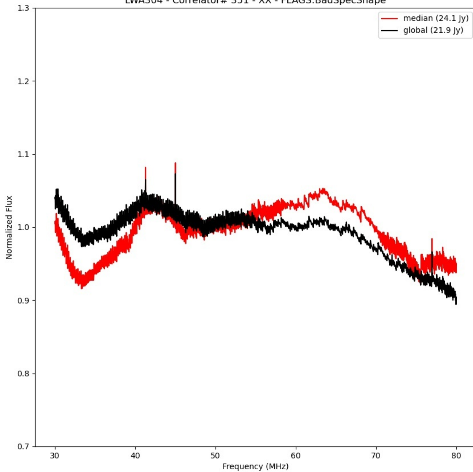
LWA304 - Correlator# 351 - XX - FLAGS:BadSpecShape
