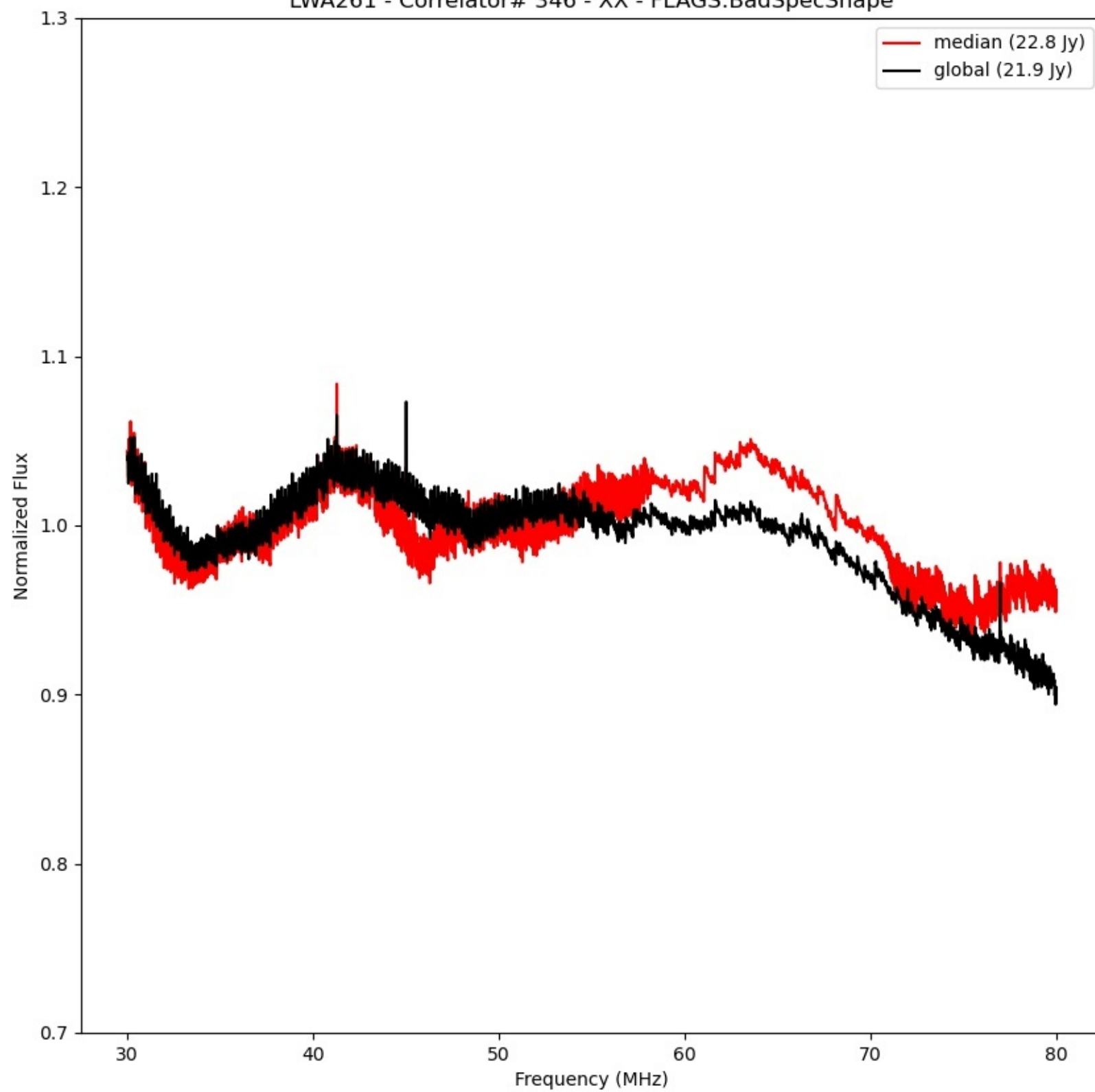
LWA261 - Correlator# 346 - XX - FLAGS:BadSpecShape
