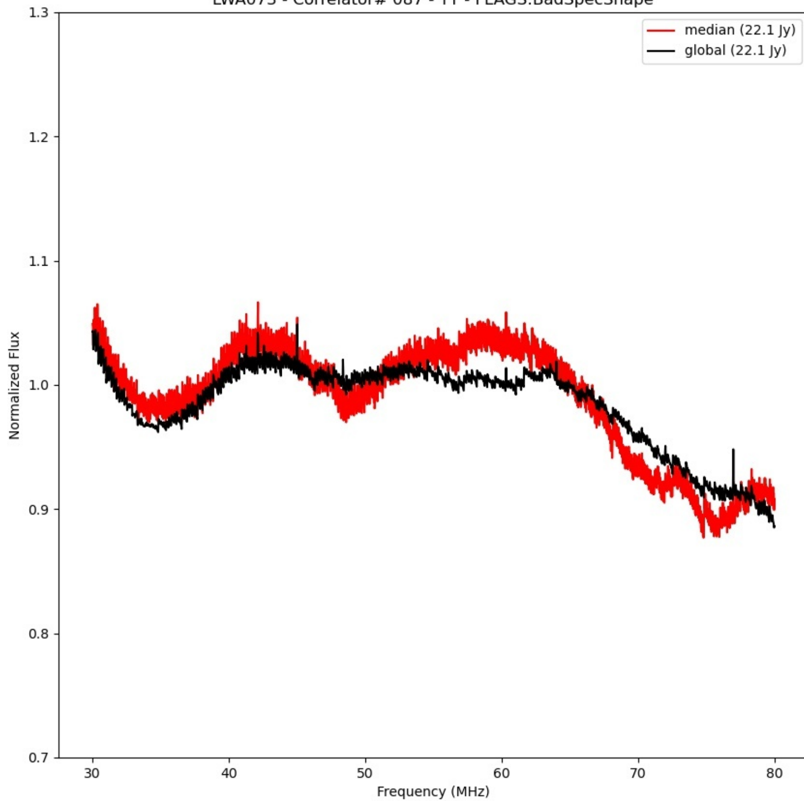
LWA073 - Correlator# 087 - YY - FLAGS:BadSpecShape
