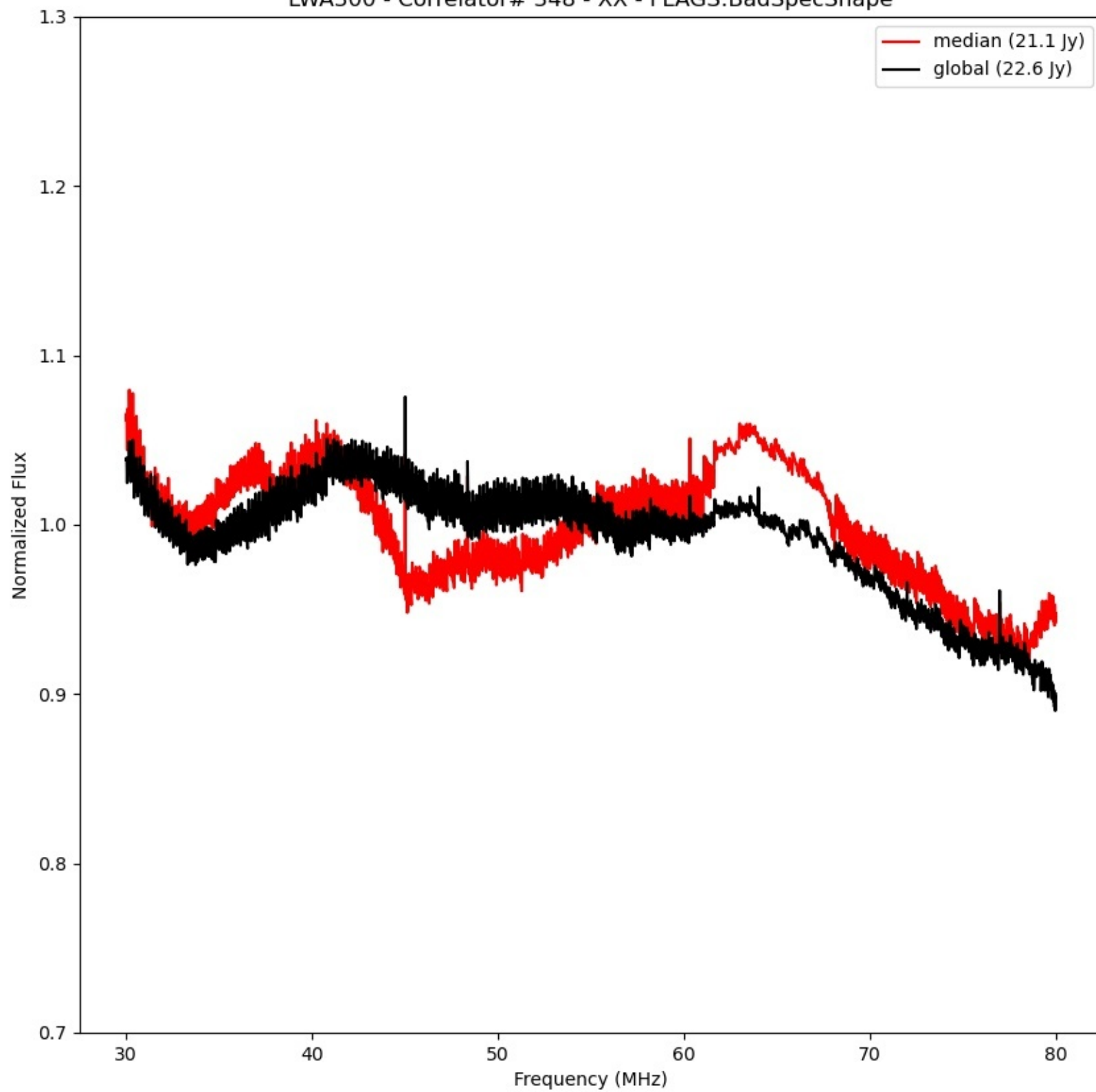
LWA300 - Correlator# 348 - XX - FLAGS:BadSpecShape
