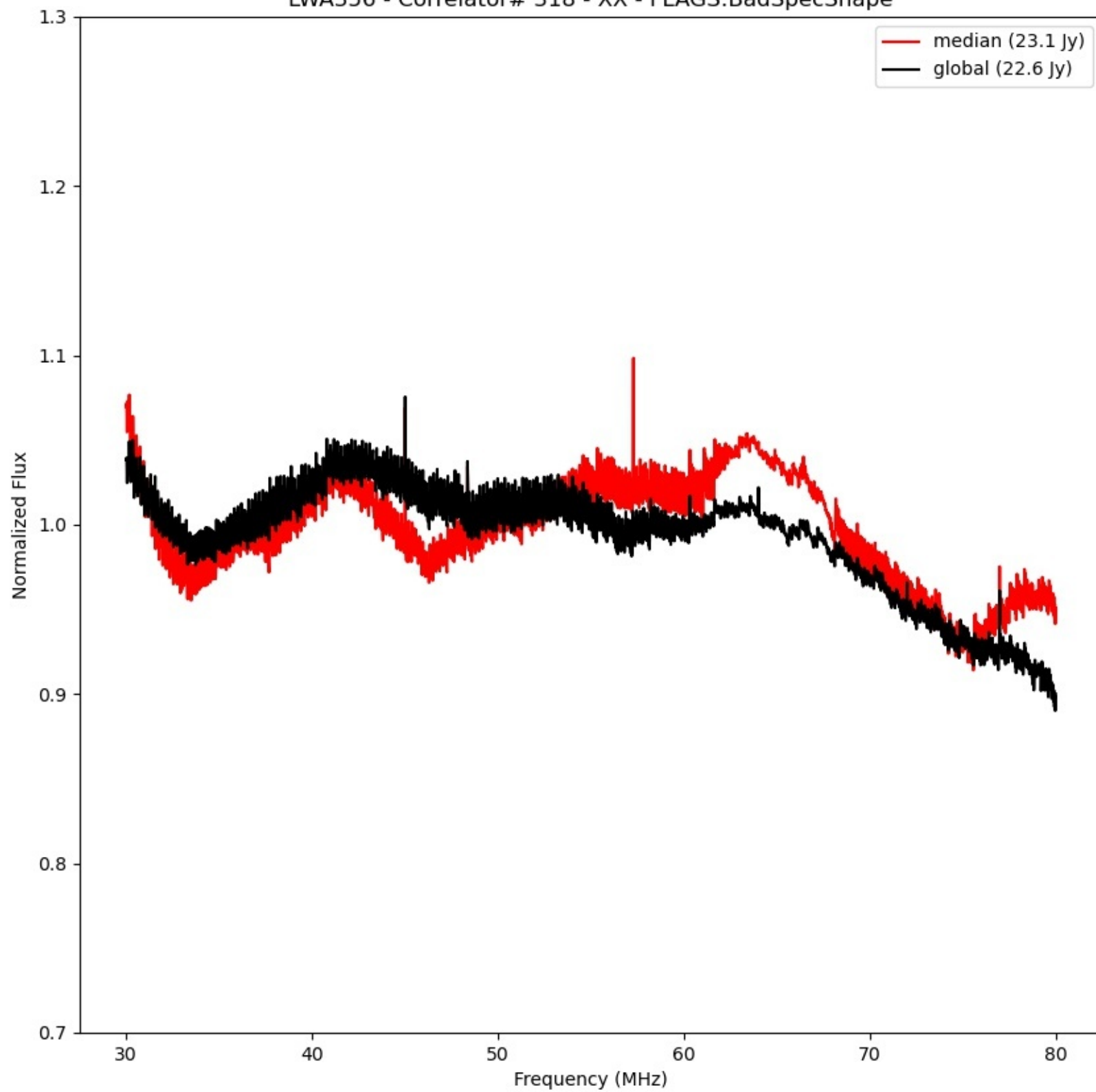
LWA356 - Correlator# 318 - XX - FLAGS:BadSpecShape
