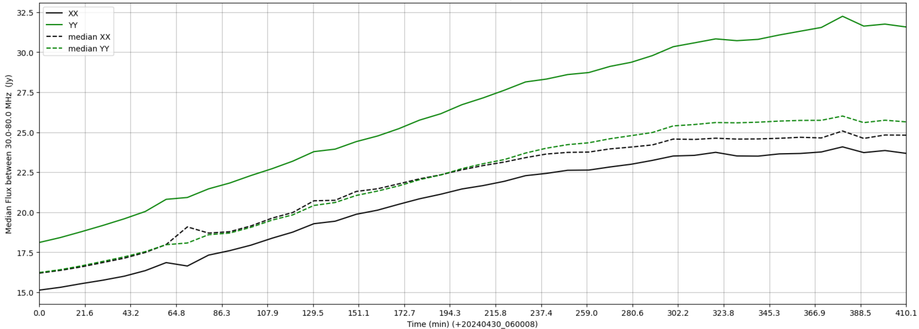
LWA316 - Correlator# 155 - XX FLAGS:BadSpecShape - YY FLAGS:Good
