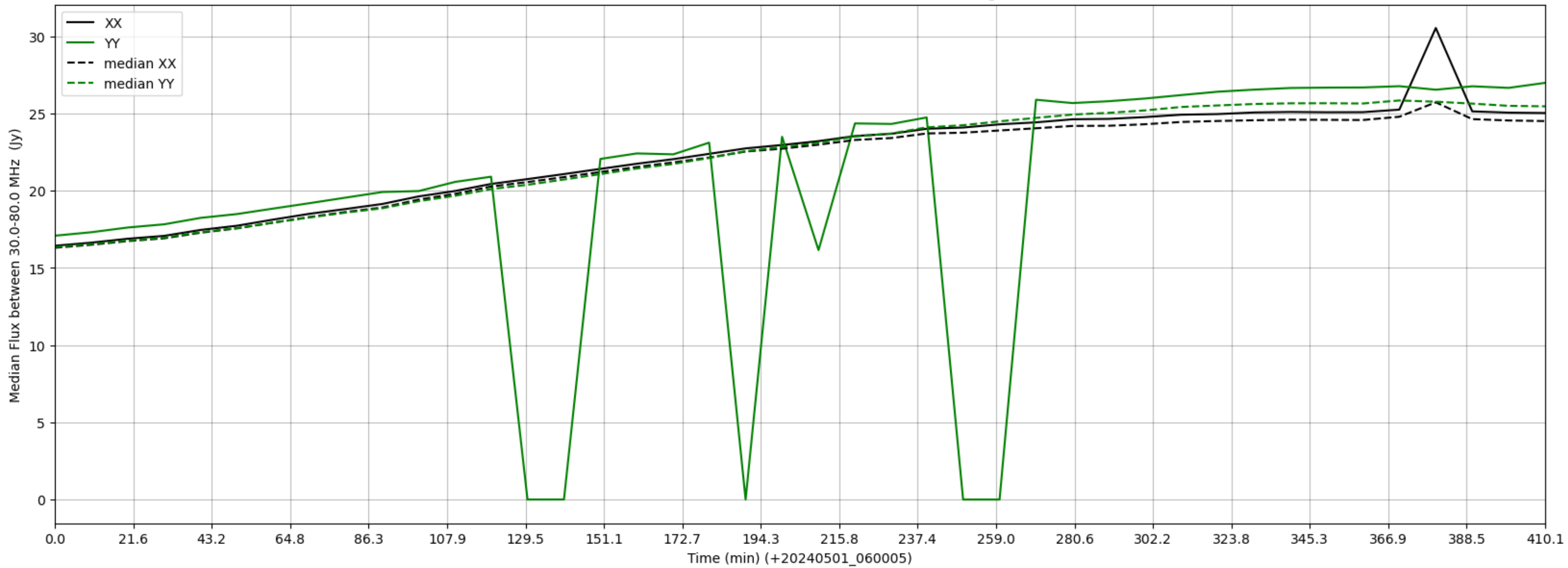
LWA205 - Correlator# 297 - XX FLAGS:Good - YY FLAGS:HighTimeVar
