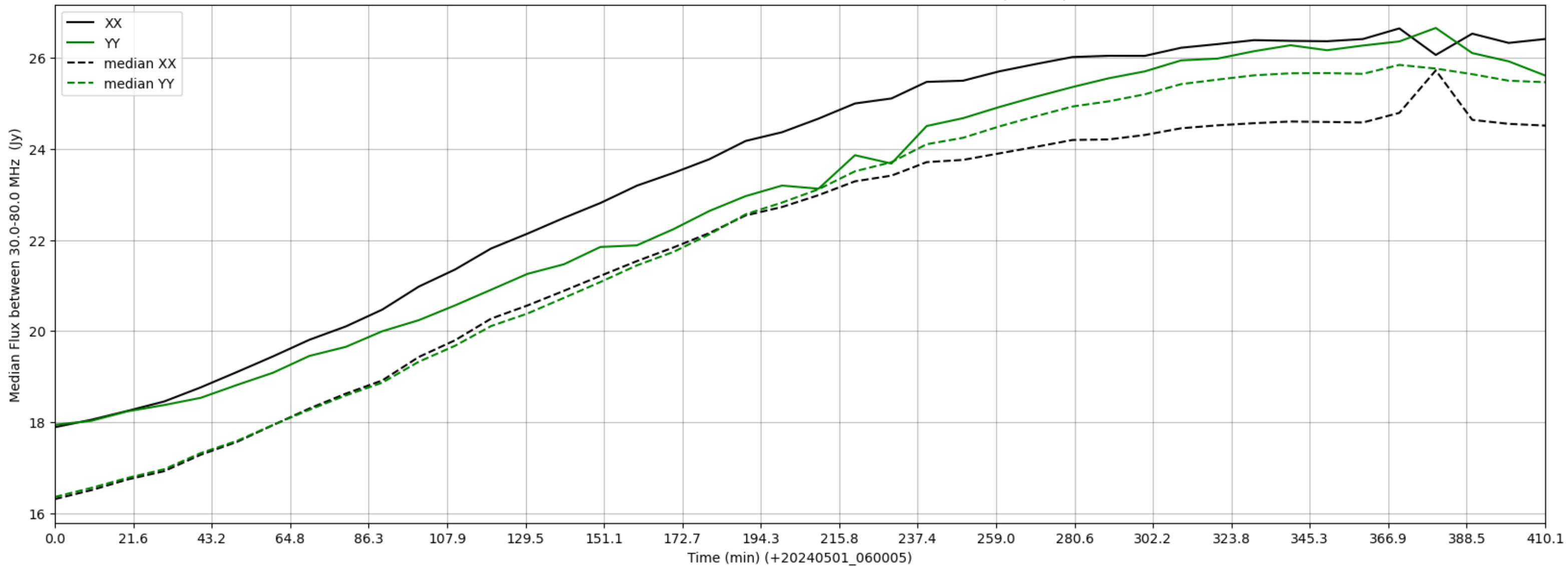
LWA288 - Correlator# 042 - XX FLAGS:Good - YY FLAGS:BadSpecShape
