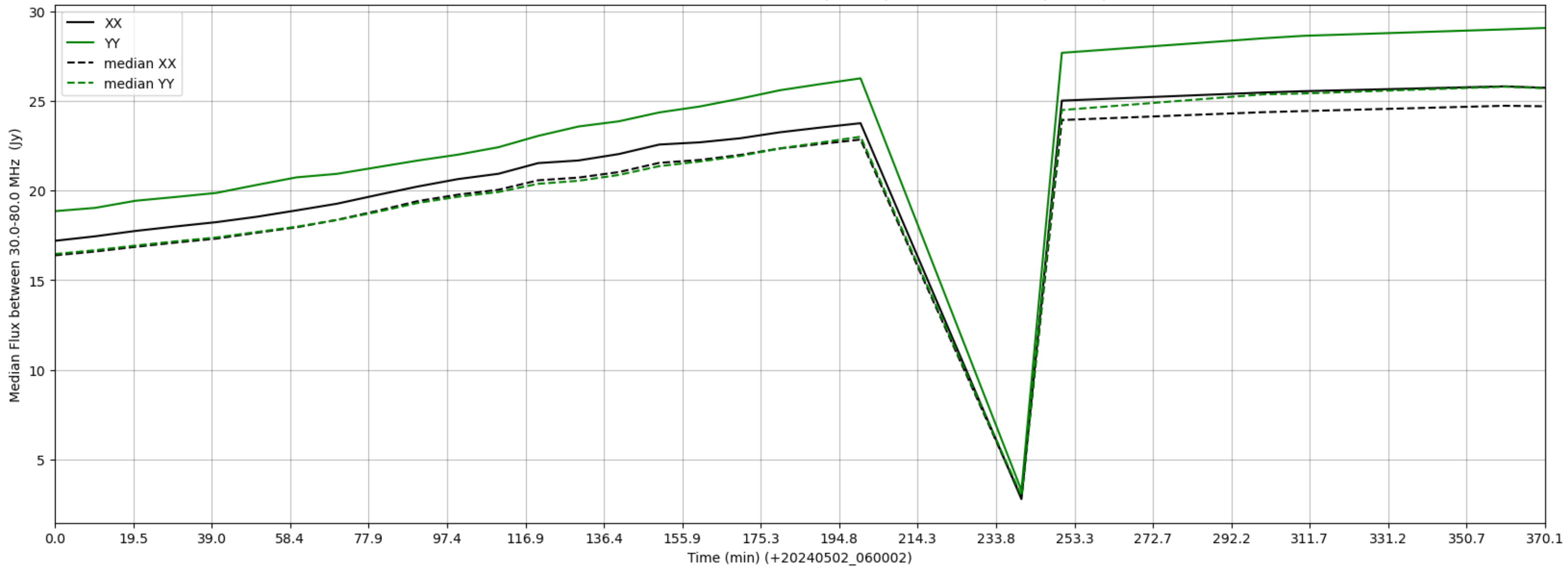
LWA282 - Correlator# 010 - XX FLAGS:BadSpecShape - YY FLAGS:BadSpecShape
