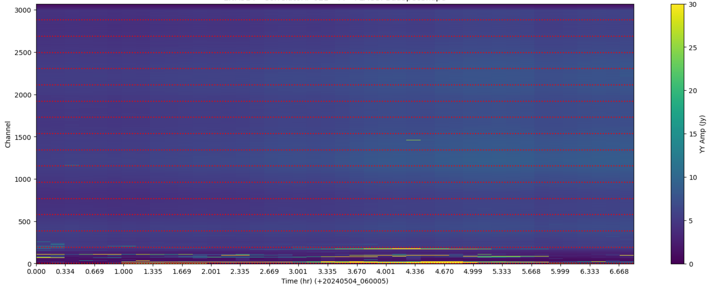
LWA314 - Correlator# 021 - YY - FLAGS: BadSpecShape
