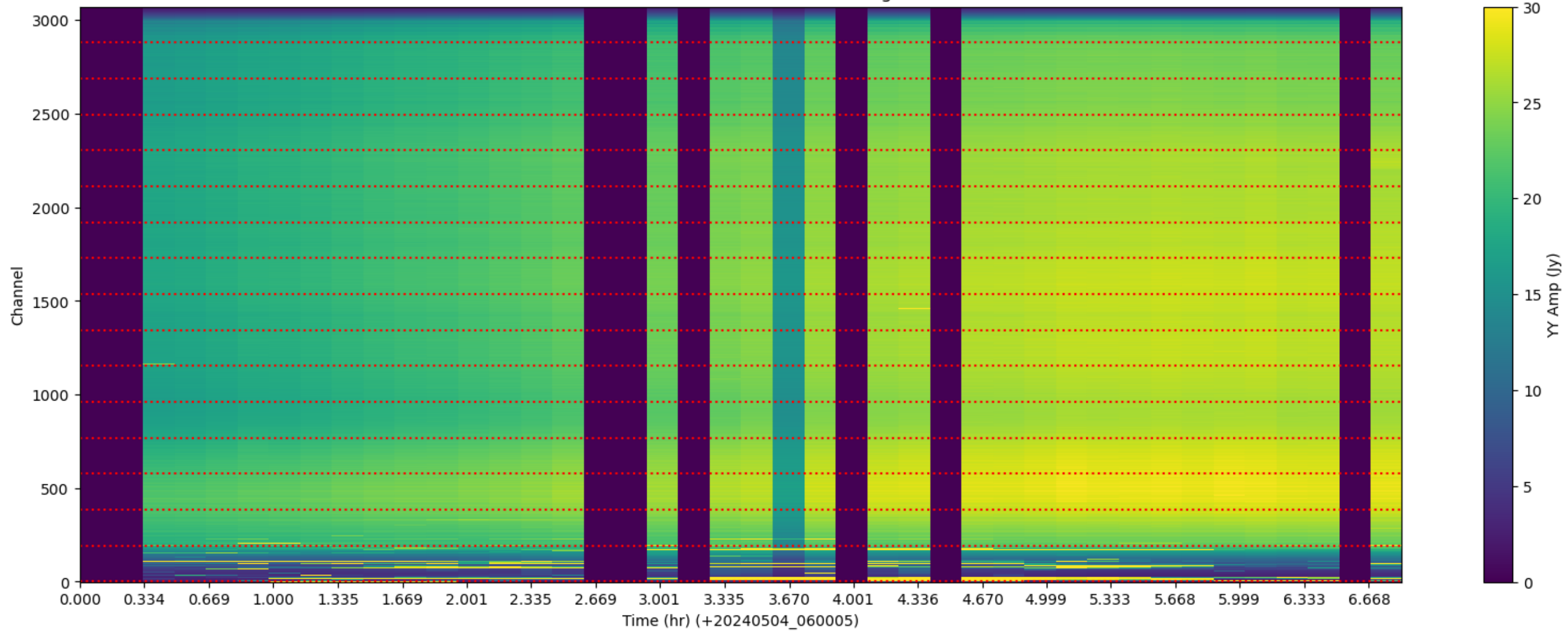
LWA205 - Correlator# 297 - YY - FLAGS: HighTimeVar
