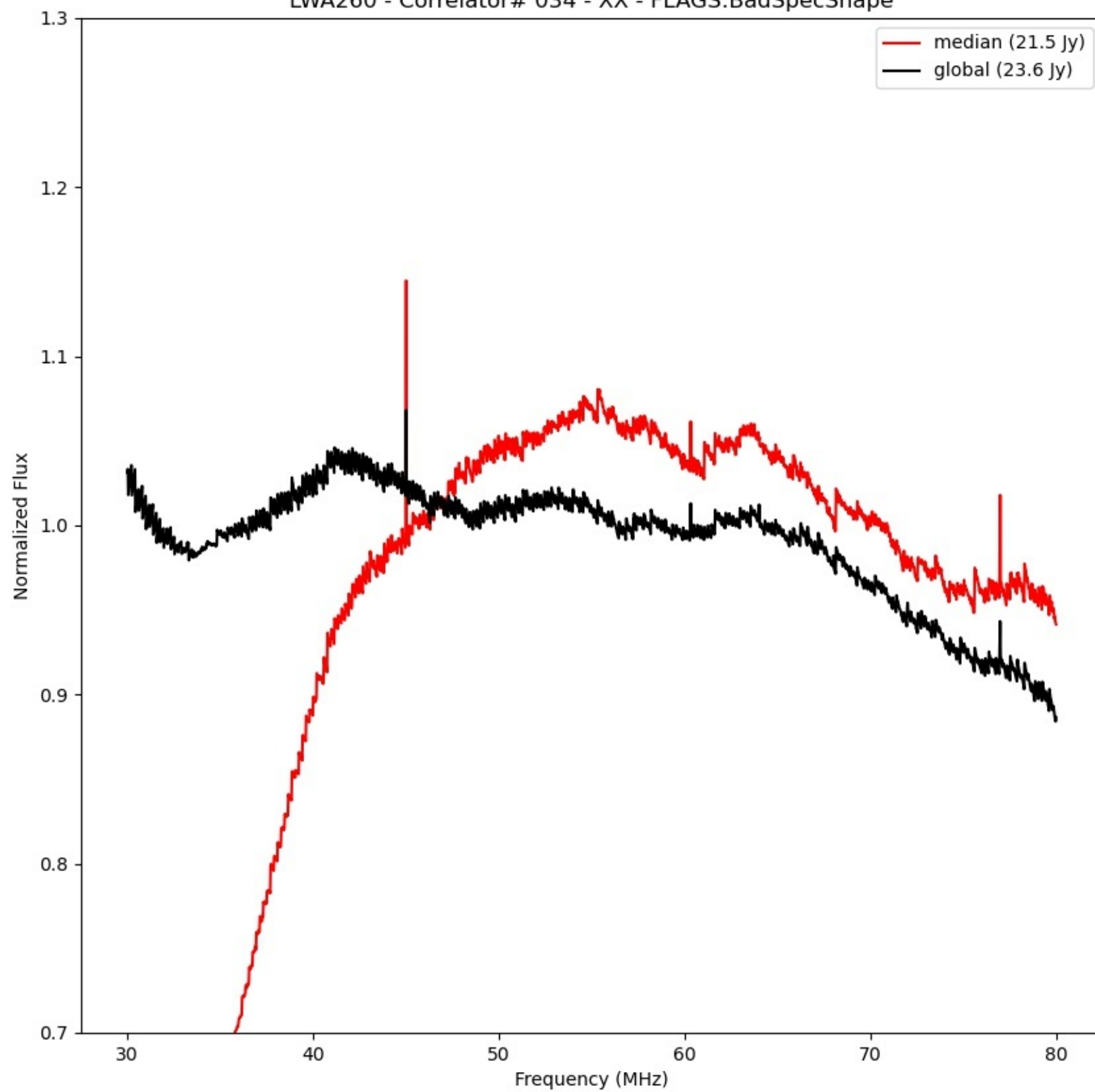
LWA260 - Correlator# 034 - XX - FLAGS:BadSpecShape
