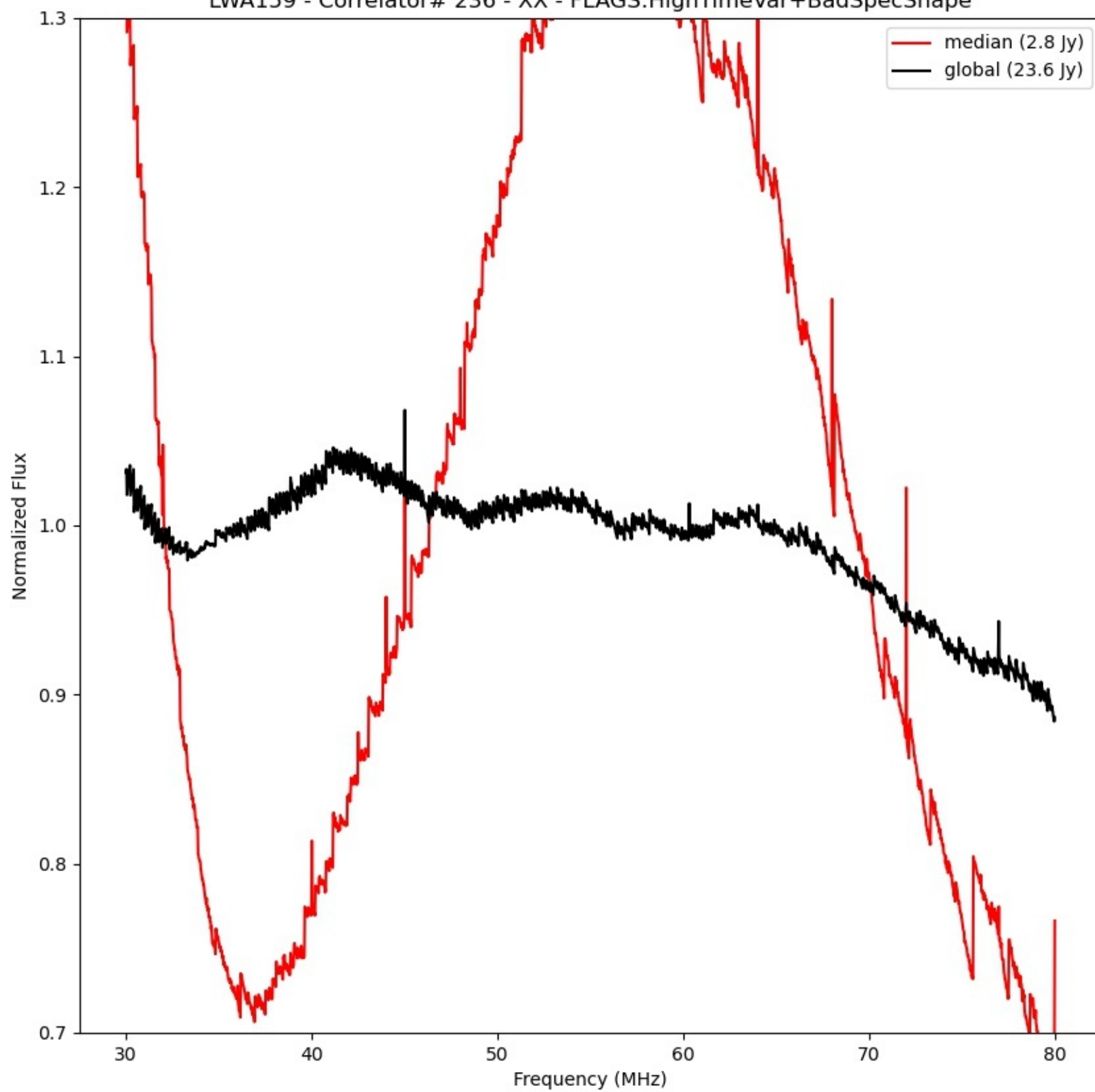
LWA159 - Correlator# 236 - XX - FLAGS:HighTimeVar+BadSpecShape
