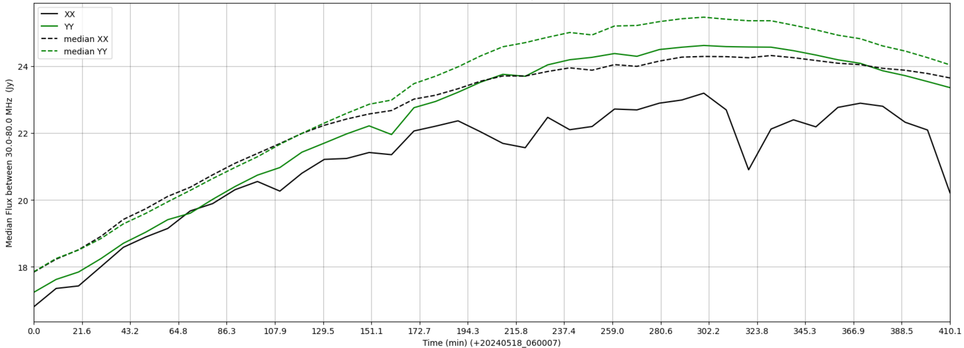
LWA234 - Correlator# 289 - XX FLAGS:BadSpecShape - YY FLAGS:Good
