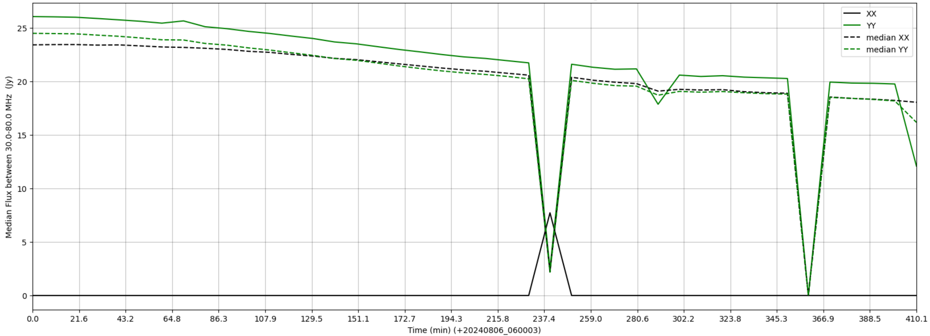
LWA221 - Correlator# 334 - XX FLAGS:LowFlux - YY FLAGS:HighTimeVar
