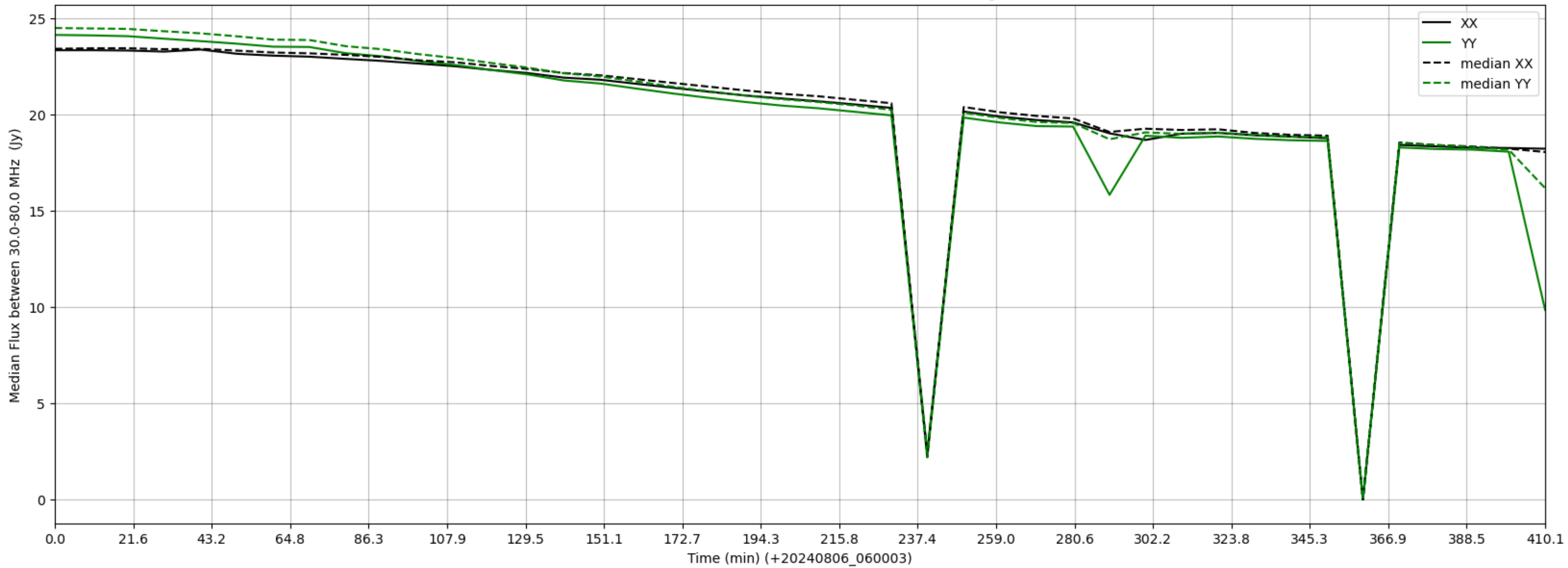
LWA243 - Correlator# 330 - XX FLAGS:Good - YY FLAGS:HighTimeVar
