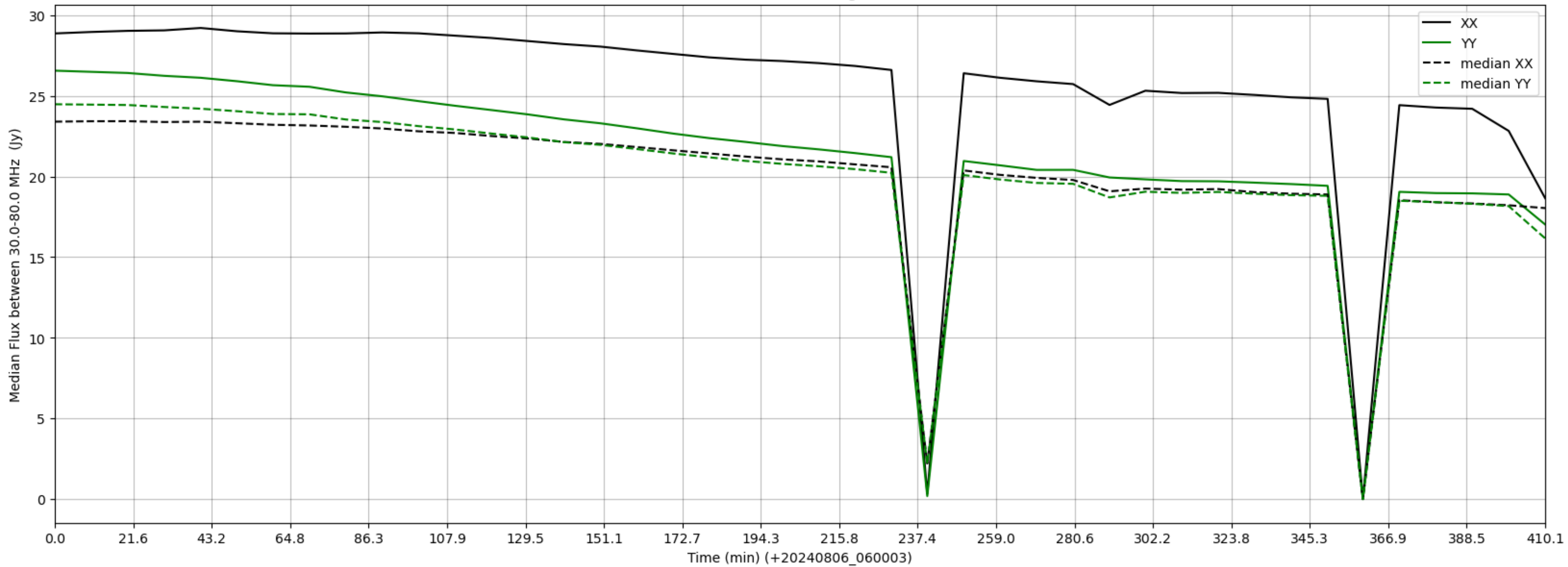
LWA277 - Correlator# 009 - XX FLAGS:HighTimeVar - YY FLAGS:Good
