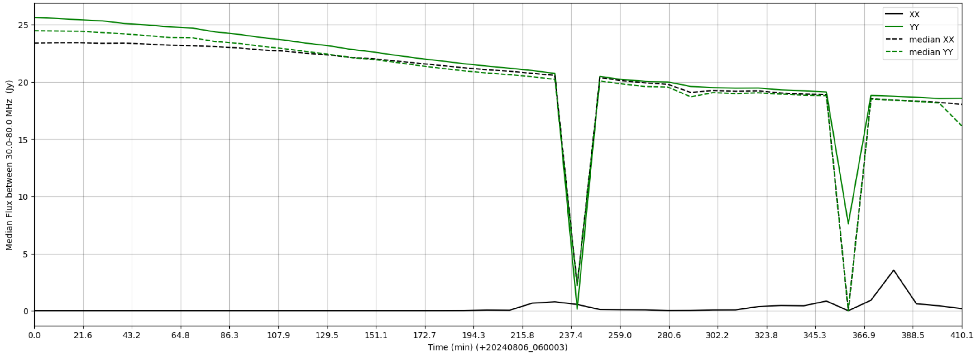
LWA362 - Correlator# 030 - XX FLAGS:LowFlux - YY FLAGS:Good
