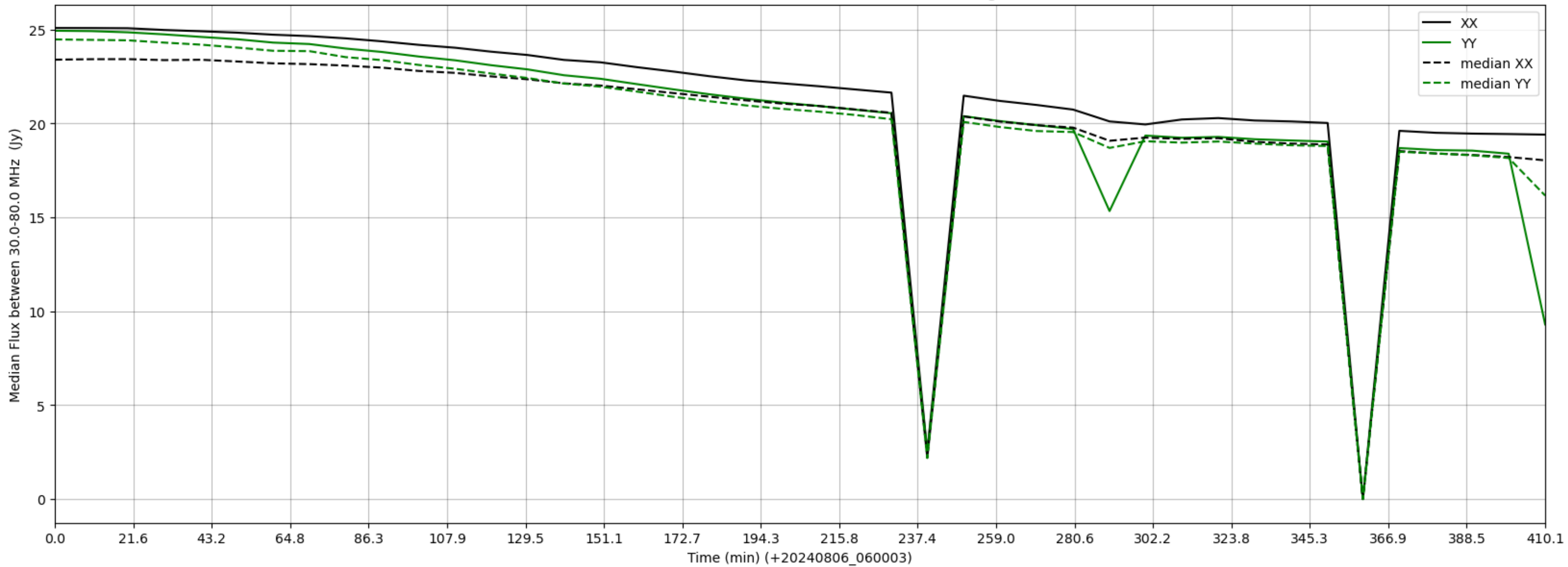
LWA242 - Correlator# 339 - XX FLAGS:Good - YY FLAGS:HighTimeVar
