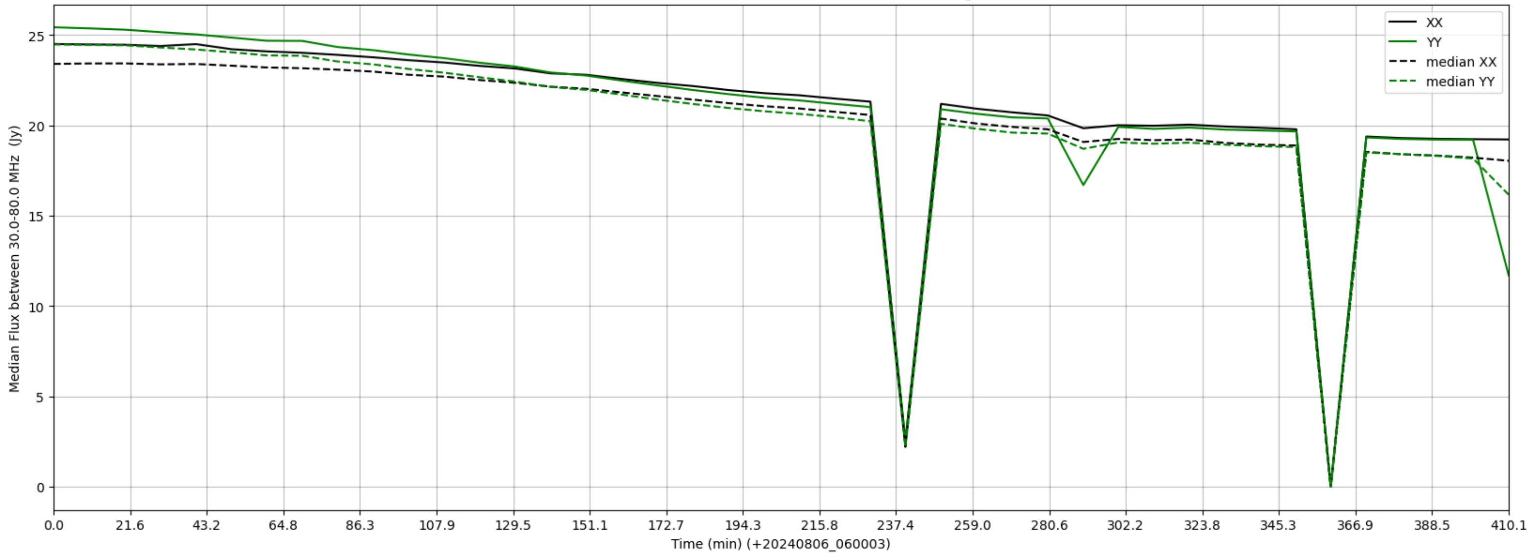
LWA236 - Correlator# 308 - XX FLAGS:Good - YY FLAGS:HighTimeVar
