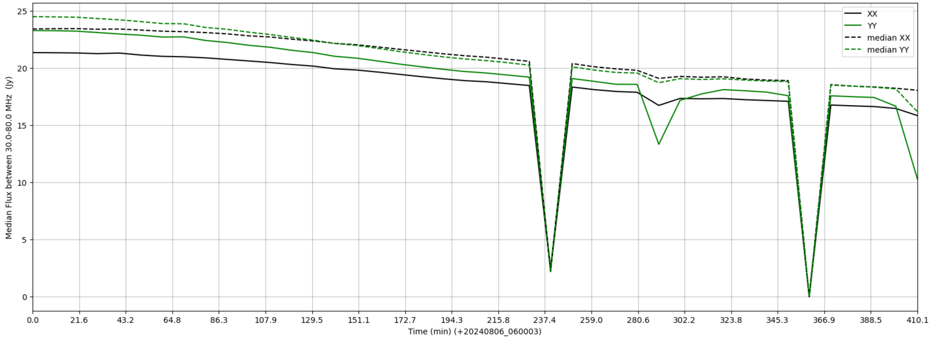
LWA226 - Correlator# 304 - XX FLAGS:Good - YY FLAGS:HighTimeVar
