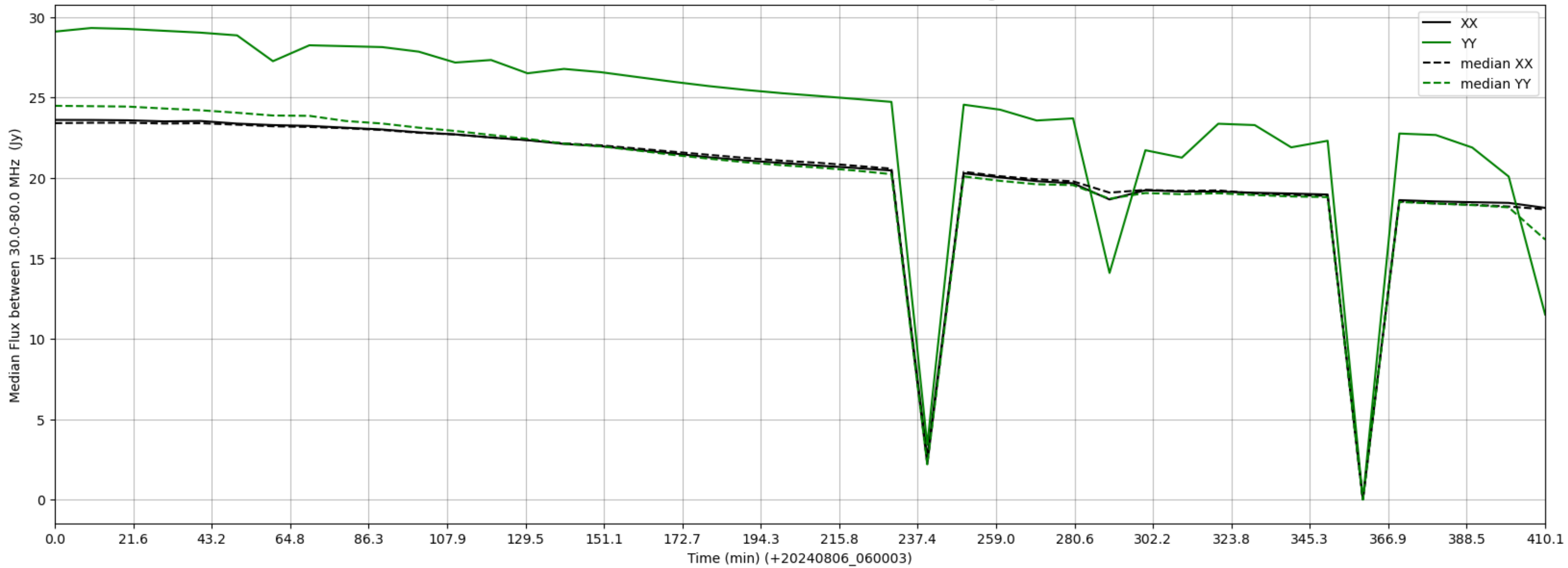
LWA197 - Correlator# 274 - XX FLAGS:Good - YY FLAGS:HighTimeVar
