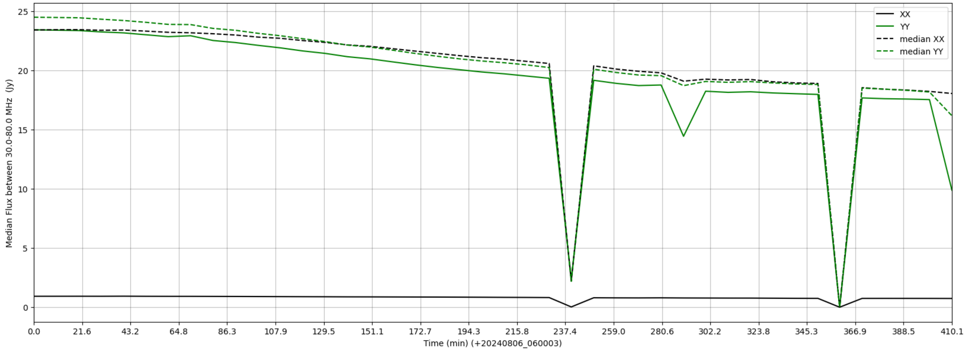
LWA234 - Correlator# 289 - XX FLAGS:LowFlux - YY FLAGS:HighTimeVar
