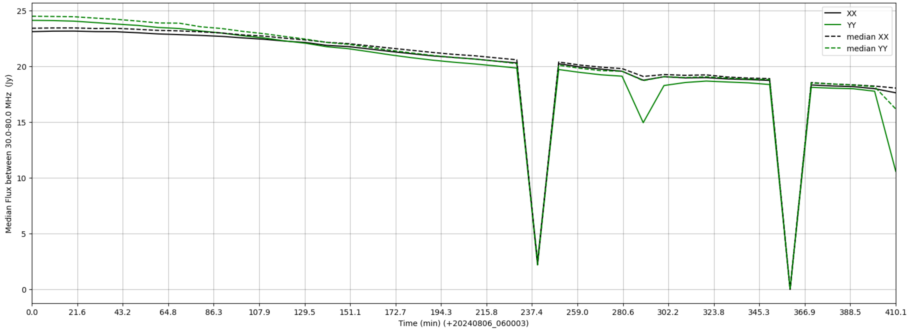
LWA228 - Correlator# 302 - XX FLAGS:Good - YY FLAGS:HighTimeVar
