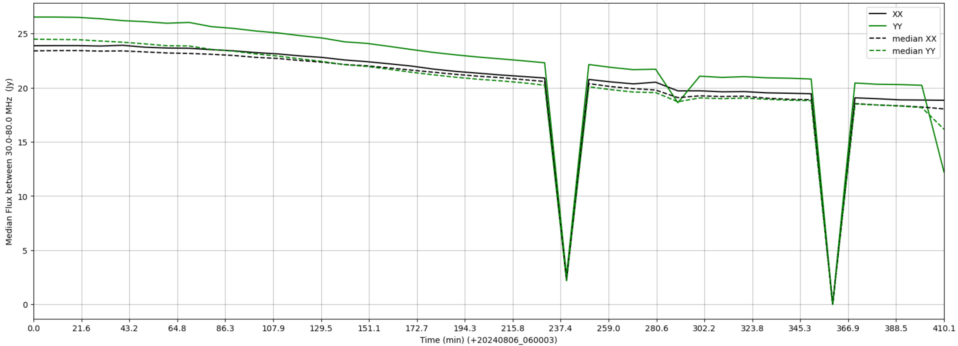
LWA247 - Correlator# 321 - XX FLAGS:Good - YY FLAGS:HighTimeVar
