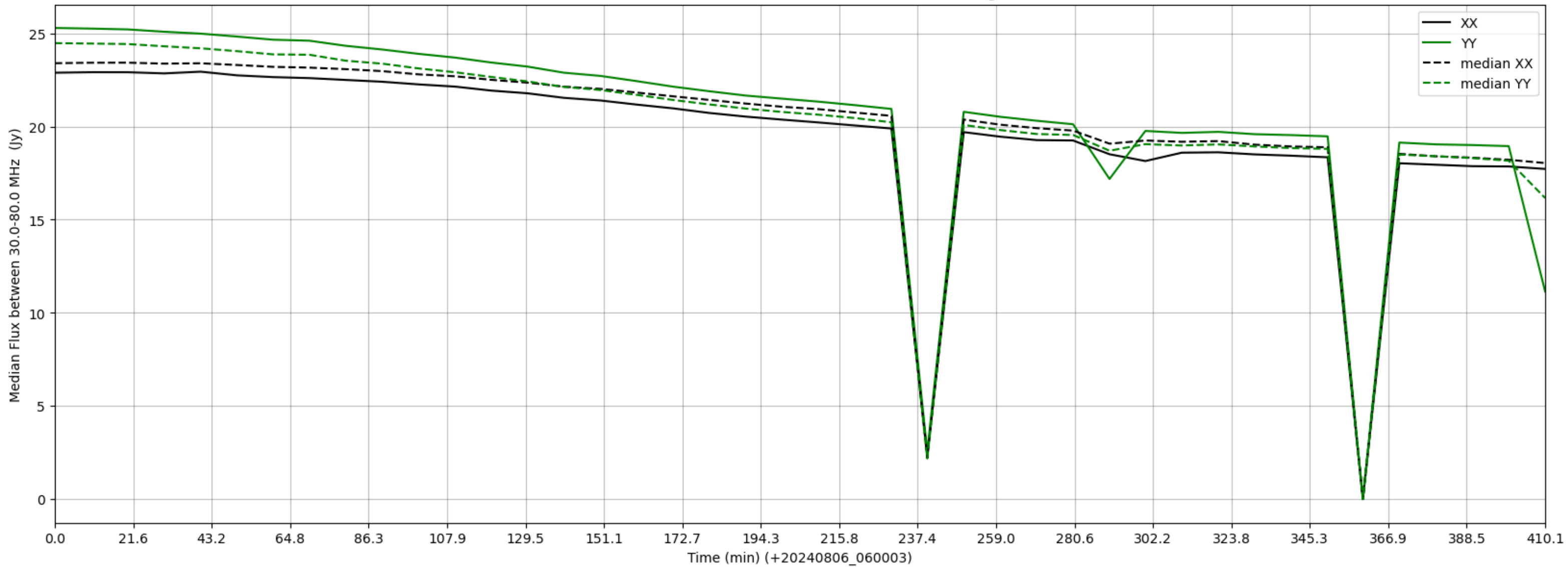
LWA240 - Correlator# 312 - XX FLAGS:Good - YY FLAGS:HighTimeVar
