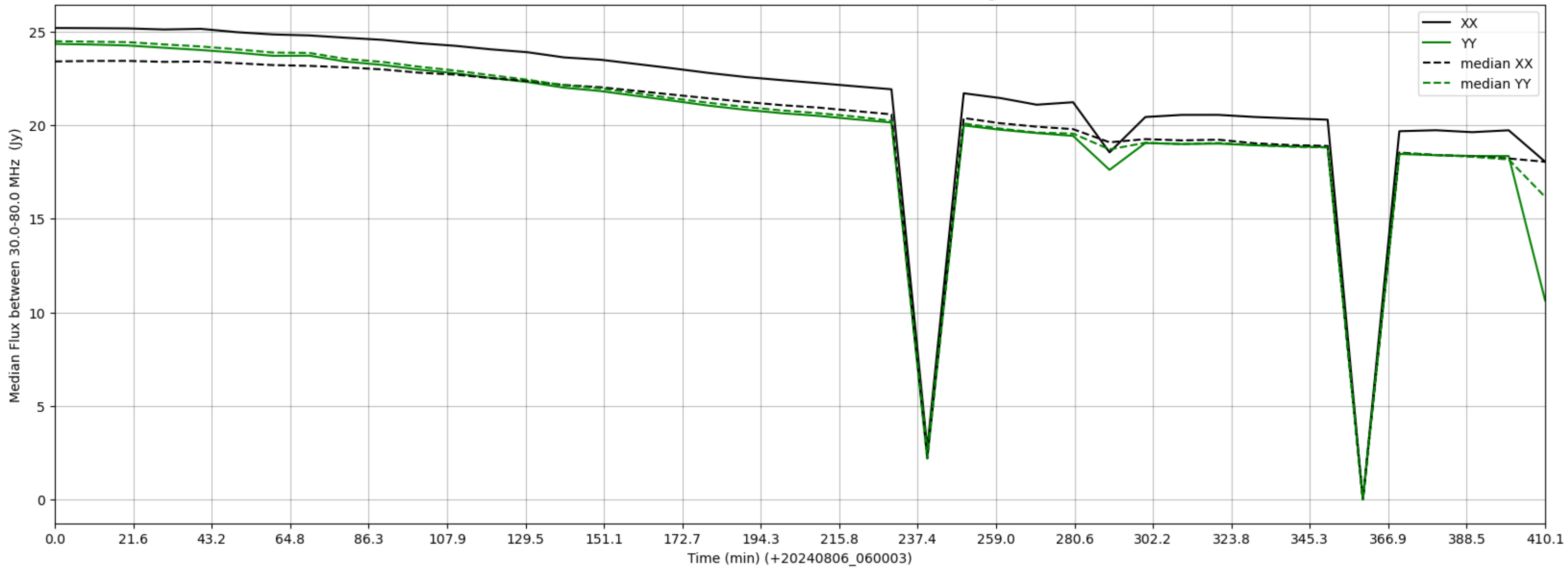
LWA254 - Correlator# 315 - XX FLAGS:Good - YY FLAGS:HighTimeVar
