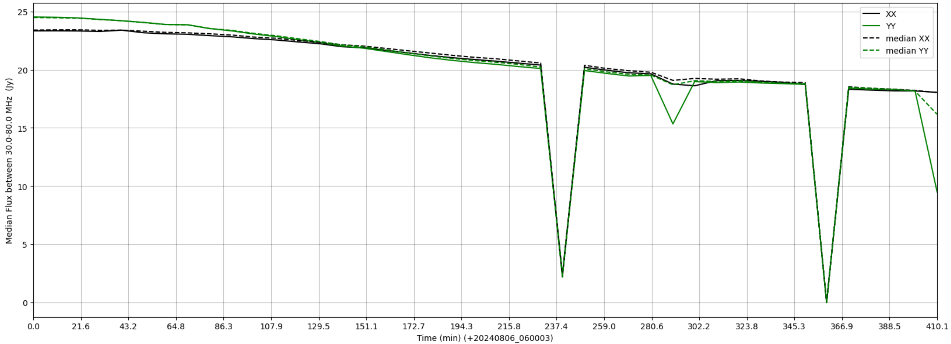
LWA237 - Correlator# 311 - XX FLAGS:Good - YY FLAGS:HighTimeVar
