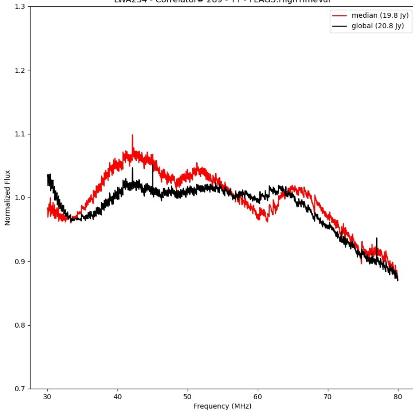
LWA234 - Correlator# 289 - YY - FLAGS:HighTimeVar
