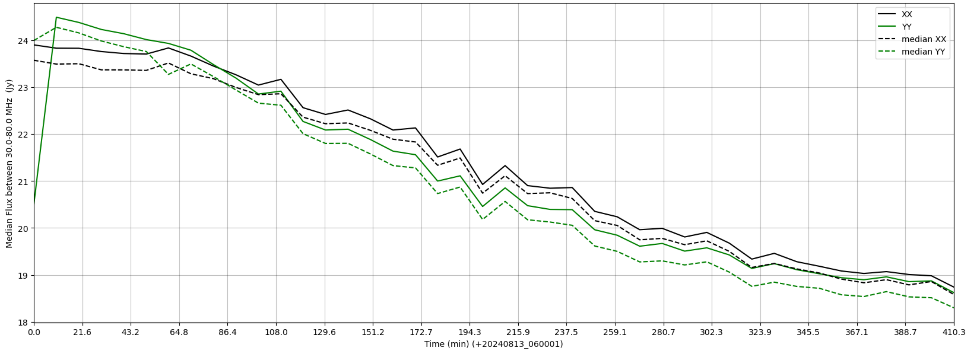
LWA061 - Correlator# 139 - XX FLAGS:Good - YY FLAGS:HighTimeVar
