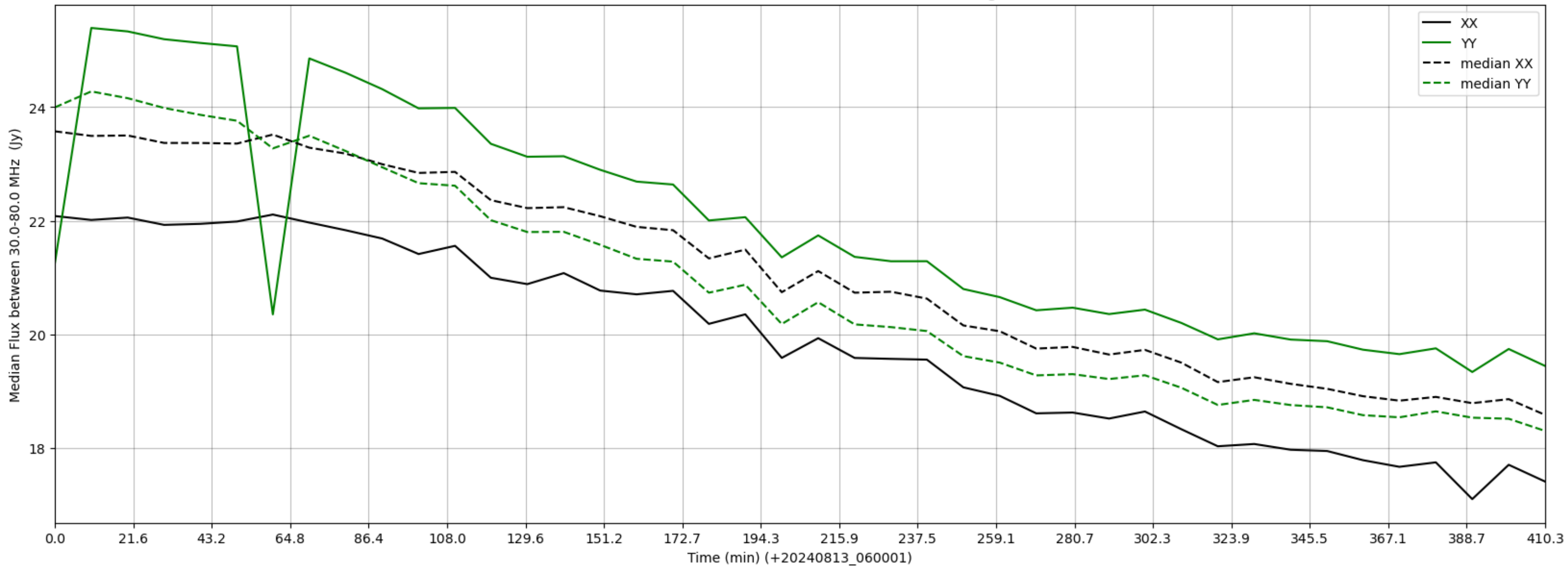
LWA108 - Correlator# 196 - XX FLAGS:Good - YY FLAGS:HighTimeVar
