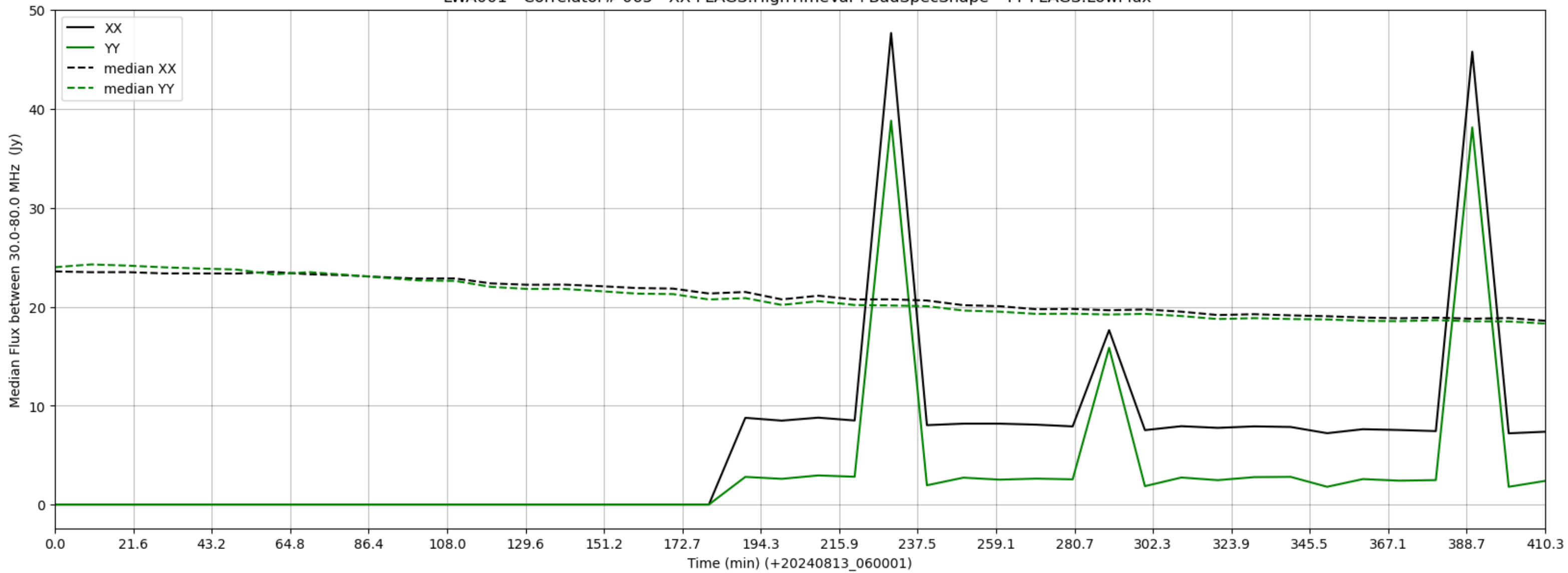
LWA001 - Correlator# 065 - XX FLAGS:HighTimeVar+BadSpecShape - YY FLAGS:LowFlux
