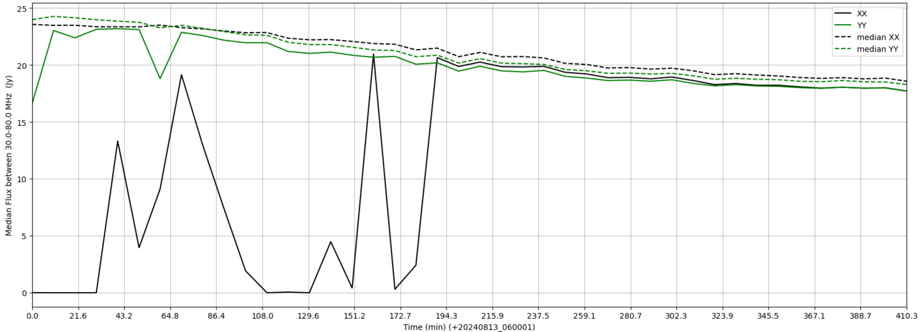
LWA042 - Correlator# 078 - XX FLAGS:HighTimeVar - YY FLAGS:HighTimeVar
