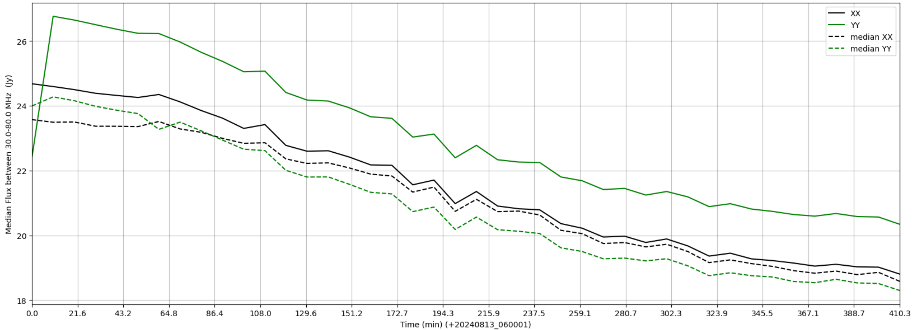
LWA064 - Correlator# 141 - XX FLAGS:Good - YY FLAGS:HighTimeVar
