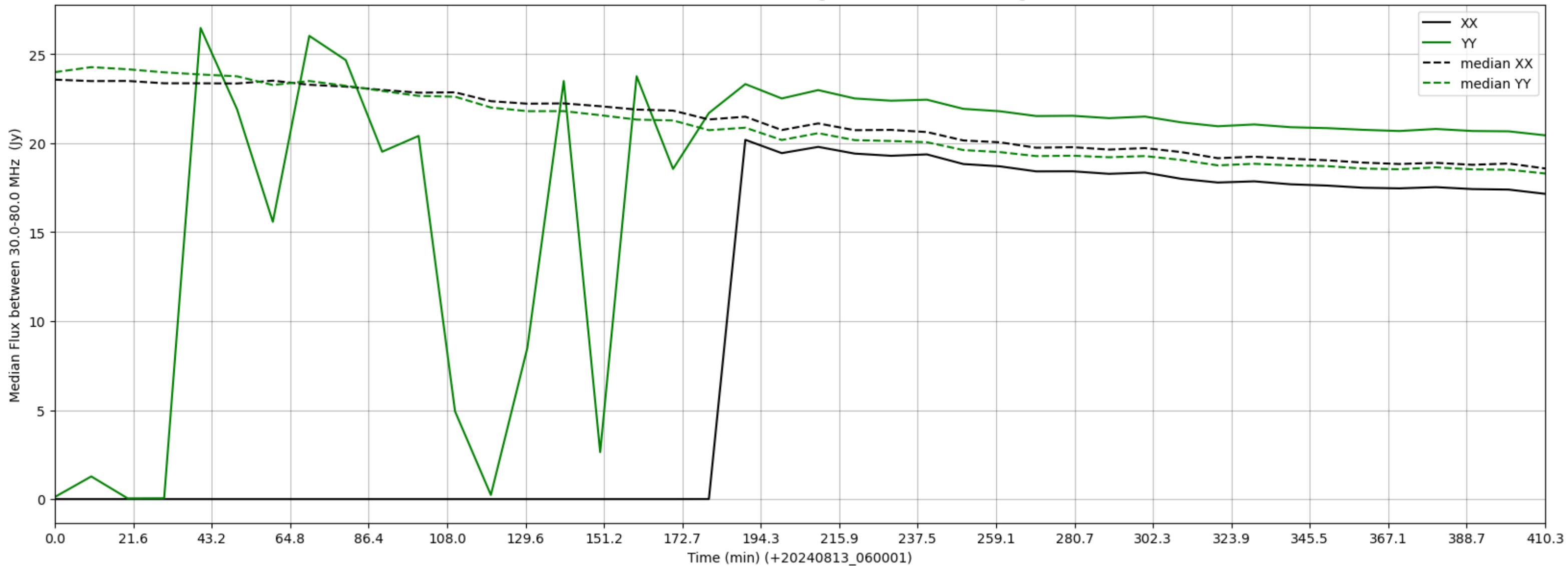
LWA045 - Correlator# 083 - XX FLAGS:HighTimeVar - YY FLAGS:HighTimeVar
