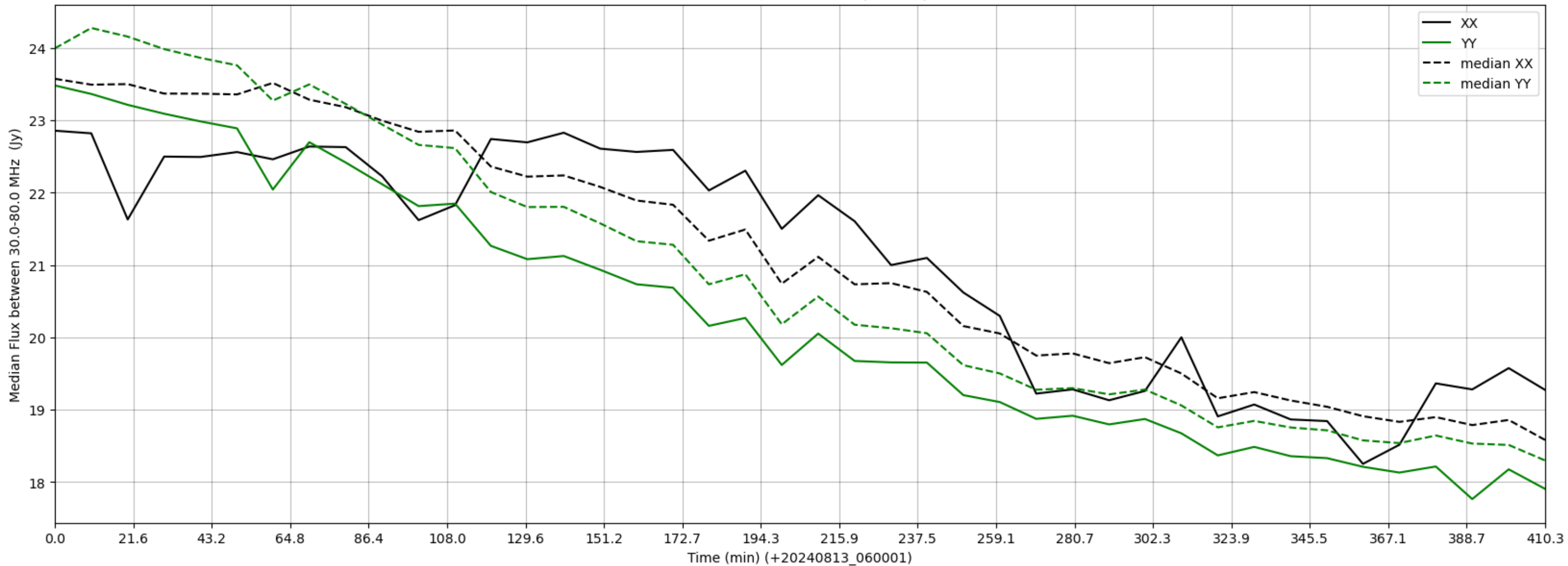
LWA109 - Correlator# 199 - XX FLAGS:BadSpecShape - YY FLAGS:Good
