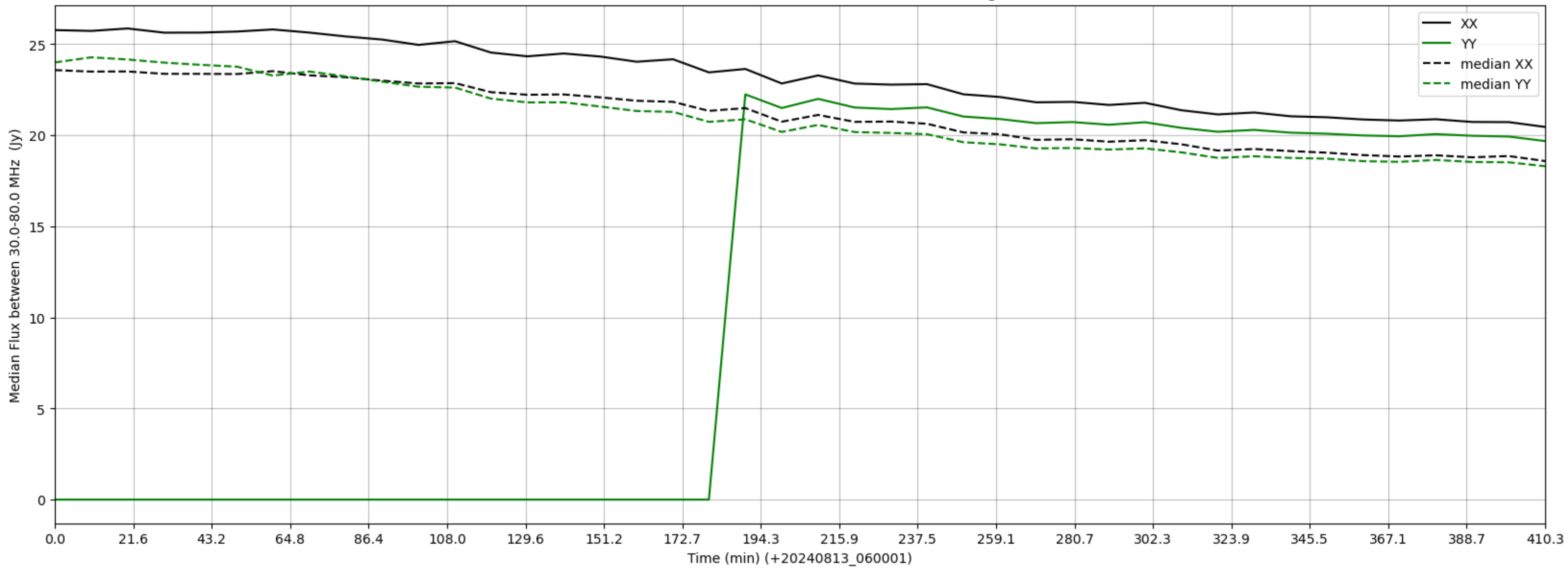
LWA012 - Correlator# 074 - XX FLAGS:Good - YY FLAGS:HighTimeVar
