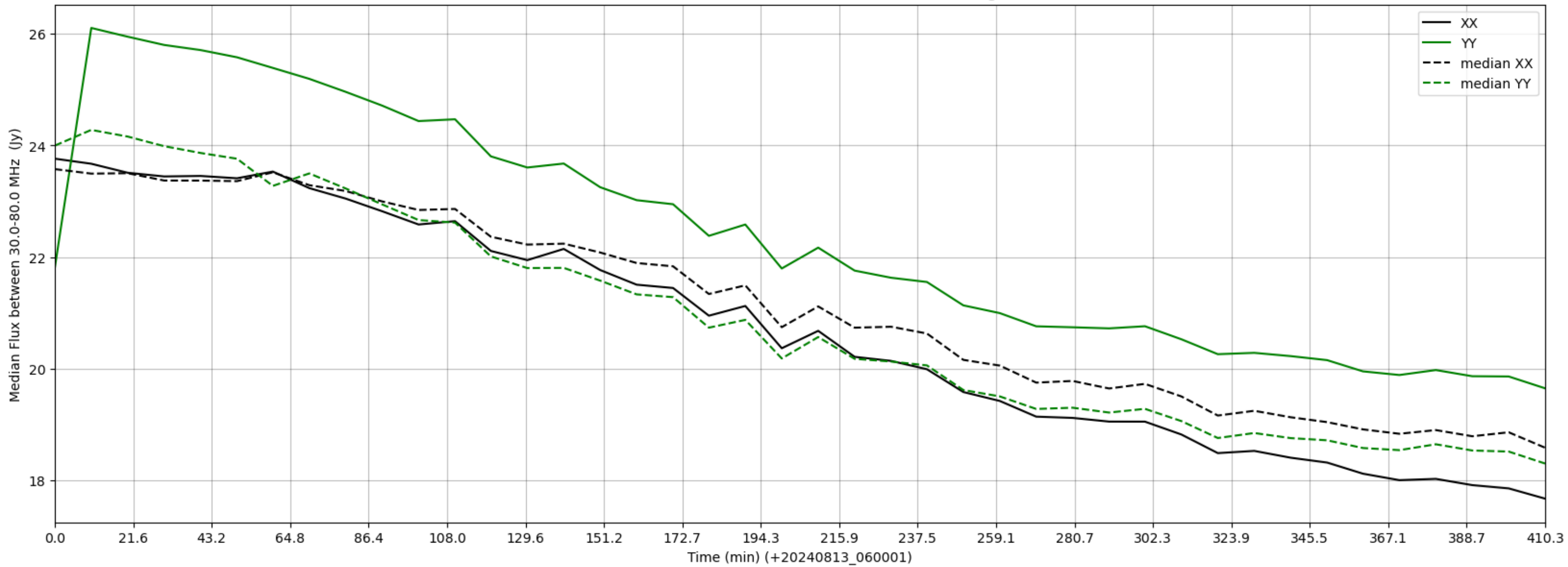
LWA265 - Correlator# 036 - XX FLAGS:Good - YY FLAGS:HighTimeVar
