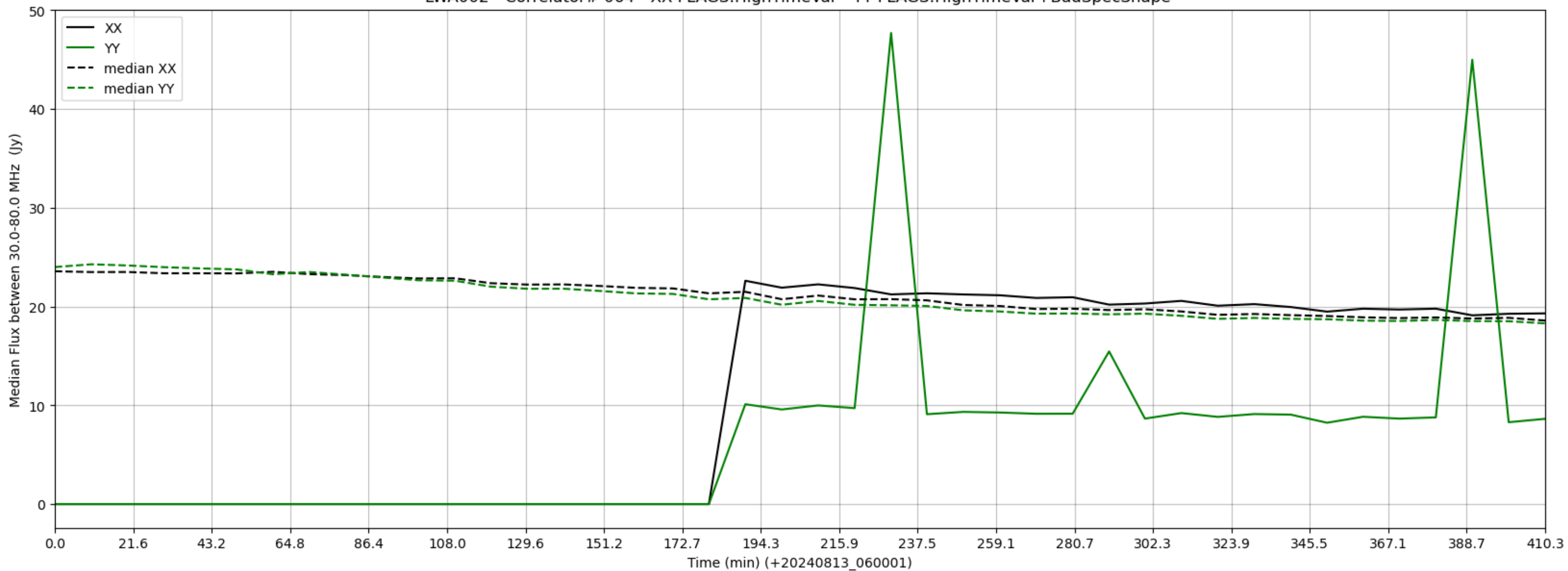
LWA002 - Correlator# 064 - XX FLAGS:HighTimeVar - YY FLAGS:HighTimeVar+BadSpecShape
