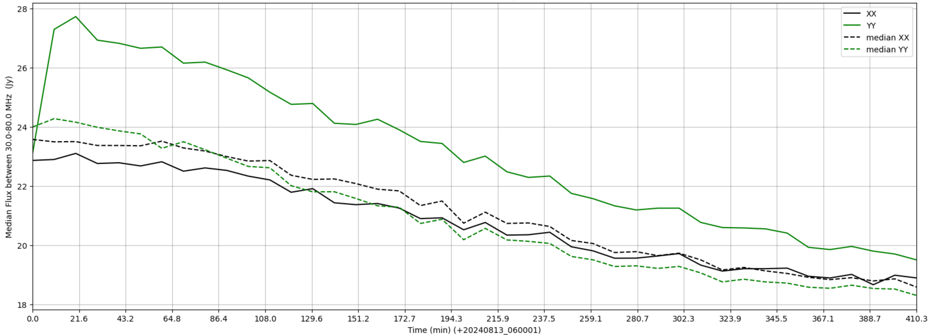
LWA294 - Correlator# 188 - XX FLAGS:BadSpecShape - YY FLAGS:Good
