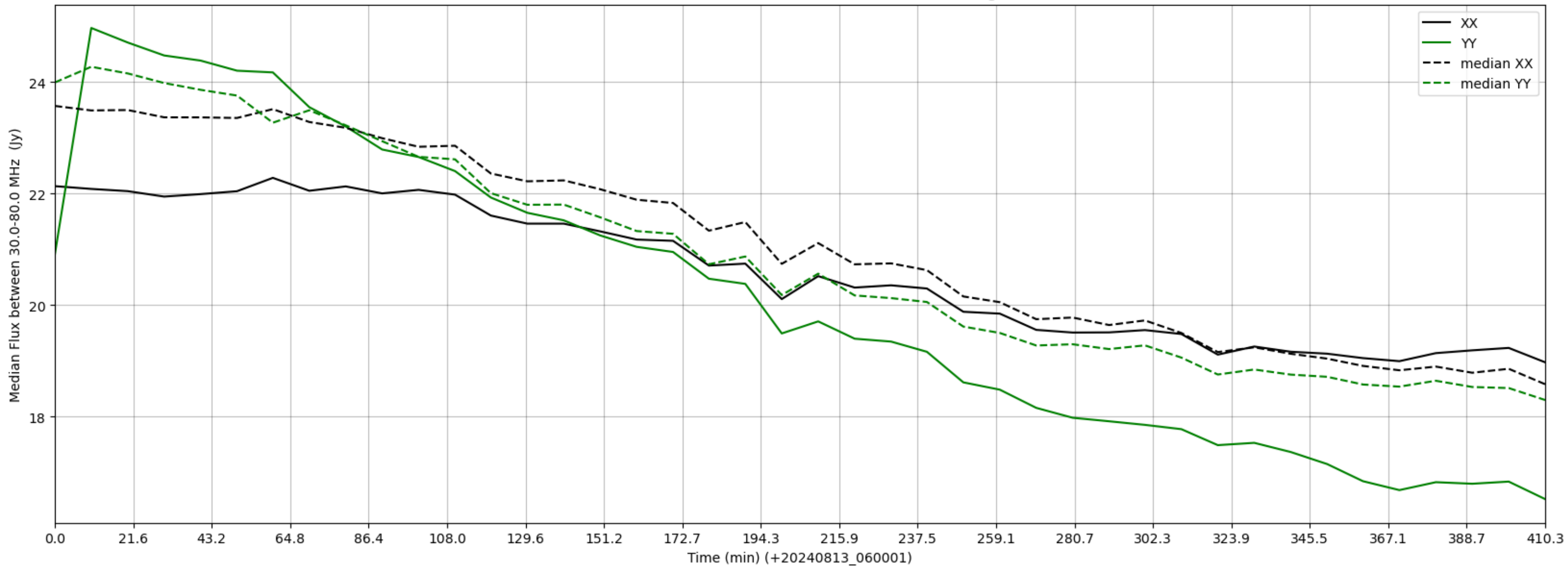
LWA271 - Correlator# 004 - XX FLAGS:Good - YY FLAGS:HighTimeVar
