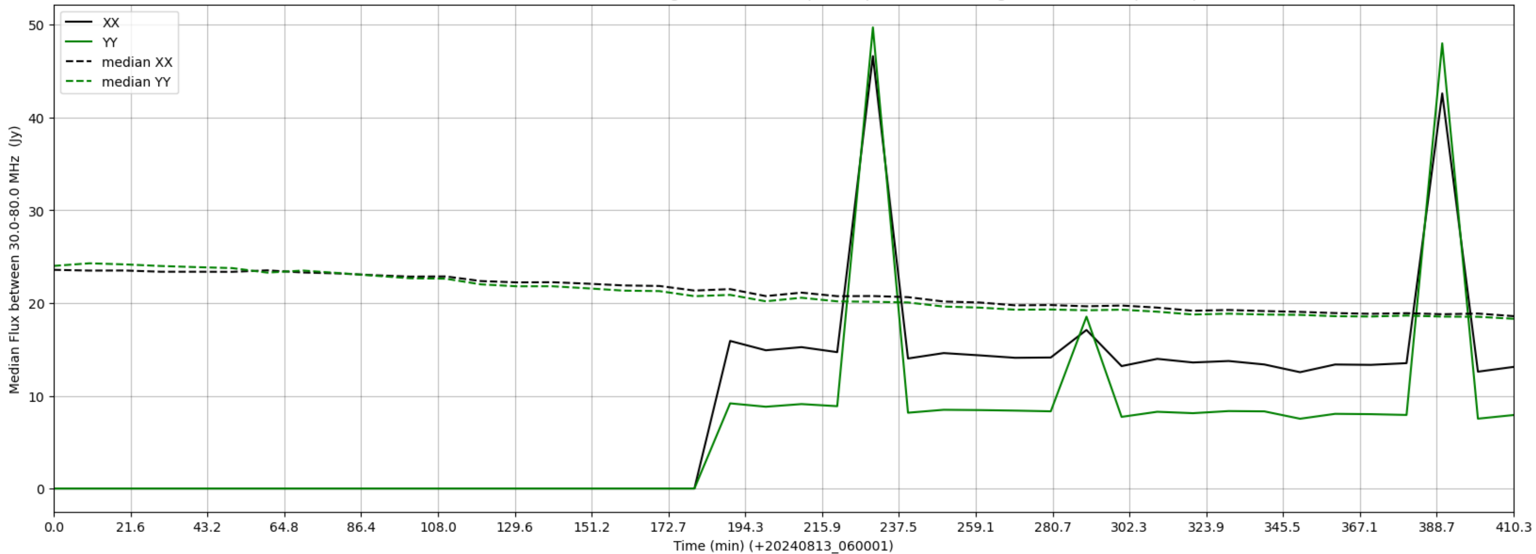
LWA006 - Correlator# 068 - XX FLAGS:HighTimeVar+BadSpecShape - YY FLAGS:HighTimeVar+BadSpecShape
