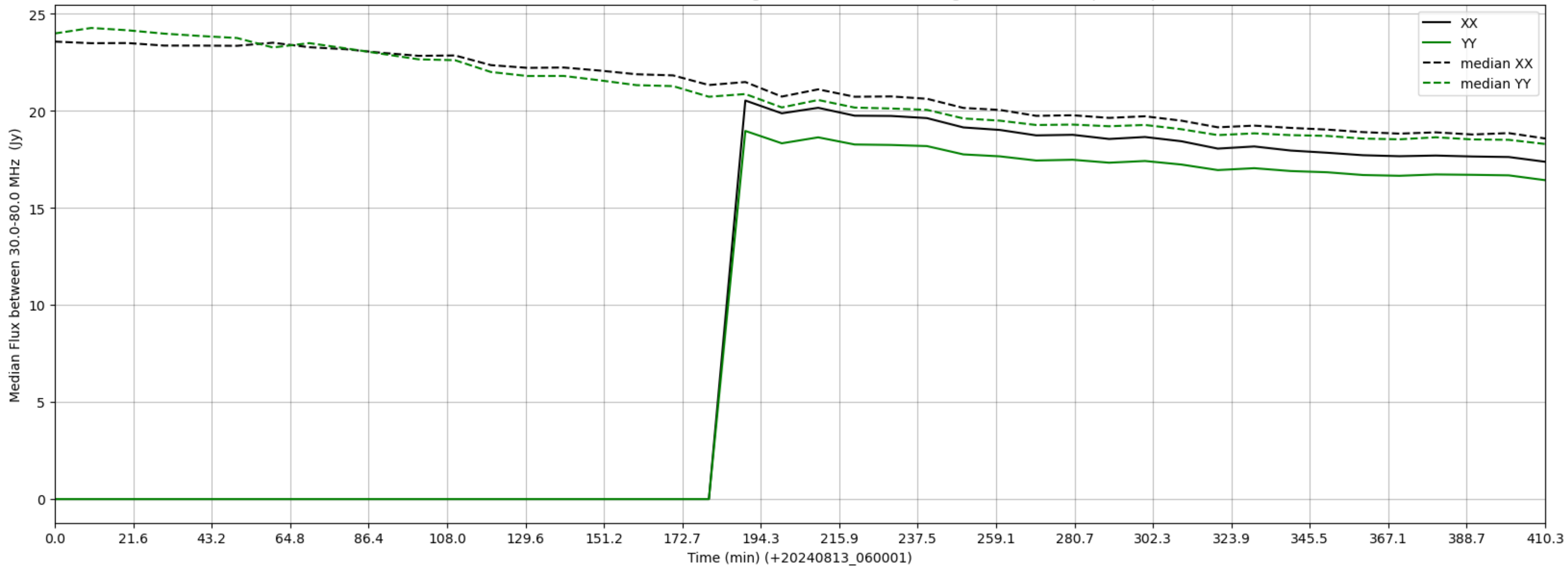
LWA005 - Correlator# 069 - XX FLAGS:HighTimeVar - YY FLAGS:HighTimeVar+BadSpecShape
