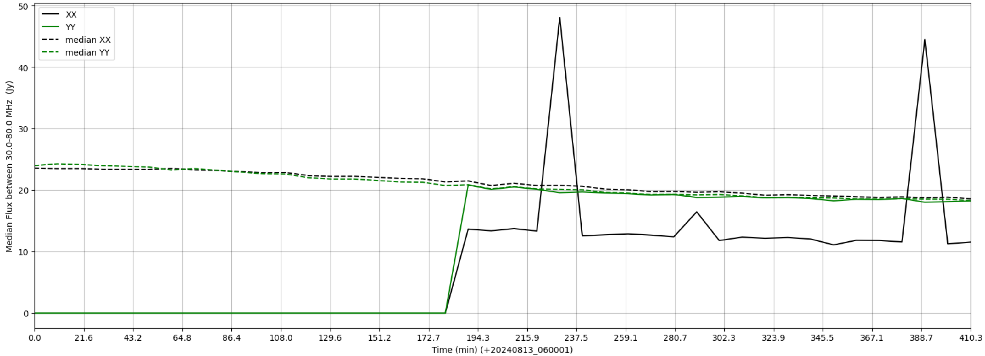
LWA007 - Correlator# 071 - XX FLAGS:HighTimeVar+BadSpecShape - YY FLAGS:HighTimeVar
