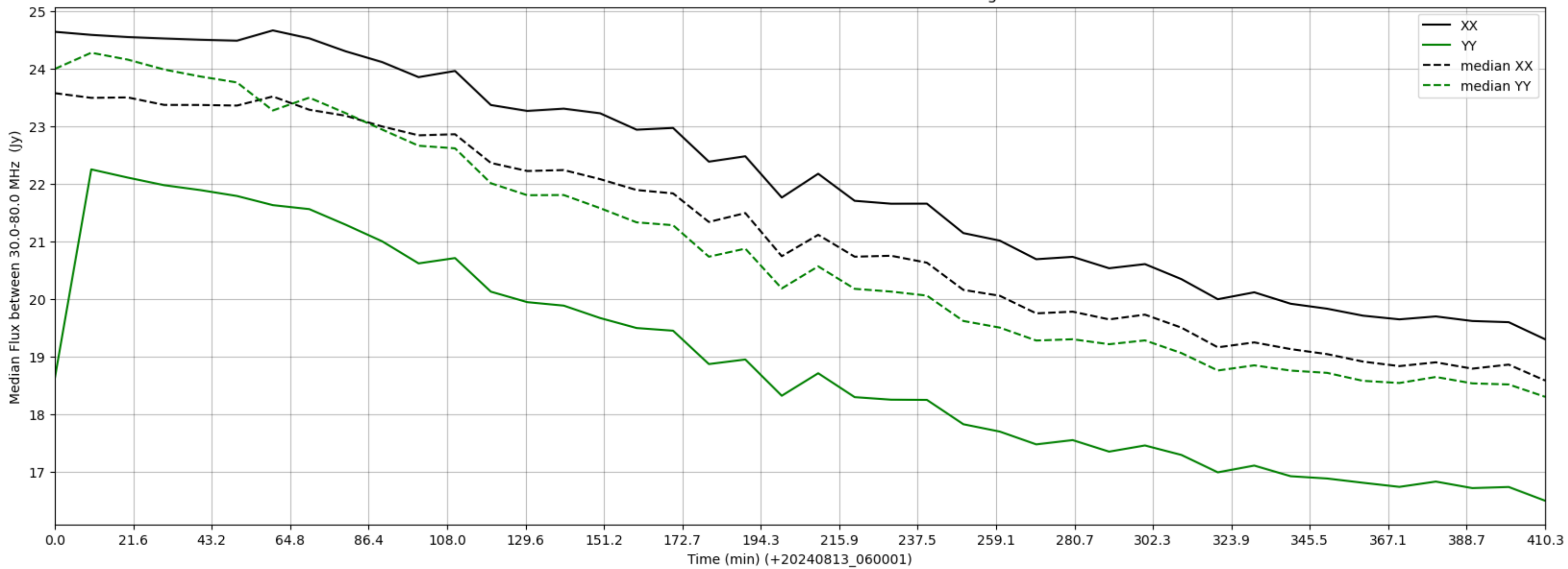
LWA021 - Correlator# 105 - XX FLAGS:Good - YY FLAGS:HighTimeVar
