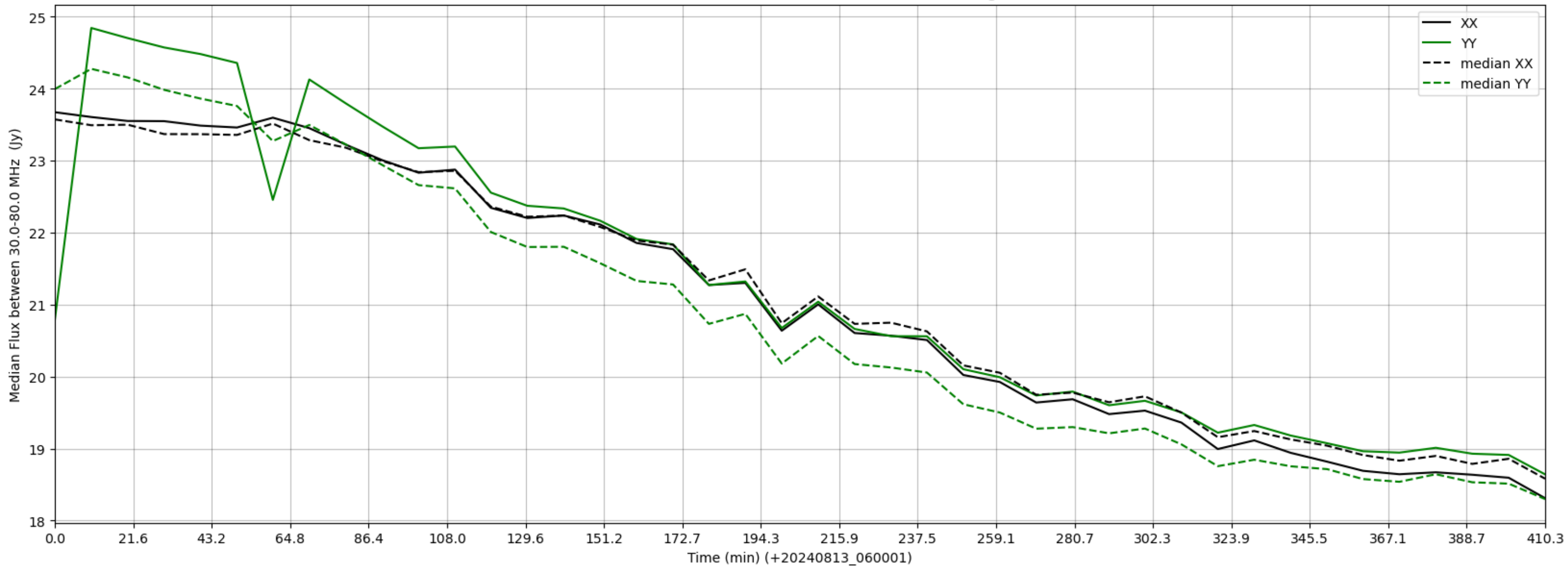
LWA013 - Correlator# 096 - XX FLAGS:Good - YY FLAGS:HighTimeVar
