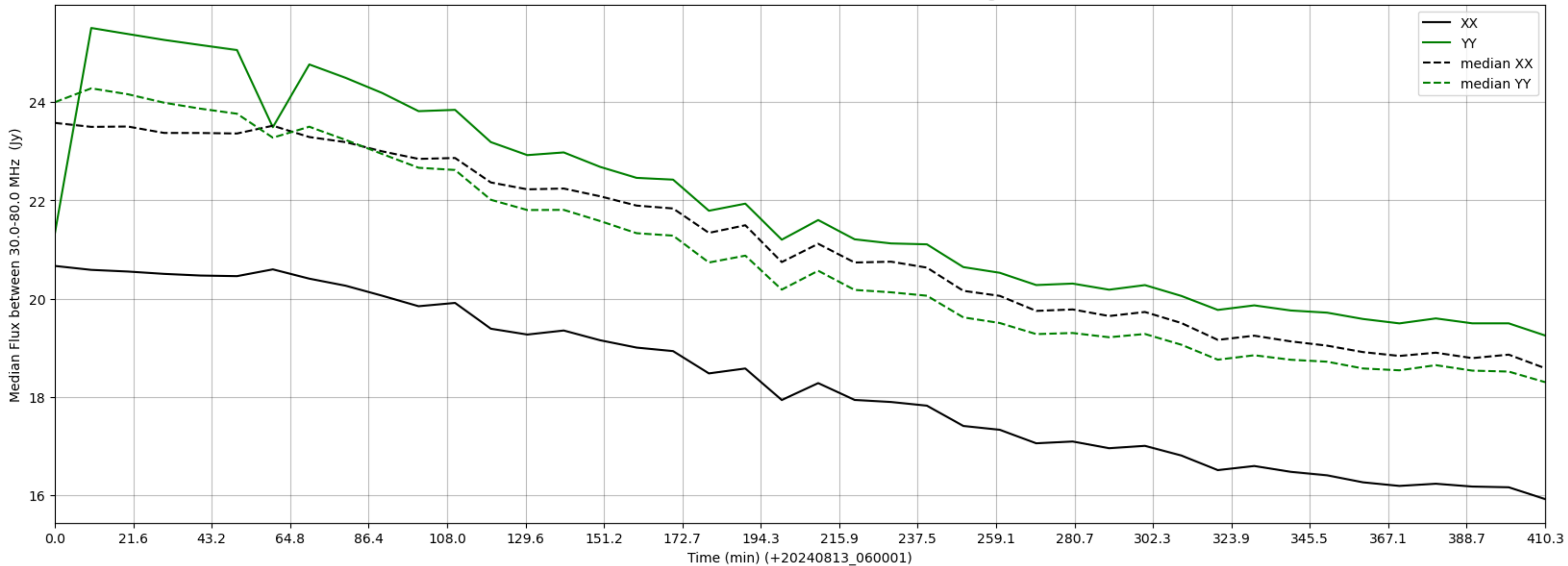
LWA206 - Correlator# 296 - XX FLAGS:Good - YY FLAGS:HighTimeVar
