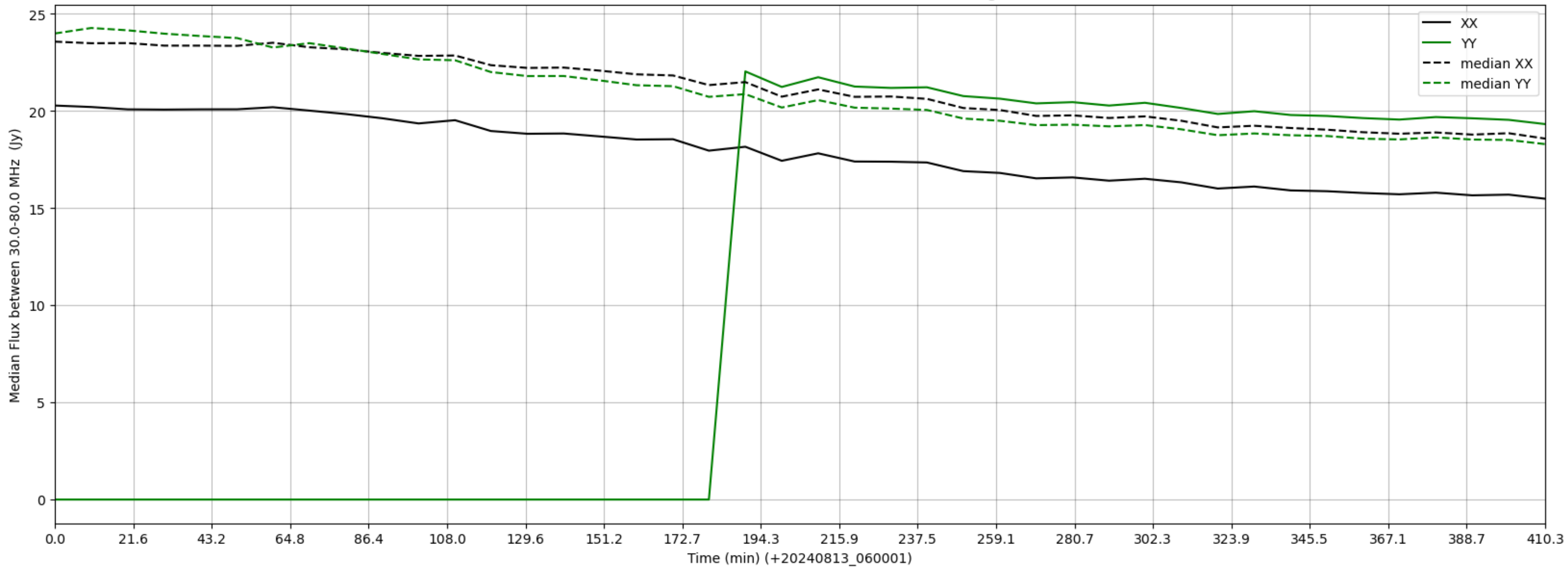
LWA038 - Correlator# 077 - XX FLAGS:Good - YY FLAGS:HighTimeVar
