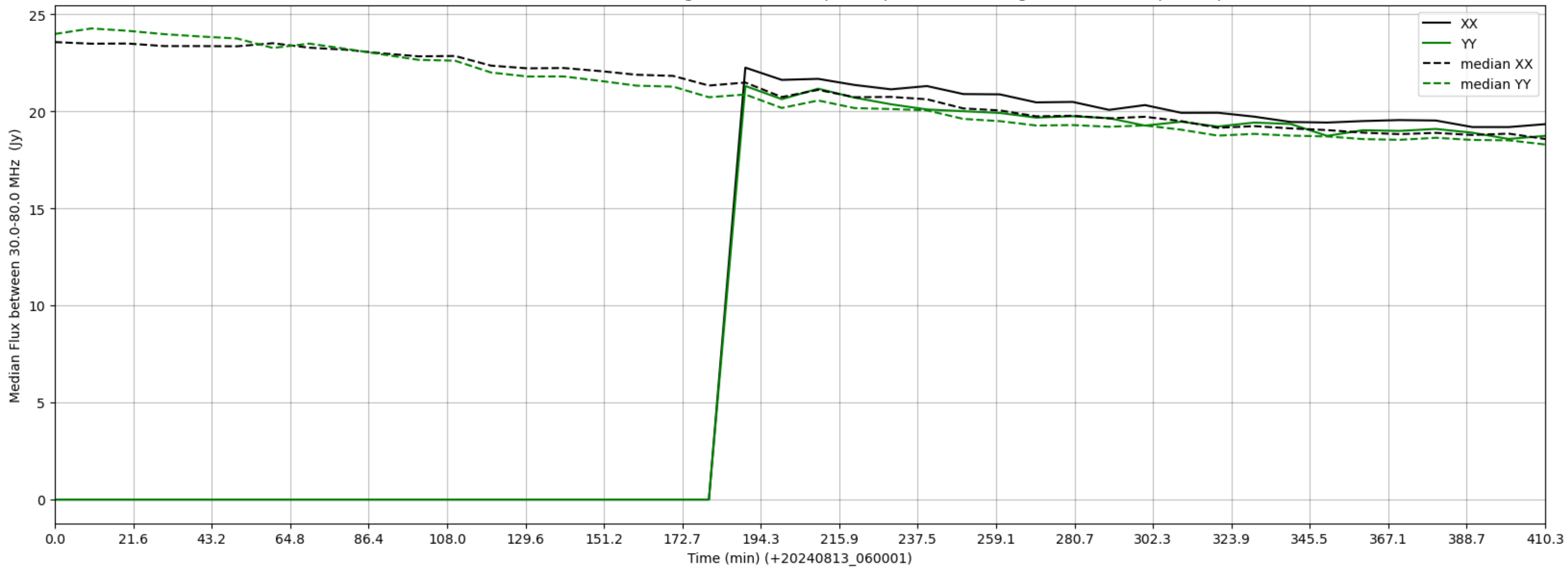
LWA004 - Correlator# 066 - XX FLAGS:HighTimeVar+BadSpecShape - YY FLAGS:HighTimeVar+BadSpecShape
