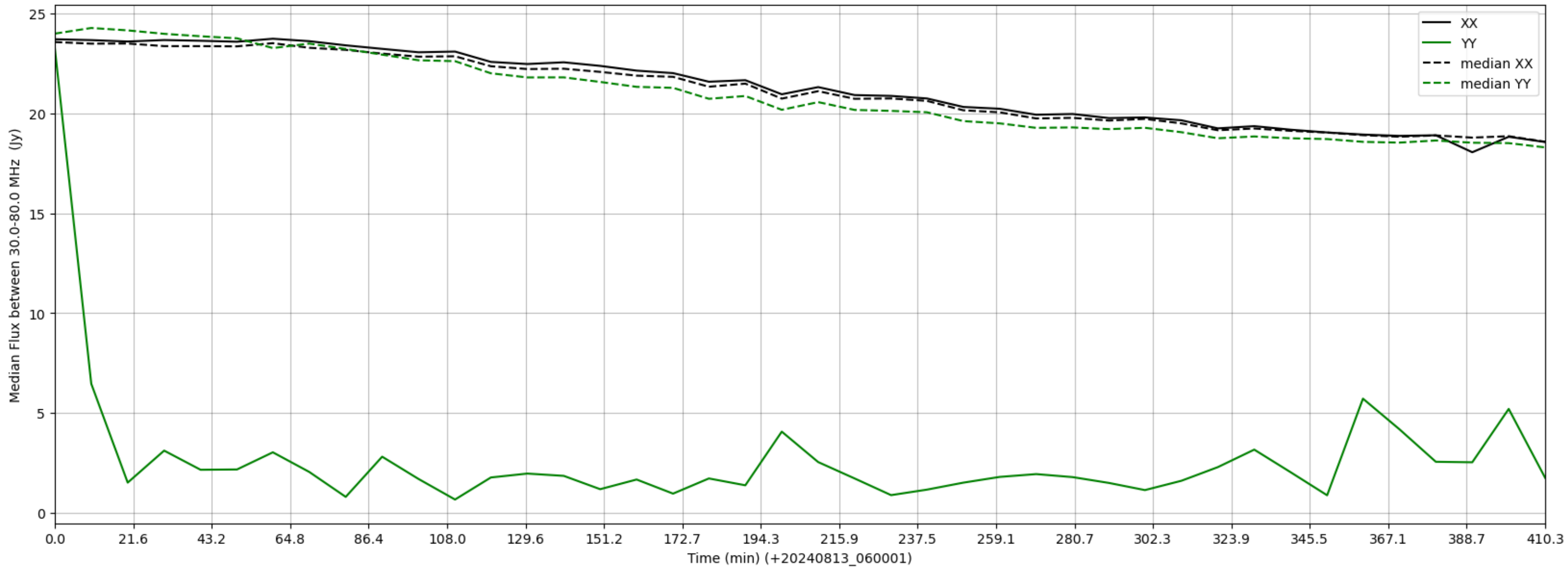
LWA128 - Correlator# 229 - XX FLAGS:Good - YY FLAGS:LowFlux
