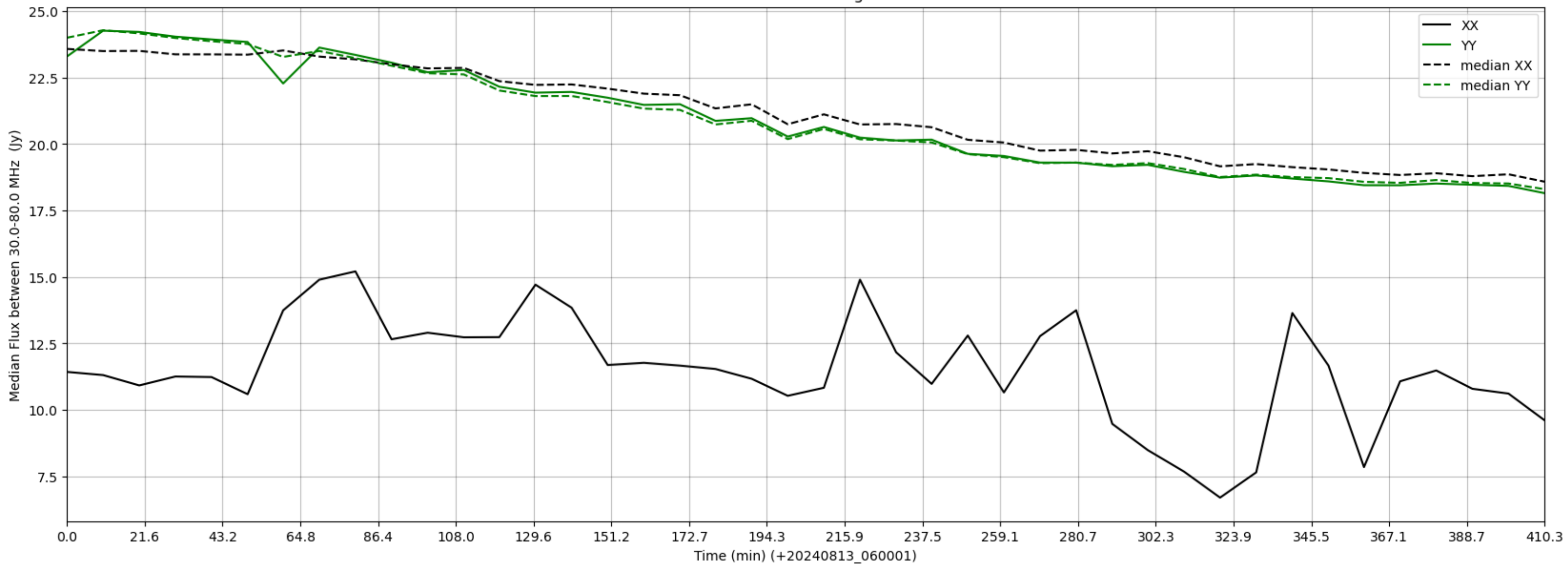
LWA073 - Correlator# 087 - XX FLAGS:HighTimeVar - YY FLAGS:Good
