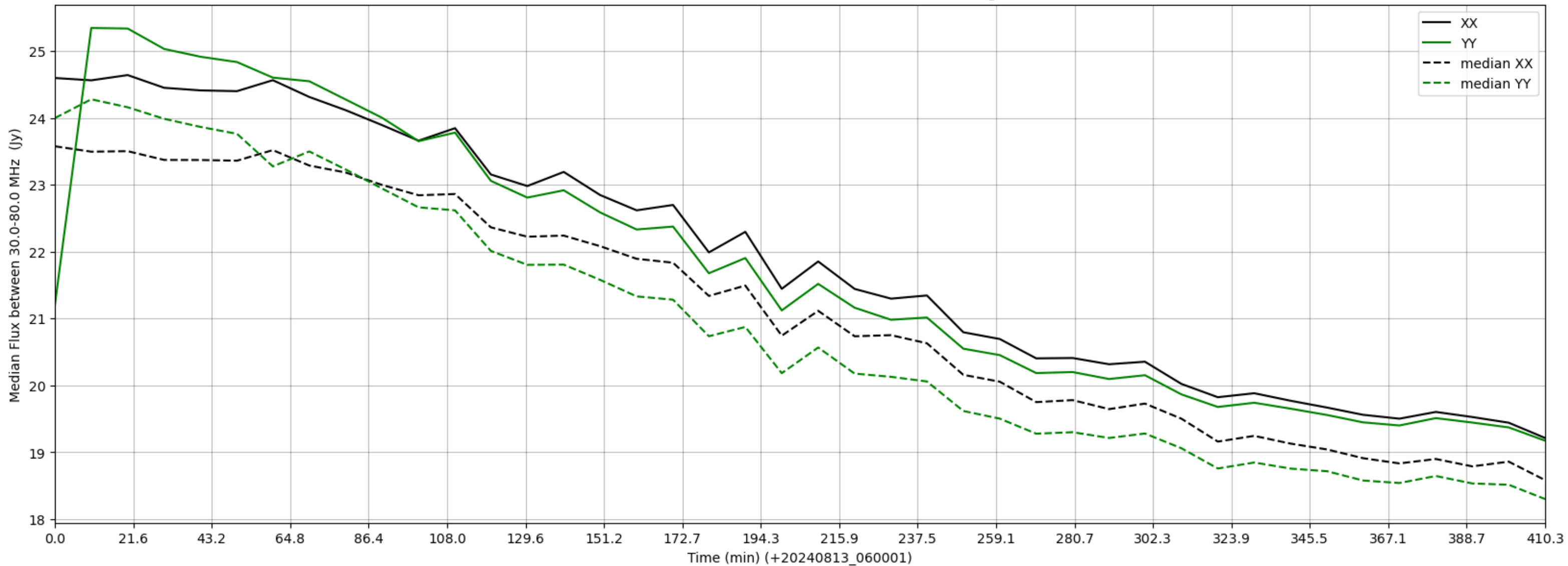
LWA248 - Correlator# 343 - XX FLAGS:Good - YY FLAGS:HighTimeVar
