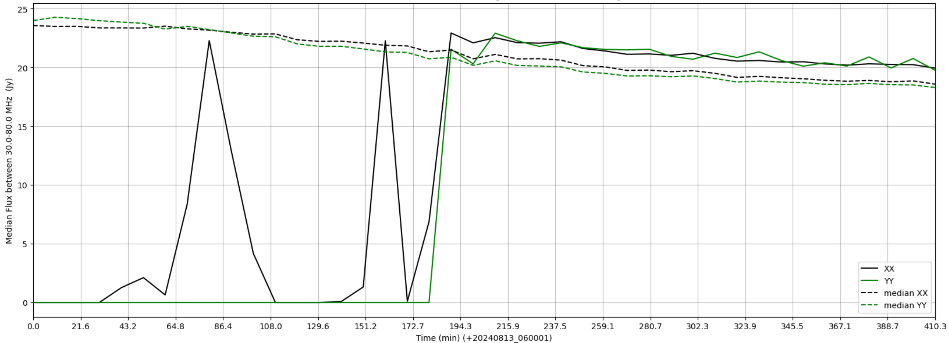
LWA009 - Correlator# 070 - XX FLAGS:HighTimeVar - YY FLAGS:HighTimeVar
