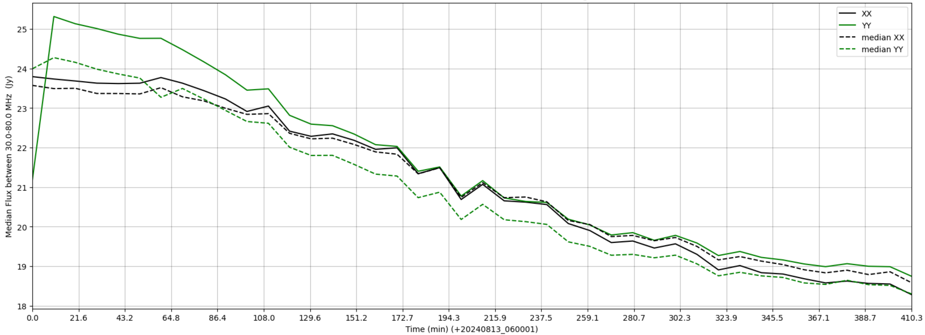
LWA062 - Correlator# 138 - XX FLAGS:Good - YY FLAGS:HighTimeVar
