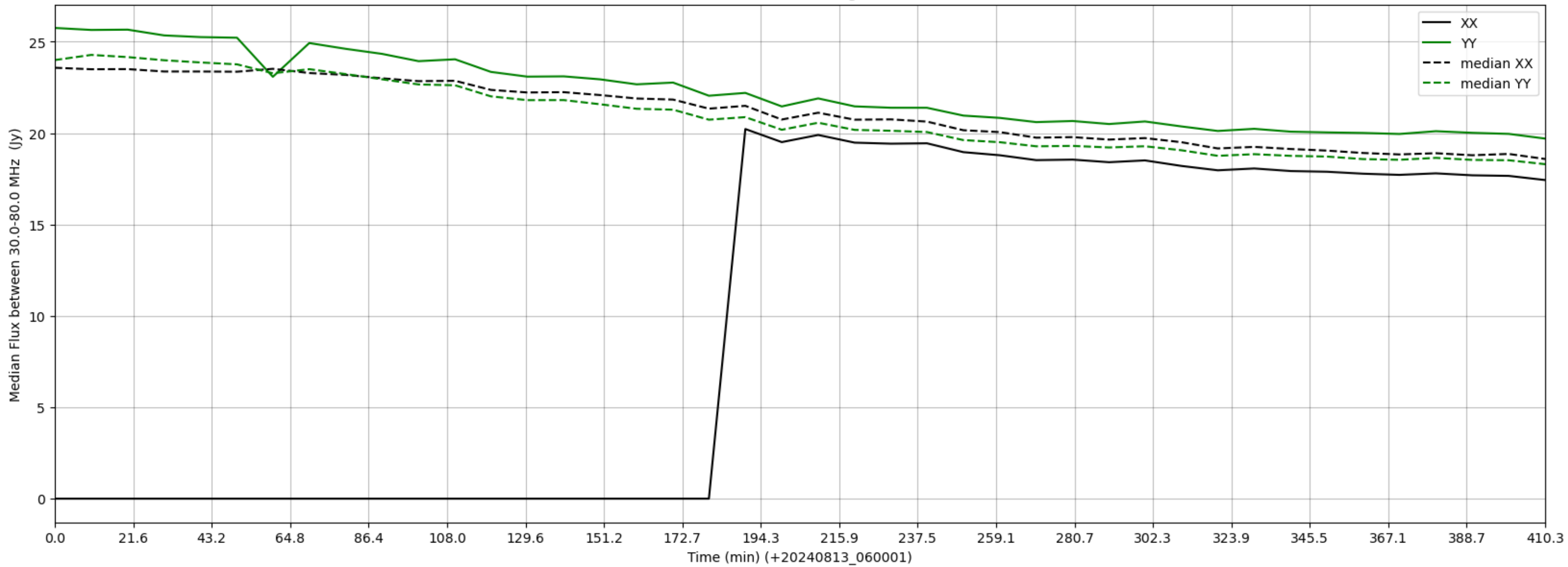
LWA046 - Correlator# 082 - XX FLAGS:HighTimeVar - YY FLAGS:Good
