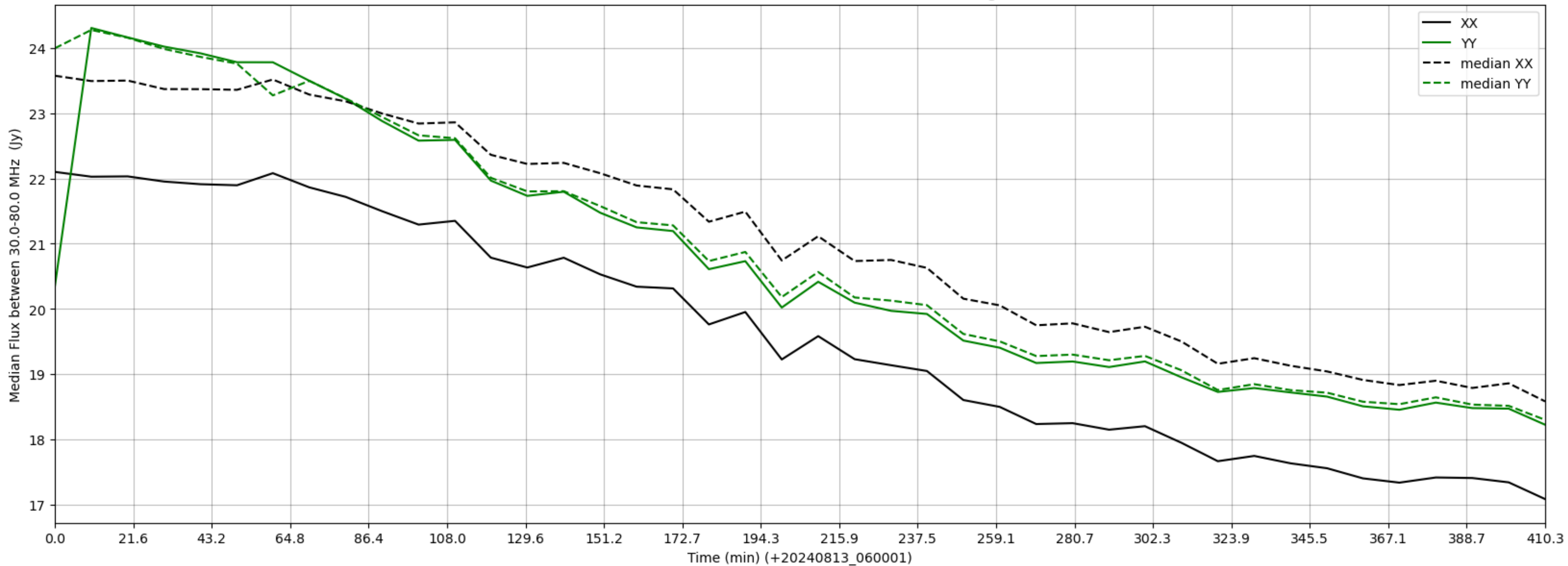
LWA245 - Correlator# 341 - XX FLAGS:Good - YY FLAGS:HighTimeVar
