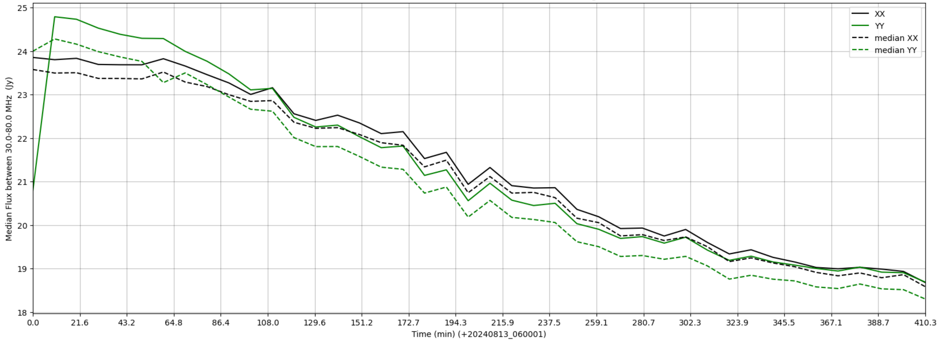
LWA093 - Correlator# 148 - XX FLAGS:Good - YY FLAGS:HighTimeVar
