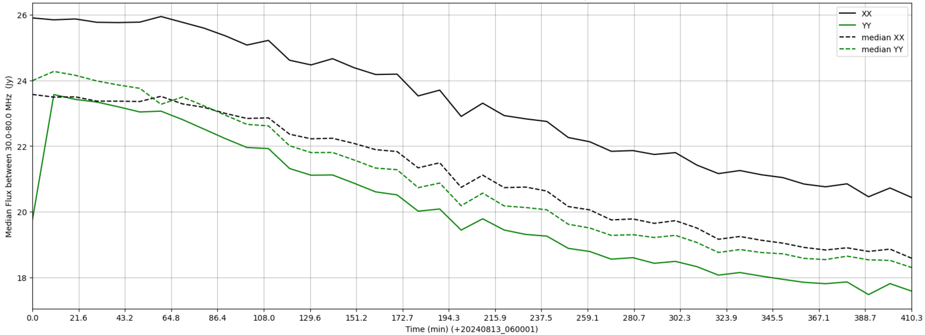
LWA125 - Correlator# 227 - XX FLAGS:Good - YY FLAGS:HighTimeVar
