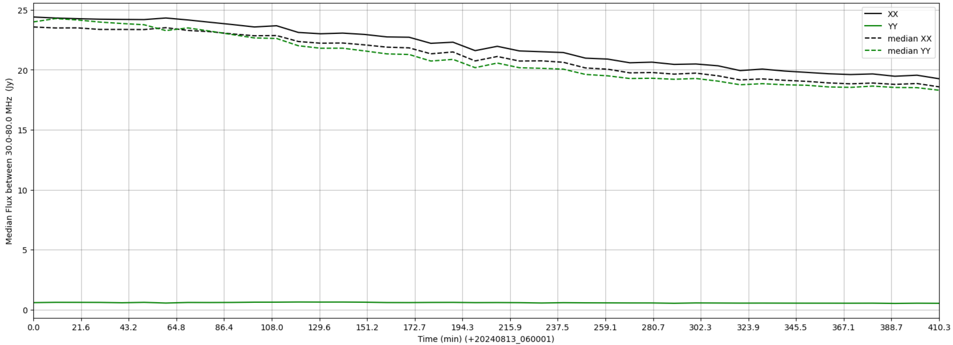
LWA105 - Correlator# 178 - XX FLAGS:Good - YY FLAGS:LowFlux
