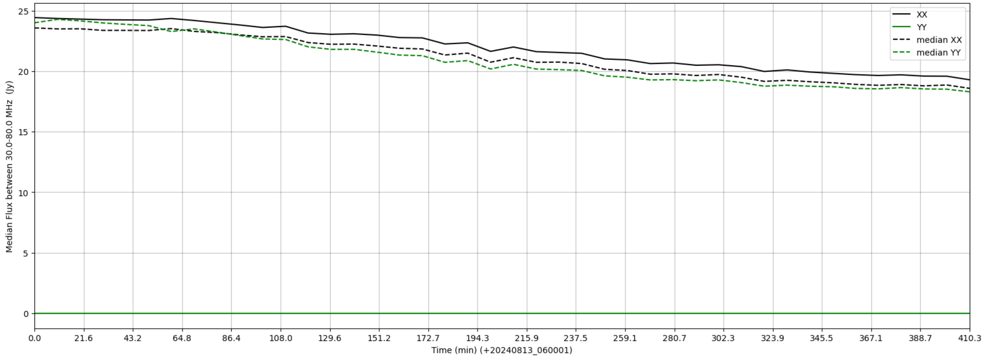
LWA051 - Correlator# 114 - XX FLAGS:Good - YY FLAGS:LowFlux
