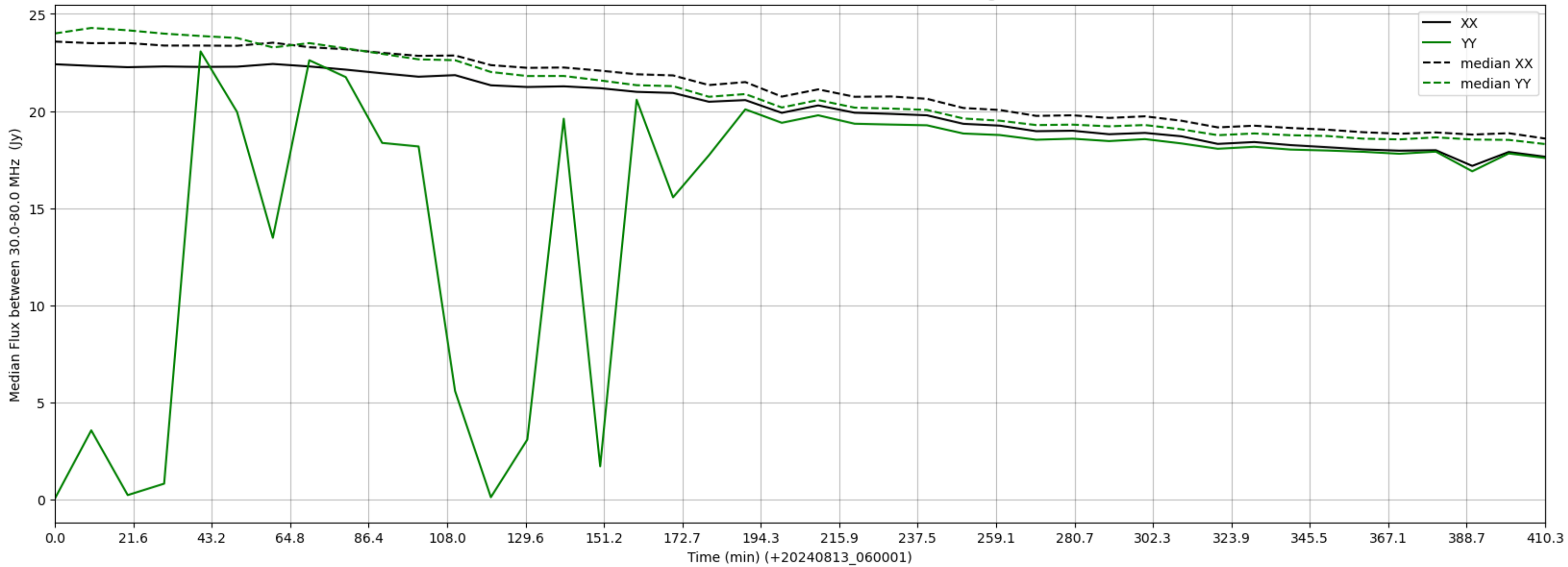
LWA112 - Correlator# 200 - XX FLAGS:Good - YY FLAGS:HighTimeVar
