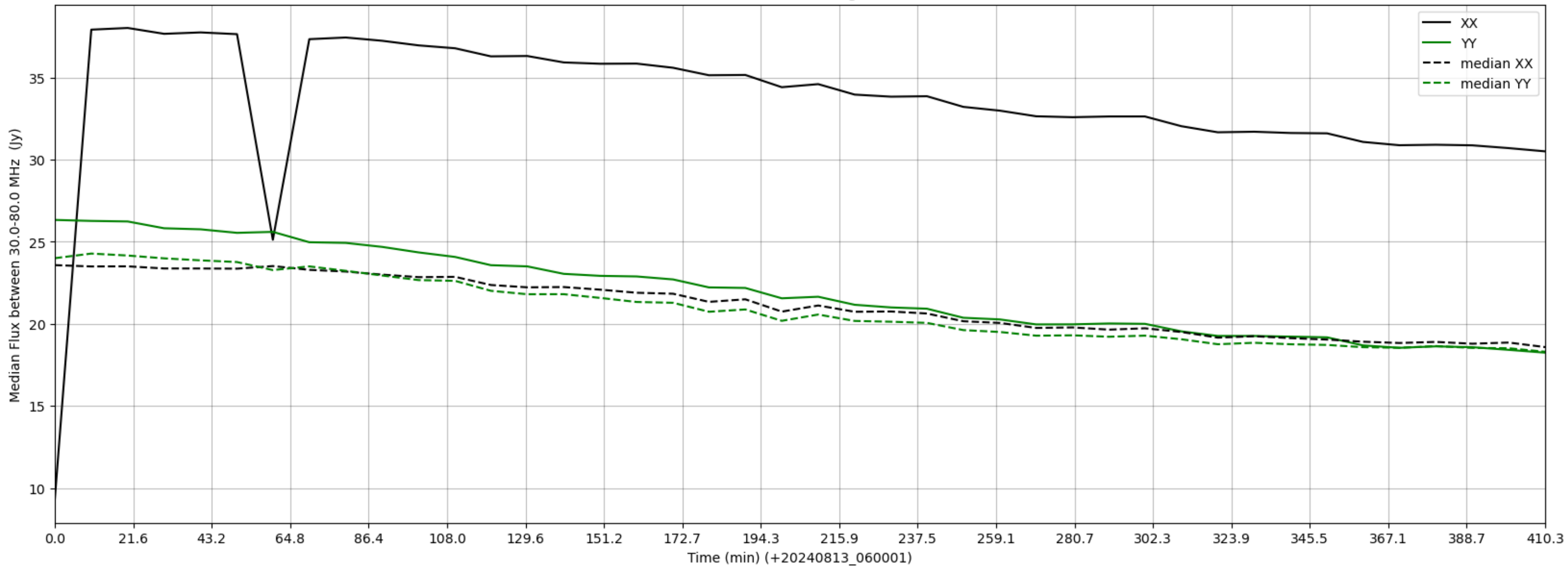
LWA286 - Correlator# 093 - XX FLAGS:HighTimeVar - YY FLAGS:Good
