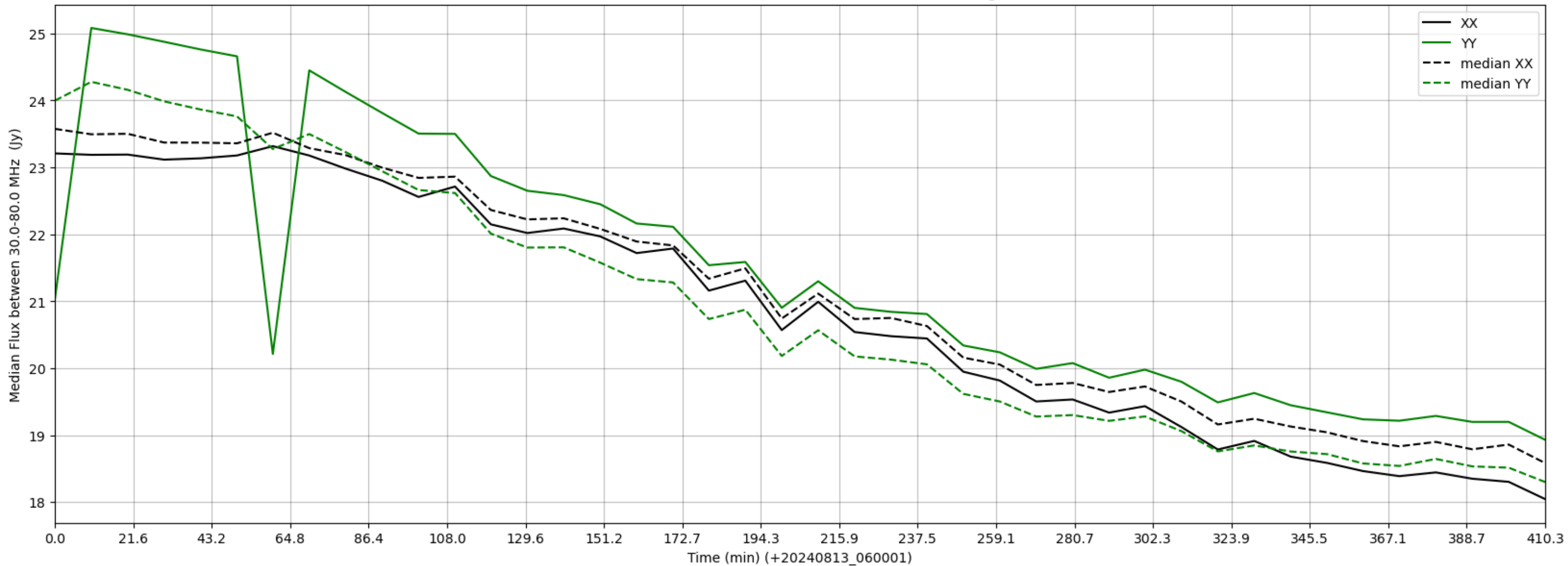
LWA016 - Correlator# 097 - XX FLAGS:Good - YY FLAGS:HighTimeVar
