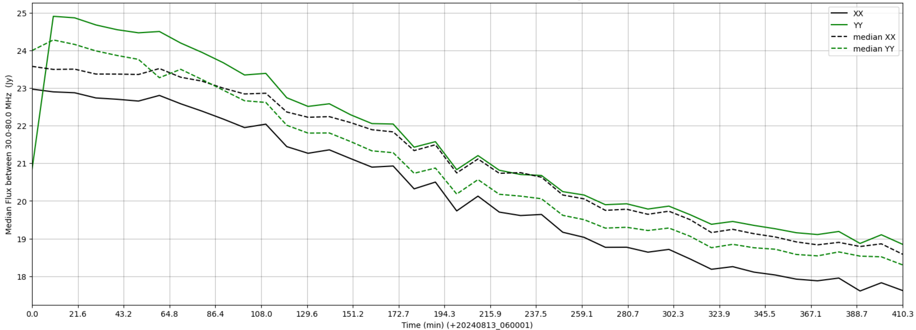
LWA182 - Correlator# 238 - XX FLAGS:Good - YY FLAGS:HighTimeVar
