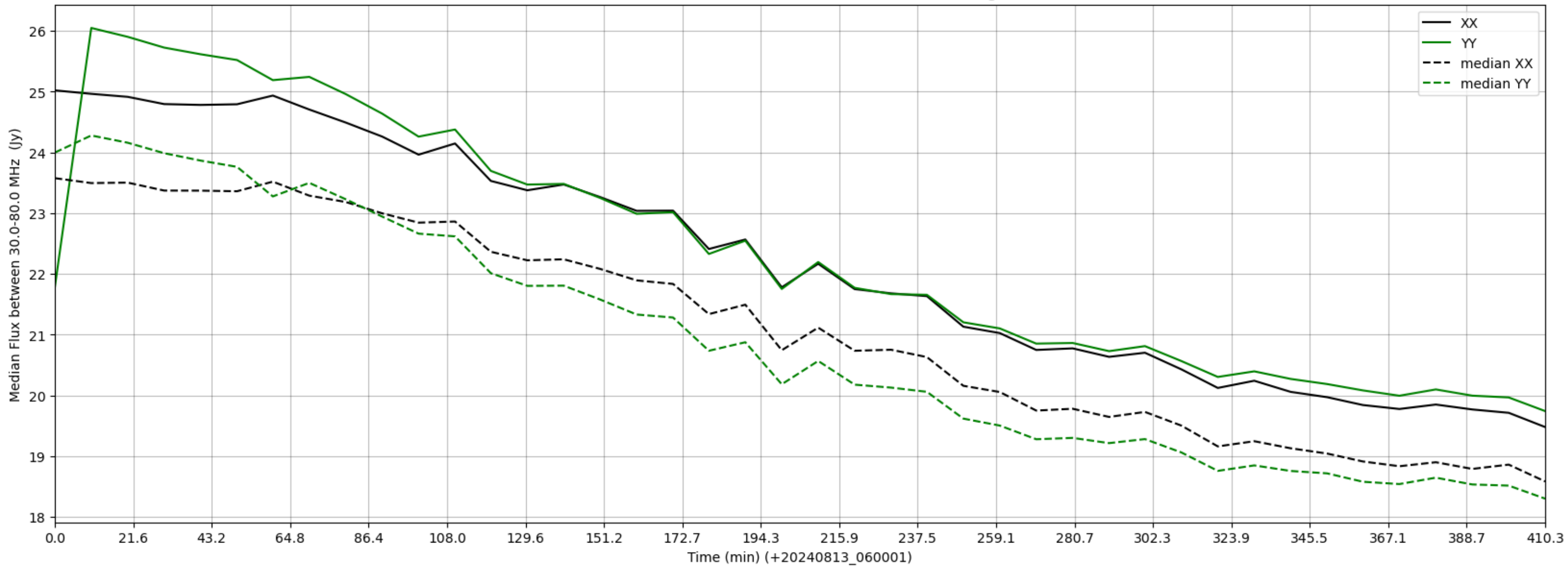
LWA176 - Correlator# 325 - XX FLAGS:Good - YY FLAGS:HighTimeVar
