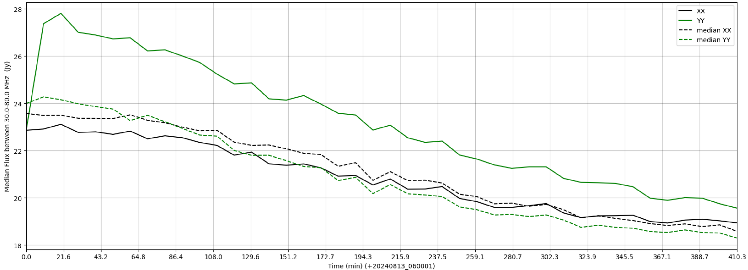
LWA348 - Correlator# 124 - XX FLAGS:BadSpecShape - YY FLAGS:HighTimeVar
