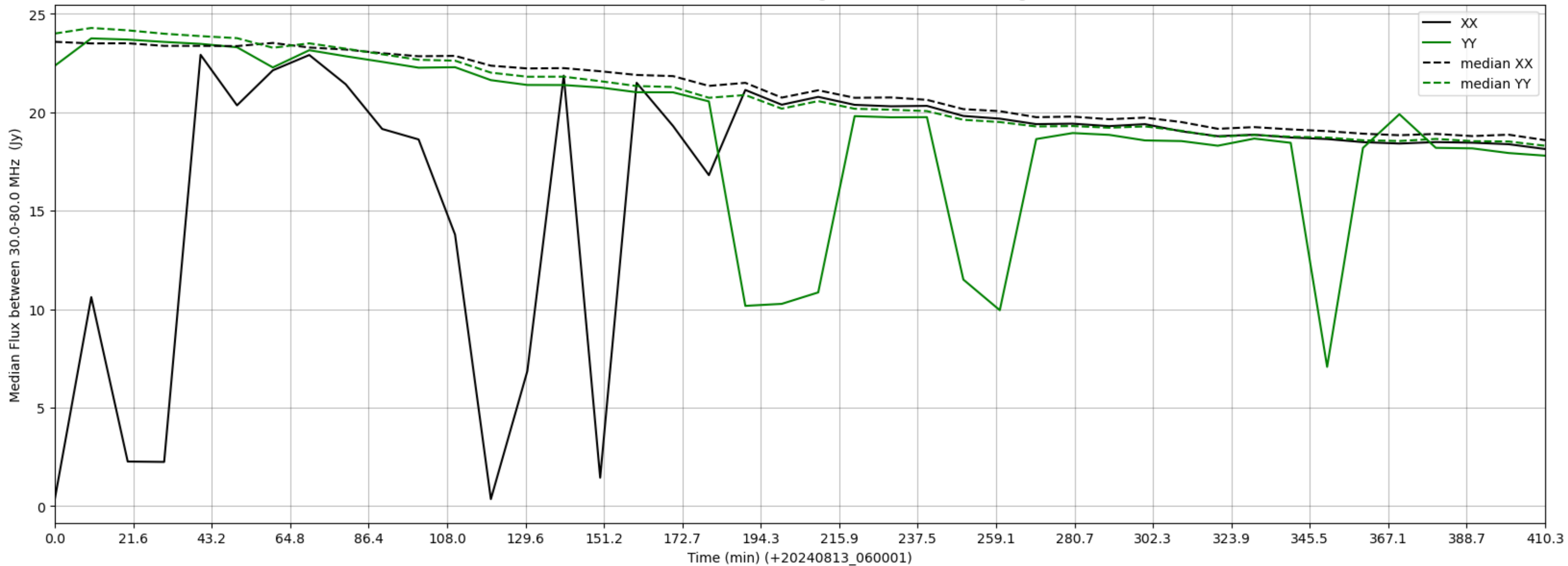
LWA043 - Correlator# 081 - XX FLAGS:HighTimeVar - YY FLAGS:HighTimeVar
