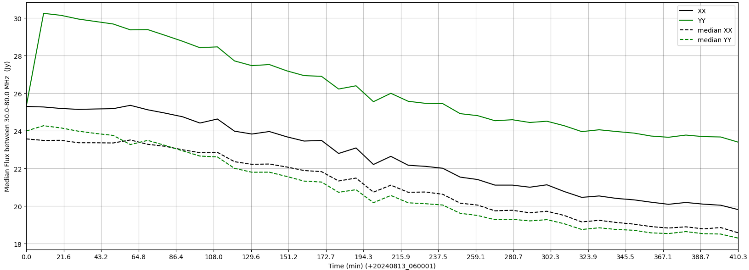
LWA246 - Correlator# 340 - XX FLAGS:Good - YY FLAGS:HighTimeVar
