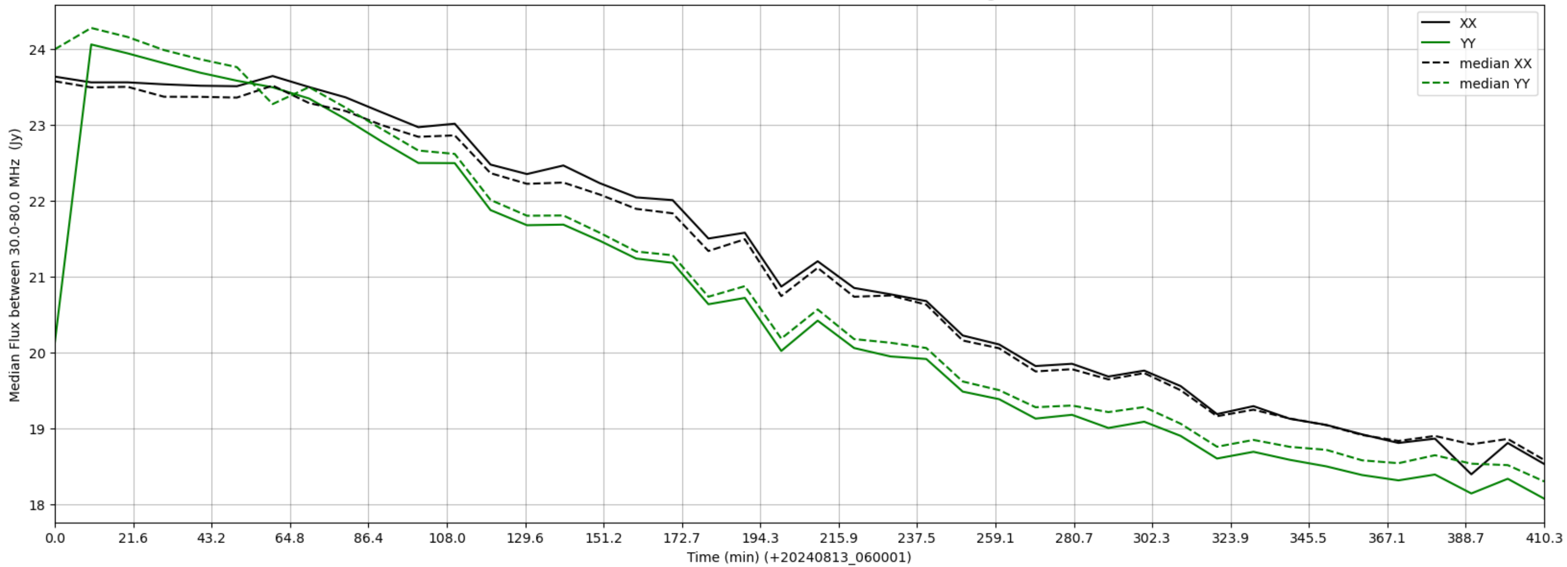
LWA149 - Correlator# 216 - XX FLAGS:Good - YY FLAGS:HighTimeVar
