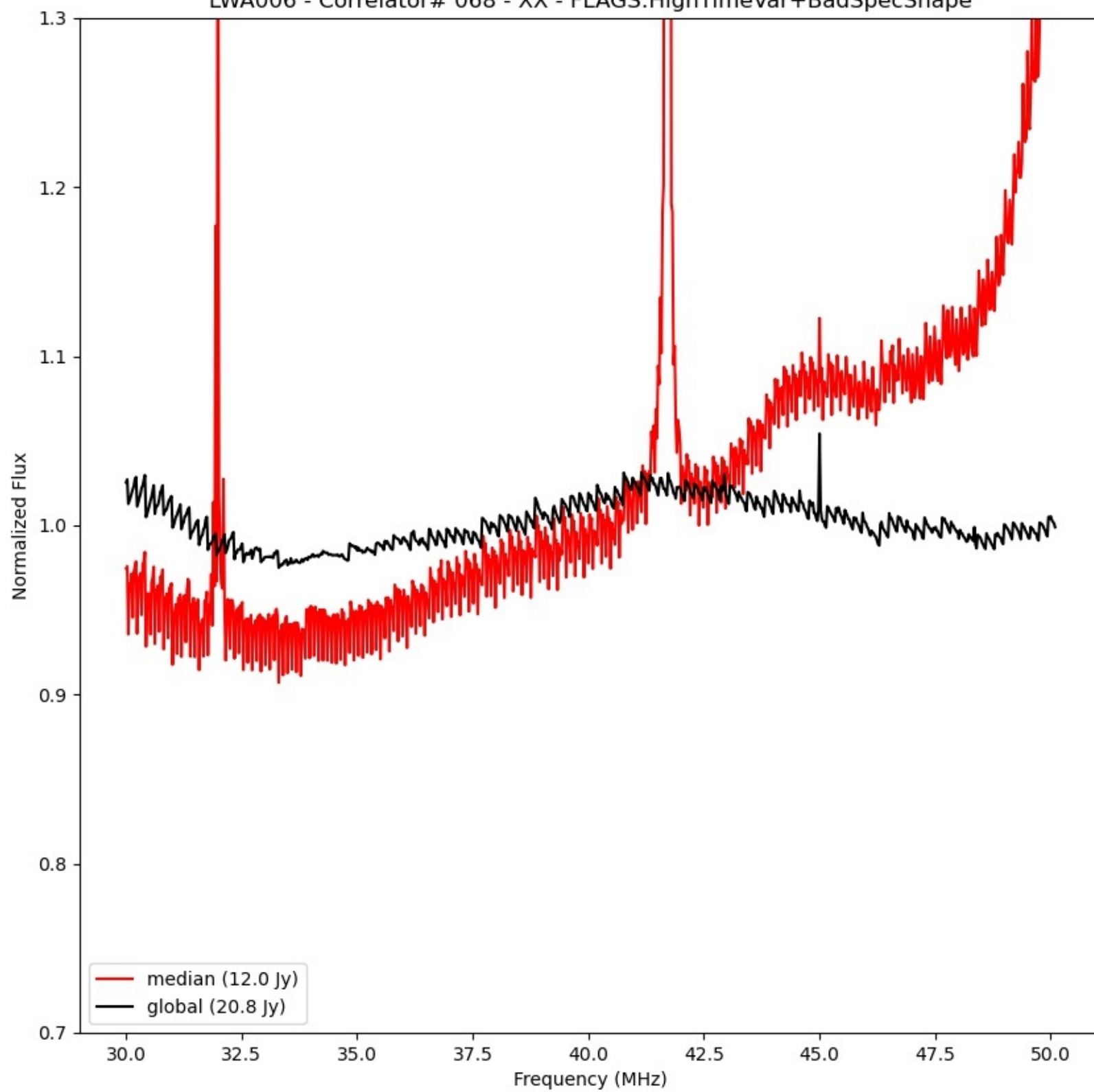
LWA006 - Correlator# 068 - XX - FLAGS:HighTimeVar+BadSpecShape
