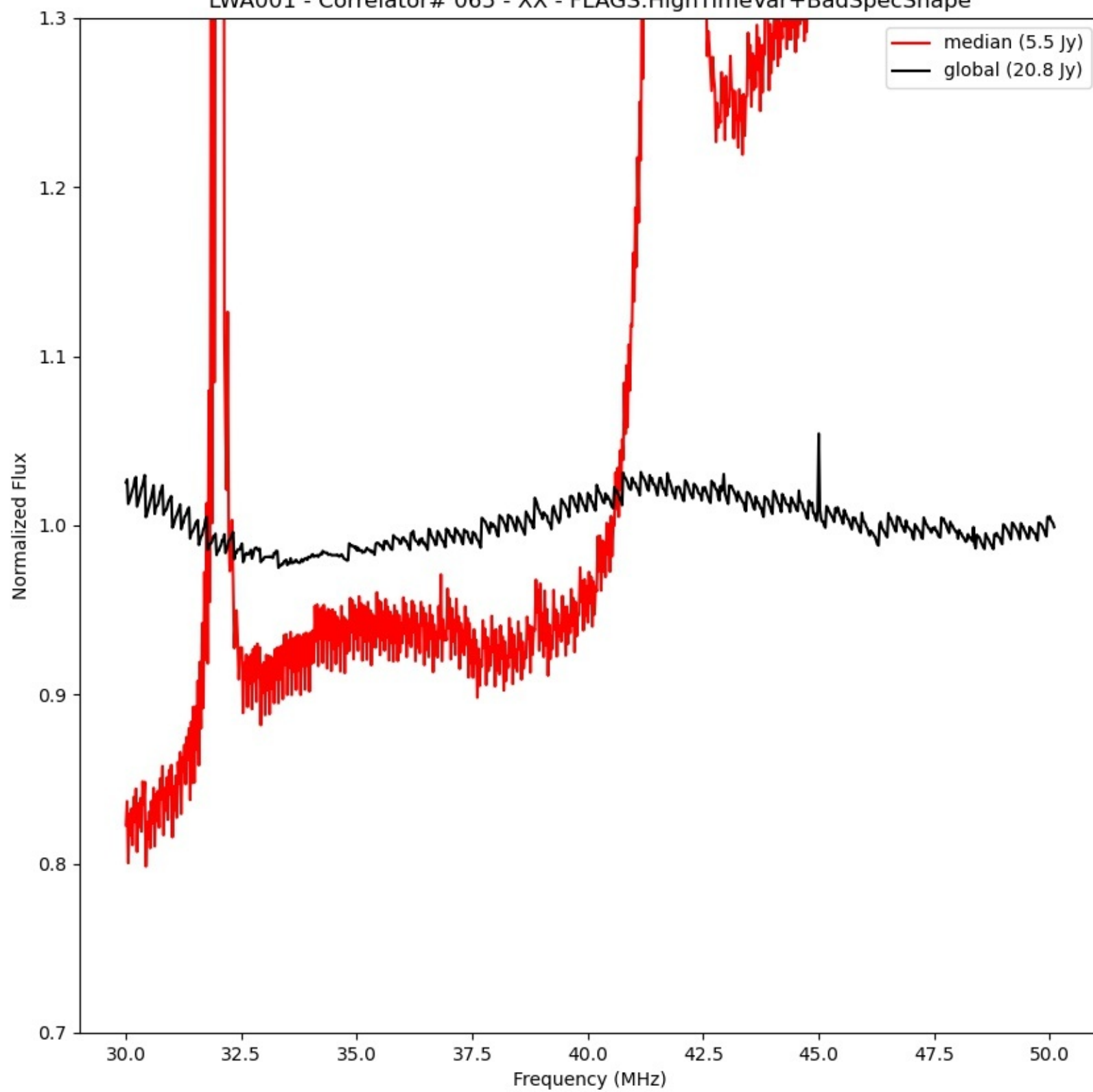
LWA001 - Correlator# 065 - XX - FLAGS:HighTimeVar+BadSpecShape
