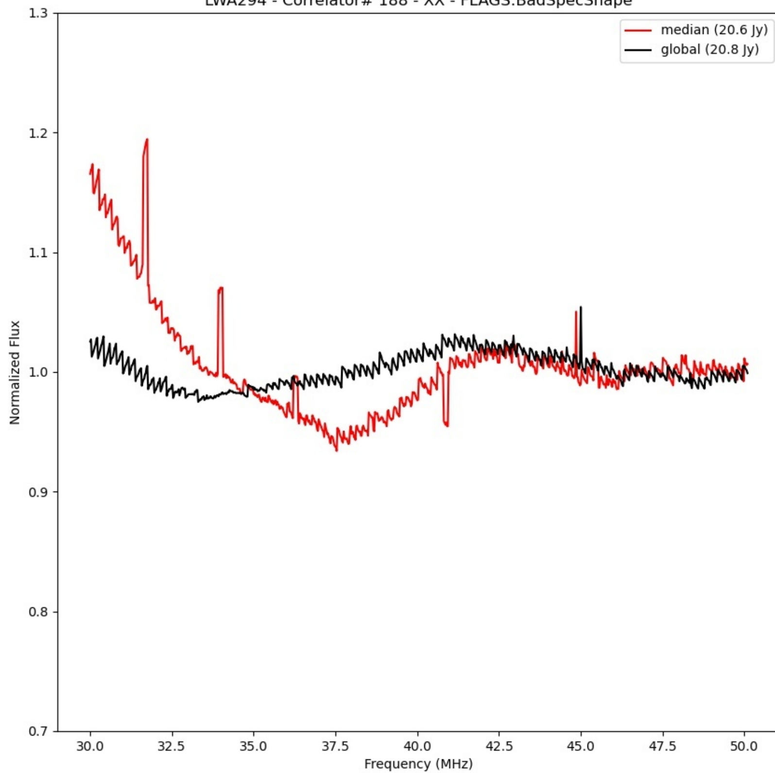
LWA294 - Correlator# 188 - XX - FLAGS:BadSpecShape
