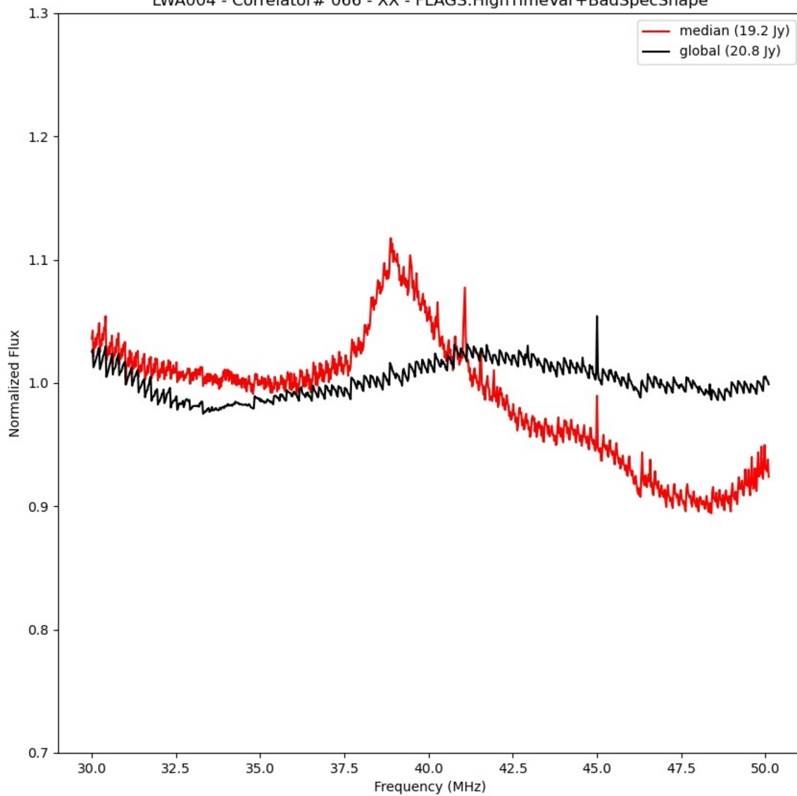
LWA004 - Correlator# 066 - XX - FLAGS:HighTimeVar+BadSpecShape
