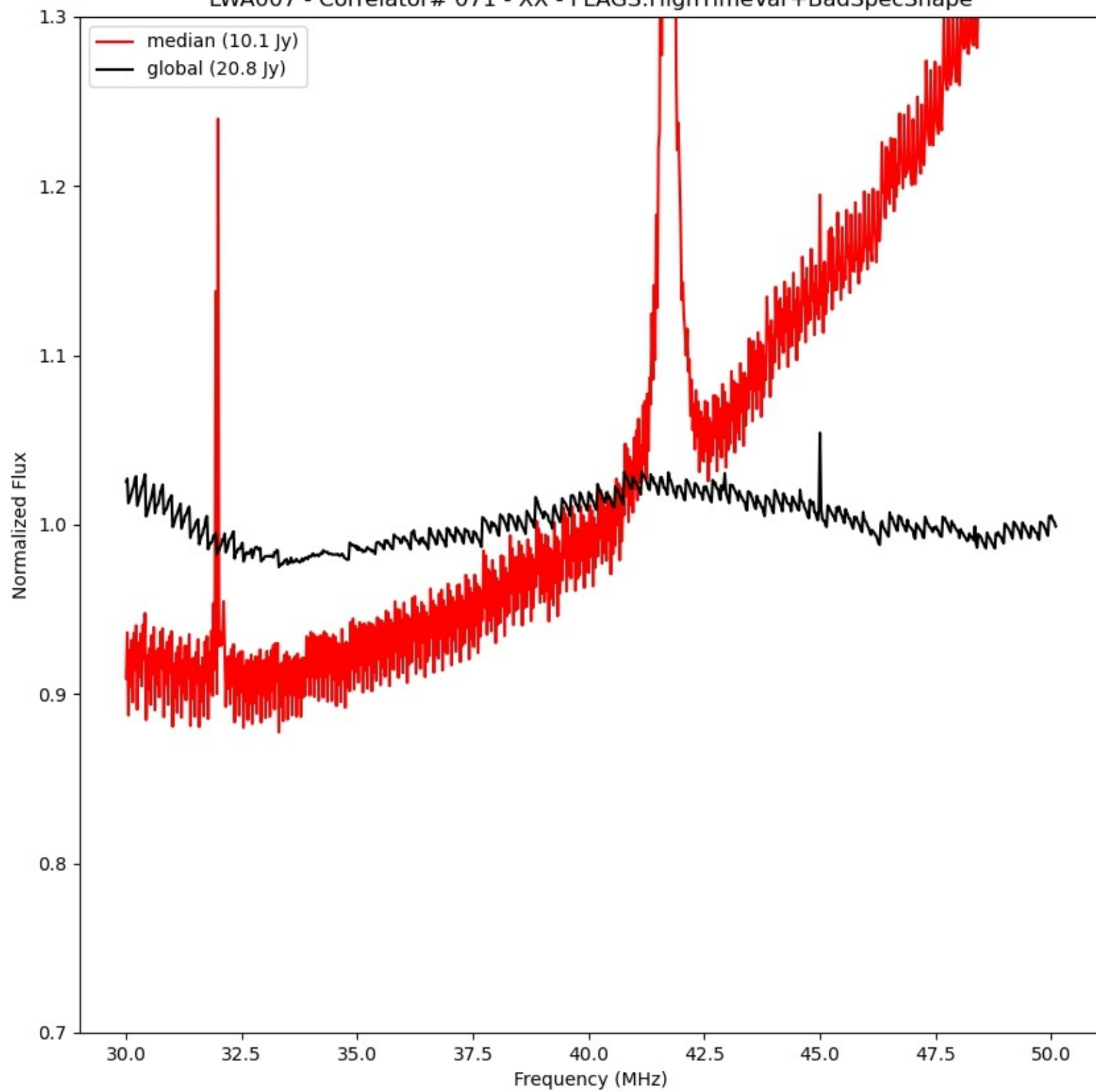
LWA007 - Correlator# 071 - XX - FLAGS:HighTimeVar+BadSpecShape
