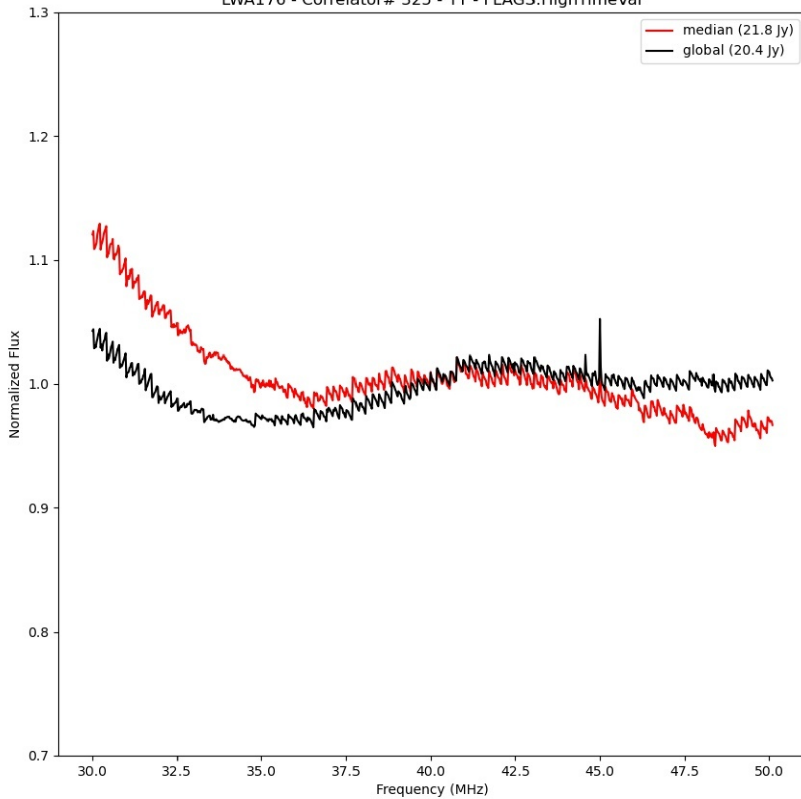
LWA176 - Correlator# 325 - YY - FLAGS:HighTimeVar
