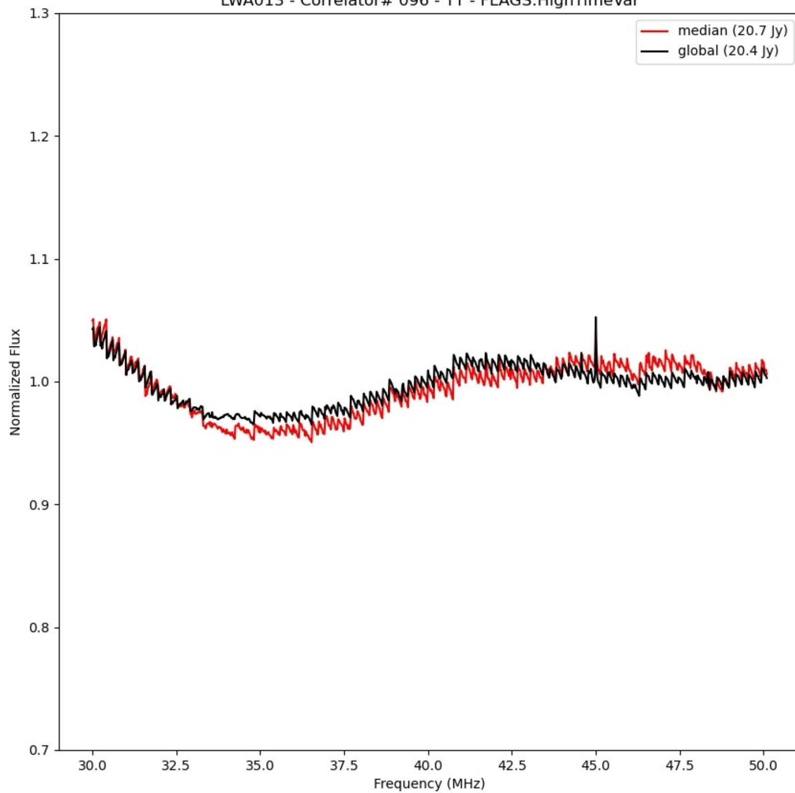
LWA013 - Correlator# 096 - YY - FLAGS:HighTimeVar
