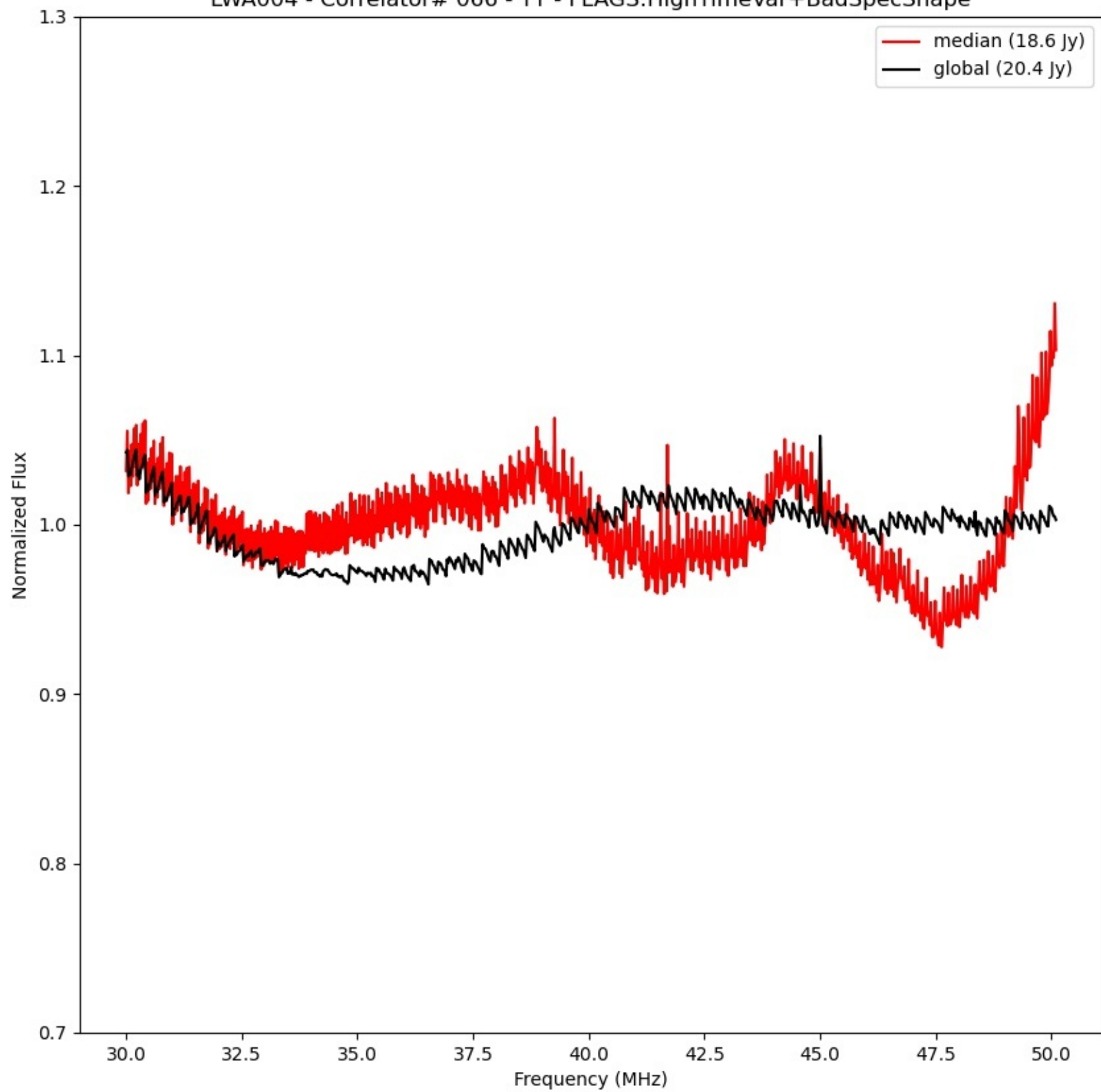
LWA004 - Correlator# 066 - YY - FLAGS:HighTimeVar+BadSpecShape
