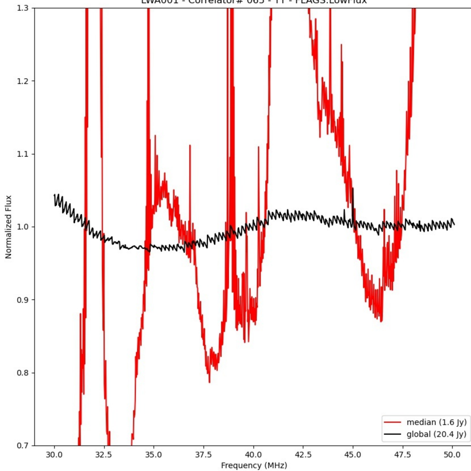
LWA001 - Correlator# 065 - YY - FLAGS:LowFlux
