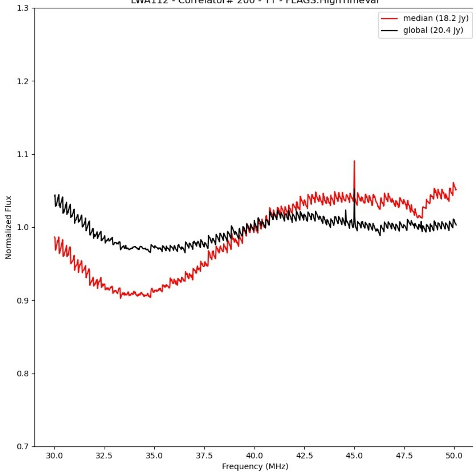
LWA112 - Correlator# 200 - YY - FLAGS:HighTimeVar
