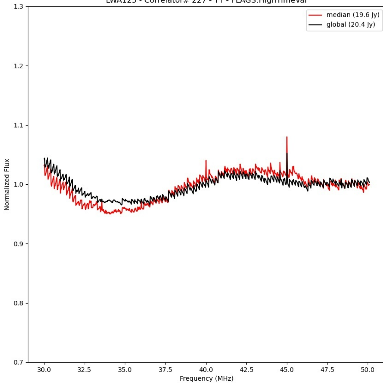
LWA125 - Correlator# 227 - YY - FLAGS:HighTimeVar
