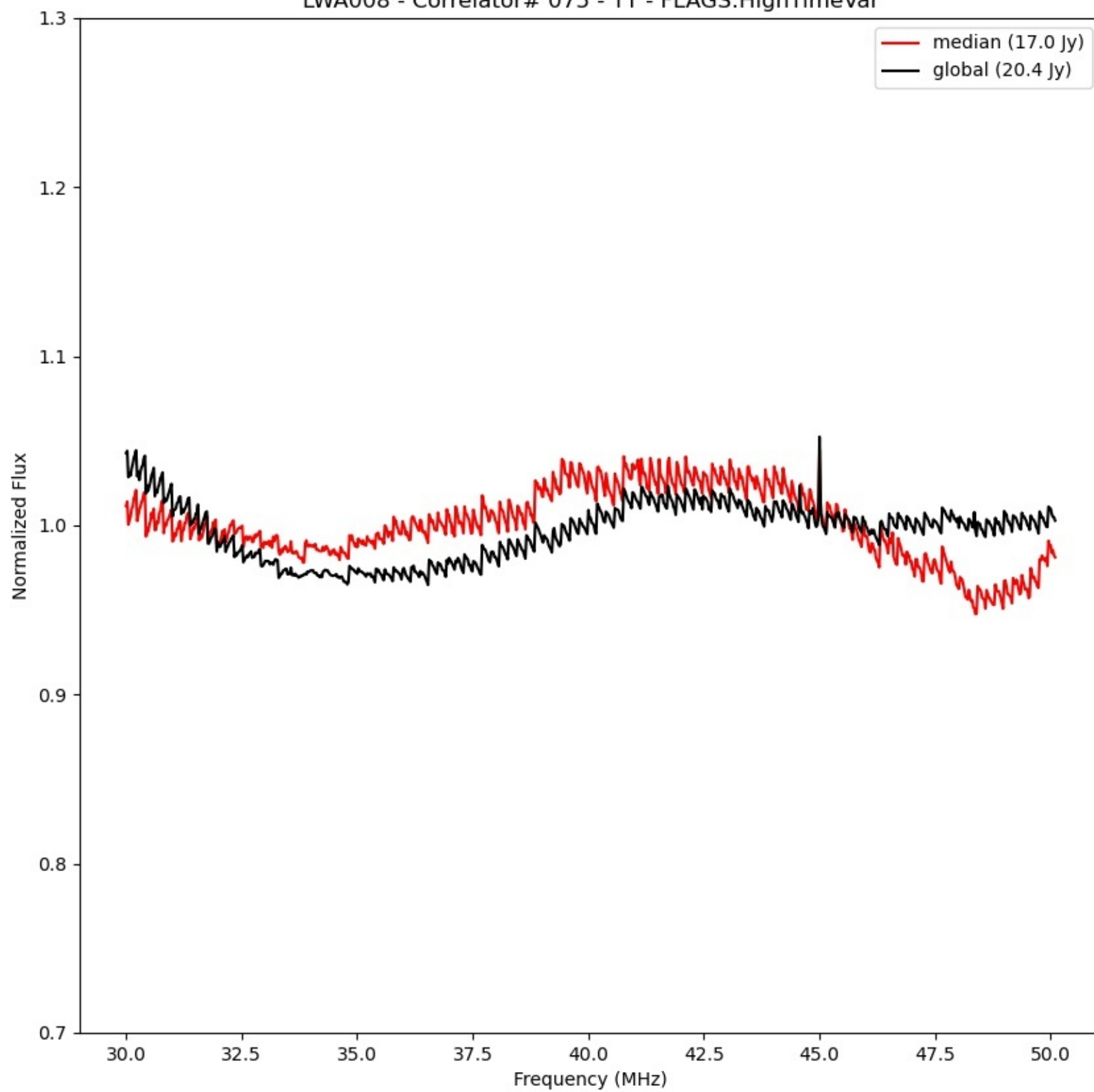
LWA008 - Correlator# 075 - YY - FLAGS:HighTimeVar
