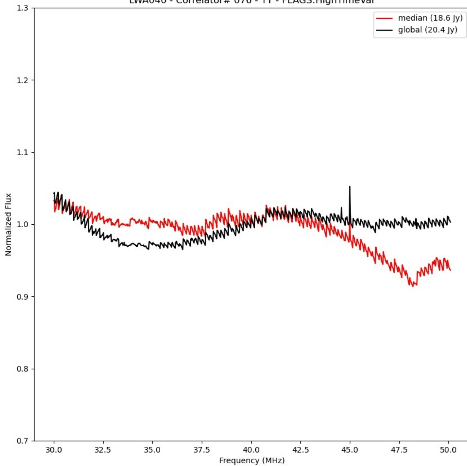
LWA040 - Correlator# 076 - YY - FLAGS:HighTimeVar
