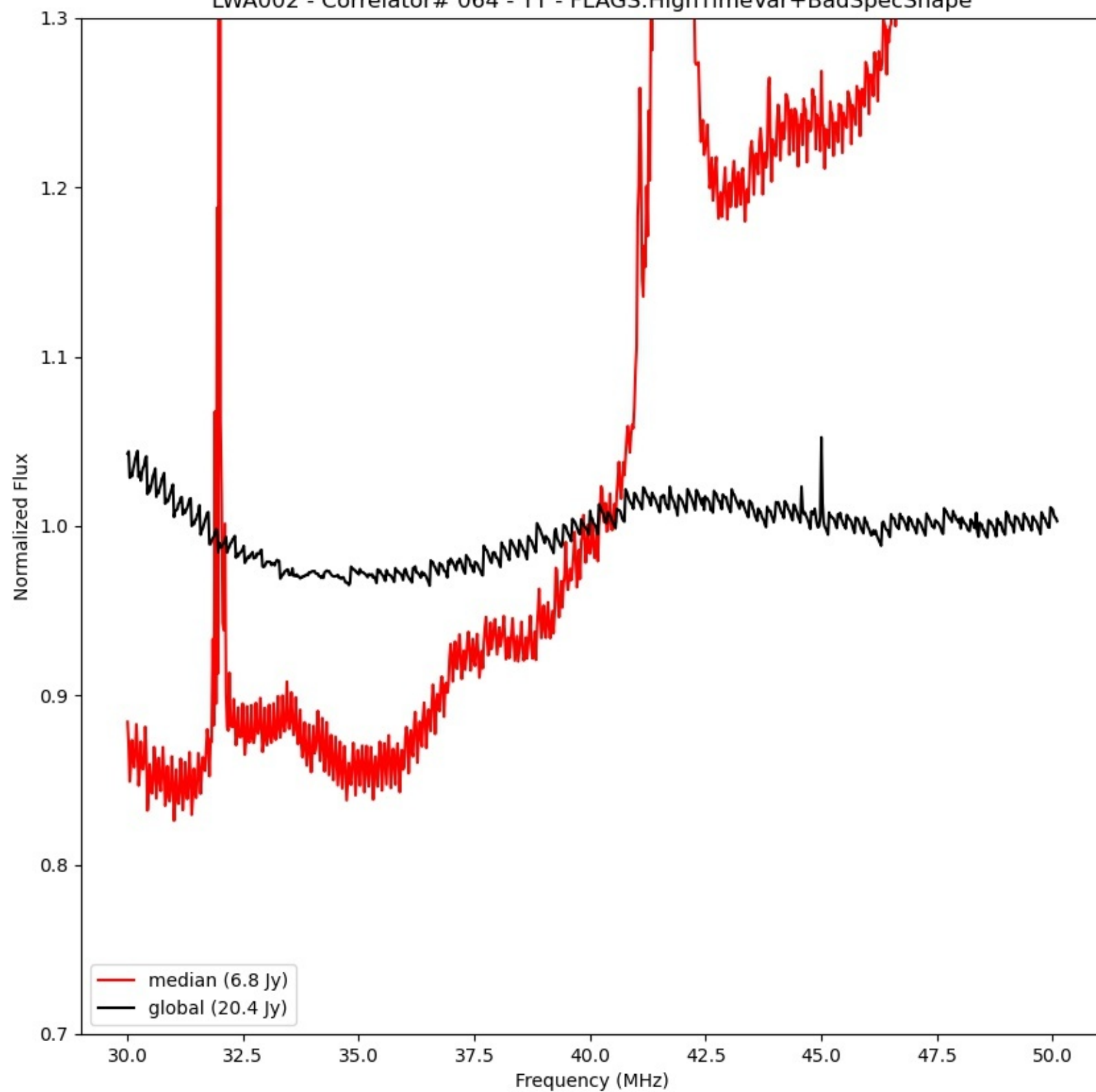
LWA002 - Correlator# 064 - YY - FLAGS:HighTimeVar+BadSpecShape
