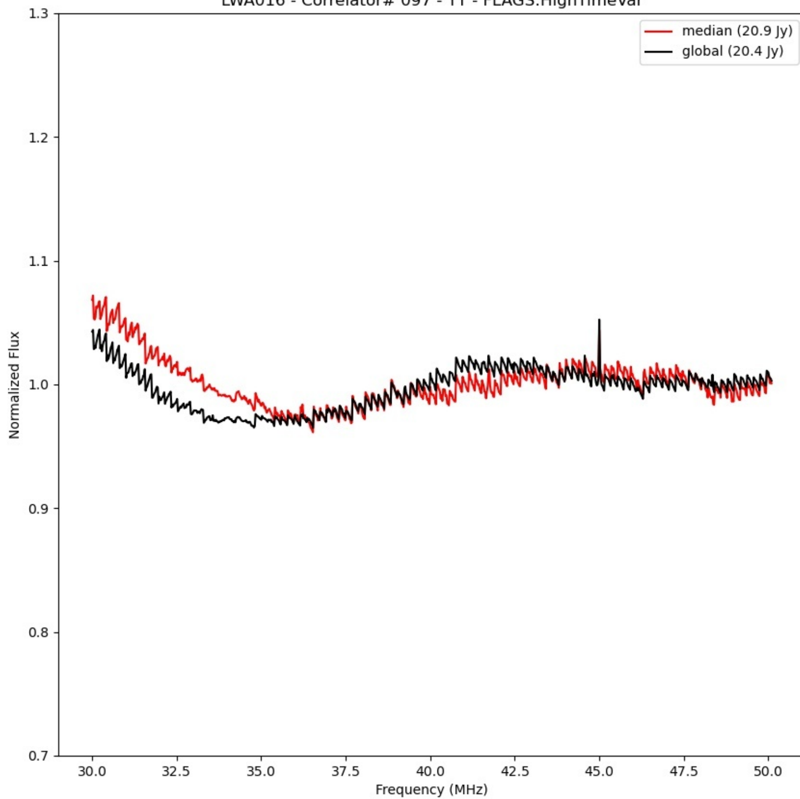
LWA016 - Correlator# 097 - YY - FLAGS:HighTimeVar
