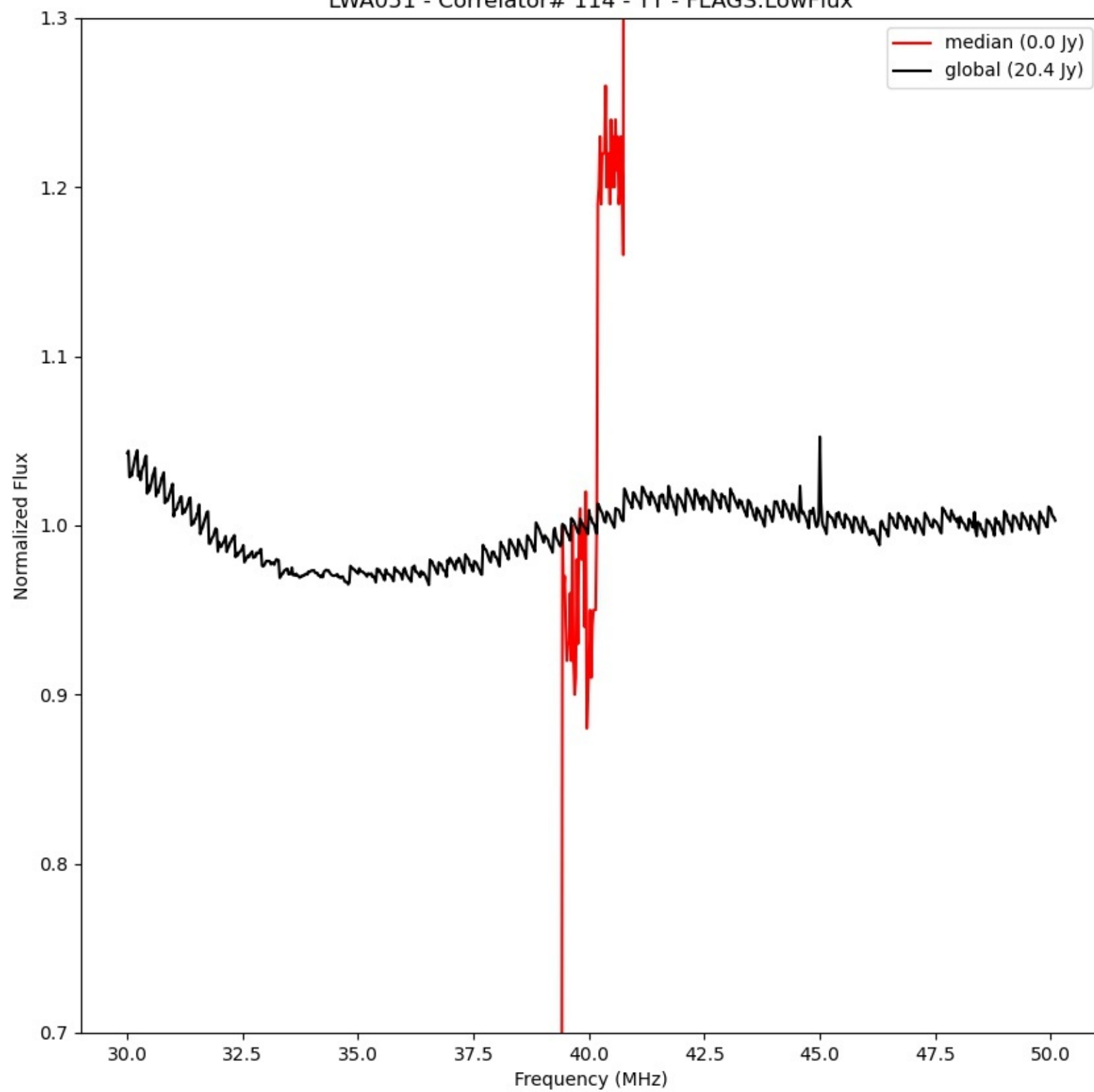
LWA051 - Correlator# 114 - YY - FLAGS:LowFlux
