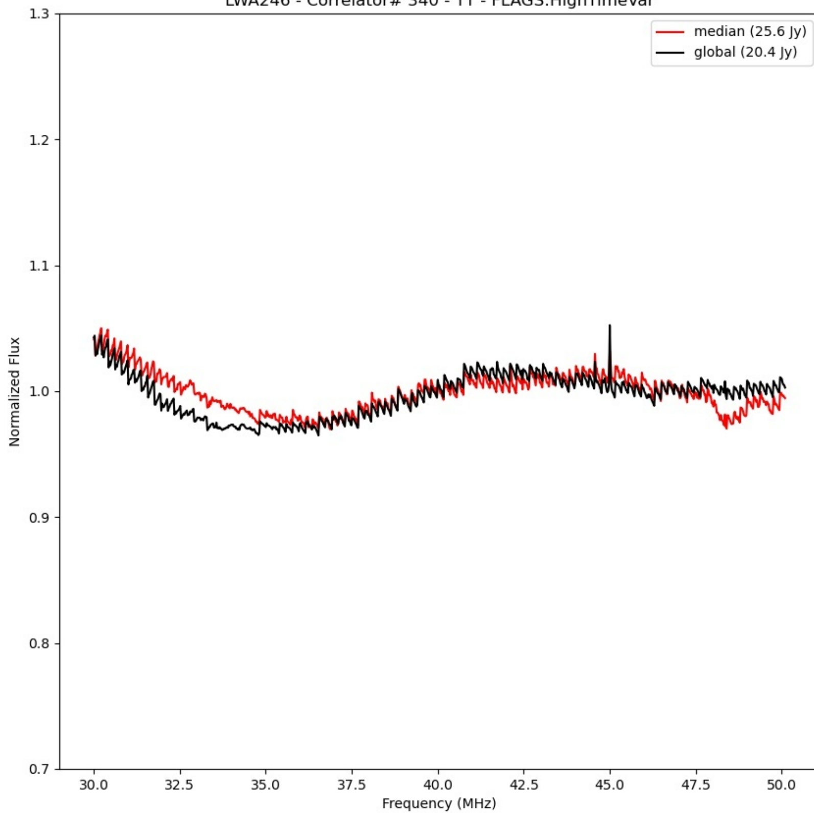
LWA246 - Correlator# 340 - YY - FLAGS:HighTimeVar
