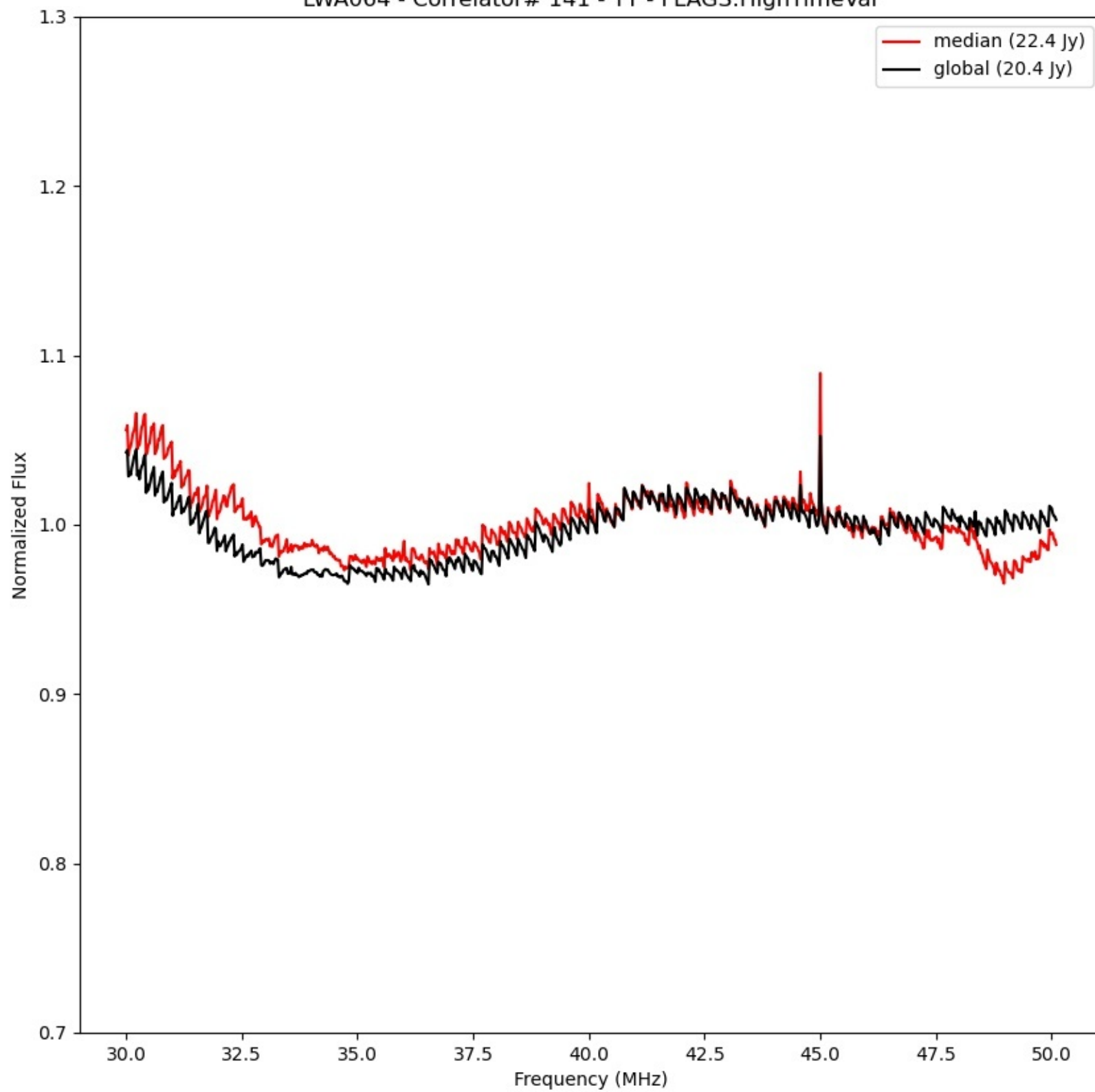
LWA064 - Correlator# 141 - YY - FLAGS:HighTimeVar
