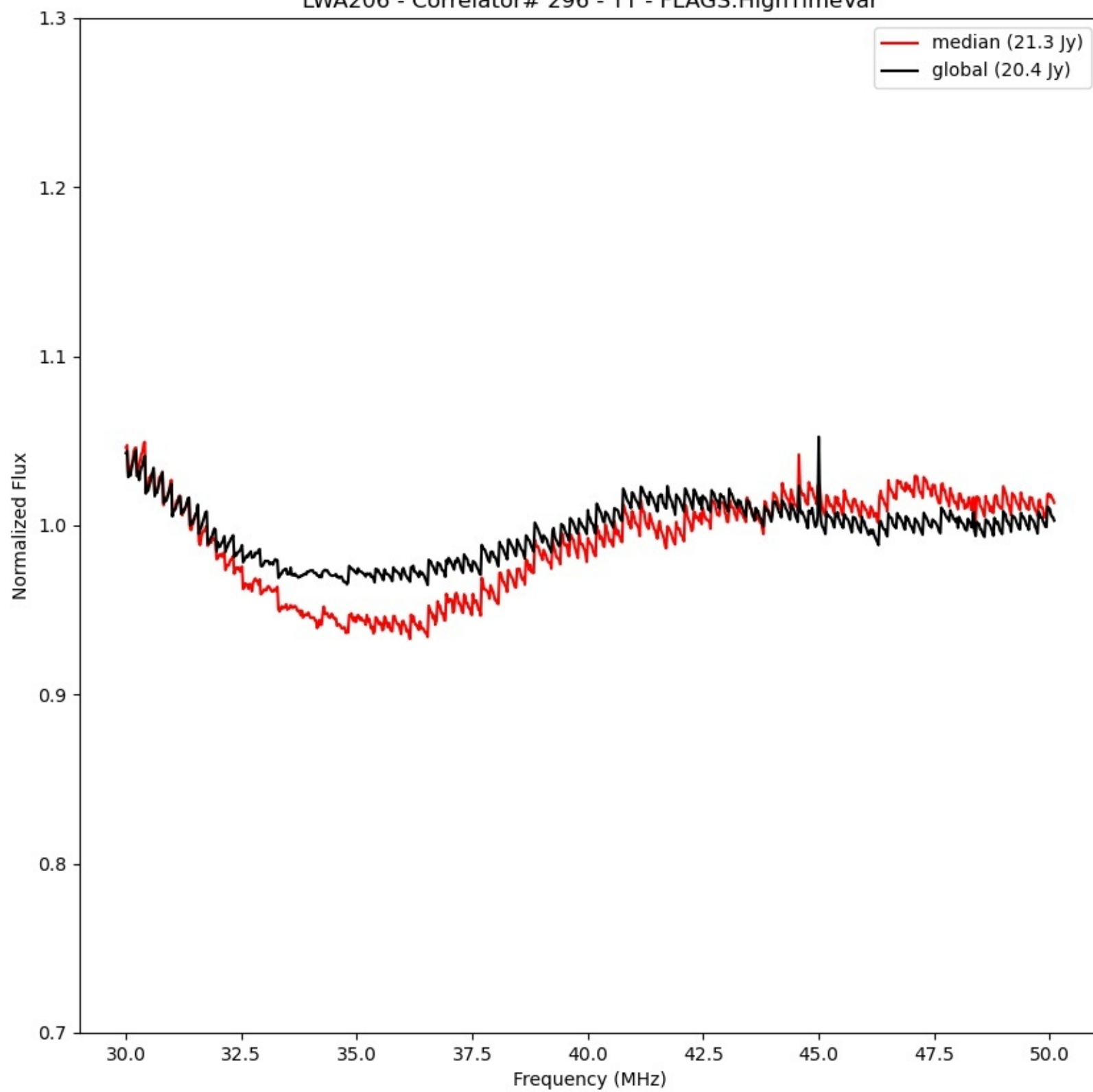
LWA206 - Correlator# 296 - YY - FLAGS:HighTimeVar
