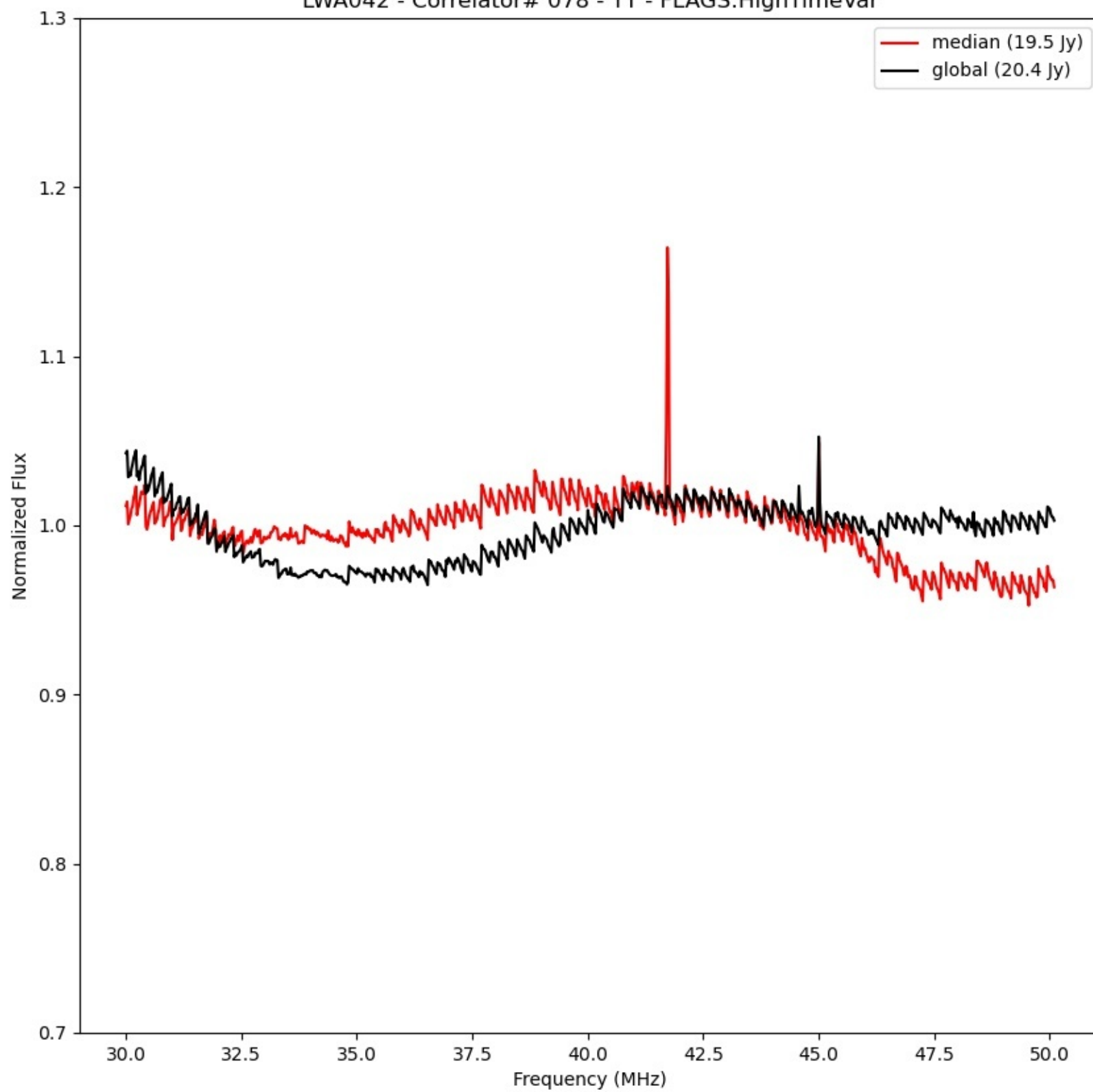
LWA042 - Correlator# 078 - YY - FLAGS:HighTimeVar
