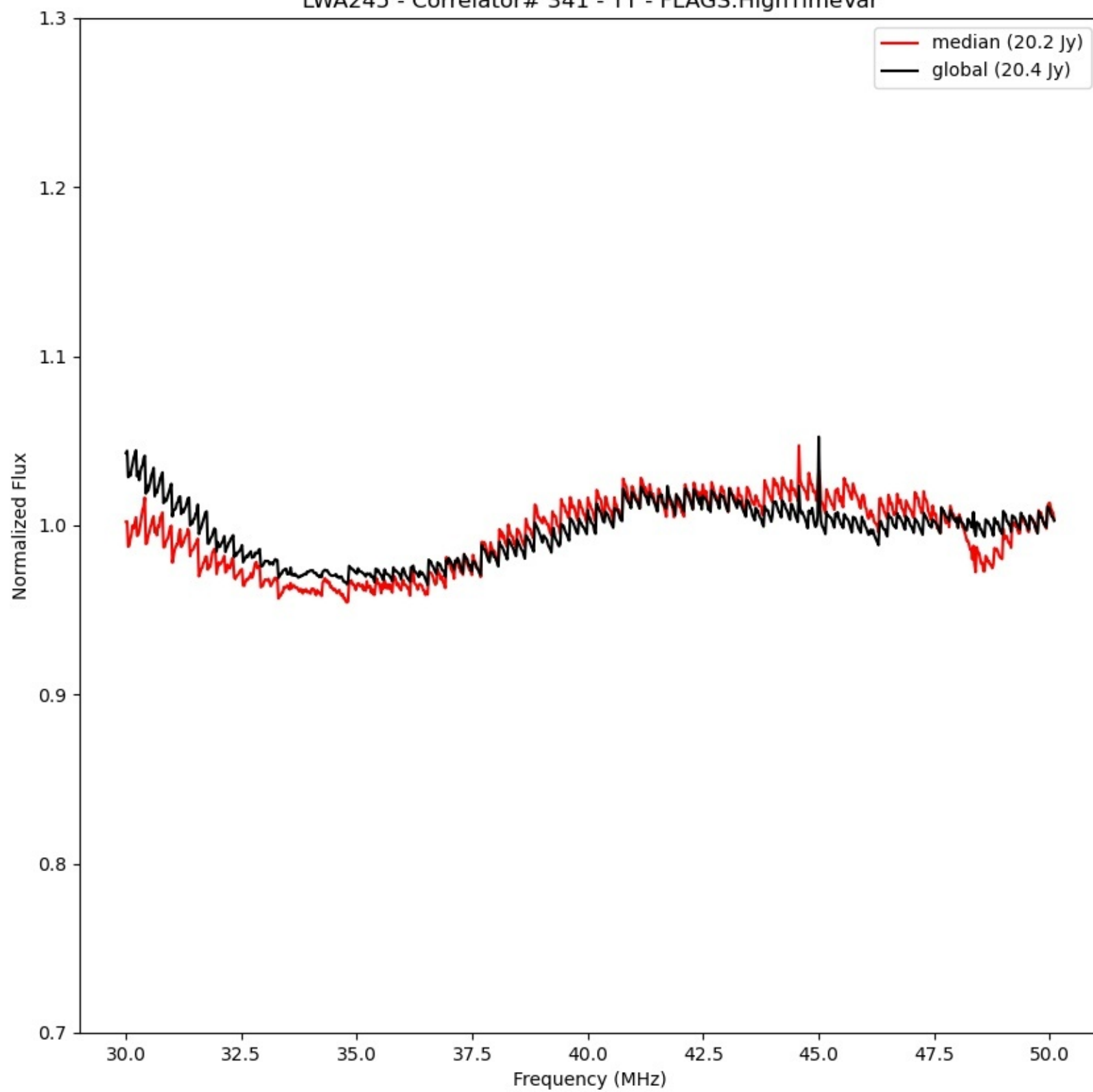
LWA245 - Correlator# 341 - YY - FLAGS:HighTimeVar
