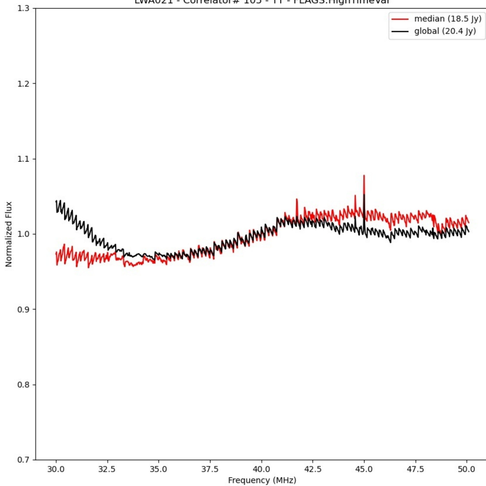
LWA021 - Correlator# 105 - YY - FLAGS:HighTimeVar
