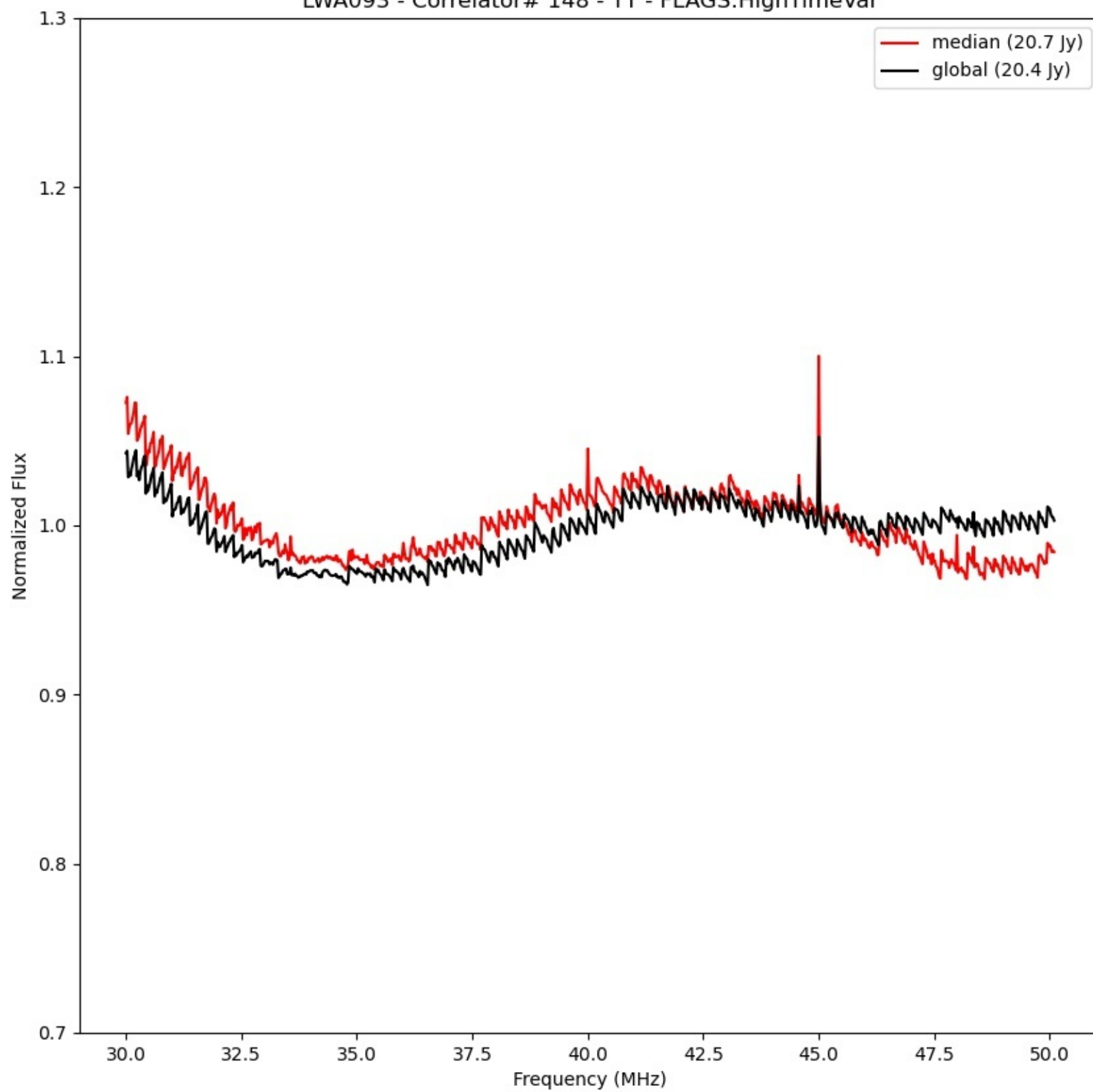
LWA093 - Correlator# 148 - YY - FLAGS:HighTimeVar
