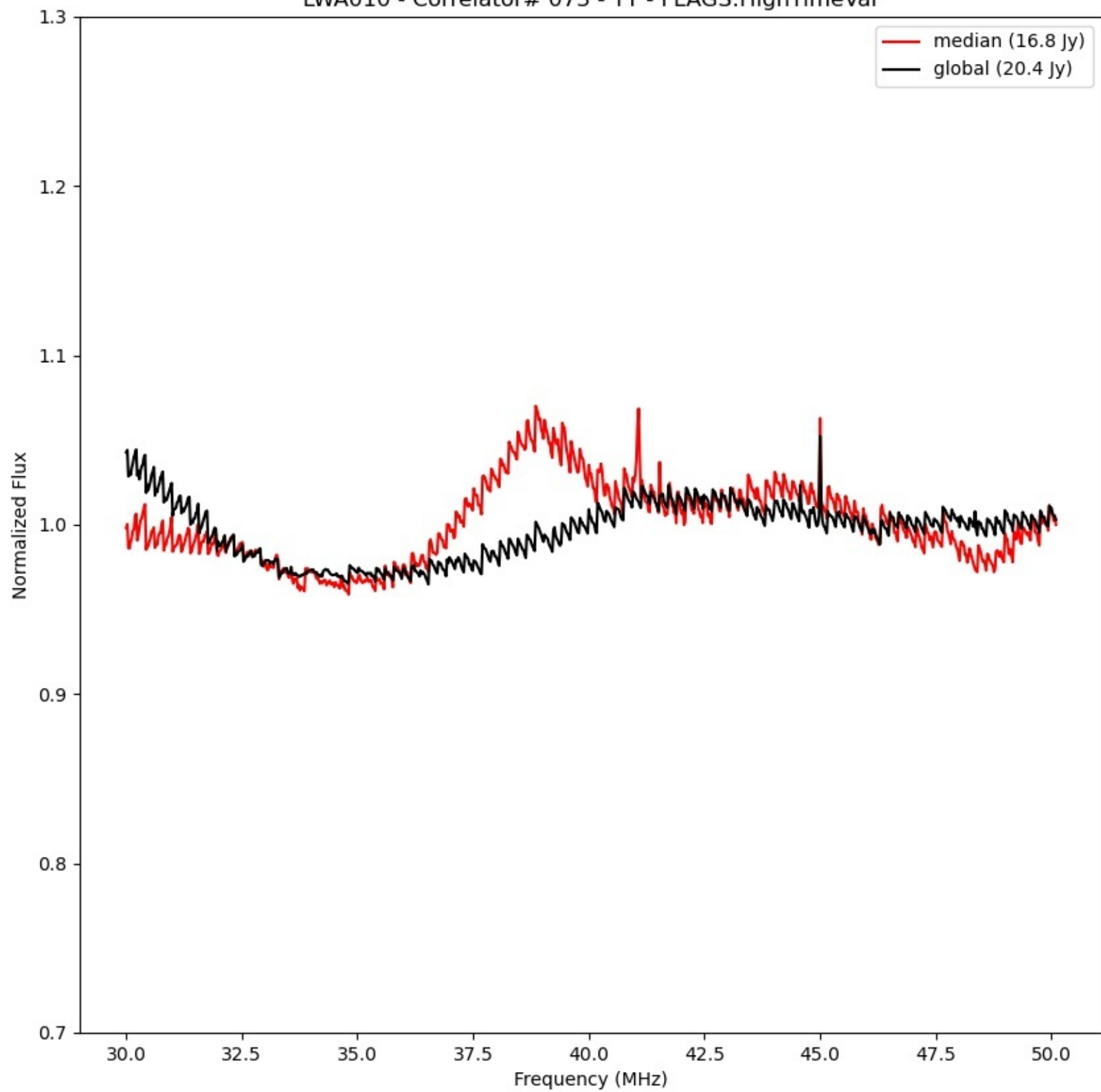
LWA010 - Correlator# 073 - YY - FLAGS:HighTimeVar
