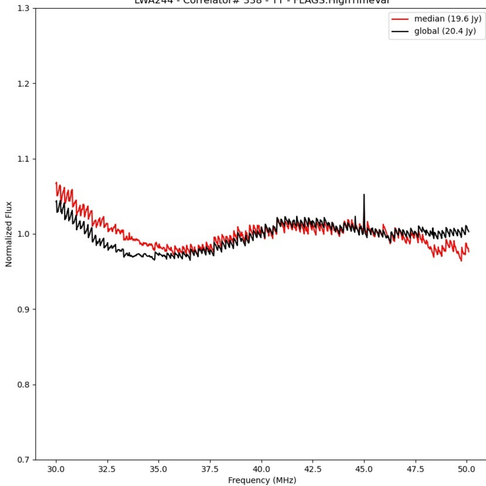
LWA244 - Correlator# 338 - YY - FLAGS:HighTimeVar
