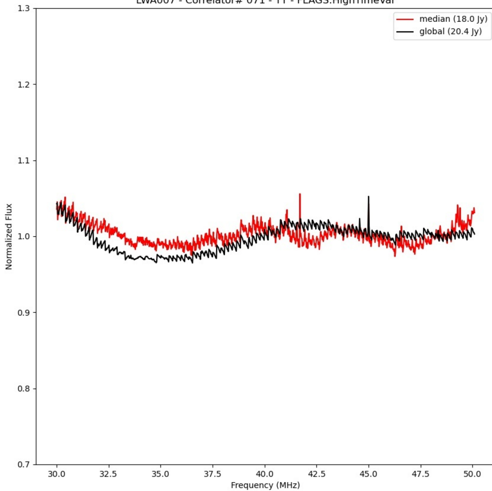
LWA007 - Correlator# 071 - YY - FLAGS:HighTimeVar
