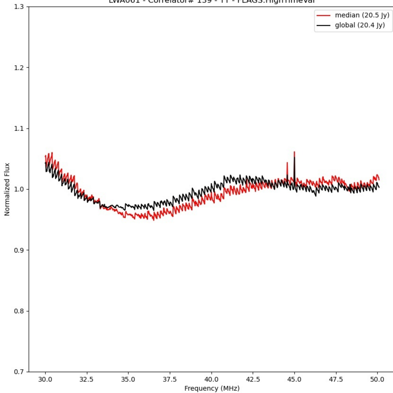
LWA061 - Correlator# 139 - YY - FLAGS:HighTimeVar
