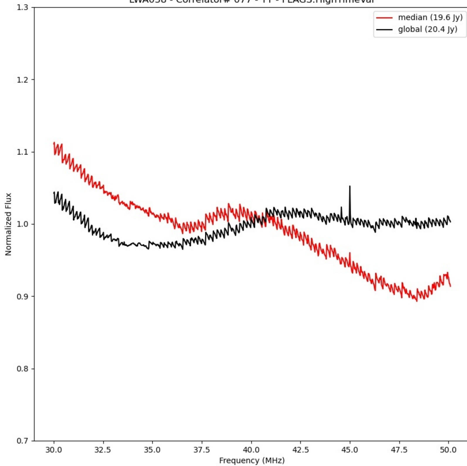
LWA038 - Correlator# 077 - YY - FLAGS:HighTimeVar
