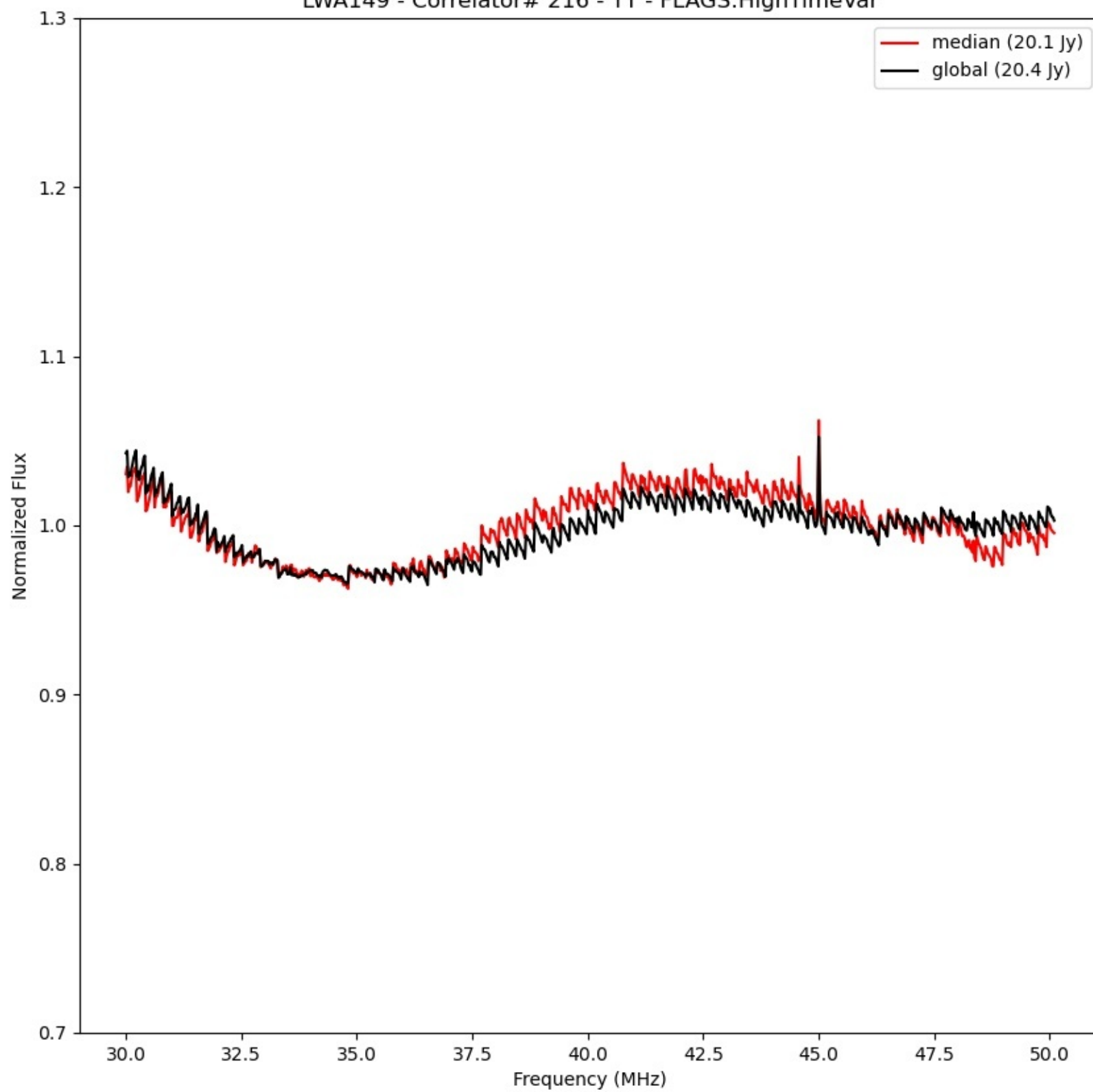
LWA149 - Correlator# 216 - YY - FLAGS:HighTimeVar
