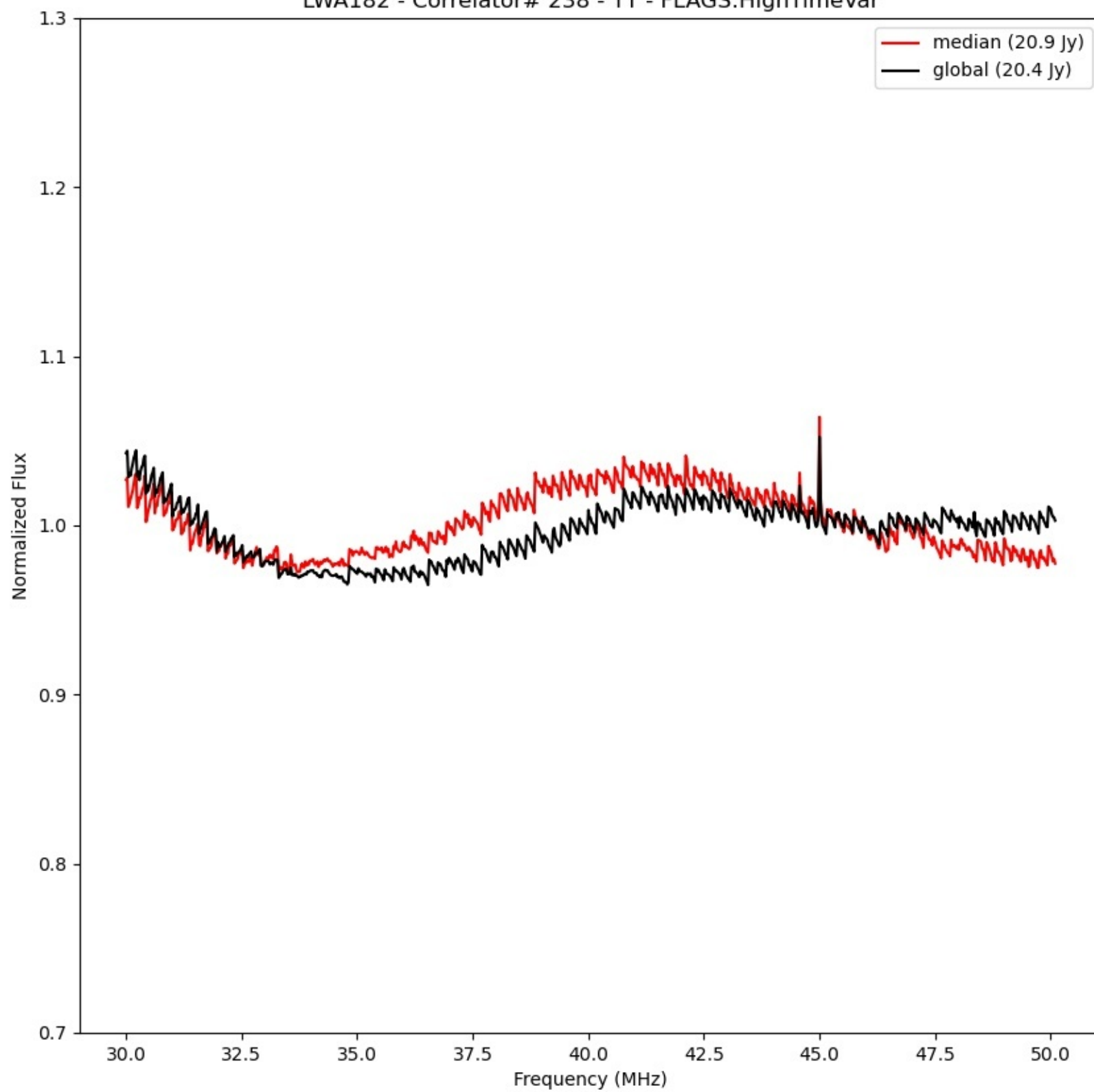
LWA182 - Correlator# 238 - YY - FLAGS:HighTimeVar
