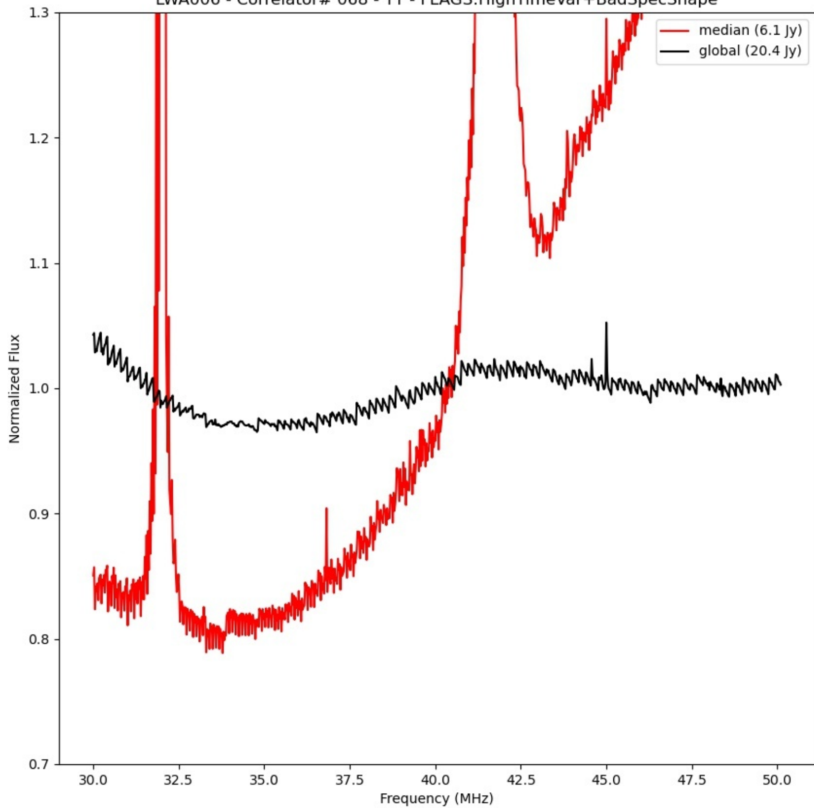
LWA006 - Correlator# 068 - YY - FLAGS:HighTimeVar+BadSpecShape
