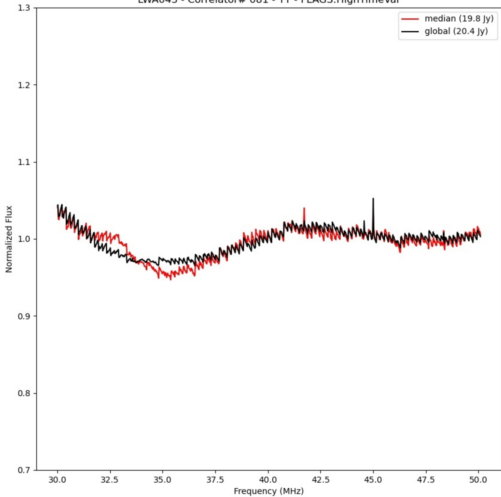
LWA043 - Correlator# 081 - YY - FLAGS:HighTimeVar
