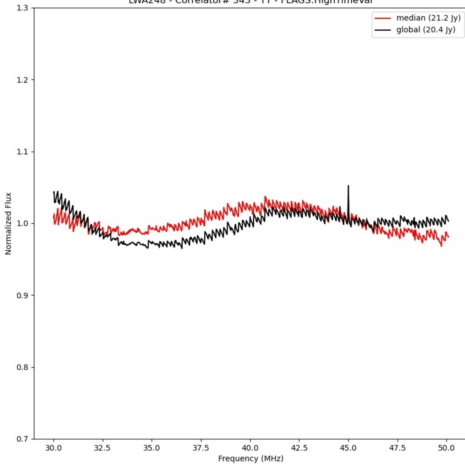
LWA248 - Correlator# 343 - YY - FLAGS:HighTimeVar
