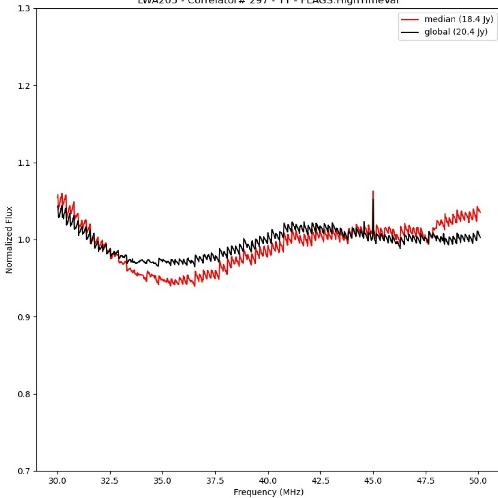
LWA205 - Correlator# 297 - YY - FLAGS:HighTimeVar
