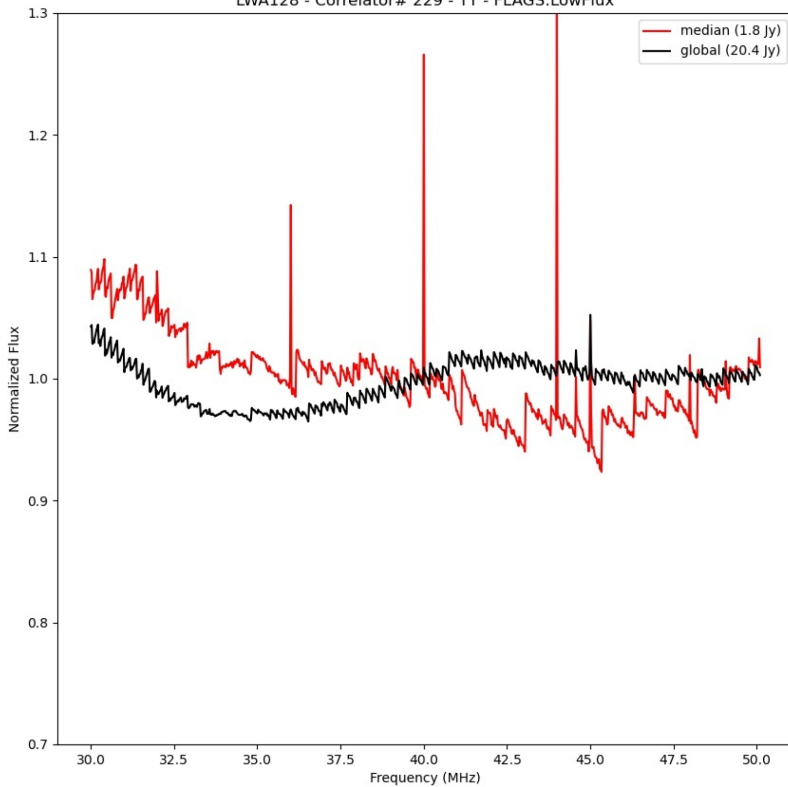
LWA128 - Correlator# 229 - YY - FLAGS:LowFlux
