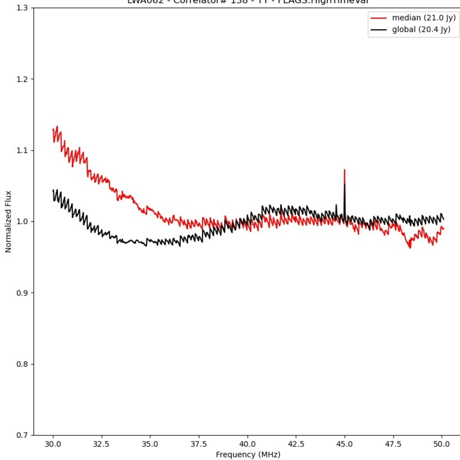
LWA062 - Correlator# 138 - YY - FLAGS:HighTimeVar
