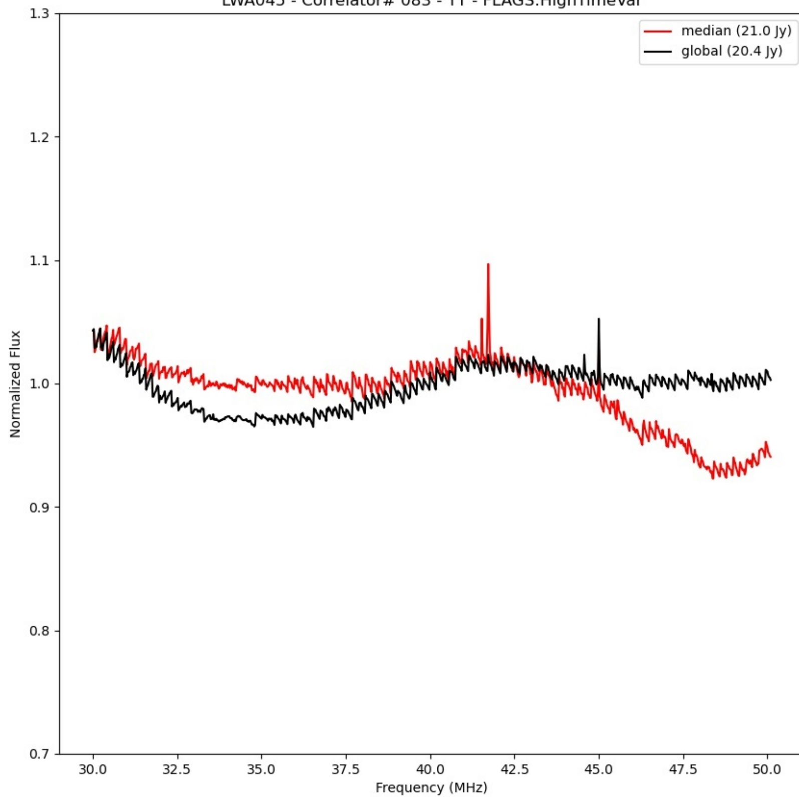
LWA045 - Correlator# 083 - YY - FLAGS:HighTimeVar
