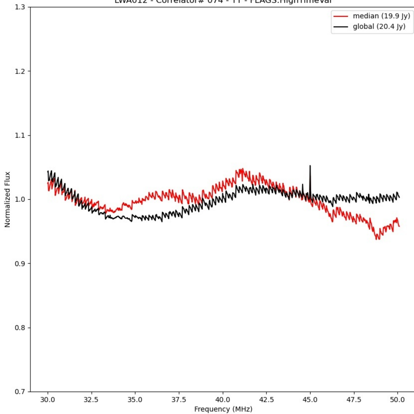
LWA012 - Correlator# 074 - YY - FLAGS:HighTimeVar
