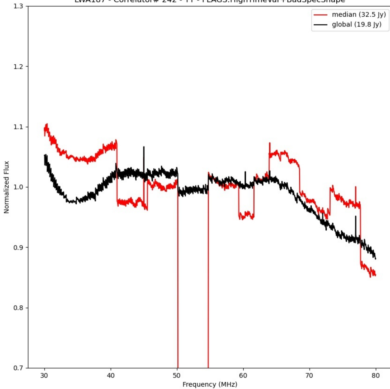
LWA187 - Correlator# 242 - YY - FLAGS:HighTimeVar+BadSpecShape
