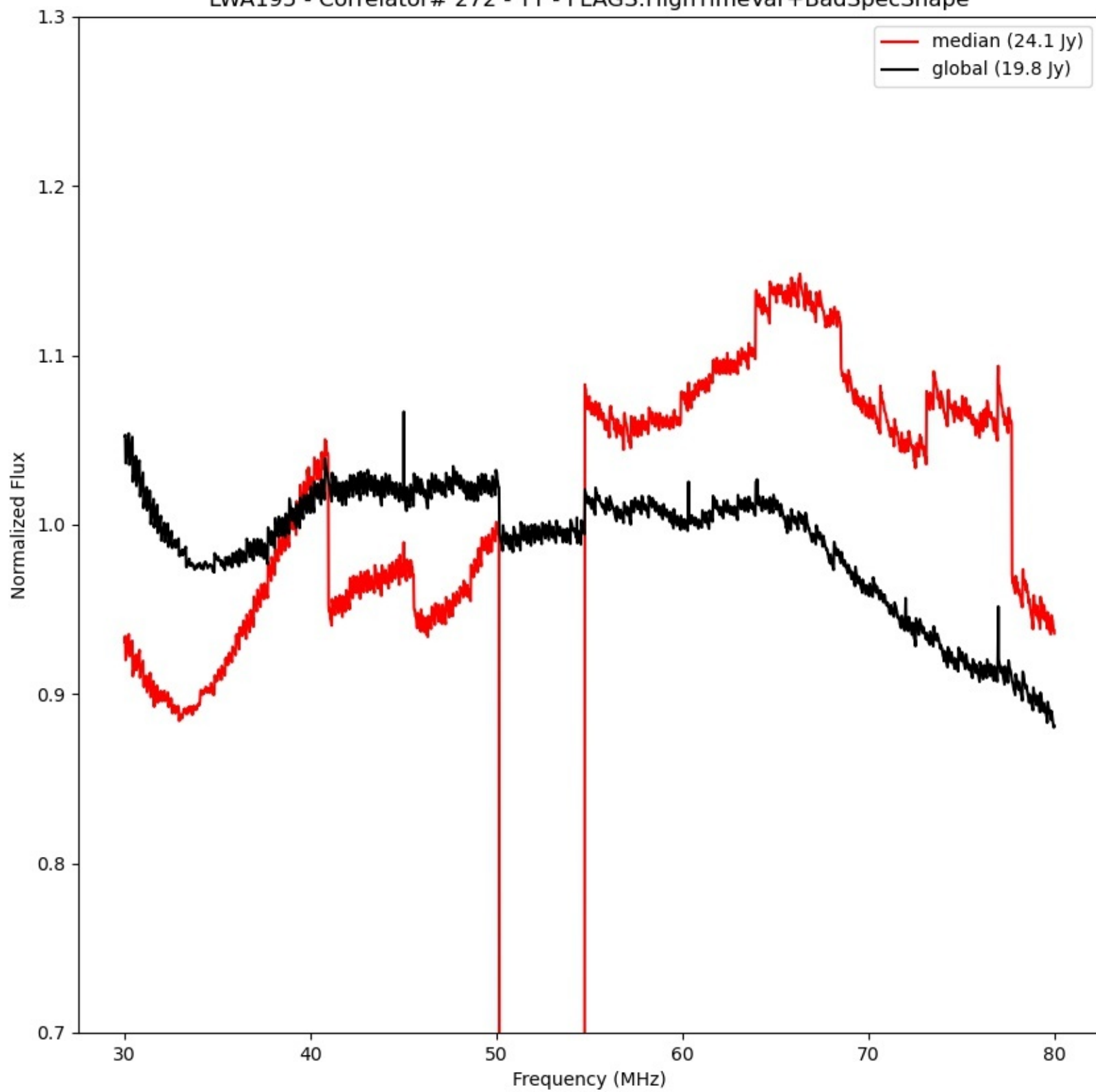
LWA195 - Correlator# 272 - YY - FLAGS:HighTimeVar+BadSpecShape
