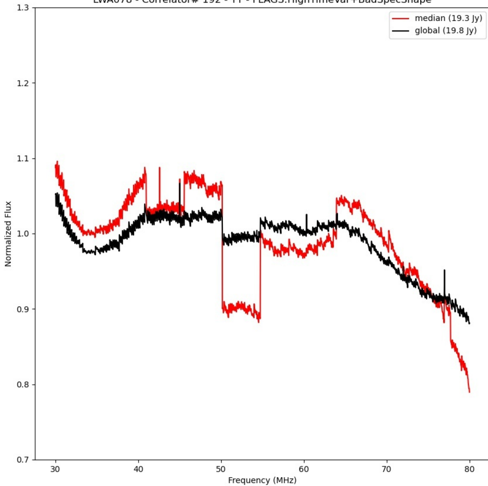
LWA078 - Correlator# 192 - YY - FLAGS:HighTimeVar+BadSpecShape
