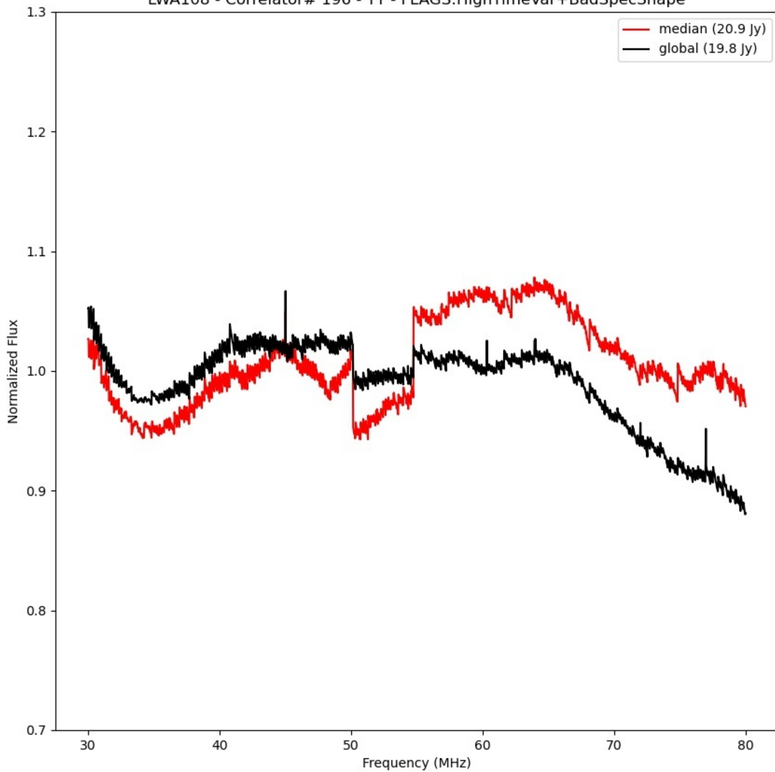
LWA108 - Correlator# 196 - YY - FLAGS:HighTimeVar+BadSpecShape
