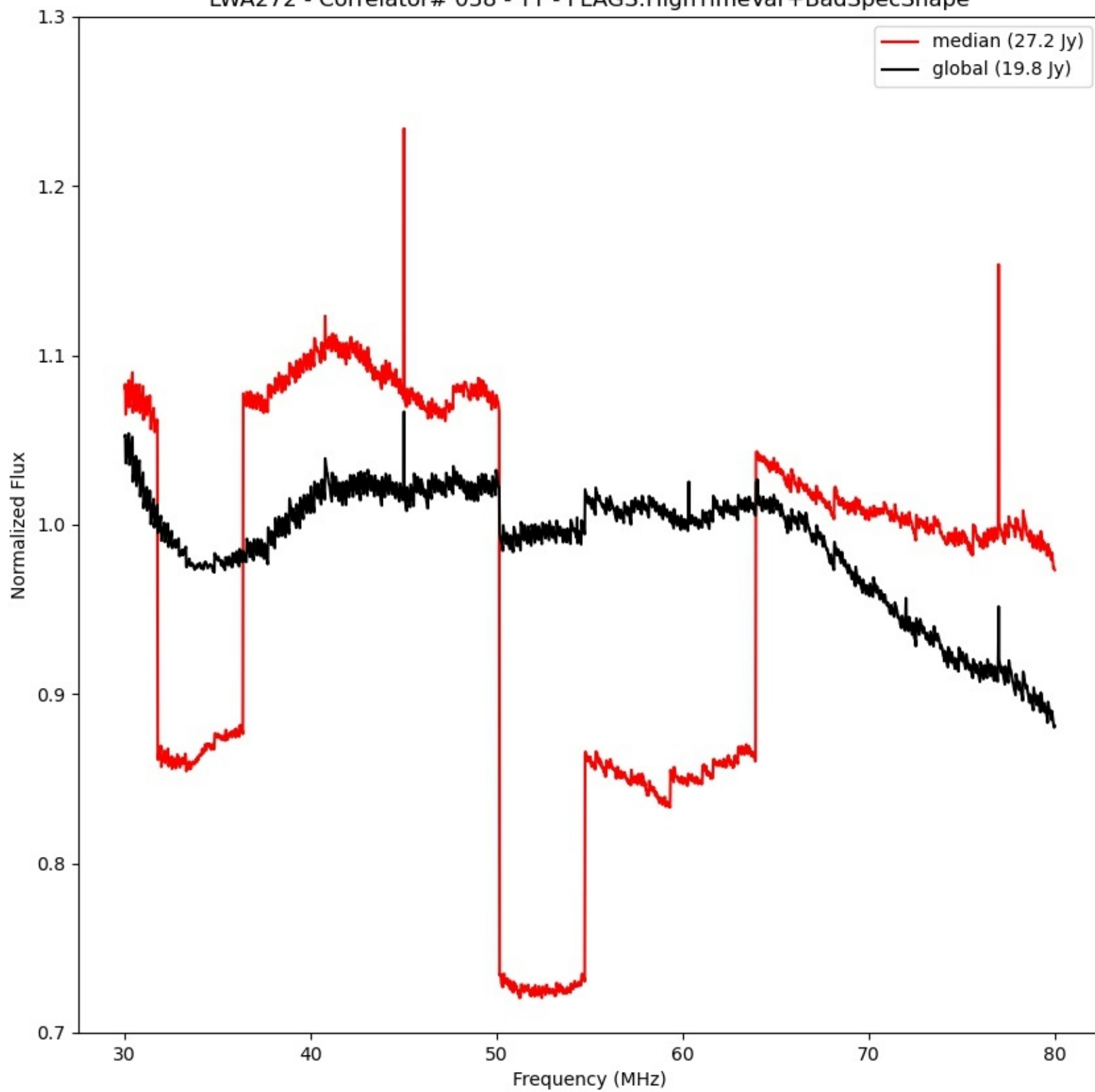
LWA272 - Correlator# 038 - YY - FLAGS:HighTimeVar+BadSpecShape
