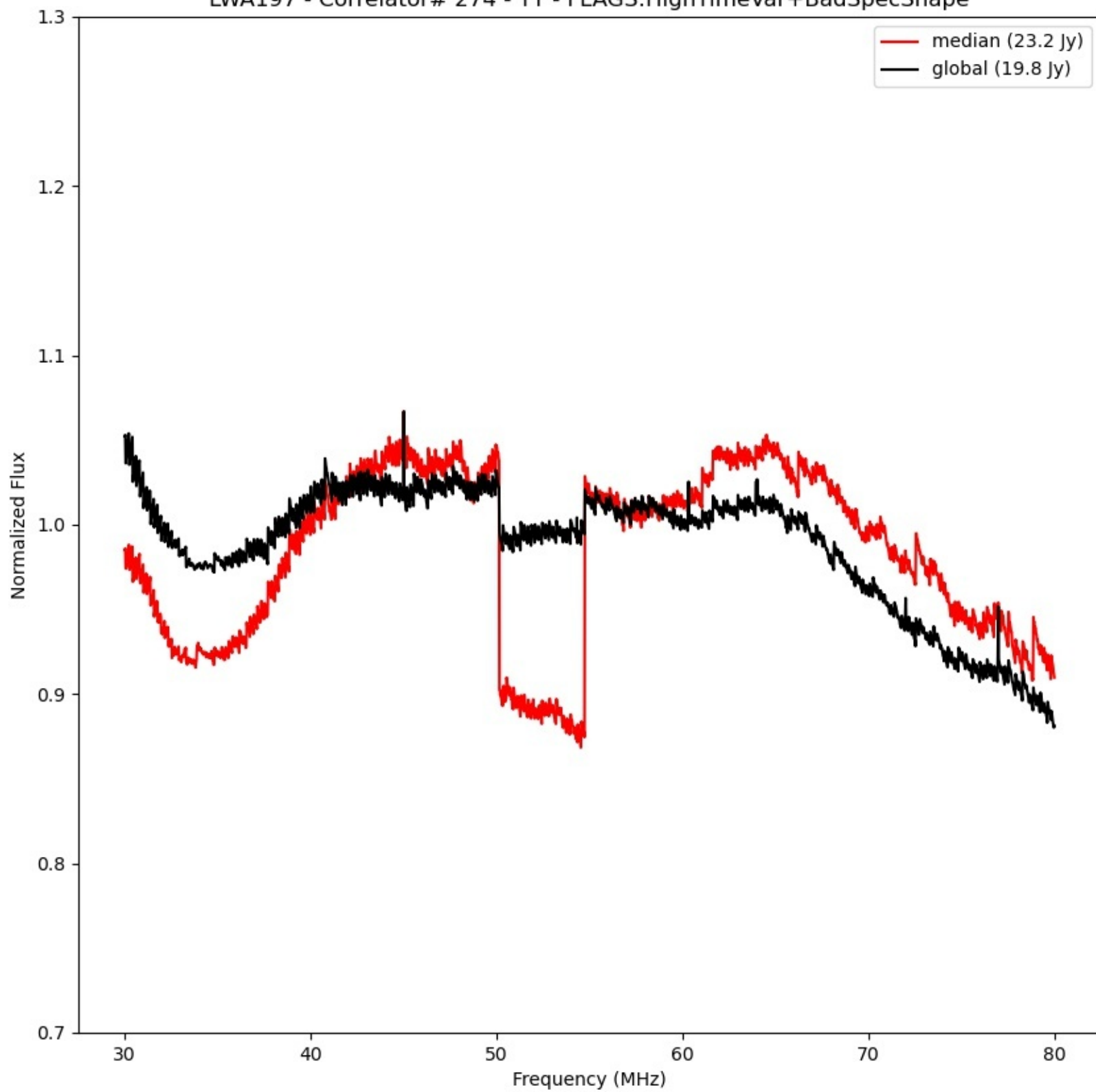
LWA197 - Correlator# 274 - YY - FLAGS:HighTimeVar+BadSpecShape
