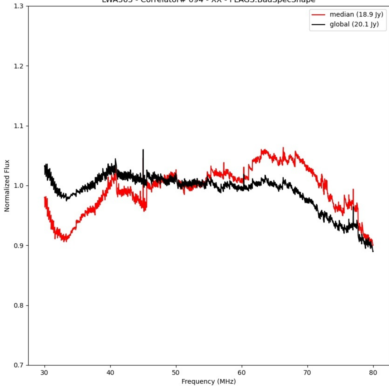
LWA363 - Correlator# 094 - XX - FLAGS:BadSpecShape
