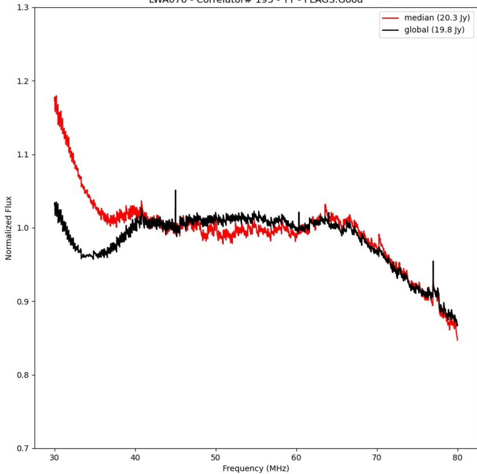
LWA076 - Correlator# 193 - YY - FLAGS:Good
