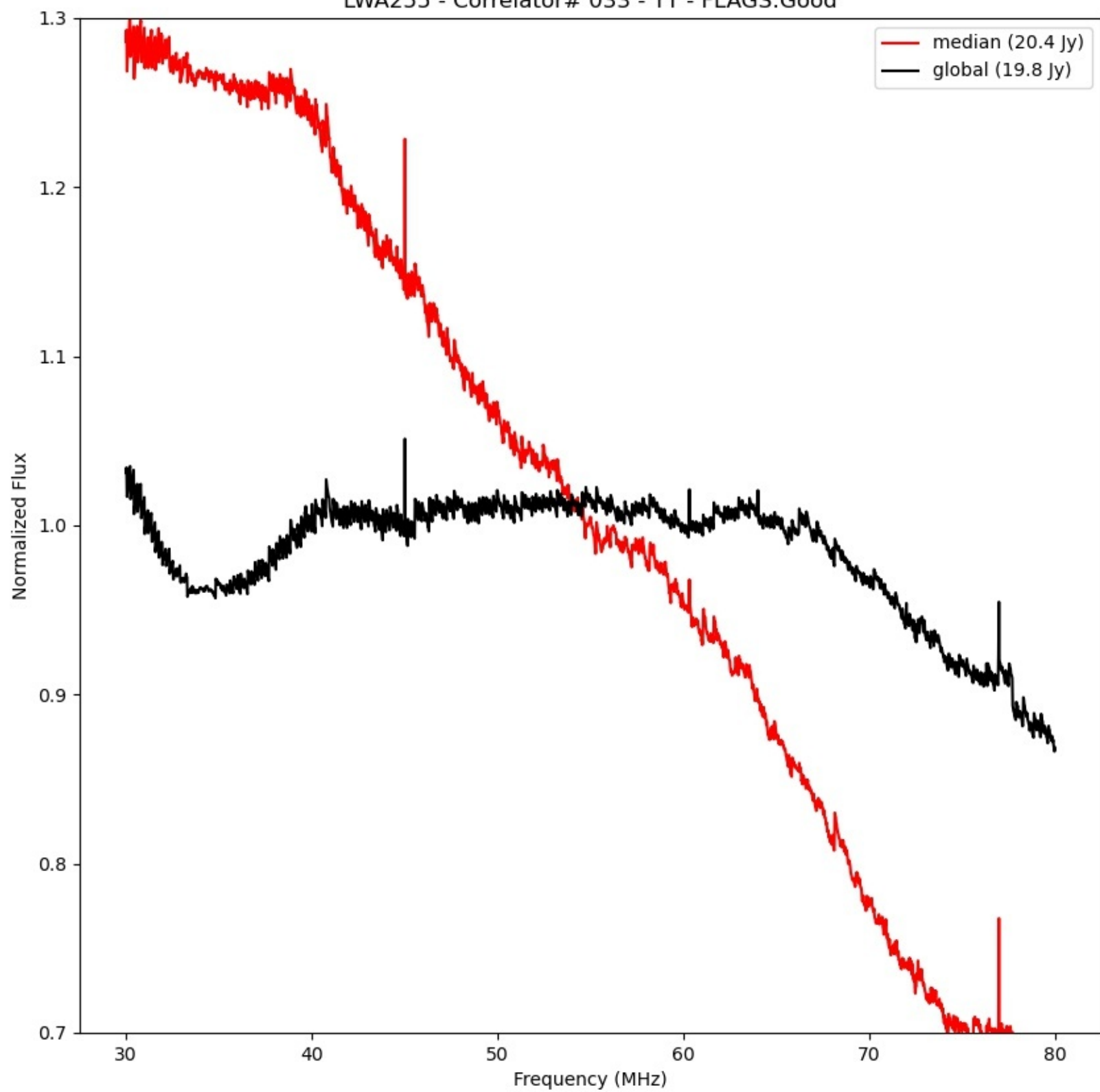
LWA255 - Correlator# 033 - YY - FLAGS:Good
