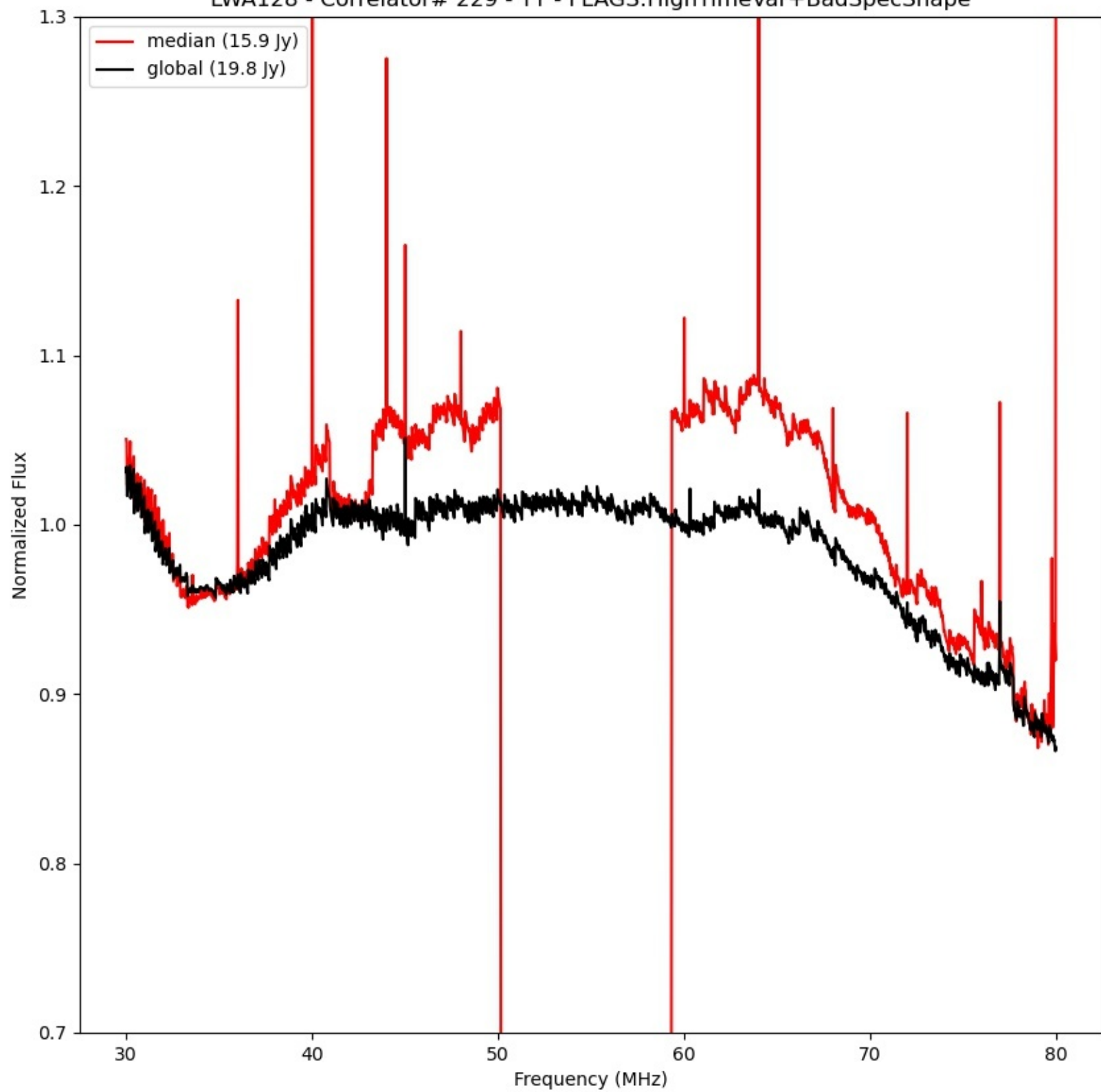
LWA128 - Correlator# 229 - YY - FLAGS:HighTimeVar+BadSpecShape
