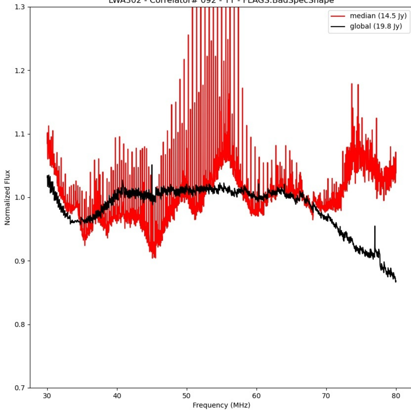
LWA302 - Correlator# 092 - YY - FLAGS:BadSpecShape
