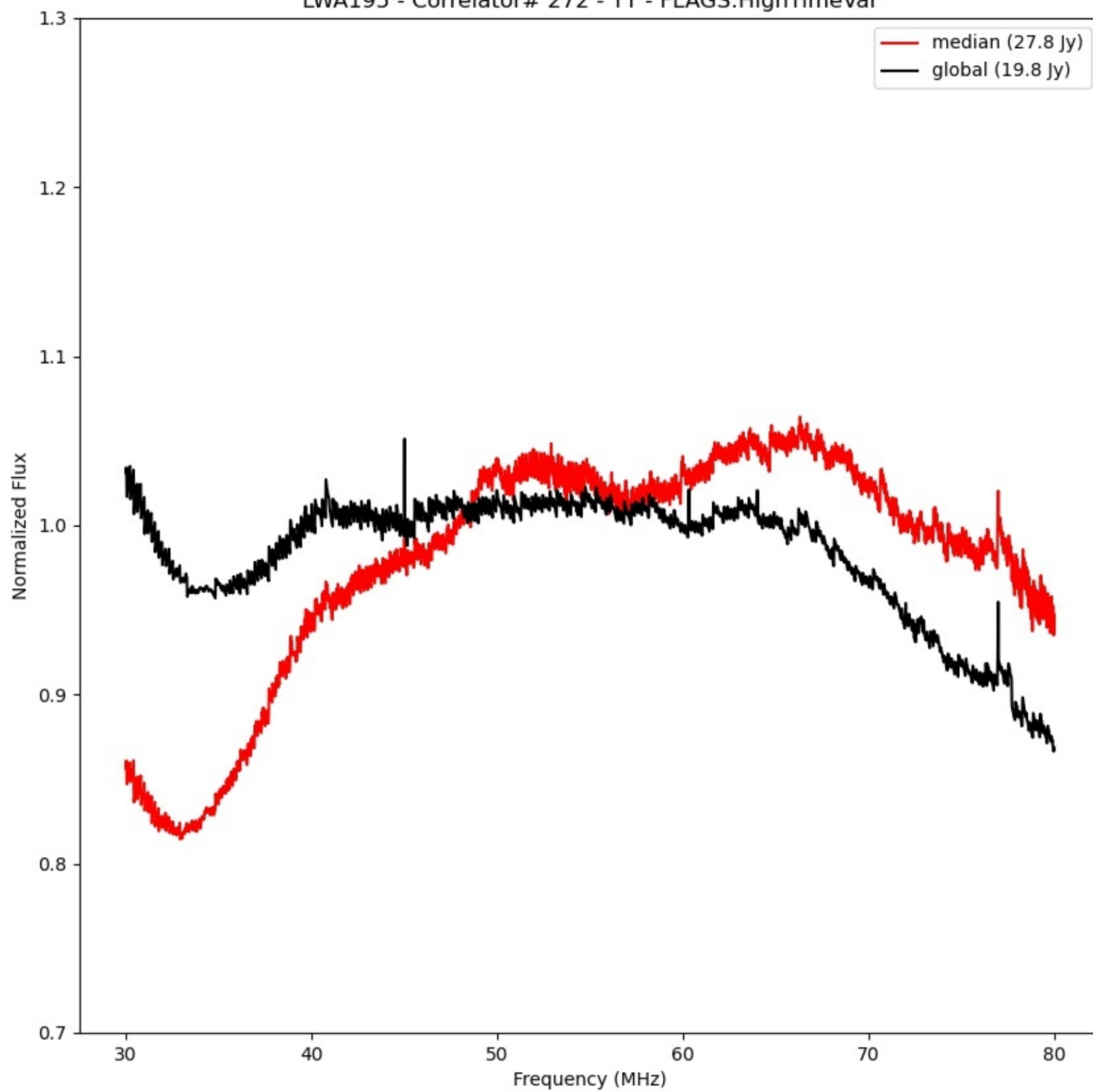
LWA195 - Correlator# 272 - YY - FLAGS:HighTimeVar
