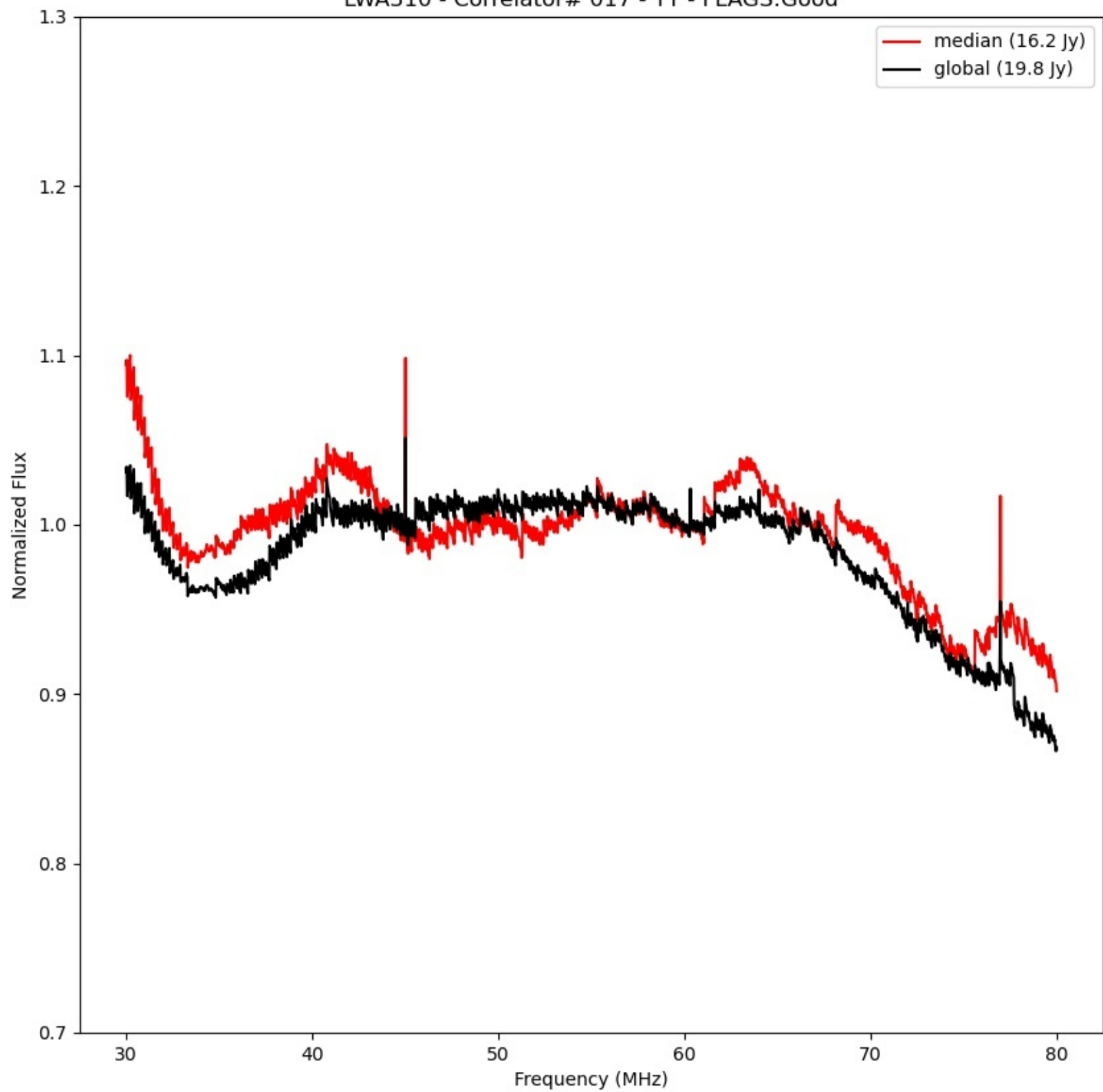
LWA310 - Correlator# 017 - YY - FLAGS:Good
