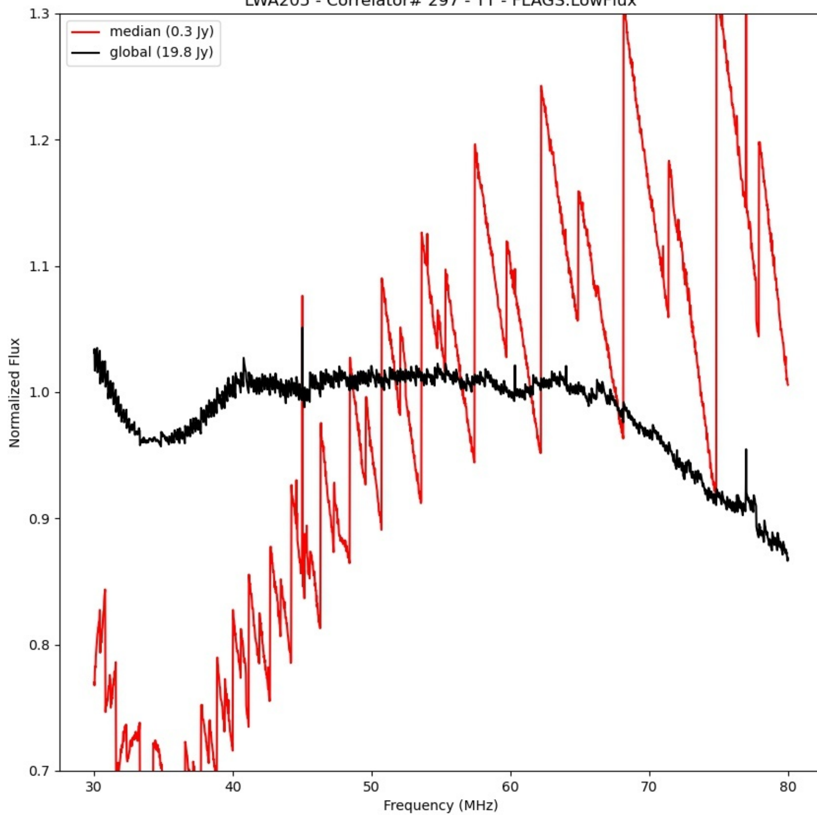
LWA205 - Correlator# 297 - YY - FLAGS:LowFlux
