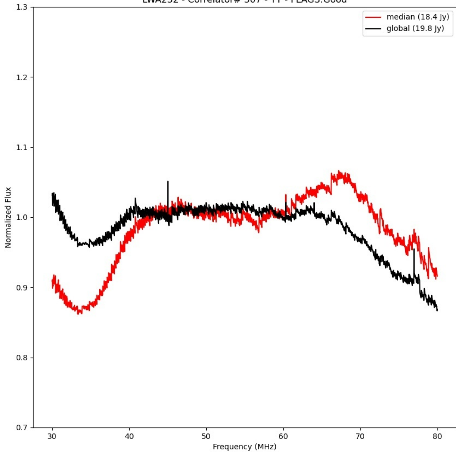
LWA232 - Correlator# 307 - YY - FLAGS:Good
