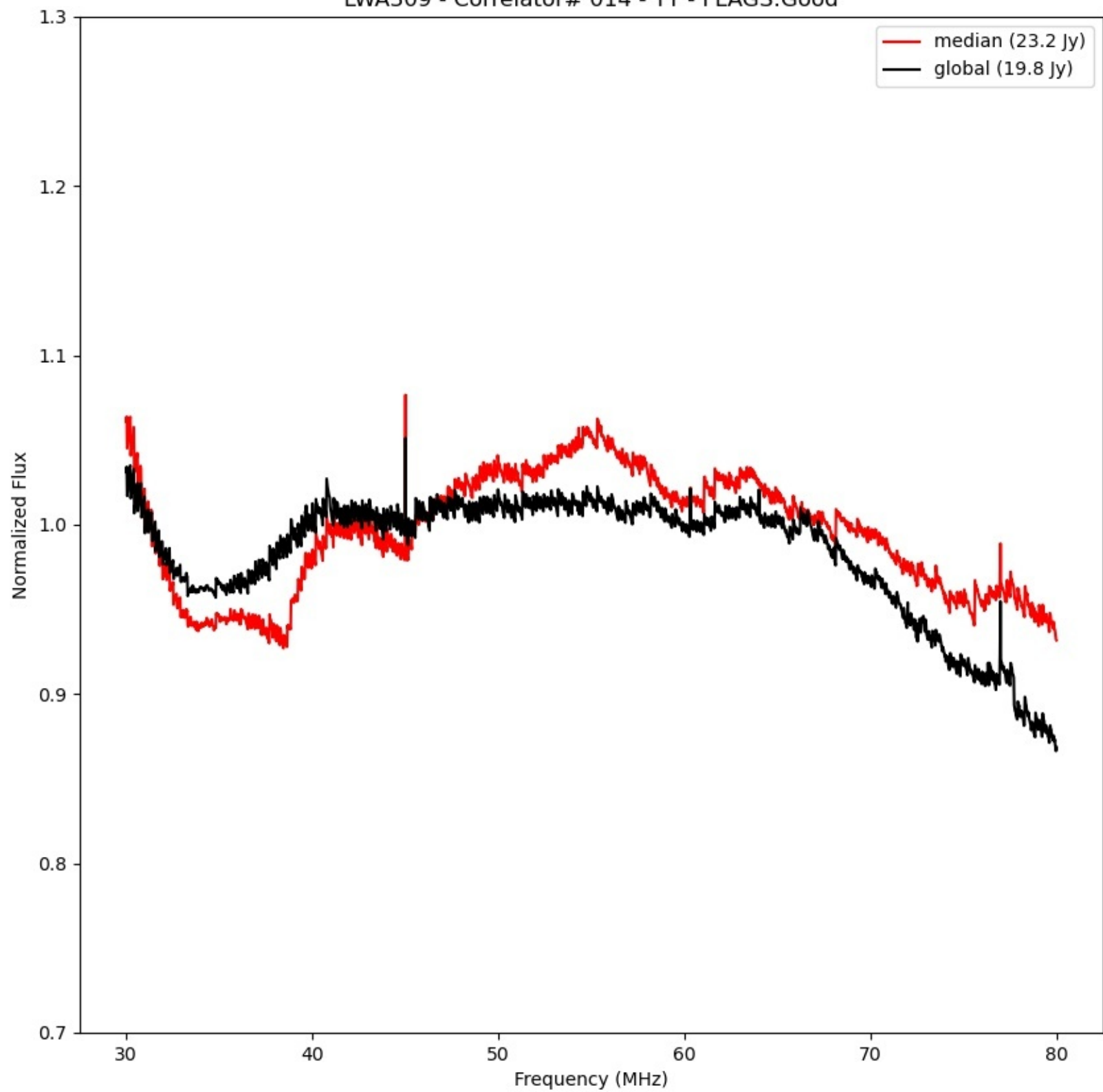
LWA309 - Correlator# 014 - YY - FLAGS:Good
