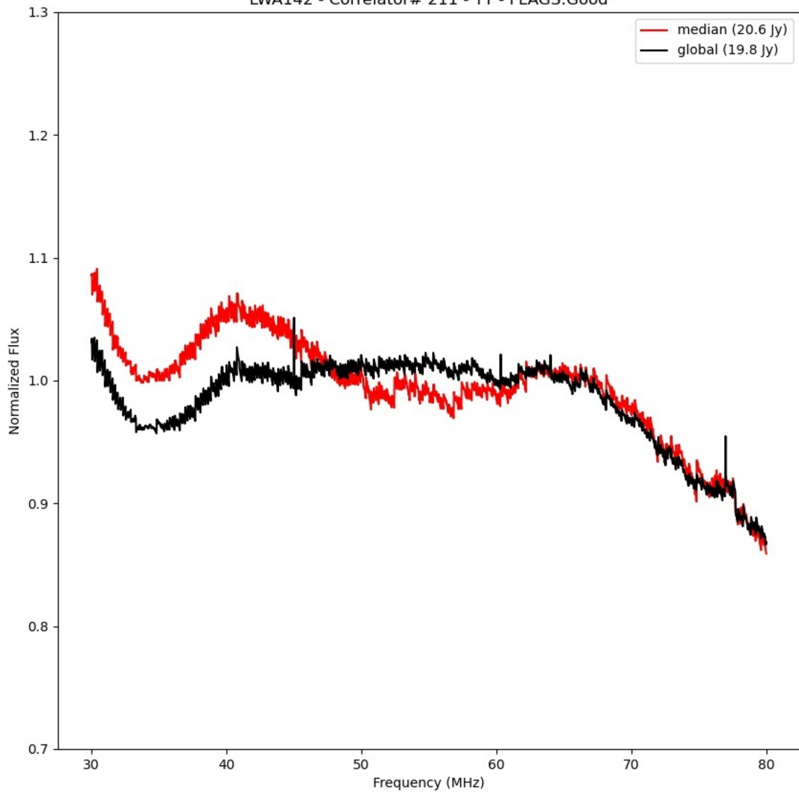
LWA142 - Correlator# 211 - YY - FLAGS:Good
