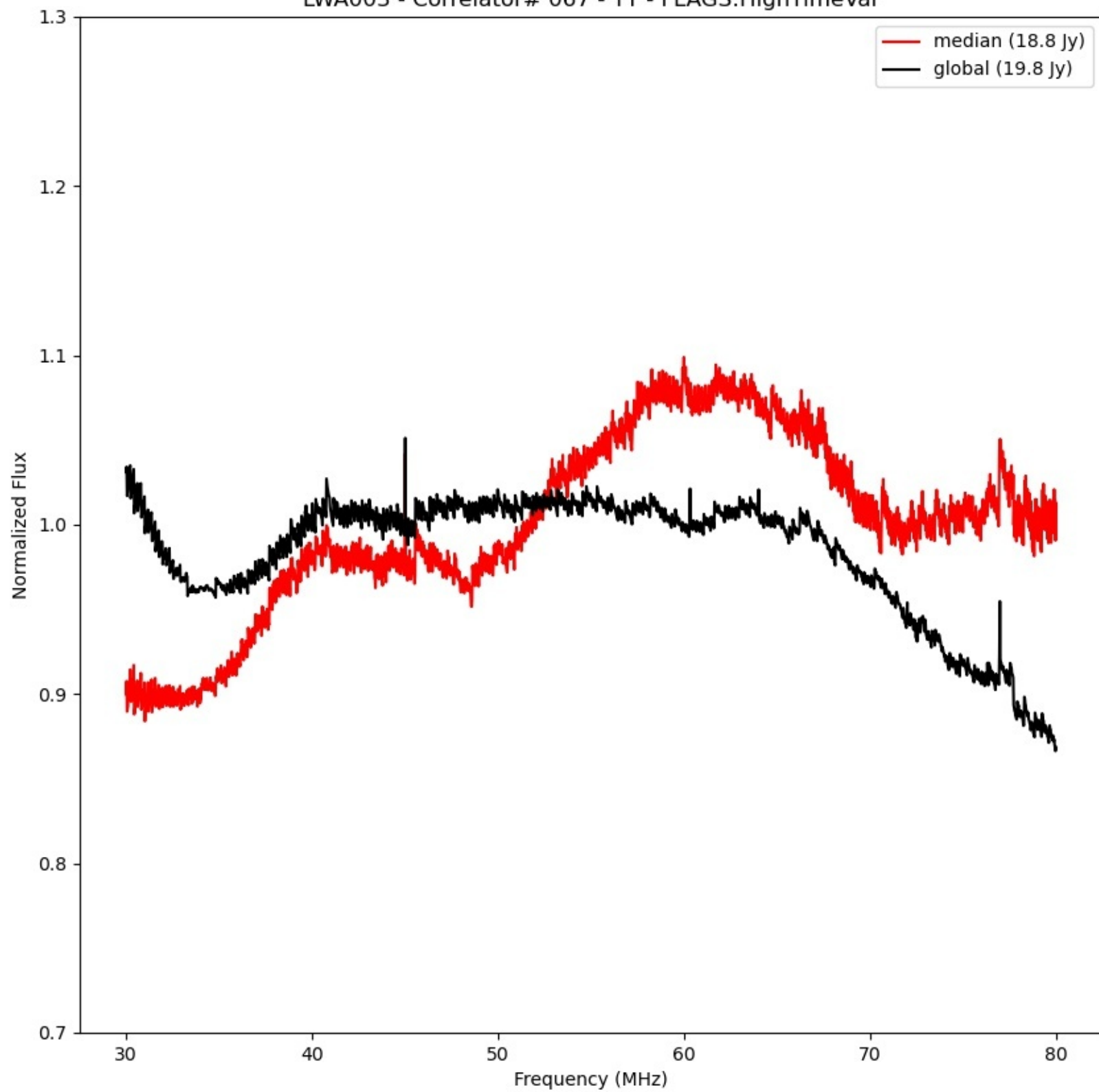
LWA003 - Correlator# 067 - YY - FLAGS:HighTimeVar
