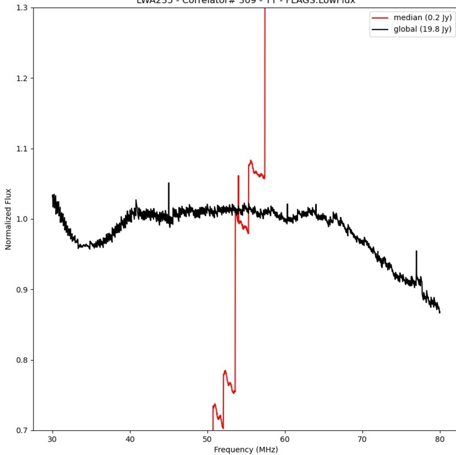
LWA235 - Correlator# 309 - YY - FLAGS:LowFlux
