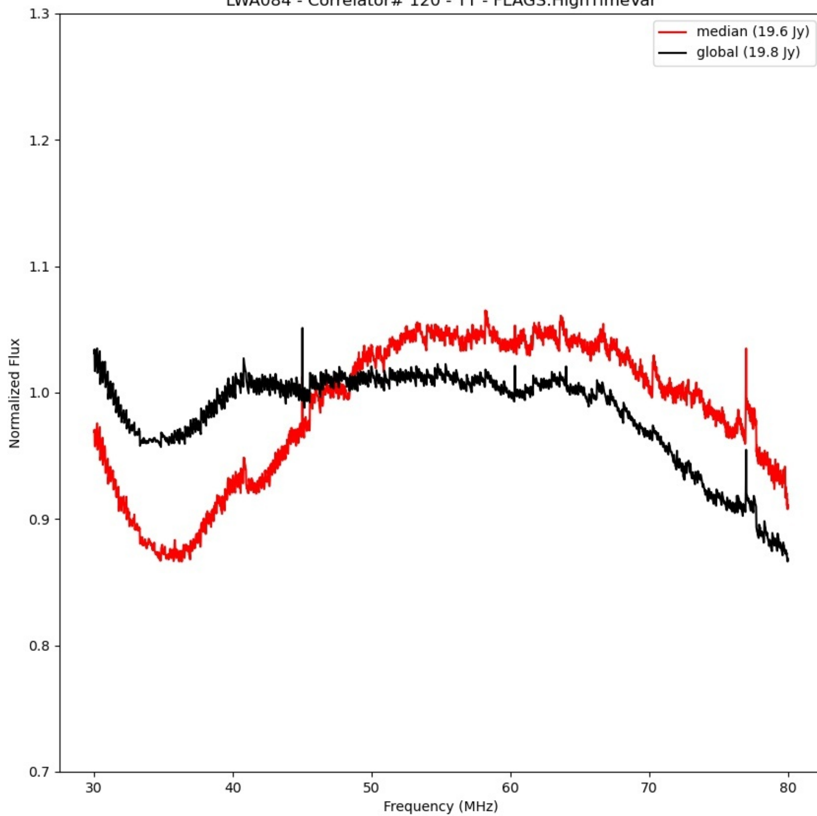
LWA084 - Correlator# 120 - YY - FLAGS:HighTimeVar
