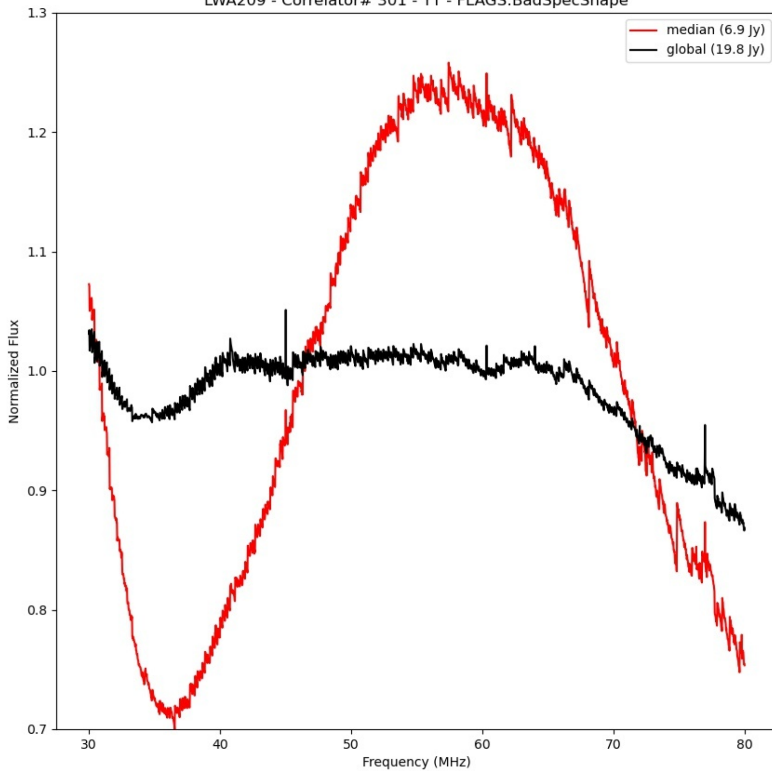
LWA209 - Correlator# 301 - YY - FLAGS:BadSpecShape
