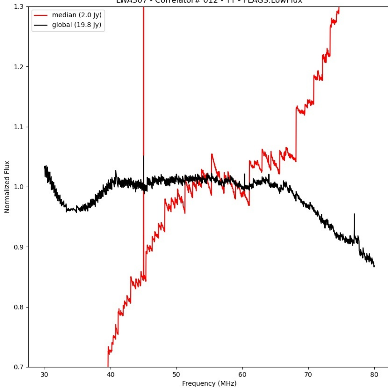
LWA307 - Correlator# 012 - YY - FLAGS:LowFlux
