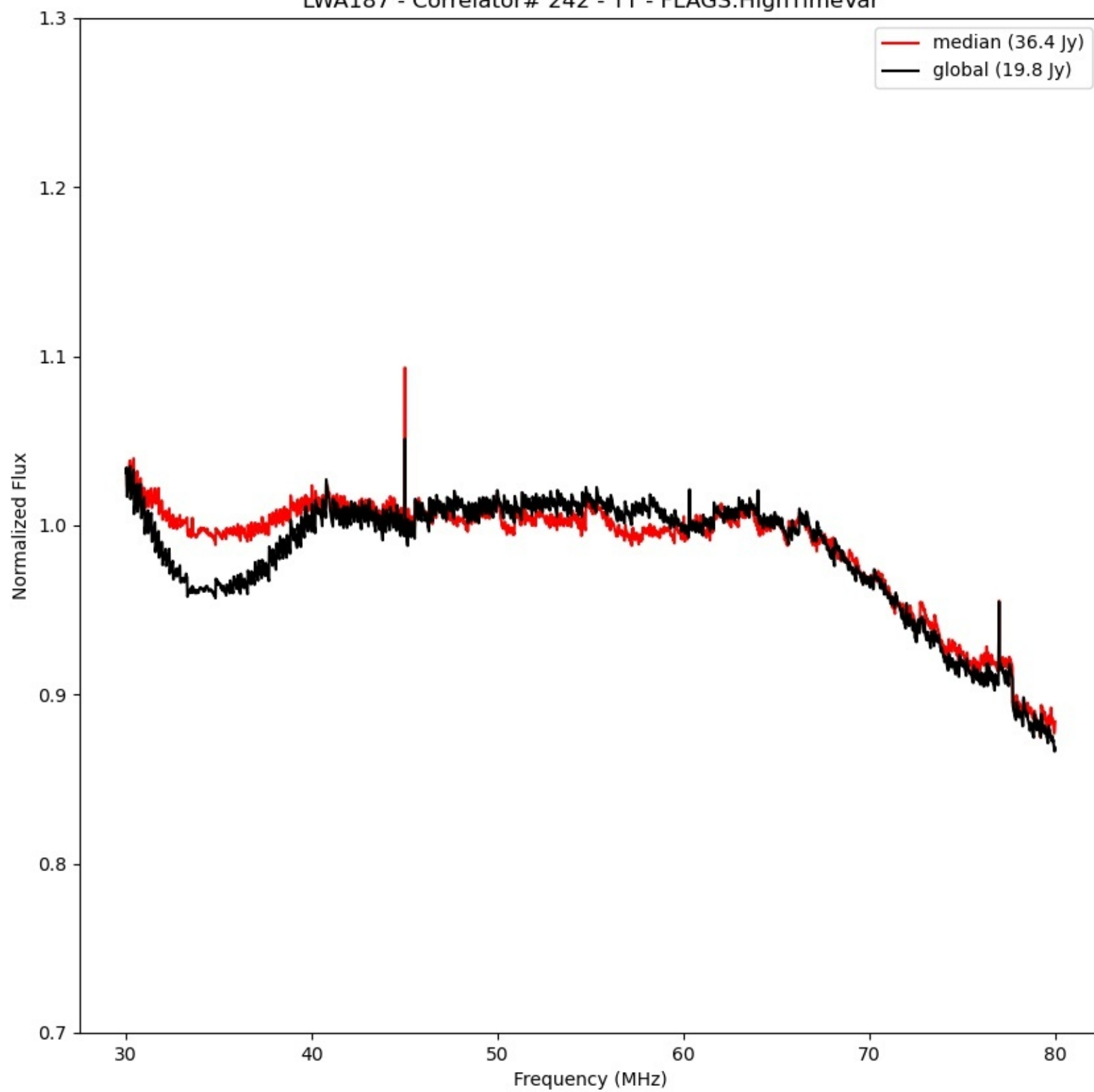
LWA187 - Correlator# 242 - YY - FLAGS:HighTimeVar
