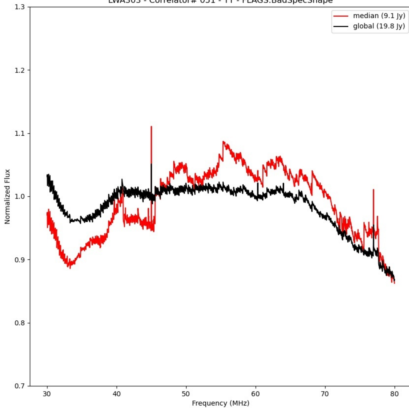
LWA303 - Correlator# 051 - YY - FLAGS:BadSpecShape
