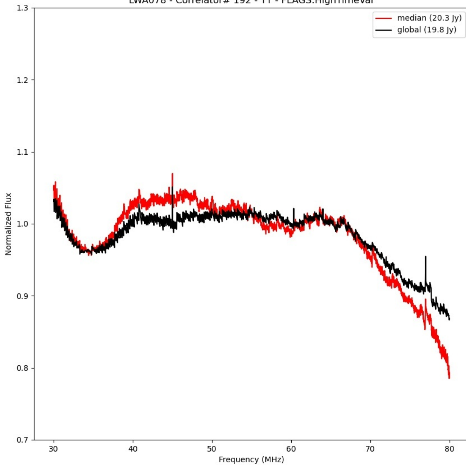
LWA078 - Correlator# 192 - YY - FLAGS:HighTimeVar
