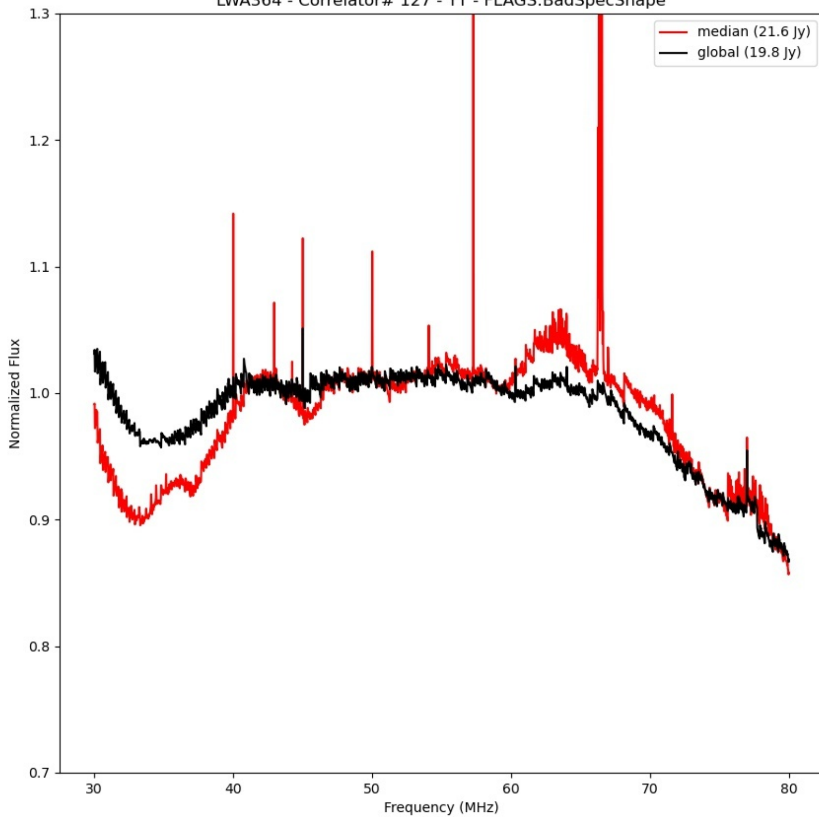
LWA364 - Correlator# 127 - YY - FLAGS:BadSpecShape
