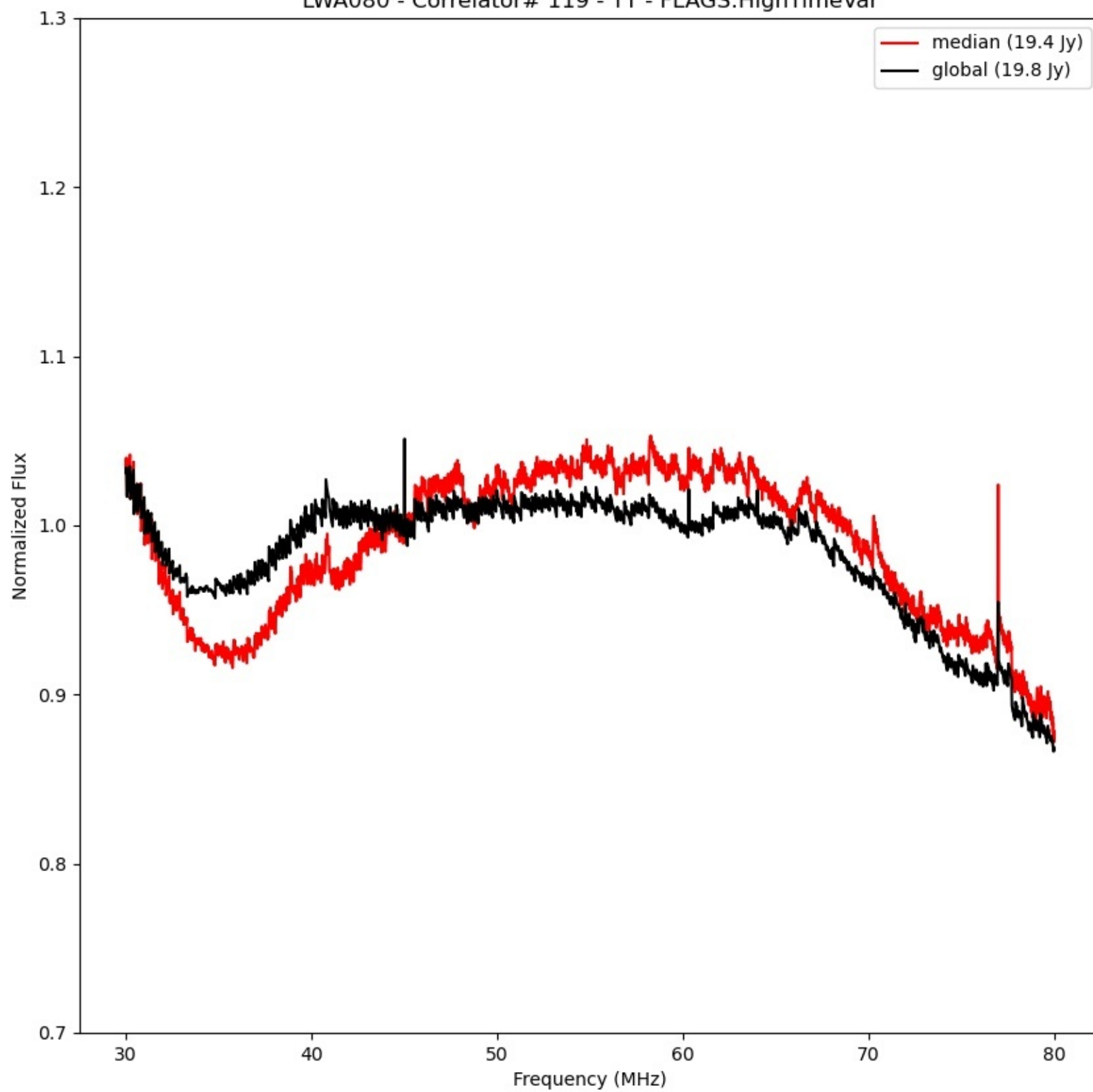
LWA080 - Correlator# 119 - YY - FLAGS:HighTimeVar
