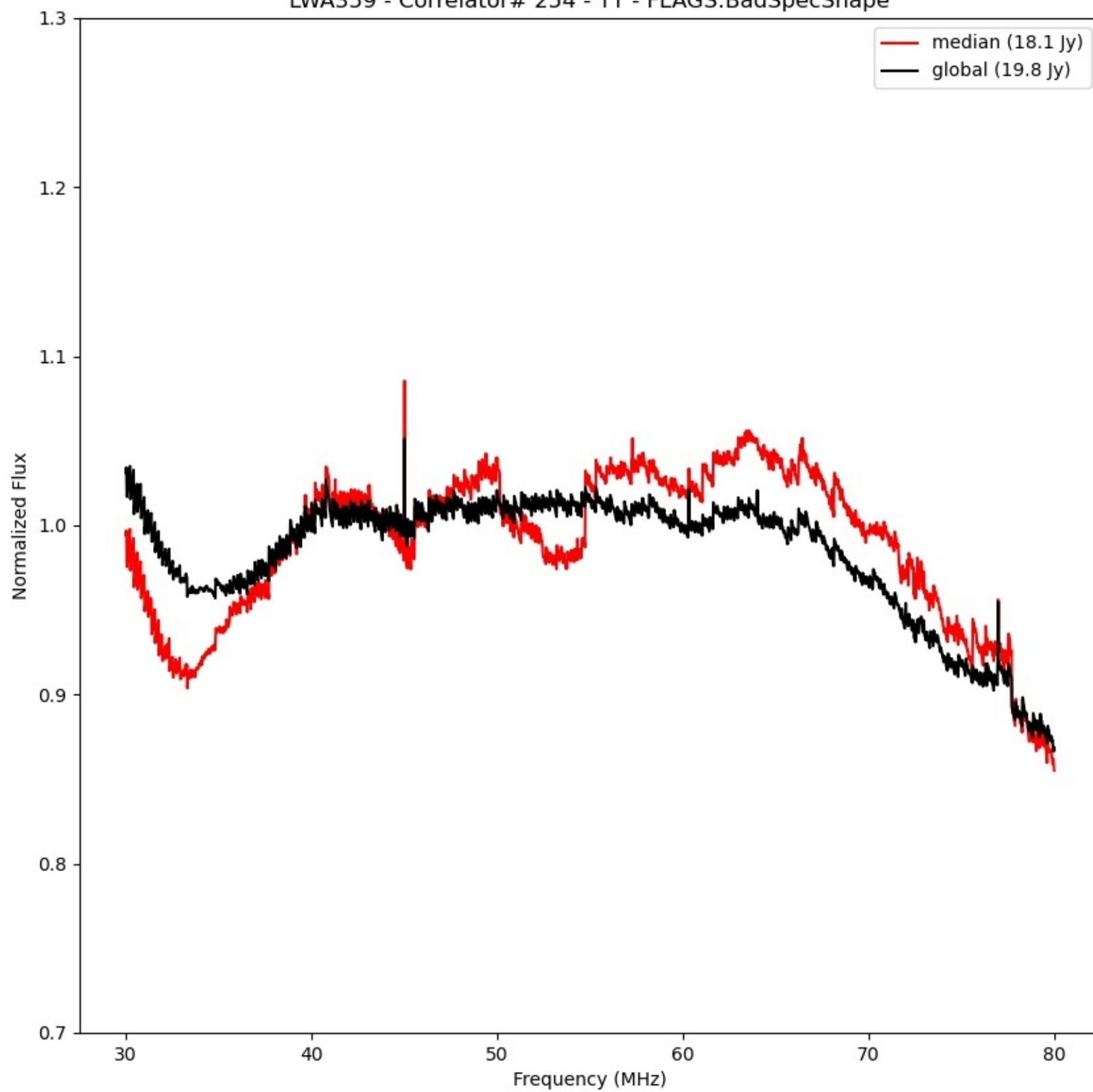
LWA359 - Correlator# 254 - YY - FLAGS:BadSpecShape
