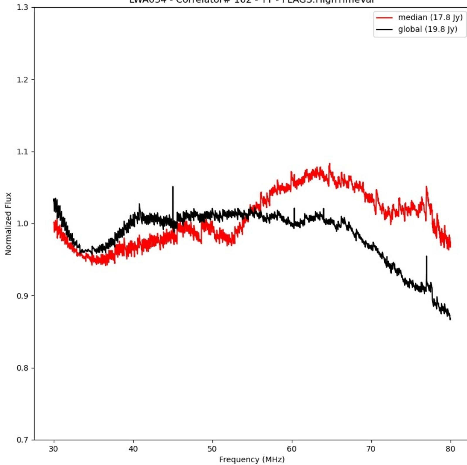
LWA034 - Correlator# 162 - YY - FLAGS:HighTimeVar
