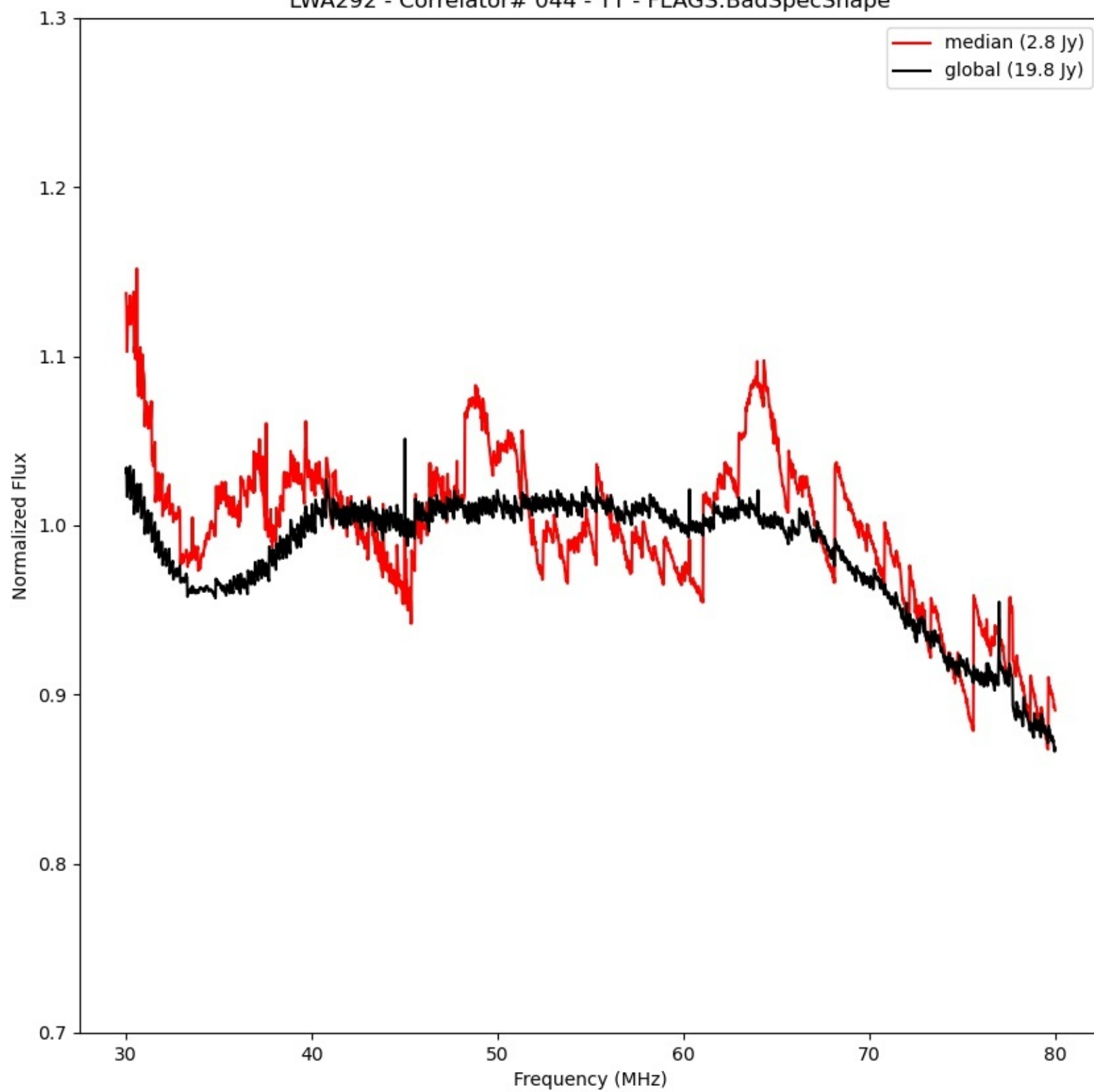
LWA292 - Correlator# 044 - YY - FLAGS:BadSpecShape
