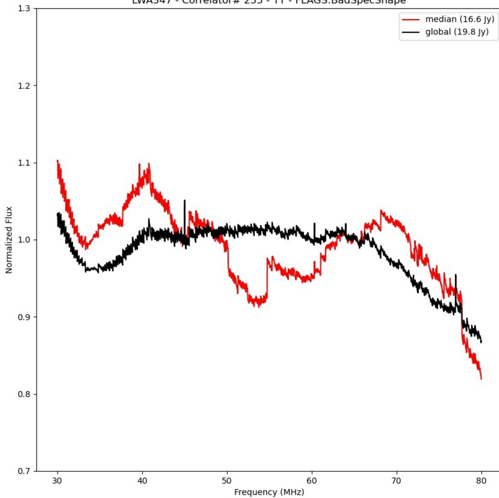
LWA347 - Correlator# 255 - YY - FLAGS:BadSpecShape
