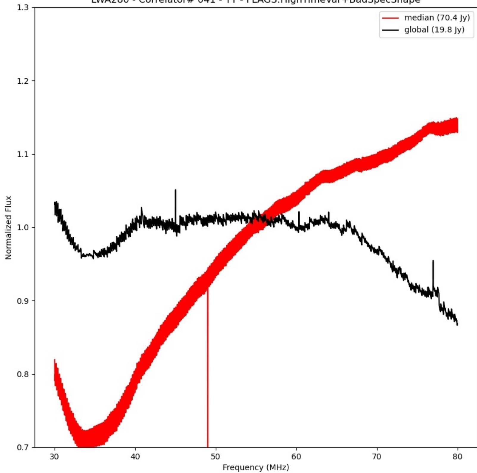
LWA280 - Correlator# 041 - YY - FLAGS:HighTimeVar+BadSpecShape
