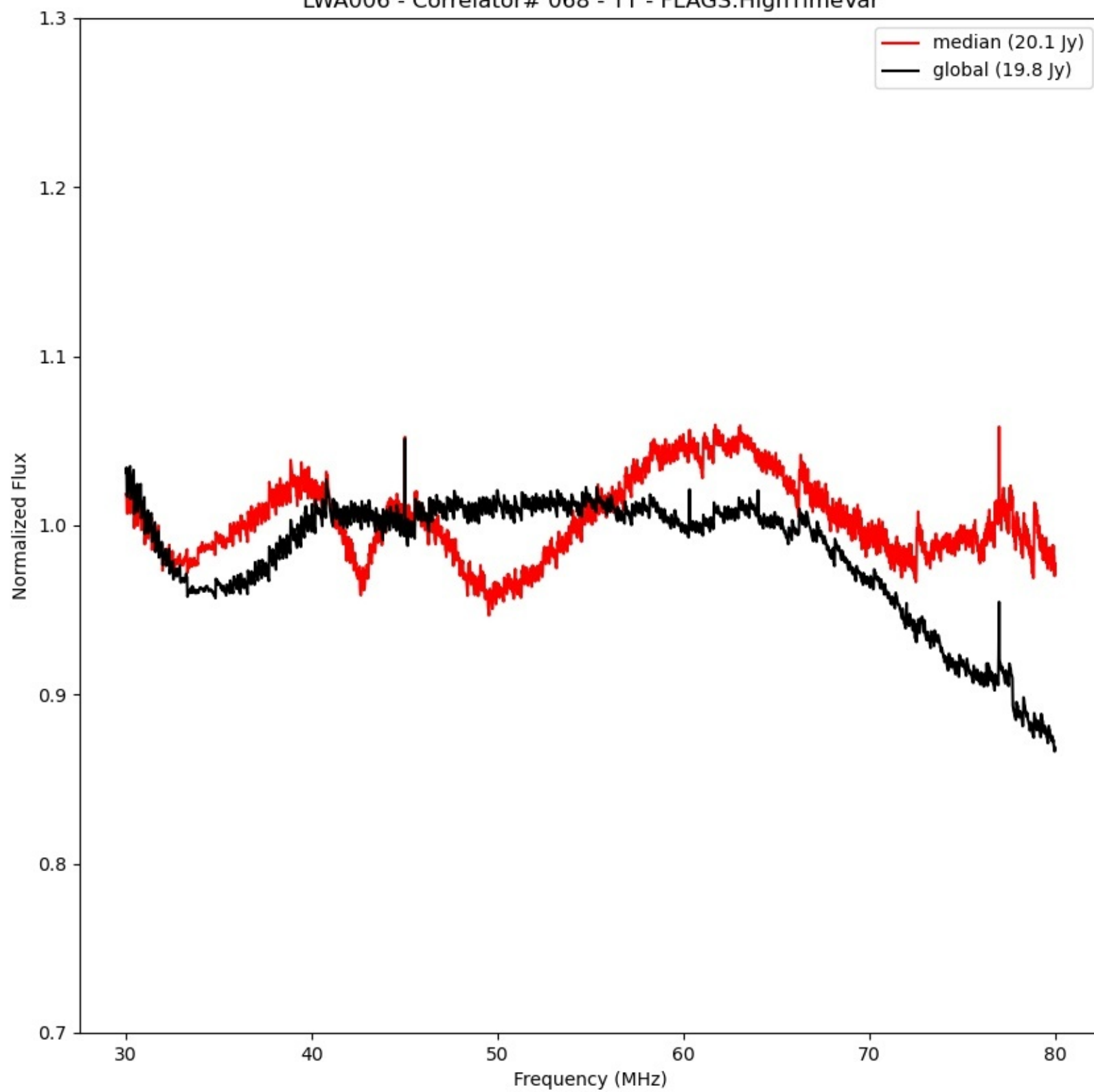
LWA006 - Correlator# 068 - YY - FLAGS:HighTimeVar
