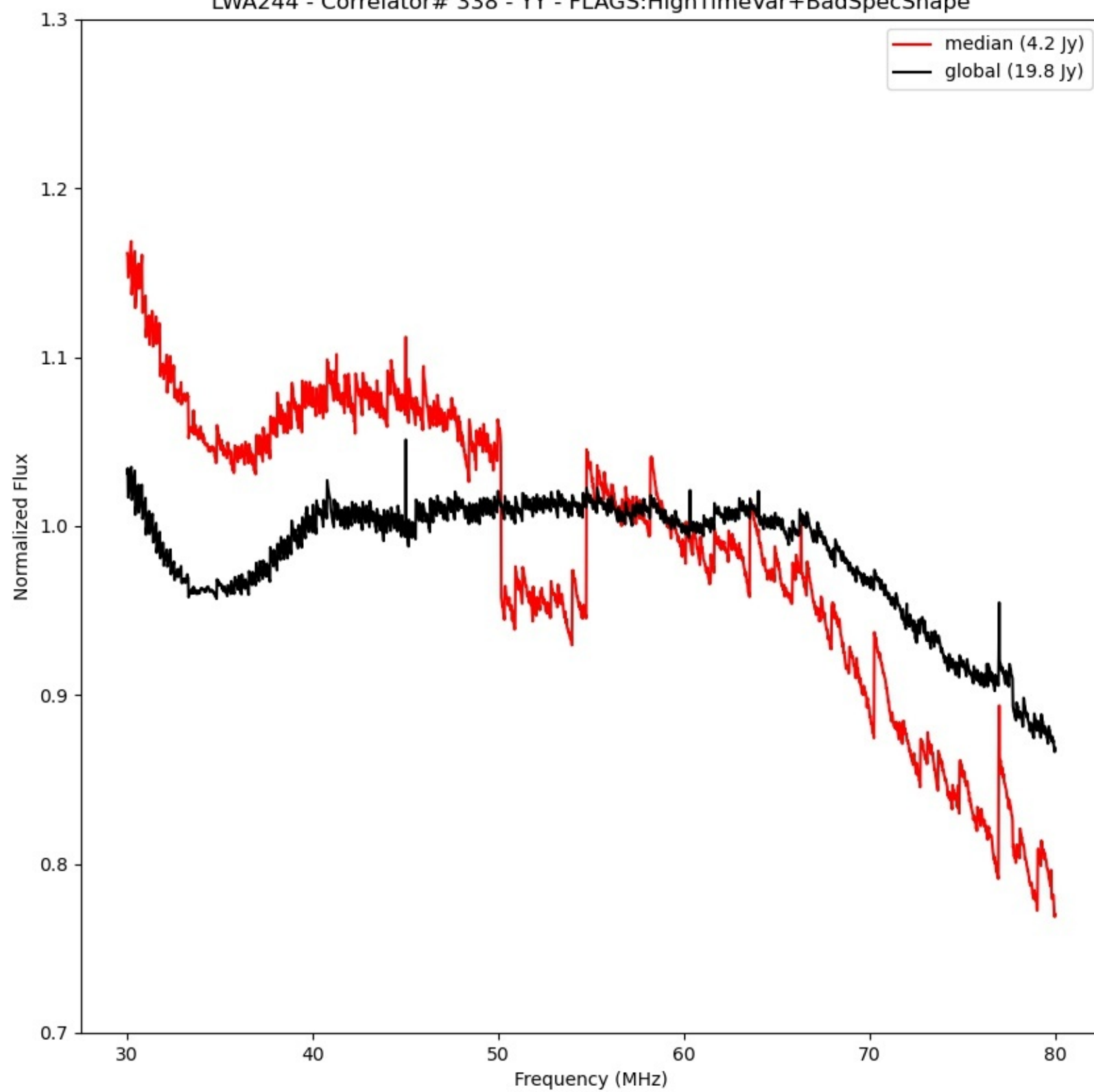
LWA244 - Correlator# 338 - YY - FLAGS:HighTimeVar+BadSpecShape
