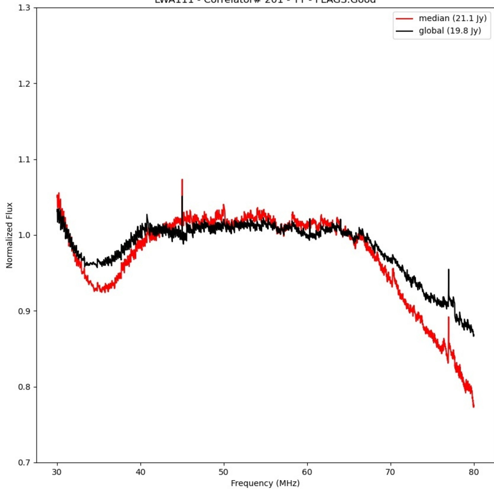
LWA111 - Correlator# 201 - YY - FLAGS:Good
