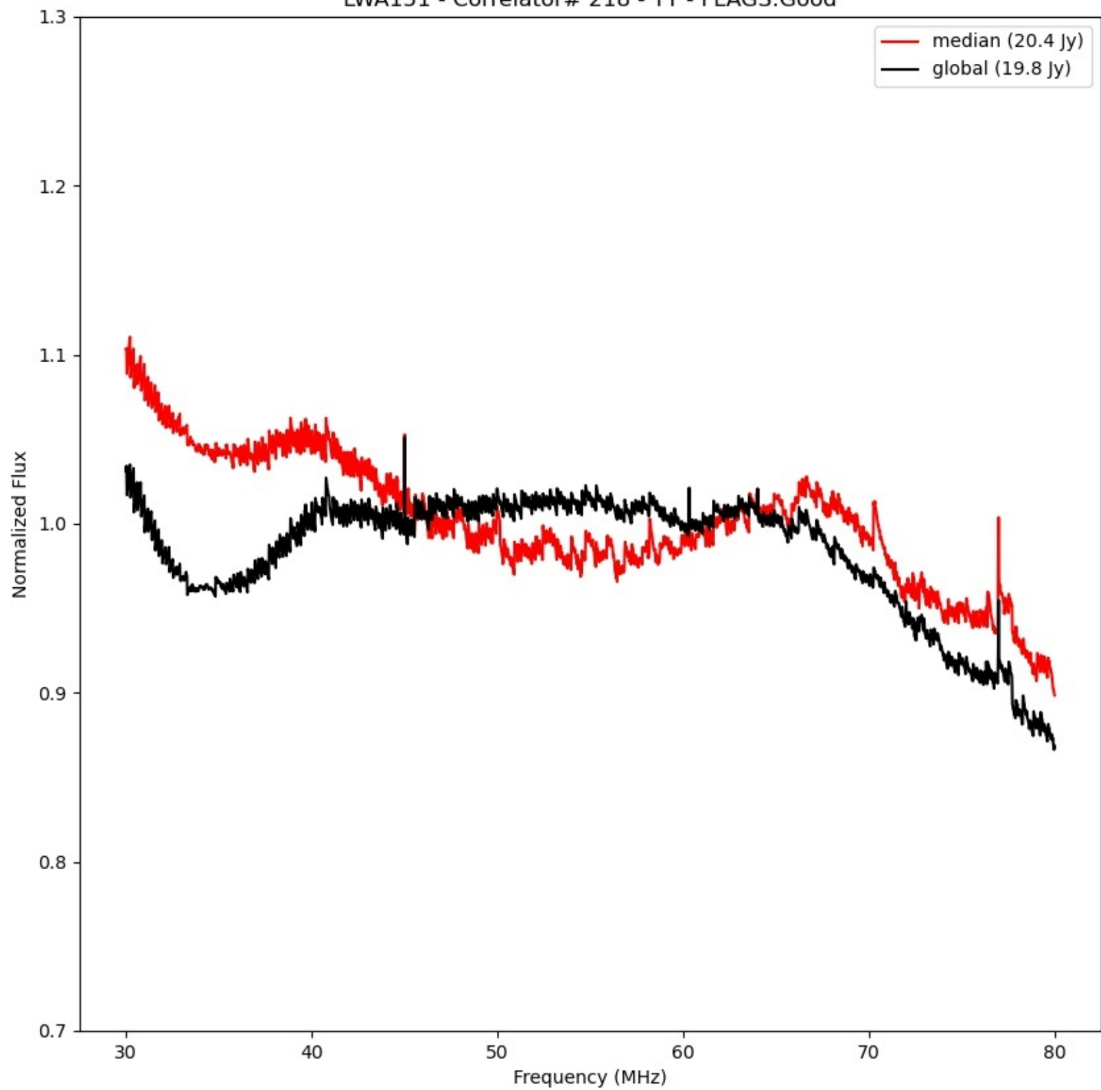
LWA151 - Correlator# 218 - YY - FLAGS:Good
