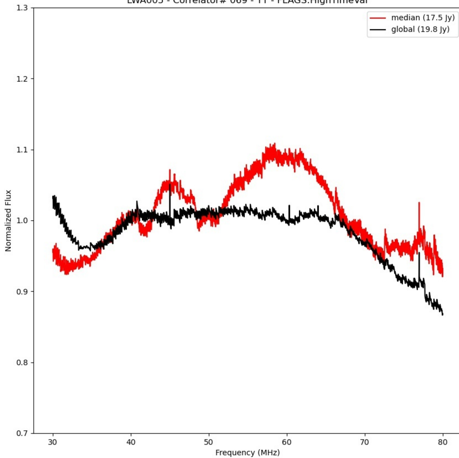
LWA005 - Correlator# 069 - YY - FLAGS:HighTimeVar
