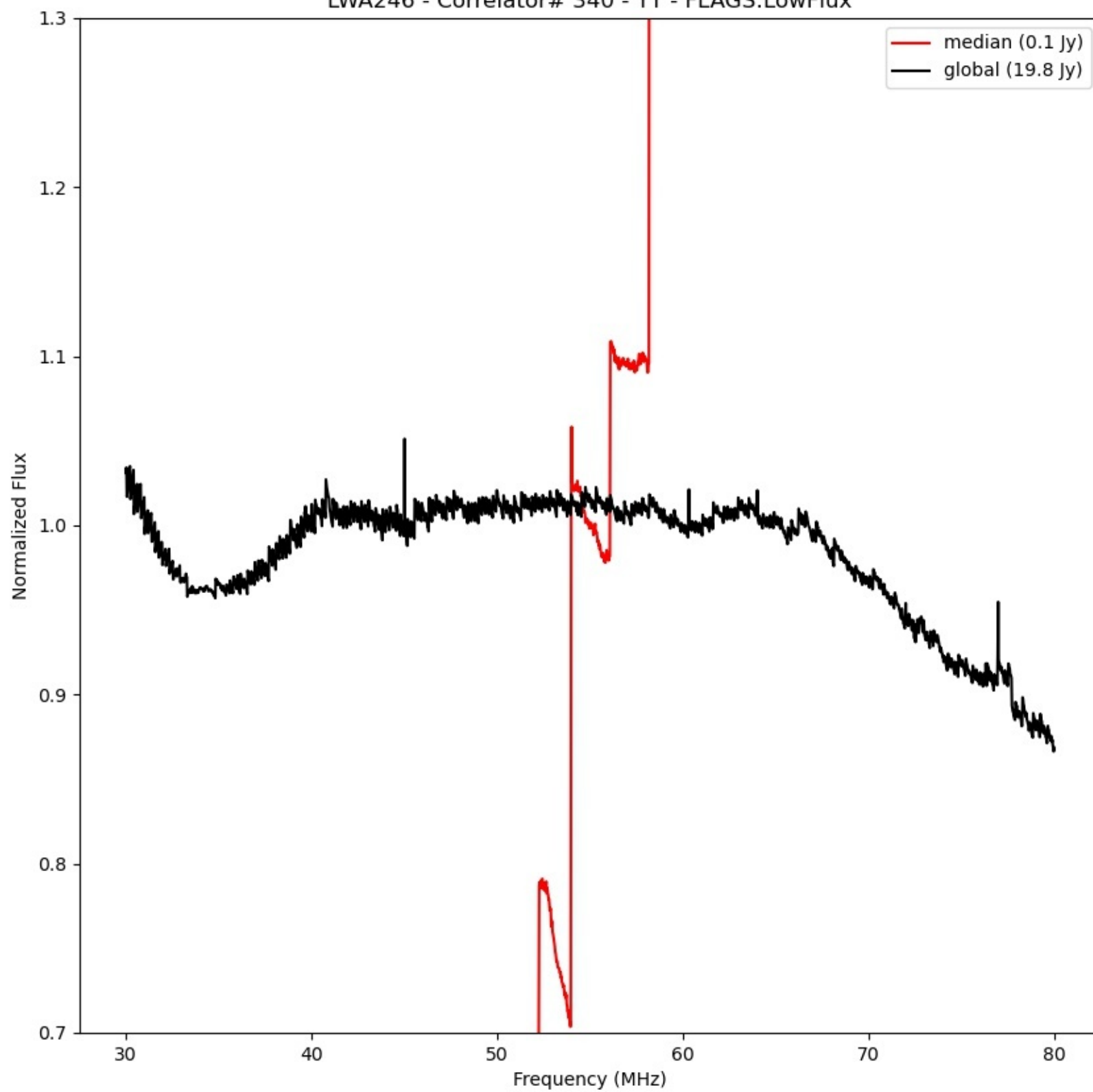
LWA246 - Correlator# 340 - YY - FLAGS:LowFlux
