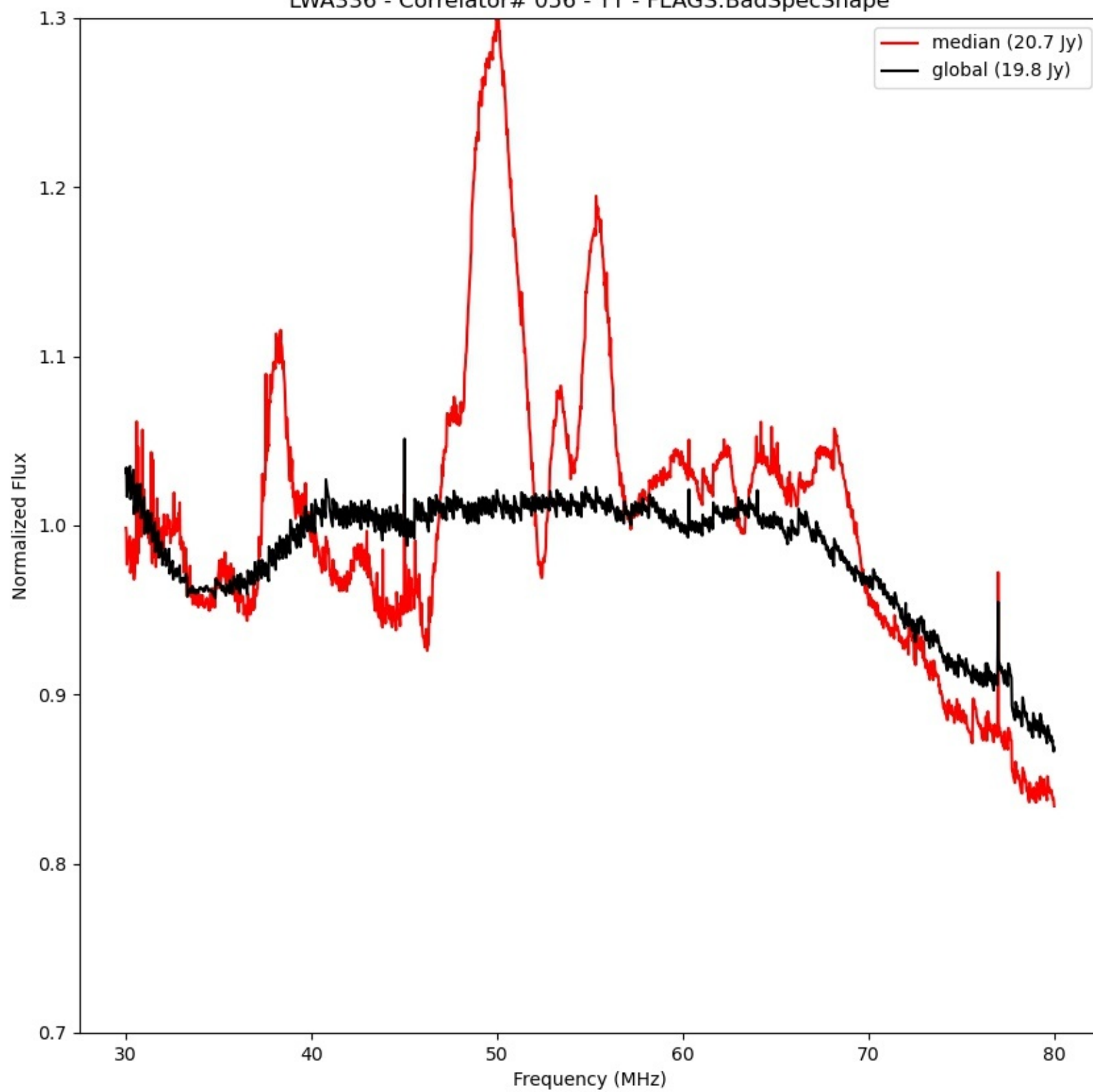
LWA336 - Correlator# 056 - YY - FLAGS:BadSpecShape
