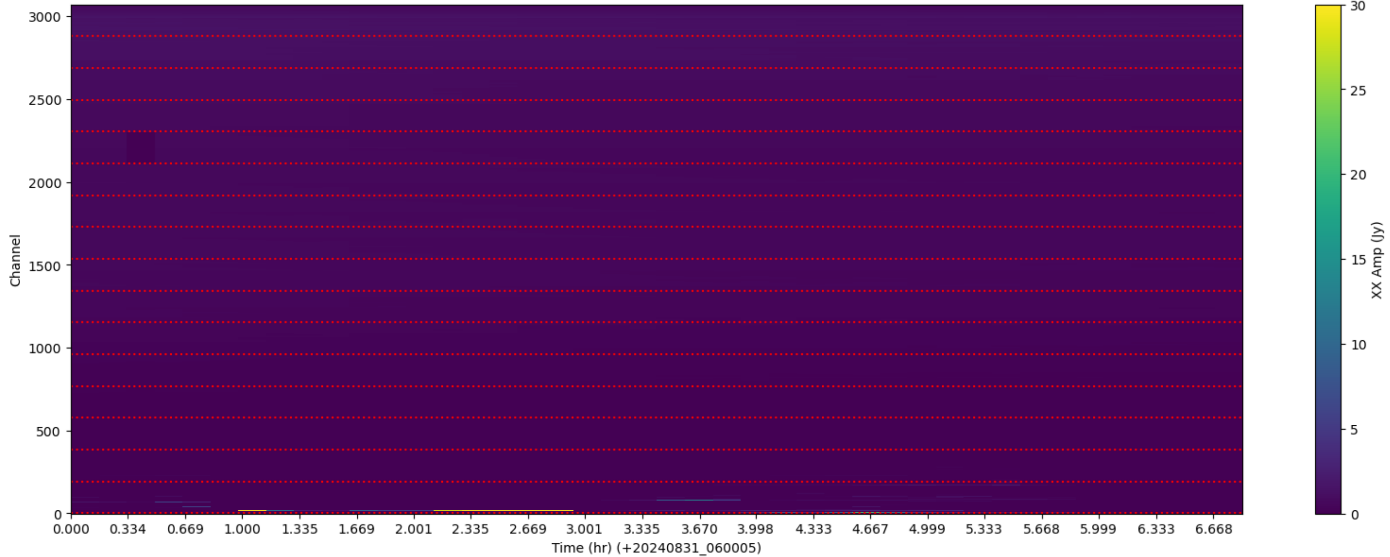
LWA135 - Correlator# 256 - XX - FLAGS: LowFlux
