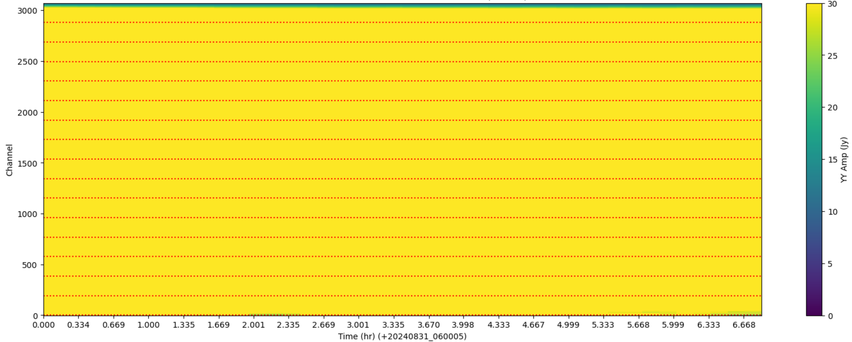
LWA002 - Correlator# 064 - YY - FLAGS: BadSpecShape
