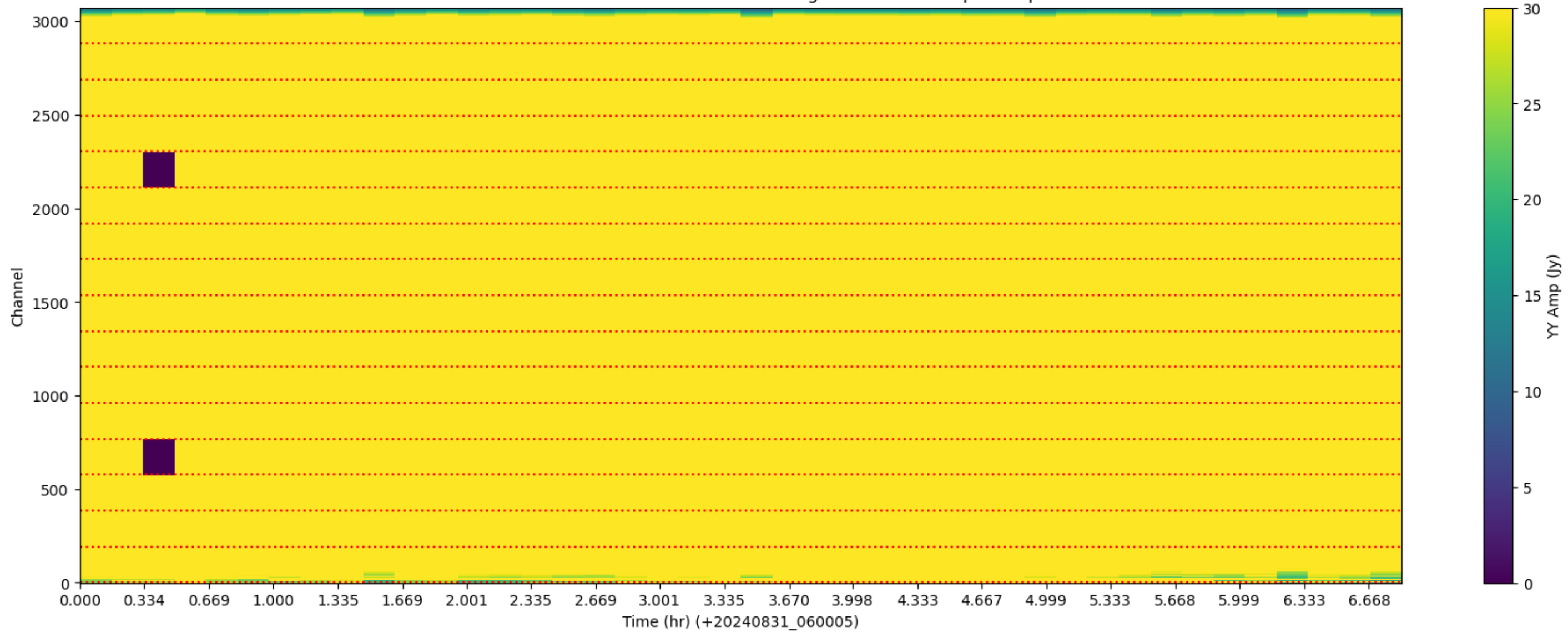
LWA158 - Correlator# 237 - YY - FLAGS: HighTimeVar+BadSpecShape
