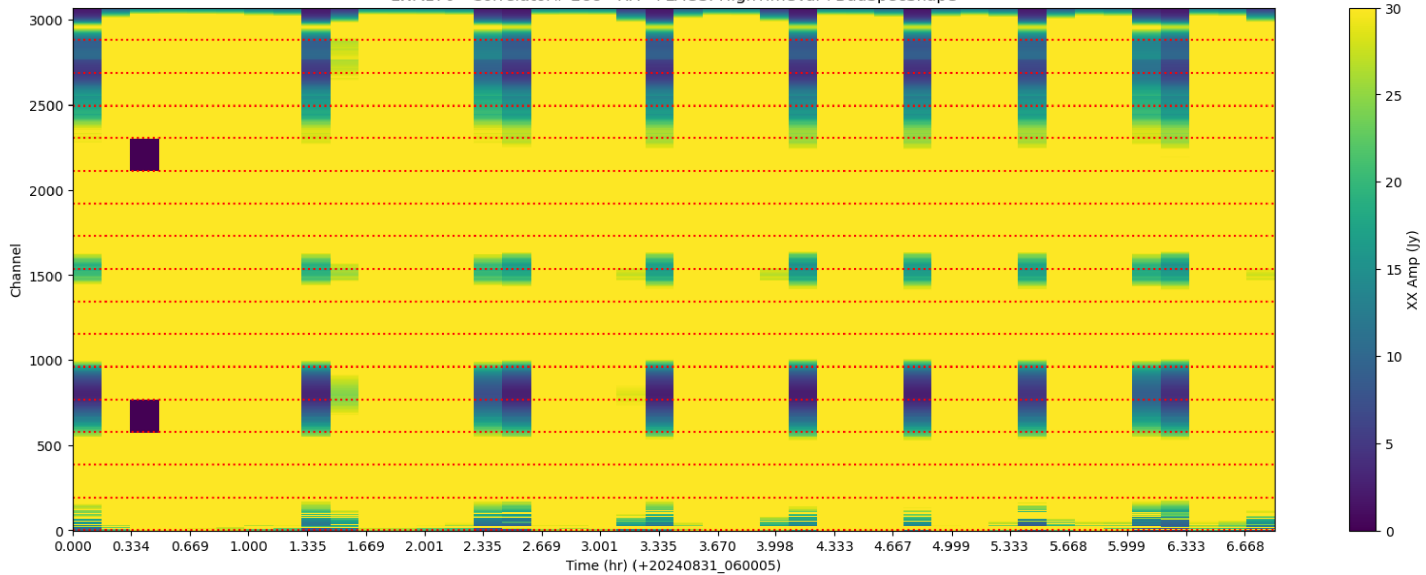
LWA170 - Correlator# 288 - XX - FLAGS: HighTimeVar+BadSpecShape
