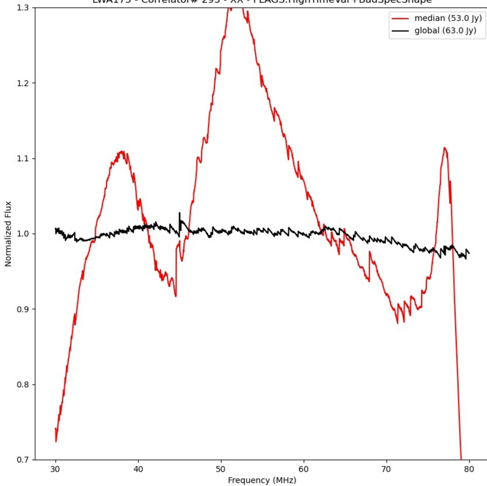
LWA175 - Correlator# 293 - XX - FLAGS:HighTimeVar+BadSpecShape
