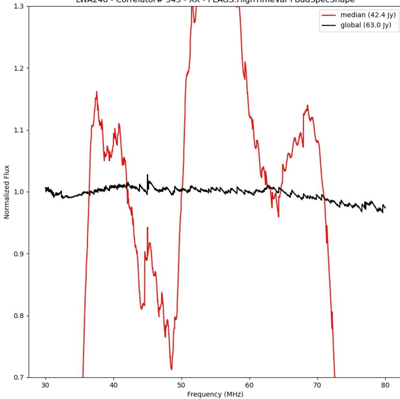
LWA248 - Correlator# 343 - XX - FLAGS:HighTimeVar+BadSpecShape
