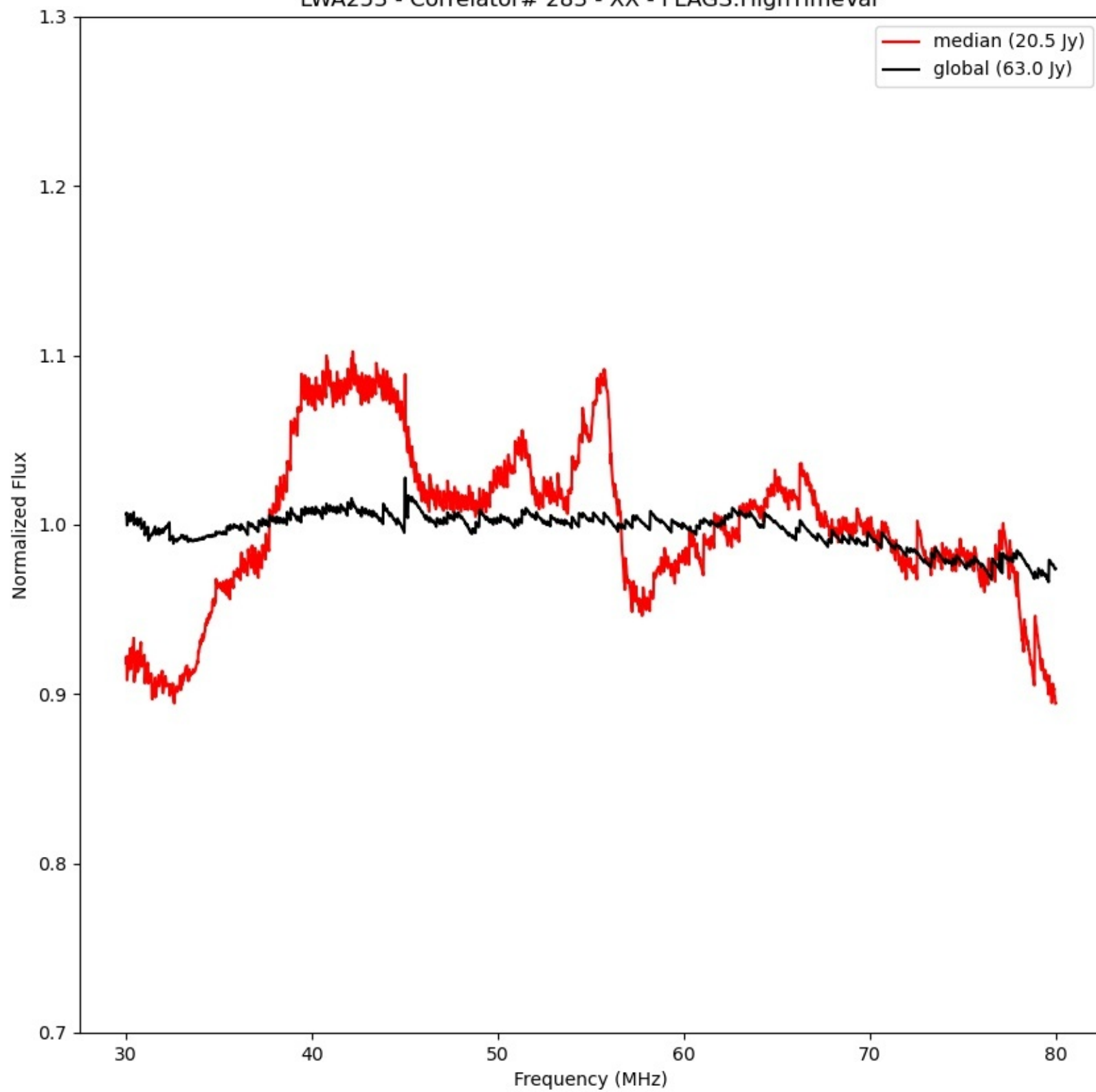
LWA253 - Correlator# 283 - XX - FLAGS:HighTimeVar
