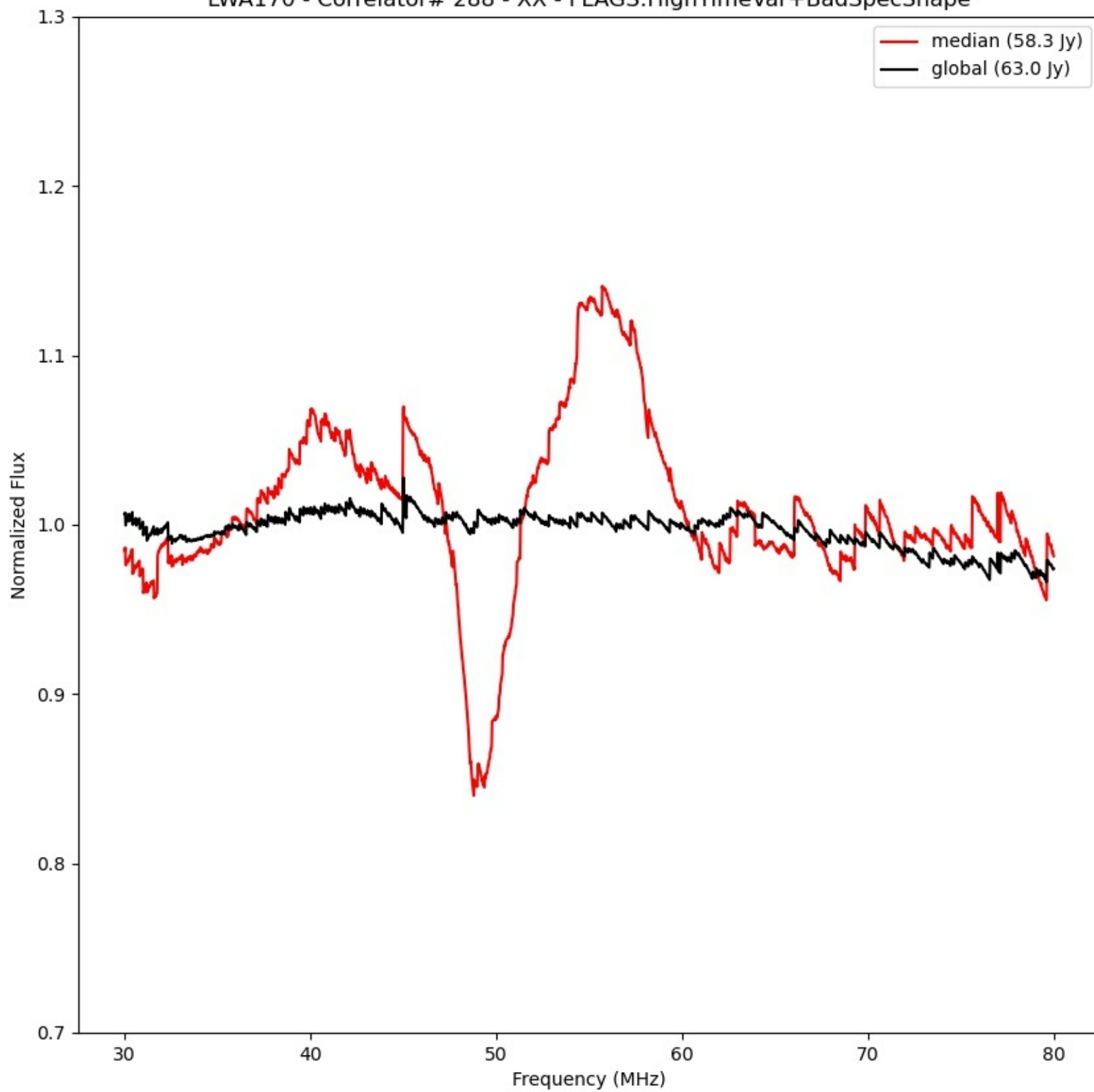
LWA170 - Correlator# 288 - XX - FLAGS:HighTimeVar+BadSpecShape
