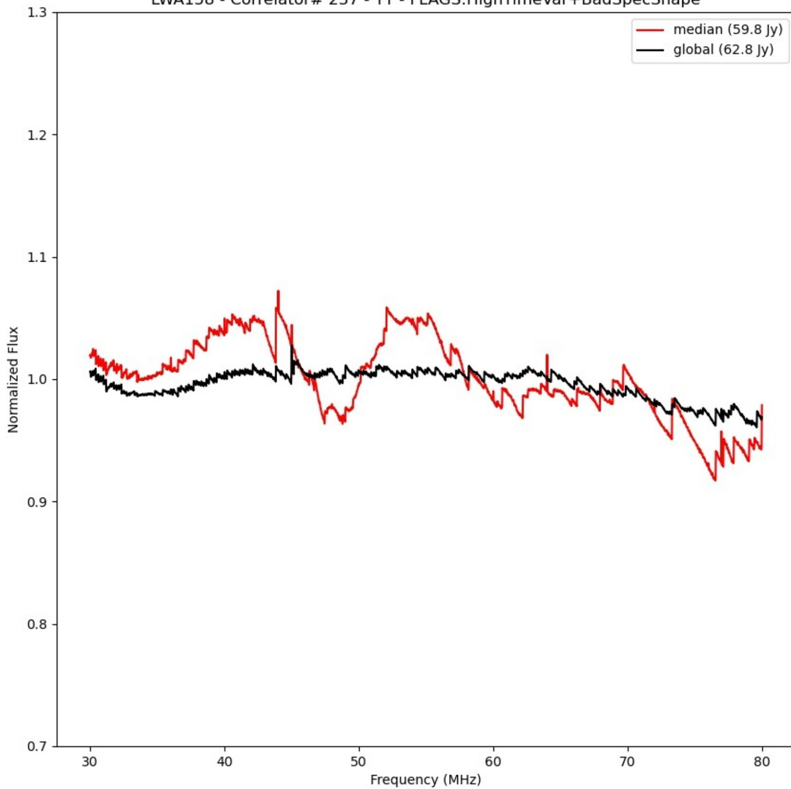
LWA158 - Correlator# 237 - YY - FLAGS:HighTimeVar+BadSpecShape
