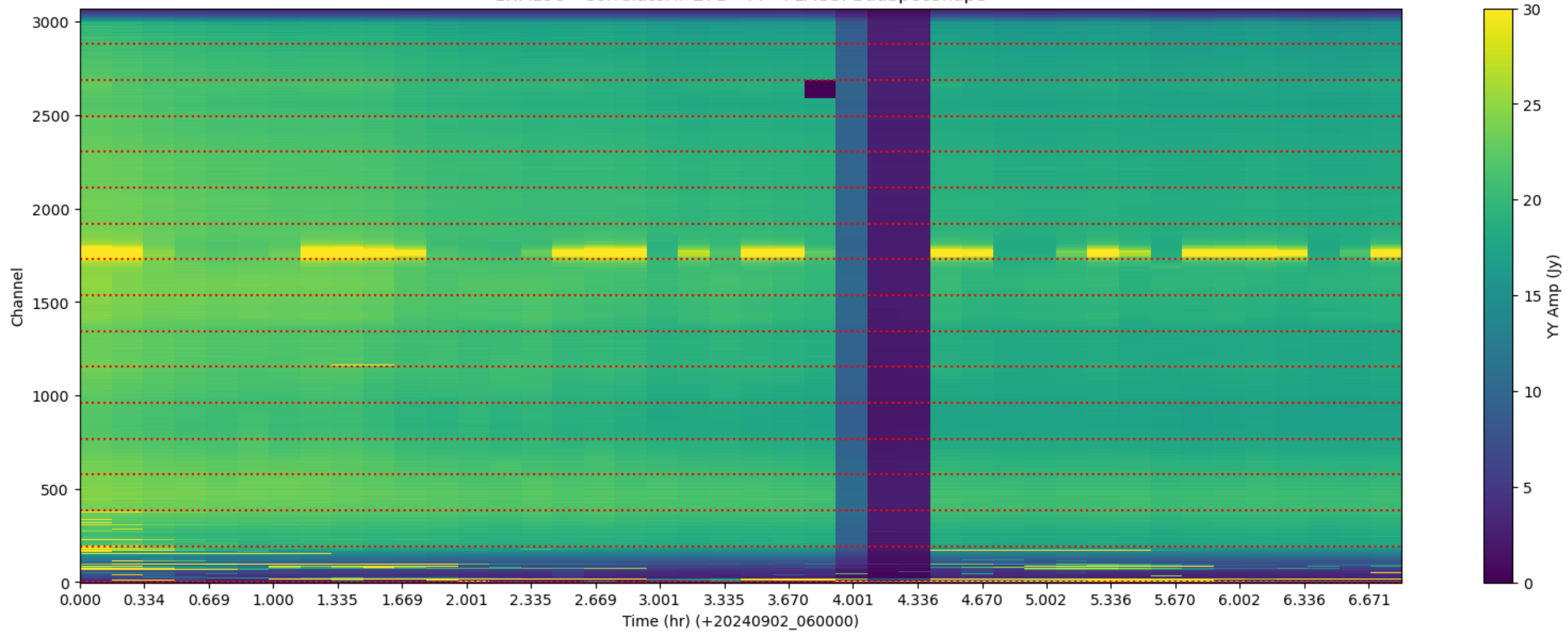
LWA198 - Correlator# 271 - YY - FLAGS: BadSpecShape
