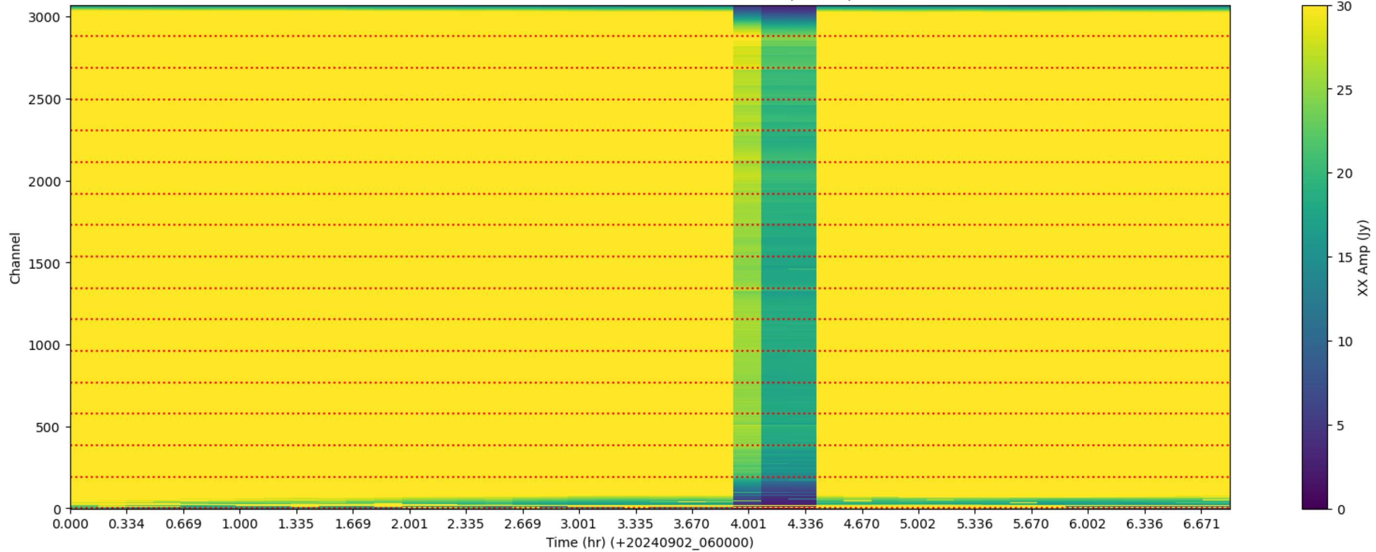
LWA010 - Correlator# 073 - XX - FLAGS: BadSpecShape
