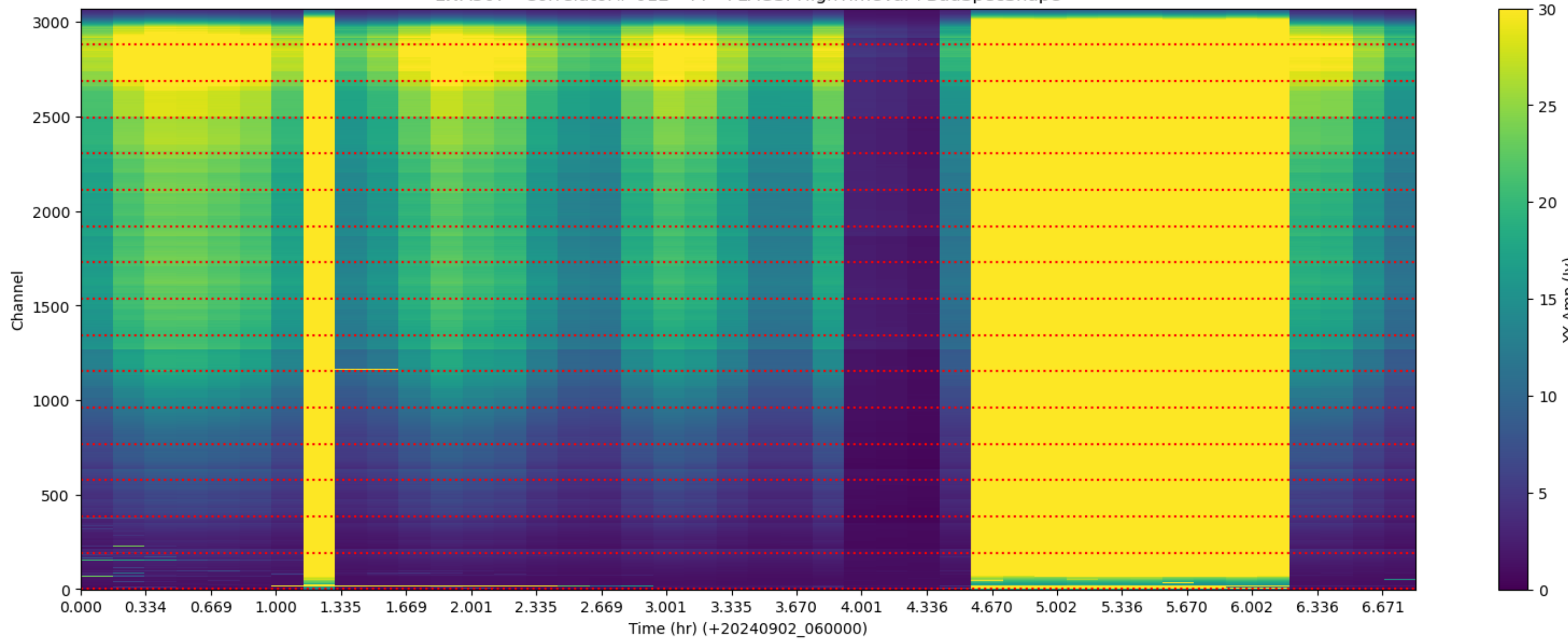
LWA307 - Correlator# 012 - YY - FLAGS: HighTimeVar+BadSpecShape
