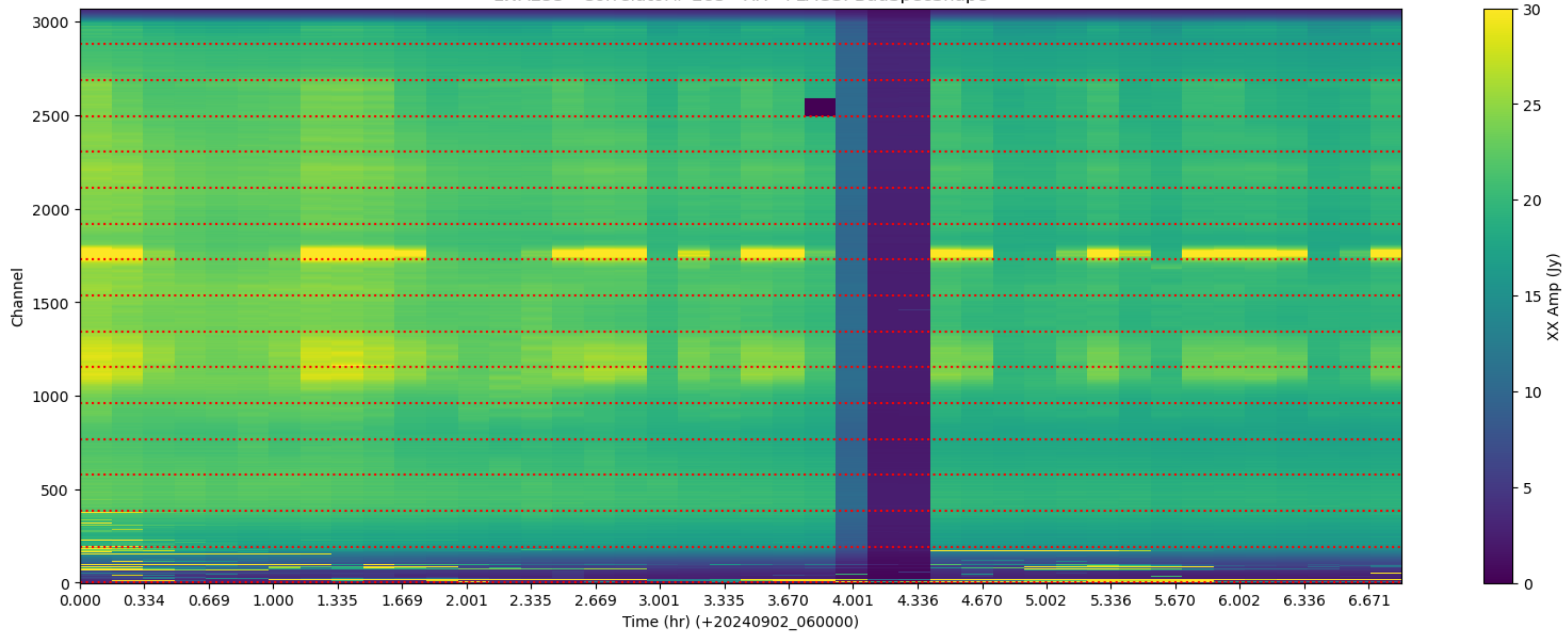
LWA253 - Correlator# 283 - XX - FLAGS: BadSpecShape
