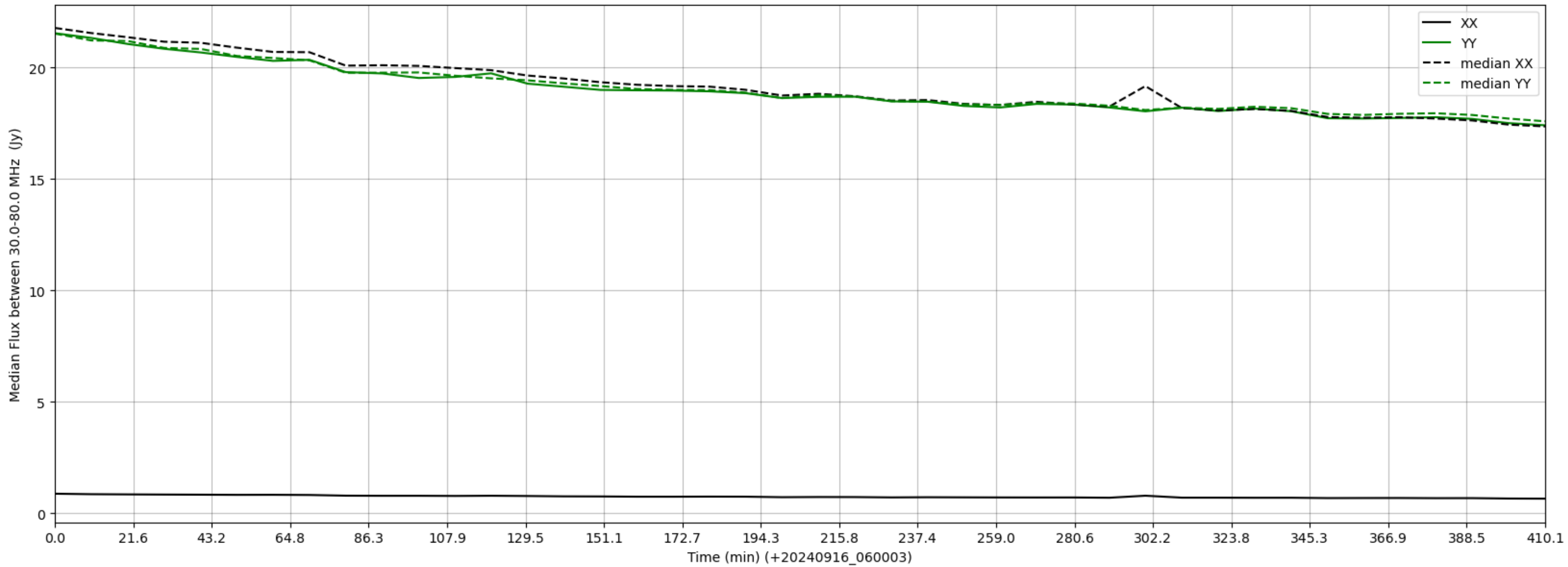
LWA284 - Correlator# 043 - XX FLAGS:LowFlux - YY FLAGS:Good
