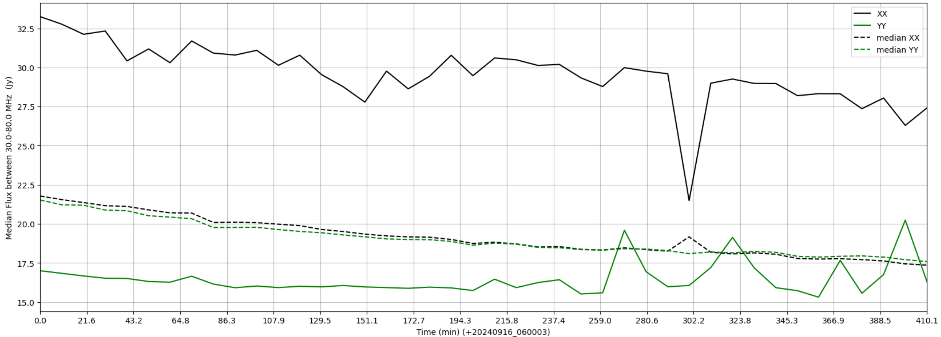
LWA310 - Correlator# 017 - XX FLAGS:Good - YY FLAGS:HighTimeVar
