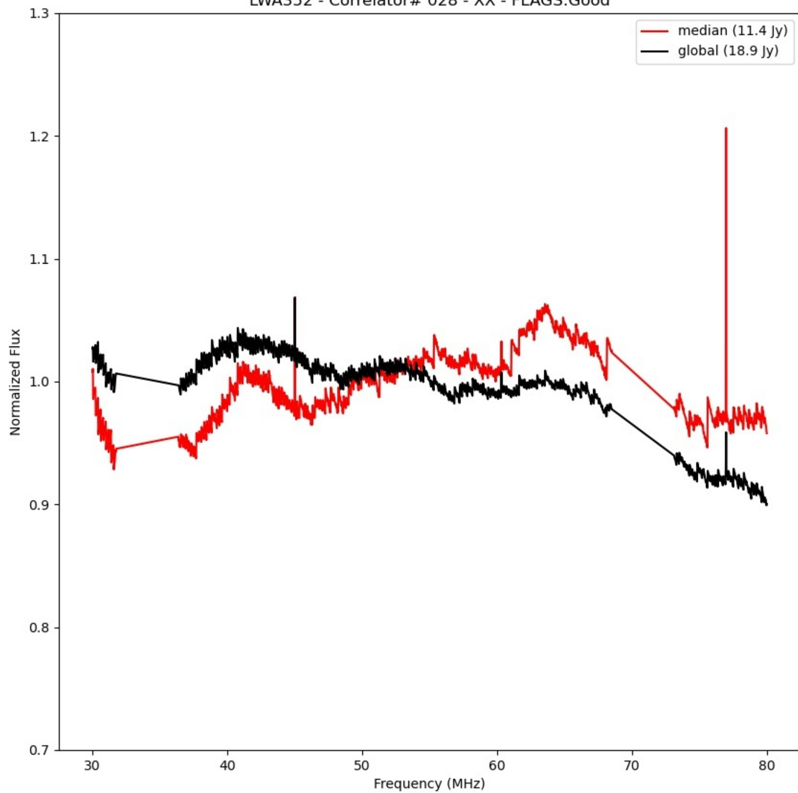
LWA352 - Correlator# 028 - XX - FLAGS:Good
