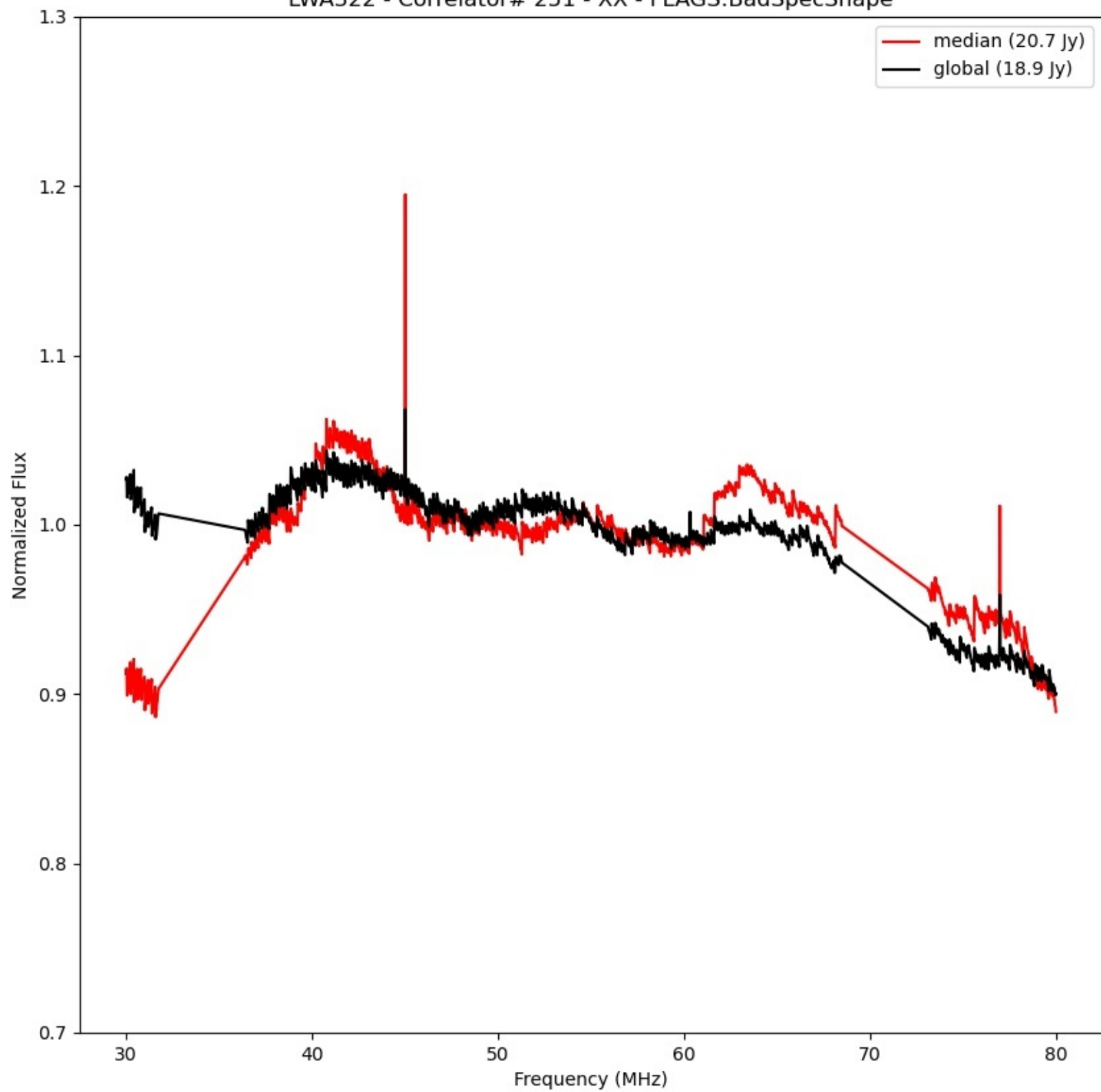
LWA322 - Correlator# 251 - XX - FLAGS:BadSpecShape
