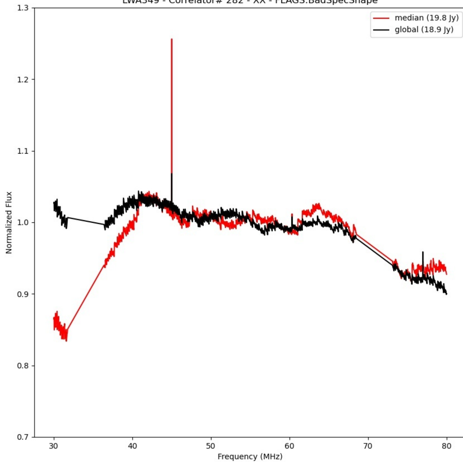
LWA349 - Correlator# 282 - XX - FLAGS:BadSpecShape
