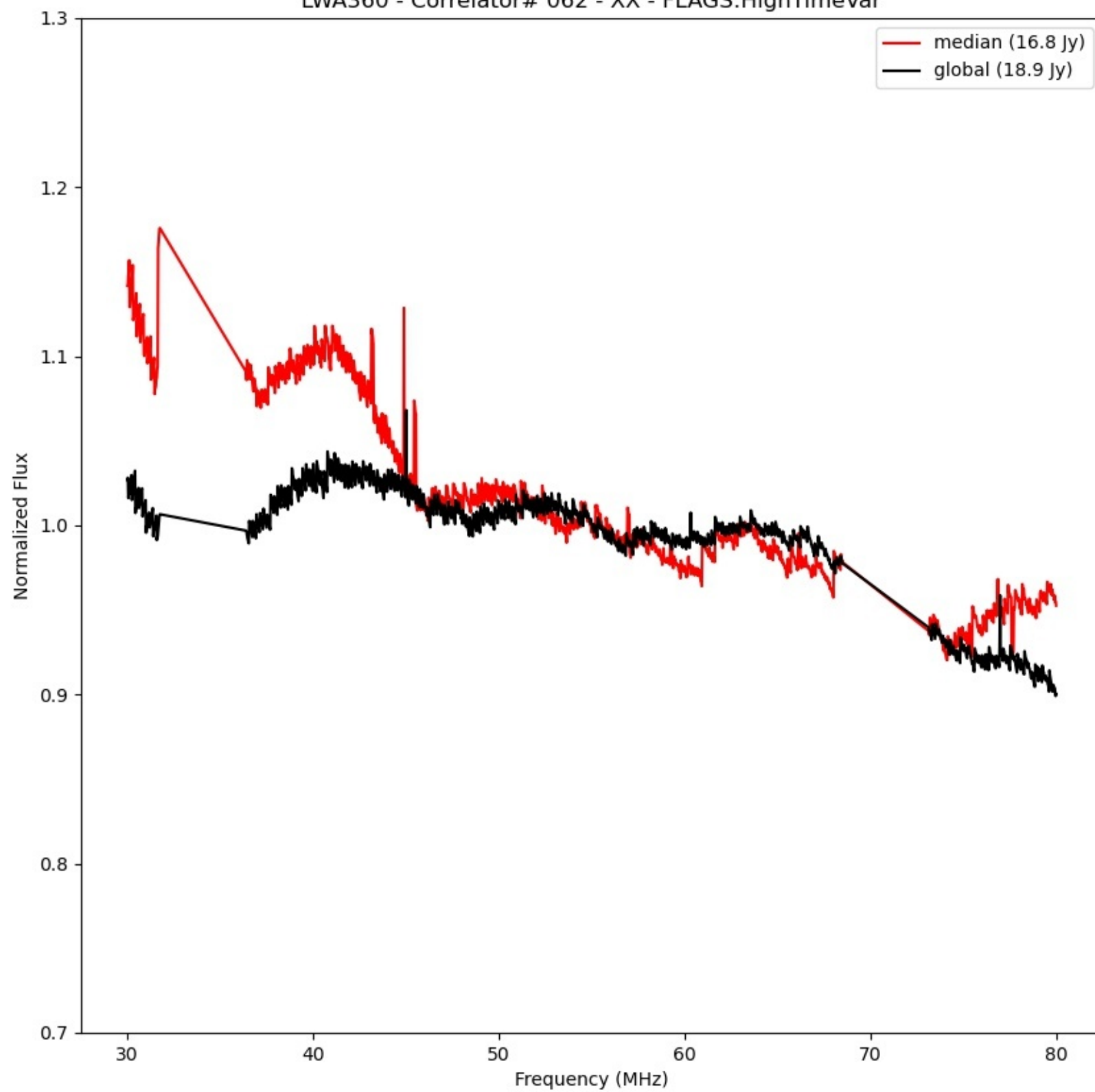
LWA360 - Correlator# 062 - XX - FLAGS:HighTimeVar
