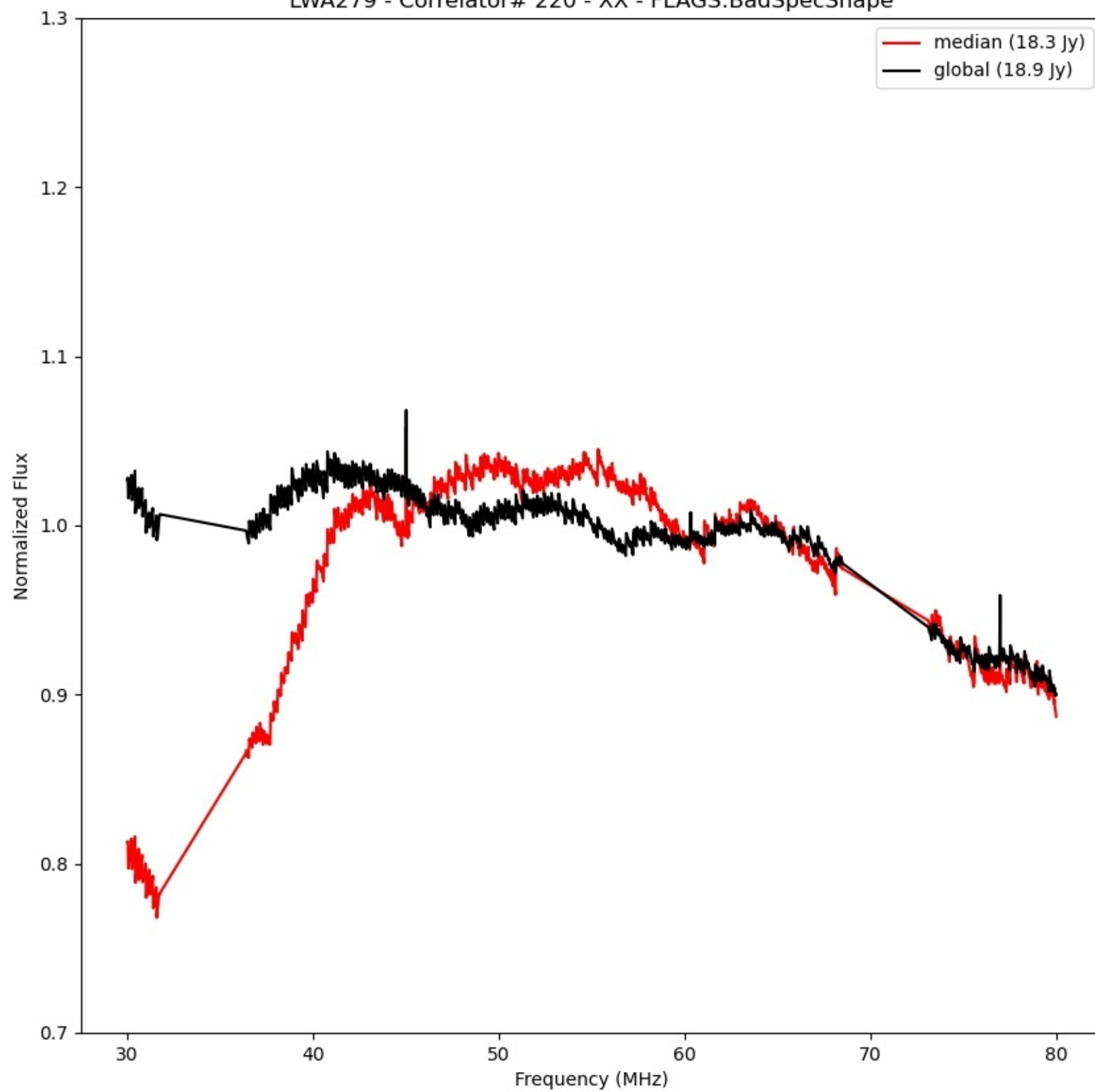
LWA279 - Correlator# 220 - XX - FLAGS:BadSpecShape
