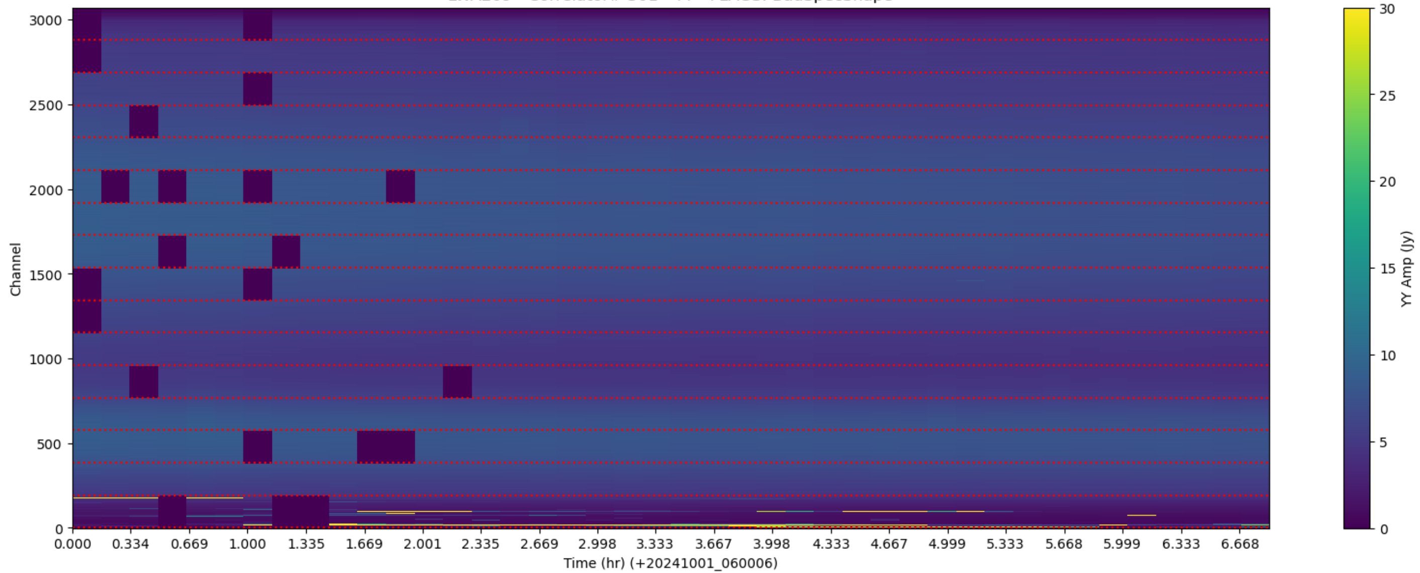
LWA209 - Correlator# 301 - YY - FLAGS: BadSpecShape
