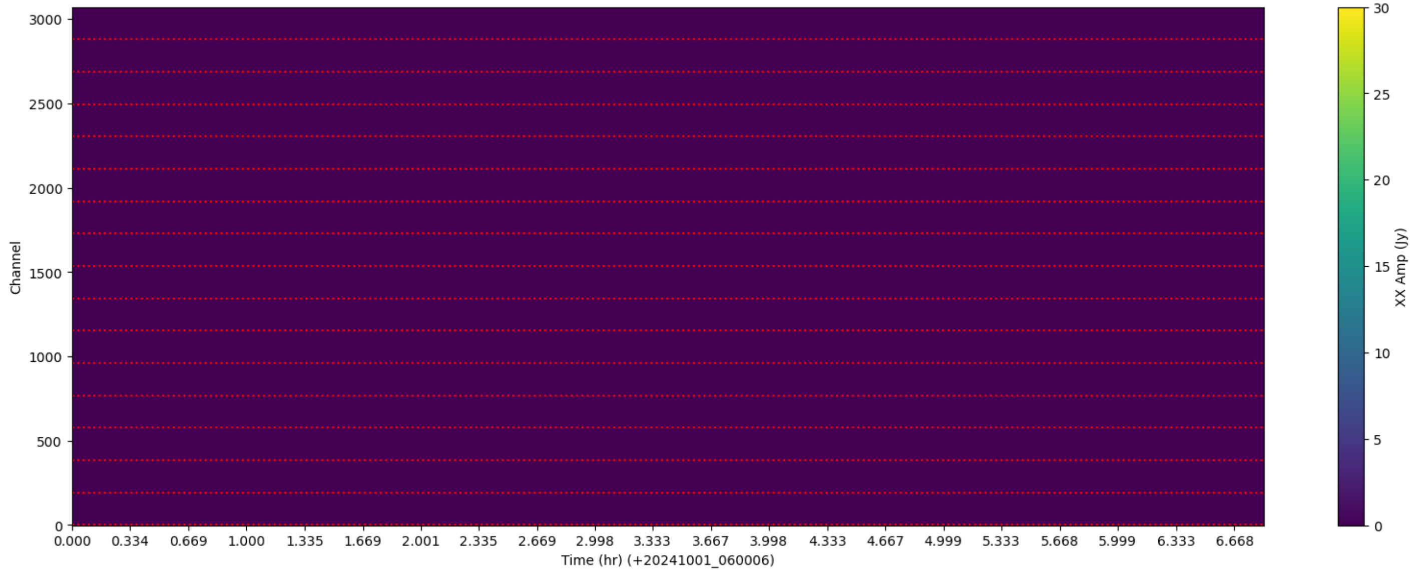
LWA209 - Correlator# 301 - XX - FLAGS: LowFlux
