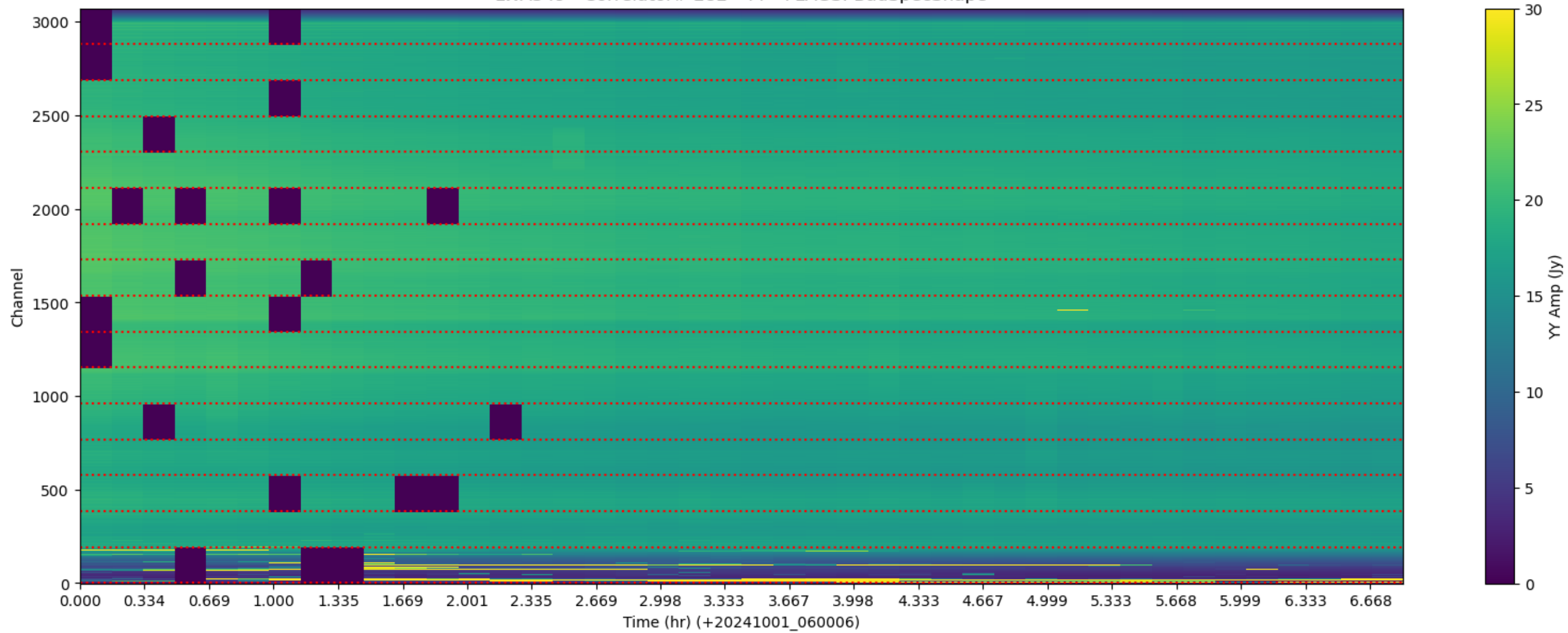
LWA349 - Correlator# 282 - YY - FLAGS: BadSpecShape
