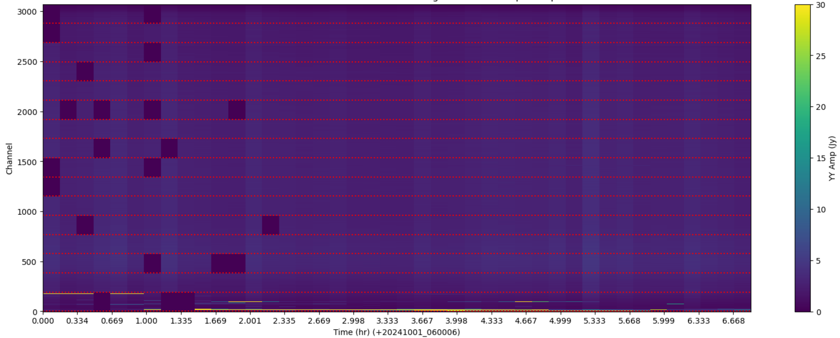
LWA244 - Correlator# 338 - YY - FLAGS: HighTimeVar+BadSpecShape
