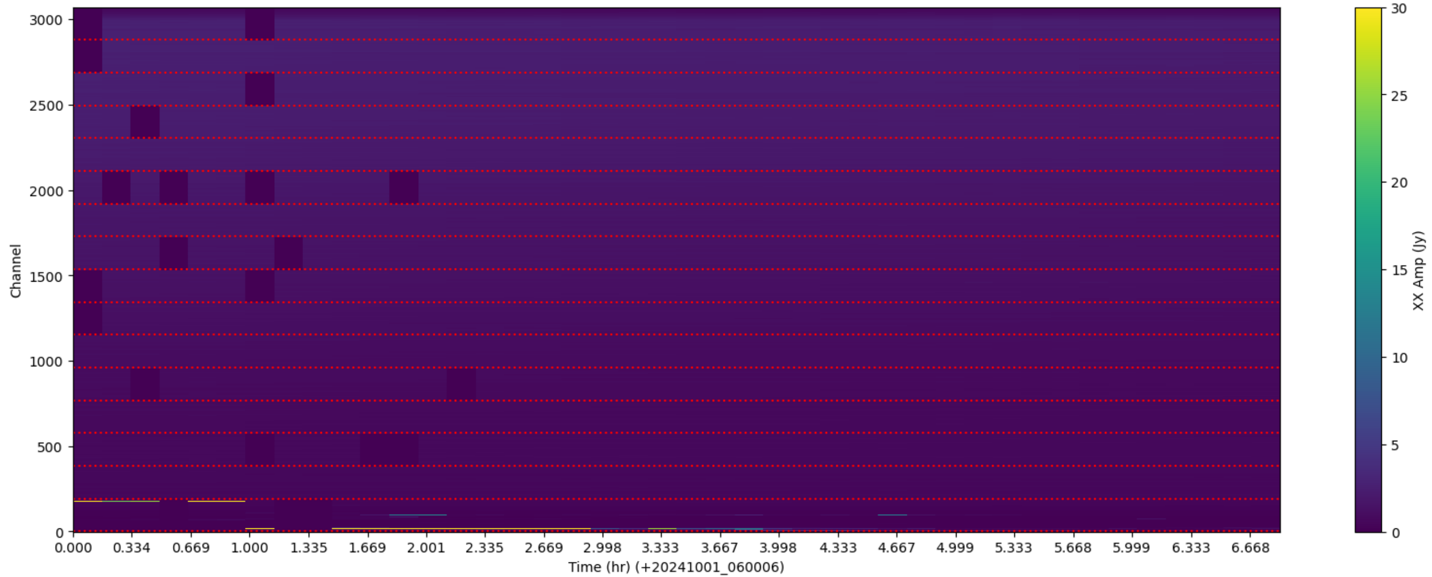
LWA235 - Correlator# 309 - XX - FLAGS: LowFlux
