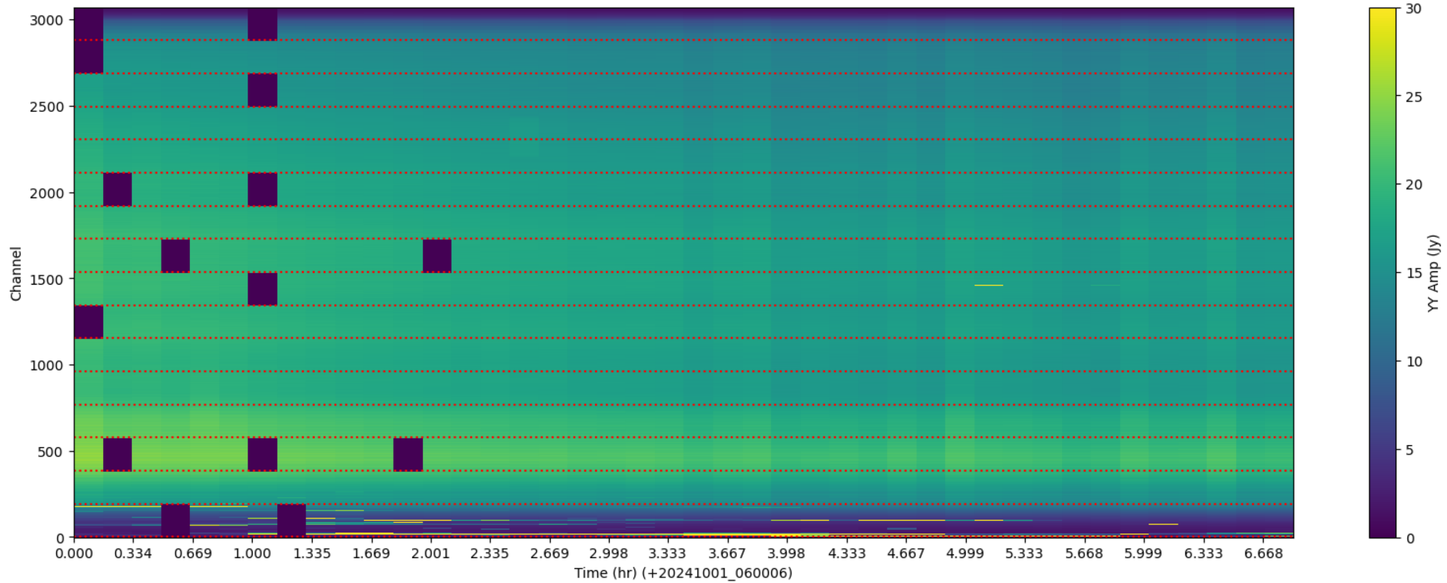
LWA307 - Correlator# 012 - YY - FLAGS: Good
