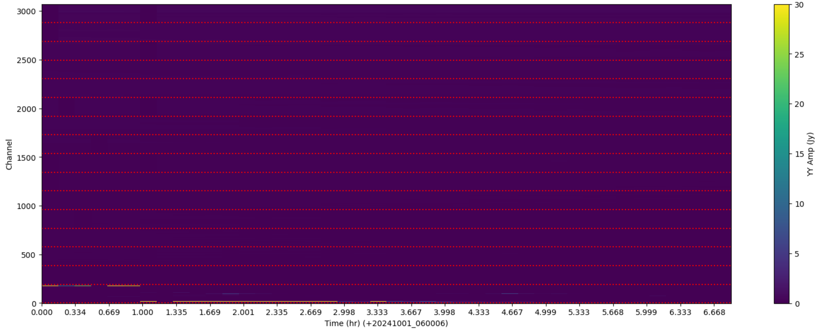
LWA066 - Correlator# 164 - YY - FLAGS: LowFlux
