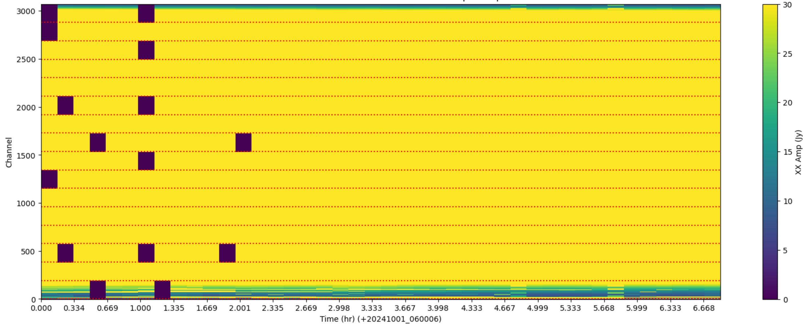
LWA362 - Correlator# 030 - XX - FLAGS: BadSpecShape
