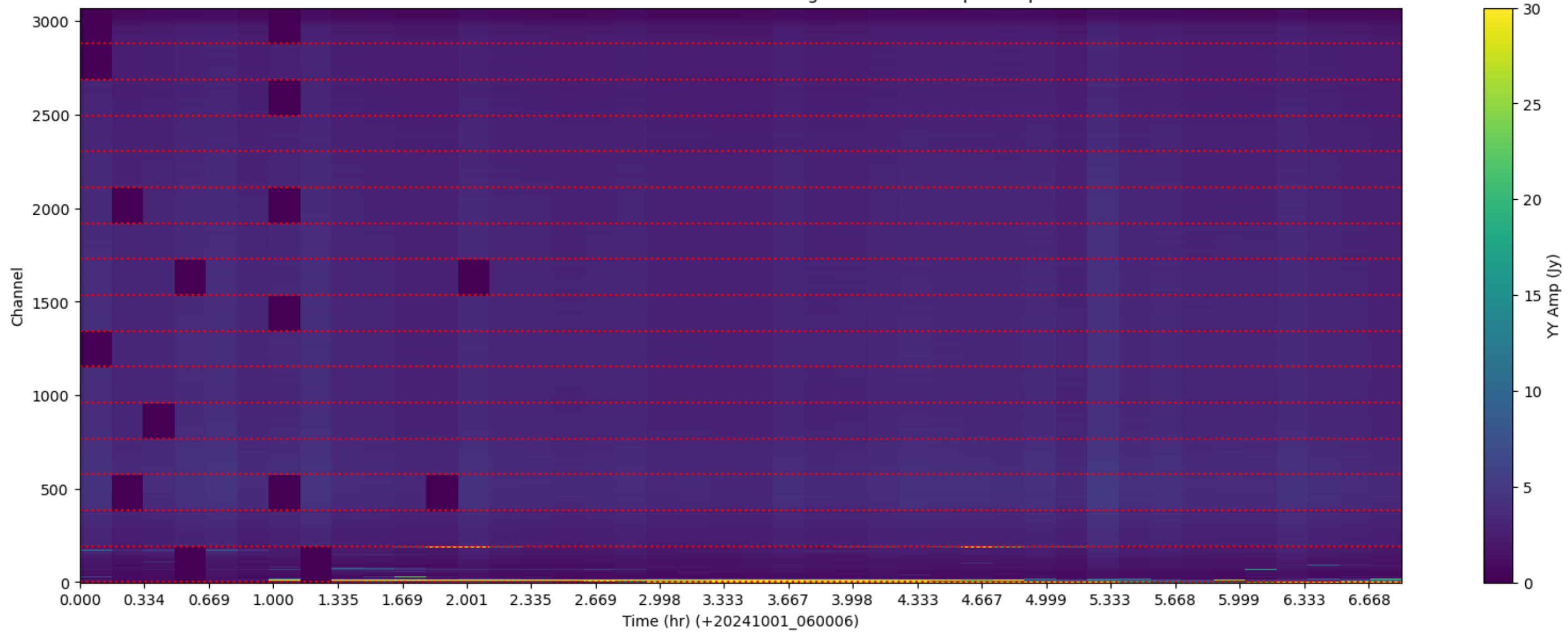
LWA305 - Correlator# 050 - YY - FLAGS: HighTimeVar+BadSpecShape
