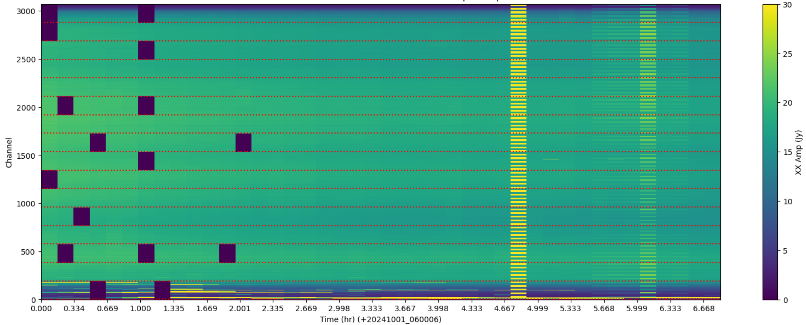
LWA005 - Correlator# 069 - XX - FLAGS: BadSpecShape
