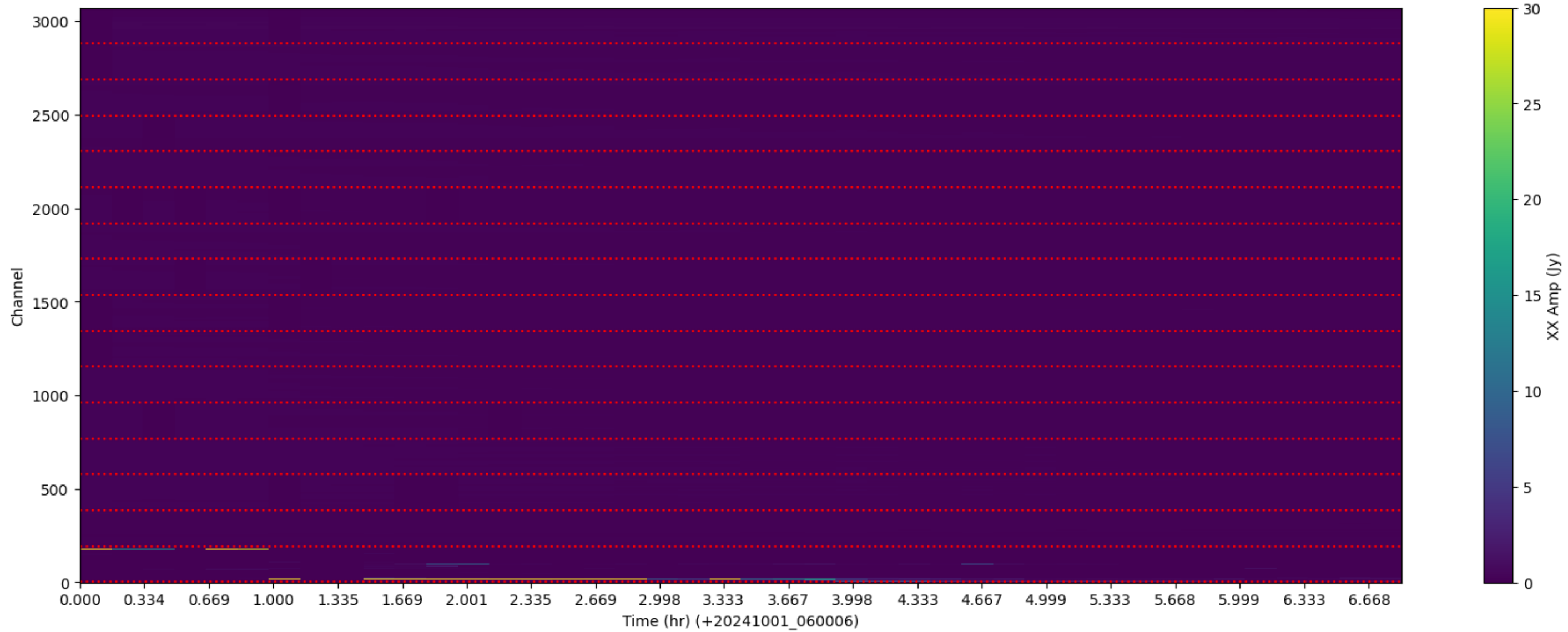
LWA215 - Correlator# 331 - XX - FLAGS: LowFlux
