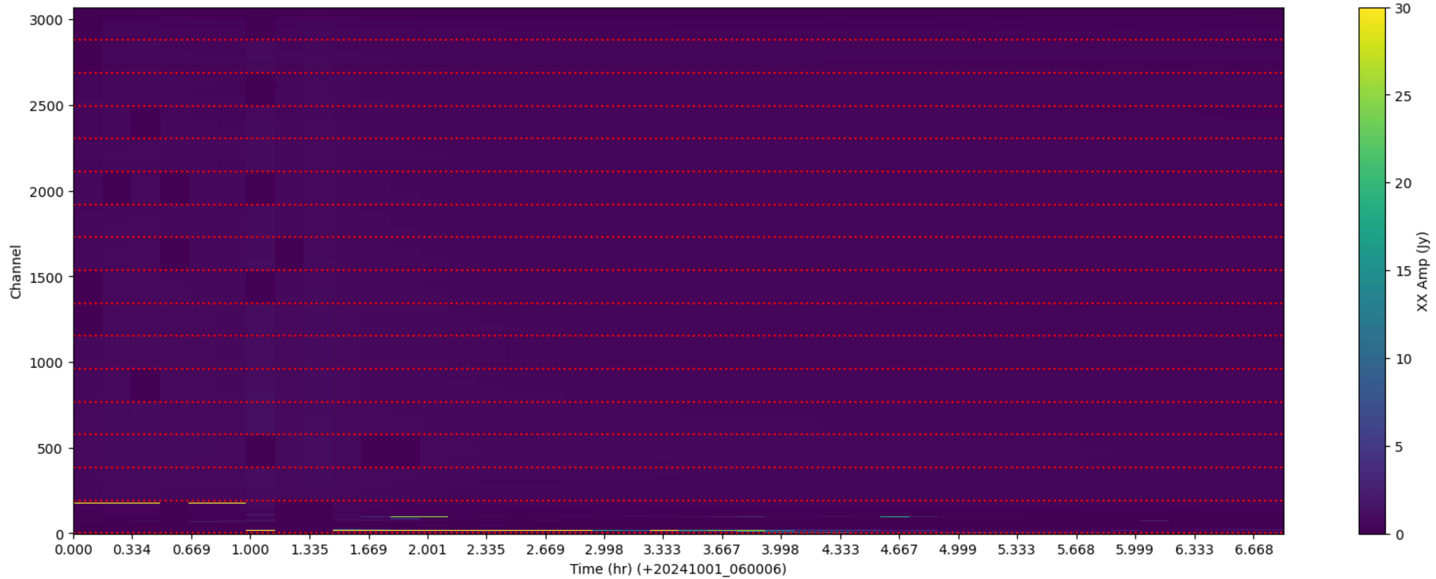
LWA150 - Correlator# 215 - XX - FLAGS: LowFlux
