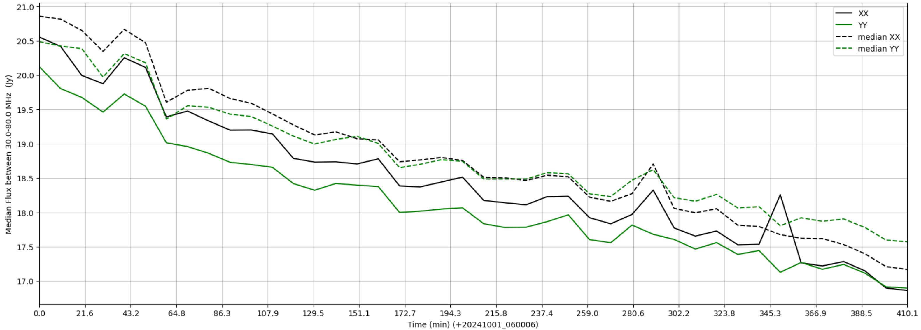
LWA280 - Correlator# 041 - XX FLAGS:Good - YY FLAGS:Good
