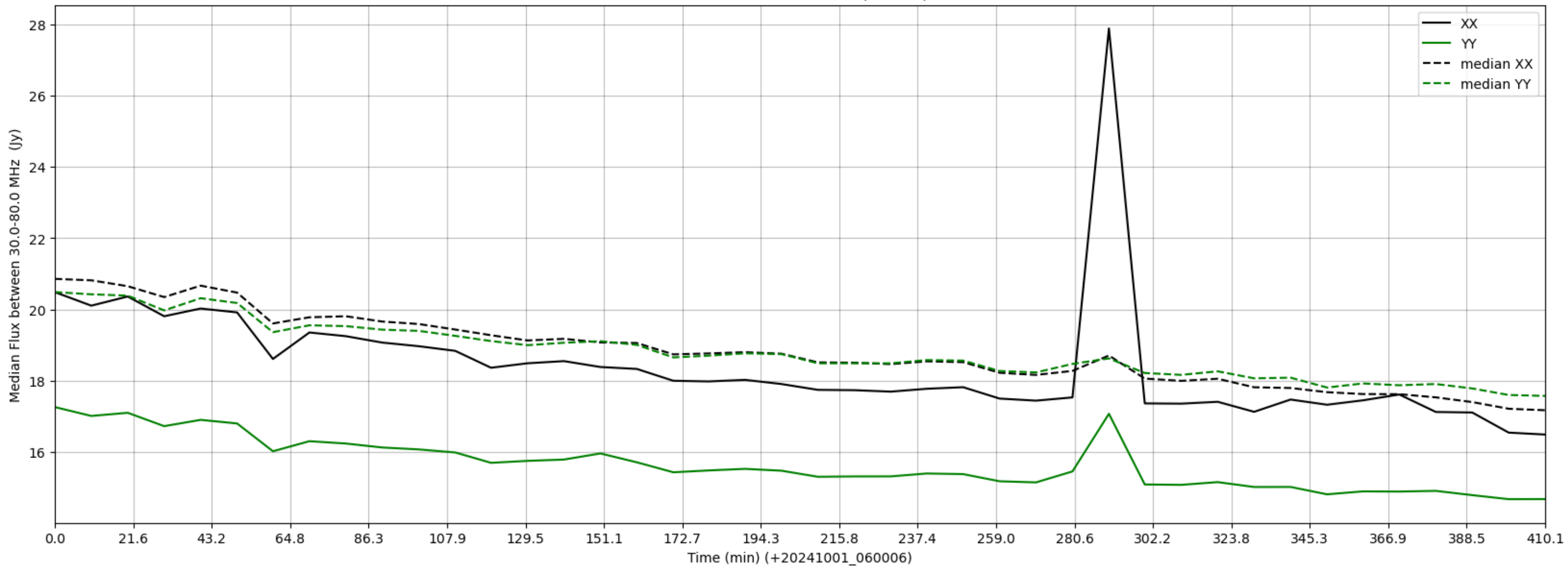
LWA005 - Correlator# 069 - XX FLAGS:BadSpecShape - YY FLAGS:Good
