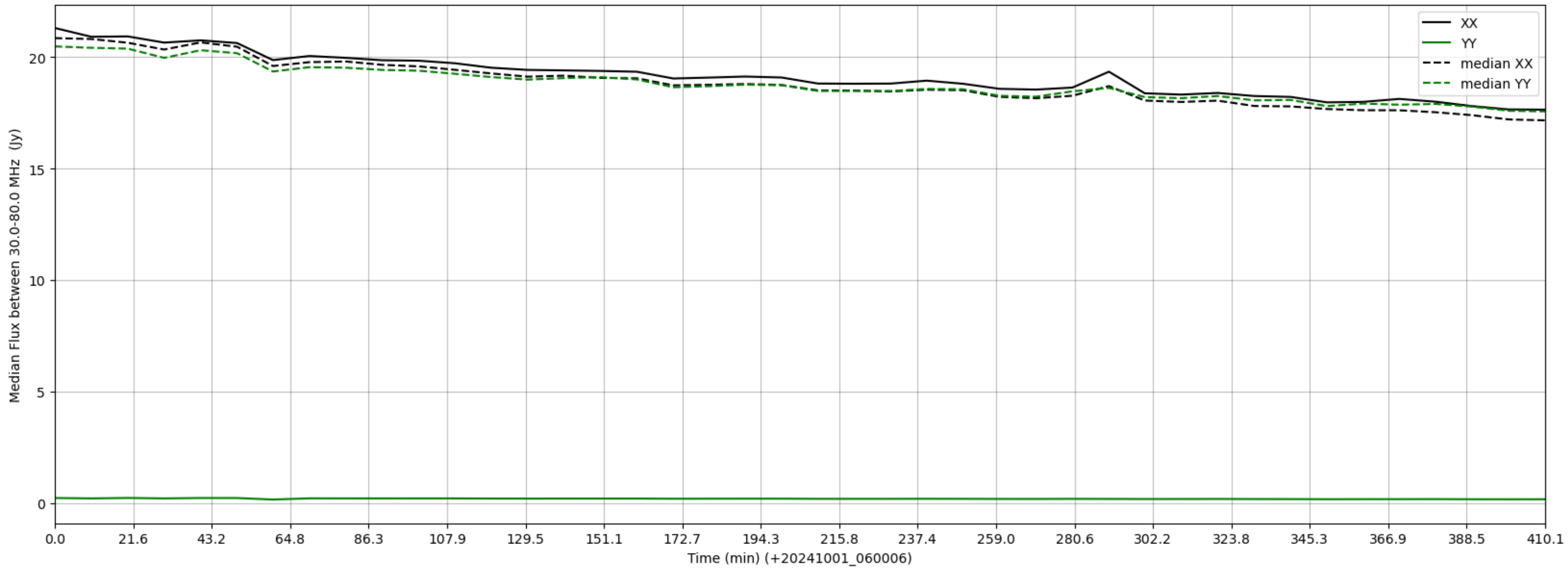
LWA066 - Correlator# 164 - XX FLAGS:Good - YY FLAGS:LowFlux
