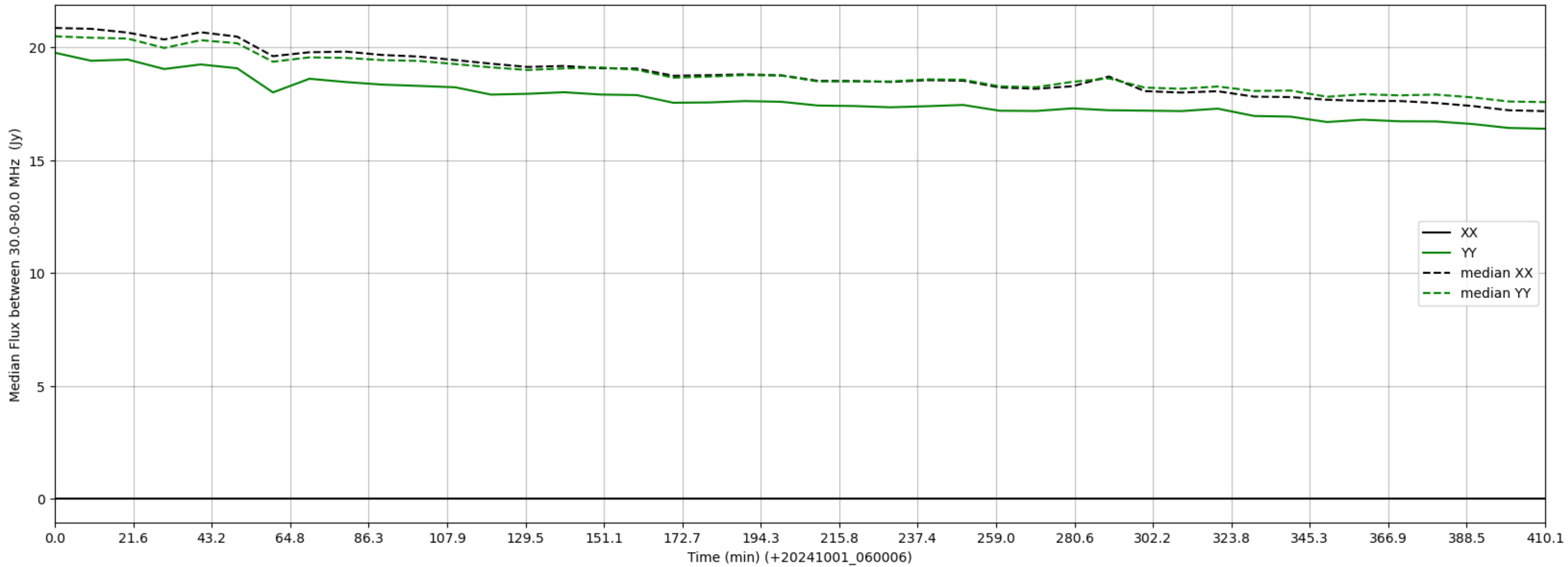
LWA339 - Correlator# 027 - XX FLAGS:LowFlux - YY FLAGS:Good
