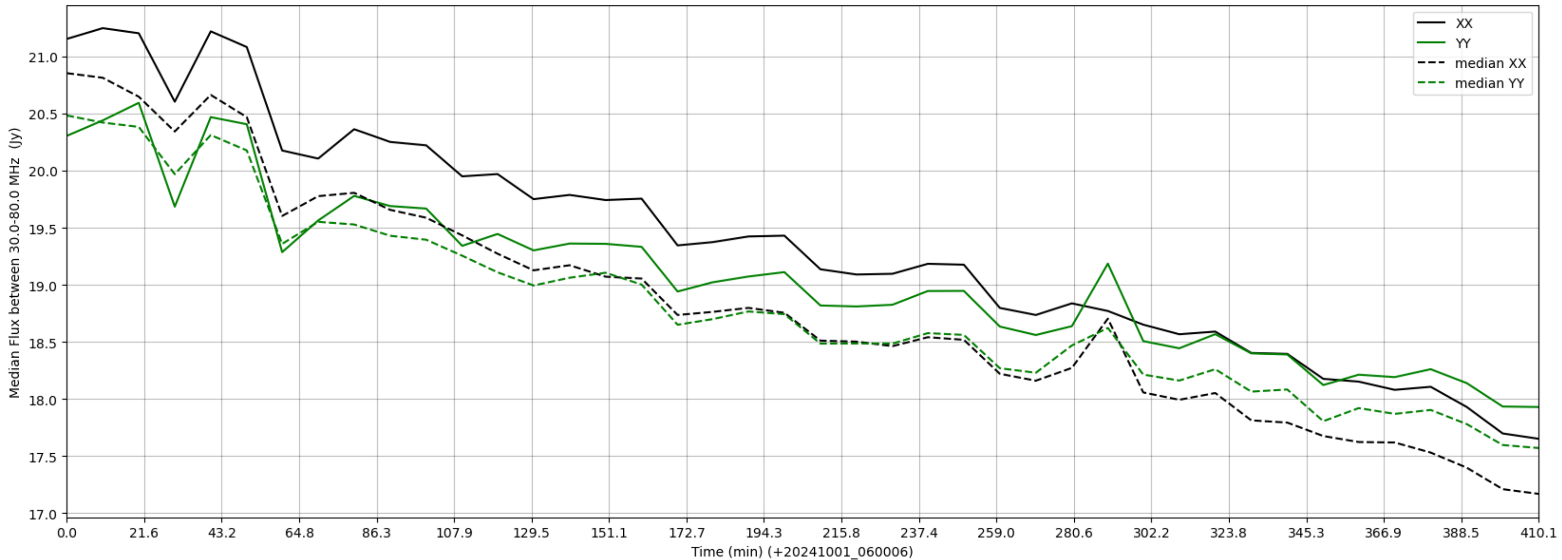
LWA253 - Correlator# 283 - XX FLAGS:Good - YY FLAGS:Good
