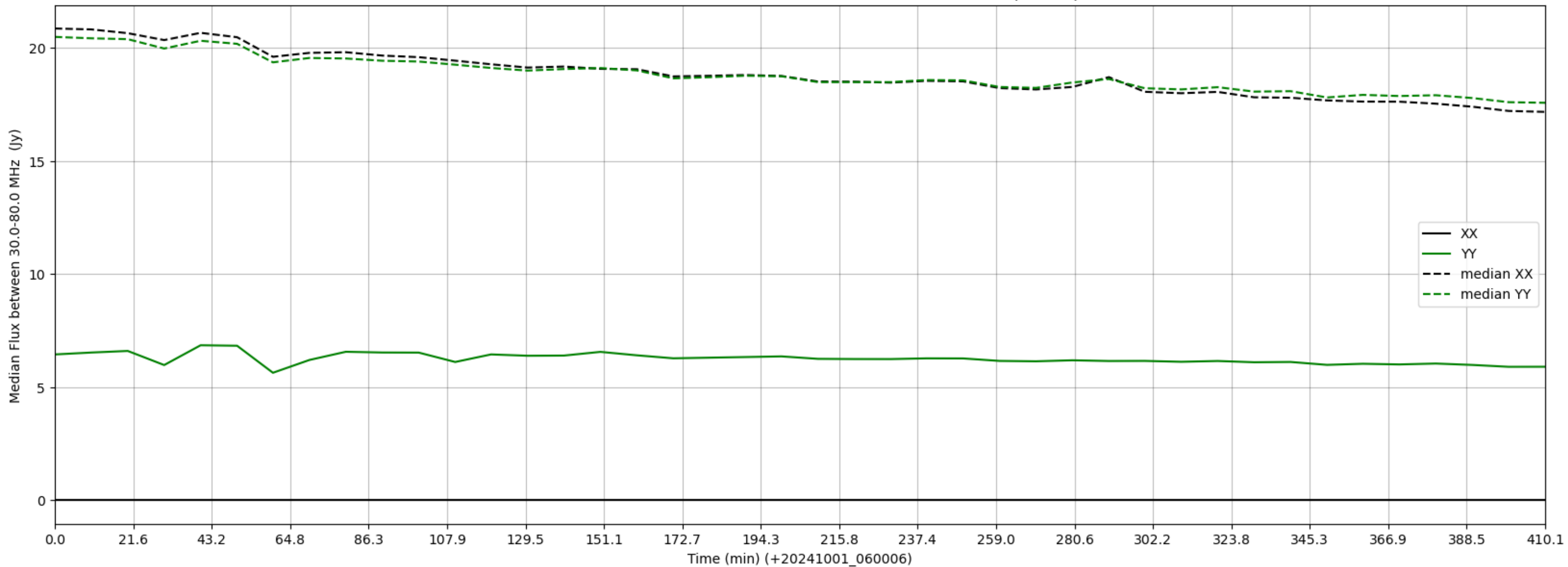
LWA209 - Correlator# 301 - XX FLAGS:LowFlux - YY FLAGS:BadSpecShape
