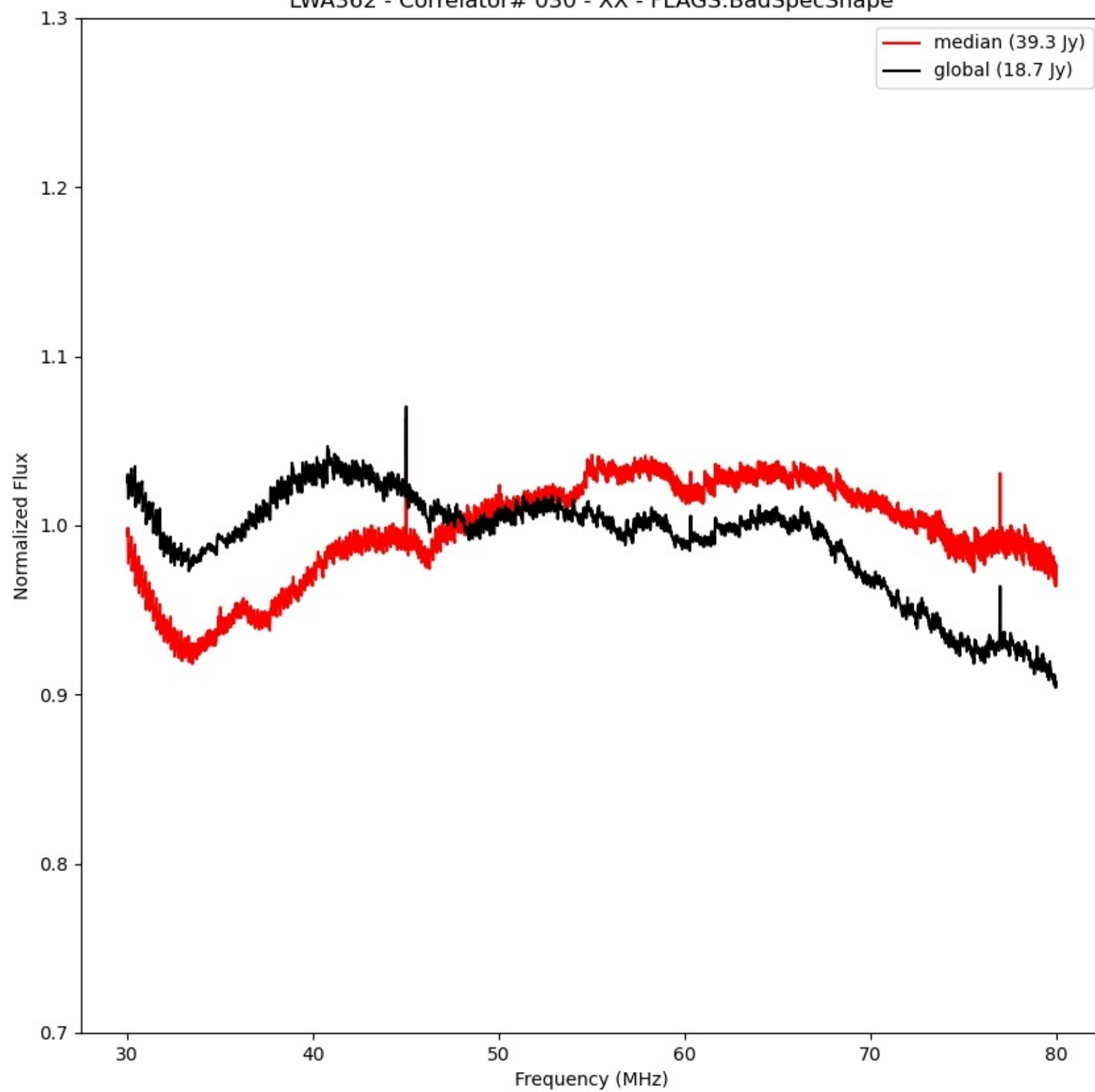
LWA362 - Correlator# 030 - XX - FLAGS:BadSpecShape
