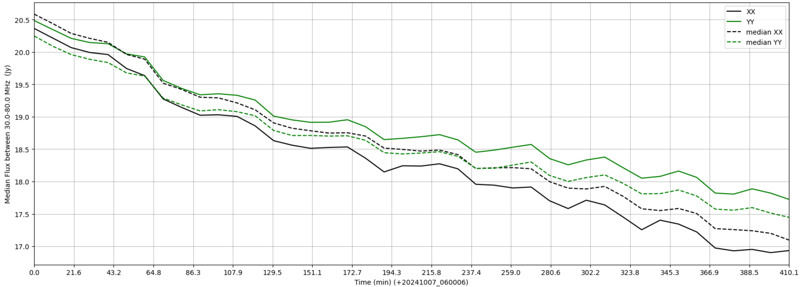
LWA001 - Correlator# 065 - XX FLAGS:BadSpecShape - YY FLAGS:Good
