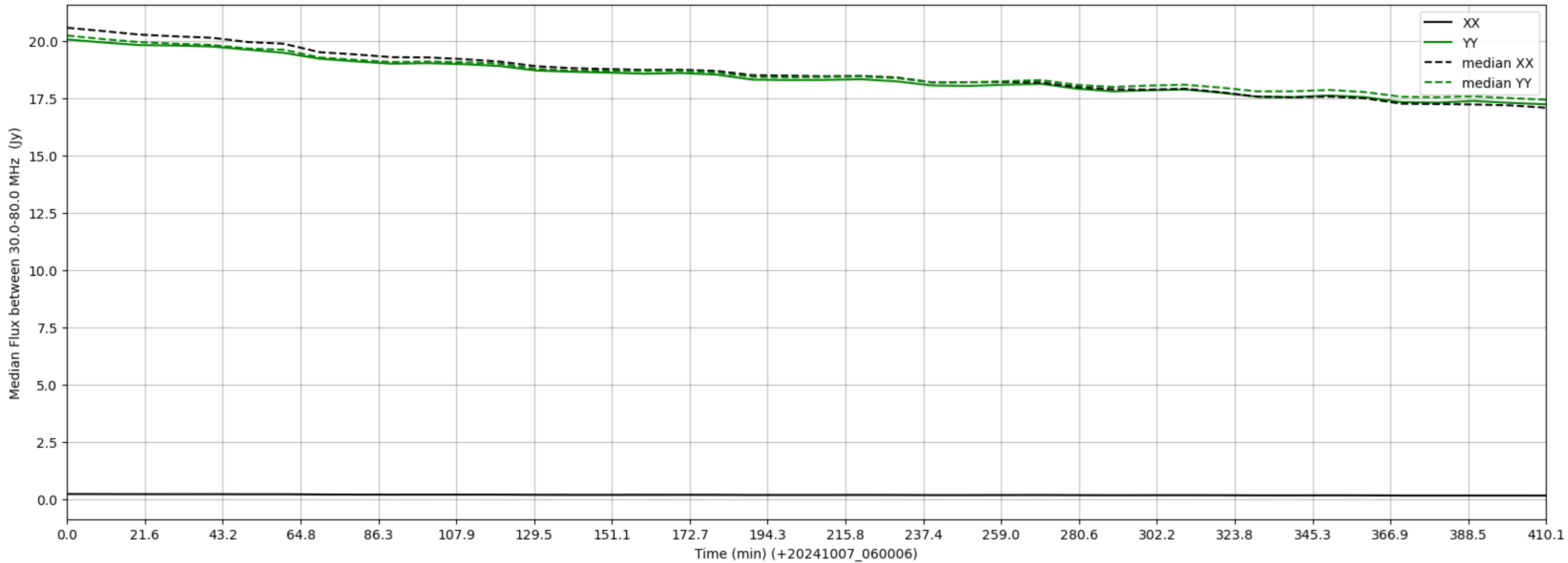
LWA215 - Correlator# 331 - XX FLAGS:LowFlux - YY FLAGS:Good
